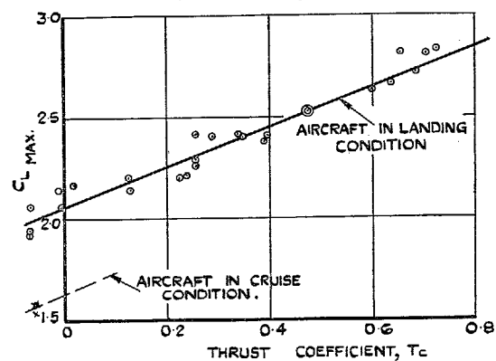
FIG. 4 (H). Effect of Engine on Stalling Speed and C_{L \max} .—Hellicat.
