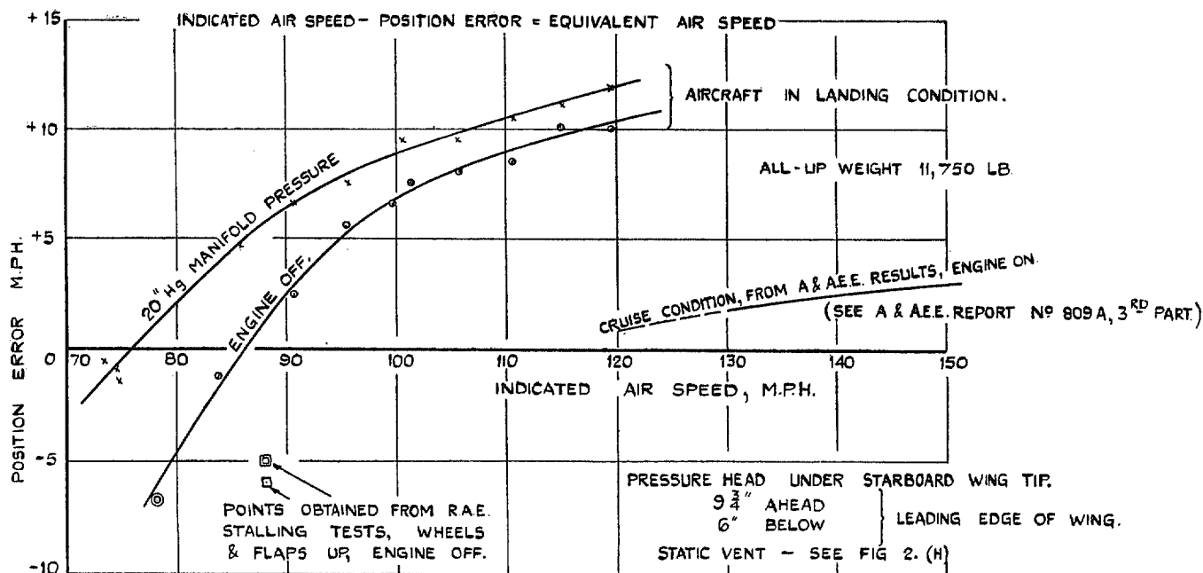
FIG. 8 (H). Position Error Curves—Hellcat.
