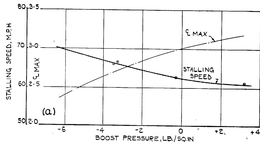
EFFECT OF ENGINE ON STALLING SPEED & C_L \text{ MAX} ALL-UP WEIGHT = 12,200 LB. AIRCRAFT IN LANDING CONDITION
