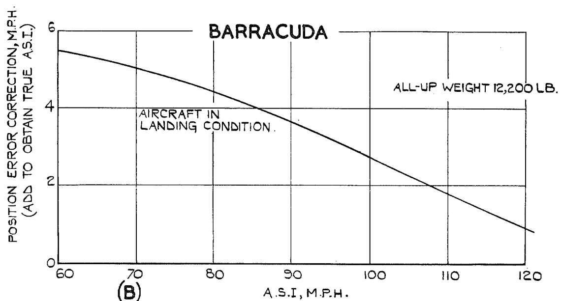
FIG. 5. Position Error Curves.
