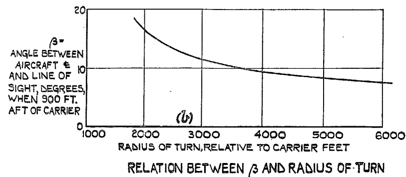
FIG. 9. Improvement in View Due to Use of Curved Approach Path.
