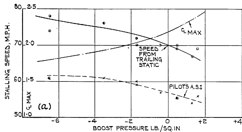
EFFECT OF ENGINE ON STALLING SPEED & C_L \text{ MAX} ALL-UP WEIGHT = 6600 LB. AIRCRAFT IN LANDING CONDITION
