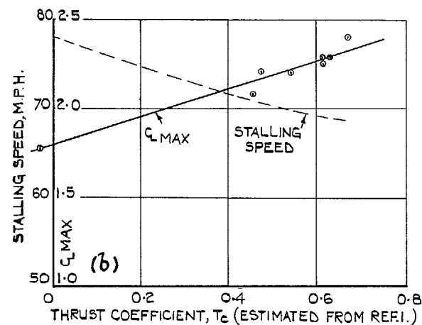
EFFECT OF ENGINE ON STALLING SPEED & C_L \text{ MAX} . ALL-UP WEIGHT = 6600 LB. AIRCRAFT IN LANDING CONDITION FIG. 2 (S). Stalling Speed and C_L \text{ max} .—Seafire MB.125.
