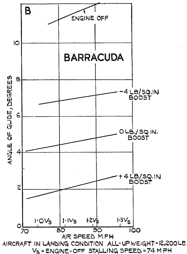
FIG. 3. Effect of Engine on Gliding Angle.
