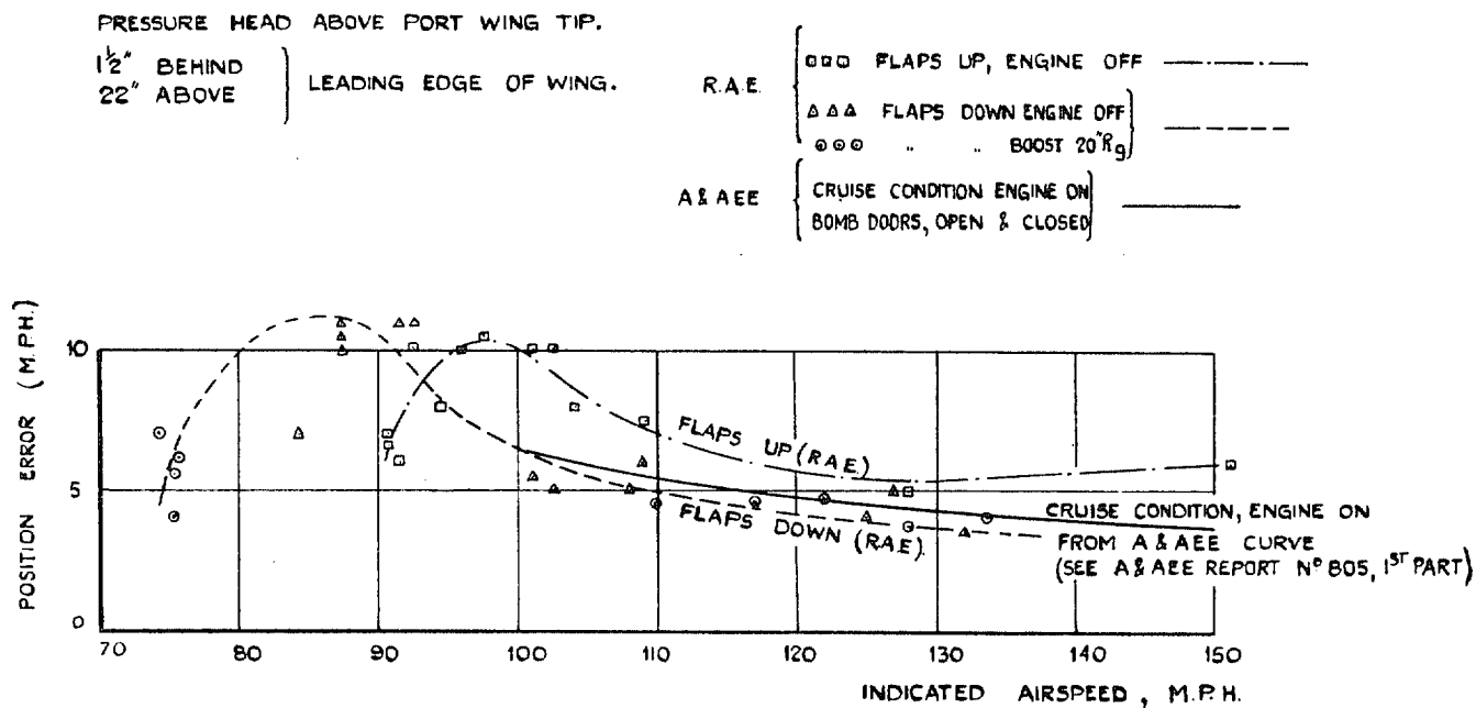
FIG. 8 (A). Position Error Curves.
