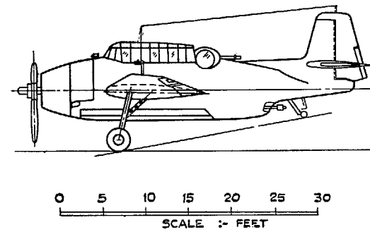
FIG. 1 (A). General Arrangement of Avenger I.
