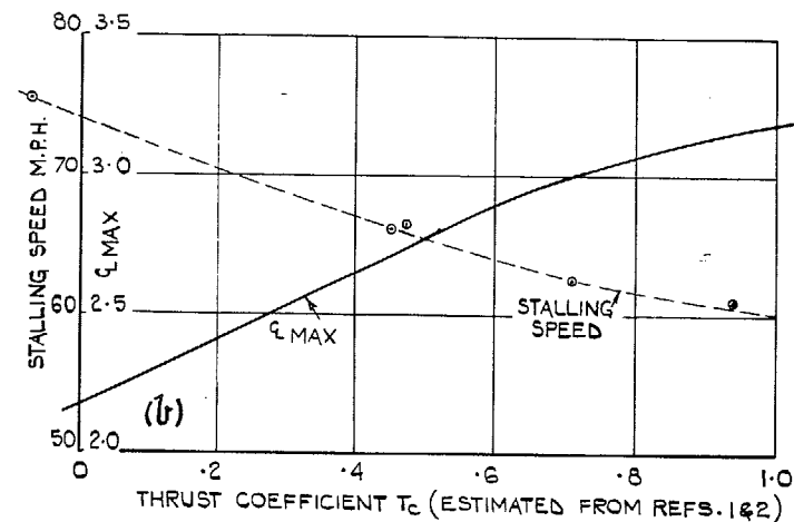
EFFECT OF ENGINE ON STALLING SPEED & C_L \text{ MAX} ALL-UP WEIGHT = 12,200 LB. AIRCRAFT IN LANDING CONDITION. FIG. 2 (B). Stalling Speed and C_L \text{ max} .—Barracuda LS.540.
