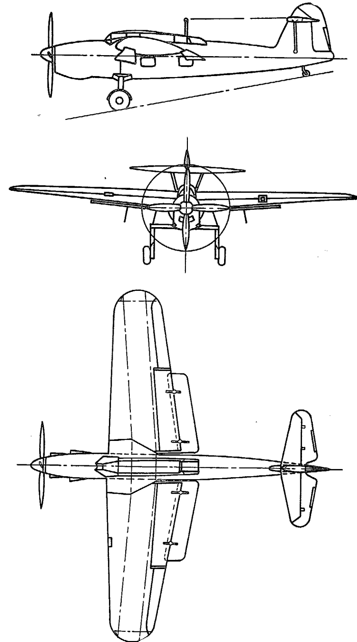
FIG. 1 (B). General Arrangement of Barracuda.
