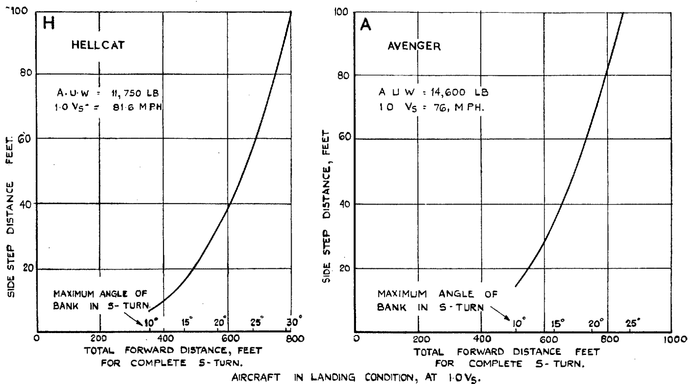
FIG. 10. Estimated Sidestep Distances for Hellcat and Avenger.
