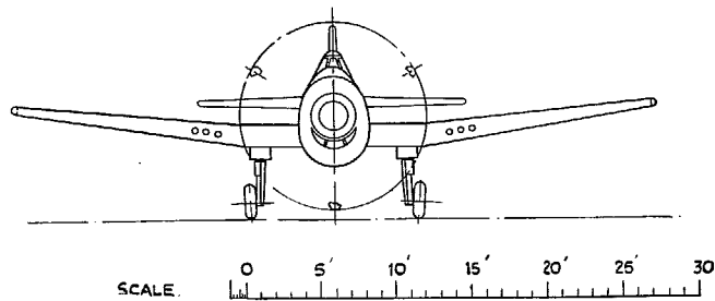
FIG. 1 (H). General Arrangement of Hellcat I.
