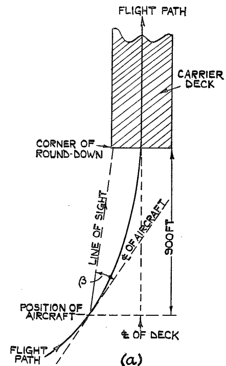
FIG. 9. SIMPLE DIAGRAM SHEWING EFFECT OF CURVED APPROACH PATH ON VIEW FROM COCKPIT
