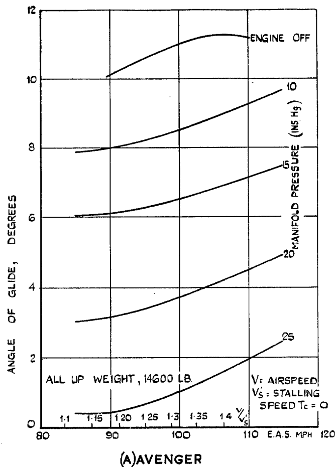
FIG. 5. Effect of Engine on Gliding Angle.
