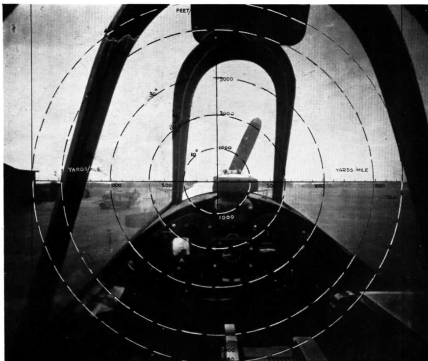
Photograph A. Camera position corresponding to pilot's left eye when seated with head central, seat fully up. Centre of graticule corresponds to a direction of sight inclined down at 10.3^\circ to wing chord.
