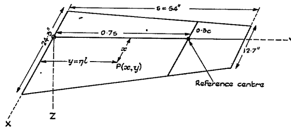
FIG. 5.—Wing Dimensions.
