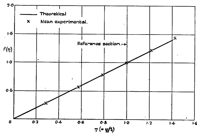
FIG. 6.—Flexural Mode.
