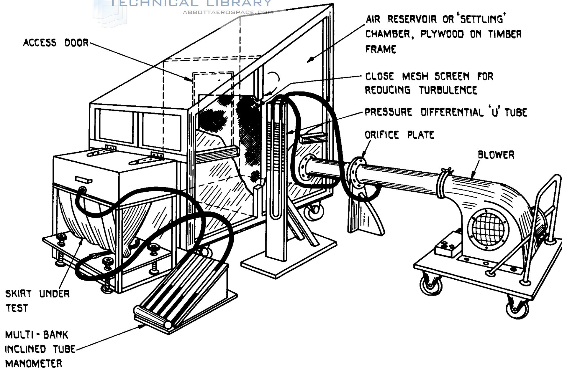
FIG.1(b) TEST RIG FOR FLEXIBLE SKIRTS
