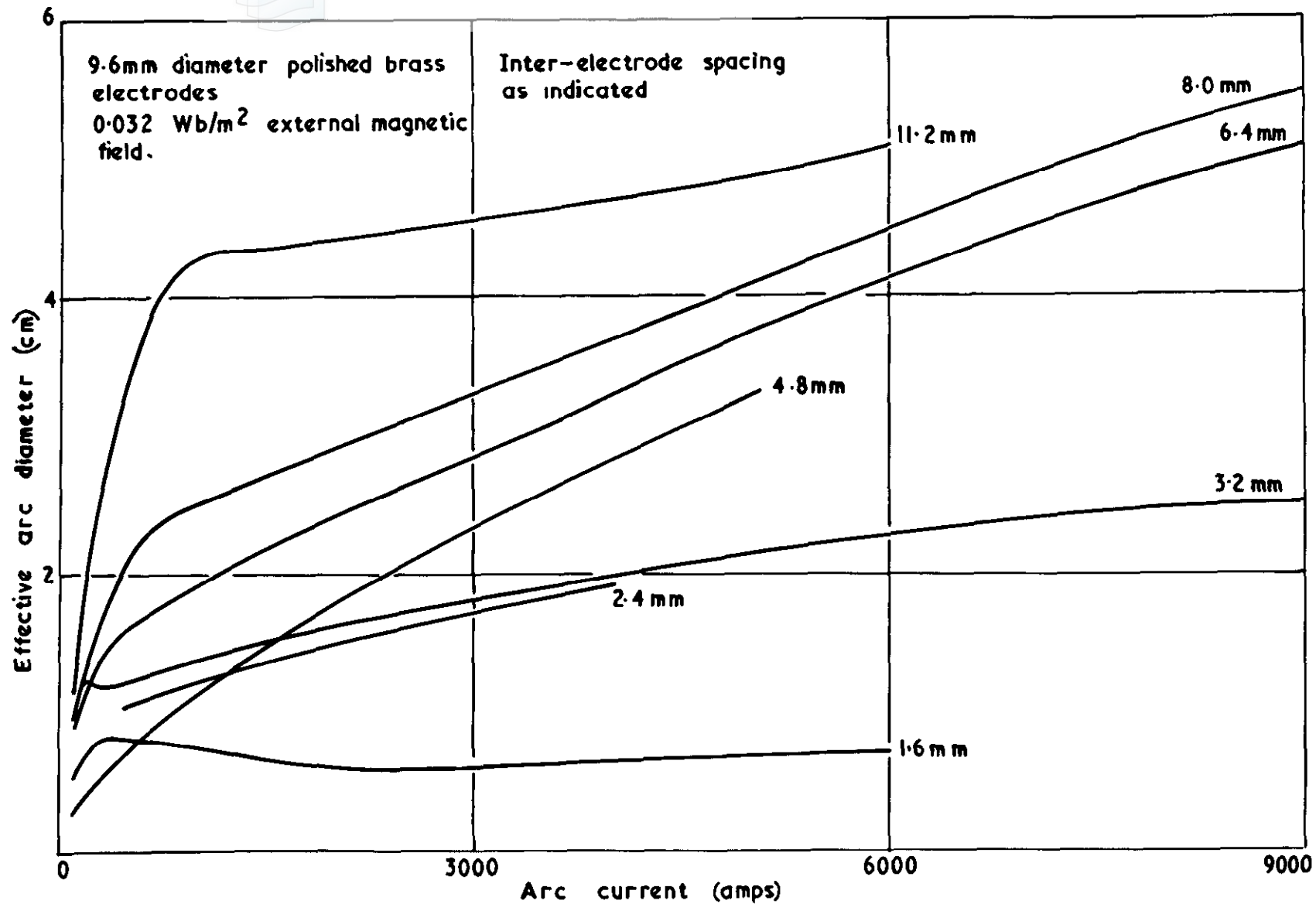
Effective arc diameter as a function of arc current
