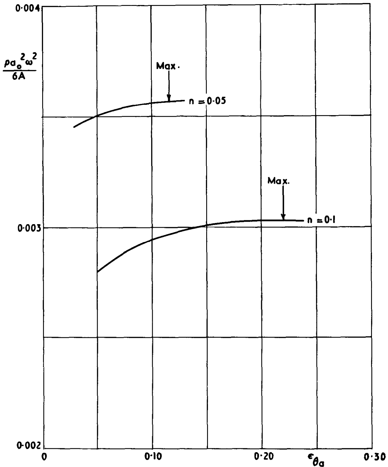
FIG.2. Variation of \rho a_o^2 \omega^2 / 6A with circumferential strain at bore, \epsilon_{\theta_a} ; \alpha^\circ = 10 .
