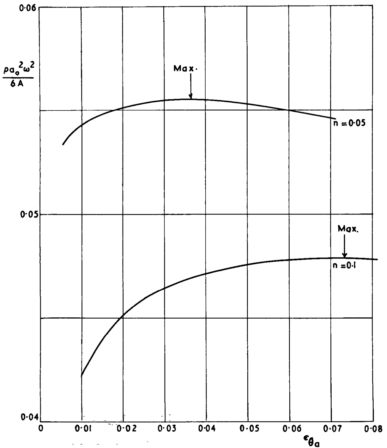
FIG.1. Variation of \frac{\rho a_o^2 \omega^2}{6A} with circumferential strain at bore, \epsilon_{\theta a} : \alpha^o = 2.
