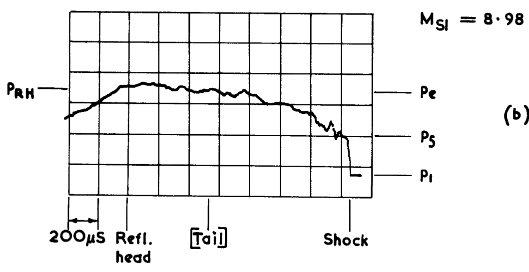
Pressure records with nozzle designed for M_{Sl} = 8.8 , M_3 = 3.06
