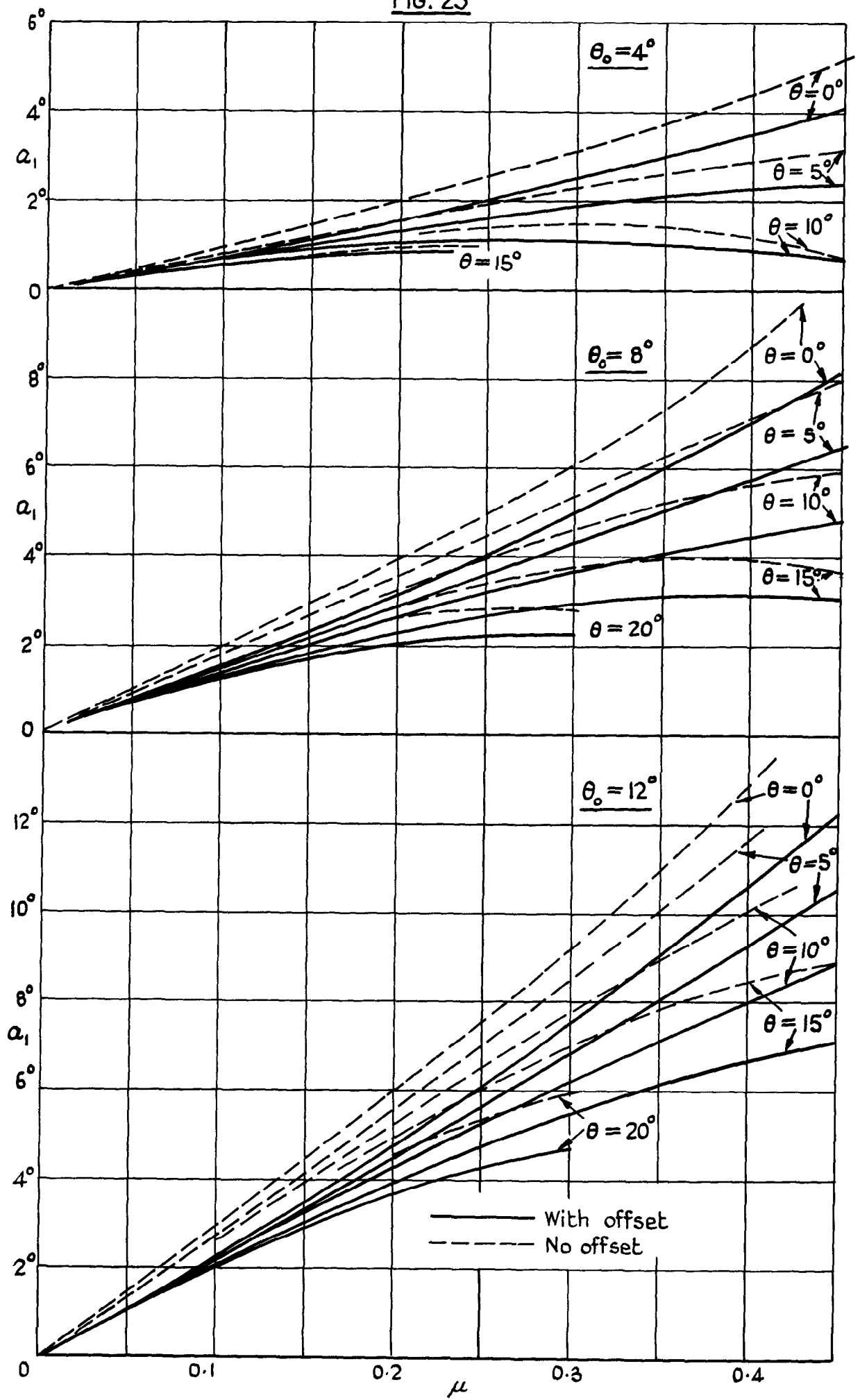
Theoretical flapping angles (with and without offset)
