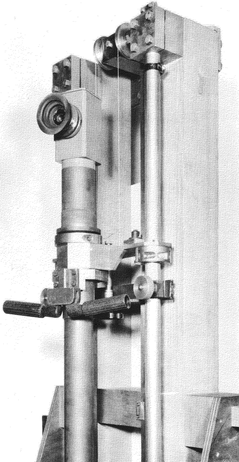
Head of periscope.
