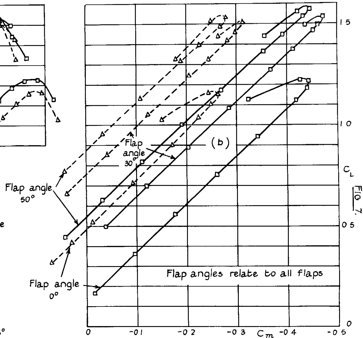
Effect of flaps with large tail.
