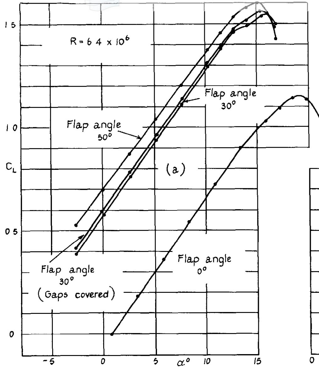
Vickers M.T. 1000 (C 132 D) Effect of flaps without tail.
