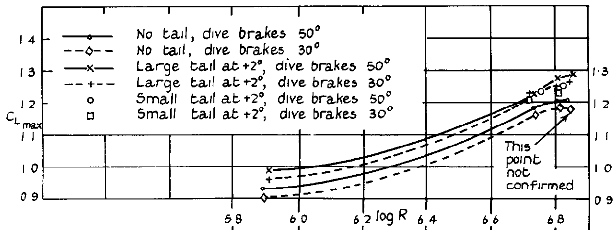
(b) Effect of dive brakes on C_{Lmax}
