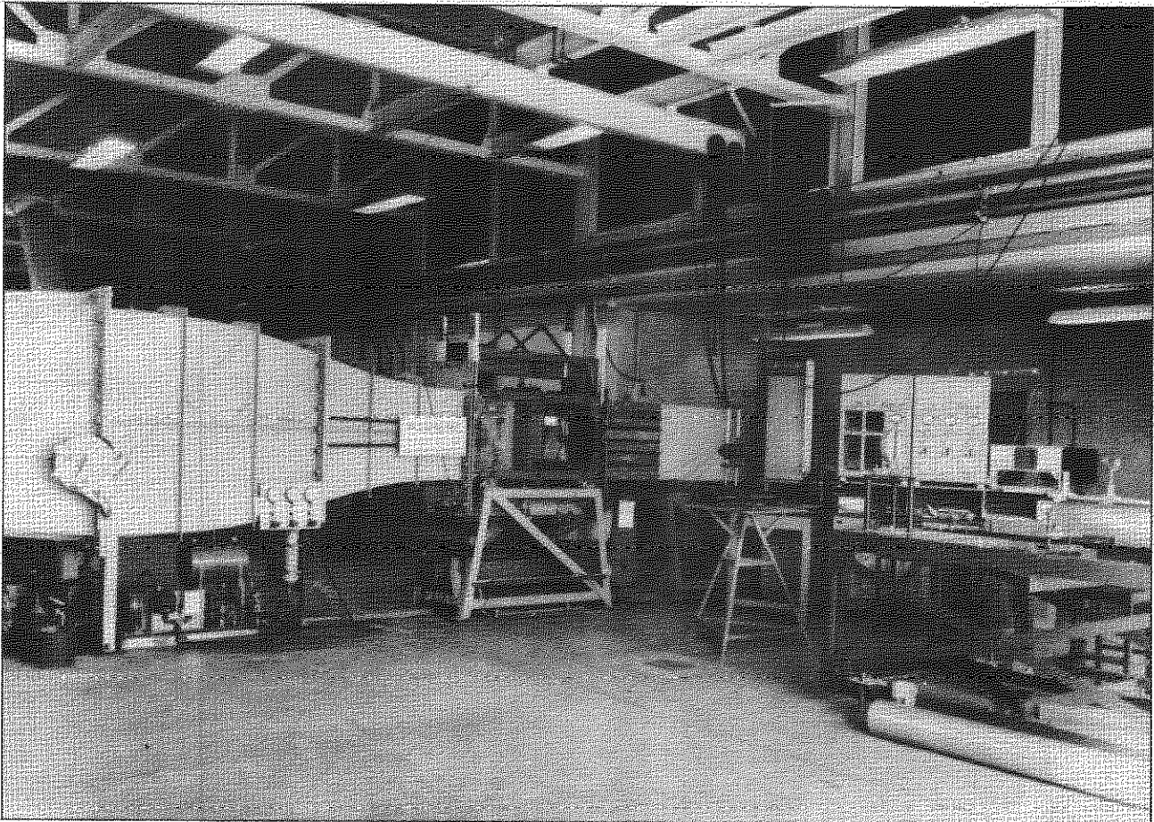
FIG.10. 15 inch x 16 inch WIND TUNNEL
