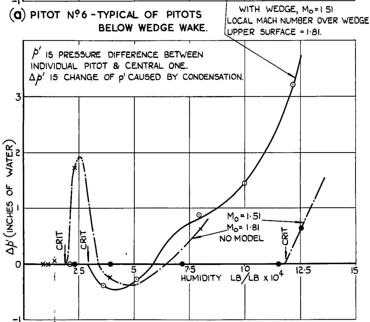
FIG.8(a&b) VARIATION OF PITOT PRESSURE WITH HUMIDITY WITH & WITHOUT MODEL.
