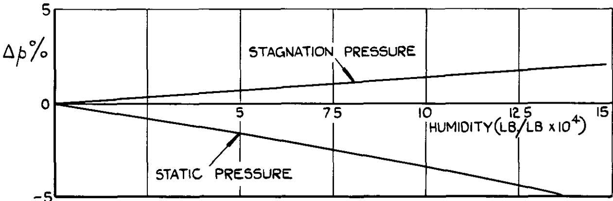
(b) DROP IN STATIC & STAGNATION PRESSURE, \Delta p\%
