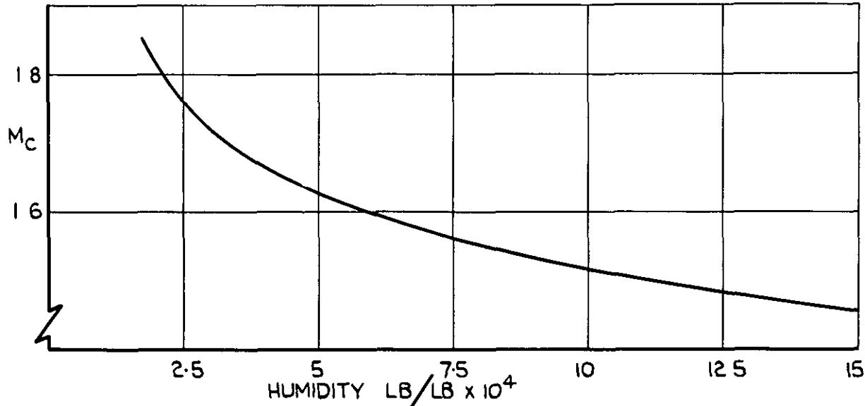
(a) MACH NUMBER, M_c , AT CONDENSATION SHOCK. (FROM FIGURE 4.)
