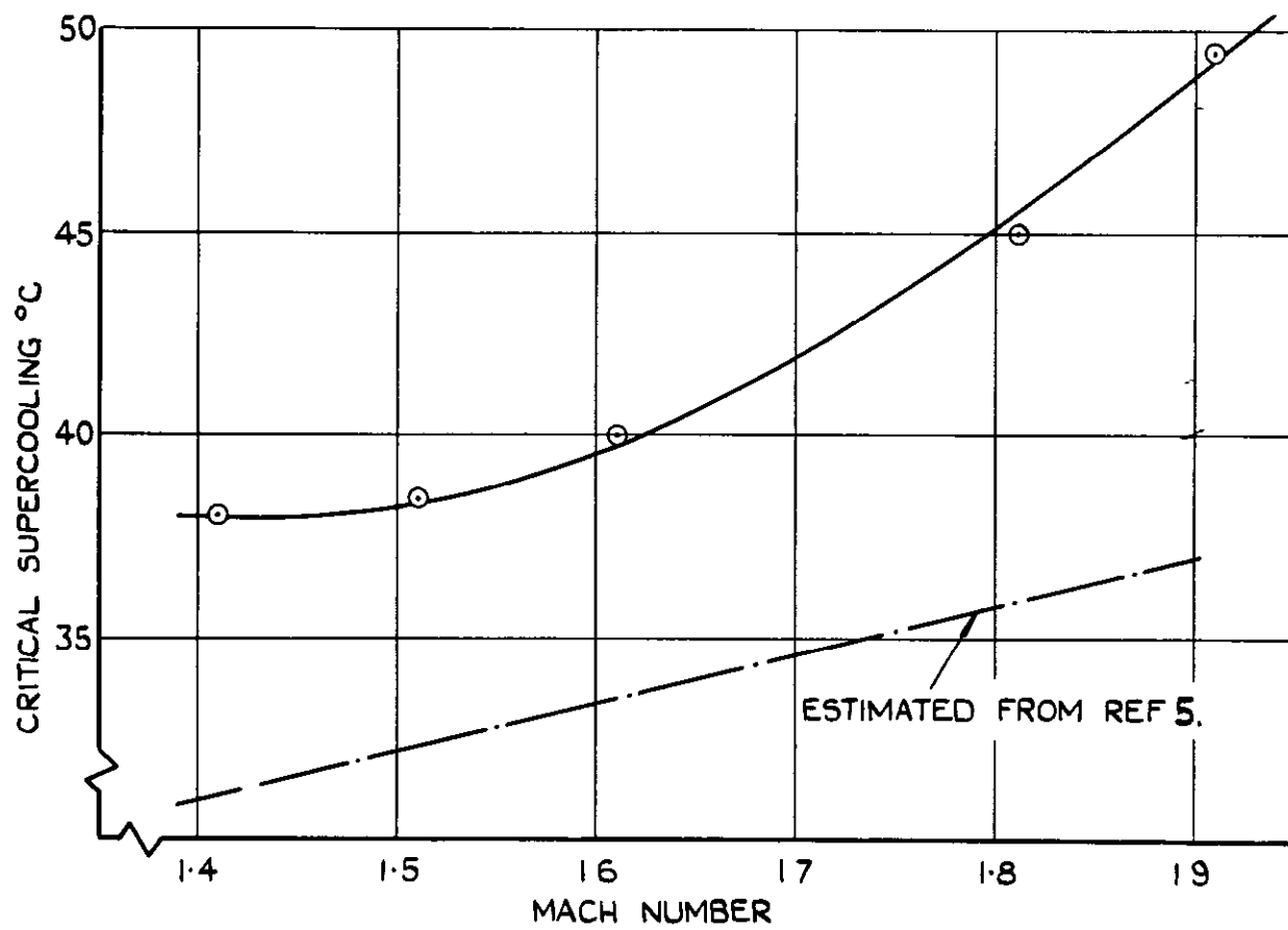
FIG.4. CRITICAL SUPERCOOLING AGAINST MACH NUMBER.
