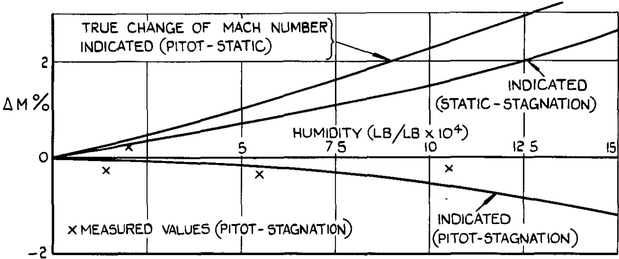
(c) DROP IN MACH NUMBER, \Delta M\%
