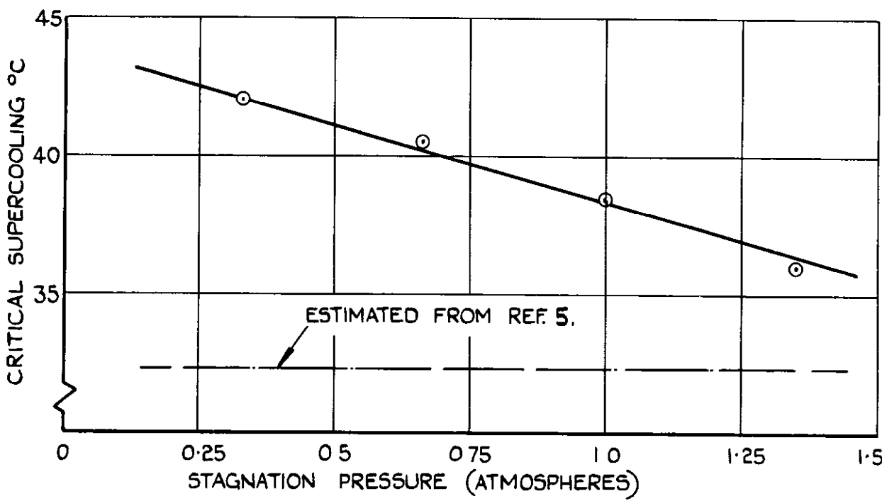
FIG.5. CRITICAL SUPERCOOLING AGAINST STAGNATION PRESSURE.
