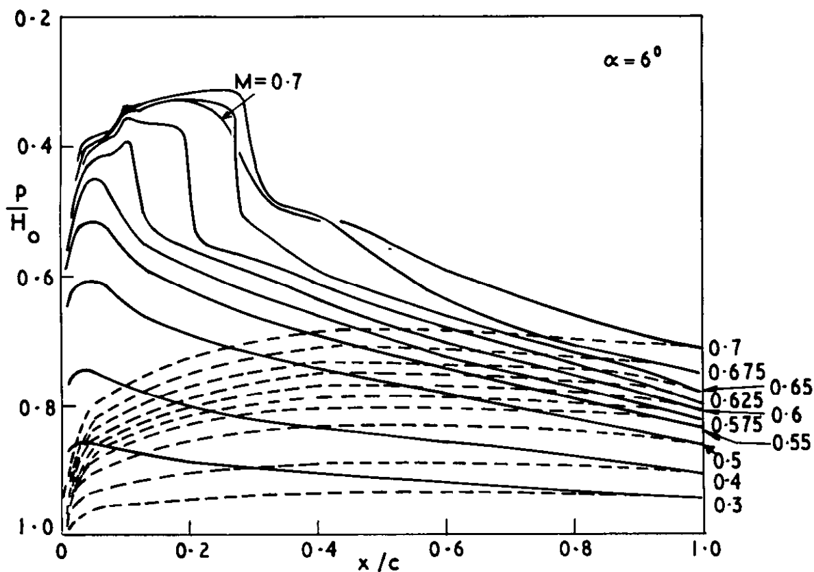
i NPL 9615 Pressure distributions, \alpha = 6^\circ
