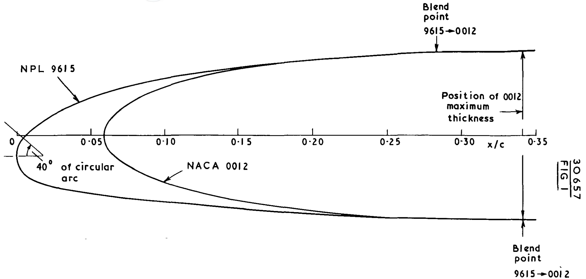
Comparison of profiles ahead of position of maximum thickness
