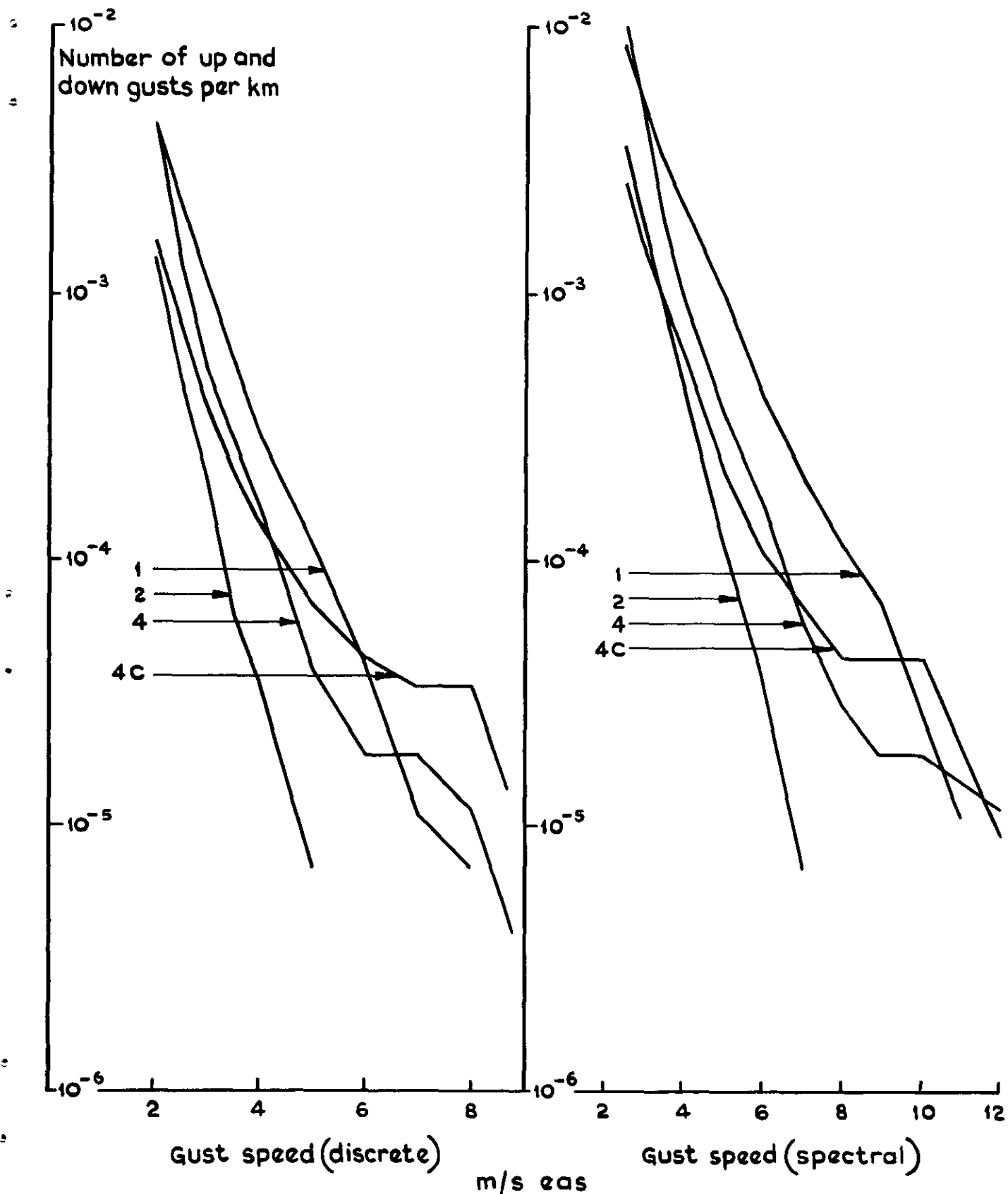
Fig. 7 Gusts encountered by each Comet fleet during climb and descent between 17750 ft and 29750 ft
