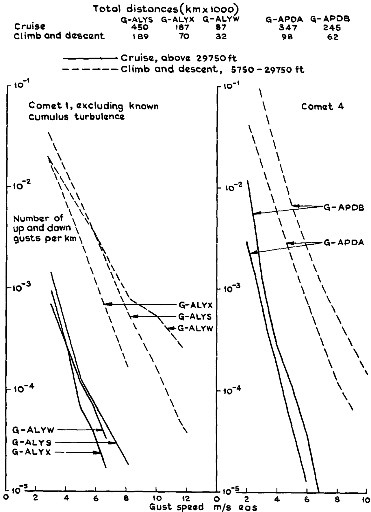
Fig.12 Gusts recorded on individual aircraft spectral gust response factor
