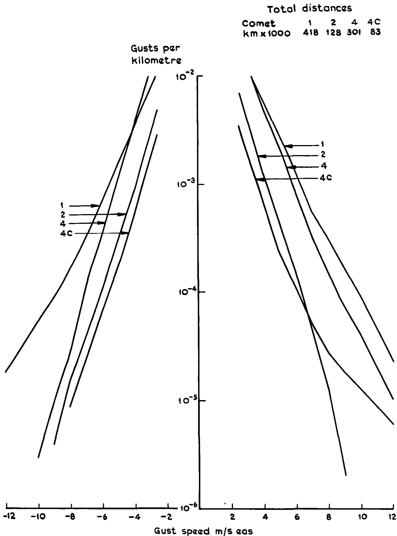
Fig.4 Gusts encountered by each Comet fleet during climb and descent at all altitudes. Spectral gust response factors
