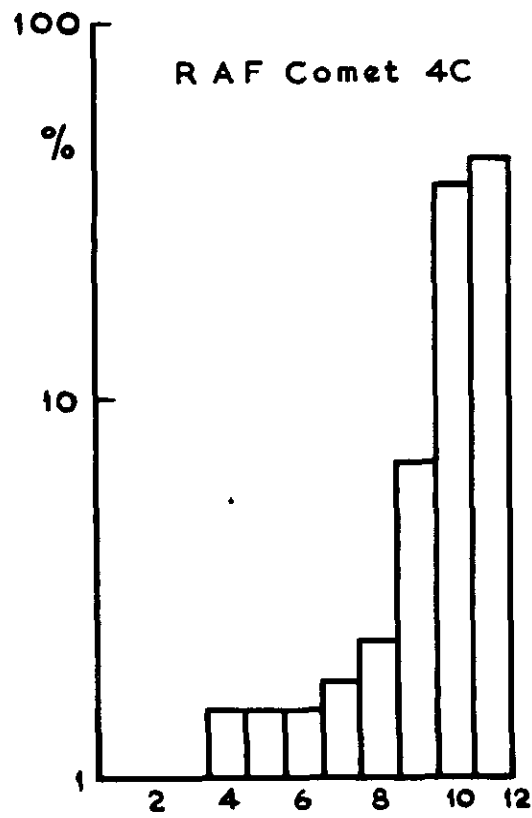
Fig.1 Distance flown in each altitude band, as a percentage of the total distance, (climb, cruise and descent)
