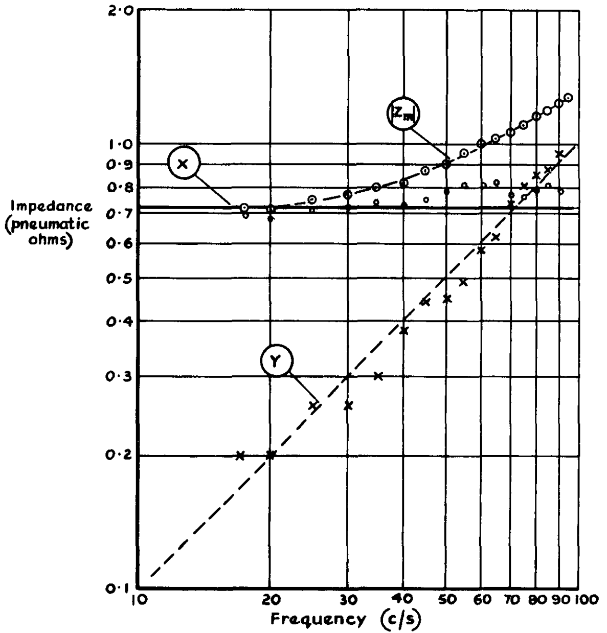
Fig.3 Impedance of Fleisch flowhead
