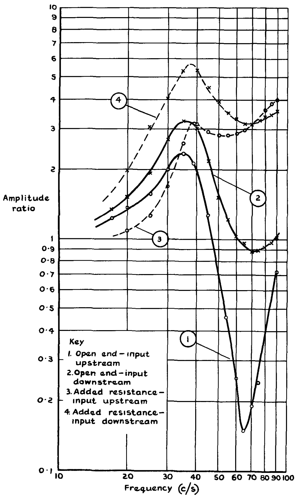
Fig.5 Sensitivity with asymmetric transducer
