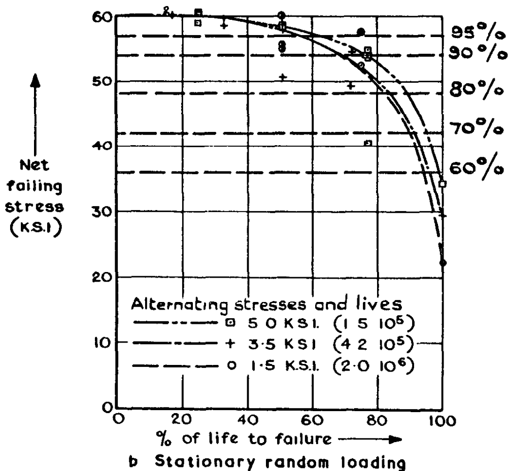
Fig.10a&b Partial damage tests-16 K.S.I.mean small D.T.D 5014 lugs
