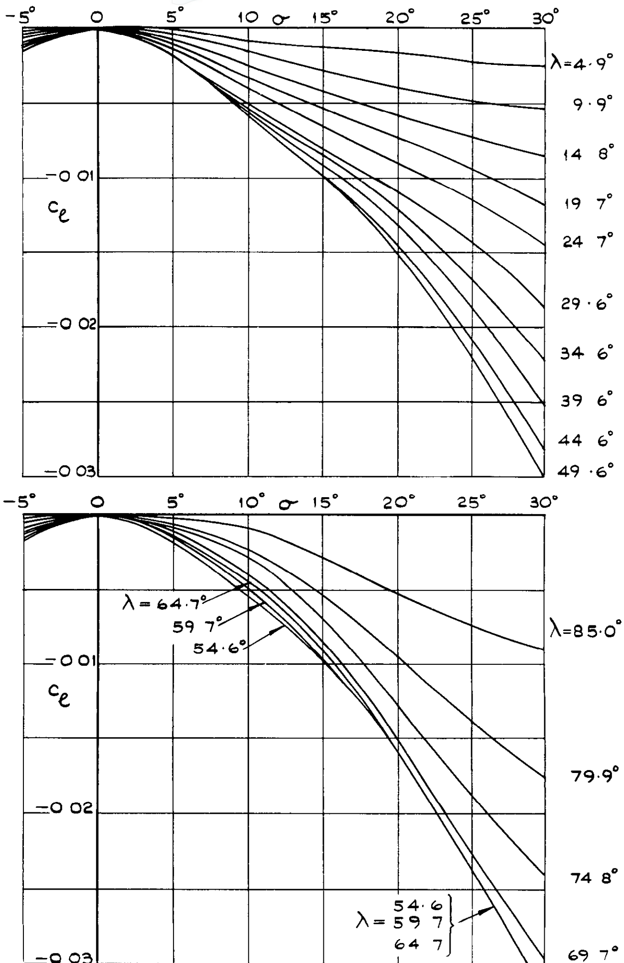
FIG.27 (a) C_l v \sigma FOR W_2
