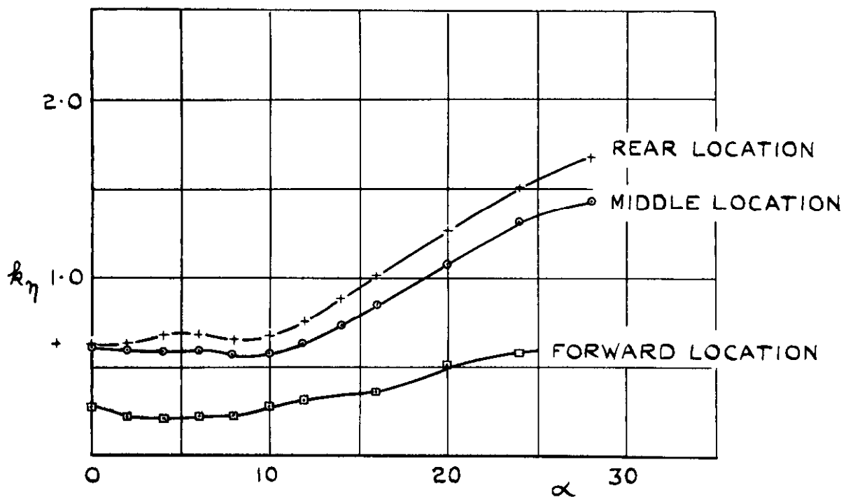
FIG.19 (a) CONTROL EFFECTIVENESS
