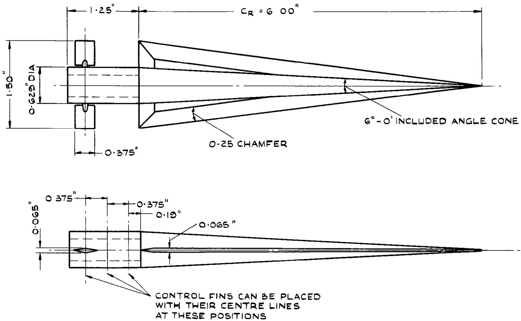
FIG. 1 DRAWING OF MODEL w_2
