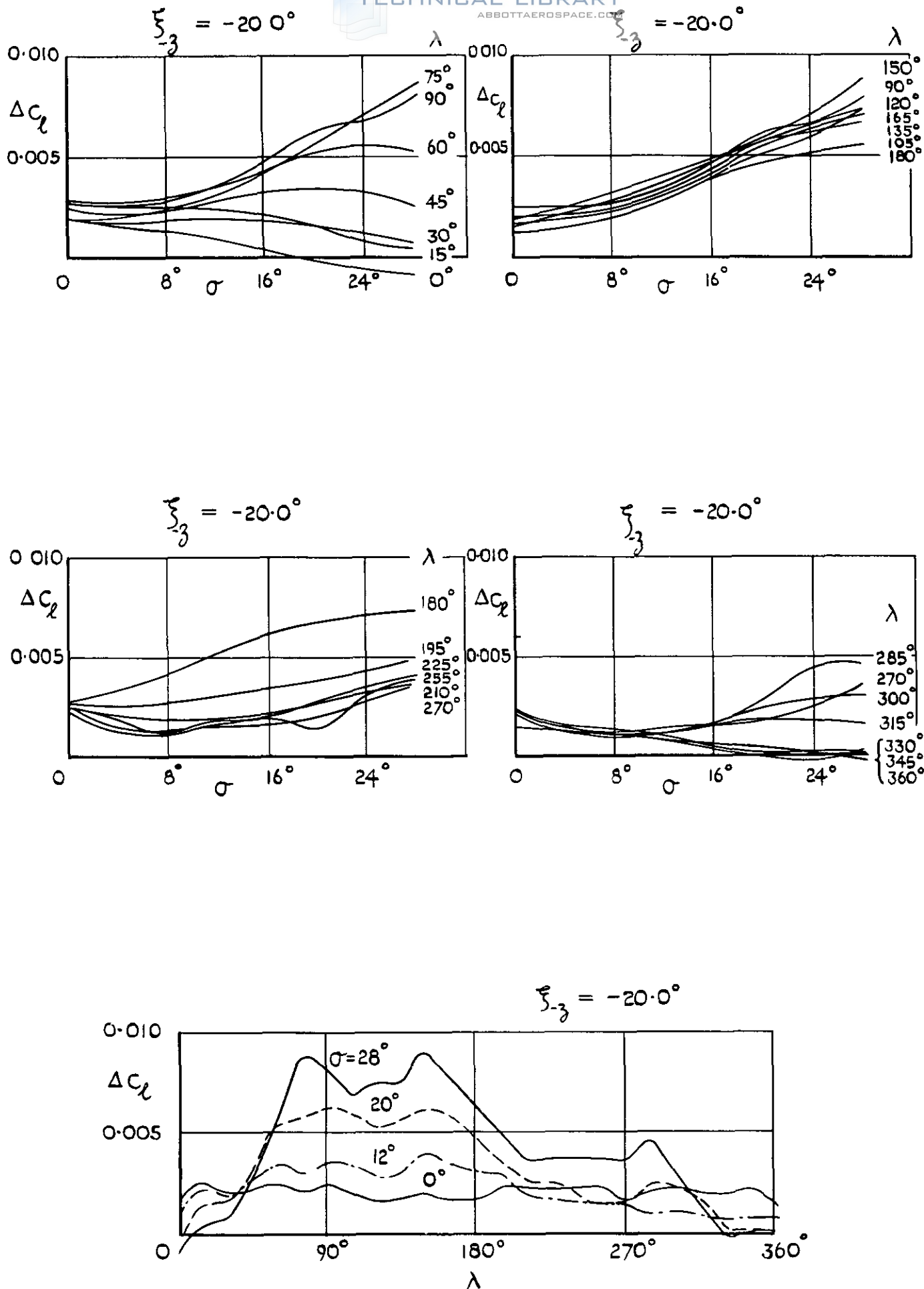
FIG. 32 INCREMENT IN C_l DUE TO MOVEMENT OF ONE CONTROL PANEL ON W_4, BC^F
