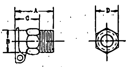
HINGED LID OIL CUP MATERIAL - BRASS & STEEL
