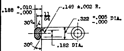
AN276-3 BEARING (BRONZE)
