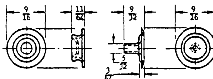
(A) EYELET
