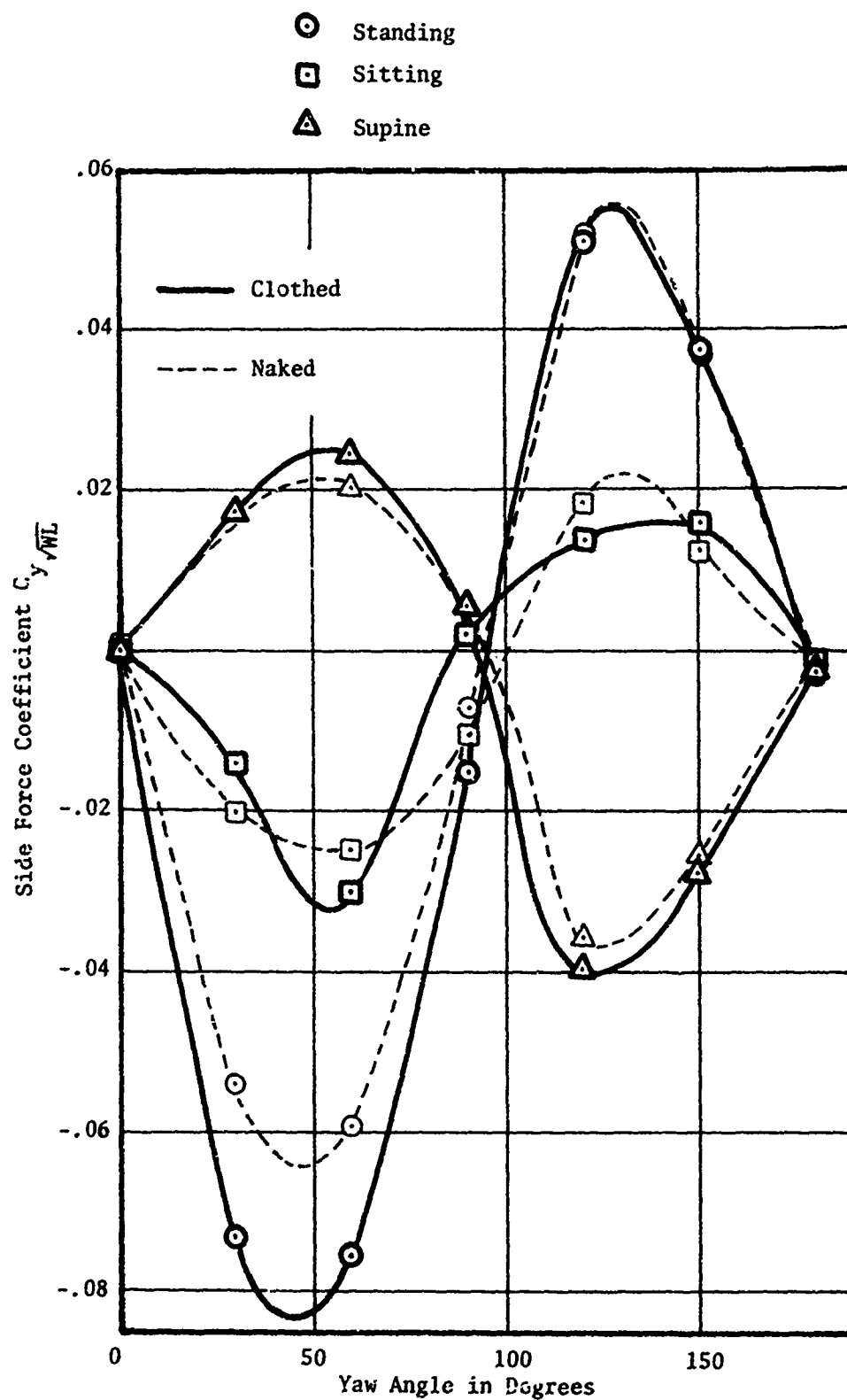
Figure 7. Mean Side Force of Fourteen Clothed and Naked Subjects as a Function of Yaw Angle. C_{y\sqrt{WL}} = Y/q_0\sqrt{WL} Where W = Subject Weight and L = Subject Height
