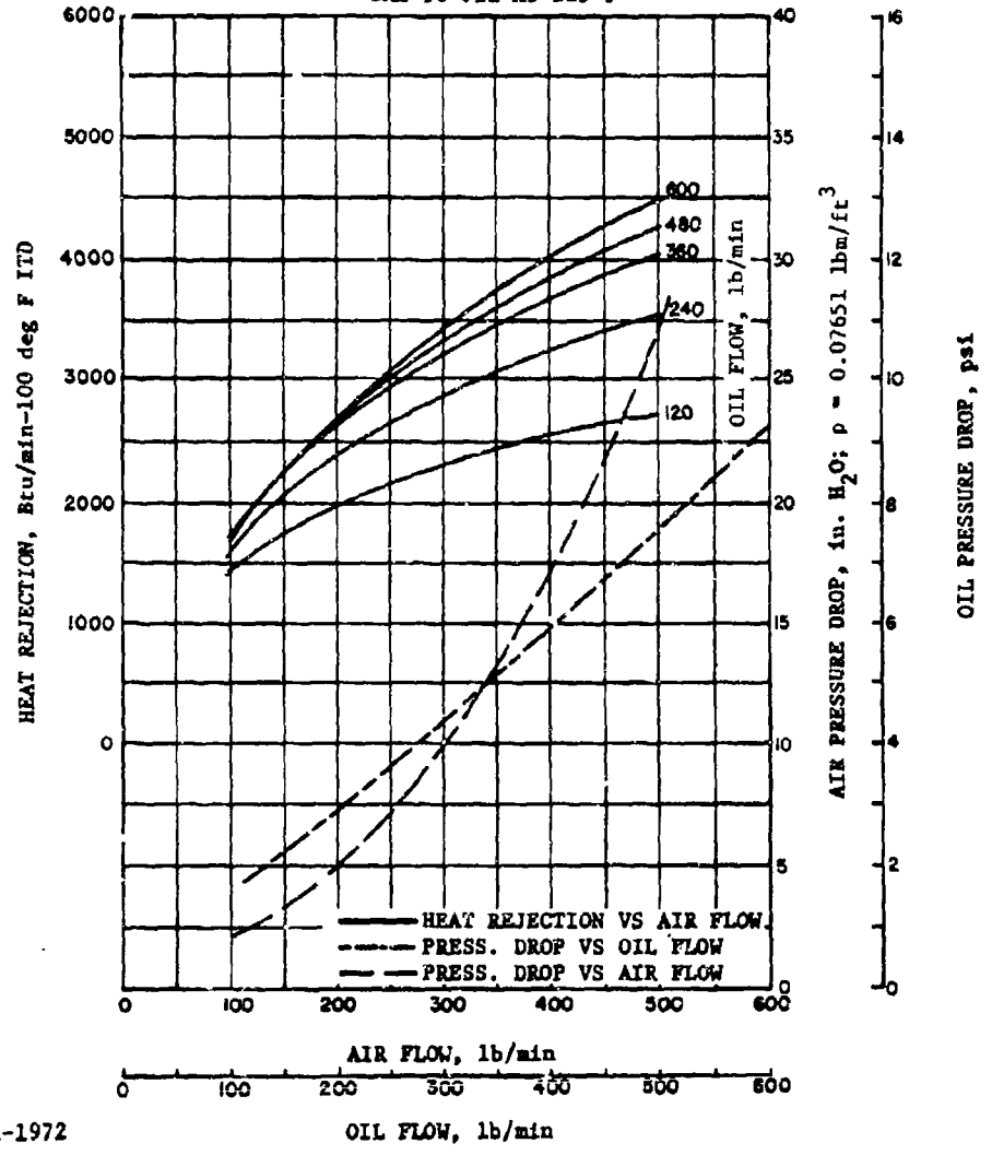
Figure A-11. 14 Fins/in., Core Depth 4.5 in., Oil Cooler Performance, I
