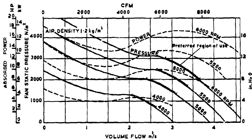
Figure B-30. Mixed Flow Fan Performance, Model 305 MP3 311 (Courtesy of Airscrew Hawden Ltd., Weybridge, Surrey, England)
