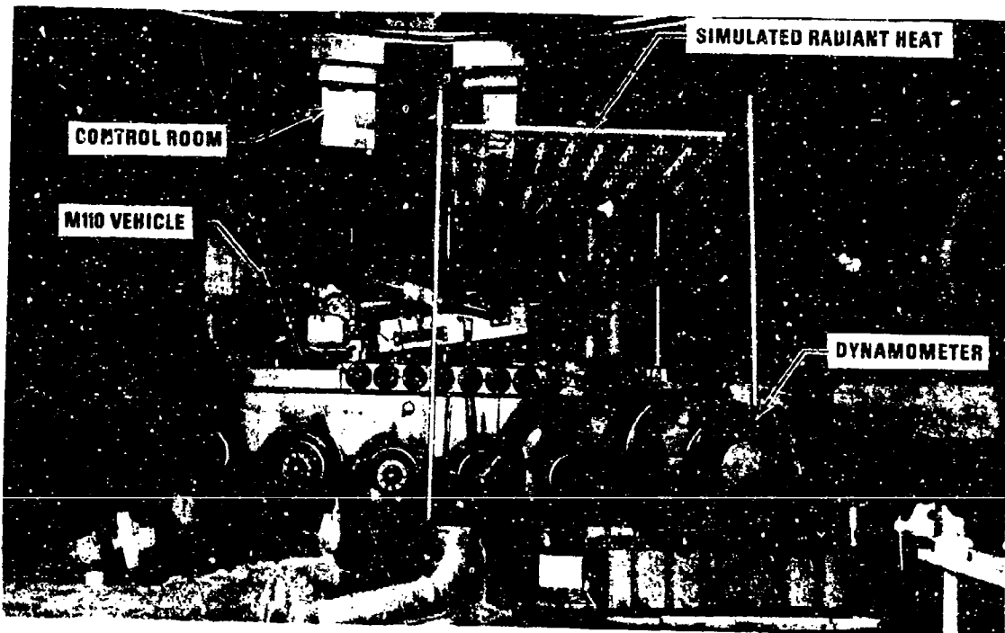
Figure 9-8. M110 Vehicle Cooling Test Installation (USATACOM)
