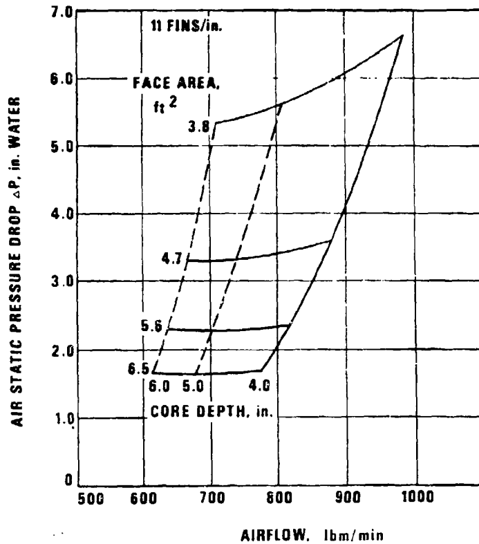
Figure 3-21. Radiator Core Performance Characteristics, 11 Fins/in. (Courtesy of Harrison Radiator Division-GMC)
