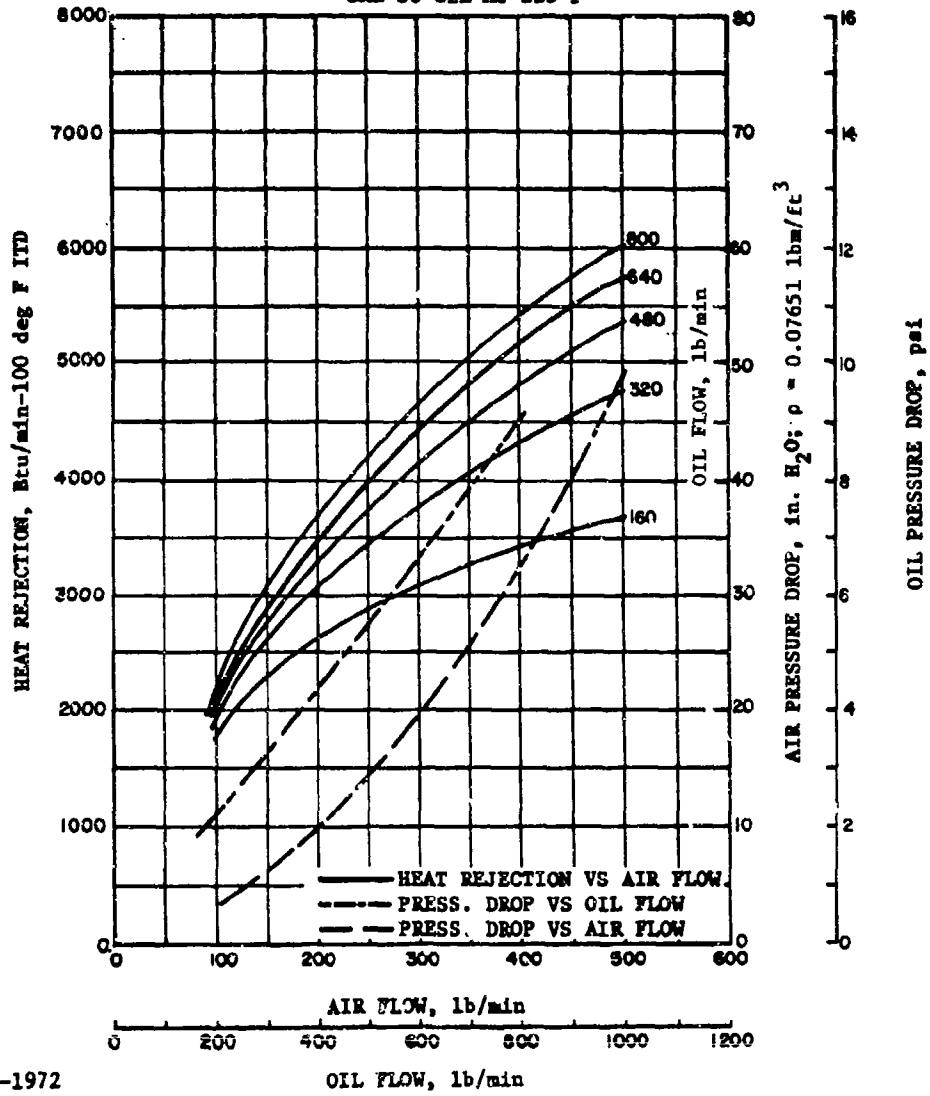
Figure A-16. 18 Fins/in., Core Depth 6 in., Oil Cooler Performance, I
