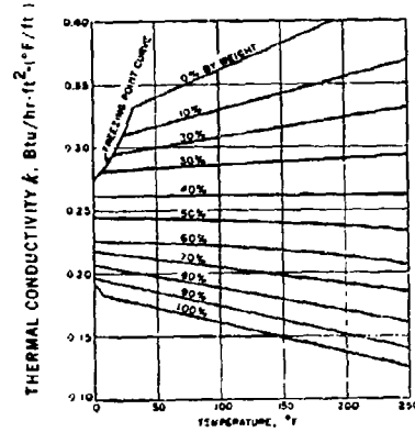
(B) THERMAL CONDUCTIVITY OF AQUEOUS SOLUTIONS OF ETHYLENE GLYCOL
