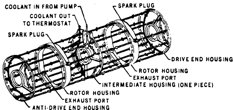
Figure 2-23. Schematic Diagram of Housing Cooling System for Curtiss-Wright Wankel Engine RC2-60-U5 (Ref. 36) (Release Granted by Society of Automotive Engineers, Inc., Paper No. 720468.)
