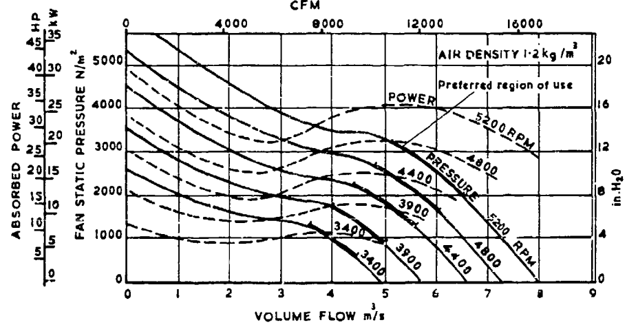
Figure B-31. Mixed Flow Fan Performance, Model 380 MP3 311 (Courtesy of Airscrew Howden Ltd., Weybridge, Surrey, England)
