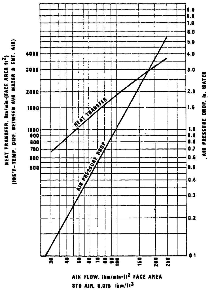
Figure A-39. 11 Fins/in. Radiator Core Performance Characteristics (Courtesy of Young Radiator Company)
