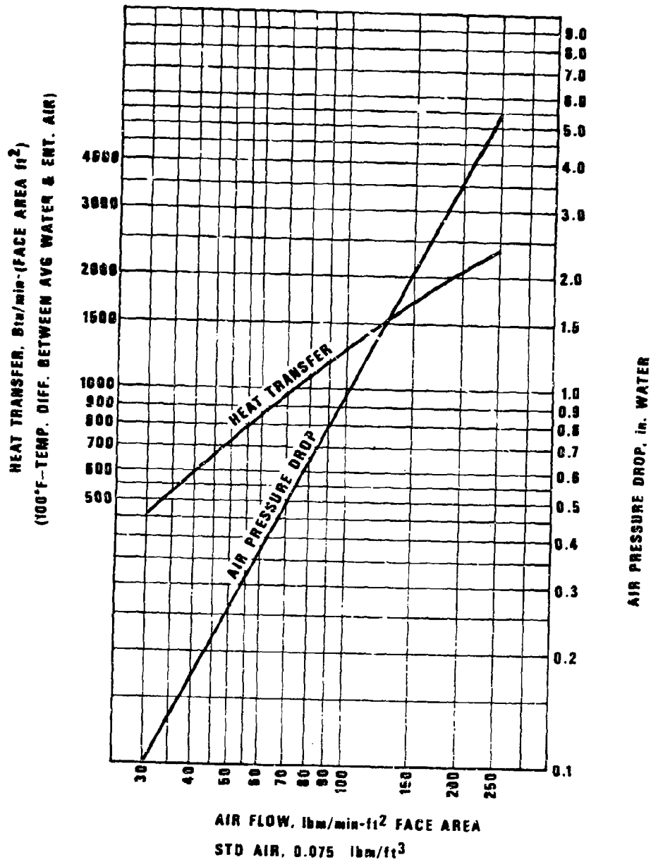
Figure A-41. 8 Fins/in. Radiator Core Performance Characteristics (Courtesy of Young Radiator Company)
