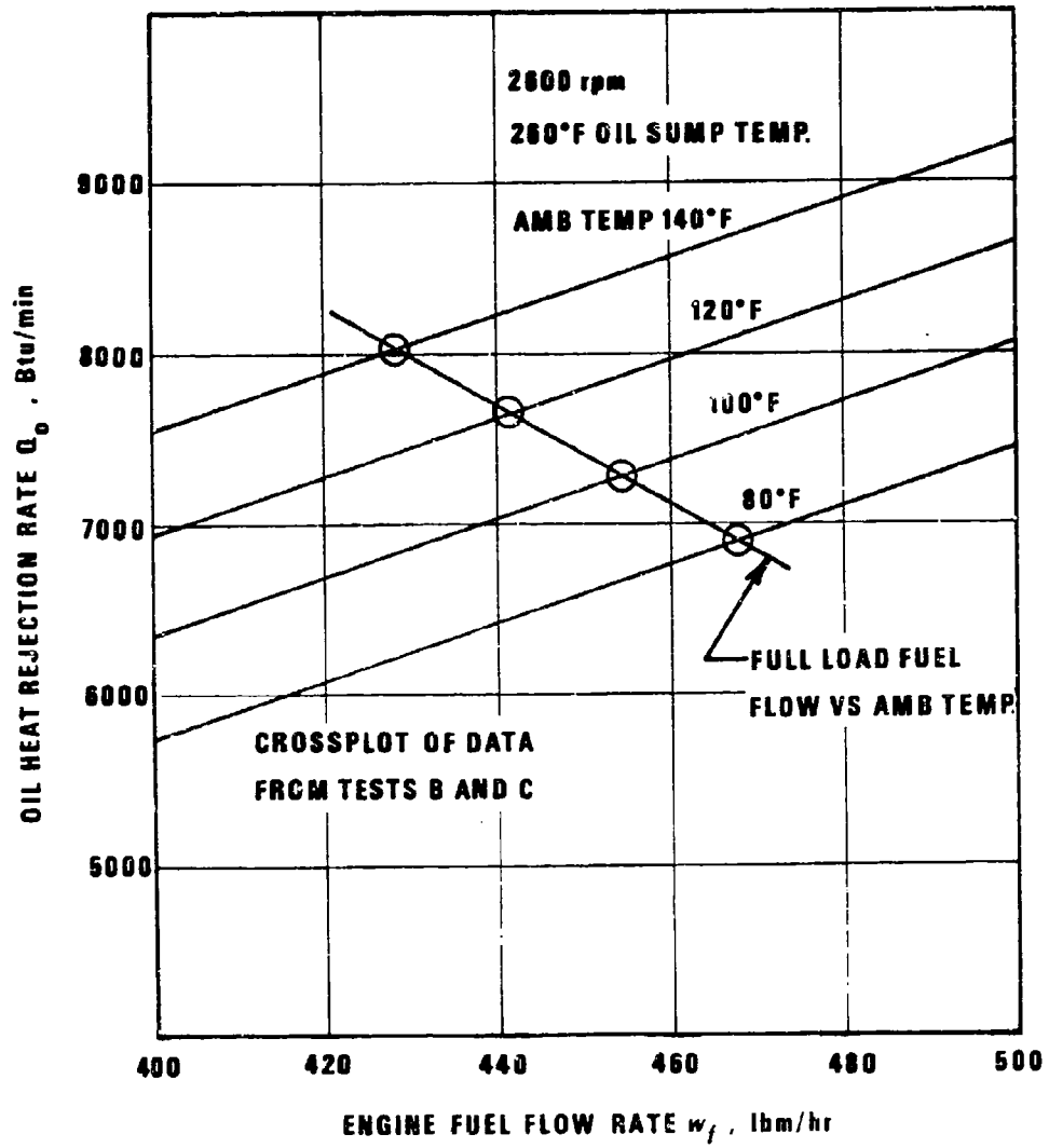
Figure 8-25. AVCR-1100-38 Engine Oil Heat Rejection vs Fuel Flow
