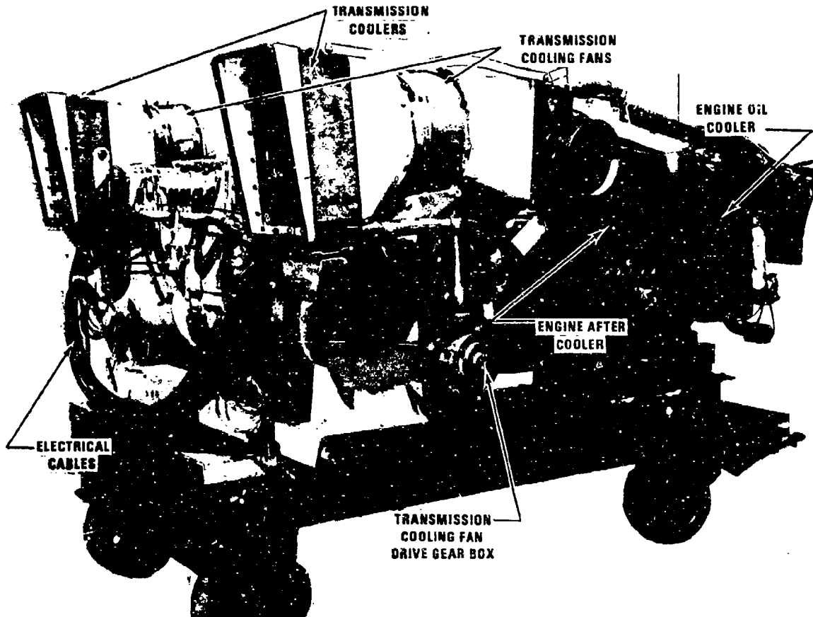
Figure 1-44. XM803 Experimental Tank Power Plant Test Run and Stall Check—Power Plant Removed (USATACOM)
