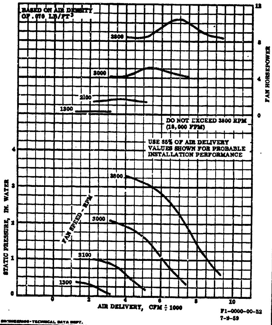
Figure B-34. Cooling Fan Performance Curve No. F1-0000-00-52
