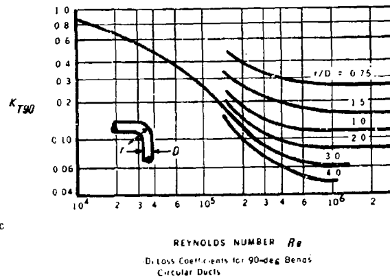
Figure 7-6. Loss Coefficient for 90-deg Constant Area Bends With Following Ducts (Ref. 3) (Reprinted with permission, Copyright © Society of Automotive Engineers, Inc. All rights reserved.)
