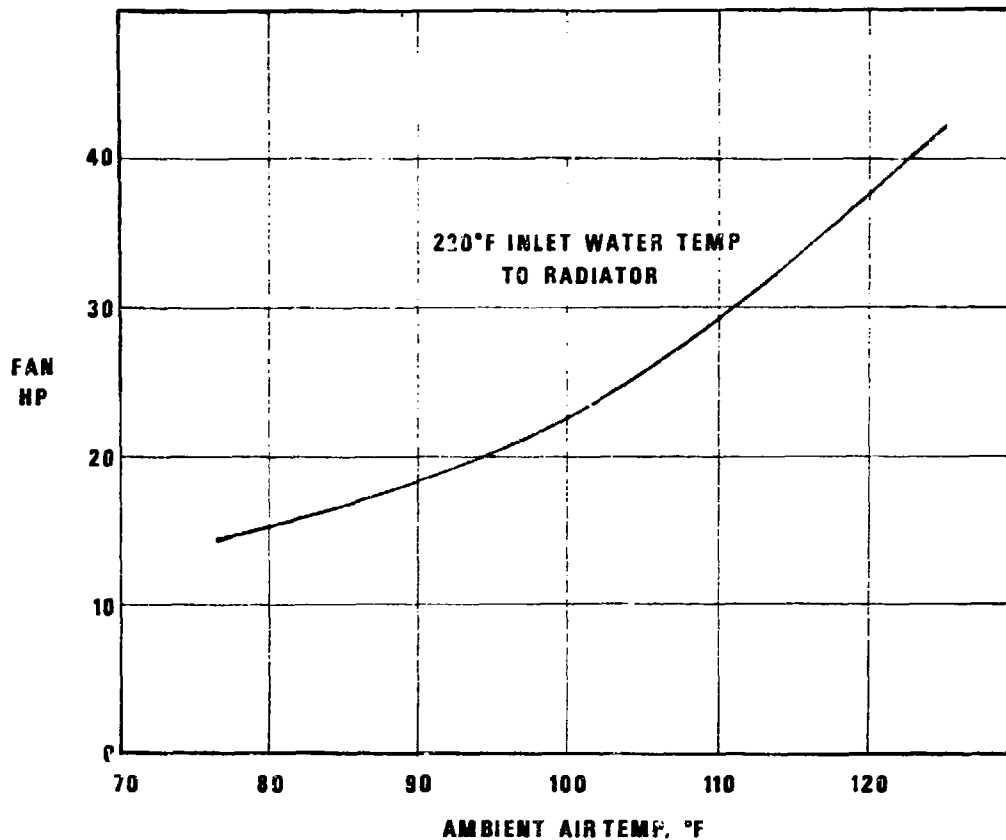
Figure 8-44. of Ambient Temperature on Required Fan Power
