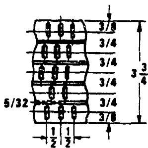
(A) RADIATOR CORE TYPE 1
