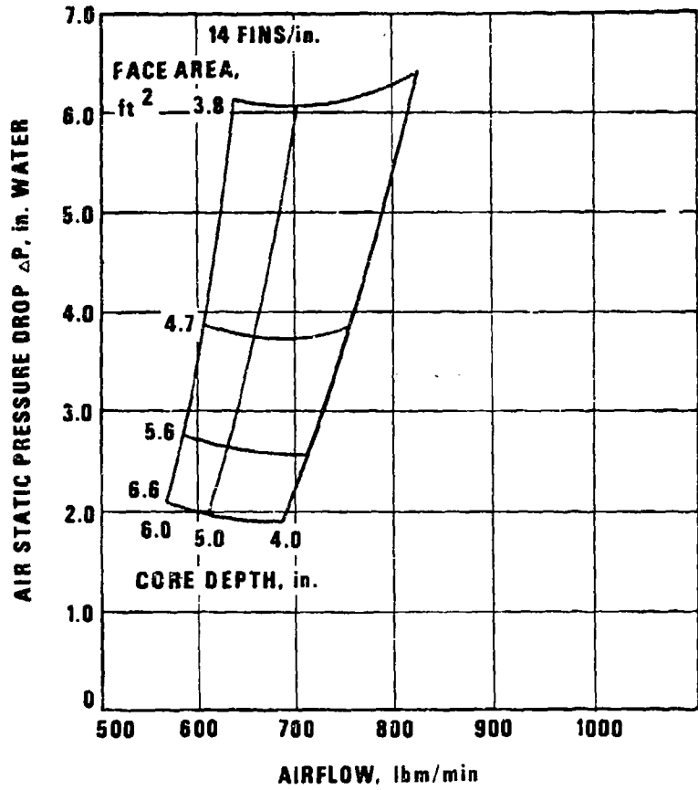
Figure 3-22. Radiator Core Performance Characteristics, 14 Fins/in. (Courtesy of Harrison Radiator Division-GMC)
