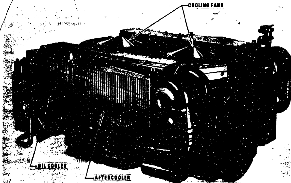
Figure 2-13. AVCR-1100-3B Tank Engine Oil Cooler Mounting
