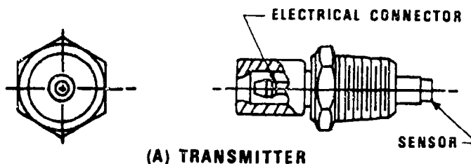
(A) TRANSMITTER
