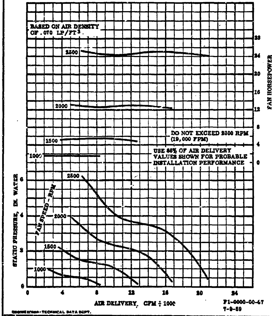
Figure B-40. Cooling Fan Performance Curve No. F1-0000-00-67
