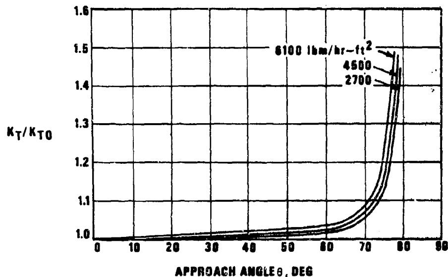
Figure 7-12. Effect of Angle on Heat Exchangers (Ref. 3) (Release granted by Society of Automotive Engineers, Inc., Aerospace Applied Thermodynamics Manual.)
