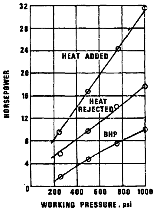
MODEL GPU-2.5 (SINGLE CYLINDER-RHOMBIC) 3000 RPM, 1300°F HEATER, 100°F WATER
