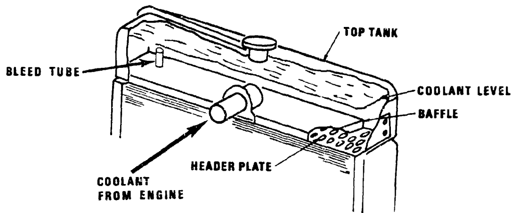
Figure 3-19. Radiator Deaeration System With Partial Baffle (Ref. 16) (Courtesy of Society of Automotive Engineers, Inc., Paper No. 670525 and Modine Manufacturing Company)
