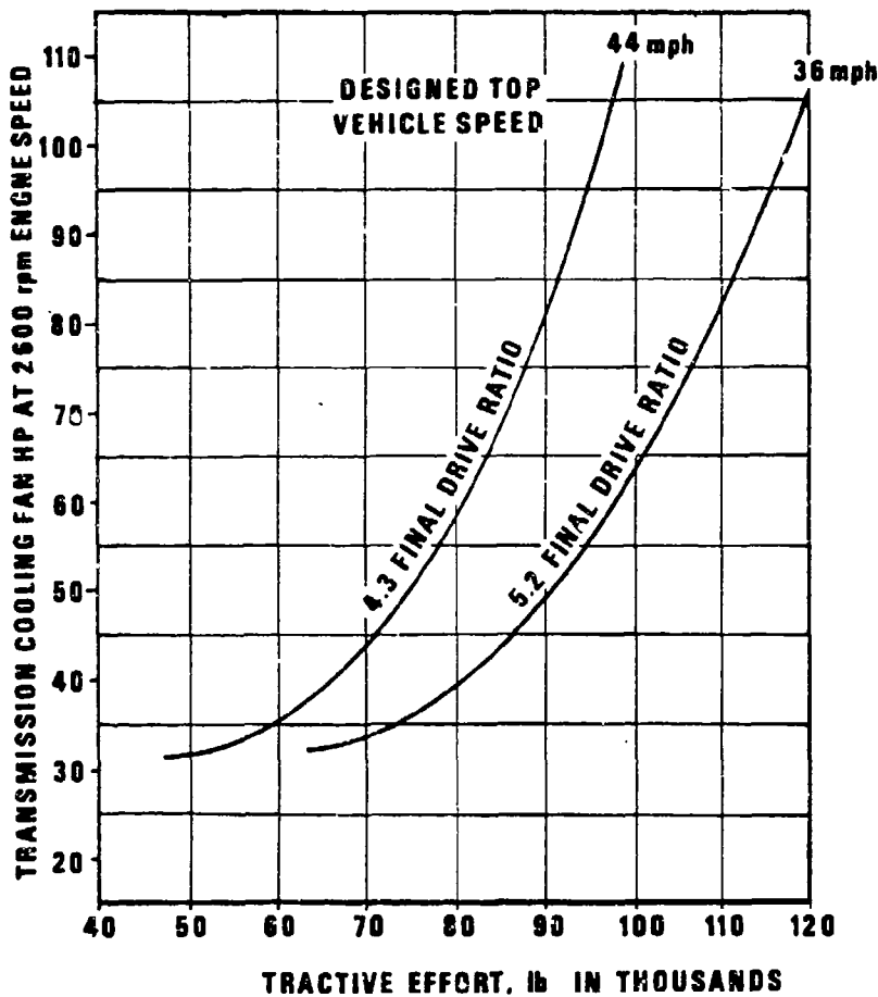
Figure 8-7. Effects of Transmission Gear Ratio Selection and Required Tractive Effort on Transmission Cooling Fan Horsepower Requirements
