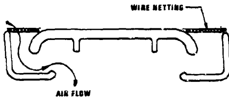
Figure 6-10. Tabie-top Grille Cross Section (USATACOM)
