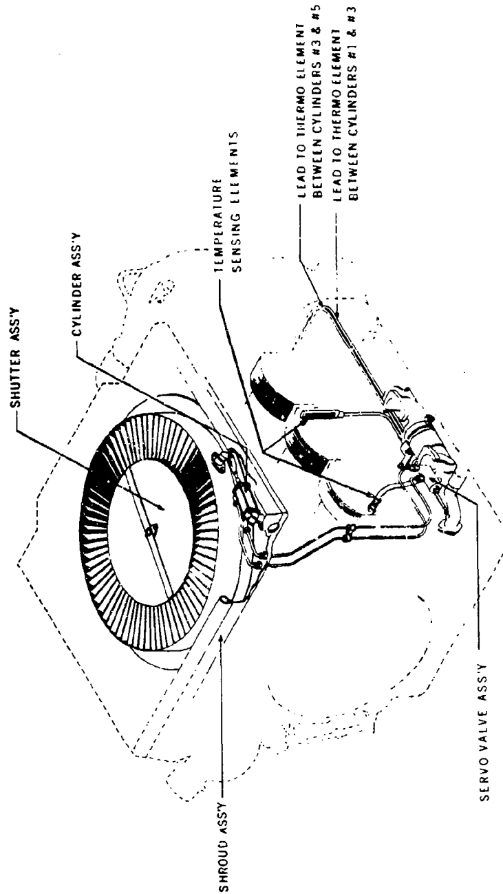
Figure 5-7. AOS-895-3 Air-cooled Engine Winterization Shutter Assembly (Ref. 2)
