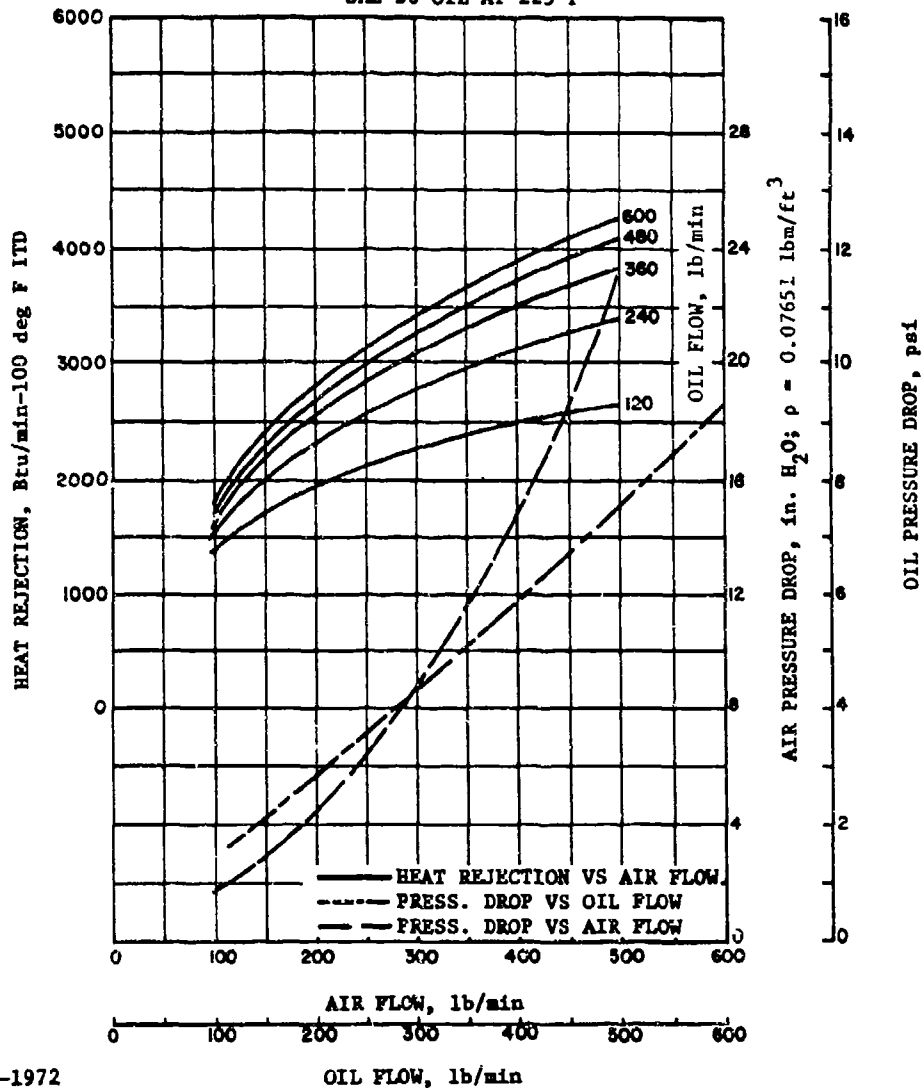
Figure A-10. 12.5 Fins/in., Core Depth 4.5 in., Oil Cooler Performance, i
