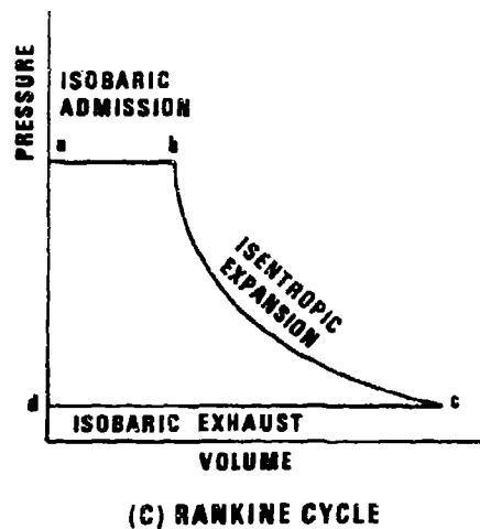
Figure 2-2. Thermodynamic Cycles—Brayton, Stirling, and Rankine (Refs. 3 and 19)
