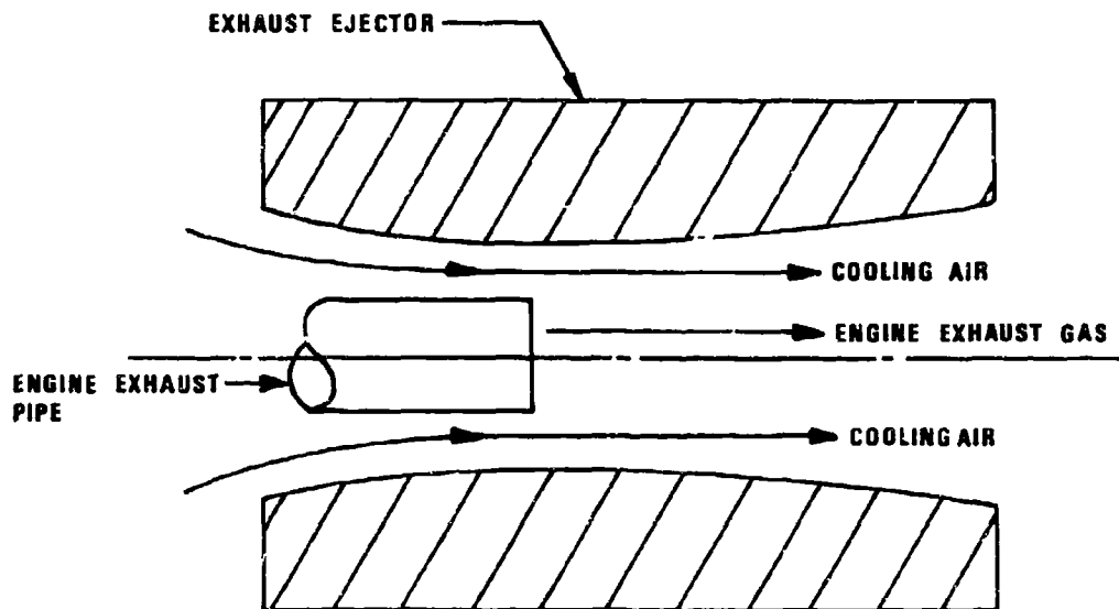
Figure 4-19. Exhaust Ejector
