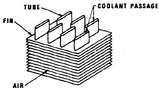
(B) PLATE-FIN CORE (Ref. 20)
