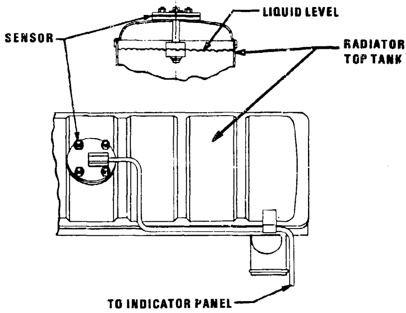
Figure 5-33. Radiator Coolant Level Sensor Installation (Courtesy of Teledyne Continental Motors)
