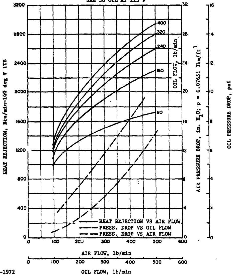
Figure A-5. 11 Fins/in., Core Depth 3 in., Oil Cooler Performance, I
