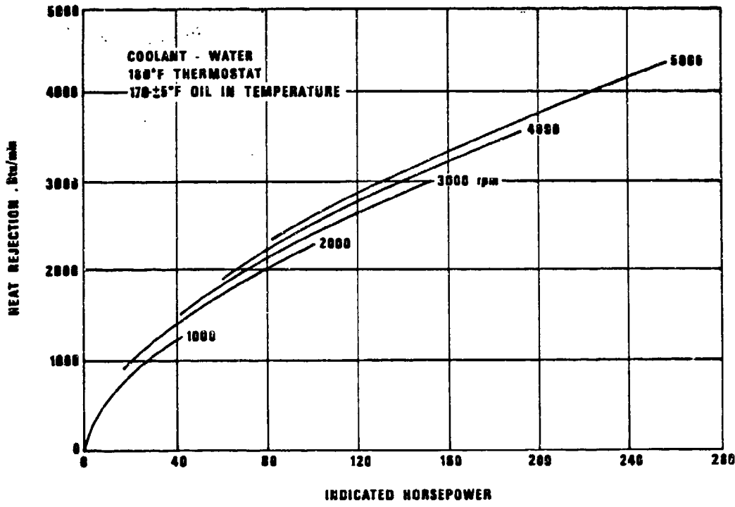
Figure 2-25. Curtiss-Wright Model RC2-60-U5 Engine Coolant Heat Rejection, Water Coolant (Courtesy of Curtiss-Wright Corporation)
