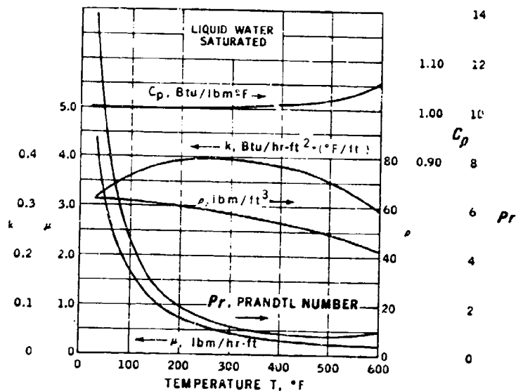
Figure 3-43. Properties of Water (Ref. 2) (From Compact Heat Exchangers by W. Kays and A. London, 1964. Used with permission of McGraw-Hill Book Company.)
