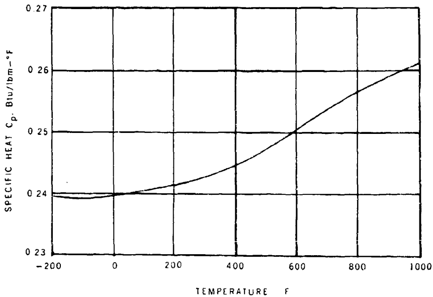
Figure 3-42. Properties of Air
