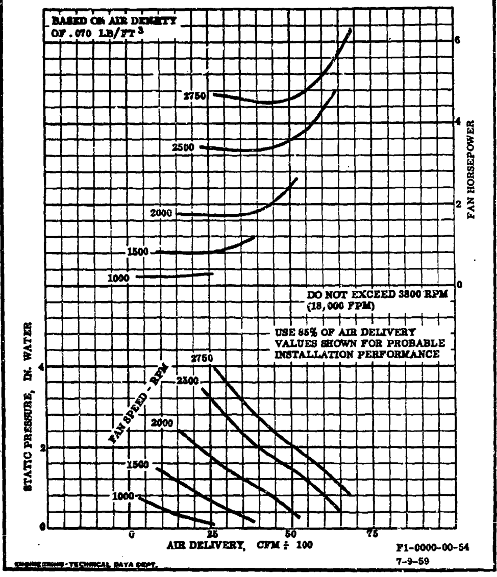
Figure B-35. Cooling Fan Performance Curve No. F1-0000-00-54
