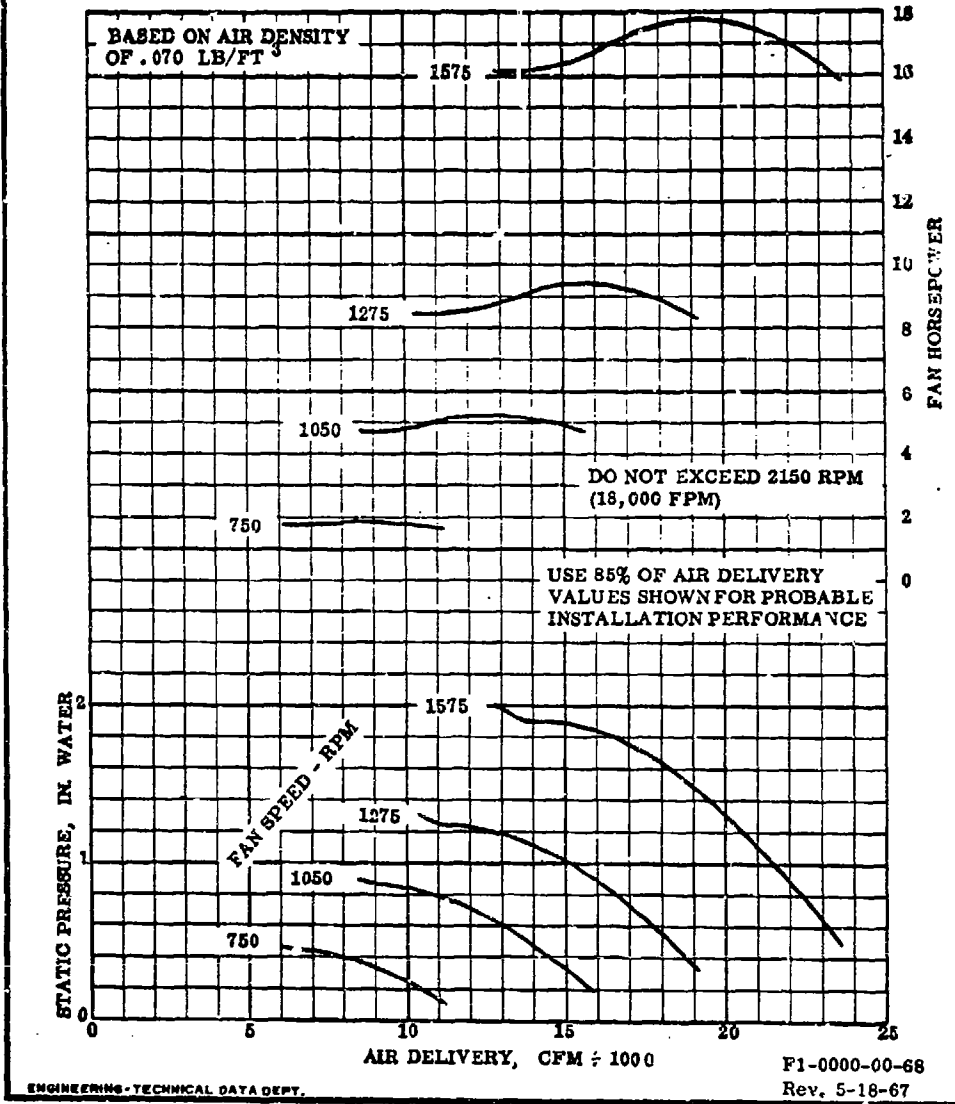
Figure B-41. Cooling Fan Performance Curve No. F1-0000-00-68
