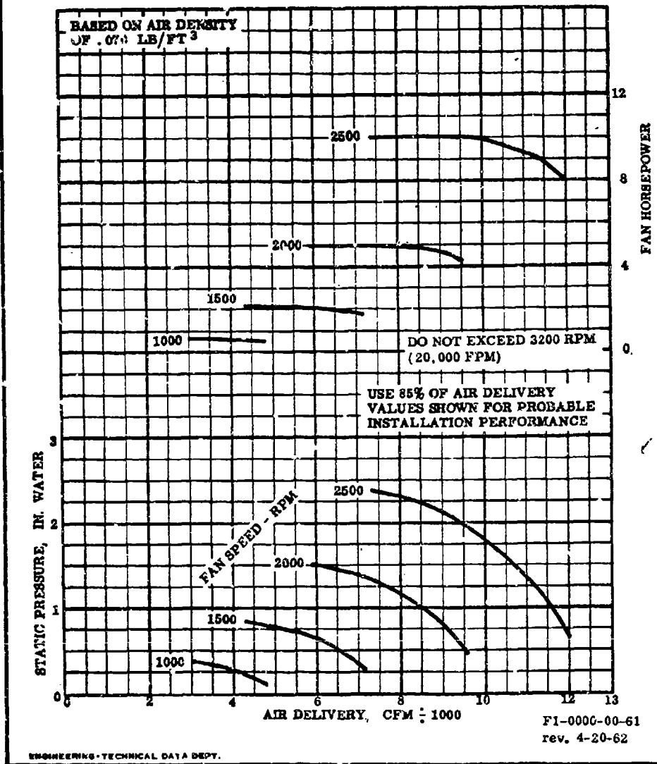
Figure B-38. Cooling Fan Performance Curve No. F1-0000-00-61
