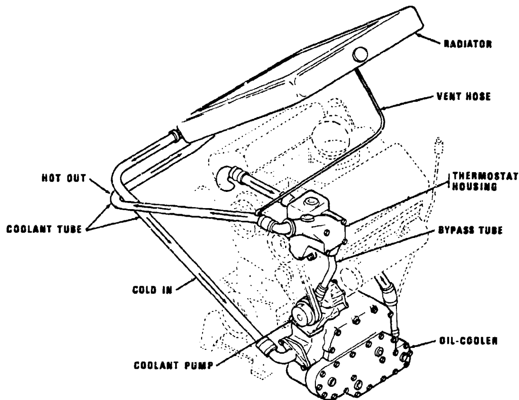
Figure 5-21. External Type Thermostat Bypass Arrangement (M113A1) (Ref. 10)
