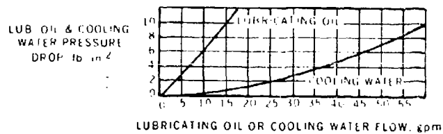
(B) PERFORMANCE CURVES
