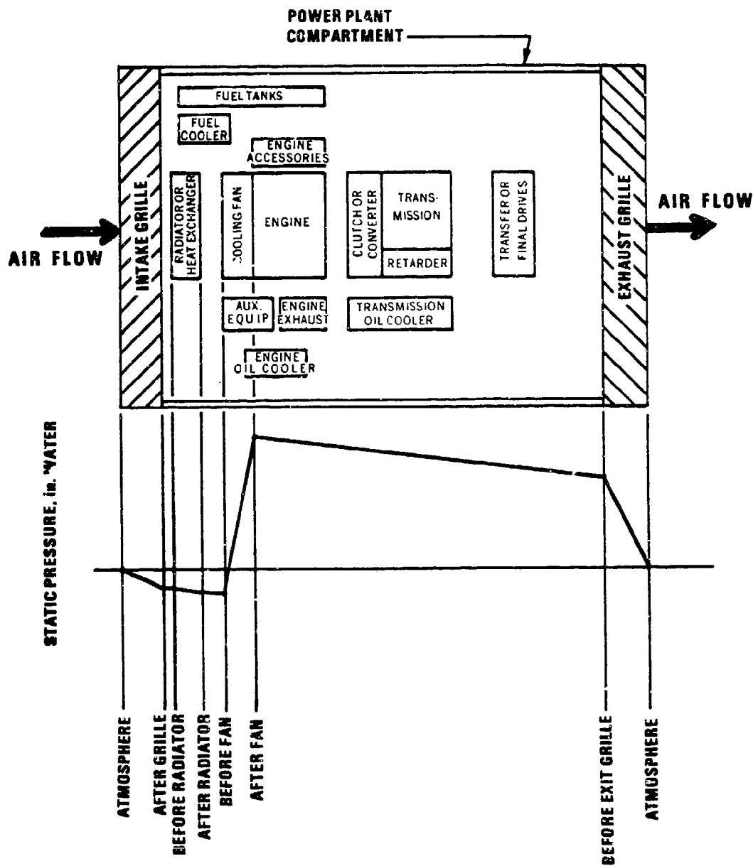
Figure 8-5. Cooling Air Static Pressure Profile
