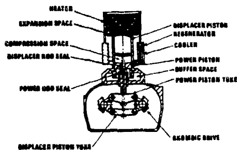
Figure 2-17. Cut-away View of the Stirling Engine (Ref. 5)
