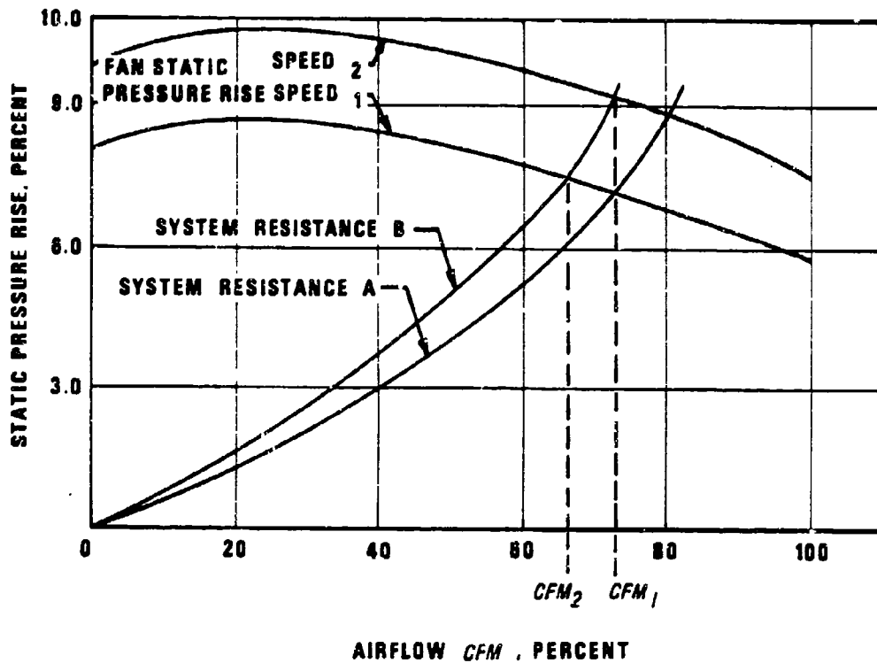
Figure 4-7. Change in Operating Characteristics of a Fan and Cooling System
