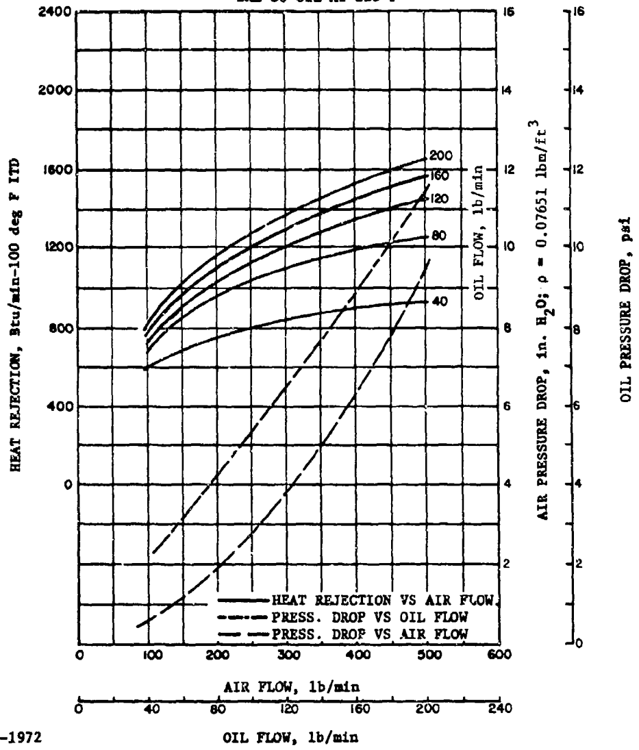
Figure A-2. 12.5 Fins/in., Core Depth 1.5 in., Oil Cooler Performance, I
