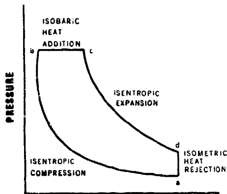
(C) DIESEL CYCLE
