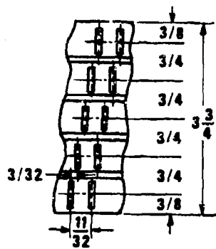
(C) RADIATOR CORE TYPE 5
