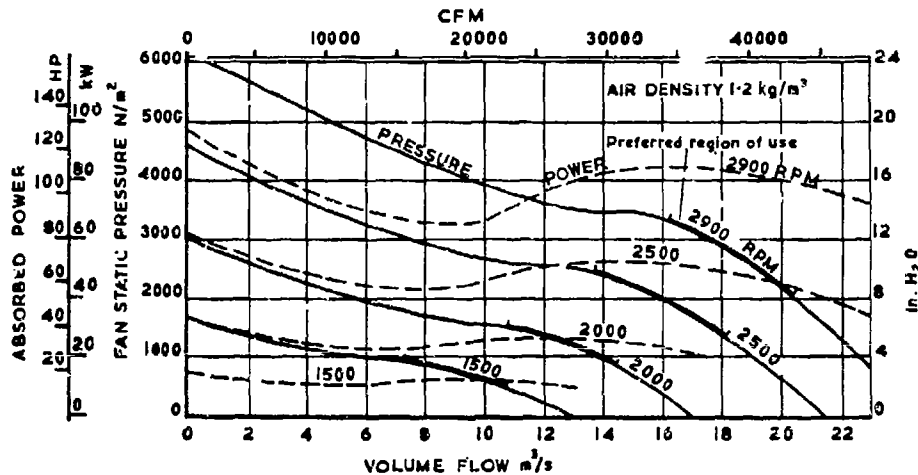
Figure B-33. Mixed Flow Fan Performance, Model 680 MP3 311 (Courtesy of Airscrew Hawden Ltd., Weybridge, Surrey, England)
