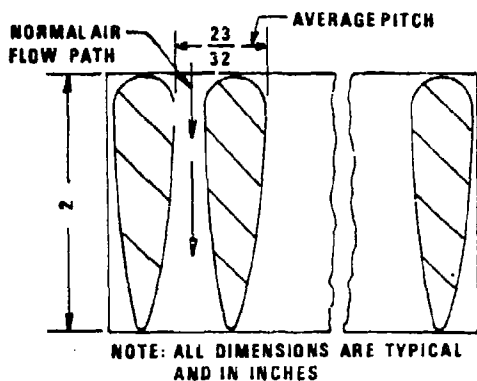
Figure 6-6. Venturi Type Louver Bar Grille Assembly (Ref. 2)
