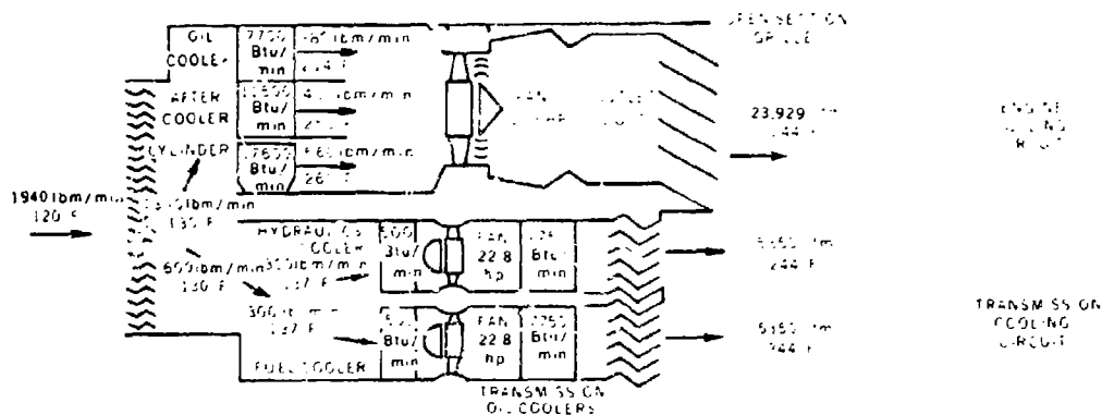
Figure 7-14. XM803 Experimental Tank Cooling System Analysis Diagram (Ref. 8)
