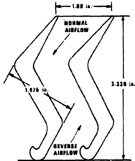
Figure 6-11. Chevron Type Grille Design Characteristics, MBT70 Prototype Tank (USATACOM)
