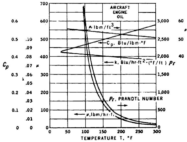
Figure 3-45. Properties of Aircraft Engine Oil (Ref. 2) (From Compact Heat Exchangers by W. Kays and A. London, 1964. Used with permission of McGraw-Hill Book Company.)
