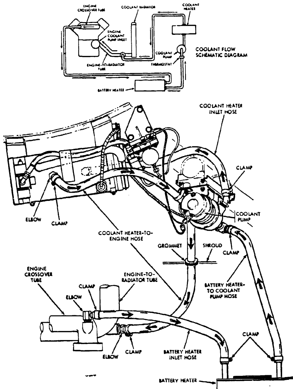
Figure 1-50. SHERIDAN, M551, Standby Winterization Kit (Ref. 13)
