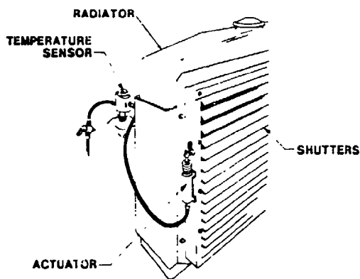
Figure 5-3. Thermal Actuated Radiator Shutters (Courtesy of Kysor of Cadillac)
