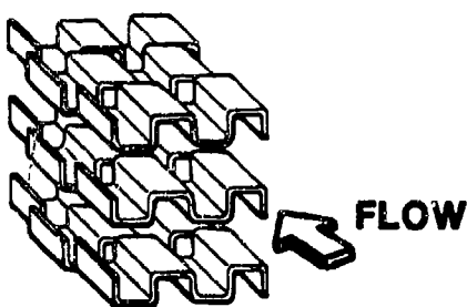
(A) OFFSET FIN (sometimes called segmented fin, serrated fin, or strip fin)
