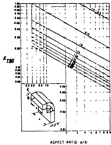
(A) Loss Coefficient for 90-deg Bends, Rectangular Ducts, Re = 100,000
