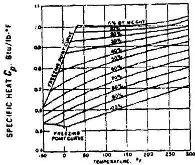
(A) SPECIFIC HEAT OF AQUEOUS SOLUTIONS OF ETHYLENE GLYCOL
