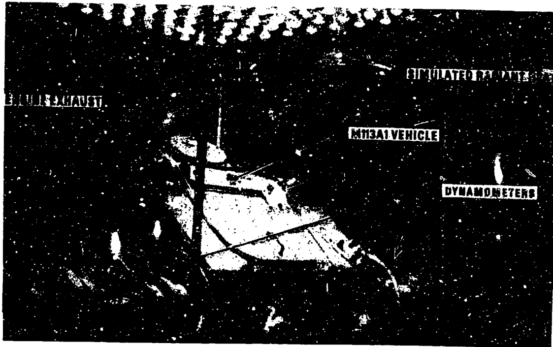
Figure 9-7. M113A1 Vehicle Cooling Test Installation (USATACOM)
