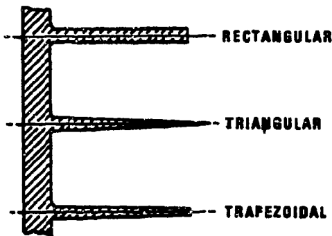
Figure 2-15. Basic Shapes of Cylinder Fins
