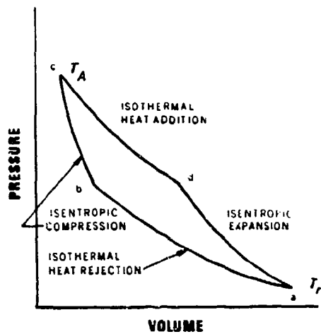
(A) CARNOT CYCLE
