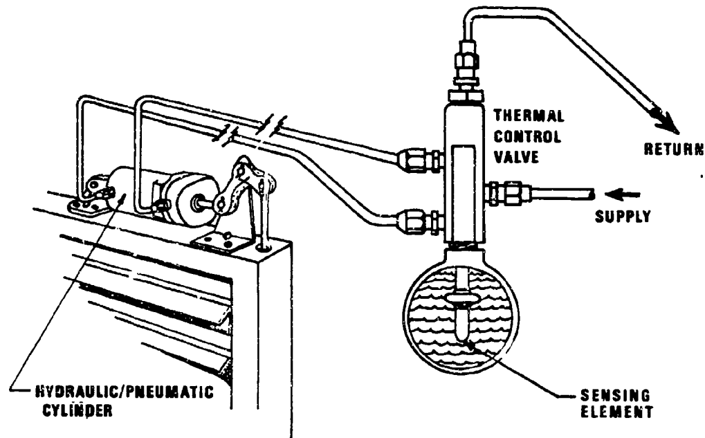
Figure 5-4. Hydraulic or Thermally Controlled Shutter Systems (Courtesy of Kysor of Cadillac)
