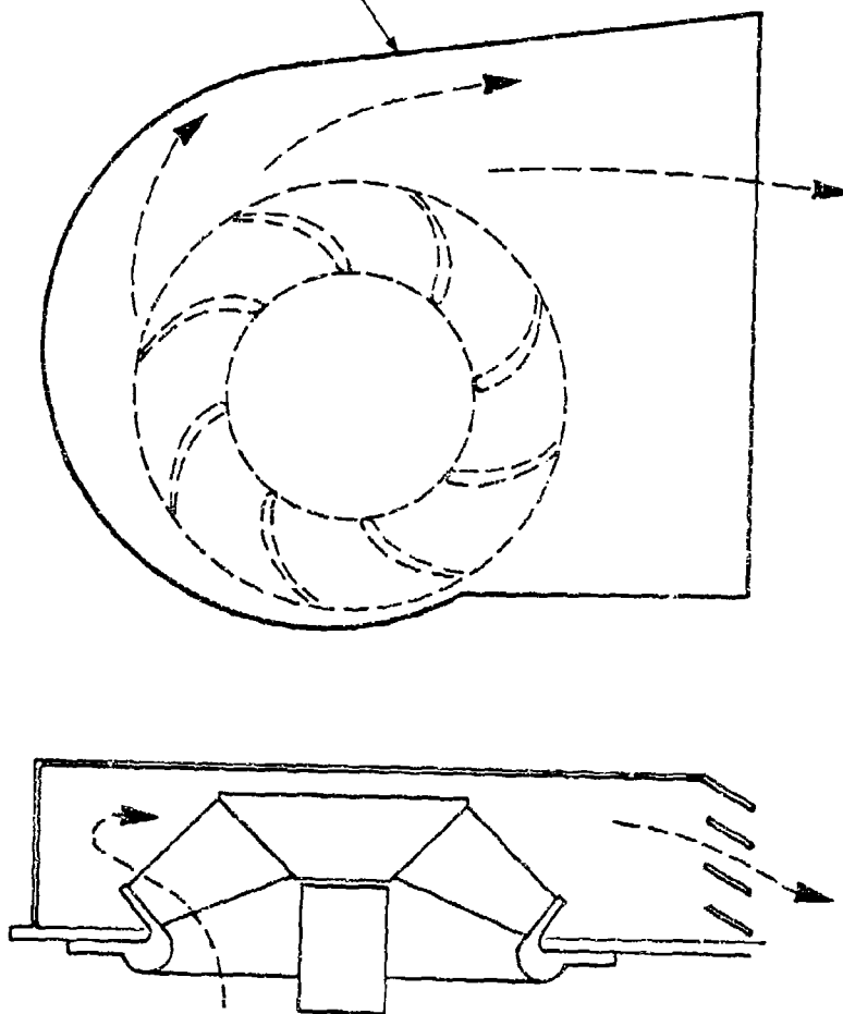
Figure B-27. Mixed Flow Fan With Valute Casing
