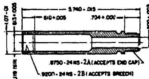
Figure 6-11. Thruster Body
