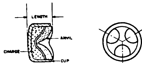
Figure 4-9. Percussion Primer
