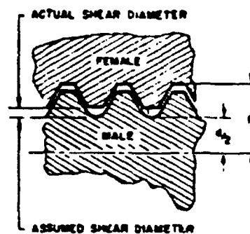
Figure C-1. Thread Parameters
