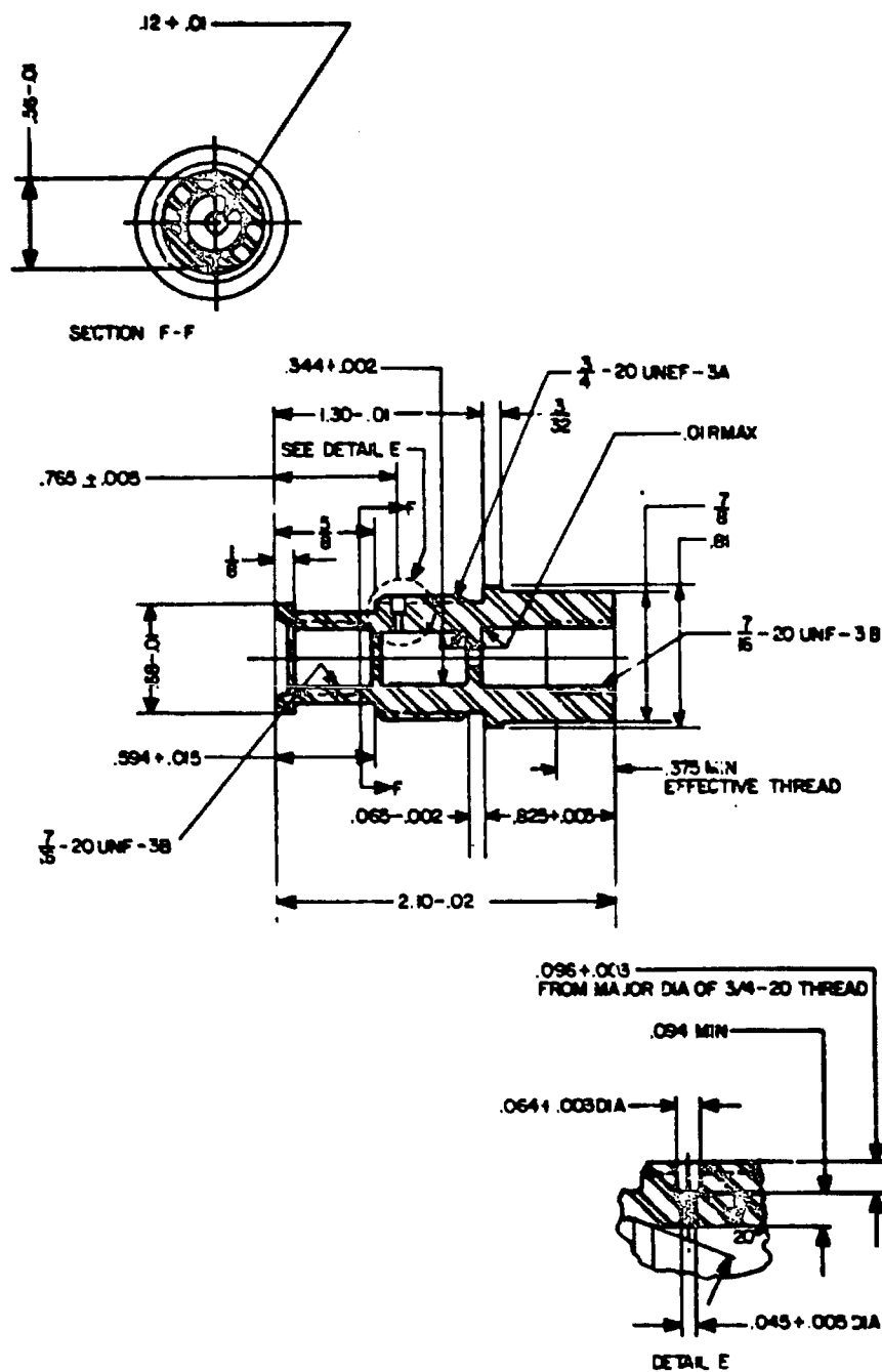
Figure 6-23. Housing
