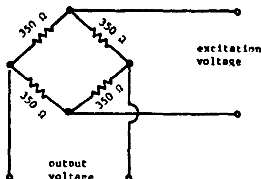
Figure 7-4. Wheatstone Bridge Strain Gage Transducer
