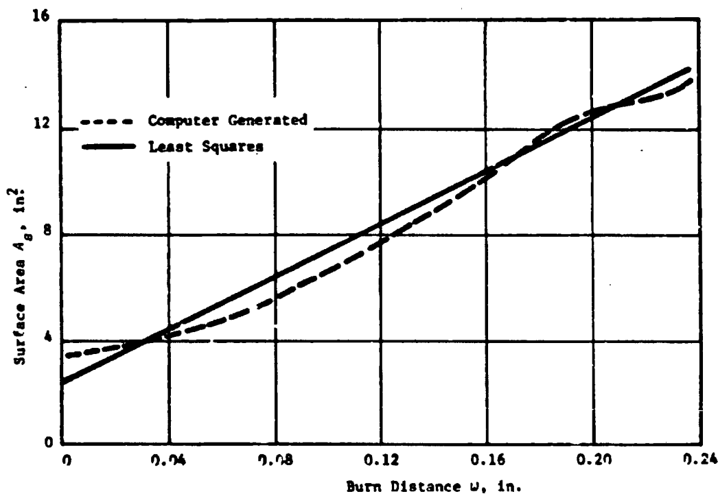
Figure 5-11. Surface Development vs Burn Distance for High-Low System
