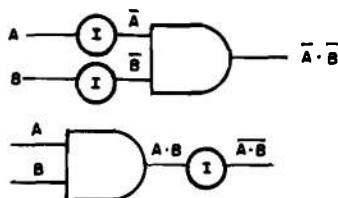
Figure A-4. Symbolic Representation of not A AND not B, also not (A \text{ AND } B)^2
