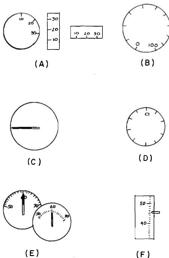
Figure 16-79. Recommended Readout Display Scales
