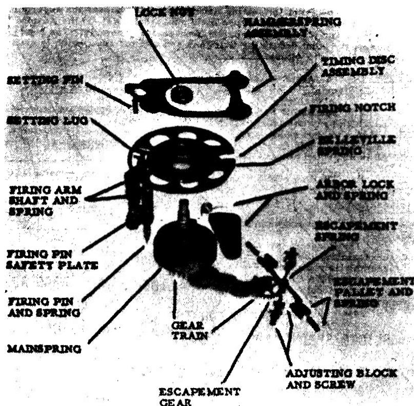
Figure 12-9. Timing Mechanism of Fuze, MTSQ, M564
