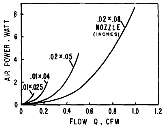
Figure 23-26. Air Power Expended in Typical Rectangular Nozzles
