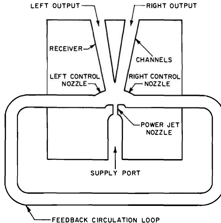
Figure 24-8. Sonic Oscillator 1 6
