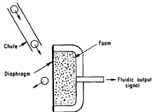
Figure 23-19. Flueric Moving-part Detector 4
