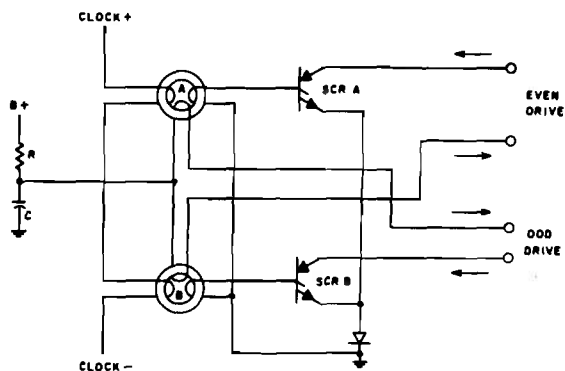
Figure 11-16. Two Phase Driver
