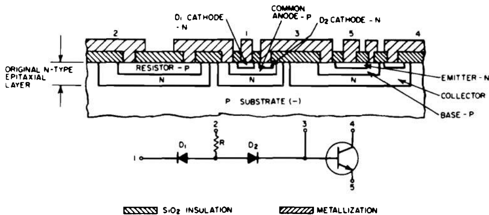
Figure 8-9. Typical Diffused Integrated Circuit Components 7,13
