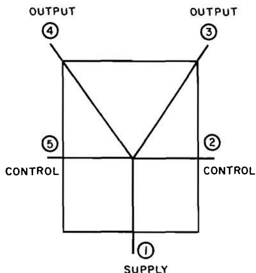
Figure 24-16. Five Port Flip-flop Schematic
