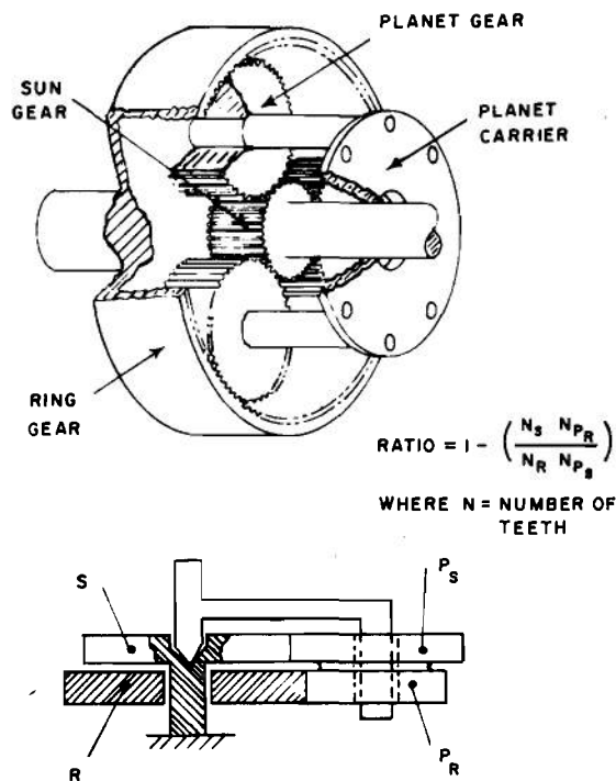
Figure 16-11. Epicyclic Gearing
