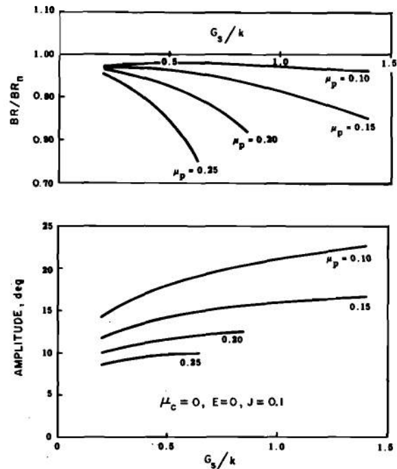
Figure 16-37. Pallet Friction Variation
