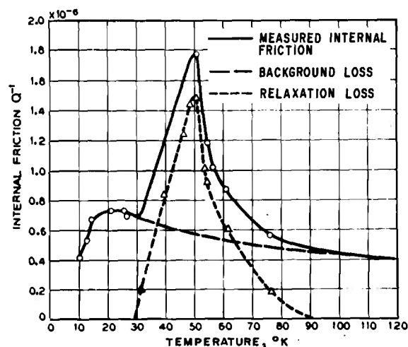
Figure 4-8. Friction Losses in Quartz 12
