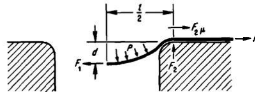
Figure 23-13. Forces Acting on Tape Segment 4
