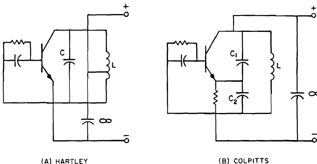
Figure 11-1. Parallel Resonant Oscillators
