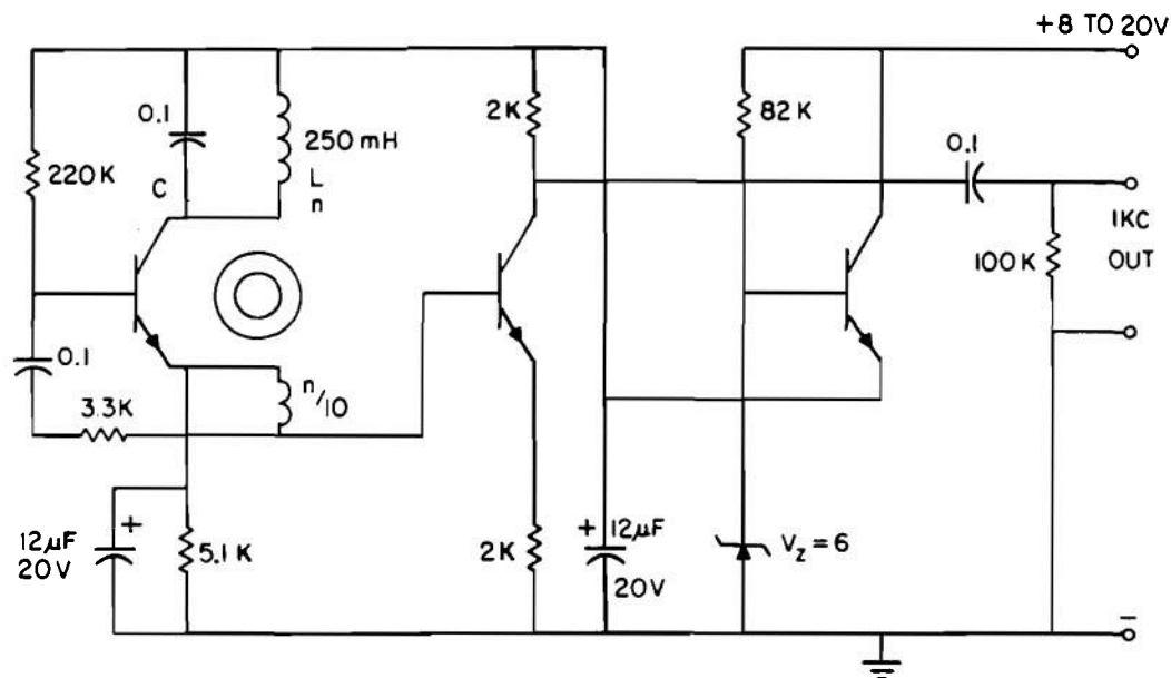
Figure 11-2. Tuned-output Oscillator
