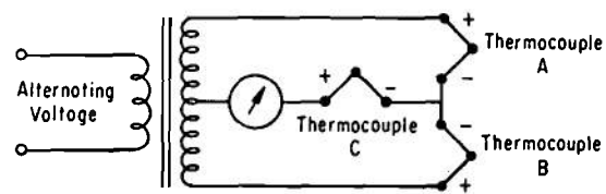
Figure 23-28. Three-thermocouple Compensated Type Flow Meter 7
