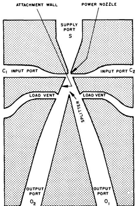
Figure 24-14. Bistable Flip-flop
