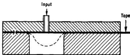
Figure 23-12. Tape Actuator 4
