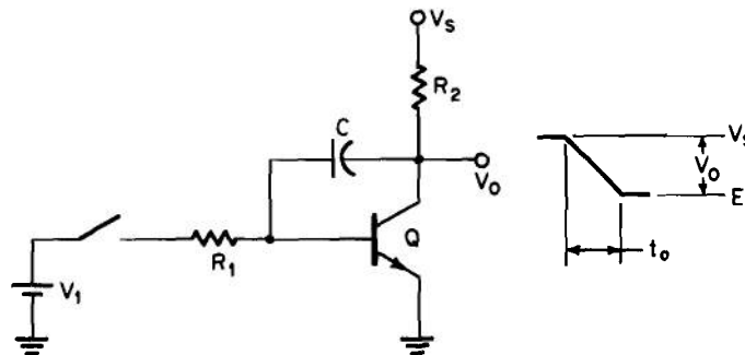
Figure 10-12. Miller Integrator
