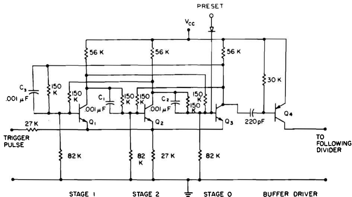
Figure 11-14. Ternary Divider
