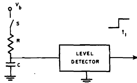
(A) ANALOG CHARGING CIRCUIT
