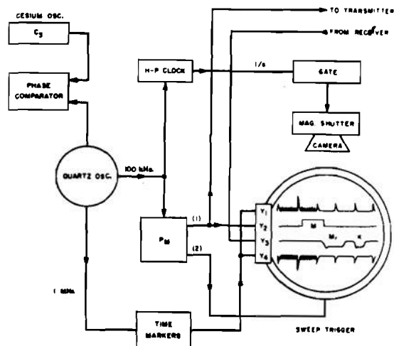
Figure 5-20. Equipment Used at Mojave To Generate and Record Pulses 5
