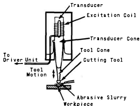
Figure 25-14. Ultrasonic Machining 2
