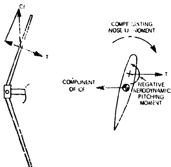
Figure 5-55. Compensation for Negative Pitching moment With Coning Angle and Aft Blade CG
