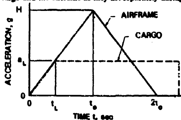
(A) ACCELERATION-TIME HISTORY OF CARGO AND AIRFRAME
