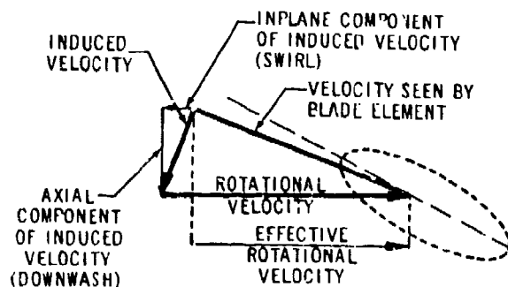
Figure 5-1. Vector Diagram of Swirl in Hover
