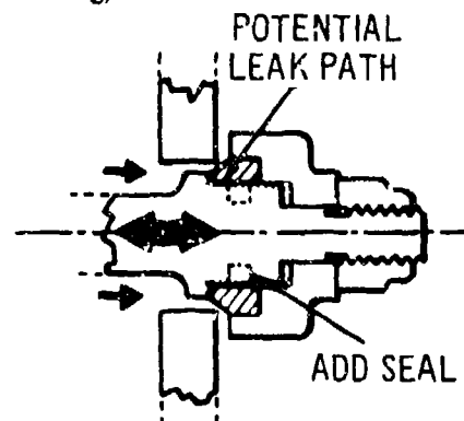
Figure 9-51. Secondary Leak Path Seal
