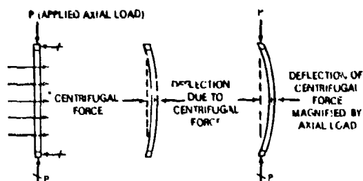
Figure 6-10. Centrifugal Force Deflections
