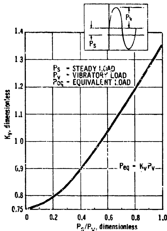
Figure 16-2. Equivalent Steady Load for Combination of Steady and Vibratory Loads (Reversing)
