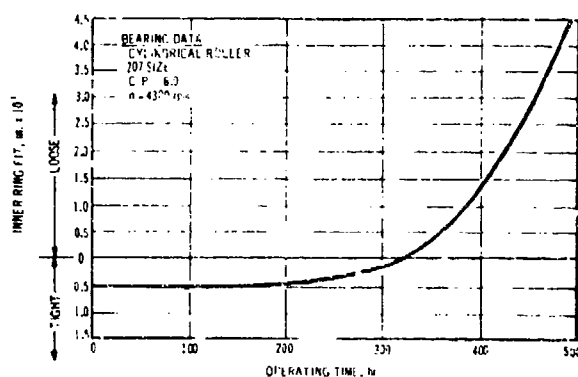
Figure 4-27. Creep Wear — Inner Ring Fit vs Operating Time
