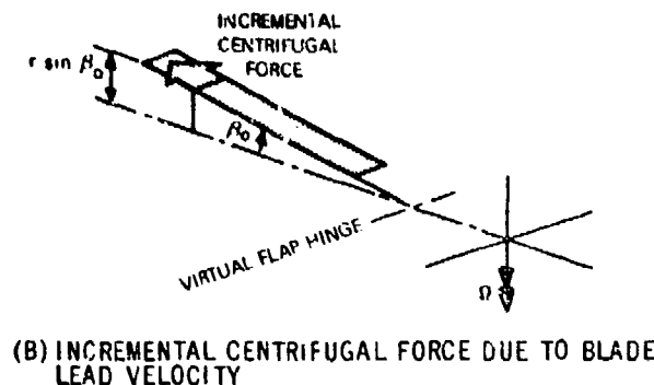
Figure 5-13. Mechanism of Flap-lag Instability
