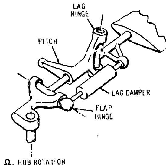
Figure 5-3. Articulated Rotor Schematic
