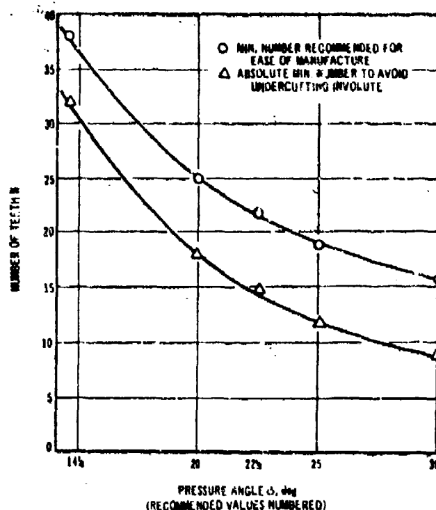
Figure 4-33. Involute Spline Data \phi vs N
