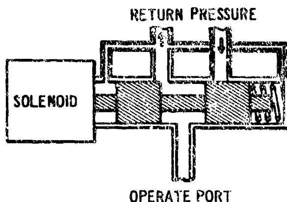
Figure 9-38. Direct-operated Valve
