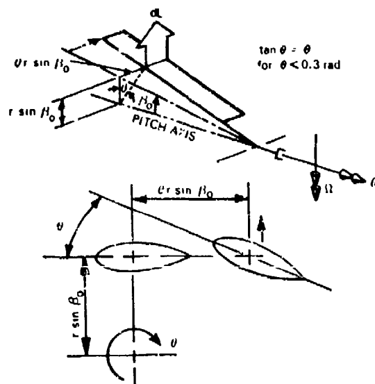
Figure 5-12. Pitch-flap Coupling of Rotors
