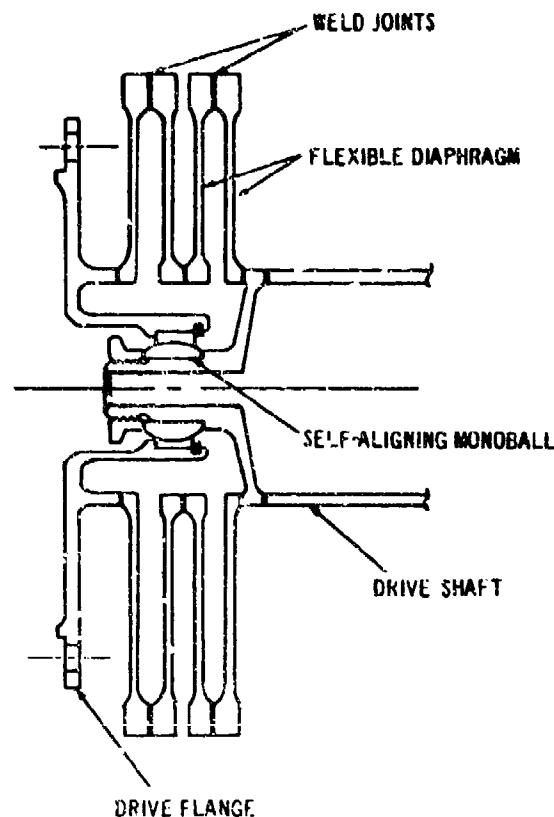
Figure 4-38. Flexible Diaphragm Coupling
