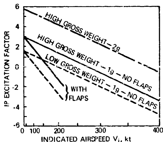
Figure 5-36. IP Excitation Diagram for Typical STOL Aircraft
