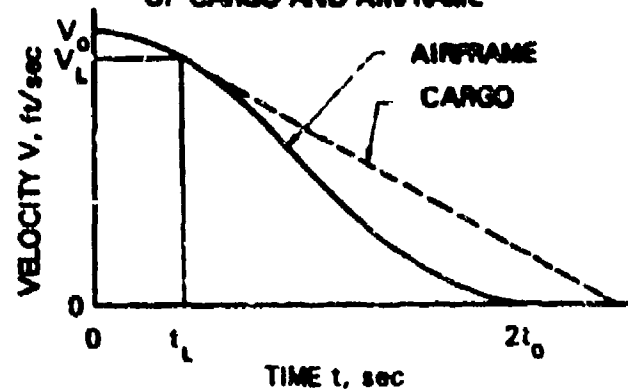
(B) VELOCITY-TIME HISTORY OF CARGO AND AIRFRAME
