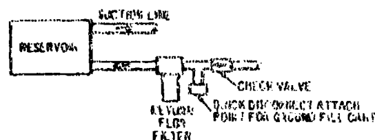
Figure 9-18. Hydraulic System Ground FOS Provisions
