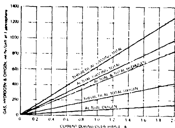
Figure 7-12. Gases Emitted from Nickel-Cadmium Sintered Plate Cell During Overcharge at 70°-75°F
