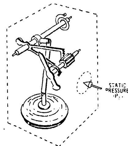
Figure 9-63. Altimeter Schematic
