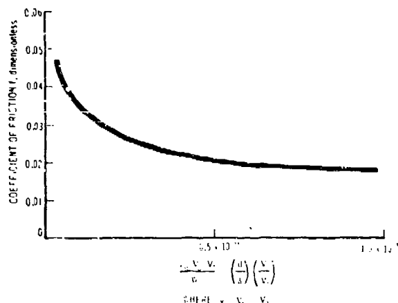
Figure 4-5. Friction Coefficient vs EHD Parameters — Region I and II
