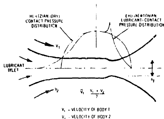
Figure 4-4. Elastic Body Contact Pressure Distribution and Interface Contour
