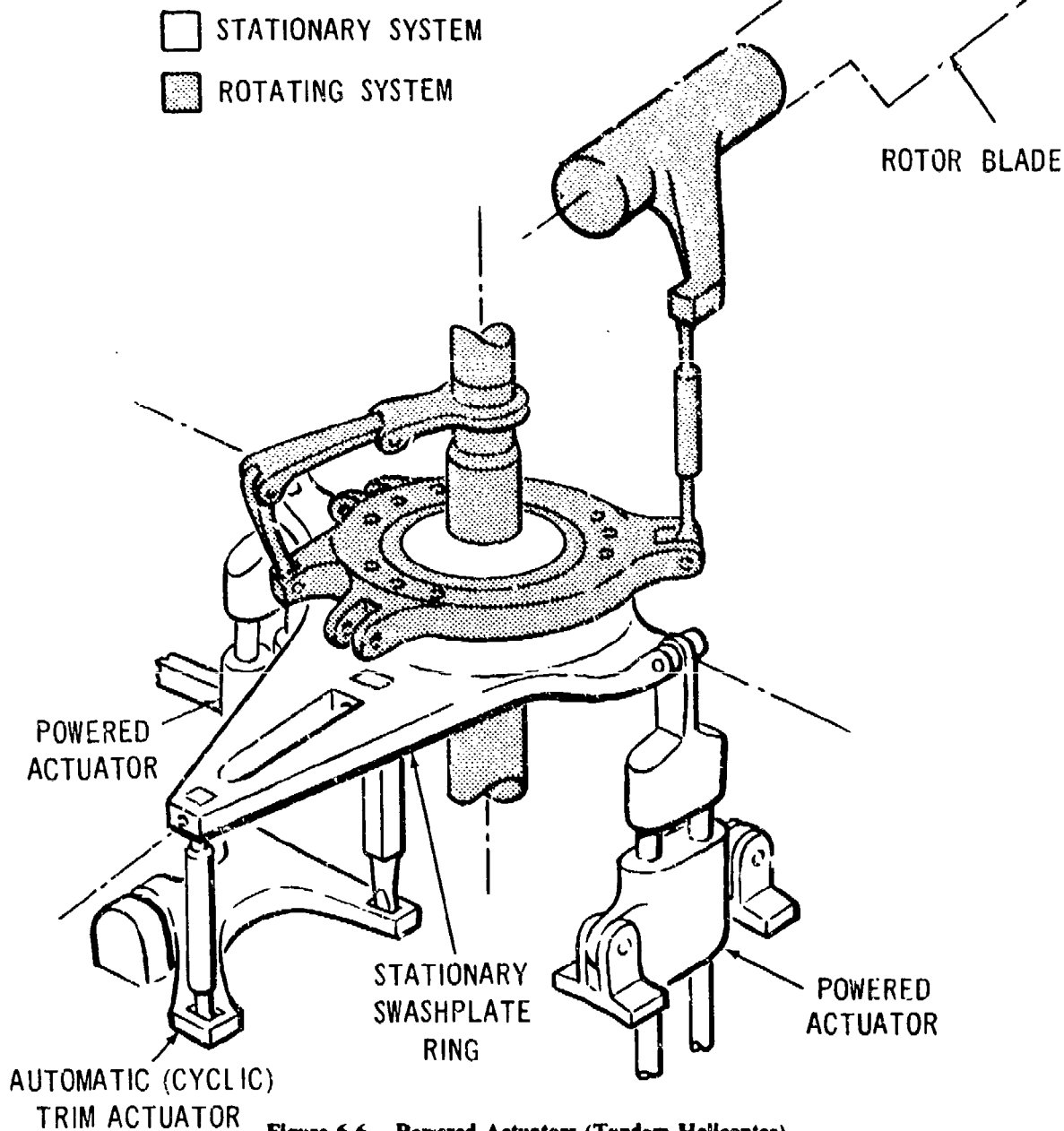
Figure 6-6. Powered Actuators (Tandem Helicopter)
