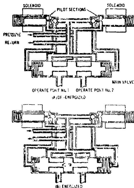
Figure 9-39. Pilot-operated Valve
