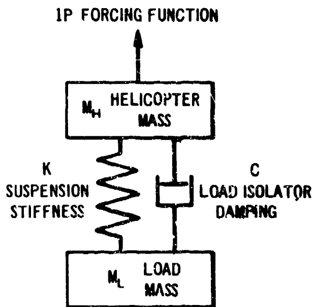
Figure 13-9. Helicopter/Load Dynamics Schematic
