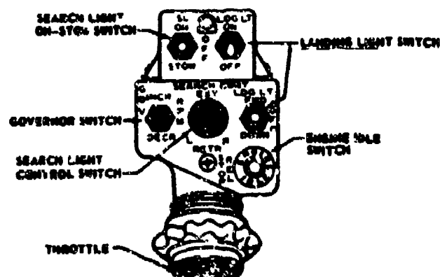
Figure 13-4. Example of Collective Control Head
