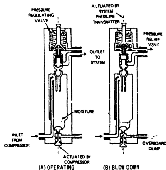
Figure 9-54. Moisture Separator Incorporating System Pressure Regulating Valve
