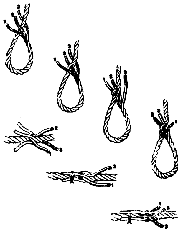
Figure 17-16. Cable Splicing
