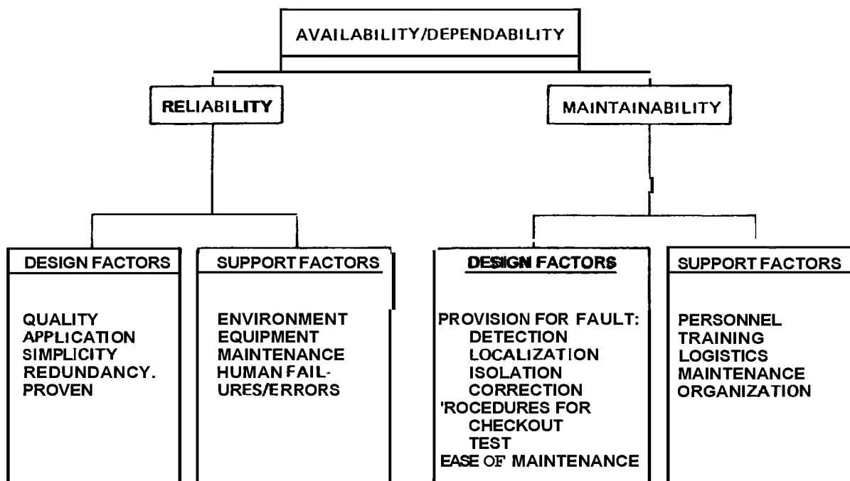
FIGURE 1-4. Reliability/Maintainability Relationships?
