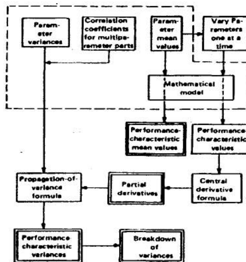
Figure 10-6. Moment Method
