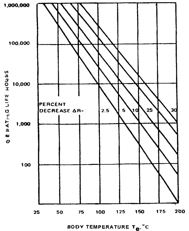
FIGURE 9-7. Determination of Resistor Longevity as Related to Body Temperature, for MIL-R-11 Resistors, All Styles'
