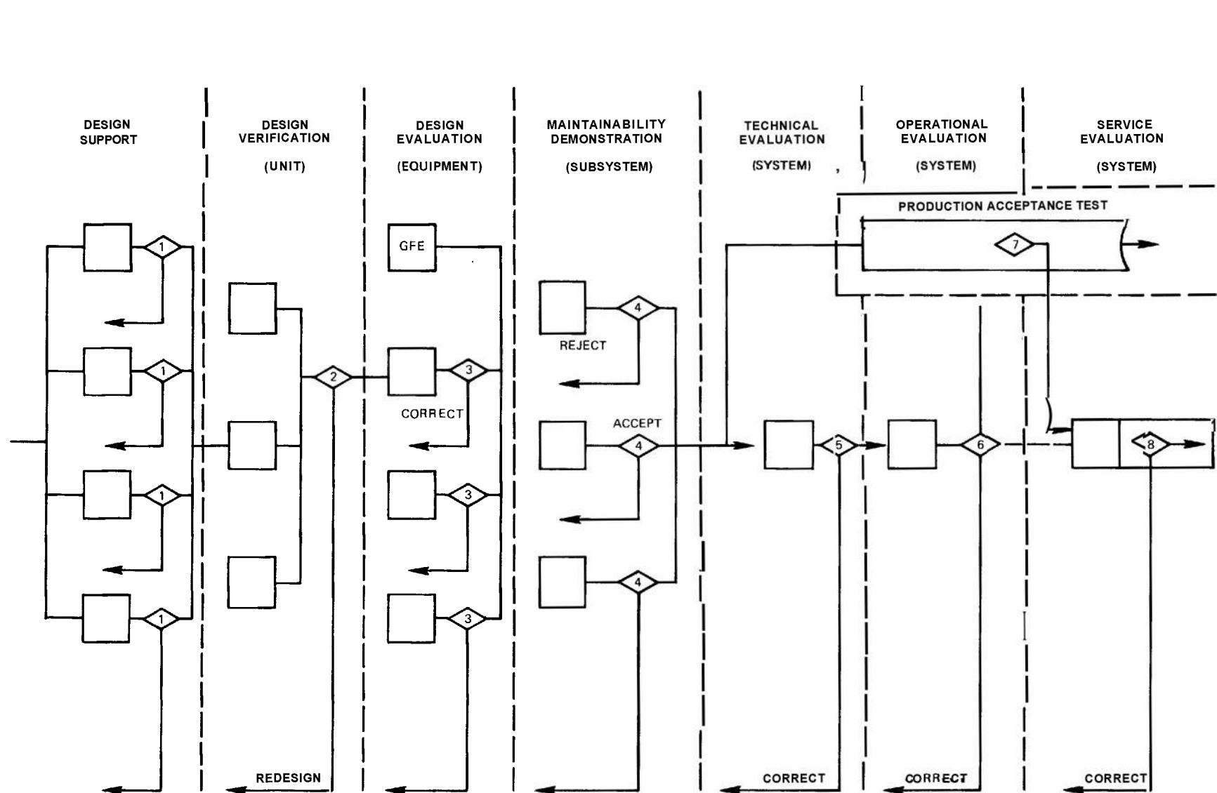
Figure 6-1. Decision Points Requiring Maintainability Test Data
