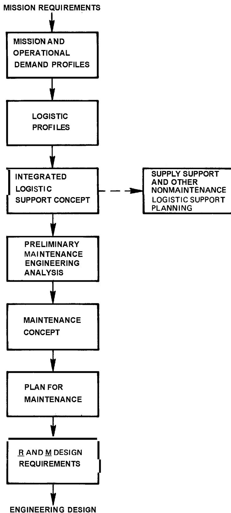
Figure 3-8. Maintenance Engineering Analysis During Early Program Stages
