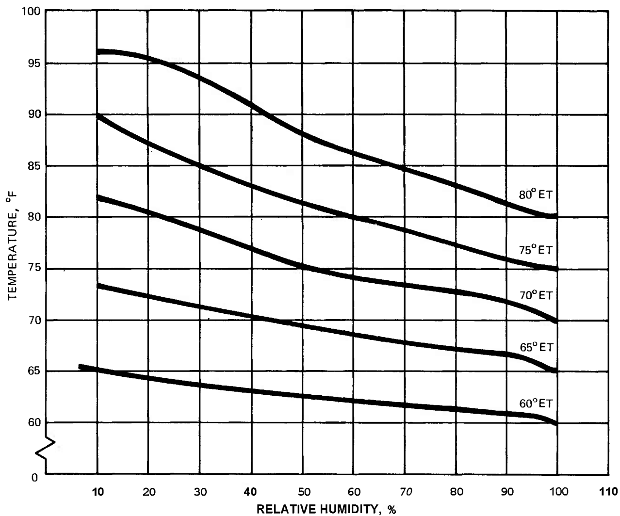
Figure 5-14. Effective Temperature (ET) Curves
