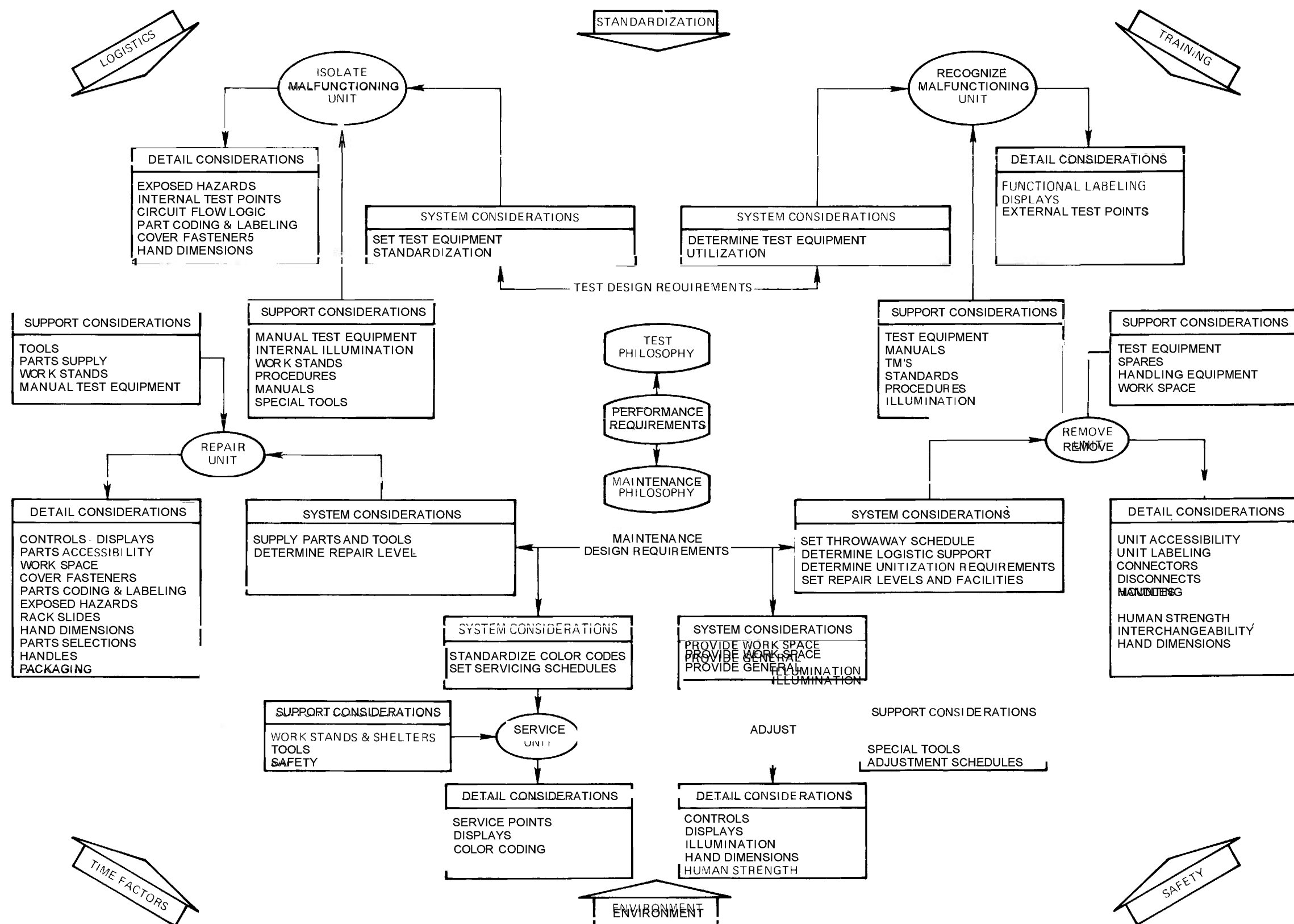
Figure 5-12. Maintainability Design Considerations
