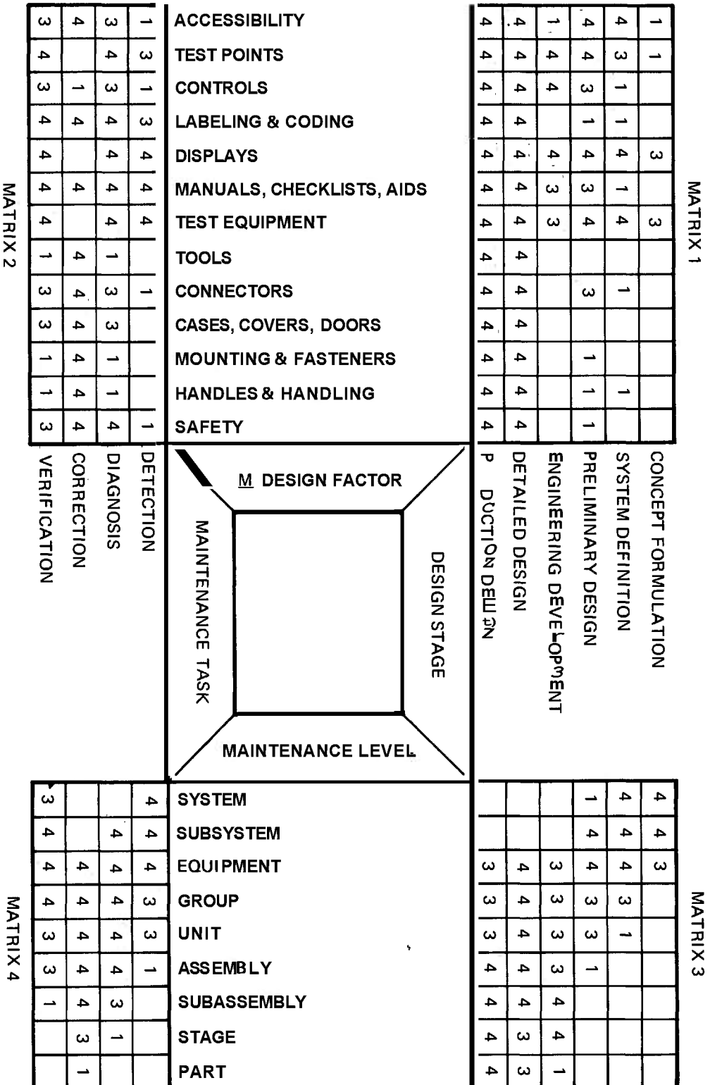
Figure 5-7. Maintainability Design Relations
