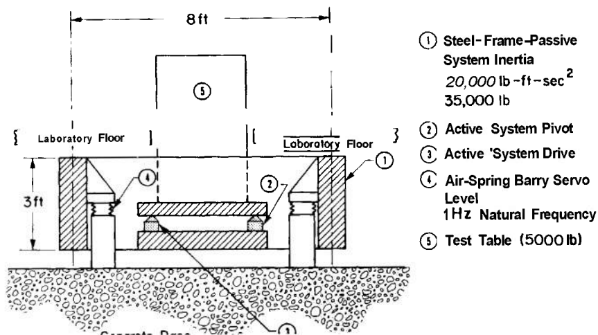
FIGURE 4-73. Active (Servocontrol) Base-motion Isolation System (Ref. 1).
