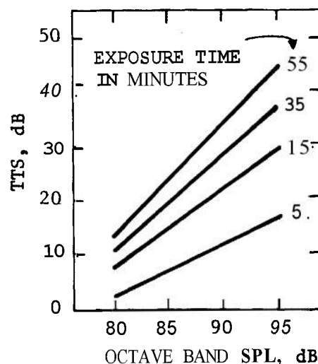
FIGURE 7-5. Temporary Threshold Shift (TTS) as a Function of Sound Pressure Level (SPL) for Exposure to an Octave Band of 2 to 4 kHz (Ref. 31).
