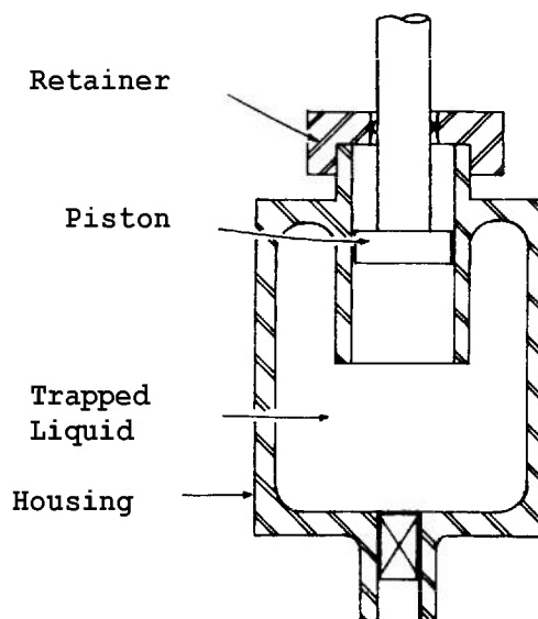
FIGURE 4-62. Liquid Spring or Dashpot (Ref. 63).
