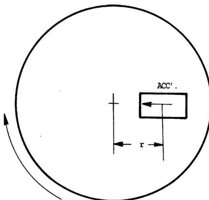
FIGURE 6-10. Accelerometer Mounted on Centrifuge for Calibration.
