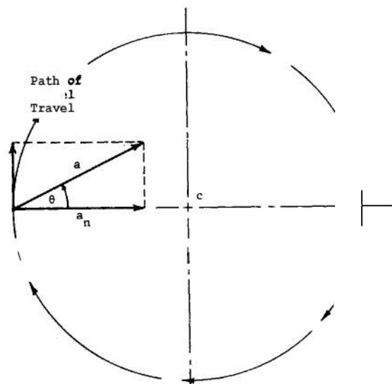
FIGURE 6-2. Total Acceleration as the Vector Sum of the Normal and Tangential Components.
