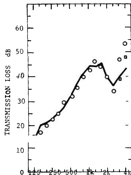
(A) Each leaf 2.7 \text{ lb ft}^{-2} , spacing 3\text{--}5/8 \text{ in.}
