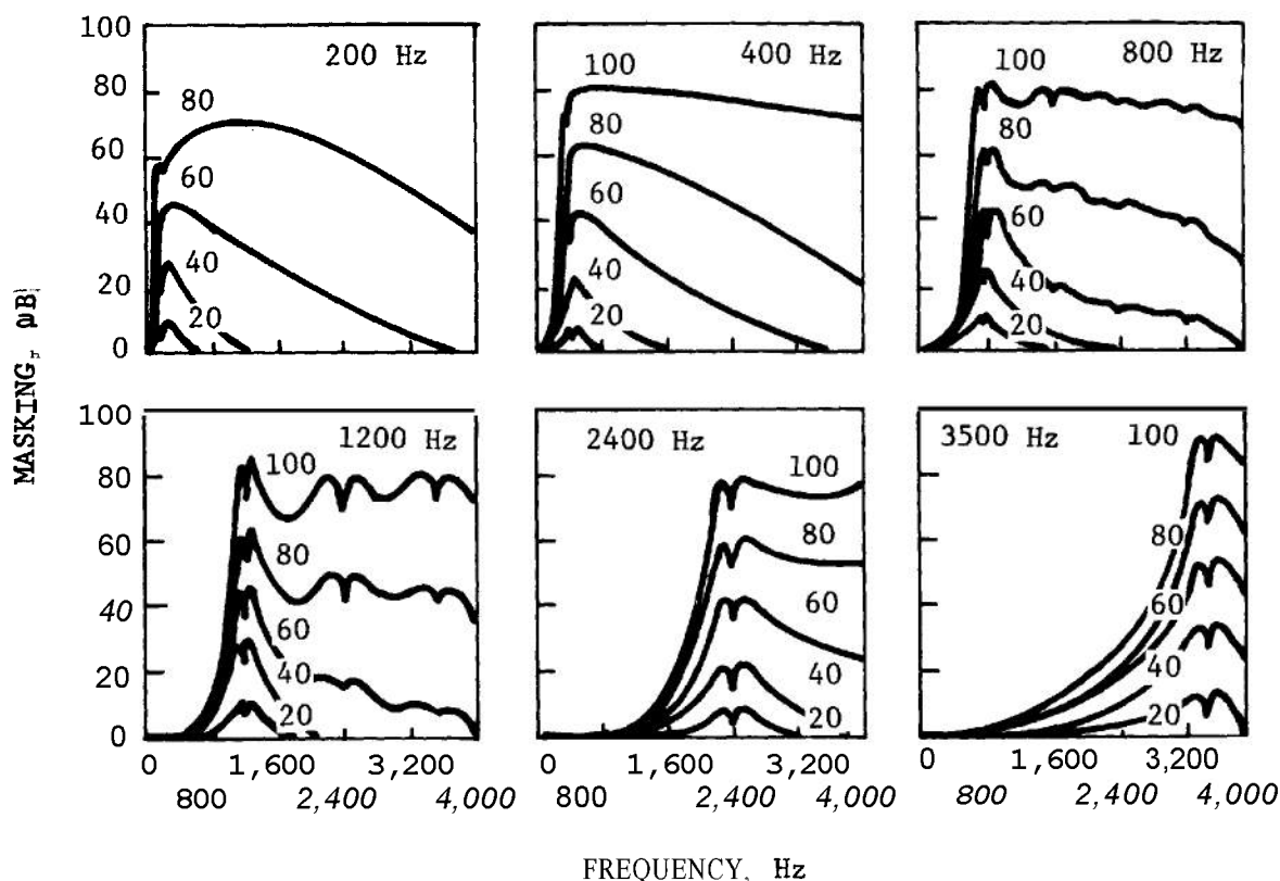
FIGURE 7-16. Masking as a Function of Frequency for Masking by Pure Tones of Various Frequencies and Levels, (Number at top of each graph is the frequency of masking tone. Number of each curve is level above threshold of masking tone) (Ref. 77).
