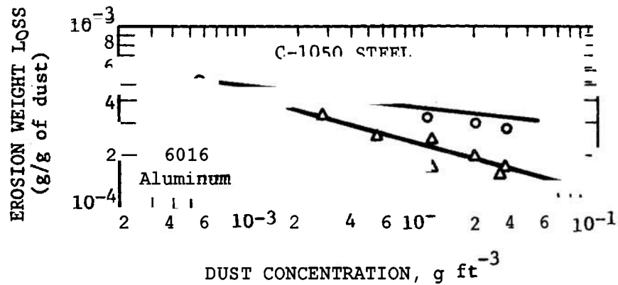
FIGURE 3-20. Erosion Loss vs Dust Concentration (Material type: noted; material temperature: ambient; dust velocity: 475 fps; dust size: 0-74 μm.)
