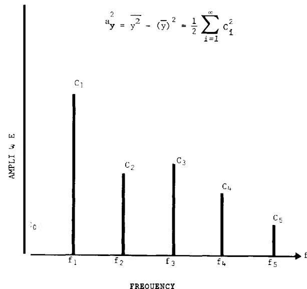
FIGURE 4-47. Typical Discrete Frequency Spectrum (Ref. 2).
