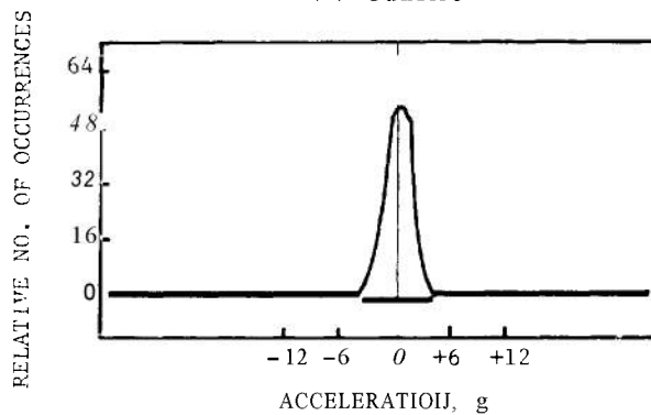
(B) No gunfire
