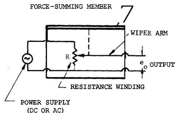
FIGURE 6-4. Potentiometric Accelerometer.
