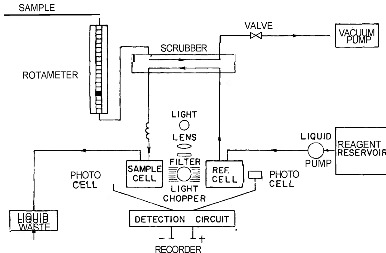
FIGURE 2-20. Schematic Diagram of a Typical Colorimetric Monitor
