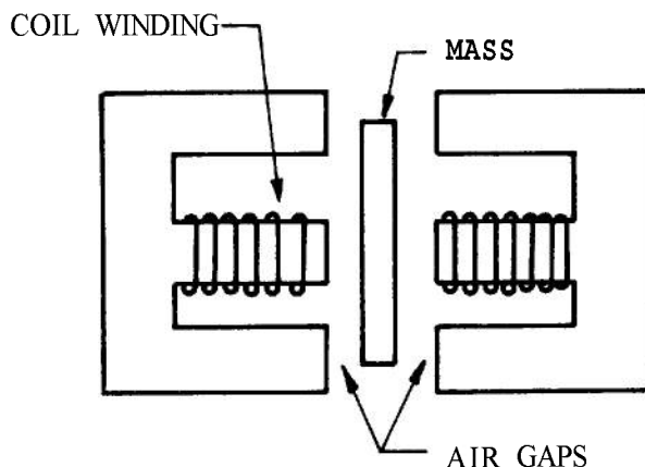
FIGURE 6-5. Inductive Accelerometer.
