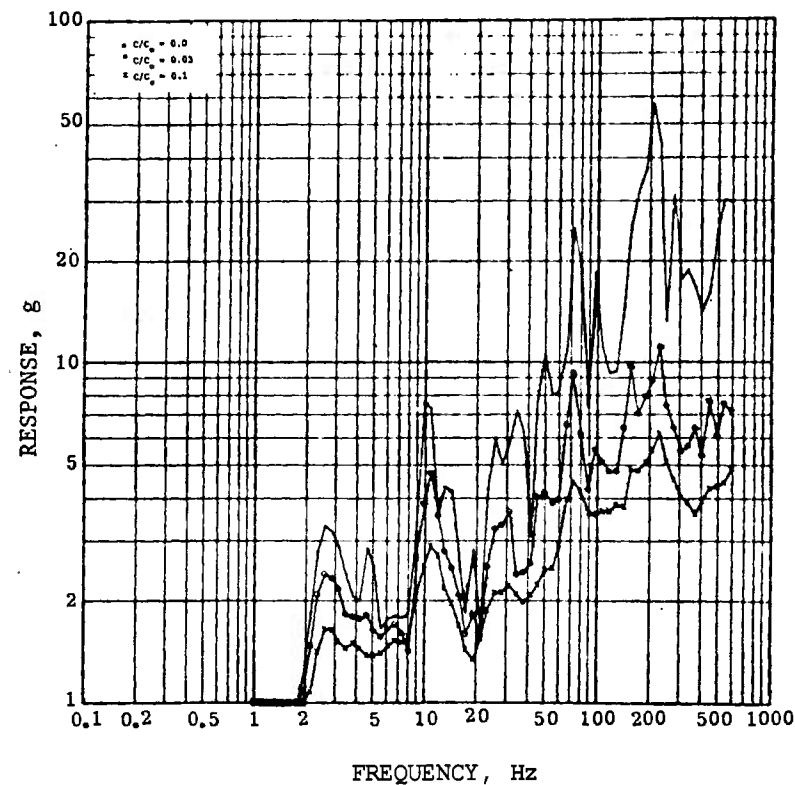
(B) Shock spectrum
