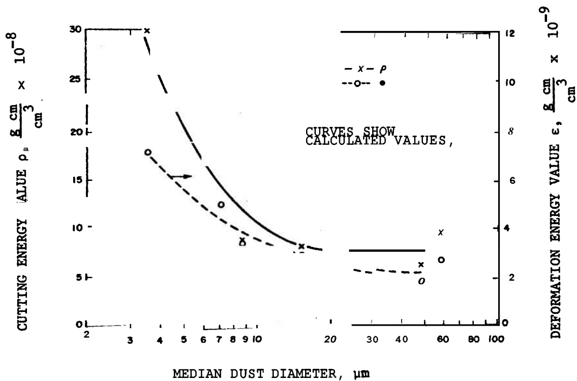
FIGURE 3-27. Effect of Dust Size on Energy (Data obtained with type 4140 steel at ambient temperature and a dust velocity of 800 ft s -1 ).
