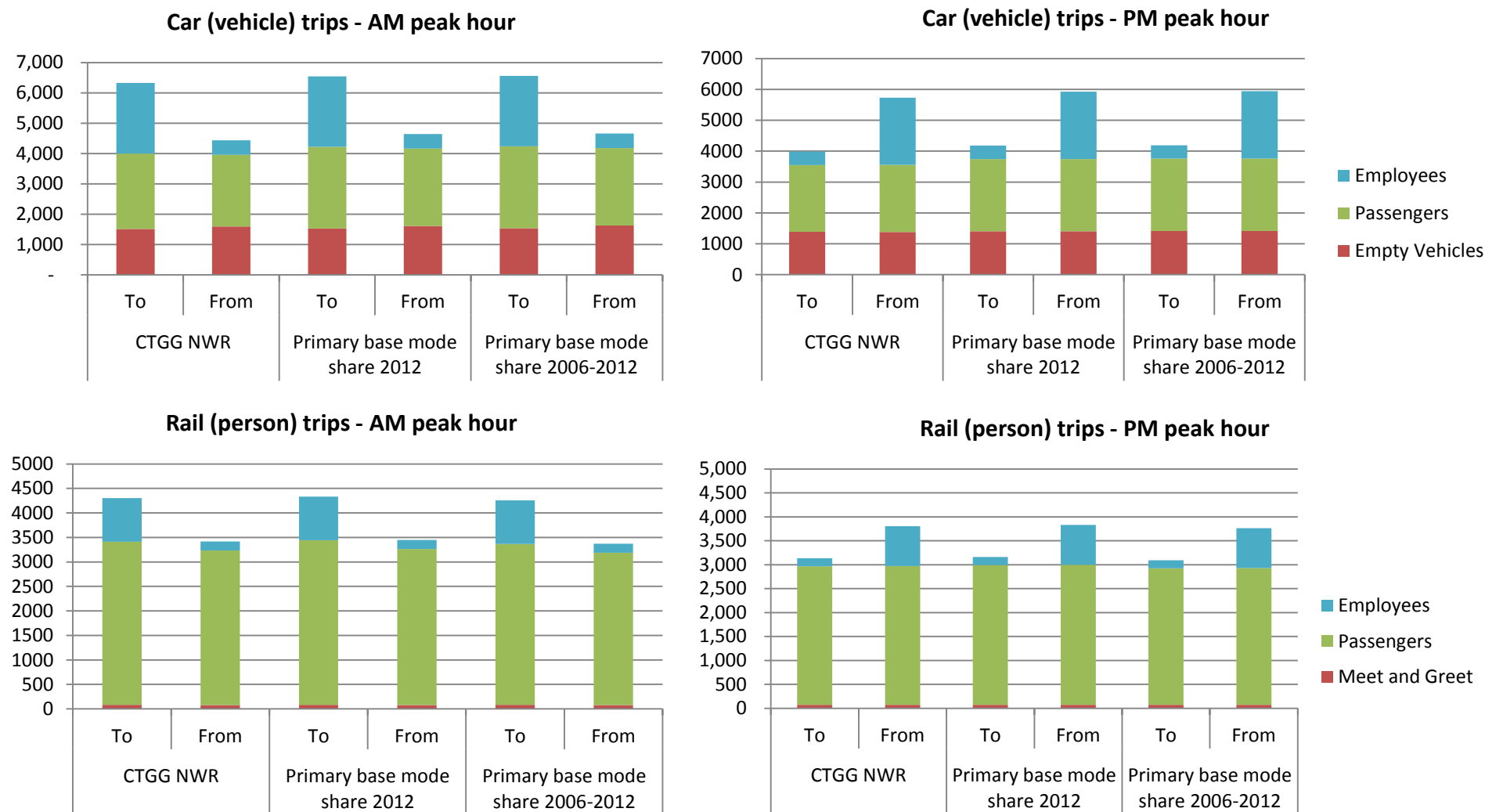
Figure 3-10: Impact of base mode share on car vehicle and rail passenger forecasts
