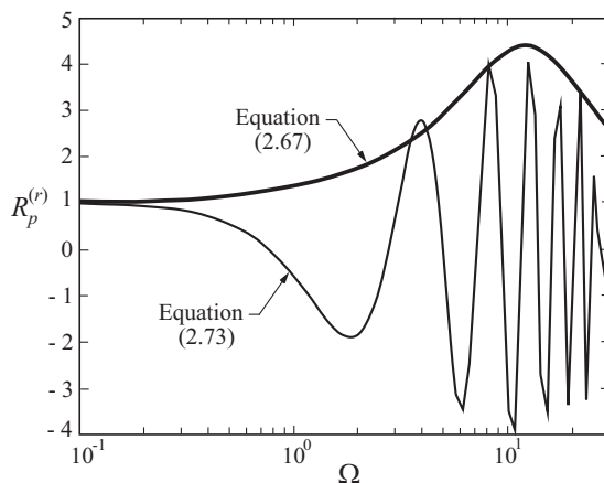
FIGURE 2.20. QSHOD response function with a time lag: thick line: QSHOD theory with n_s = 0 , A = 14 , B = 0.85 ; thin line: QSHOD model including a surface layer having first order (time lag) dynamics.
