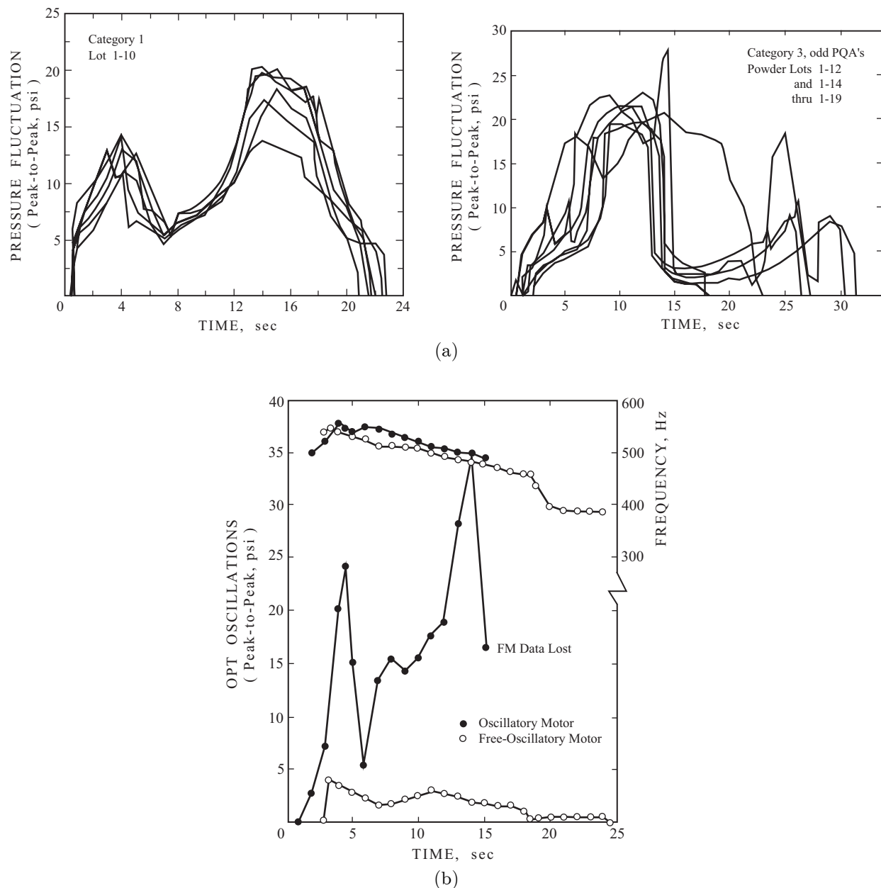
FIGURE 1.20. Frequencies and amplitudes of combustion instabilities in the Minuteman II, stage 3 motor: (a) change of behavior after Lot 1-10 (Fowler and Rosenthal 1971); (b) frequencies and amplitudes measured during static tests (Bergman and Jessen 1971).
