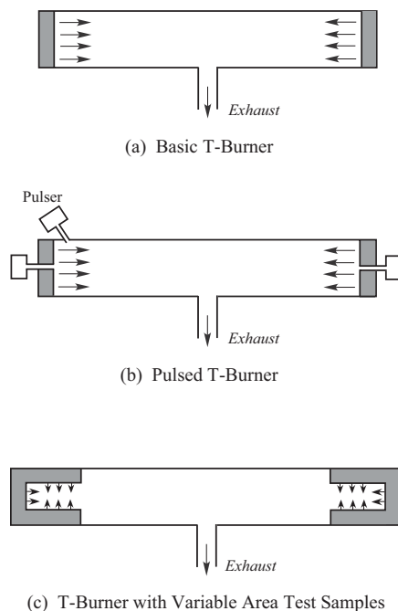
FIGURE 1.21. A sketch of the basic T-burner and two variants.
