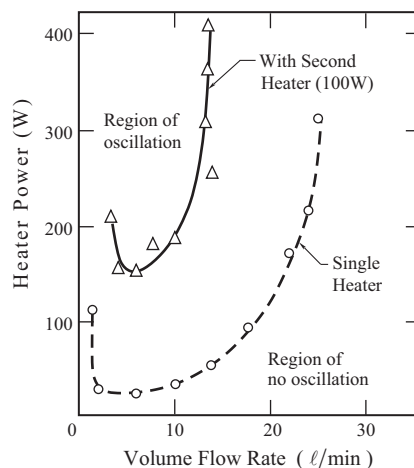
FIGURE 2.67. The effect of a second heater on the stability of oscillations; adapted from Figure 7 of Kalto and Sajiki (1977).
