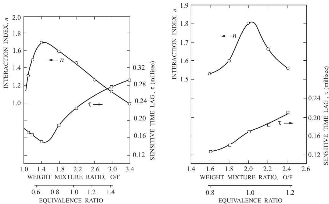
FIGURE 2.35. Early measurements of the time lag and pressure index in a gas rocket (Crocco, Grey and Harrije, 1960).
