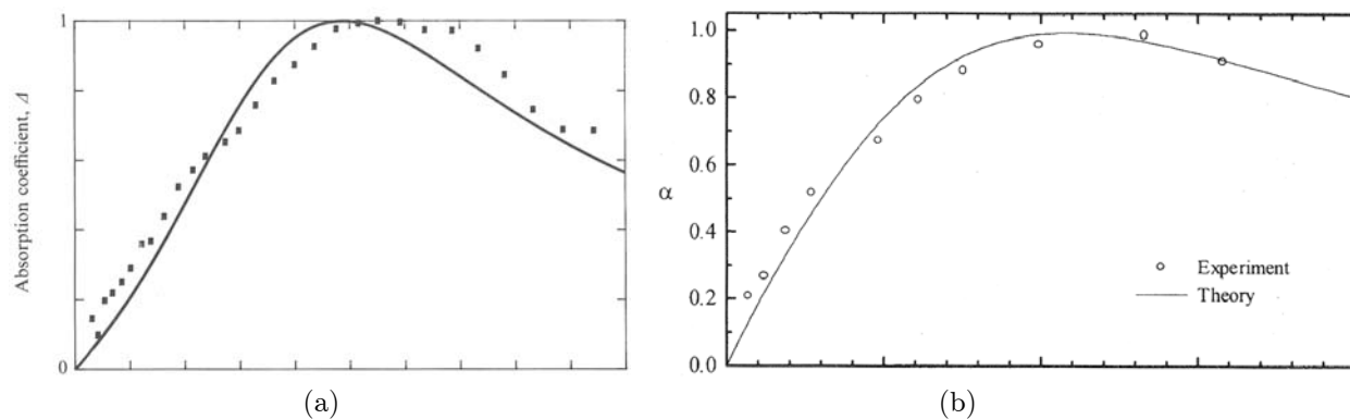
FIGURE 8.19. Absorption coefficient for a portion of acoustic liner (a) from Figure 7 of Hughes and Dowling (1990); (b) from Figure 7 of Jing and Sun (1998).
