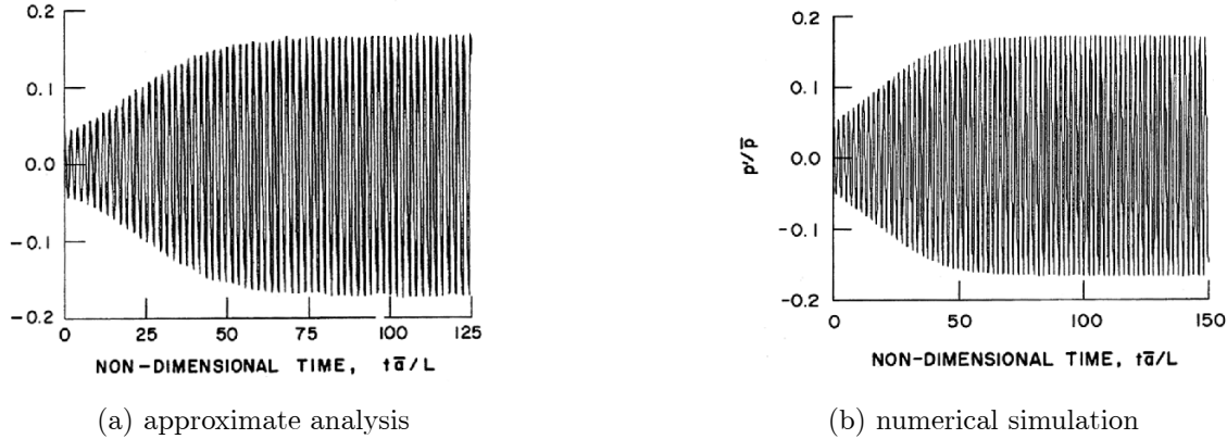
FIGURE 6.21. Growth of unstable motions according to (a) the approximate analysis; and (b) a numerical simulation of the same problem (Culick and Yang 1992).
