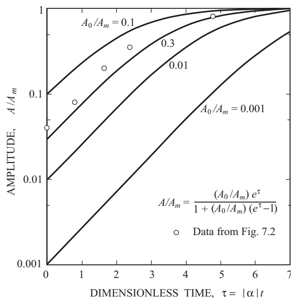
FIGURE 7.11. Nonlinear growth of oscillations for several values of the initial amplitude ratio A_0/A_m (Culick 1971).
