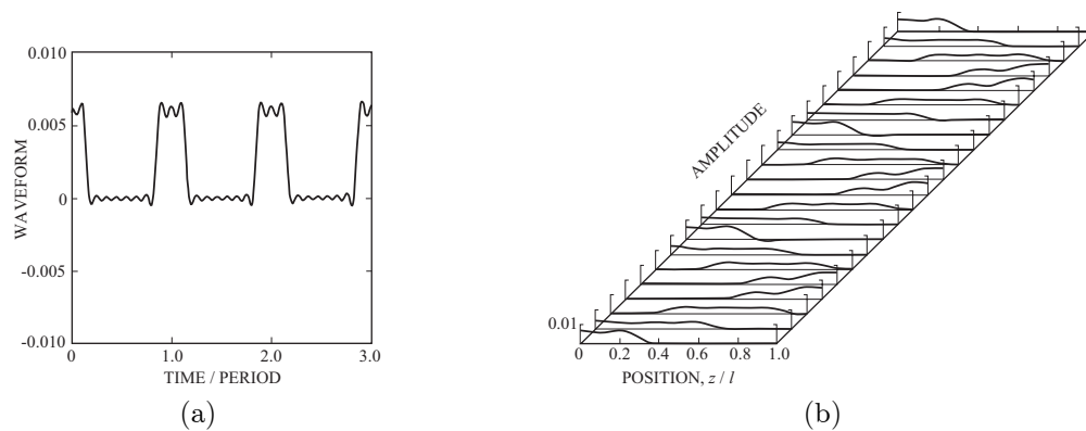
FIGURE 7.60. Propagation of a rectangular pulse without losses (10 modes): p'(z, 0) = 0.006p_0 ; 0 \leq z \leq 0.3L . (a) Waveform at z = 0 ; (b) pulse shapes for three cycles.
