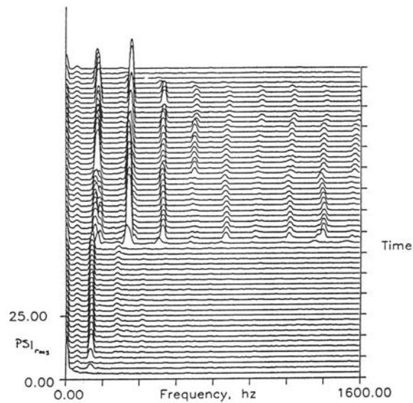
FIGURE 1.32. A waterfall plot showing an instability, having fundamental frequency < 200 Hz but with developing components at higher frequencies (Brown 1995).
