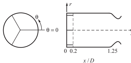
FIGURE 8.12. The combustion chamber with a three-bladed baffle analyzed by Wicker, Yoon and Yang (1995).
