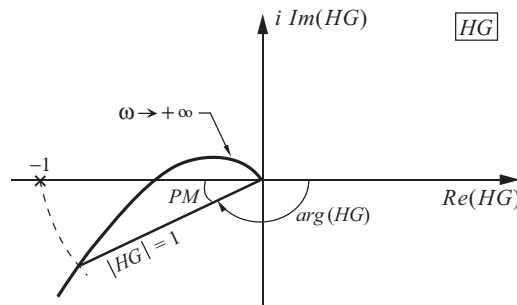
FIGURE G.13. The Nyquist plot for 'any' HG near |HG|_{\pi} , i.e., the magnitude of HG when the phase or arg of HG is \pi .
