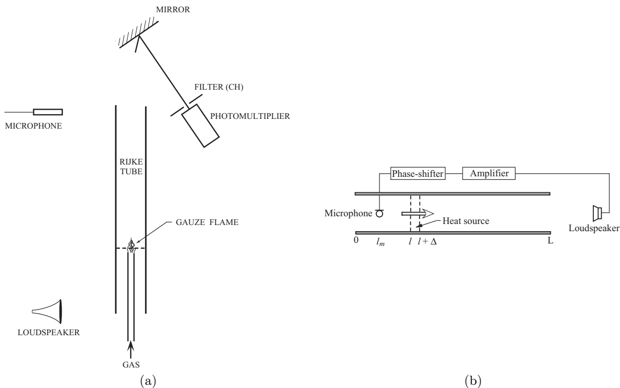
FIGURE 9.6. Feedback control of a Rijke tube by injection of acoustic waves. (a) Emitted radiation as the sensed variable (Dines 1983); (b) pressure as the sensed variable with air forced by a blower through the horizontal tube (Heckl 1985, 1986).
