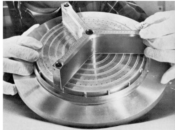
FIGURE 8.8. An injector with baffles and azimuthal slots (Harrje and Reardon 1972).
