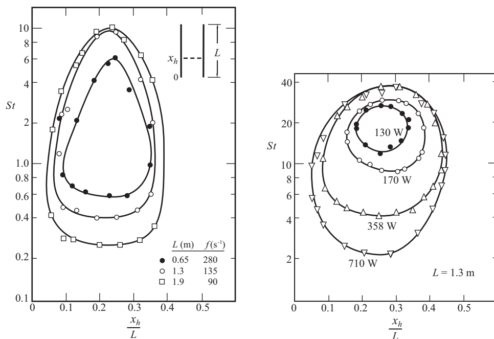
FIGURE 2.66. The effect of tube length and heater location on the generation of oscillations in a Rijke tube, St = \omega d/V ; (a) heater power input 500W, (b) L = 1.3 m (Marone and Tarakanovskii 1967).
