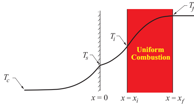
FIGURE 2.13. Sketch of the model of a solid propellant burning with uniform combustion in the gas phase.
