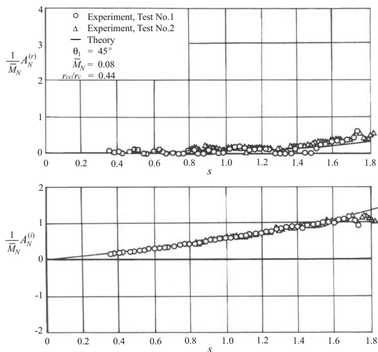
FIGURE 6.36. Comparison of the theoretical and experimental admittance results for nozzle 45-08-2.5, longitudinal modes (Bell 1972).
