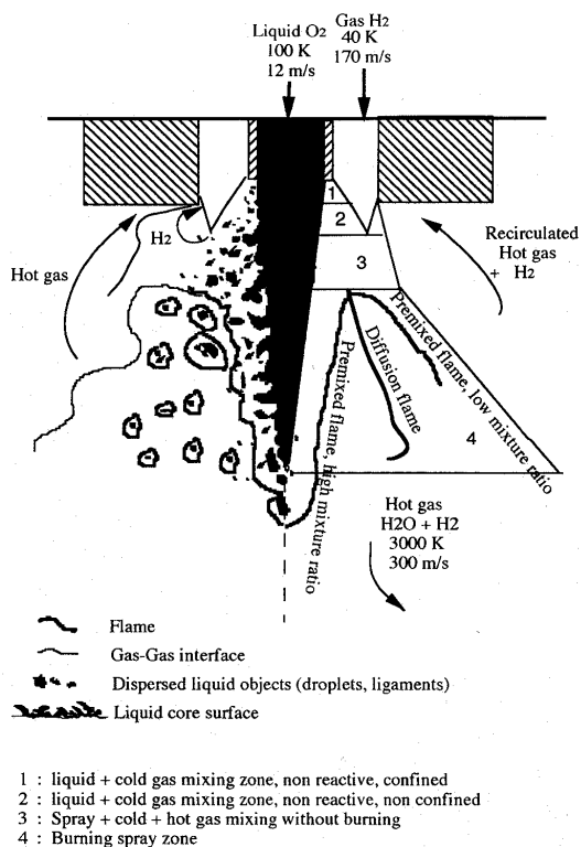
FIGURE 1.25. A sketch showing some of the processes taking place in a coaxial injector (Vingert et al. 1993).
