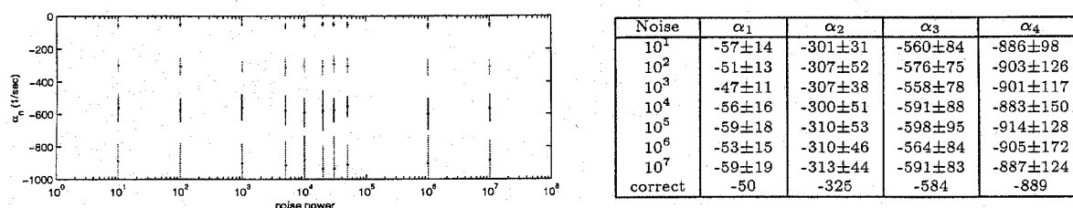
FIGURE 7.43. Values of decay rates (modal attenuation) found with Berg's method with multiplicative ( \xi_n ) noise.
