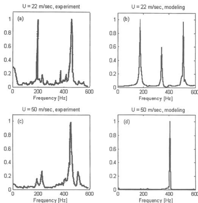
FIGURE 2.44. Normalized spectra of pressure fluctuations at the step of Figure 2.43 for two mean flow velocities at the dump plane. (a), (c) experimental results (Smith 1985); (b), (d) results from the kicked oscillator model.
