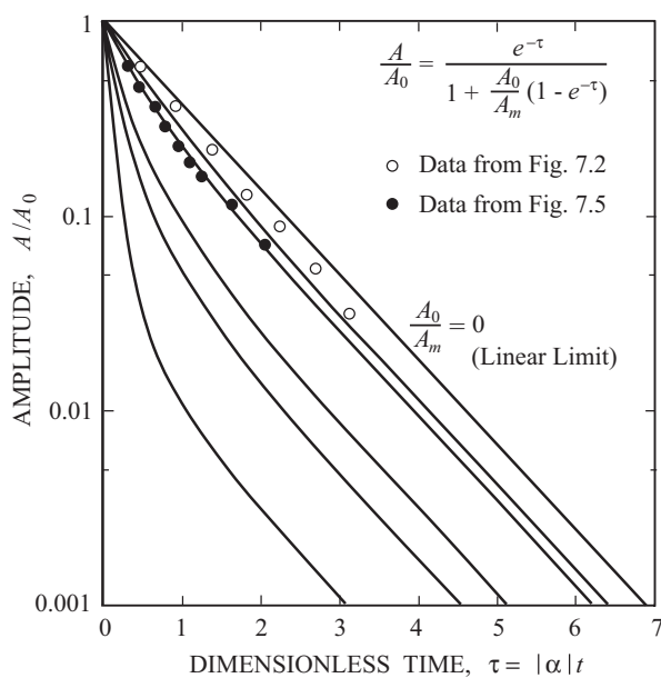
FIGURE 7.12. Nonlinear decay of oscillations for several values of the initial amplitude ratio A_0/A_m (Culick 1971).
