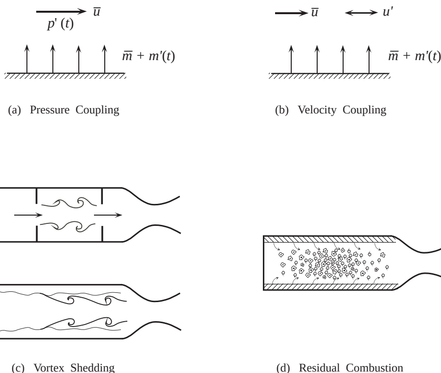
FIGURE 2.1. The four possible mechanisms for combustion instabilities in solid propellant rockets.
