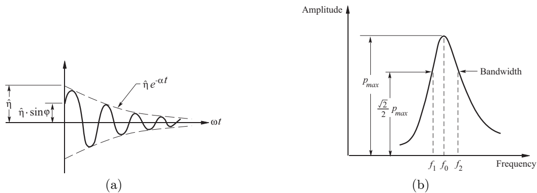
FIGURE 8.14. Two methods for measuring the damping factor: (a) decay rate, \alpha ; (b) bandwidth.
