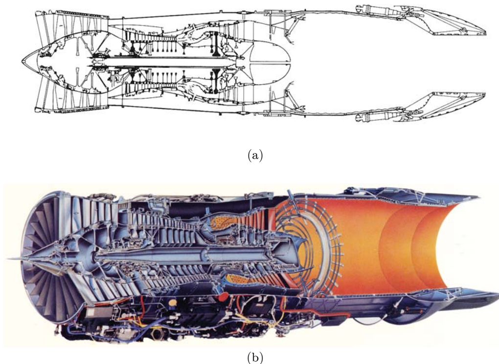
FIGURE 2.51. Two examples of aircraft gas turbine engines with thrust augmentation (a) General Electric F110 engine (taken from Jane's All The World's Aircraft , 1988–1989); (b) Pratt and Whitney F100 engine (taken from Pratt and Whitney advertising material).
