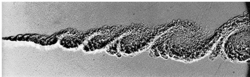
FIGURE 2.37. Large-scale coherent structures in a mixing layer at 8 atmospheres in flow past a splitter plate: upper stream ( v_1 = 10 m/s) is He; lower stream is N_2 , with \rho_2 v_2^2 = \rho_1 v_1^2 . (Brown and Roshko 1974).
