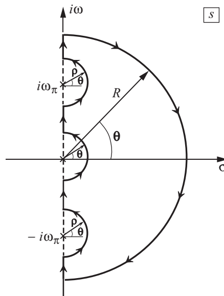
FIGURE G.3. Indentations around poles on the imaginary axis. Poles and zeros within the contour are suppressed.
