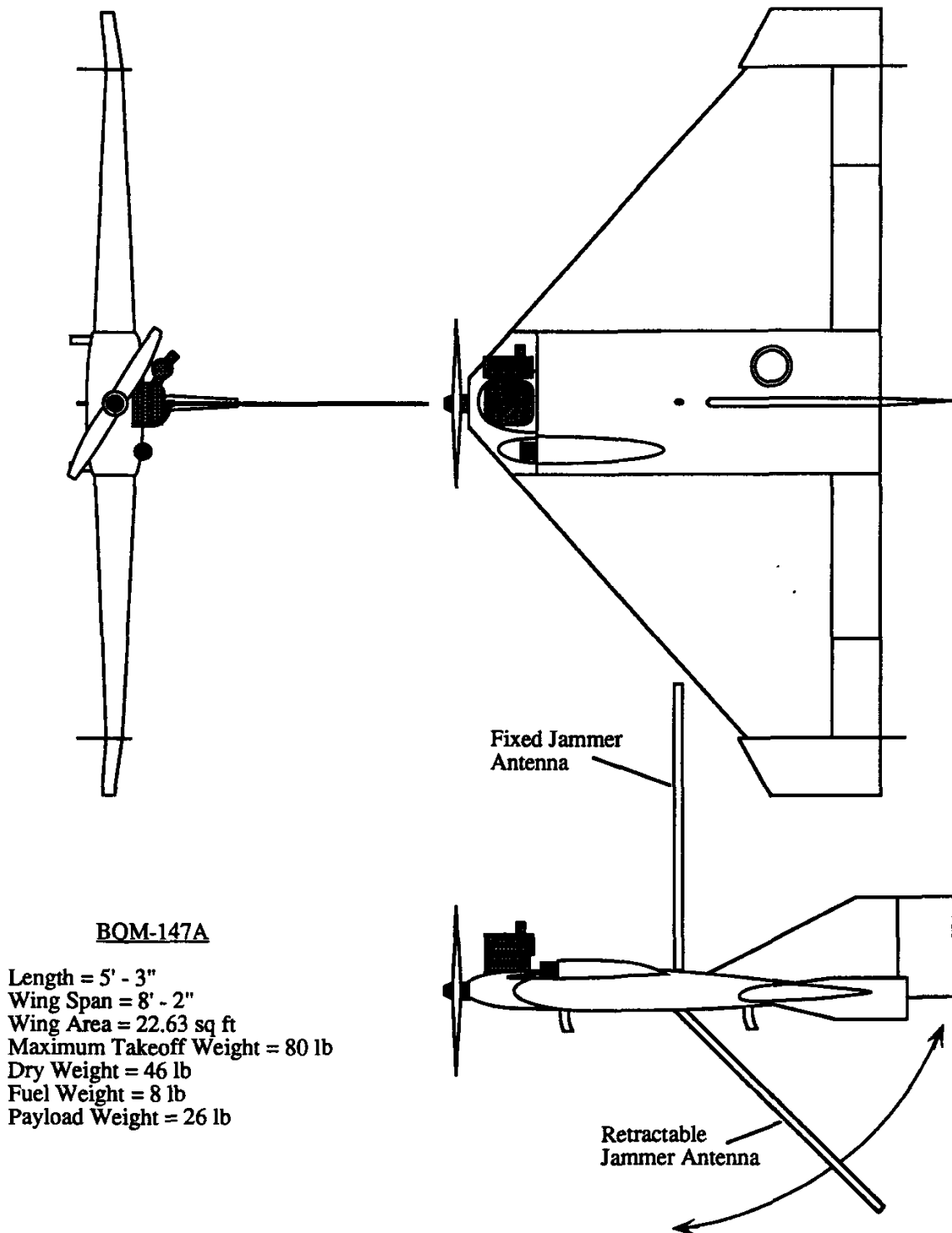
Figure 1 THREE-VIEW DRAWING
