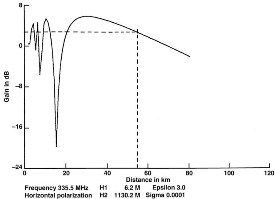
Figure 19B.A-1. Multipath Gain of the Reflecting Ground Calculated after Reference 19B-1.
