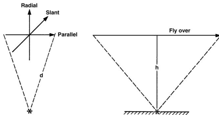
Figure 19B-4. Straight Flight Test Trajectories for ARP Measurement, d = Distance; h = Altitude.
