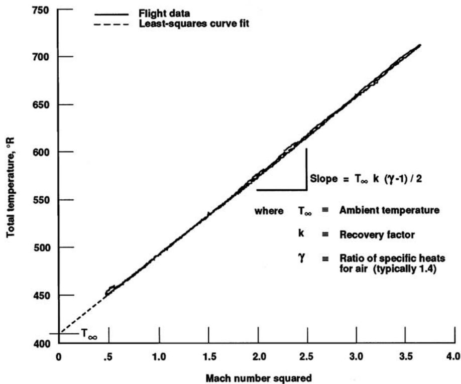
Figure 11-4. Total Temperature Calibration [11-12].
