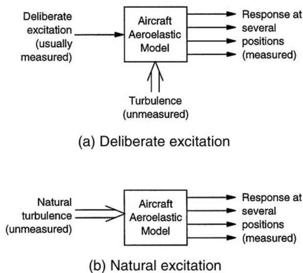
Figure 14-3. Identification of Dynamic Characteristics.
