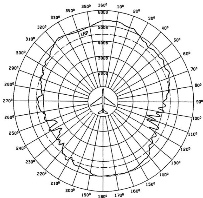
Figure 19B.A-2. Radiation Pattern of a Glide Slope Antenna, Frequency 335.5 MHz, Polarization Horizontal, Test Flight Left Circle, LRP 44 dB.
