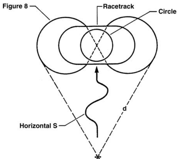
Figure 19B-5. Curved Flight Test Trajectories for ARP Measurement, Fixed Altitude d = Distance.
