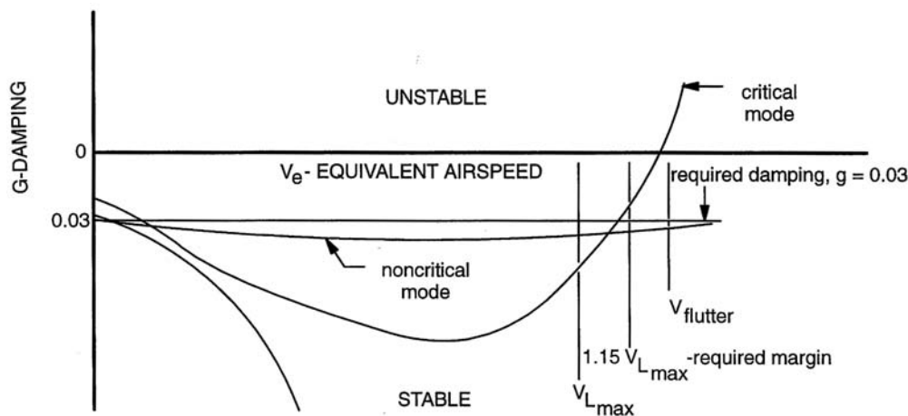
Figure 14-2b. Required Damping.
