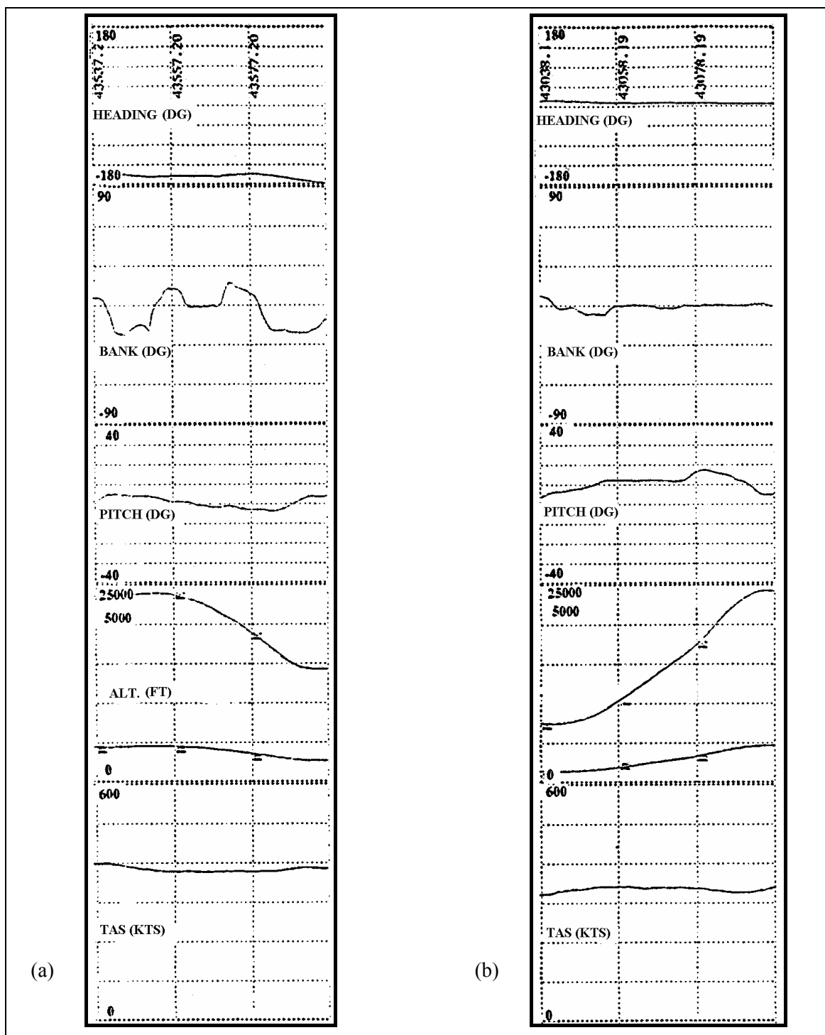
Figure D-7: Altitude Variations Without Satellite Signal Losses During Low Bank Manoeuvres (a) and in Vertical Flight (b).
