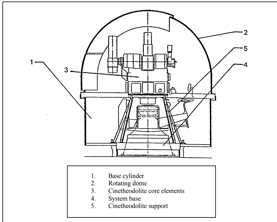
Figure 2-3: Cinetheodolite System.
