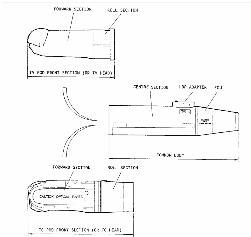
Figure 6-3: CLDP TV and IR Configurations.
