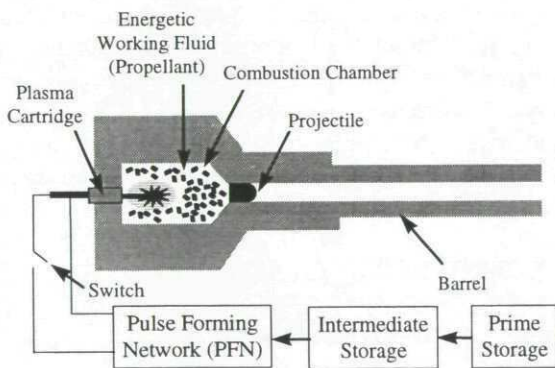
Figure 2 Schematic of an electrothermal-chemical gun
