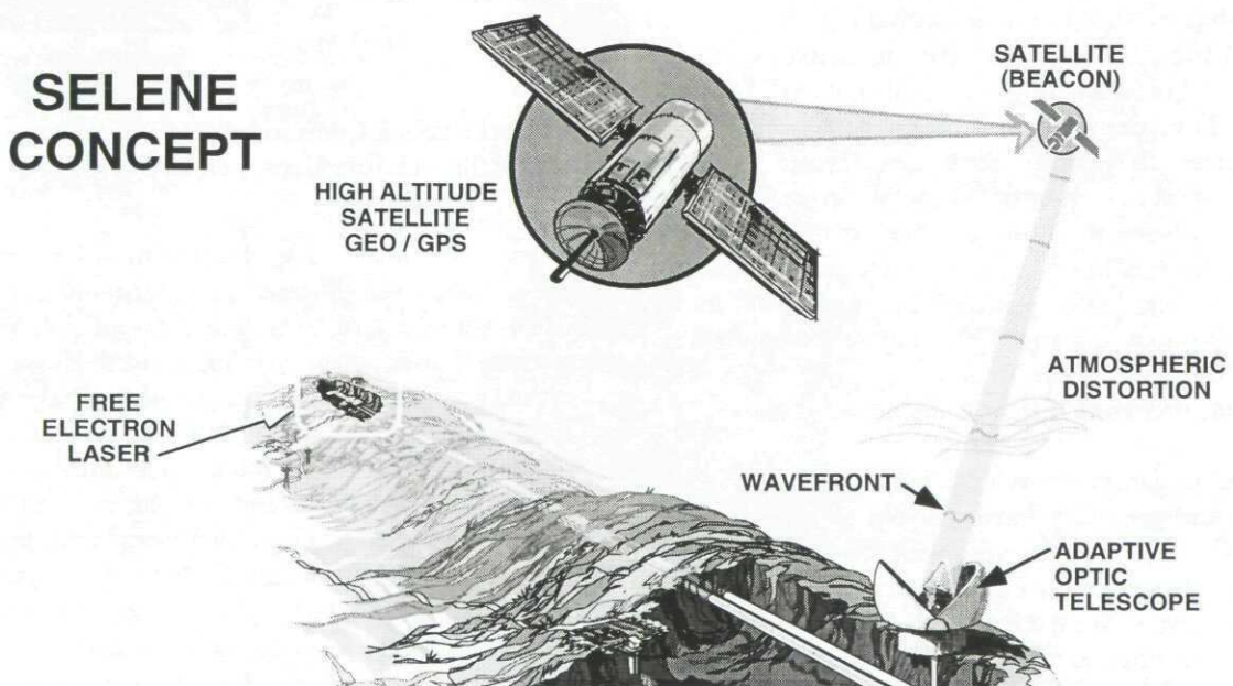
Figure 3 Laser Power Beaming Facility - SELENE System Concept
