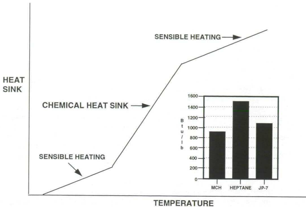
Figure 6 Endothermic Fuel Heat Sink Potential
