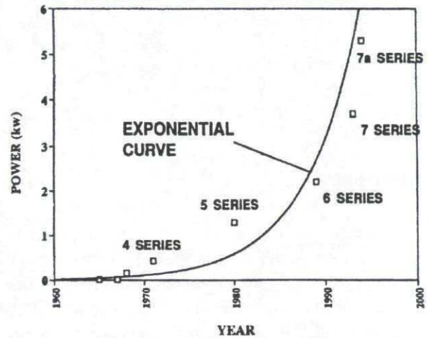
Figure 1 INTELSAT Telecommunication Satellite Power Growth
