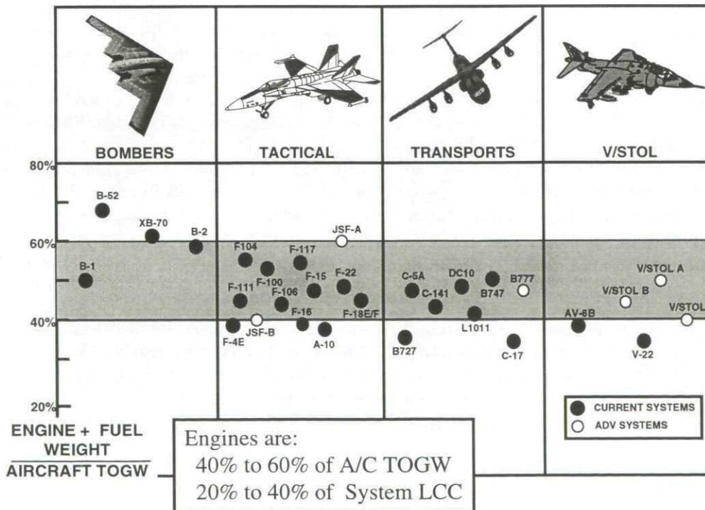
Figure 1. Turbine Engine Technology Impact
