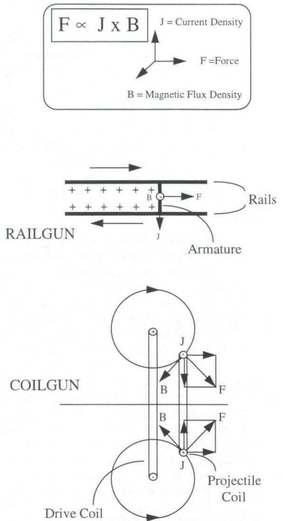
Figure 1: Generic geometries, magnetic fields, and forces in the rail gun and coil gun
