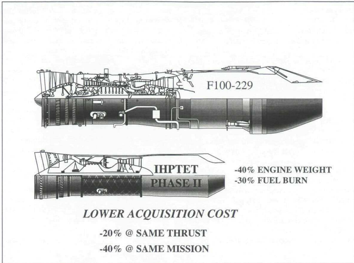
Figure 4. Revolutionary Advancement in Turbine engine Design
