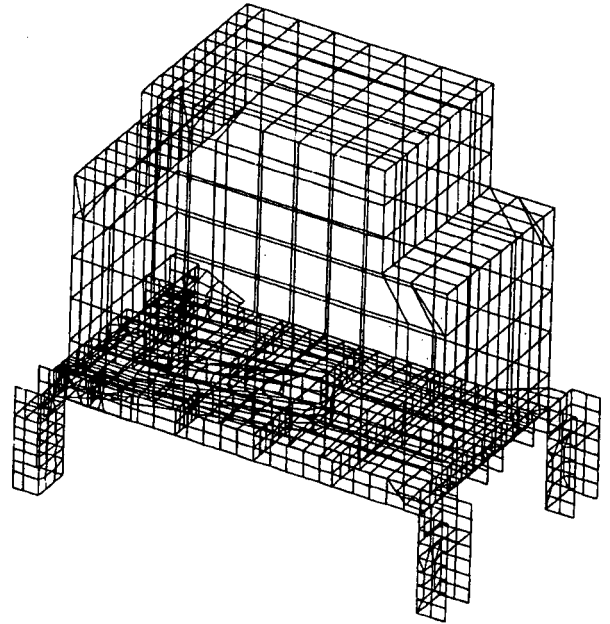
Fig.: 34 Finite Element Model IMU and Tray
