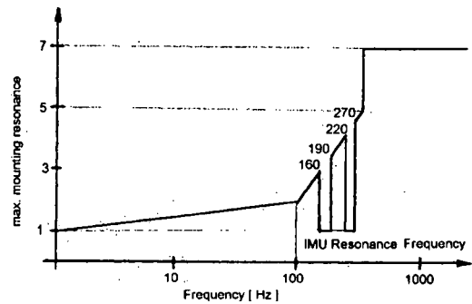
Fig.: 31 Special Equipment Vibration Limitations
