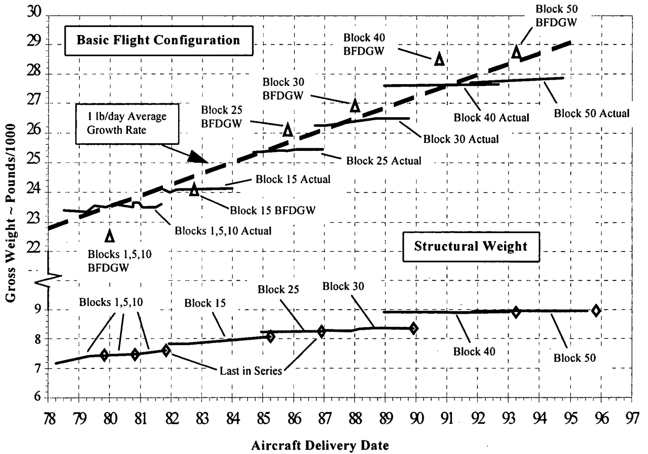
Figure 1 - F-16 Weight Growth
