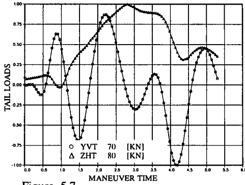
Figure 5.7 EXTREME OPERATIONAL LOADS HIGH-G-TURN
