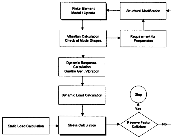
Fig.: 32 Optimization Process Tray Design
