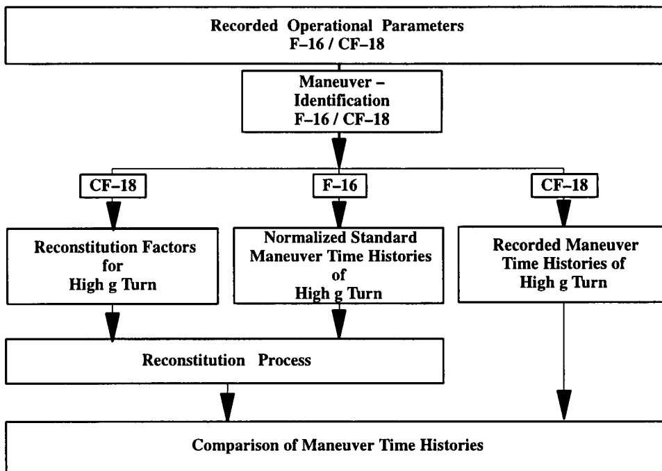
Figure 15 Reconstitution Process
