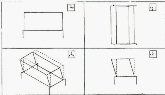
Fig.: 42a Measured Mode Shape; f = 51.66 Hz
