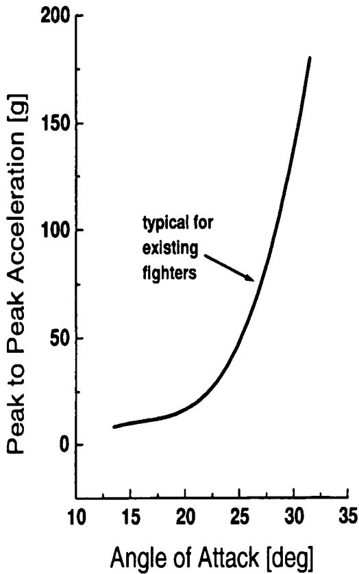
Fig.: 16 Fin Vibration Characteristics
