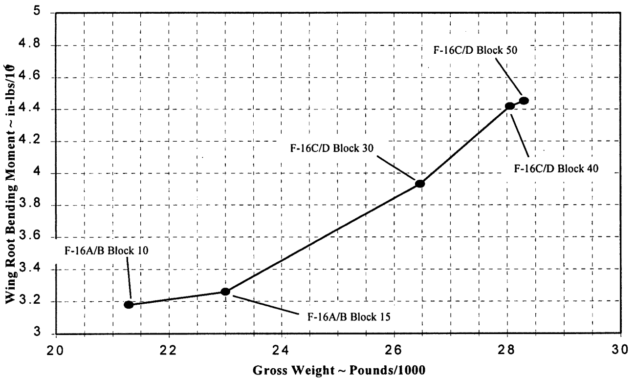
Figure 2 - Growth in Wing Load
