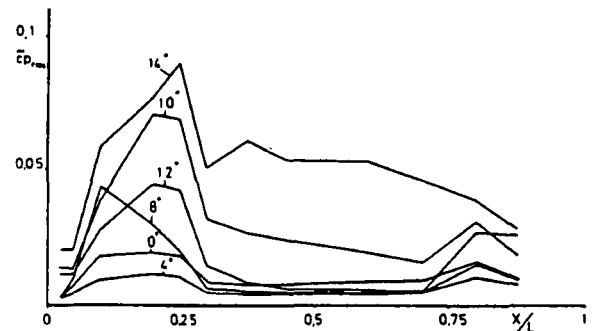
Fig.: 11 Fluctuating Pressure RMS Values
