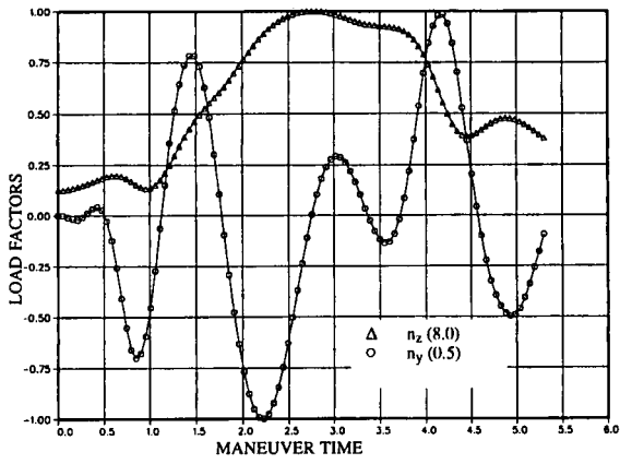
Figure 5.1 EXTREME OPERATIONAL PARAMETERS HIGH-G-TURN
