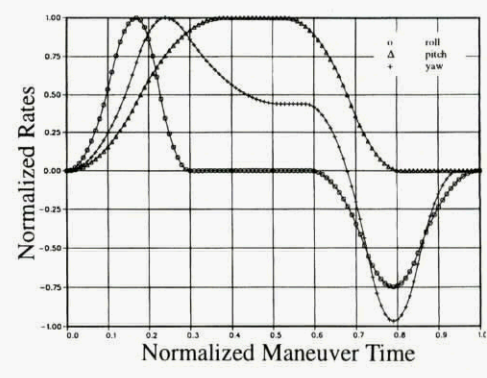
Figure 13 Standard Maneuver Traces
