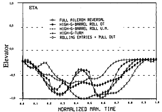
Figure 5.11 EXTREME OPERATIONAL CONTROL DEFLECTIONS OPERATIONAL MANEUVERS
