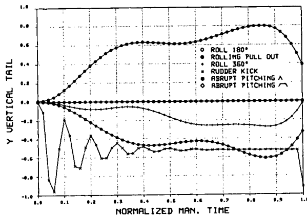
Figure 6.6 STRUCTURAL LOADS MIL-MANEUVERS
