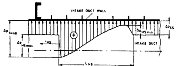
SUPERSONIC INTAKE / DUCT CASE (BURSTING CASE) SQUARE SHAPED DUCTS WITH FLAT PANELS. FUEL ON THE OTHER SIDE OF THE WALL CAUSES ATTENUATION OF THE TOTAL DIFFERENTIAL PRESSURE ON THE DUCT SKIN
