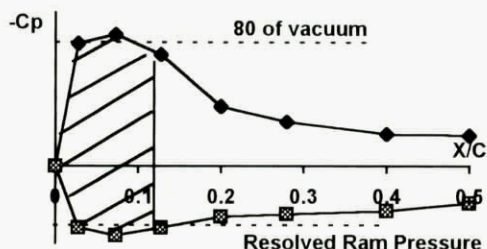
Figure 20. Pressure Distribution for Leading Edge Design Loads
