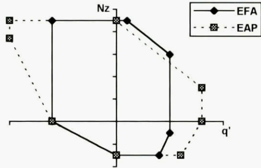
Figure 4. Comparison of EAP and EFA Design Parameters
