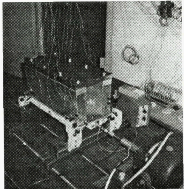
Fig.: 41 Ground Vibration Test Set Up
