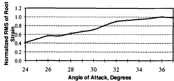
Figure 7. Normalized RMS of Root Strain on 1/6-Scale Vertical Tail
