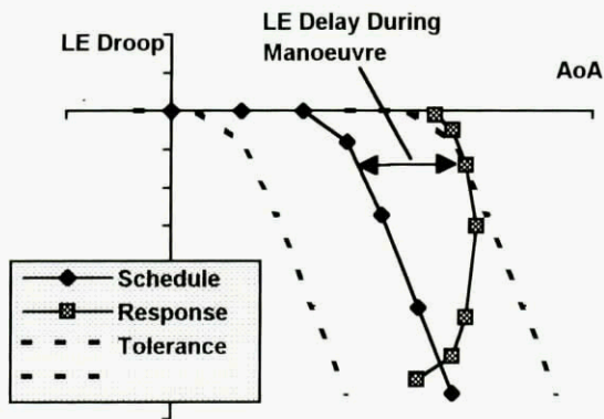
Figure 21. LE Deflections During Pitch Manoeuvres
