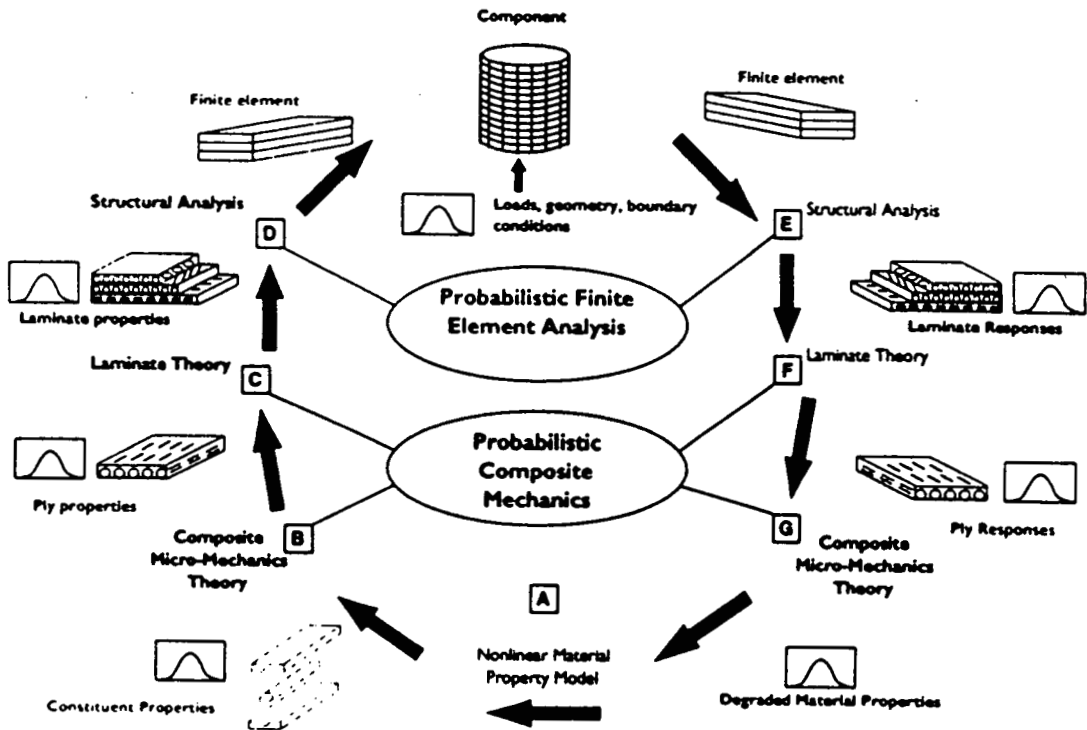
Figure 2 - Integrated Probabilistic Assessment of Composite Structures (IPACS)
