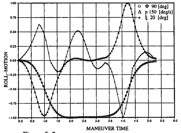
Figure 5.2 EXTREME OPERATIONAL PARAMETERS HIGH-G-TURN
