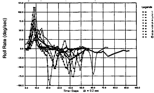
Figure 4 Unified Roll Directions
