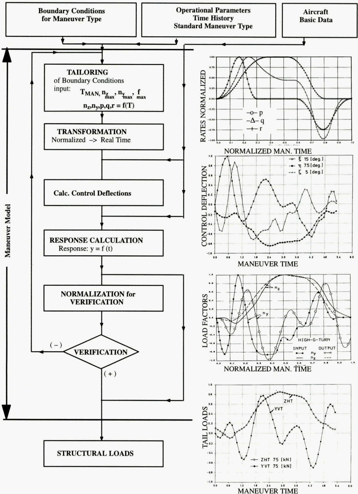
Figure 3. Procedure of the Maneuver Model
