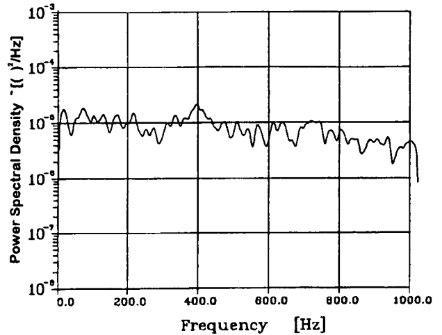
Fig.: 14 Power Spectral Density of Unsteady Pressure; Mach=0.9; \alpha=28^\circ ; Clean Configuration
