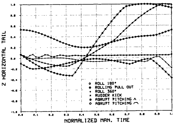
Figure 6.5 STRUCTURAL LOADS MIL-MANEUVERS
