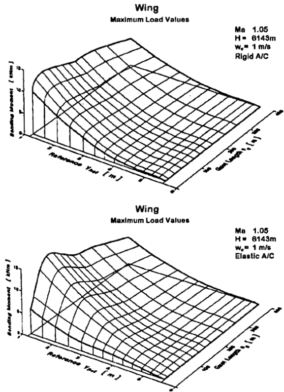
Fig.: 6 Design Gust Calculation: Wing Bending Moment
