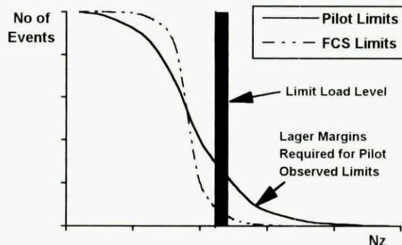
Figure 3. Effect of FCS On Load Criticalities
