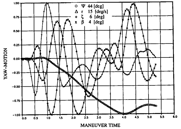
Figure 5.4 EXTREME OPERATIONAL PARAMETERS HIGH-G-TURN
