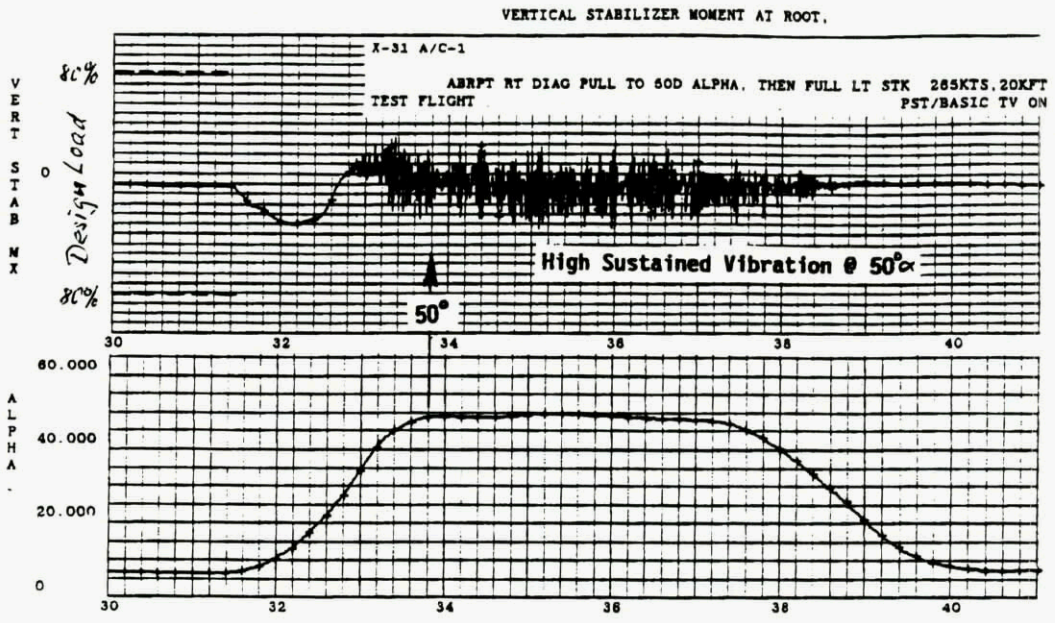
Fig. 10 X-31 - Diagonal Pull to 50° Alpha Fin Buffet - High Sustained Vibration
