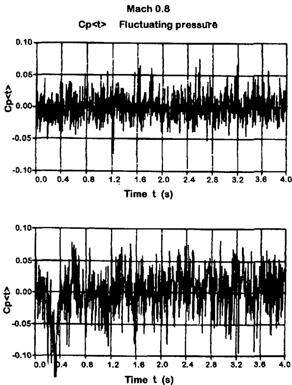
Fig.: 9 Fluctuating Pressures
