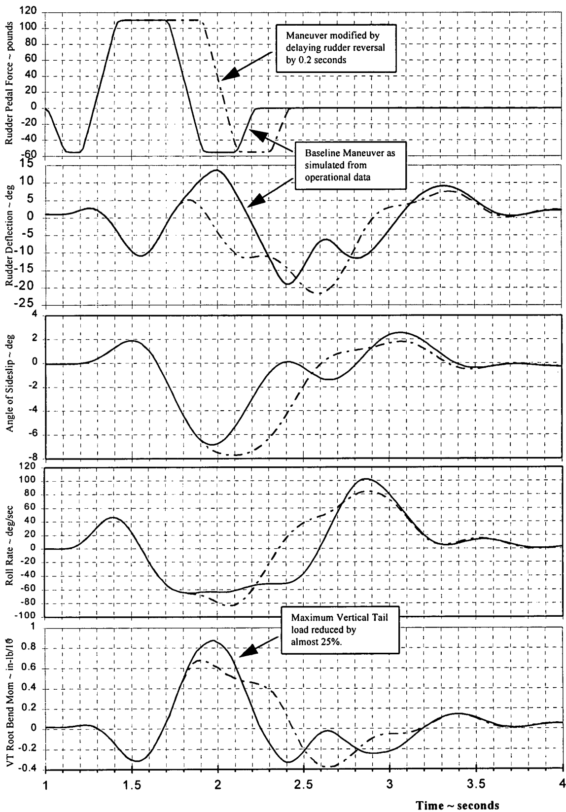
Figure 5 - Simulated Operational Rudder Reversal
