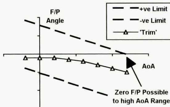
Figure 14. Foreplane Load Boundaries
