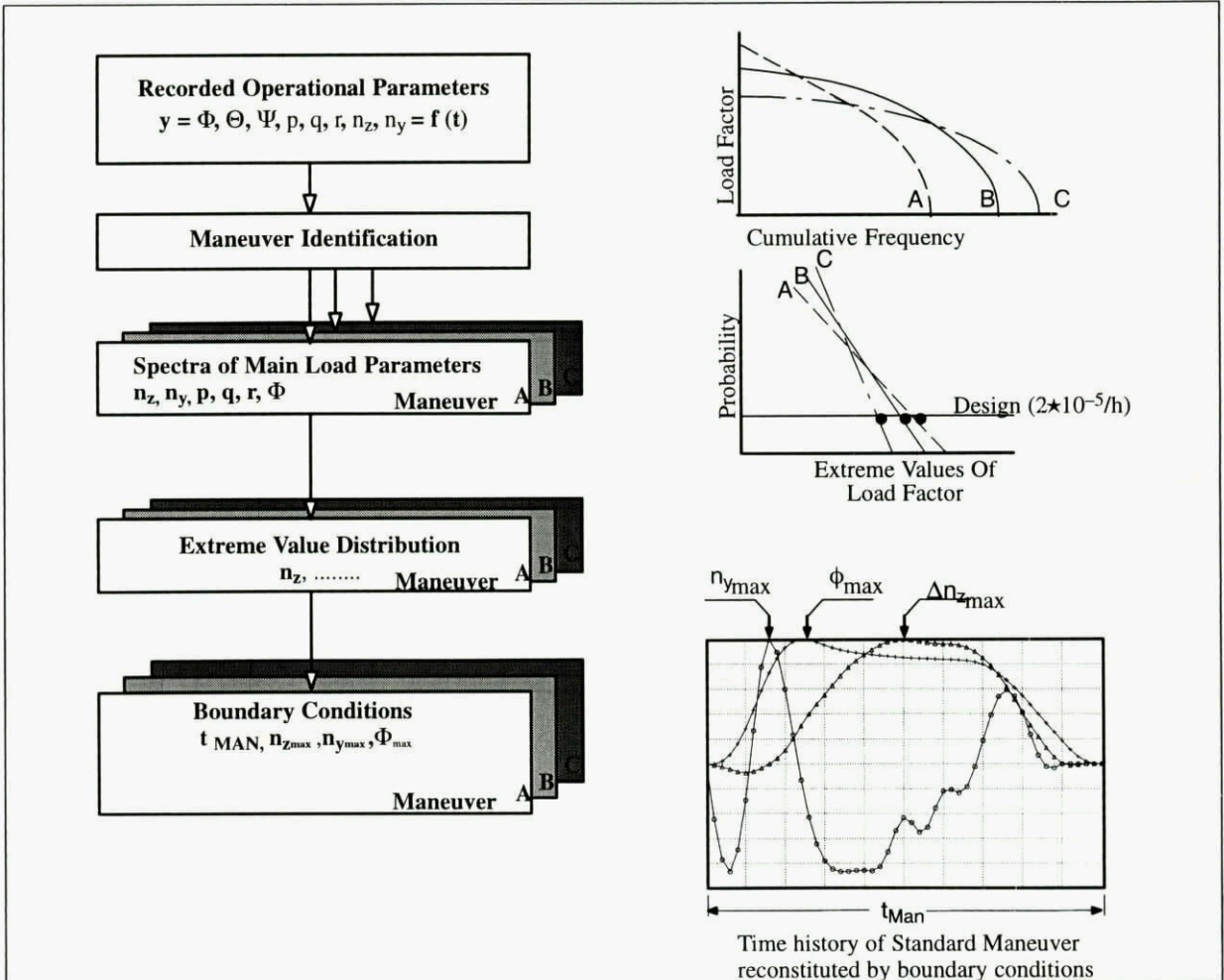
Figure 4 Boundary Conditions for Design Maneuvers
