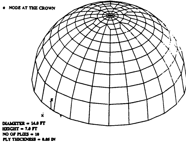
Figure 10 - Radome Structure Finite Element Model
