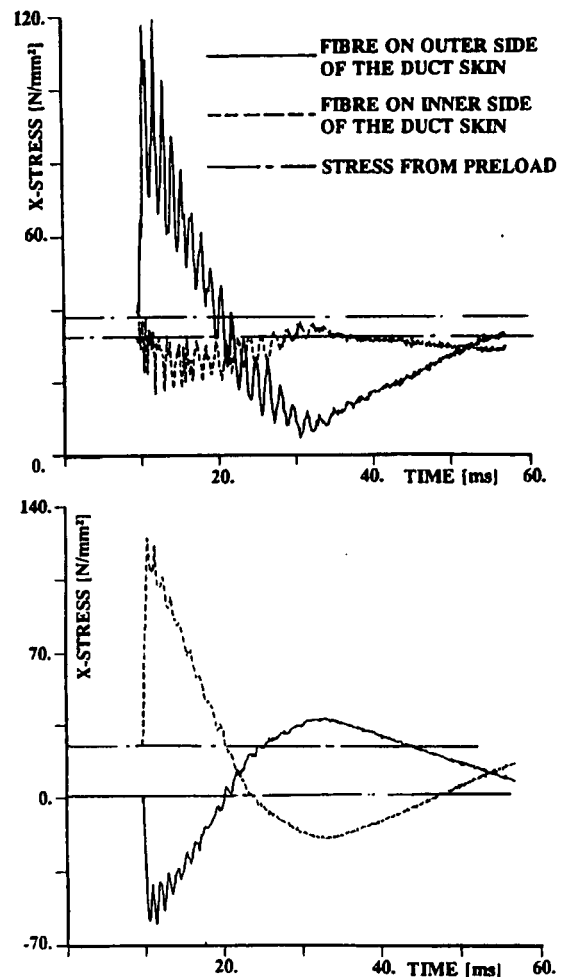
Fig.: 25 Typical Response of Different Duct Skin Elements on Hammer Shock Excitation
