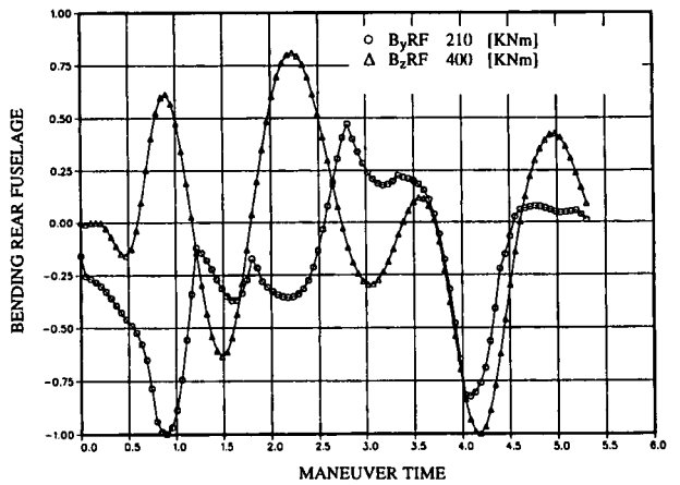
Figure 5.6 EXTREME OPERATIONAL LOADS HIGH-G-TURN
