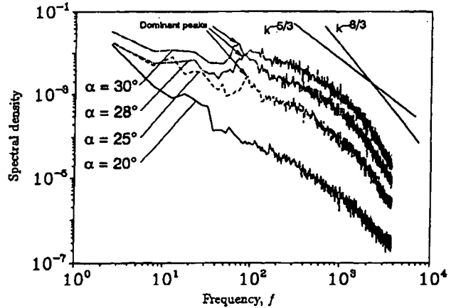
Fig.: 13 Spectral Density of Lateral Velocity
