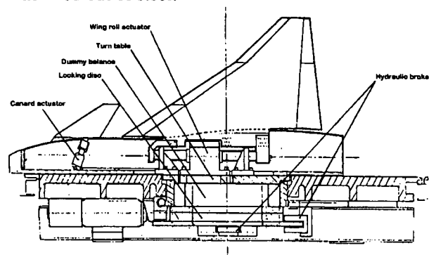
Fig.: 7 Windtunnel Model Set Up
