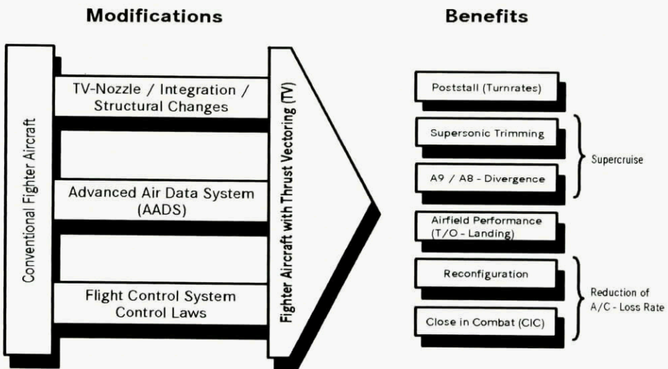
Fig. 12 EF2000 with TVNS - Modifications and Benefits
