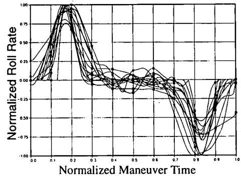
Figure 9 Comparison of Normalized Roll Rate Traces
