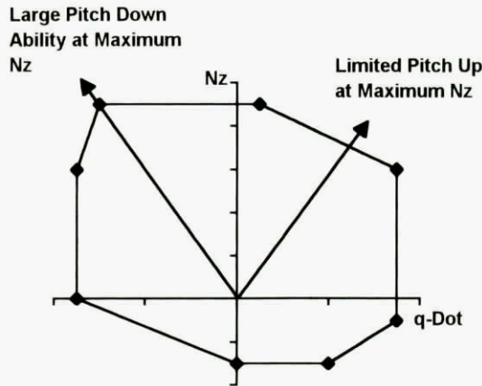
Figure 15. Normal and Pitch Acceleration Combinations
