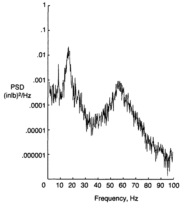
Figure 12(a). PSD of Tail Root Bending Moment, 1/6-Scale Model, \alpha = 20^\circ , q=14 psf
