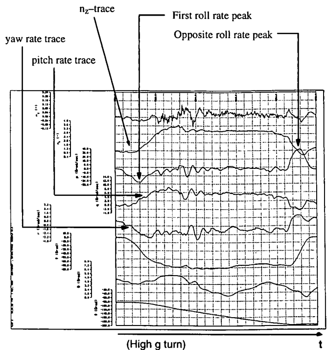
Figure 3 Identified Time Histories of Correlated Operational Parameters
