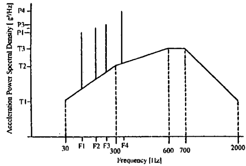
Fig. 30: Gunfire Induced Vibration Test Spectrum
