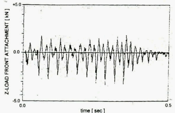
Fig.: 44 Time History from Gun Rig Test (Front gun attachment)
