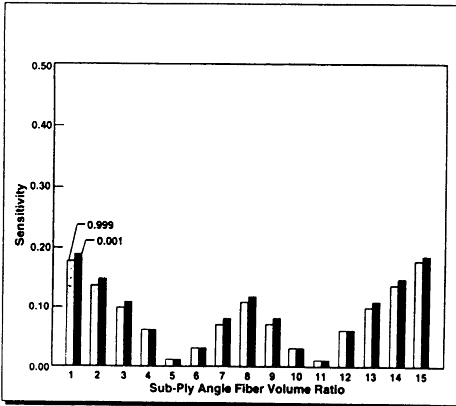
Figure 8 - Tensile Strength (AS4/3501-6 Graphite/Epoxy).
