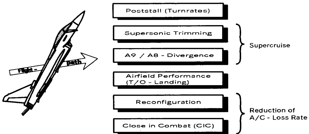
Fig. 1 Thrust Vectoring System (TVS) Benefits
