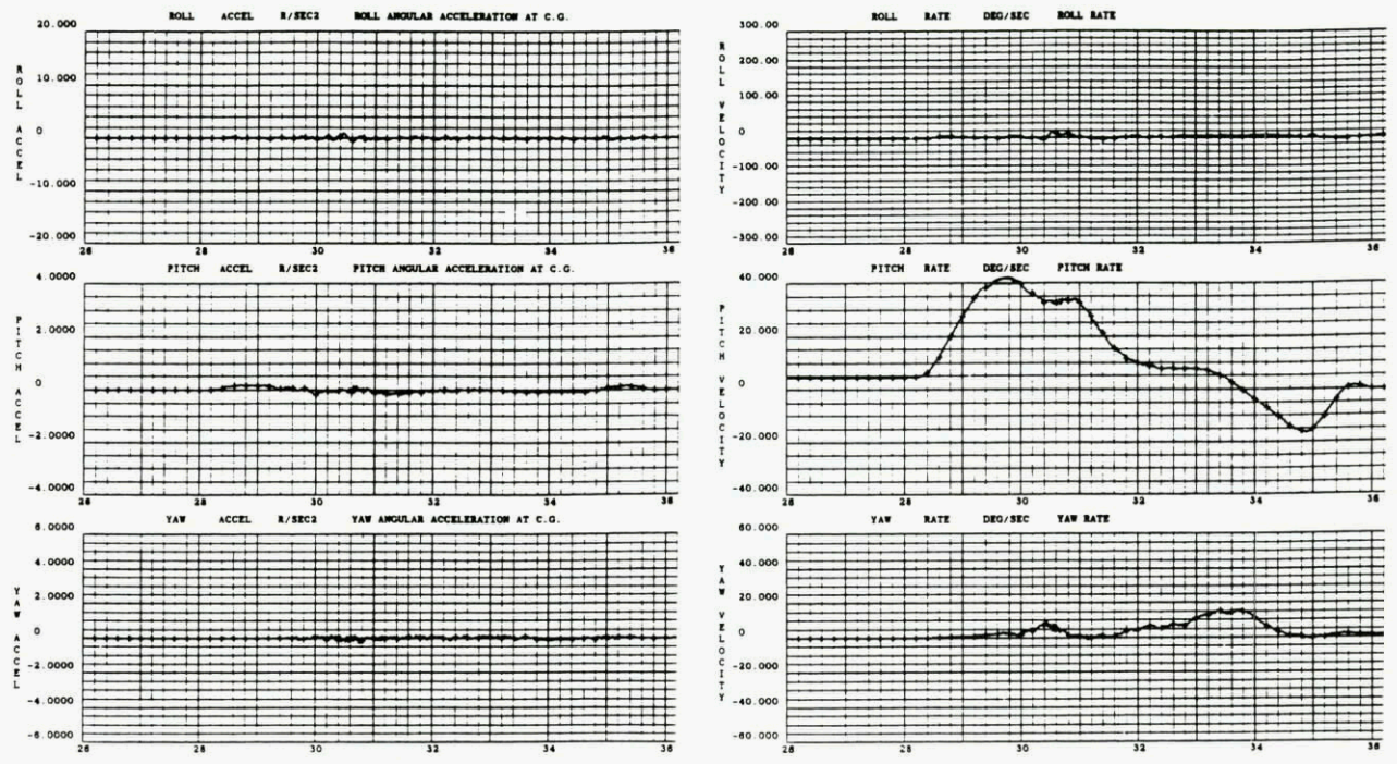
Fig. 8 X-31 - 6g abrupt WUT (Split -S) to 70° Alpha Roll/Pitch/Yaw Acceleration at c.g. v. time Fig. 9 X-31 - 6g abrupt WUT (Split -S) to 70° Alpha Roll/Pitch/Yaw Rate (p, q, r) versus time
