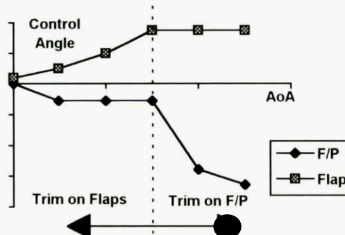
Figure 13. Flap and Foreplane Subsonic Trim Settings
