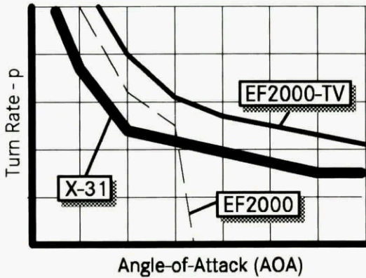
Fig. 13 EF2000 with TVNS - PST Performance
