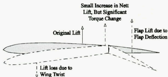
Figure 9. Lift Distribution During High Speed Rolling
