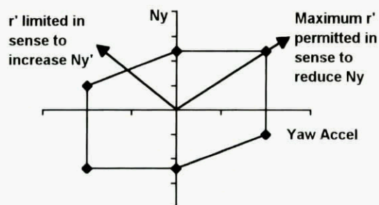
Figure 11. Combination of Lateral and Yaw Accelerations
