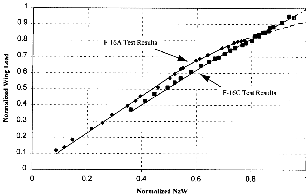
Figure 6 - Flight Measured F-16 Wing Load Trends
