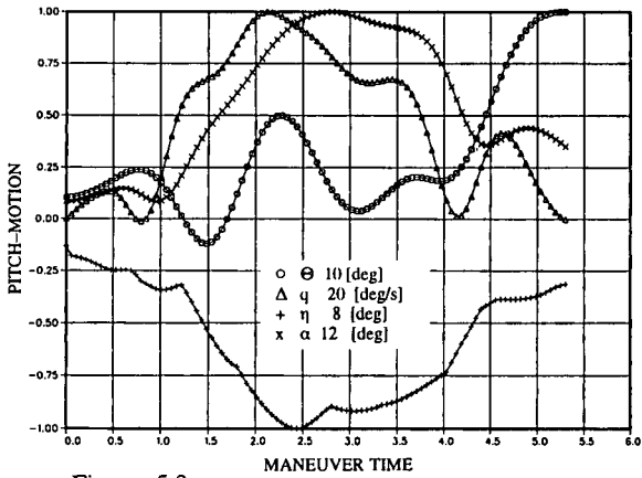
Figure 5.3 EXTREME OPERATIONAL PARAMETERS HIGH-G-TURN
