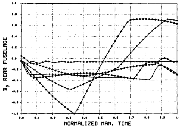
Figure 6.3 STRUCTURAL LOADS MIL-MANEUVERS
