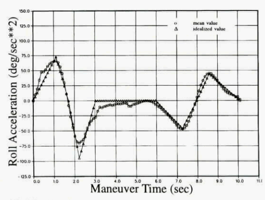
Figure 12 Idealization
