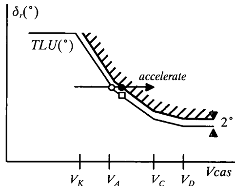
Fig. 6 Limitation of rudder deflection ( \delta_r ) by TLU, solid line is 2^\circ jamming detection threshold. ○ occurrence of TLU jamming, ● detection of TLU jamming □ commanded TLU value
