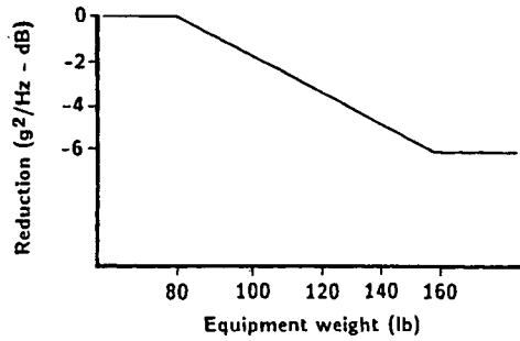
Fig.: 29 Vibration Reduction Factor
