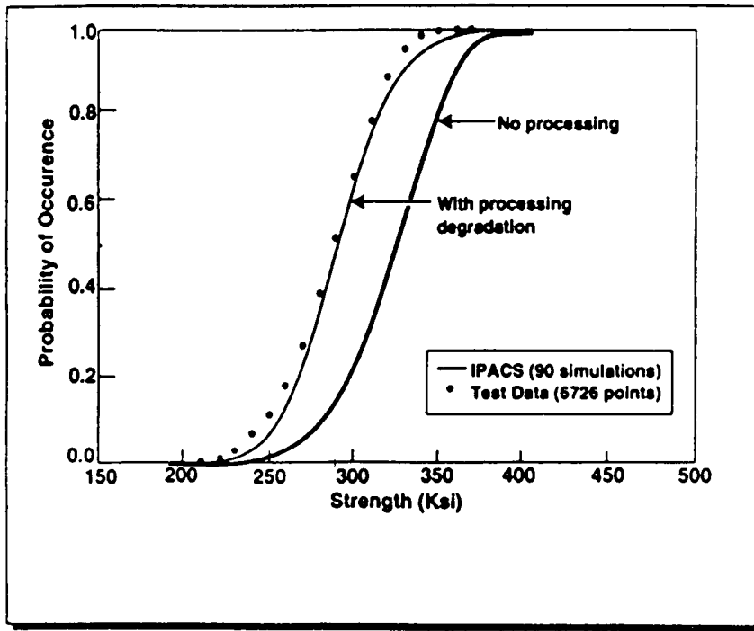
Figure 7 - Probabilistic Simulation of Longitudinal Tensile Strength Scatter in AS/E Composites.
