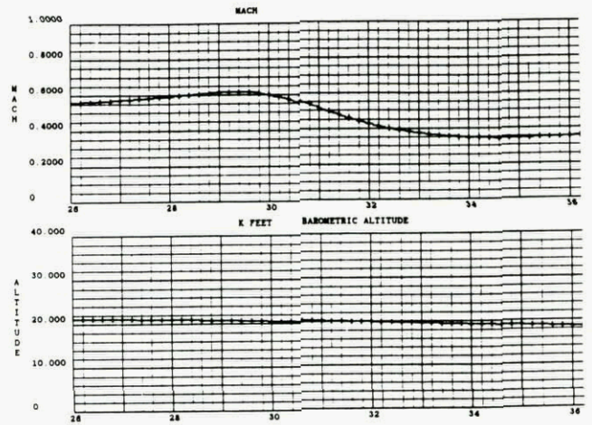
Fig. 5 X-31 - 6g abrupt WUT (Split -S) to 70° Alpha Mach/Altitude versus time
