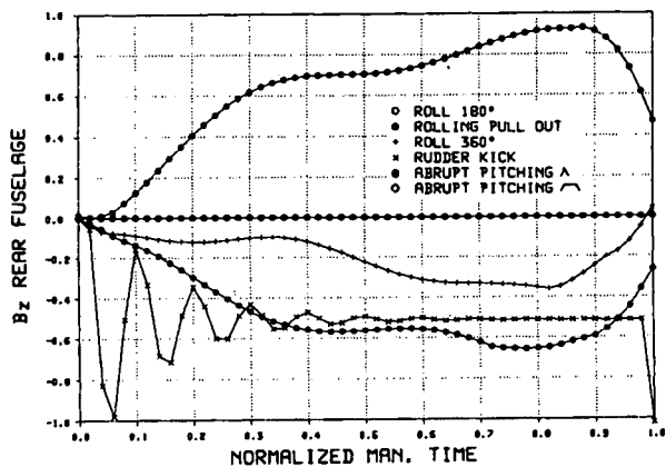
Figure 6.4 STRUCTURAL LOADS MIL-MANEUVERS
