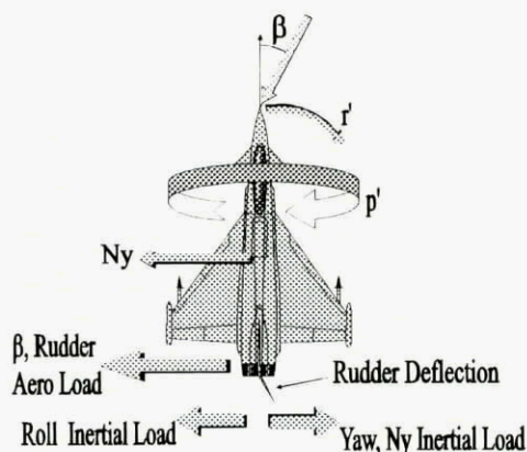
Figure 12. Loading Assumptions for Fin Design Case
