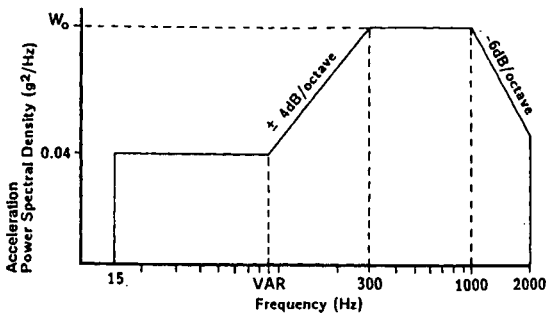
Fig.: 28 General Vibration Test Spectrum
