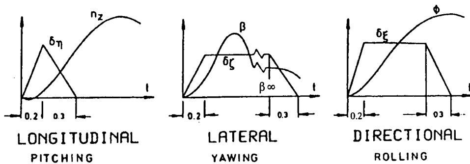
Fig. 2 COCKPIT CONTROL DISPLACEMENT AIR 2004/E
