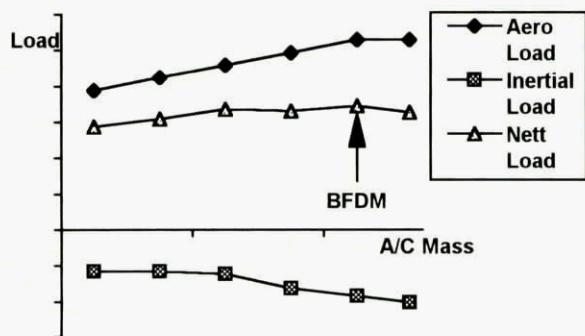
Figure 6. Variation of Wing Load
