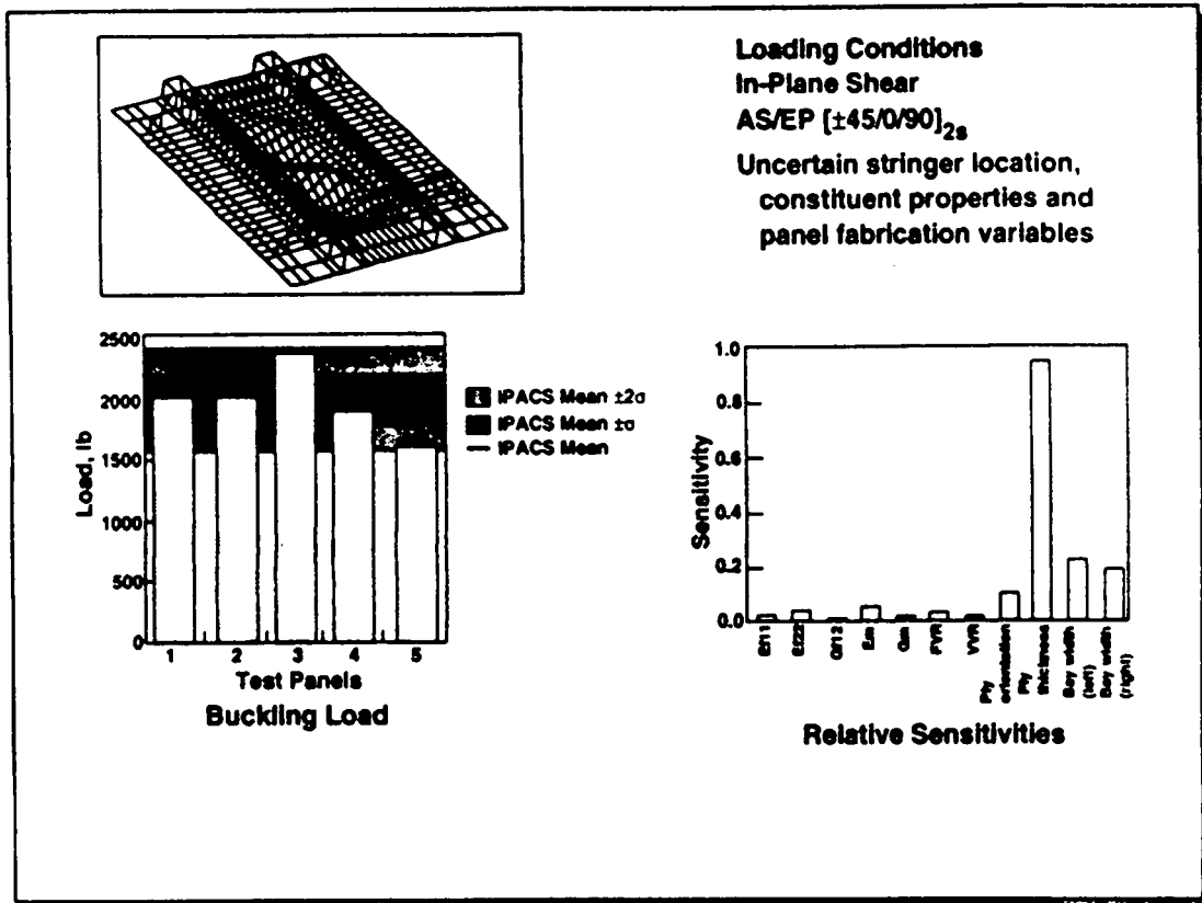
Figure 6 - Probabilistic Qualification of Composite Skin-Stringer Panel for Shear Buckling.
