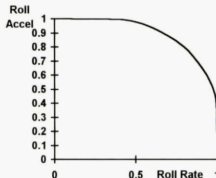
Figure 8. Roll Rate/Acceleration Combinations
