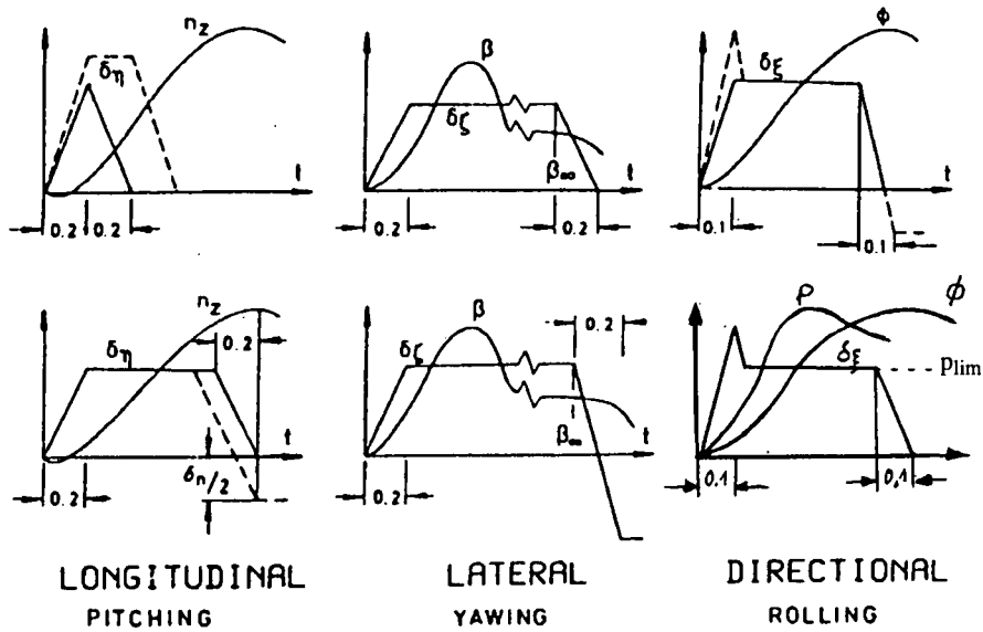
Fig. 1 COCKPIT CONTROL DISPLACEMENT MIL-A-008861A
