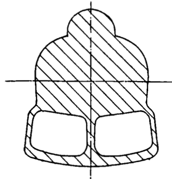
Fig.: 19a Influence of Intake/Duct Shape on Total Pressure Including Hammershock
