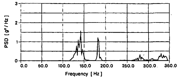
Fig.: 38 PSD of x acceleration at IMU c.g. due to butt firing (x-excitation)
