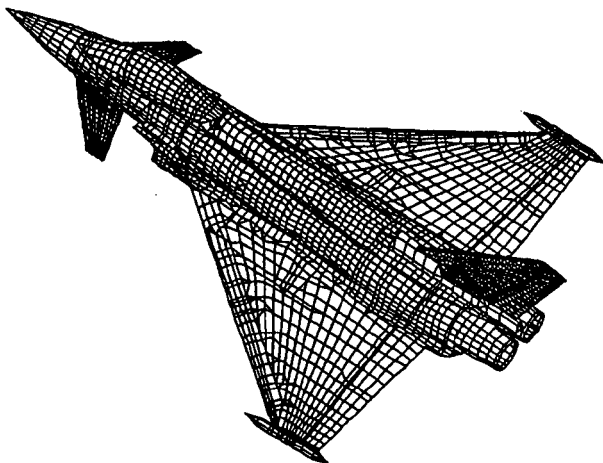
Fig. 33: Finite Element Model Total A/C Structure Idealization
