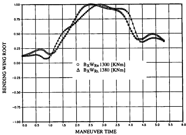
Figure 5.5 EXTREME OPERATIONAL LOADS HIGH-G-TURN
