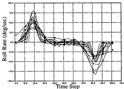
Figure 8 Shifted Roll Rate Traces
