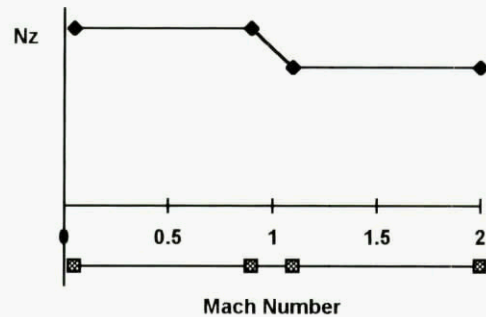
Figure 5. Normal Acceleration Requirements
