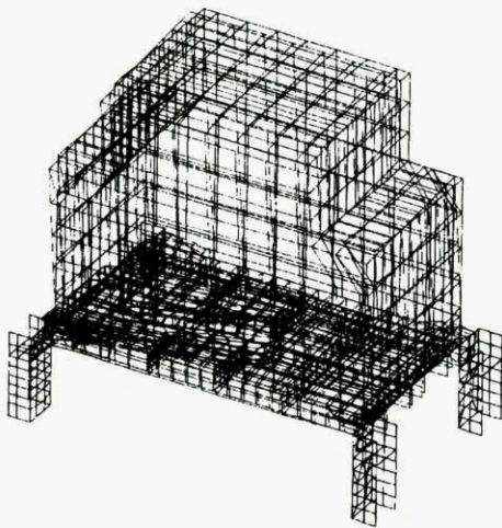
Fig.: 42b Calculated Mode Shape; f = 50.93 Hz
