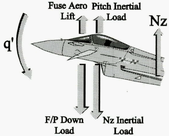
Figure 16. Balance of Forces for Front Fuselage
