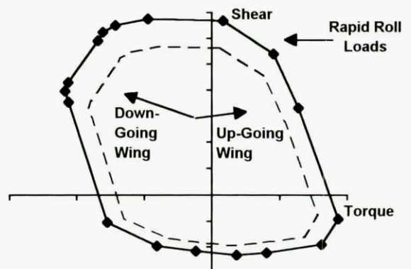
Figure 17. Wing Root Loads During Rolling
