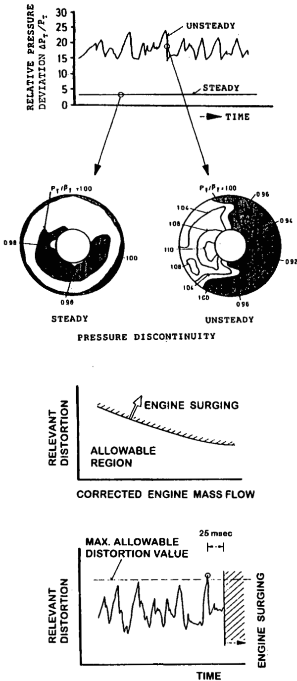
Fig.: 18 Origin of Hammershock
