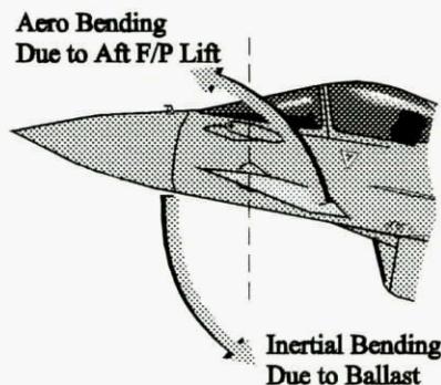
Figure 19. Combination of Ballast and Foreplane Loads
