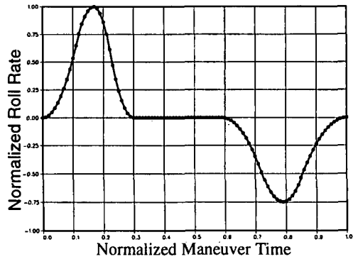
Figure 7 Normalized Roll Rate Trace
