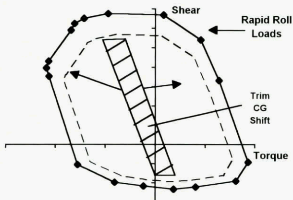
Figure 18. Effect of CG Range on Rolling Loads
