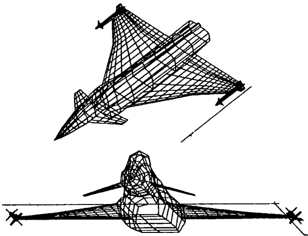
Fig.: 2 Aerodynamic Grid (Idealisation)
