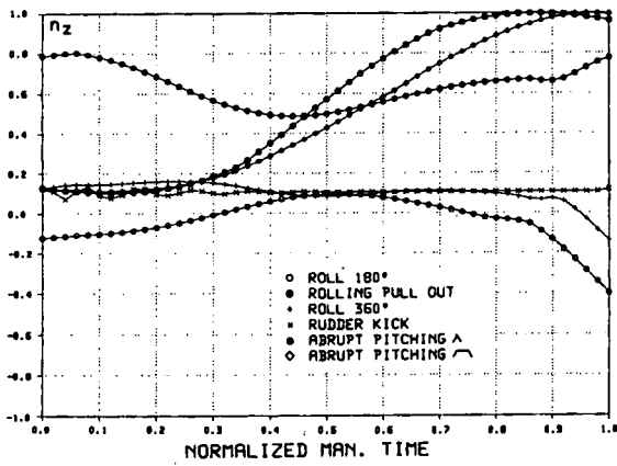
Figure 6.1 LOAD FACTORS-MIL-MANEUVERS
