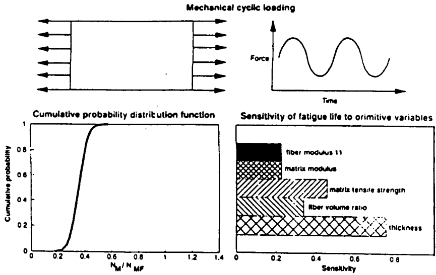
Figure 9 - Probabilistic Simulation of Fatigue Life Curve for Graphite/Epoxy (0/±45/90) 4 Laminate. Applied Stress/First Ply Failure Strength = 0.9.
