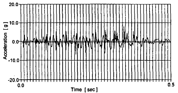
Fig. 39: IMU acceleration in z due to gunfiring (Total aircraft FE model f_{max} = 80 Hz)
