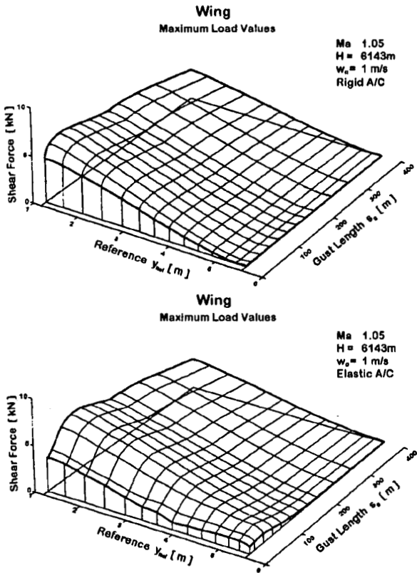
Fig.: 5 Design Gust Calculation: Wing Shear Force
