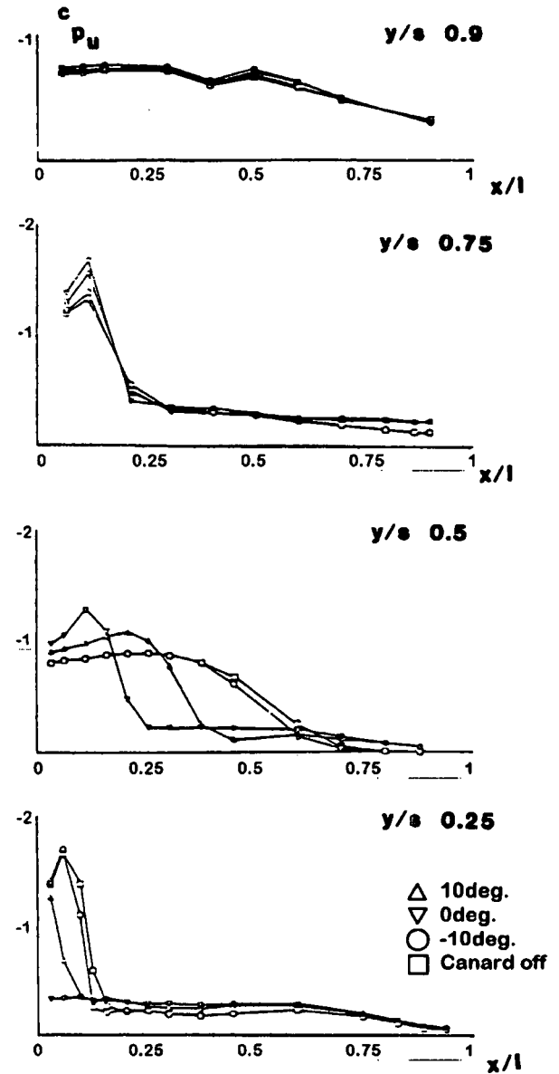
Fig.: 8 Steady Pressure Distribution
