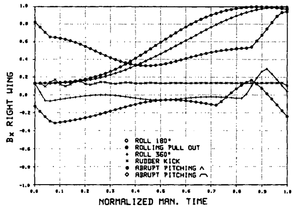
Figure 6.2 STRUCTURAL LOADS MIL-MANEUVERS
