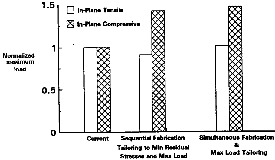
Figure 6 - Fabrication Process Tailoring Influence on the Maximum In-Service Load for P100/Copper [0/90] 3 at 316°C
