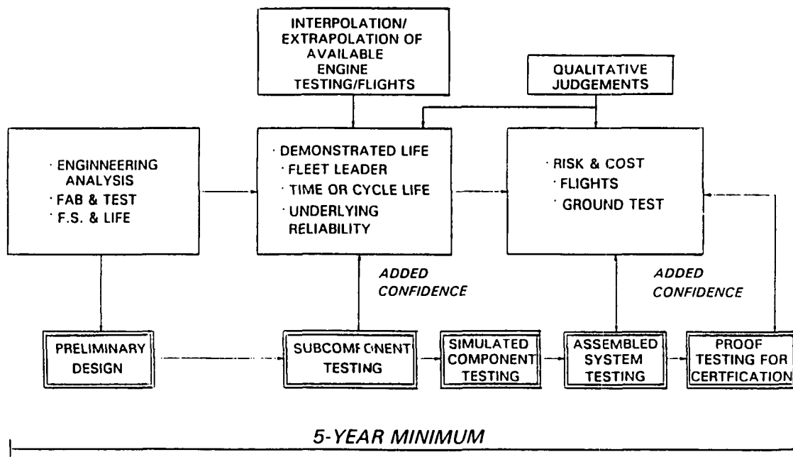
Figure 1 - Current development approach for liquid rocket propulsion
