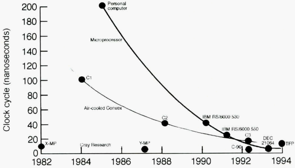
Fig. 11 - Progress in the clock speed for microprocessors.
