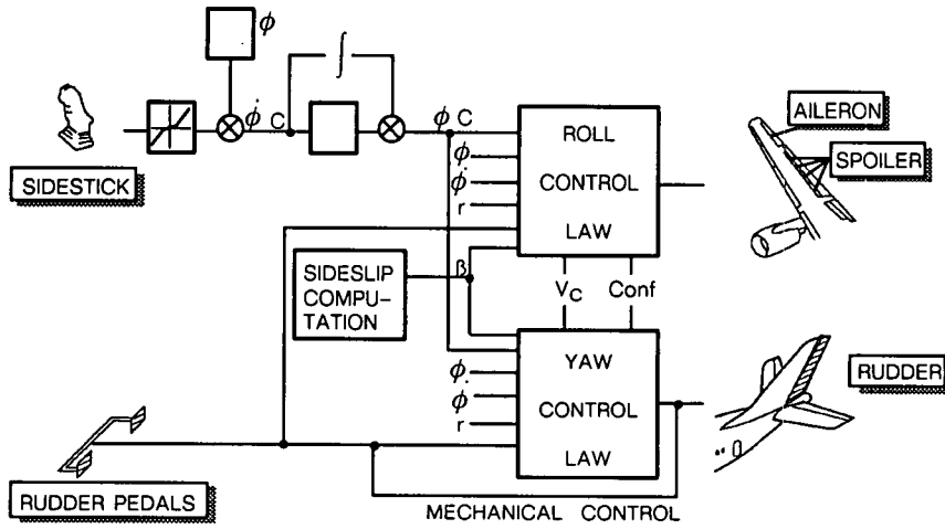
Fig. 9 Lateral Control Arrangement
