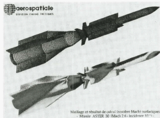
Fig. 11 Complex missile flowfield analysis at AEROSPATIALE. Euler solution at M = 2.6 and \alpha = 10^\circ
