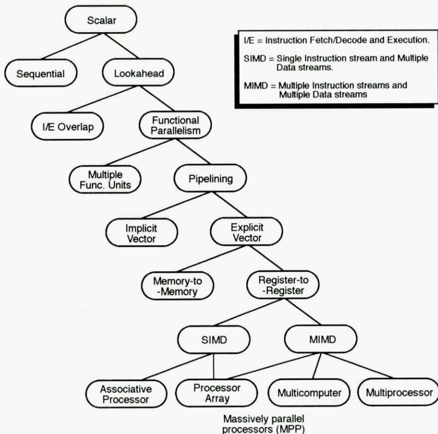
Fig. 8 - Architectural evolution of computing systems (see Ref. 5).
