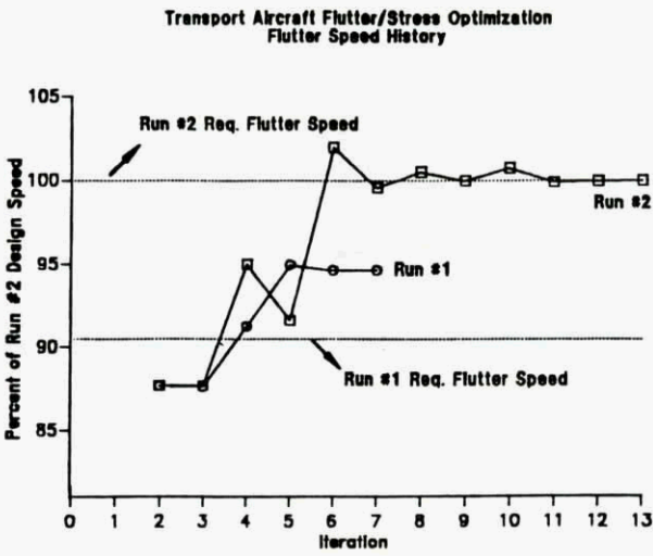
Fig. 8. Flutter Speed Versus Iteration
