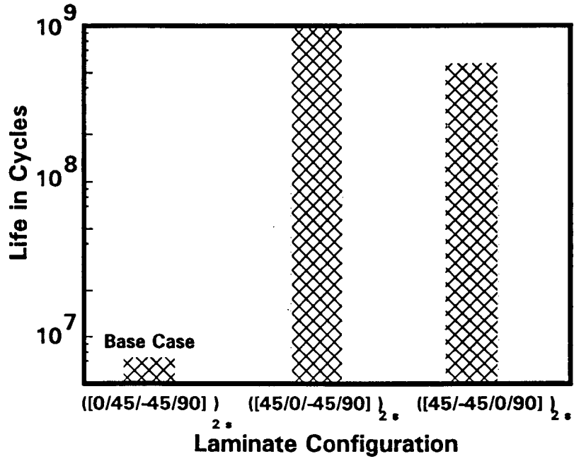
Figure 8 - Coupled Composite-materials/hygral/thermal/structural/acoustic simulation: Effect of Laminate Configuration
