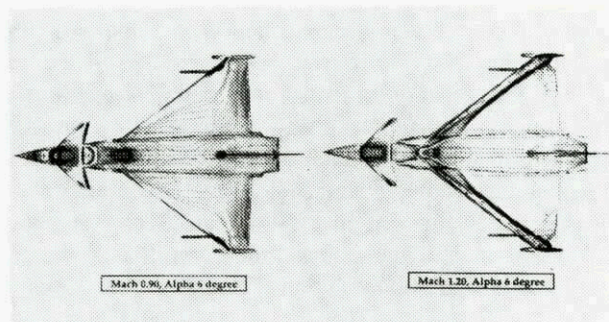
Fig. 9 Fighter Aircraft analysis using Euler Flow computations
