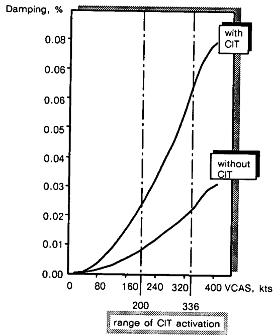
Fig. 17 Modal Damping Increase For Vertical CIT
