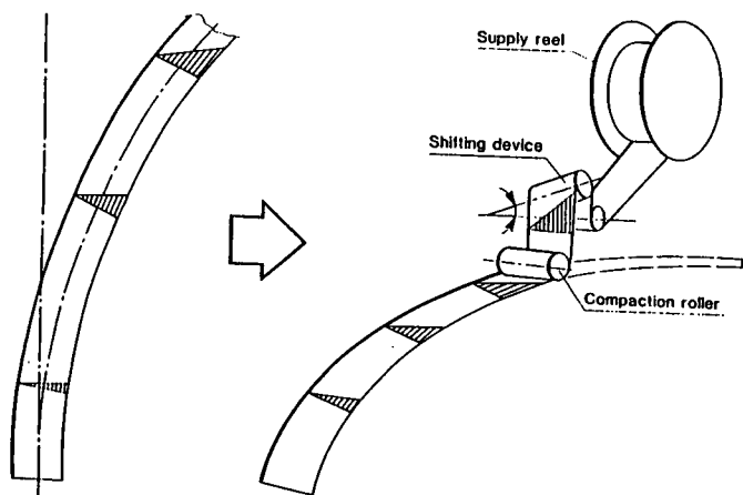
Fig. 9: Fiber shifting device for tape steering
