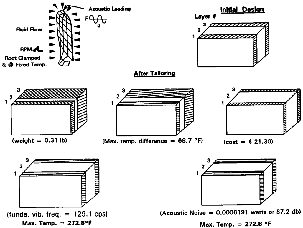
Figure 5 - Multi-material Multi-layered Composite Fan Blade: Tailored Designs Under Multi-disciplinary Loadings
