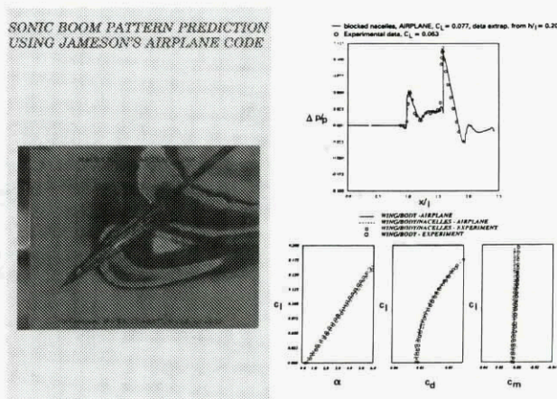
Fig. 25 Sonic boom pattern prediction using Jameson's airplane code
