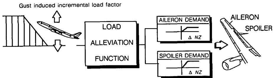
Fig. 14 Gust Load Alleviation Function
