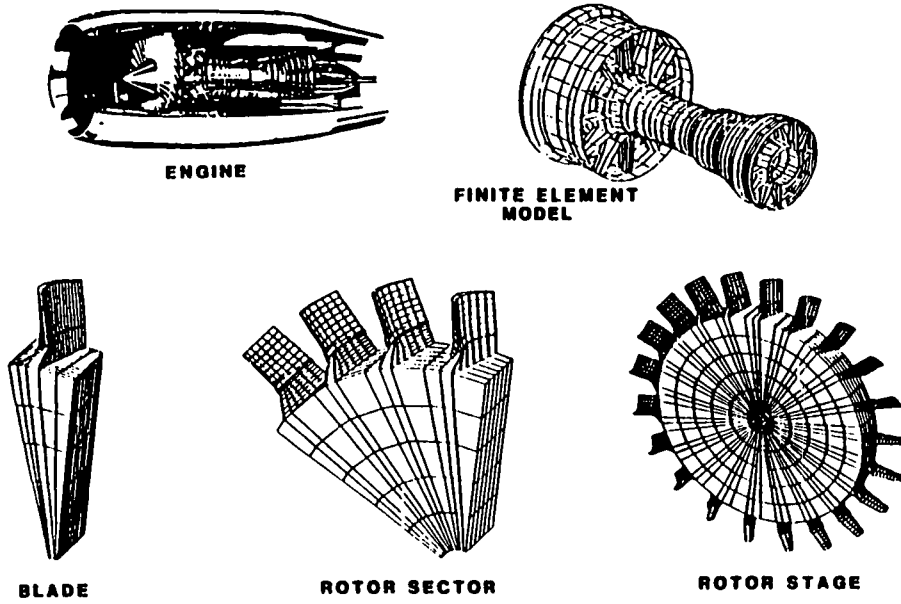
Figure 8 - Engine Structures Computational Simulator (ESCS)
