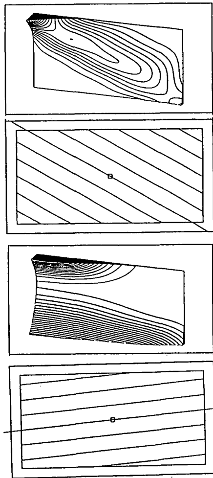
Fig. 14a: Thickness distribution for straight tape courses
