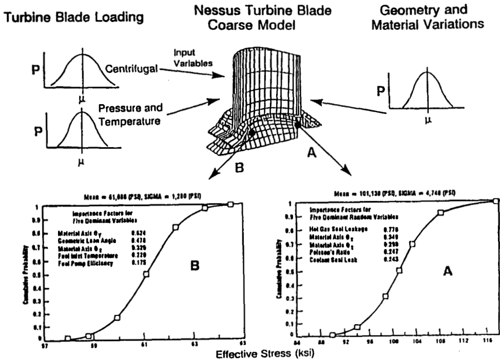
Figure 10 - Probabilistic Component Stress and Sensitivities Analyses
