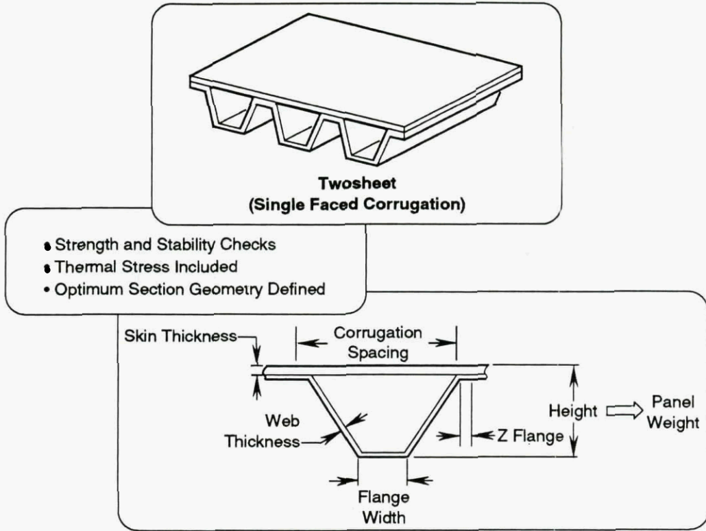
Figure 10. Detail Section Parameters of Sizing Codes
