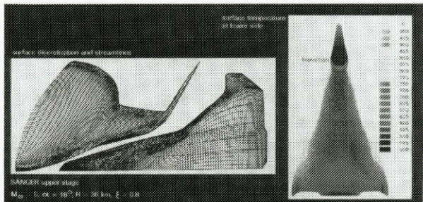
Fig. 8 Approximate methods used for the determination of heat loads at hypersonic Mach numbers
