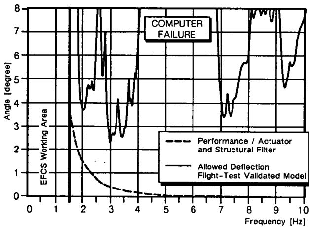
Fig. 11 Rudder-Oscillating Allowed Surface Deflection Acceptable by Static Loads Envelope
