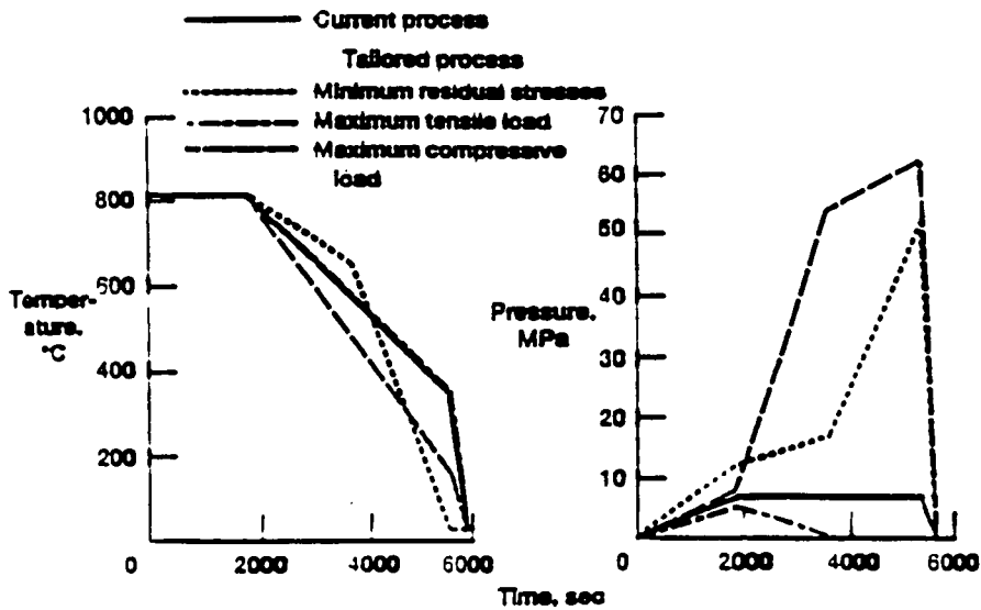
Figure 7 - Tailored Fabrication Process for [0/90] 3 Graphite/Copper by Different Objectives
