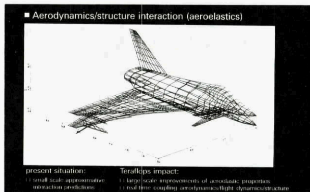
Fig. 27 Aeroelasticity - a challenge for supercomputing (Coupling of aerodynamics and structural dynamics)
