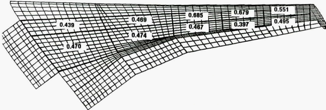
Fig. 14. Lower Wing Stiffening Ratios
