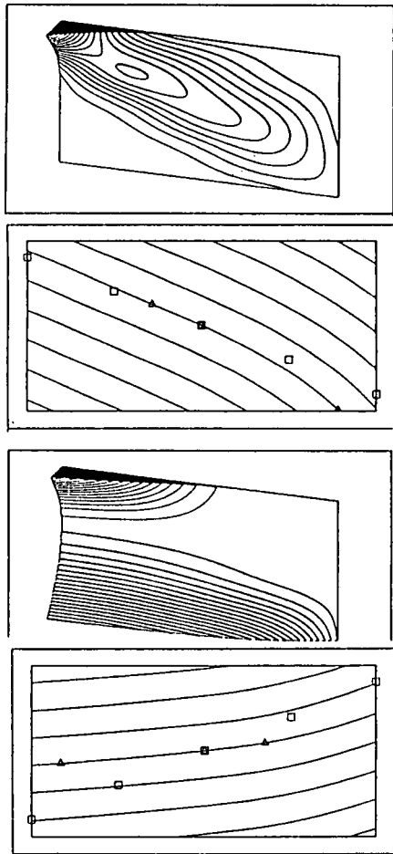
Fig. 14b: Thickness distribution for curved tape courses
