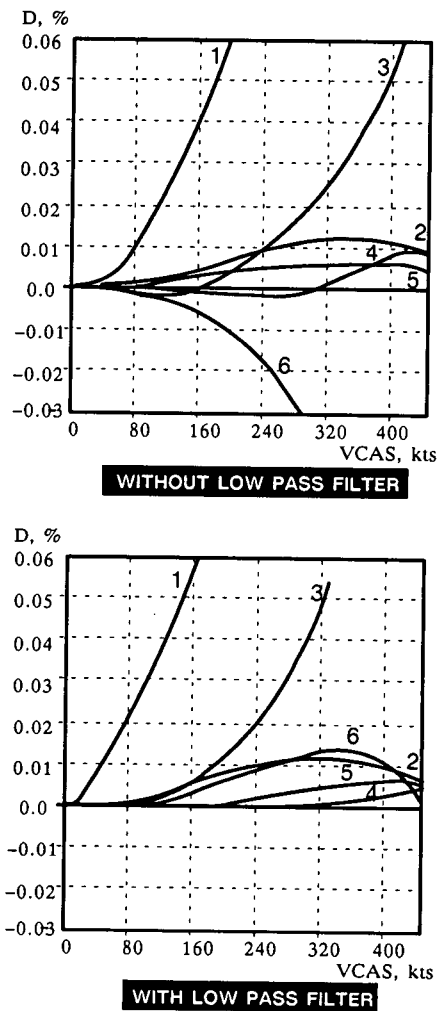
Fig. 7 Influence of Low Pass Filters on The Mode Damping of Flutter Calculation
