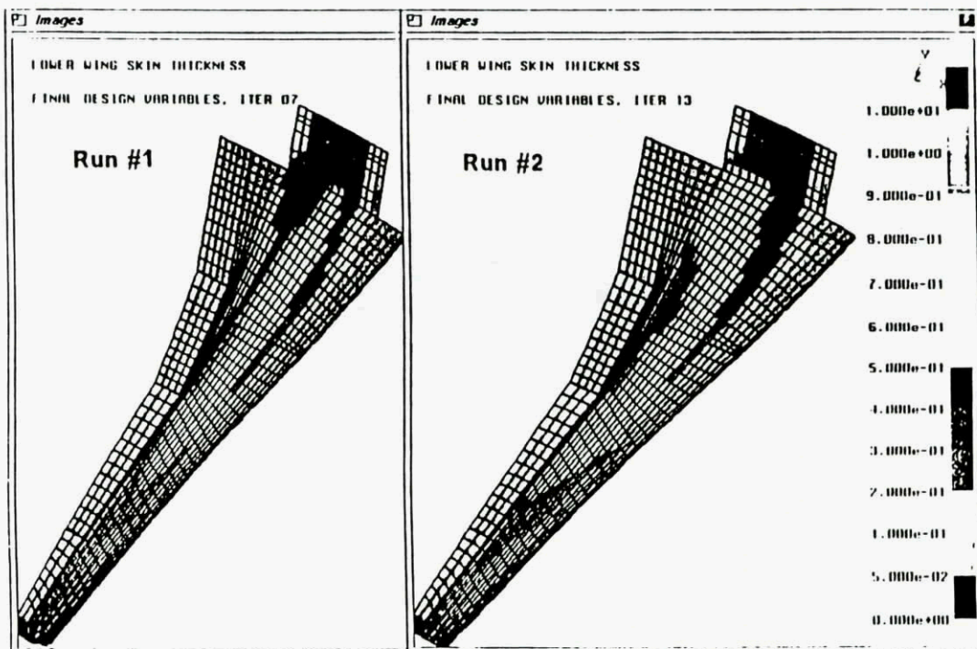
Fig. 10. Comparison of Skin Thickness Distributions
