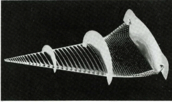
Fig. 16 Simulation of hypersonic flow at RWTH Aachen using Navier-Stokes solution with real gas effects
