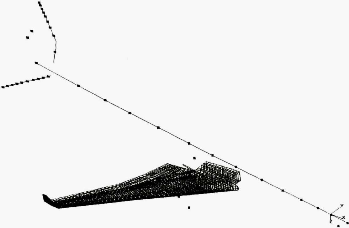
Fig. 7. 3-D Finite Element Model for Stress and Flutter Design
