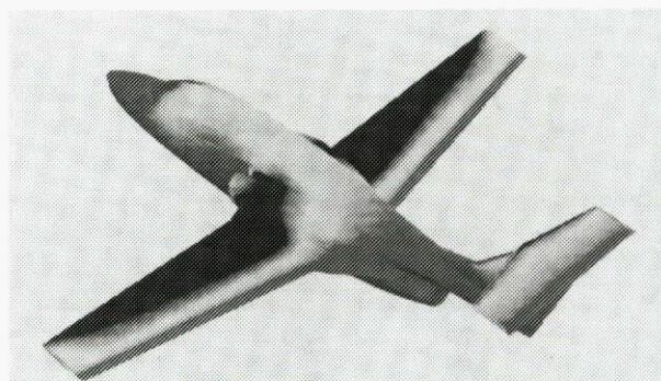
Fig. 7 JPATS-Fanranger surface pressure analysis using panel methods applied during design (HISSS at Dasa, M = 0,5 , \alpha = 5^\circ )
