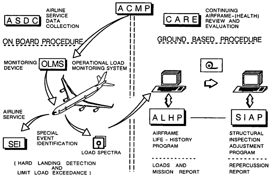
Fig. 4: Airframe Condition Monitoring Procedure, ACMP
