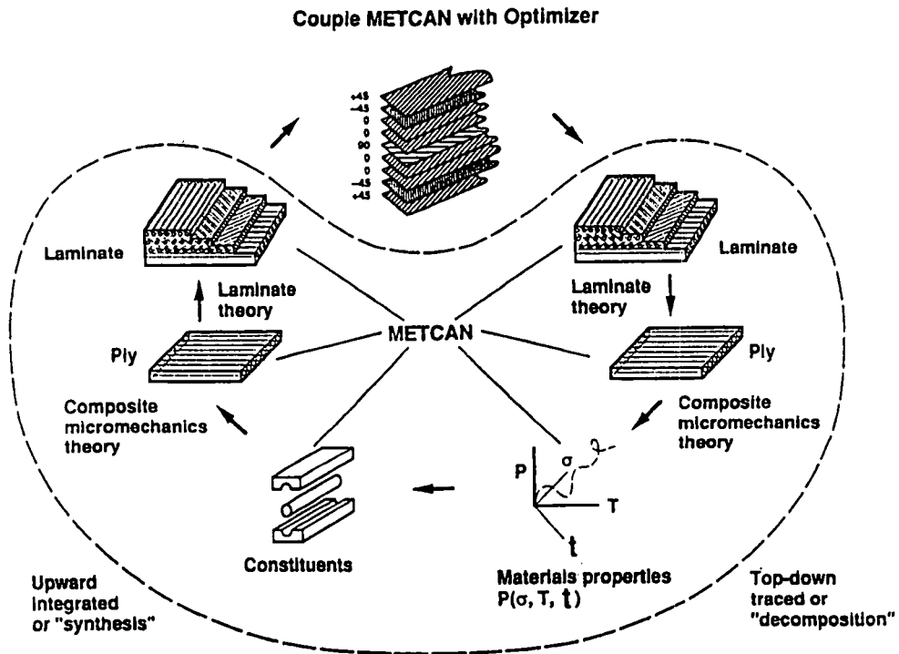
Figure 5 - Metal Matrix Laminate Tailoring (MMLT)
