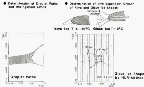
Fig. 28 Water droplet paths and icing on Do 328 wing section
