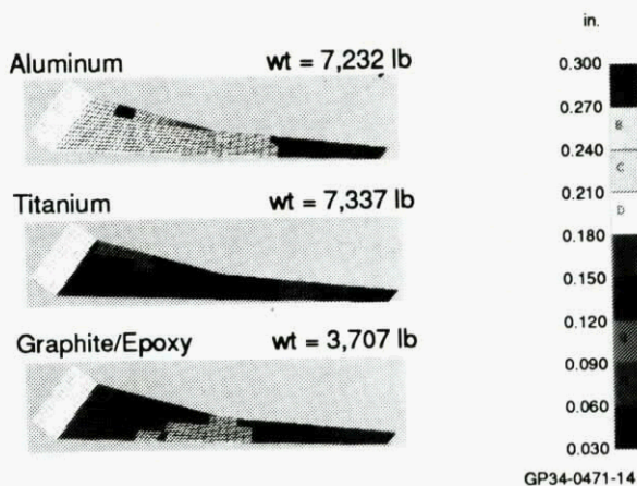
Figure 14. Composite Material Has Potential Weight Benefit
