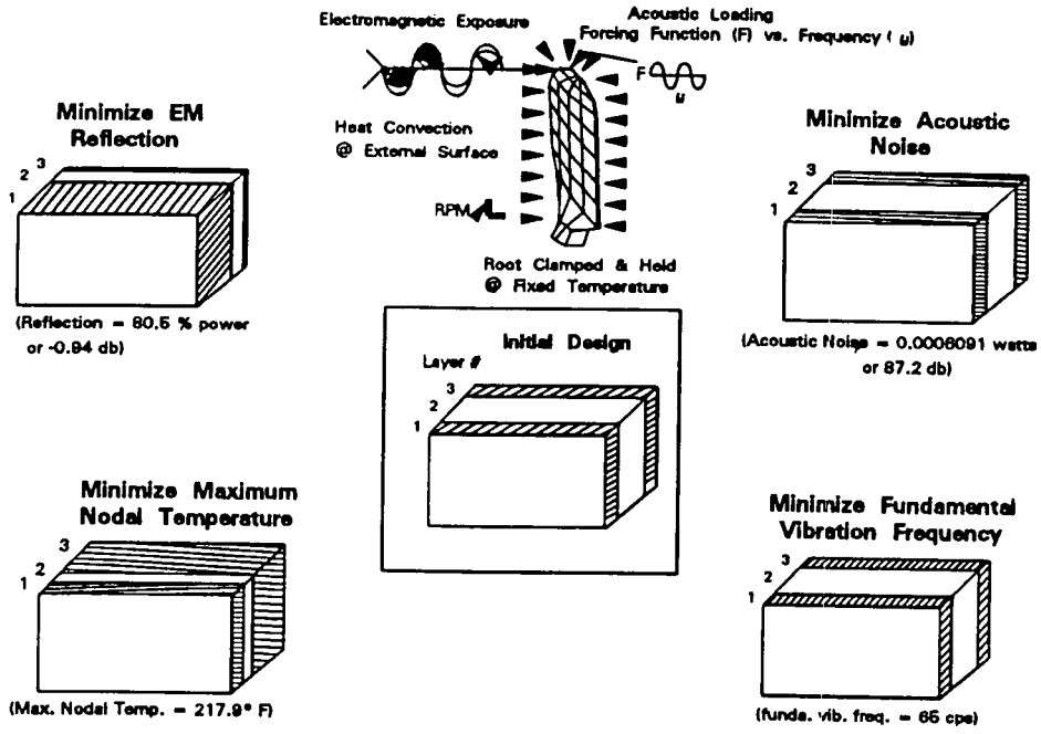
Figure 4 - Fan blade laminate configuration for multi-disciplinary tailoring
