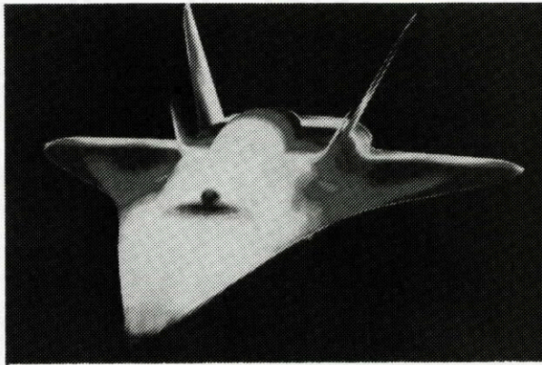
Fig. 12 Euler analysis of a TSTO-configuration at M = 0,9 and \alpha = 10^\circ with upper stage
