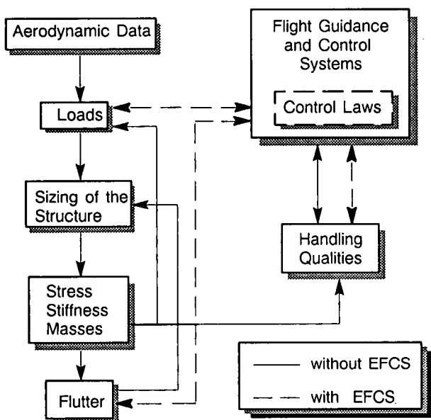
Fig 1: Aircraft Design
