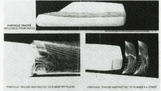
Fig. 18 Application of Navier-Stokes numerical flow simulation for the development of a station wagon car
