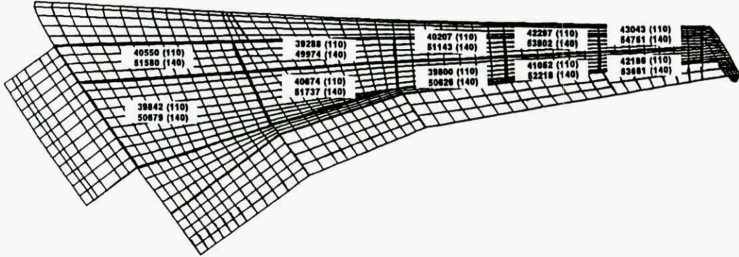
Fig. 12. Lower Surface 2-Bay Crack Stress Allowables
