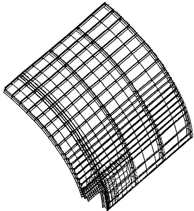
Fig. 7: structural model of fuselage cut-out
