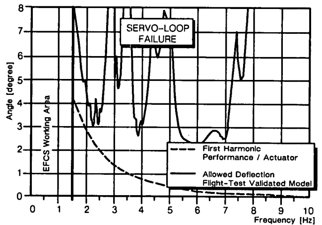
Fig. 12 Antisymmetrical Inboard Aileron-Oscillating Allowed Surface Deflection Acceptable by Static Loads Envelope
