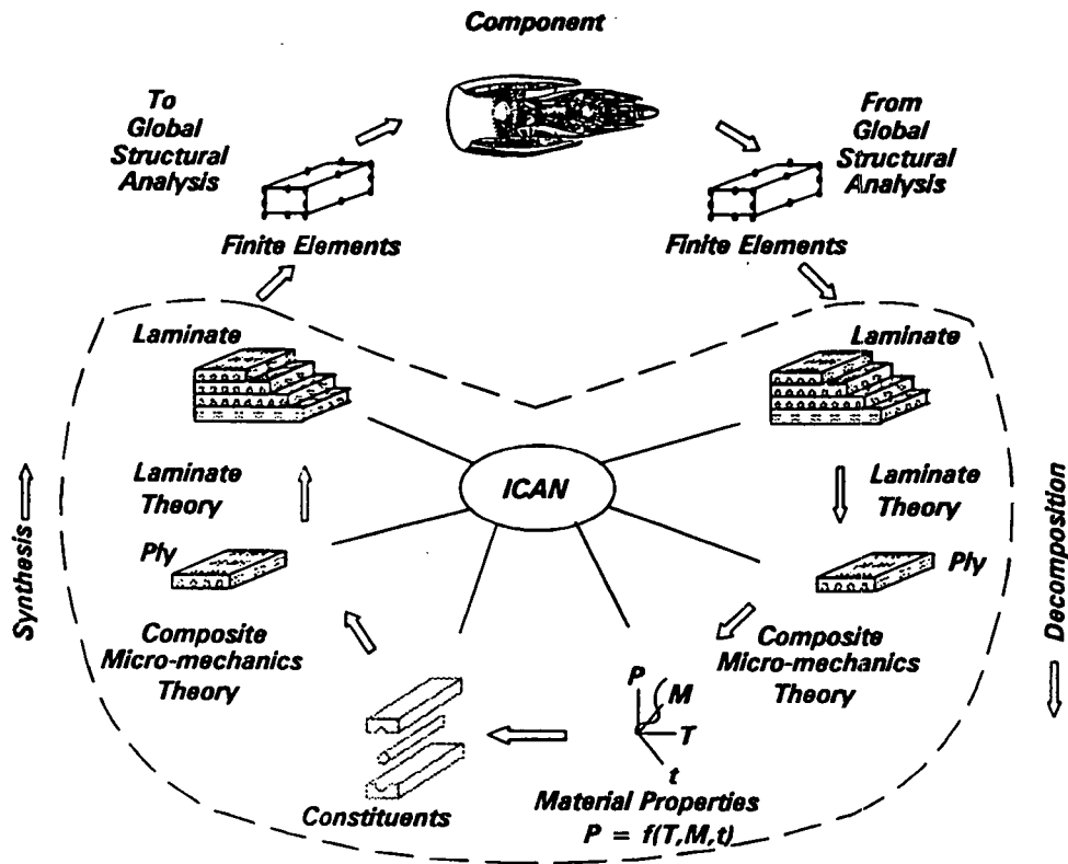
Figure 3 - Integrated Composite Analysis (ICAN)
