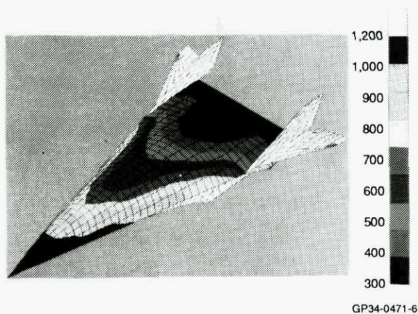
Figure 6. Maximum Temperature Gradients Ascent Trajectory
