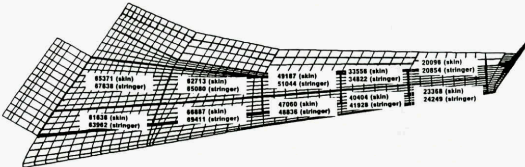
Fig. 13. Upper Surface Panel Buckling Stress Allowables
