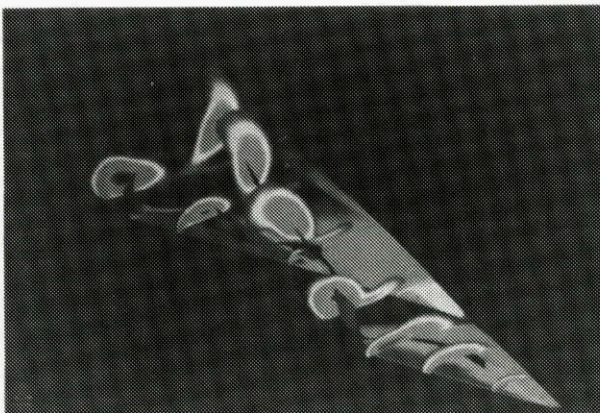
Fig. 21 Euler simulation of canard-wing vortex flows within the European research initiative IEPG TA 15.
