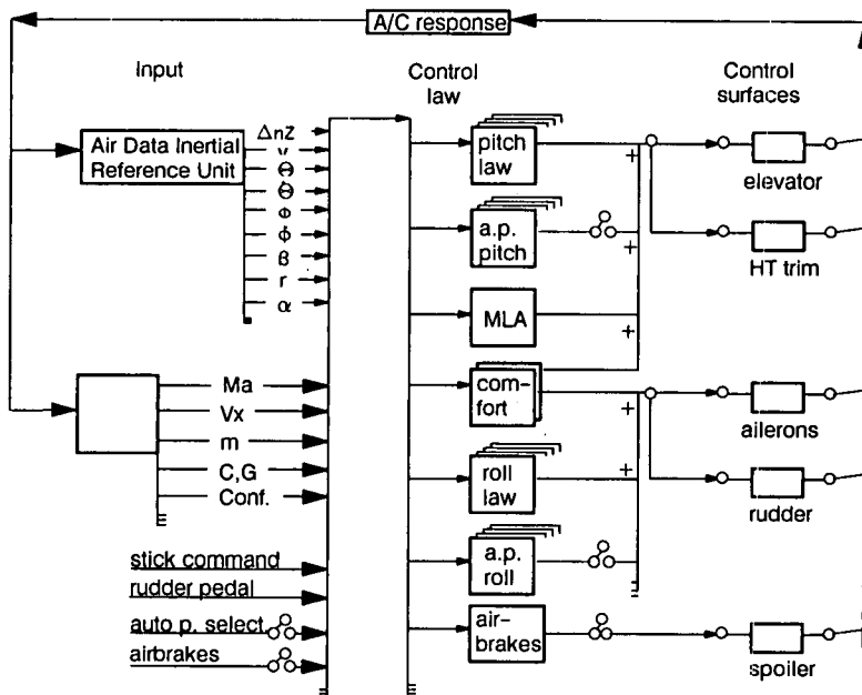
Fig. 3: Simplified Electronic Control Circuit
