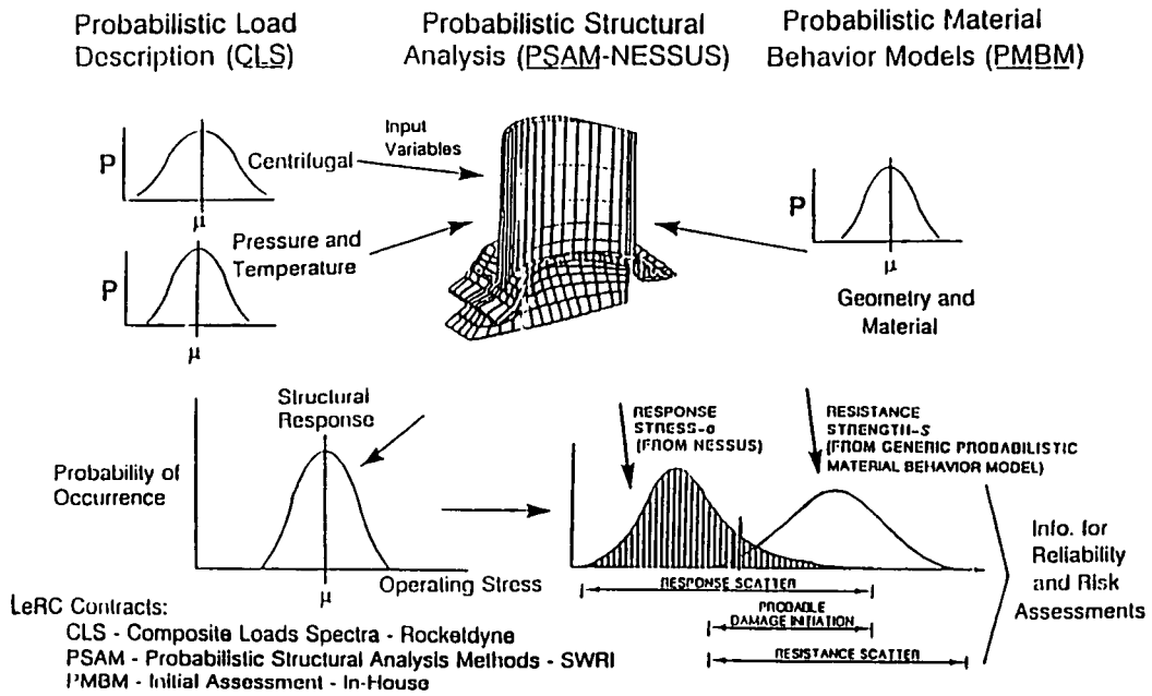
Figure 10 - Probabilistic Simulation of Component Reliability
