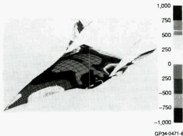
Figure 8. Maximum Temperature Gradients Ascent Trajectory
