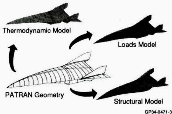
Figure 3. Different Analysis Models Generated From Same Geometry
