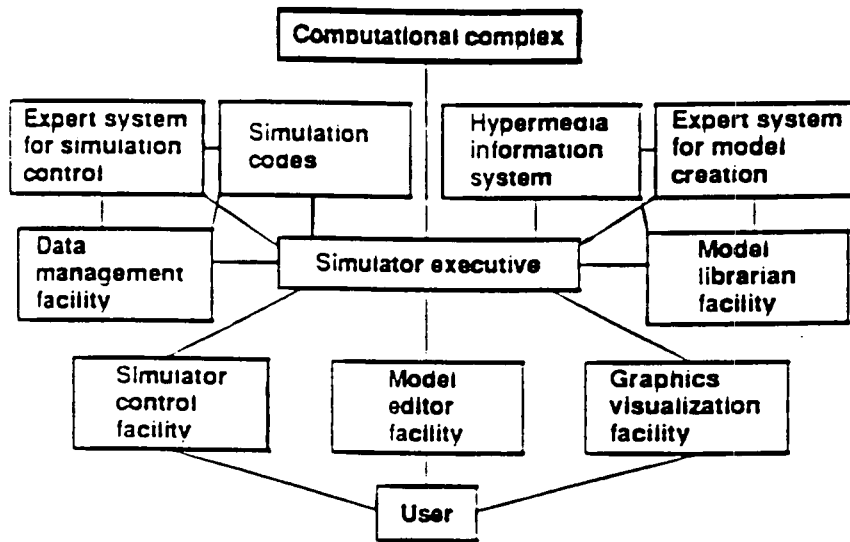
Figure 14 - Simulator Architecture
