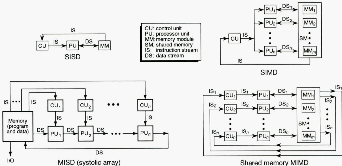
Fig. 7 - Block diagrams for SISC, SIMD, MISD and MIMD machines.
