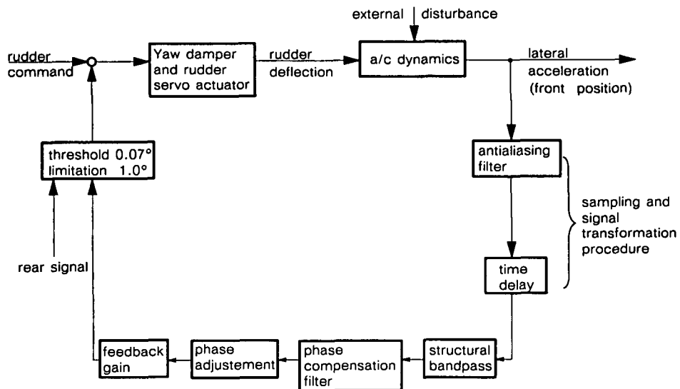
Fig. 15 Principle Scheme For Lateral CIT
