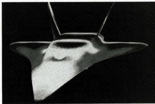
Fig. 13 Euler analysis of a TSTO-configuration at M = 0,9 and \alpha = 10^\circ without upper stage
