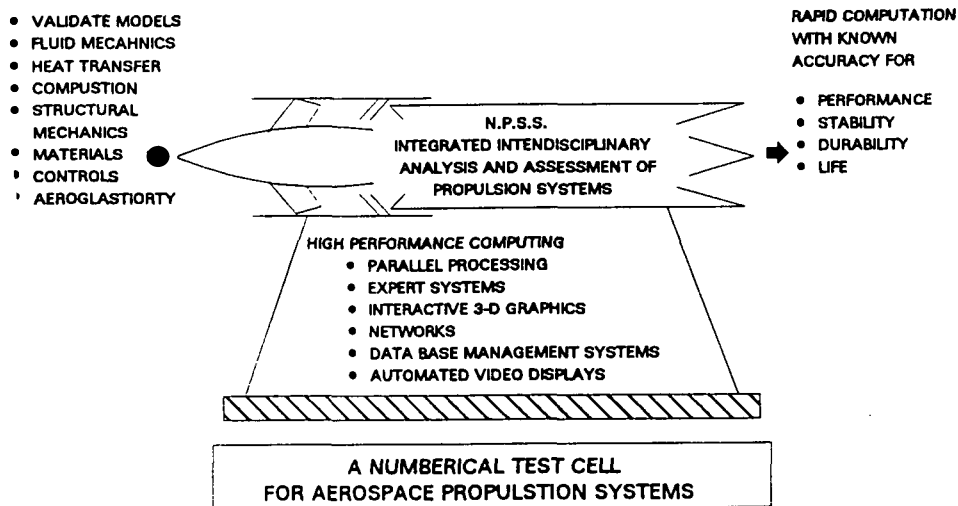
Figure 13 - Numerical Propulsion System Simulator
