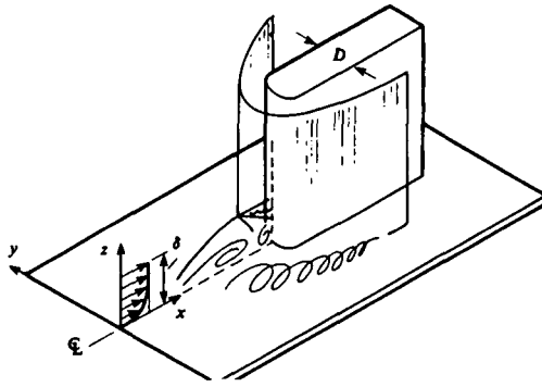
Figure 21: Geometry for blunt fin
