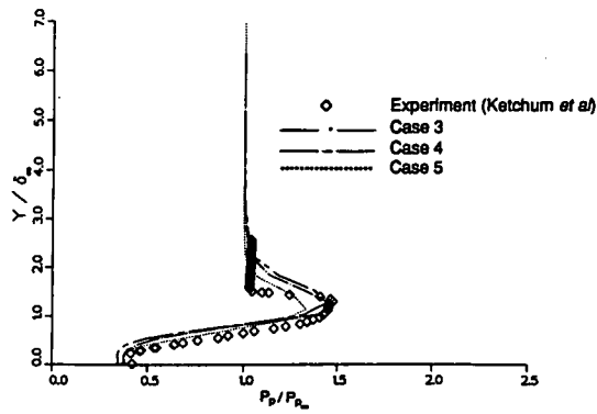
Figure 34: Pitot pressure for swept compression corner for \alpha = 20^\circ and \lambda = 40^\circ
