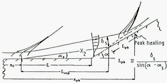
Fig. 22 - Approximation to the growth length of the reattaching boundary layer to the location of peak heating [50]
