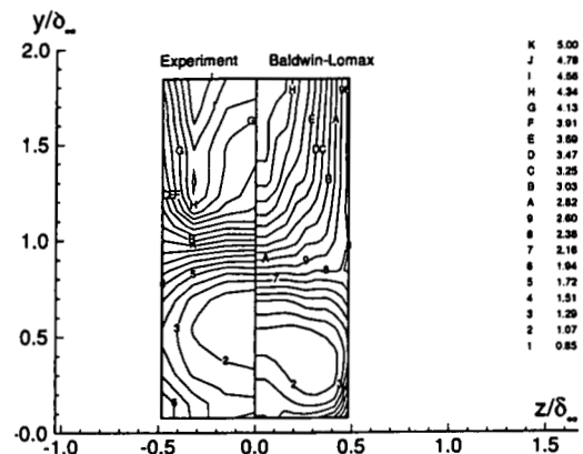
Figure 55: Pitot pressure for crossing shock at M_\infty = 8.3, \alpha = 15^\circ, Re_{\delta_\infty} = 1.7 \times 10^5, x = 8.3\delta_\infty , Baldwin-Lomax model
