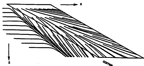
Figure 40: Skin friction lines for swept compression corner
