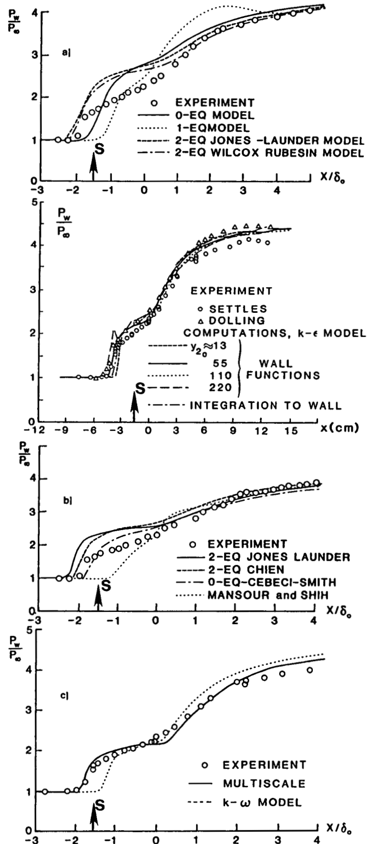
Fig. 43. Measured and computed wall pressure distributions in a 24-deg., Mach 3 compression ramp interaction: a) Viegas and Horstman (1979); b) Viegas, Rubesin and Horstman (1985); c) Champney (1989); d) Wilcox (1990).
