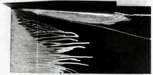
Fig. 18: Surface flow visualization, M = 6 , unswept shock generator, \alpha = 3^\circ
