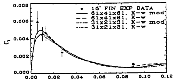
Figure 17: Skin friction for sharp fin at M_\infty = 8.2, \alpha = 15^\circ, Re_{\delta_\infty} = 1.9 \times 10^5
