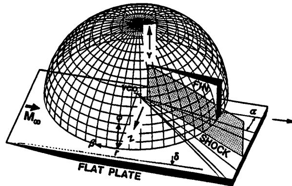
Figure 63: Spherical polar coordinates
