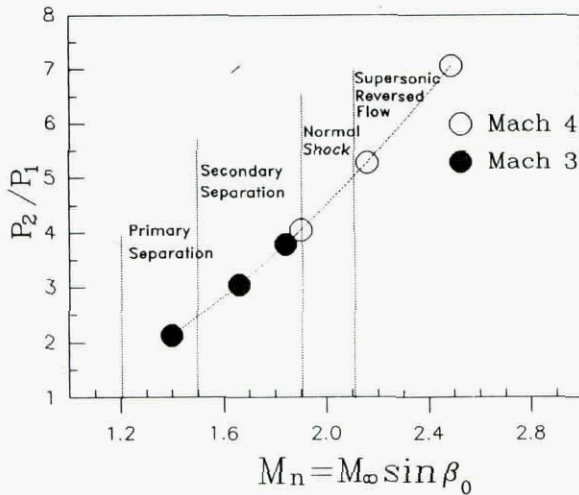
Fig. 22 - Interaction Test Matrix of Alvi and Settles.
