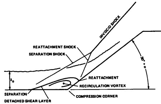
Figure 27: Flowfield for cylinder/flare
