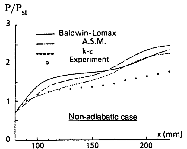
Fig. 34 - 2D supersonic flow. Wall pressure distributions. Interaction with separation.
