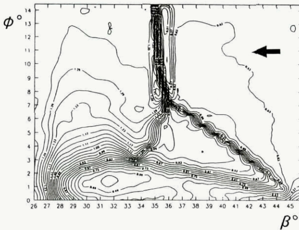
Fig. 27 - Flowfield Density Map of Mach 3, \alpha = 16^\circ Interaction.
