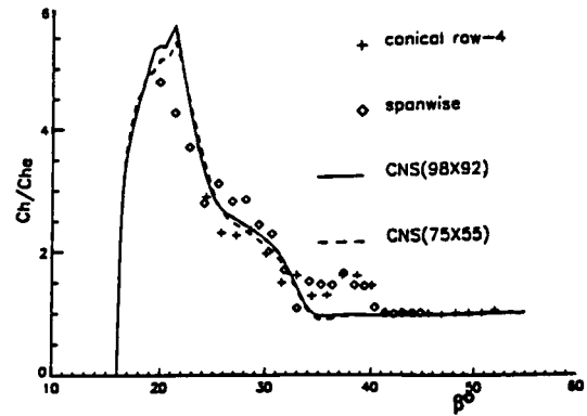
Figure 10: Heat transfer for sharp fin at M_\infty = 5.0, \alpha = 16^\circ, Re_{\delta_\infty} = 2.4 \times 10^5
