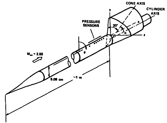
Figure 26: Geometry for cylinder/flare
