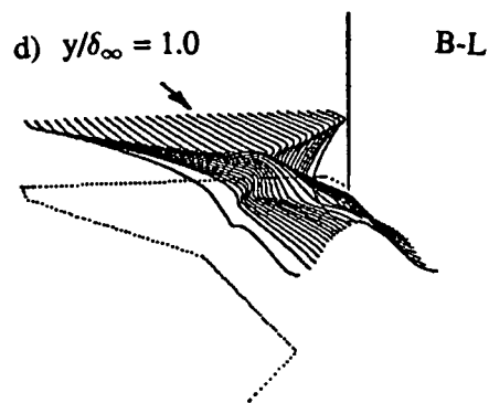
Figure 62: Streamline structure for crossing shock at M_\infty = 8.3 , Re_{\delta_\infty} = 1.7 \times 10^5 , \alpha = 15^\circ
