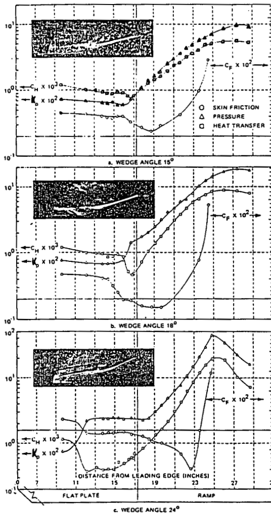
Fig. 7 - Pressure, skin friction and heat transfer distributions over laminar 2D compression ramp interactions at Mach 14.1 with Re_L=105,000 and T_w/T_0=0.1 [32]
