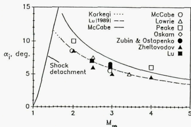
Fig. 8 - Incipient Separation Criterion for Sharp-Fin Interactions.
