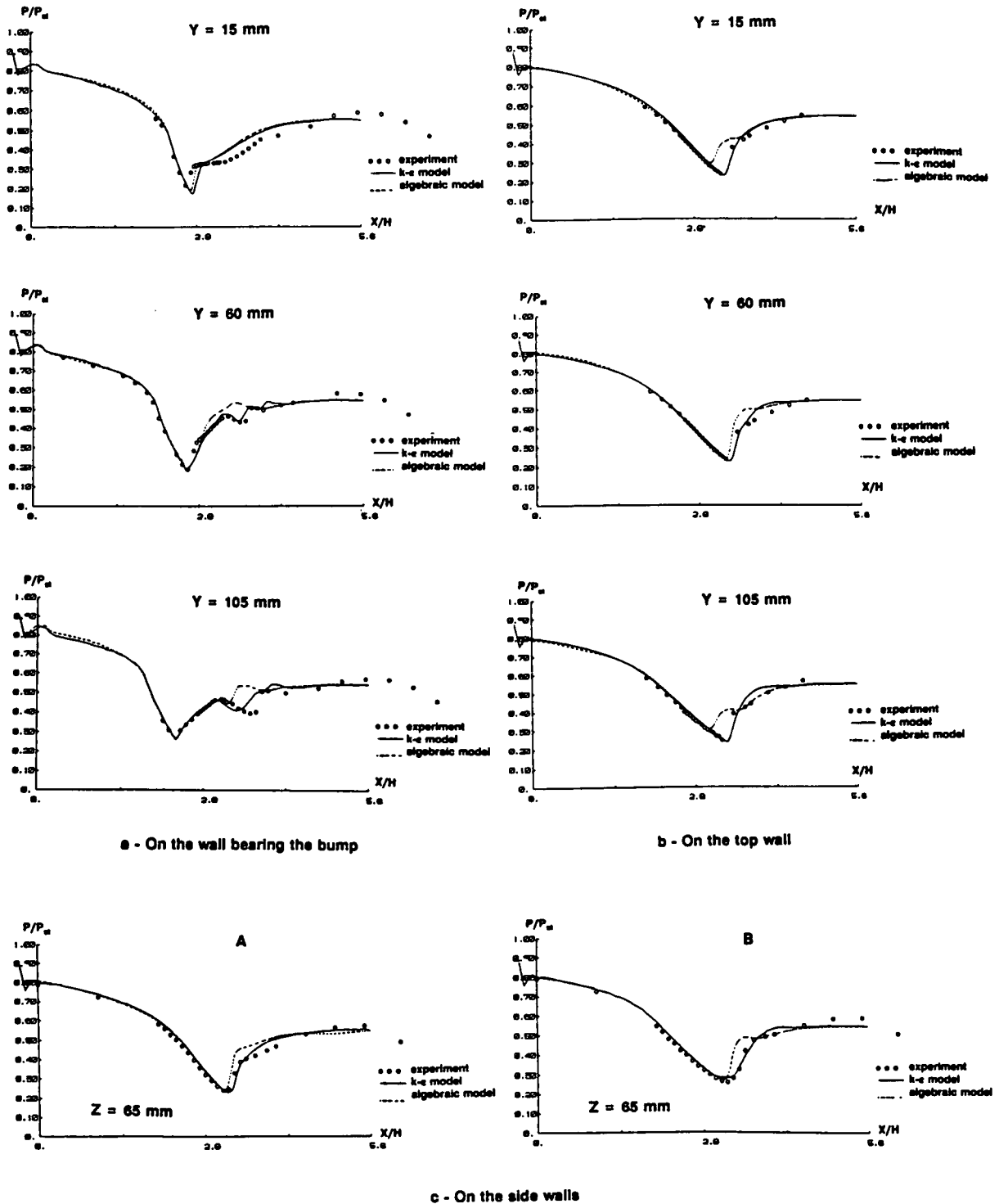
Fig. 47 - 3D transonic flow. Wall pressure distributions
