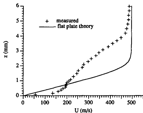
Fig. 31: Velocity profile at y/x = 0.8
