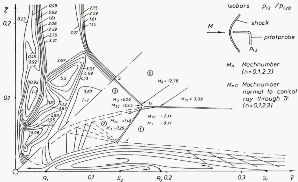
Fig. 9: Pitot pressure contours and wave pattern in corner flow (from [25])
