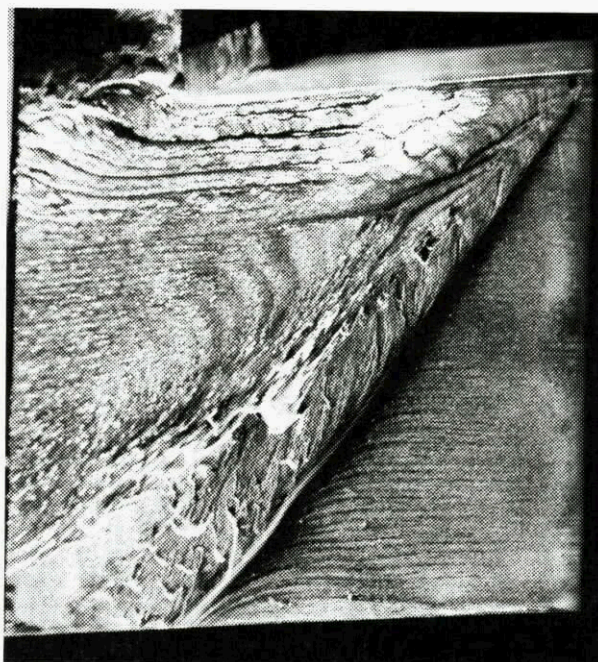
Fig. 13: Surface flow visualization, M = 2 , unswept shock generator, \alpha = 9^\circ
