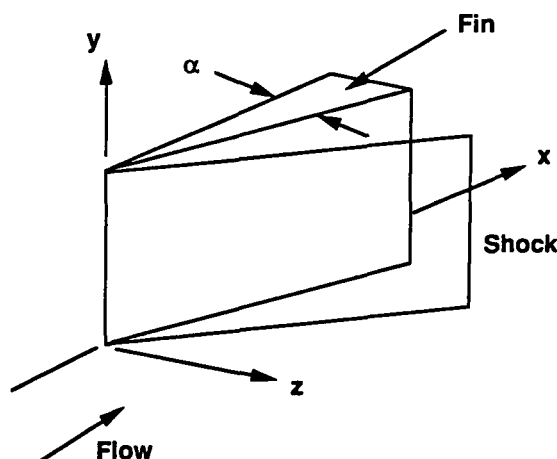
Figure 1: Geometry of sharp fin
