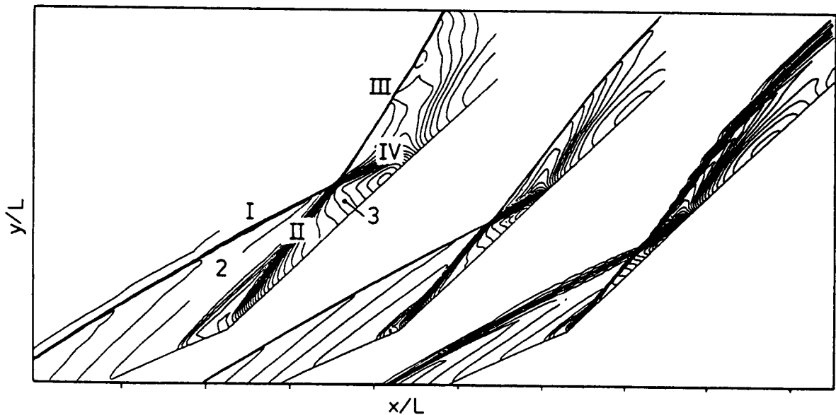
Fig. 56 - Pressure contours near the hinge line of the hyperboloid / flare configuration at Mach 25, Re_L=120,000 , T_w=800 K, T_\infty=192 K (flight conditions, 77 km altitude); left: frozen air perfect gas model; center: chemical nonequilibrium air model; right: thermochemical equilibrium air model [106]
