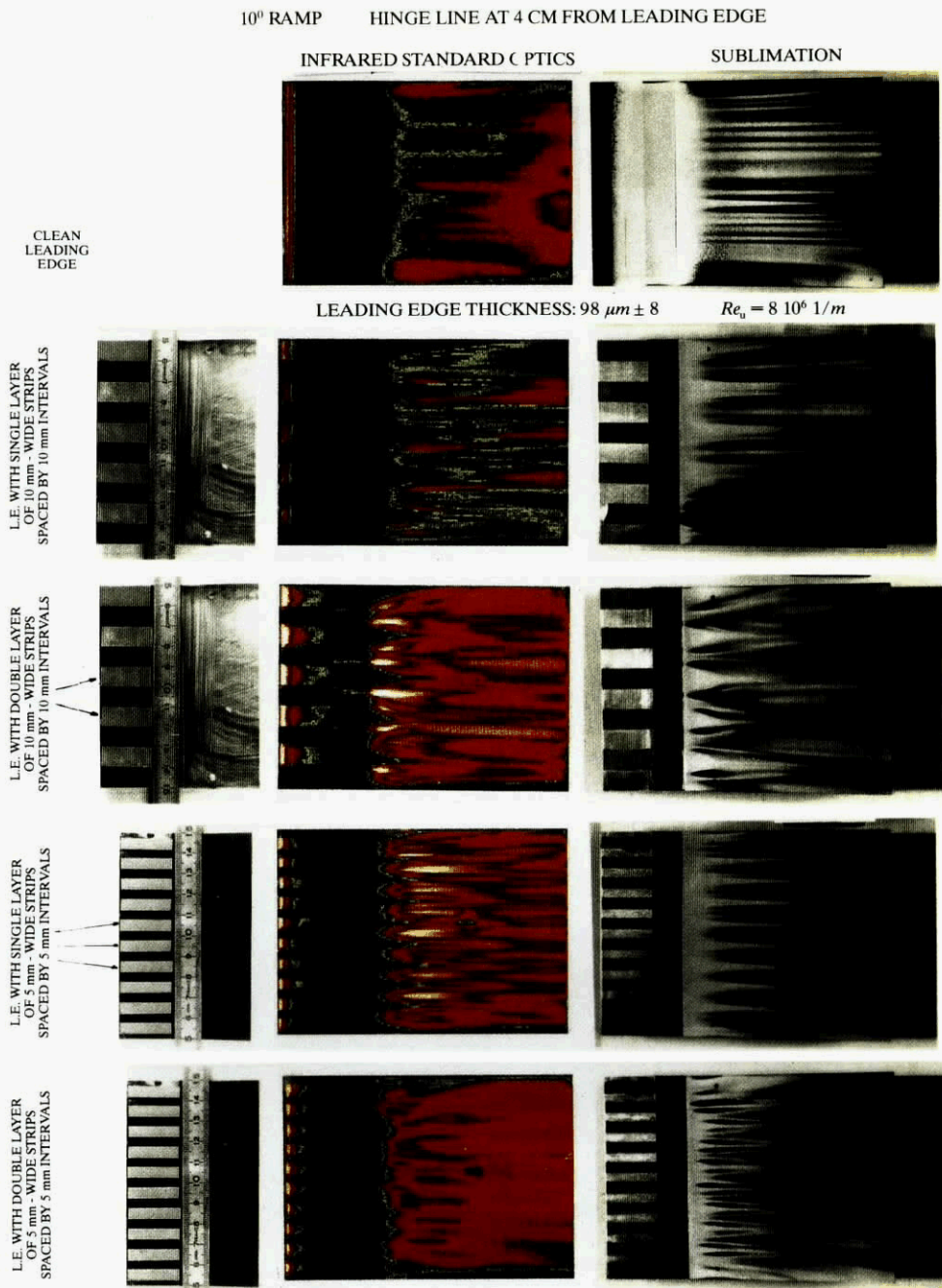
Fig. 27 - Infrared and sublimation observation of effect of leading edge perturbations on the formation of striations over a flat plate / 10^\circ ramp configuration at Mach 6 with Re_L=320,000 and T_w/T_0=0.6 [21,43]
