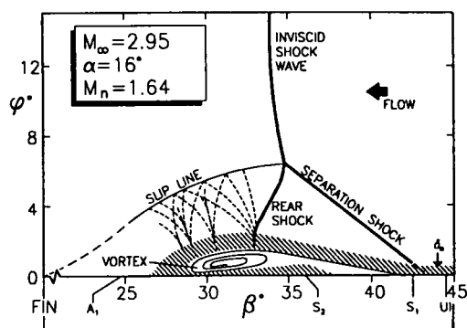
Fig. 49: Swept shock wave/turbulent boundary layer structure (after [4])
