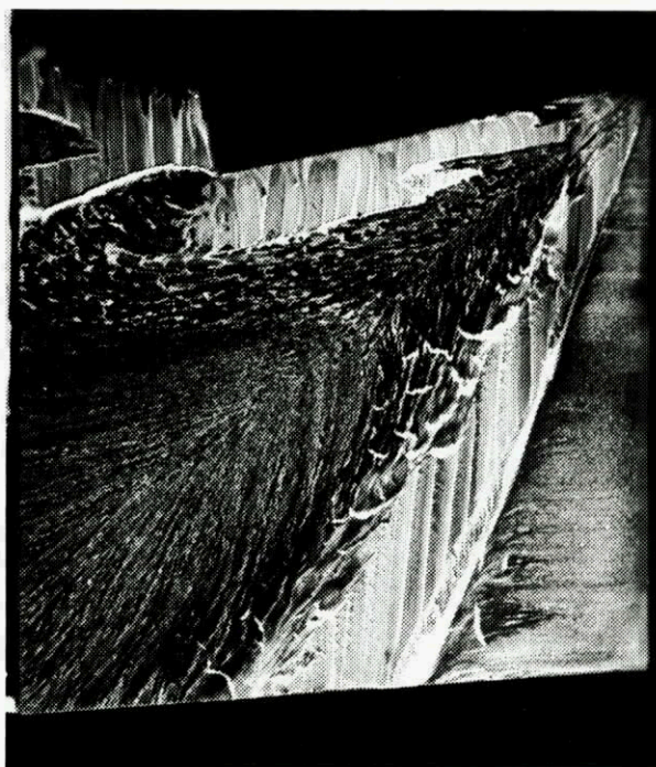
Fig. 15: Surface flow visualization, M = 2 , unswept shock generator, \alpha = 15^\circ
