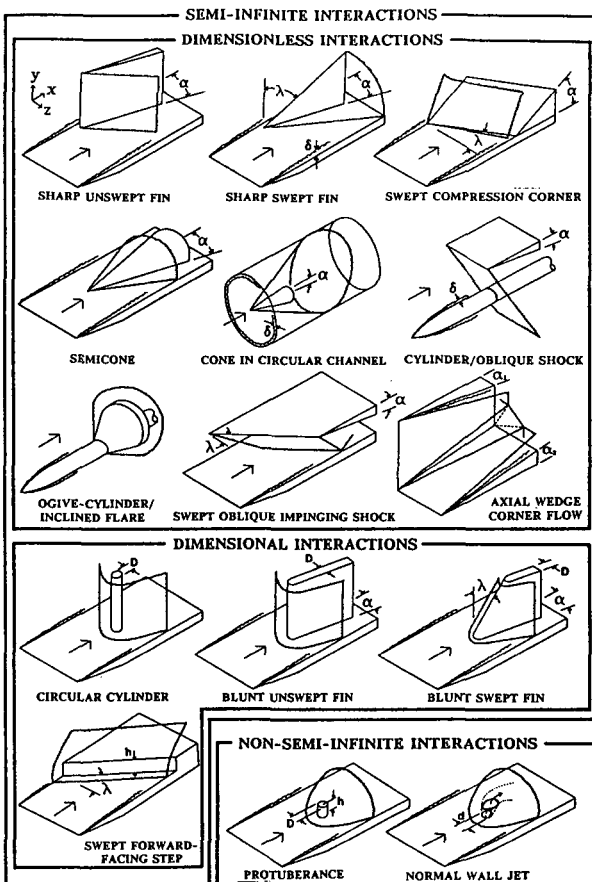
Fig. 3 - Interaction Classifications.
