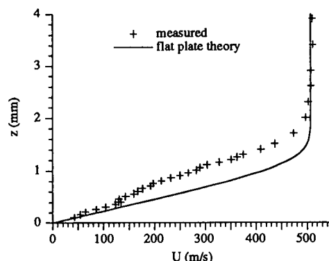
Fig. 30: Velocity profile at y/x = 1.4
