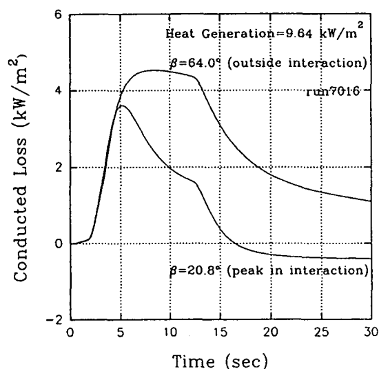
Fig. 49 - Comparison of Conduction Loss Calculations for Mach 4, \alpha = 16^\circ Interaction.
