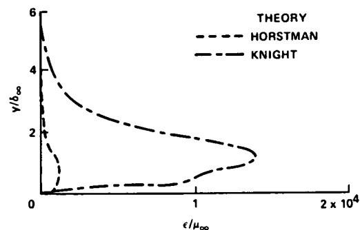
Figure 18: Turbulent eddy viscosity for sharp fin at M_\infty = 3.0, Re_{\delta_\infty} = 9.0 \times 10^5, \alpha = 20^\circ
