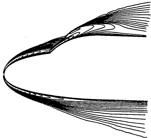
Fig. 59 - Temperature contours over double ellipsoid configuration at zero angle of attack, Mach 6.6 - equilibrium gas computation [111]
