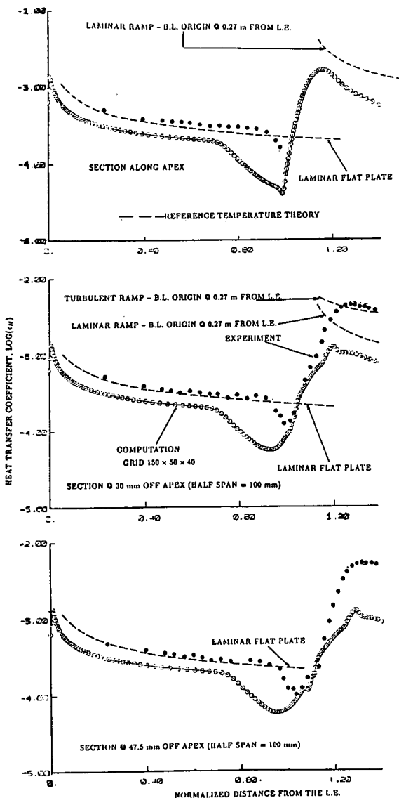
Fig. 52 - Comparison of measured and computed (laminar) heat transfer distributions over a flat plate / 30° swept, 15° ramp configuration at Mach 10, with Re_{apex} = 2.1 \times 10^6 and T_w/T_0 = 0.26 [94,99]
