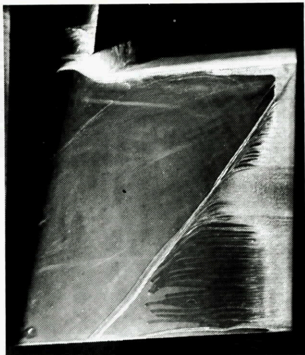
Fig. 14: Surface flow visualization, M = 2 , evidence of primary separation
