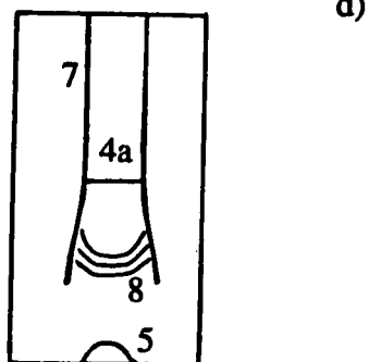
Figure 61: Shock structure for crossing shock at M_\infty = 8.3 , Re_{\delta_\infty} = 1.7 \times 10^5 , \alpha = 15^\circ
