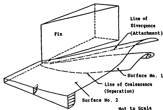
Figure 20: Entrainment into vortex for sharp fin
