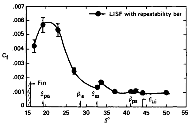
Fig. 13 - Skin Friction Coefficient vs. \beta for Mach 4, \alpha = 16^\circ Interaction.
