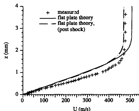
Fig. 34: Velocity profile at y/x = 0.38
