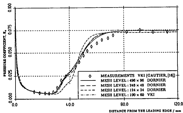
Fig. 39 - Comparison of measured and computed pressure distributions over a flat plate / 7.5° ramp configuration at Mach 6 with Re_L = 400,000 and adiabatic wall temperature [78]
