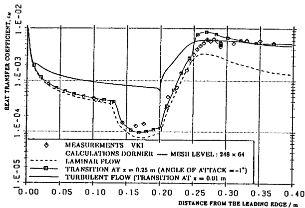
Fig. 48 - Comparison of measured and computed heat transfer distributions over the flat plate / rear 15° ramp configuration at Mach 14.1 with Re_L = 1.3 \times 10^6 and T_w/T_0=0.12 - laminar, turbulent and transitional computations with turbulence model "switched-on" at reattachment [75,78]
