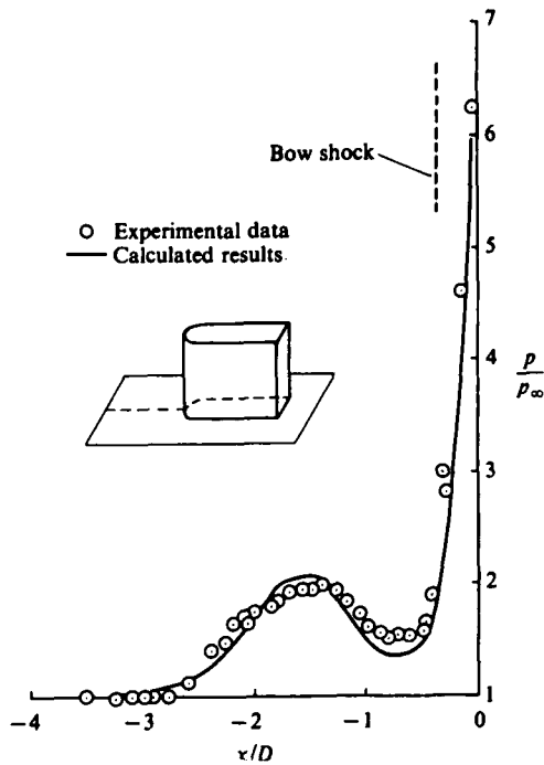
Figure 24: Static pressure for blunt fin on centerline
