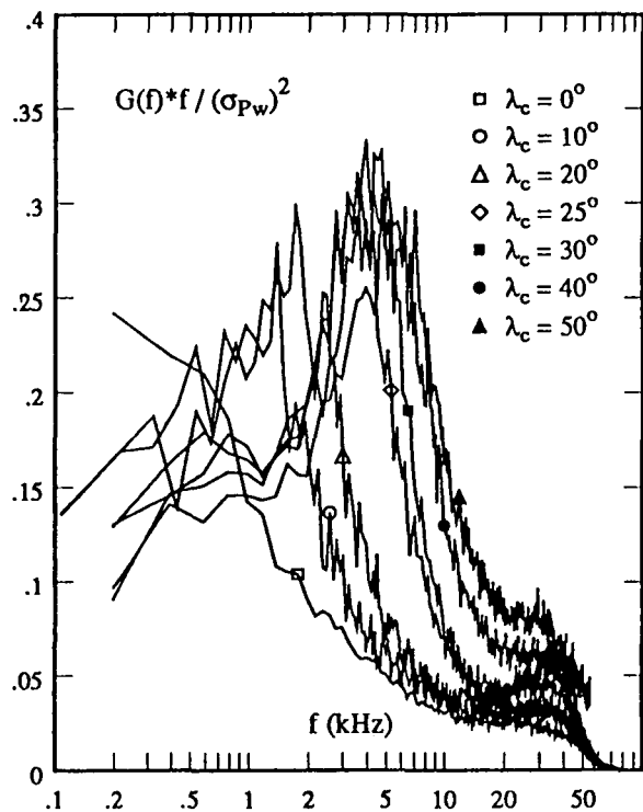
Fig. 20. Power spectra at position of maximum rms near separation in unswept and swept compression ramp interactions (from Dolling & Erenil, 1992).
