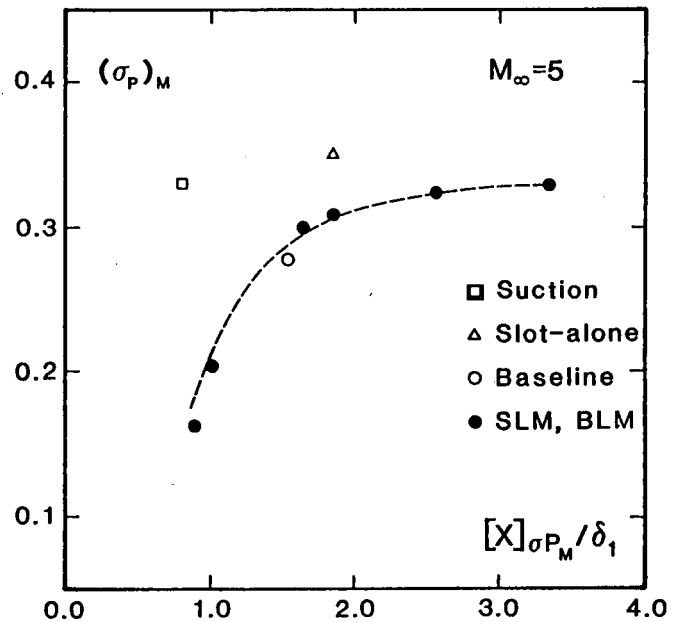
Fig. 11. Variation of (\sigma p)_{\max} with separated flow length in a Mach 5 compression ramp flow.
