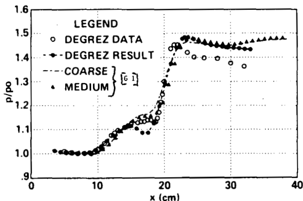
Fig. 47: Comparison of computed [61, 30] and measured [28] pressure distribution on flat plate ( y = 5 \text{ cm} ) in fin-type configuration ( \delta = 6^\circ , M_\infty = 2.25 , Re_{xF} = 1.08 \cdot 10^5 )
