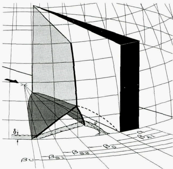
Fig. 17 - Projection of Quasiconical Interaction Flowfield onto Spherical Polar Coordinate Surface.
