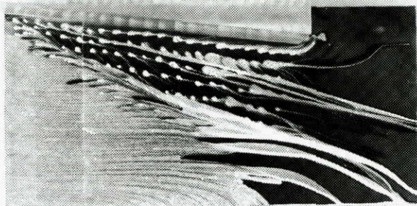
Fig. 20: Mixed surface flow visualization, M = 6 , unswept shock generator, \alpha = 6^\circ
