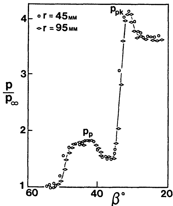
Fig. 5 - Surface Pressure Distributions (per Ref. 16).
