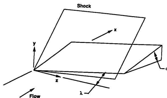
Figure 31: Geometry for swept compression corner
