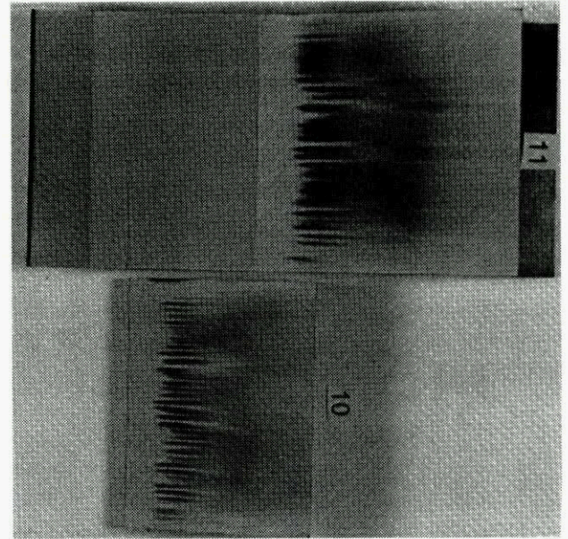
Fig. 24 - Oil flow [41] (Mach 10) and sublimation [43] (Mach 6) surface visualization of streamwise striations
