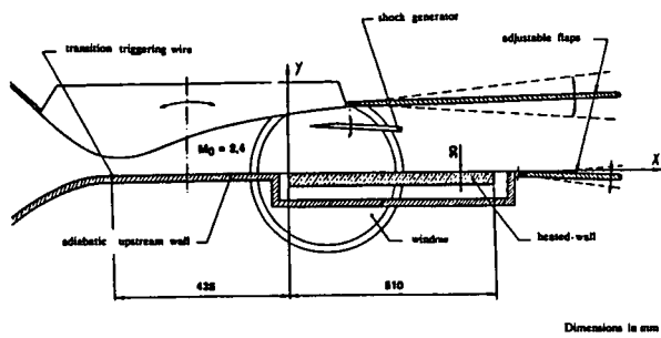
Fig. 23 - 2D supersonic flow. Test arrangement
