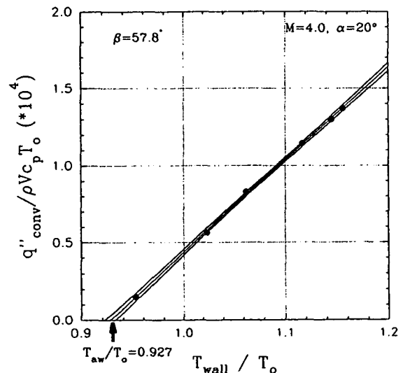
Fig. 46 - Example of the Determination of Adiabatic Wall Temperature.
