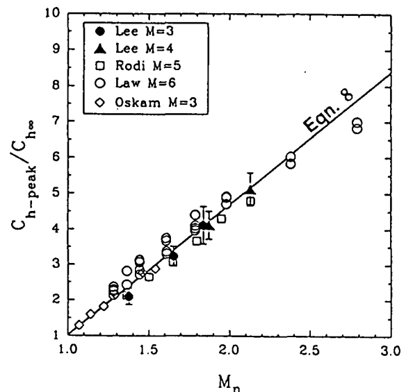
Fig. 12 - Interaction Peak Heating Correlation (per Lee et al. ).
