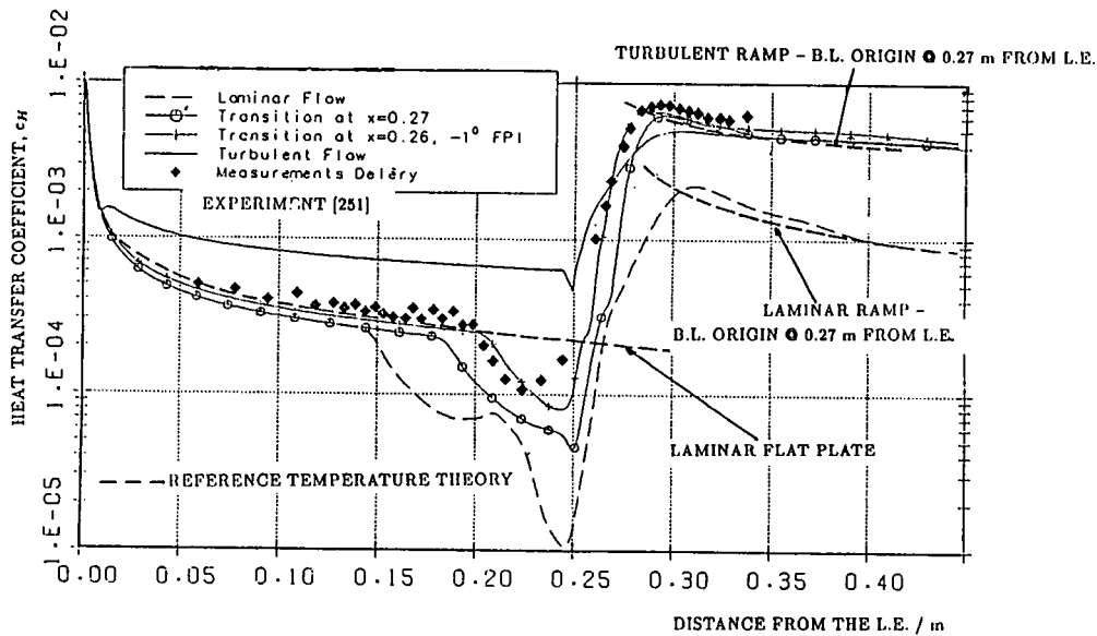
Fig. 47 - Comparison of measured and computed heat transfer distributions over the flat plate / rear 15° ramp configuration at Mach 10 with Re_L = 2.1 \times 10^6 and T_w/T_0=0.26 - laminar, turbulent and transitional computations with turbulence model "switched-on" at reattachment [88]
