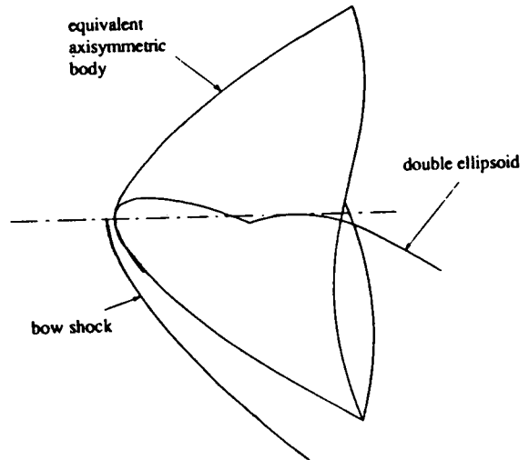
Fig. 53 - Schematic representation of the definition of the axisymmetric equivalent of a configuration at angle of attack
