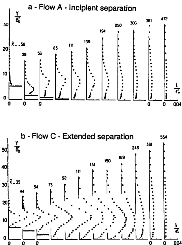
Fig. 6 - 2D transonic flow. Turbulence kinetic energy profiles
