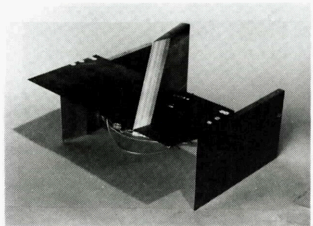
Fig. 10: Asymmetric dihedron model
