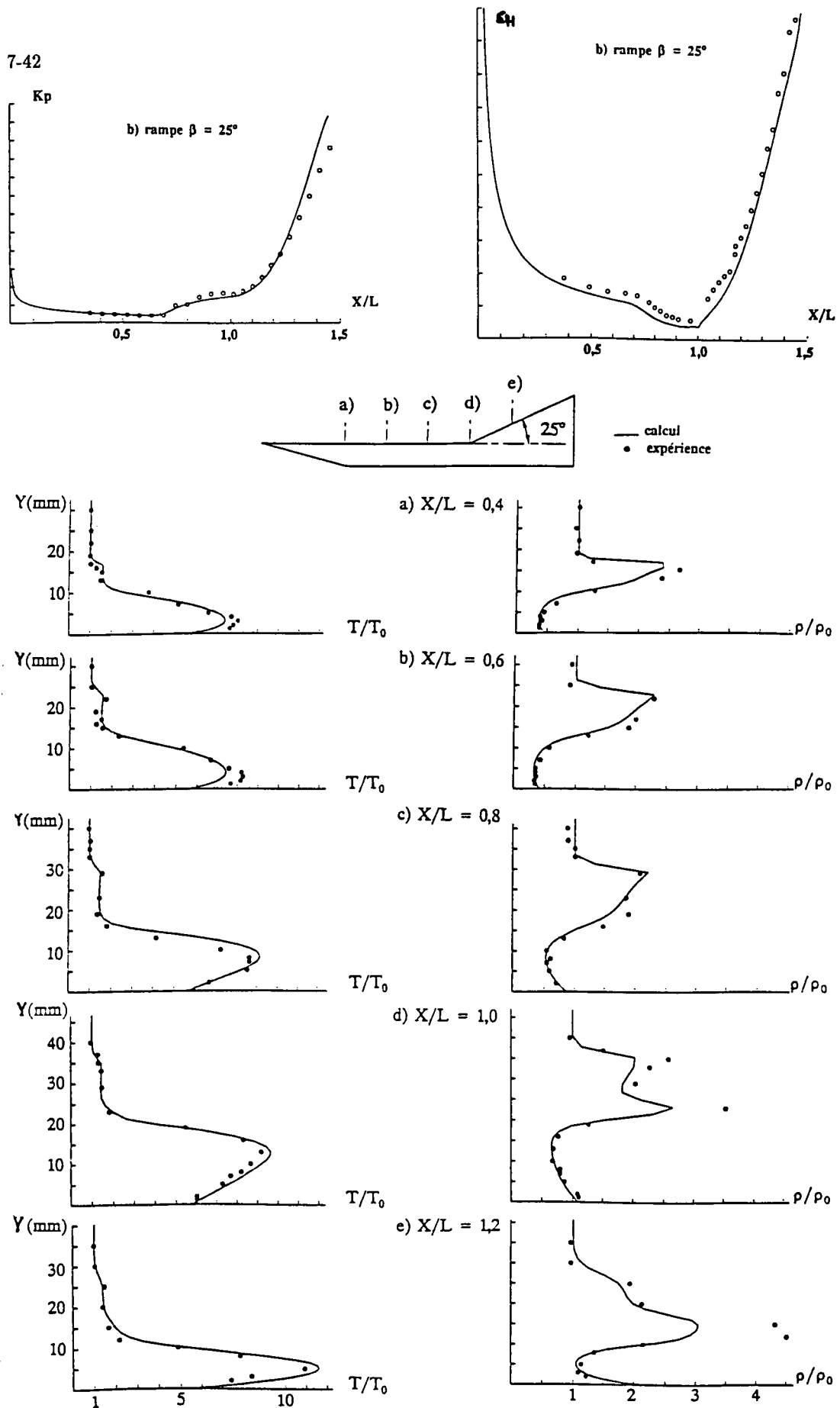
Fig. 42 - Comparison of measured and computed pressure and heat transfer distributions, and temperature and density profiles over a flat plate / 25° ramp configuration at Mach 10 with Re_L=30,000 [85]
