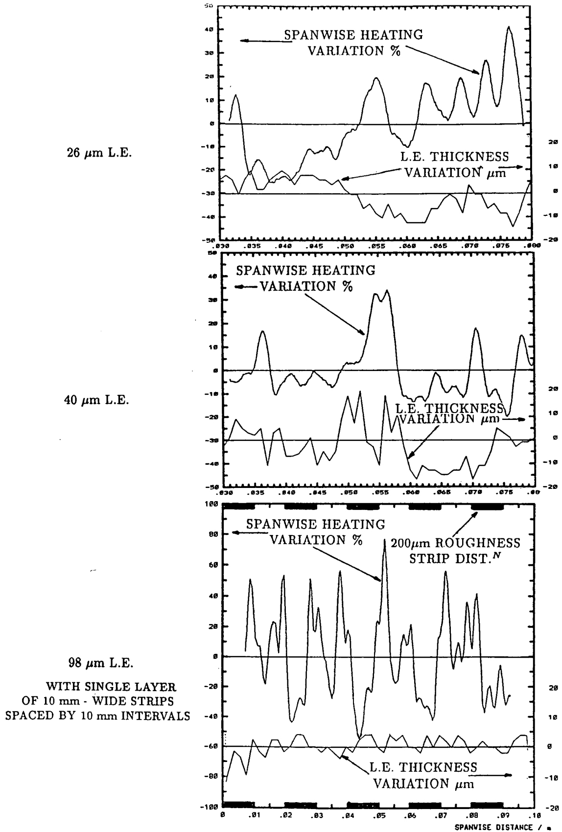
Fig. 31 - Effect of model leading edge thickness and/or disturbance distribution on spanwise heat transfer distribution on 10° deflected ramp at Mach 6, Re_L = 320,000 [21,43]
