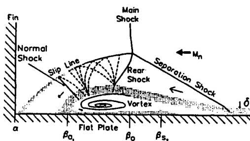
Figure 19: Quasi-conical flowfield model for single fin [1]
