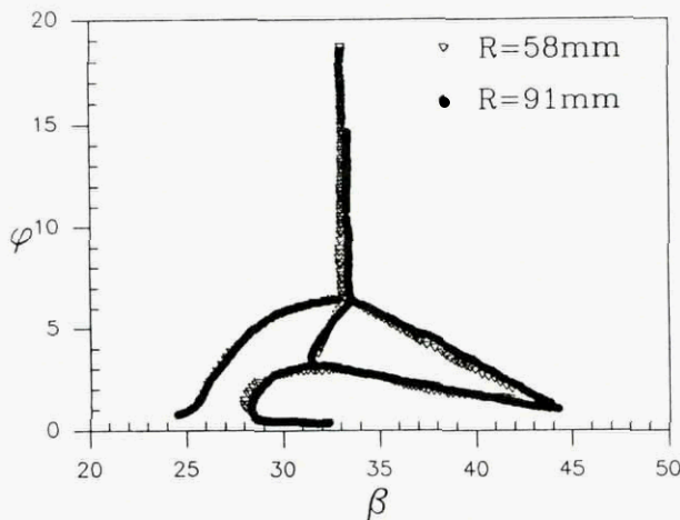
Fig. 23 - Overlay of PLS Cuts at Different Locations.
