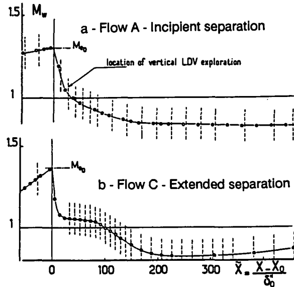
Fig. 3 - 2D transonic flow. "Wall" Mach number distributions
