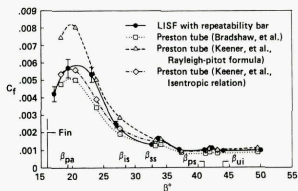
Fig. 41 - Comparison of LISF and Preston Tube c_f .
