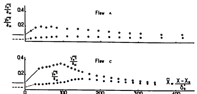
Fig. 9 - 2D transonic flow. Variation of maximum turbulence intensities
