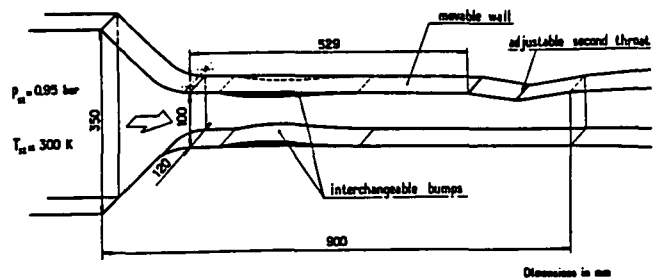
Fig. 2 - Arrangement of the two-dimensional transonic channel
