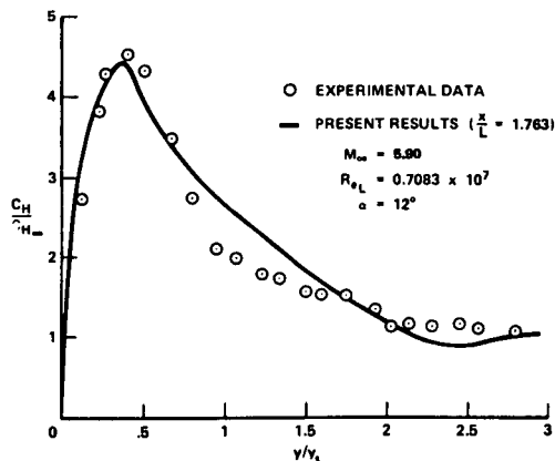
Figure 9: Heat transfer for sharp fin at M_\infty = 5.9, \alpha = 12^\circ, Re_{\delta_\infty} = 1.3 \times 10^5
