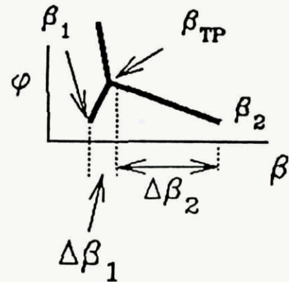
Fig. 28 - Flowfield Diagram Defining \Delta\beta_1 and \Delta\beta_2 .
