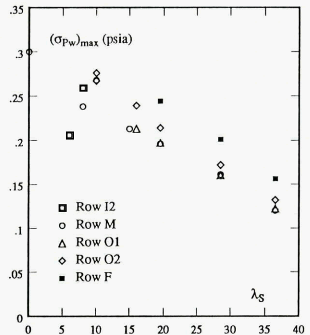
Fig. 18. Maximum rms level near separation in Mach 5 swept compression ramp interactions as a function of separation line sweepback (from Erenkil & Dolling, 1992).
