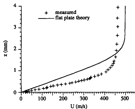
Fig. 33: Velocity profile at y/x = 0.5
