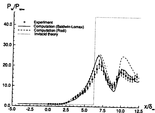
Figure 50: Surface pressure for crossing shock at M_\infty = 8.3 , \alpha = 15^\circ , Re_{\delta_\infty} = 1.7 \times 10^5
