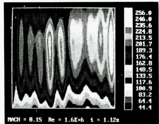
Fig. 25 - Thermosensitive paint [59] (Mach 10) and infrared [60] (Mach 8.15) visualization of streamwise striations
