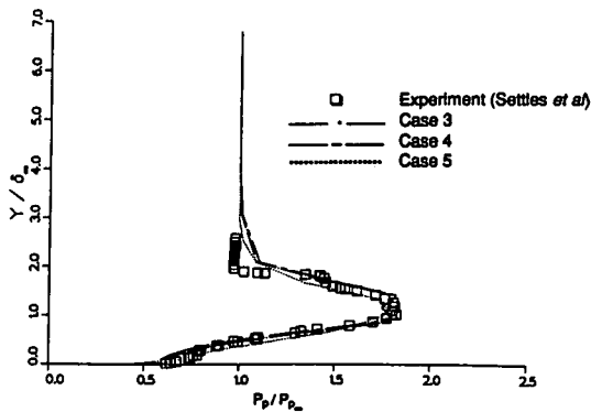
Figure 35: Pitot pressure for swept compression corner for \alpha = 20^\circ and \lambda = 40^\circ
