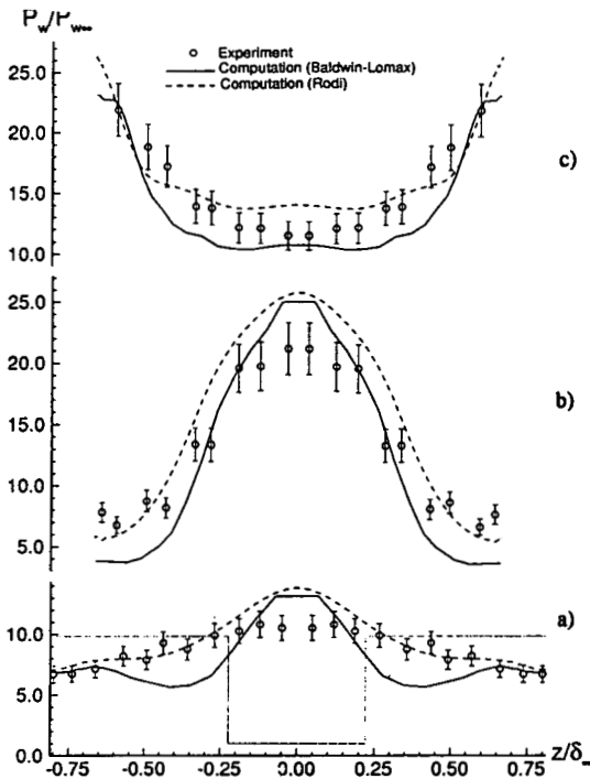
Figure 52: Surface pressure for crossing shock at M_\infty = 8.3, \alpha = 15^\circ, Re_{\delta_\infty} = 1.7 \times 10^5
