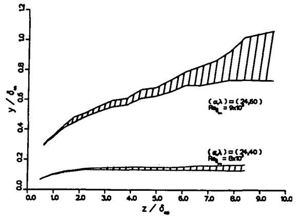
Figure 43: Height of entrainment surface for swept compression corner
