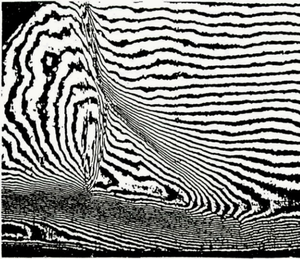
Fig. 26 - Conical Holographic Interferogram of Mach 3, \alpha = 10^\circ Interaction Structure.
