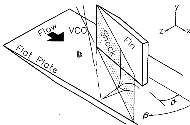
Fig. 1 - Sharp Fin Interaction Test Geometry.
