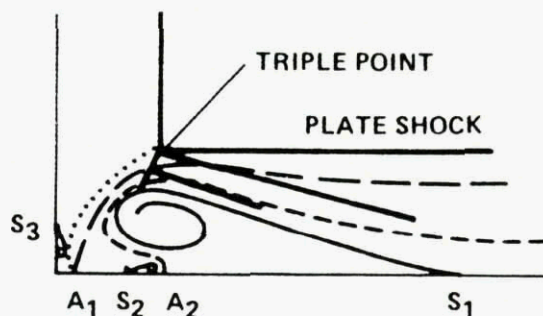
Fig. 8: Flow structure in intake-type configuration (from [20])
