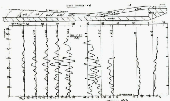
Fig. 28 - Streamwise evolution of spanwise pitot pressure distributions in the boundary / shear layer over a flat plate / 2D backward facing step configuration [52]
