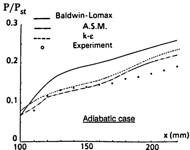
Fig. 30 - 2D supersonic flow. Wall pressure distributions. Interaction with separation.
