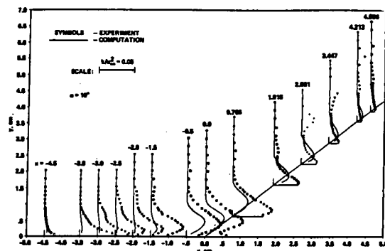
Figure 30: Turbulence kinetic energy for cylinder/flare
