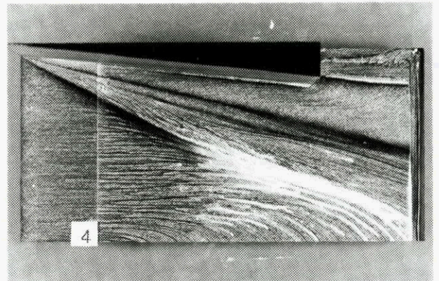
Fig. 19: Oil flow visualization, M = 6 , unswept shock generator, \alpha = 6^\circ
