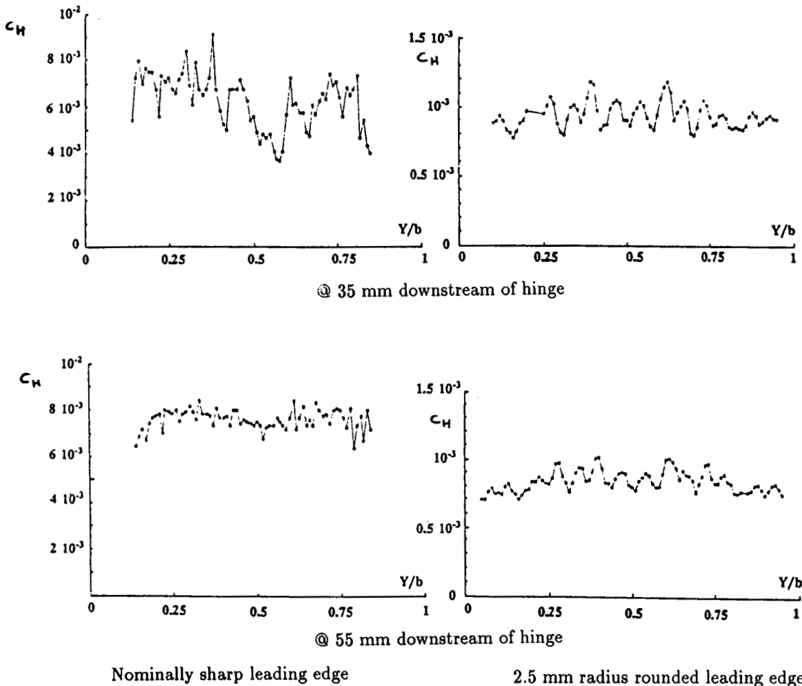
Fig. 33 - Spanwise heat transfer distributions on 15^\circ ramp at Mach 10, Re_L = 2.1 \times 10^6 [41,59]
