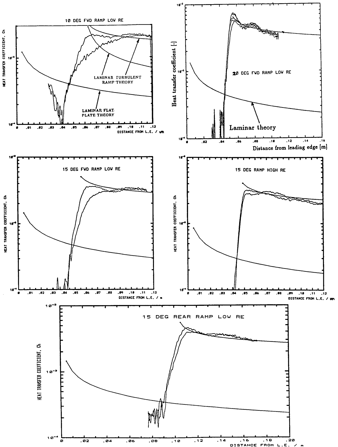
Fig. 35 - Minimum and maximum streamwise heat transfer distributions along flat plate / 2D ramp configurations at Mach 6 - effect of unit Reynolds number, ramp deflection and location (40 \mu m leading edge) [21,43]
