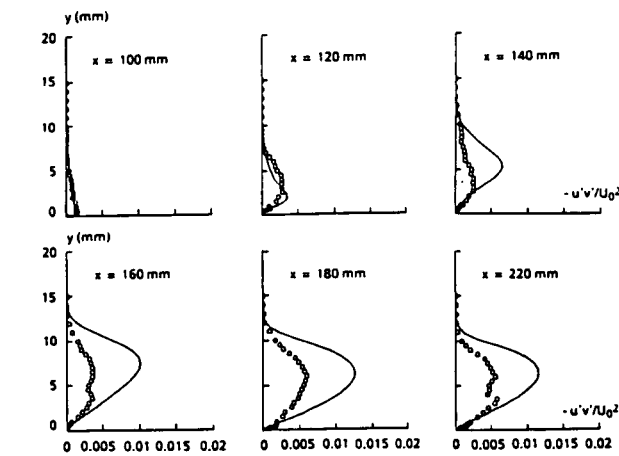
Fig. 35 - Shear tension distribution. T_{xy}/T_\infty = 1 , (k-\epsilon) model.
