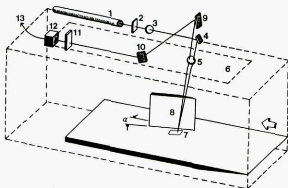
Fig. 38 - Diagram of LISF Meter
