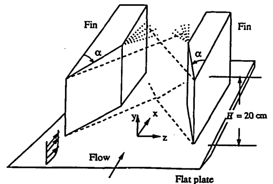
Figure 44: Geometry of crossing shock
