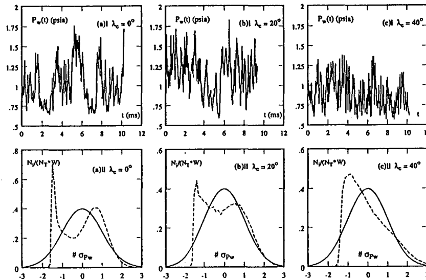
Fig. 19. Sample wall pressure signals and corresponding probability density distributions in unswept and swept compression ramp interactions (from Erenil & Dolling, 1992).
