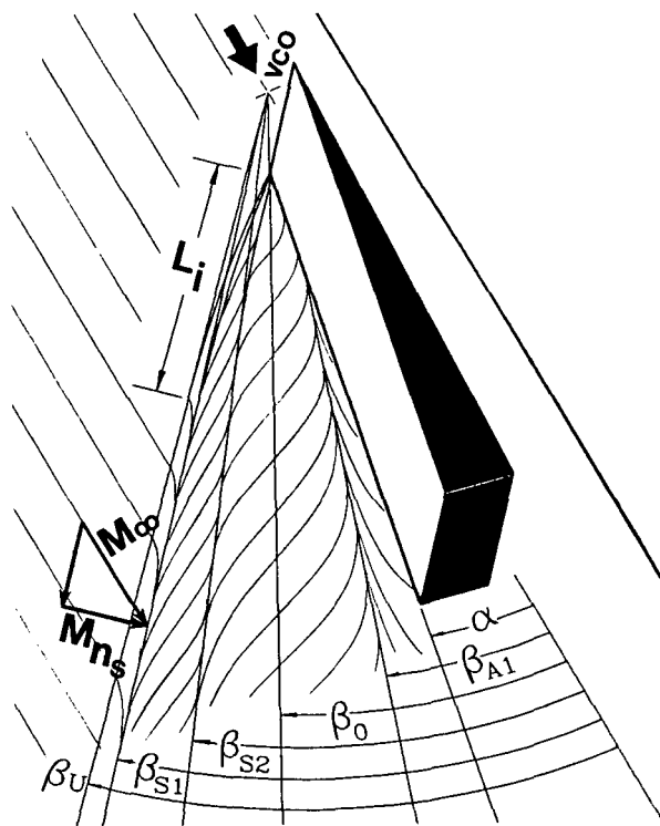
Fig. 4 - Sketch of Sharp Fin Interaction Footprint with Nomenclature Definitions.
