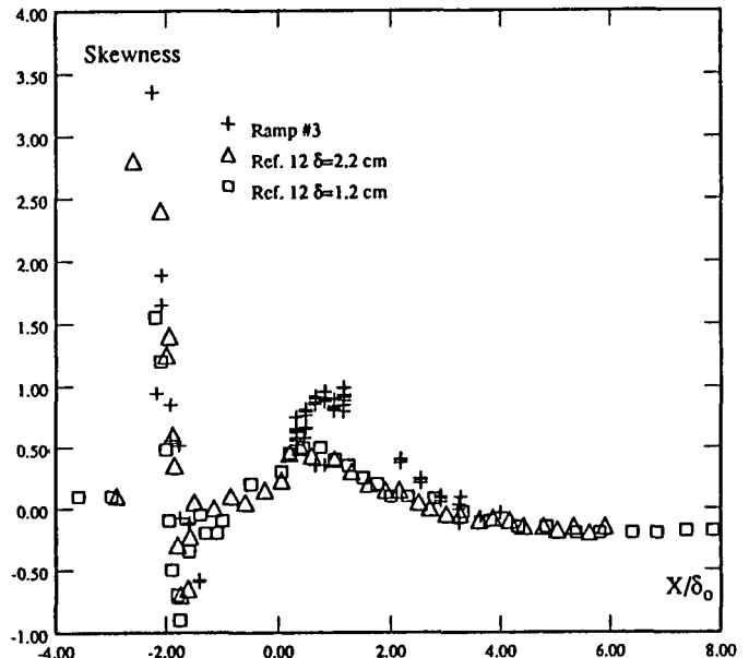
Fig. 14. Skewness coefficient distributions in Mach 5 and Mach 3 compression ramp interactions (from Gramann, 1989).
