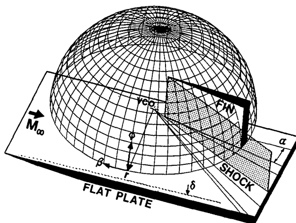
Fig. 2 - Spherical Polar Coordinate System.
