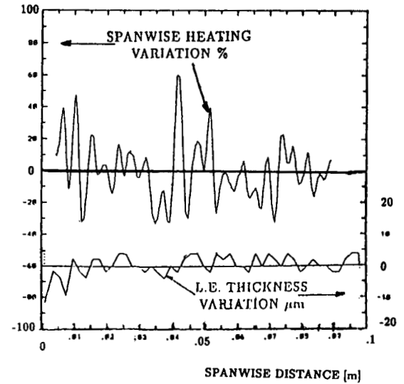
Fig. 34 - Spanwise heat transfer distribution over 10^\circ ramp at Mach 6, Re_L = 320,000 from thermogram of Fig. 27 ( 98 \mu\text{m} clean leading edge) [57]
