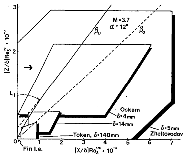
Fig. 14 - Plot of Dimensionless Interaction Footprint Showing Measurement Zones of Various Studies.
