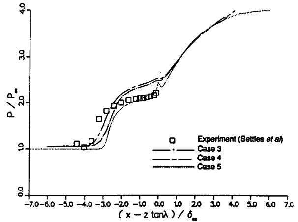
Figure 32: Surface pressure for swept compression corner for \alpha = 20^\circ and \lambda = 40^\circ
