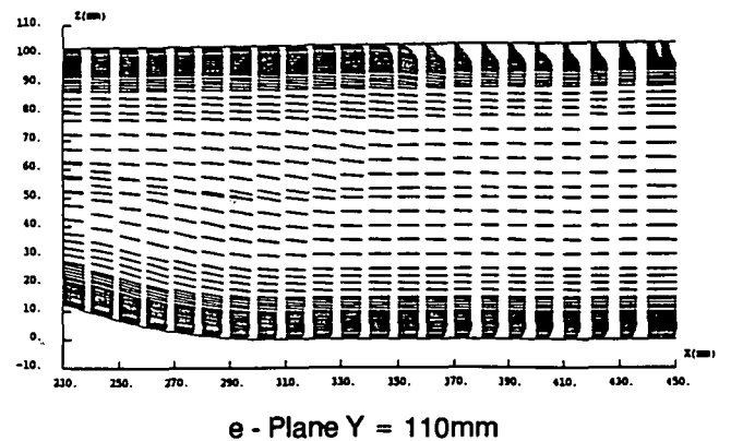
Fig. 42 - 3D transonic flow. Mean velocity field in longitudinal planes
