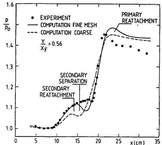
Fig. 44: Comparison of computed [30] and measured [28] pressure distribution on flat plate ( y = 5 cm) in fin-type configuration ( \delta = 6^\circ , M_\infty = 2.25 , Re_{x_F} = 1.08 \cdot 10^5 )
