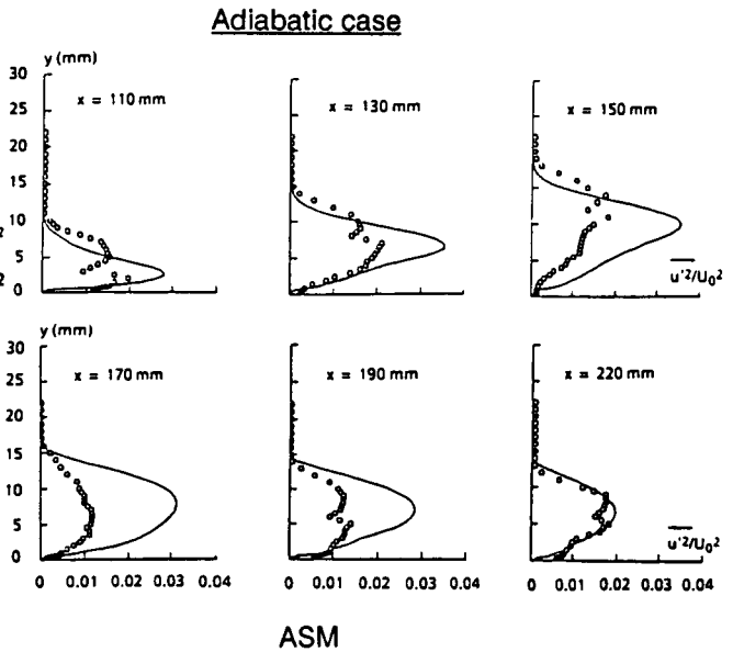
Fig. 33 - 2D supersonic flow. Normal stress profiles. Interaction with separation.
