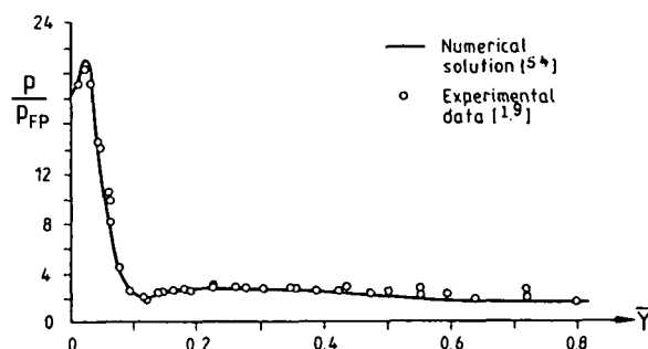
Fig. 40: Comparison of measured [19] and computed [54] pressure distribution on flat plate in intake configuration ( \delta_w = 15^\circ , M_\infty = 12.5 )
