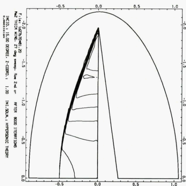
Fig. 12: Inviscid flow over asymmetric dihedron : pressure contours in crossflow plane
