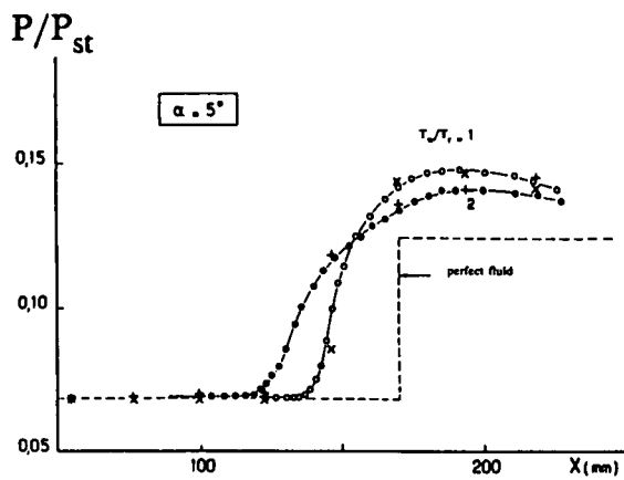
Fig. 24 - 2D supersonic flow. Wall pressure distributions. Interaction without separation
