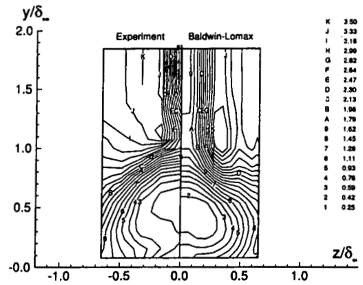
Figure 53: Pitot pressure for crossing shock at M_\infty = 8.3, \alpha = 15^\circ, Re_{\delta_\infty} = 1.7 \times 10^5, x = 5.6\delta_\infty , Baldwin-Lomax model
