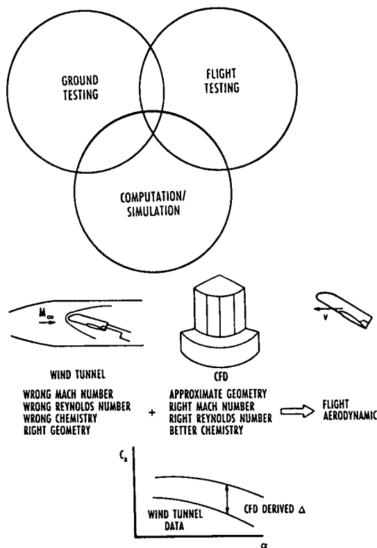
Fig. 37 - Integration of ground testing, computations and flight [68]
