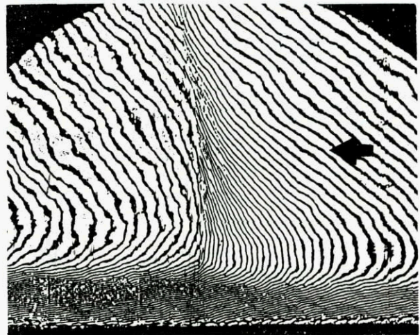
Fig. 25 - Conical Holographic Interferogram of Mach 2.35, \alpha = 7^\circ Interaction Structure.
