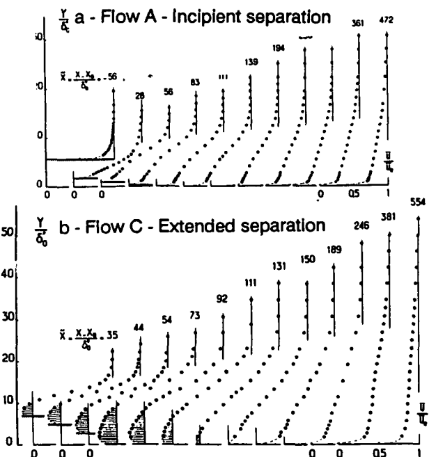
Fig. 4 - 2D transonic flow. Mean streamwise velocity profiles
