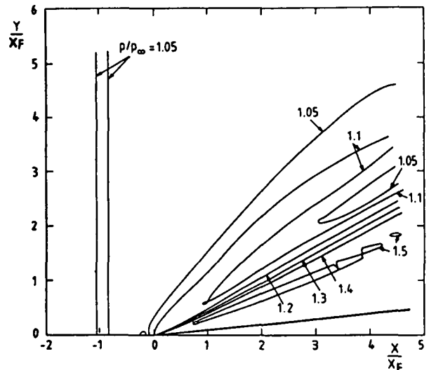
Fig. 43: Computed [30] pressure contours on flat plate in fin-type configuration ( \delta = 6^\circ , M_\infty = 2.25 , Re_{x_F} = 1.08 \cdot 10^5 )
