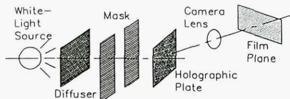
Fig. 33 - White-Light Hologram Reconstruction Setup.
