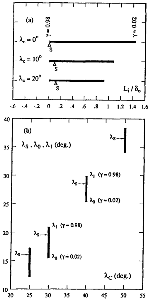
Fig. 21. Variation of intermittent region length and relative location of the separation line with ramp sweepback angle a) unswayed and moderately swept flow, and b) conically-symmetric (i.e., highly swept) flow.
