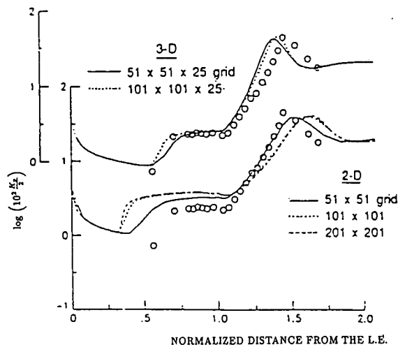
Fig. 41 - Comparison of measured and computed pressure distributions over a flat plate / 24° ramp configuration at Mach 14.1 with Re_L = 105,000 and T_w/T_0 = 0.1 [79]
