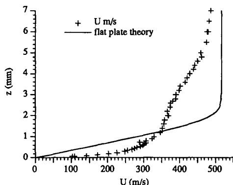
Fig. 32: Velocity profile at y/x = 0.65
