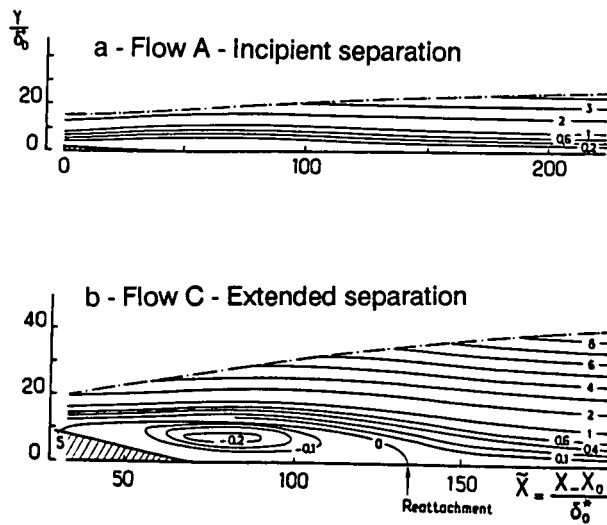
Fig. 5 - 2D transonic flow. Mean flow streamlines
