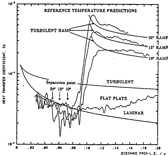
Fig. 17 - Heat transfer distributions over flat plate and flat plate / 2D ramp configurations at Mach 6 with Re_L=720,000 and T_w/T_0=0.6 [21,43]
