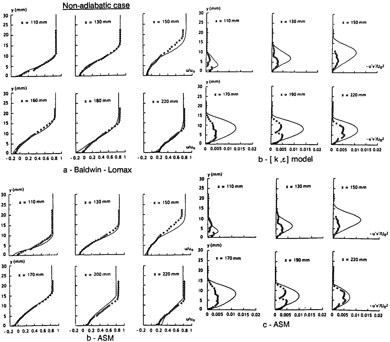
Fig. 36 - 2D supersonic flow. Shear stress profiles. Interaction with separation.
