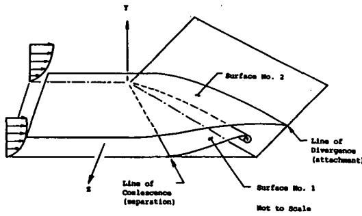
Figure 42: Flowfield model for swept compression corner
