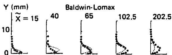
Fig. 15 - 2D transonic flow. Flow A. Shear stress profiles. Equilibrium models
