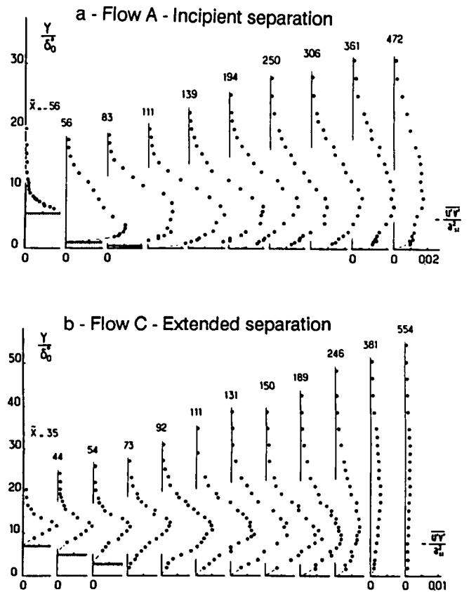
Fig. 7 - 2D transonic flow. Shear stress profiles
