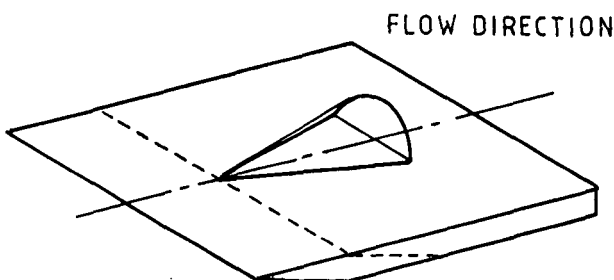
Fig. 4: Half circular cone shock generator
