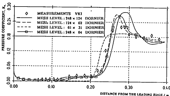
Fig. 49 - Comparison of measured and computed (laminar) pressure distributions over the flat plate / rear 15° ramp configuration at Mach 14.1 with Re_L = 1.3 \times 10^6 and T_w/T_0=0.12 - grid dependence study [78]
