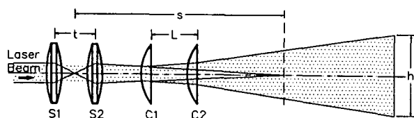
Fig. 36 - Diagram of Laser Sheet Generator (per J. T. Kegelman).
