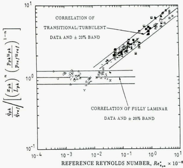
Fig. 23 - Correlation of laminar and turbulent peak heating data referenced to laminar flat plate heating level [21,43]
