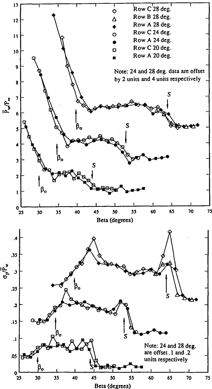
Fig. 22. Mean and rms pressure distributions in glancing shock interactions at Mach 5 (from Schmisser, 1992).
