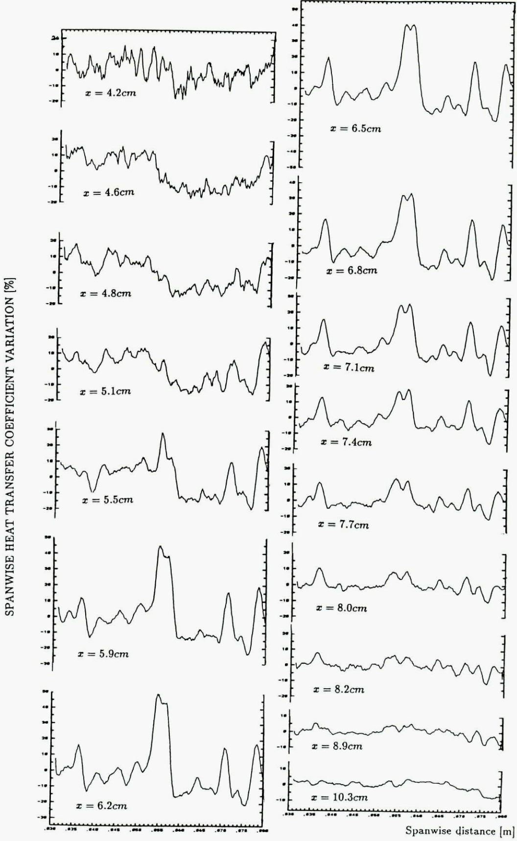
Fig. 30 - Streamwise evolution of spanwise heat transfer distribution over a 10° ramp configuration at Mach 6, Re_L=320,000 from thermogram of Fig. 26b (40 \mu m leading edge) [21,43]
