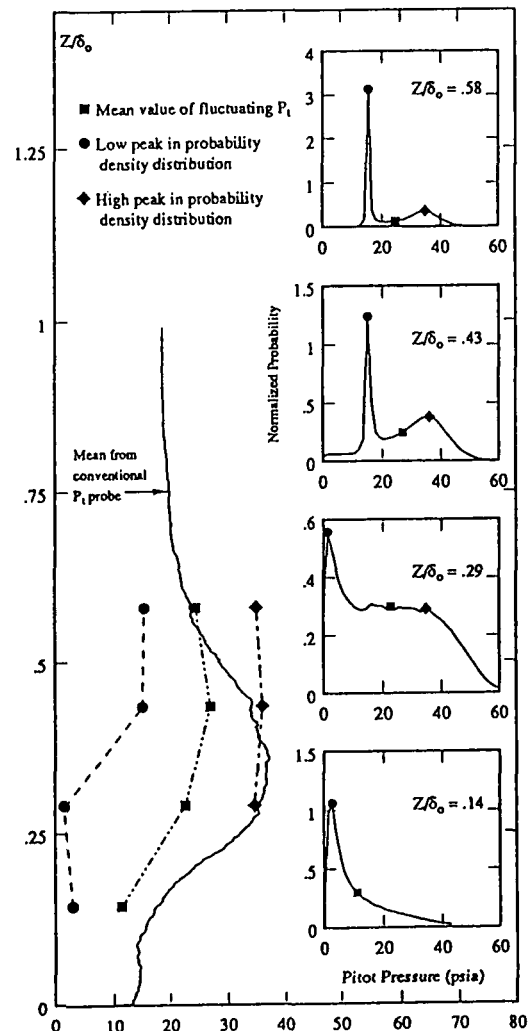
Fig. 49. Comparison of mean values from fluctuating and conventional mean pitot surveys [from McClure & Dolling (1991)].
