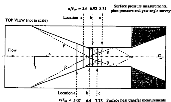
Figure 51: Geometry for crossing shock at Mach 8.3 and location of measurements. The boundary layer thickness \delta_\infty = 3.25 cm.
