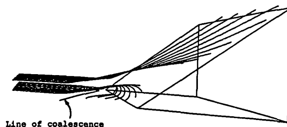
Figure 41: Streamlines for swept compression corner
