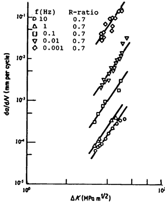
Fig 12 Effect of Frequency on crack growth in AP1 at 700 Deg.C
