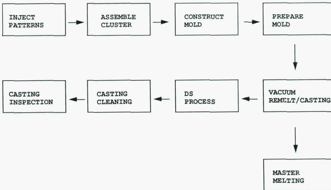
FIGURE 1: Basic steps for DS blade investment casting.
