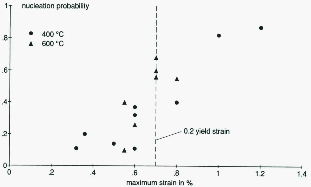
Fig. 11 : Probability of crack nucleation at inclusions
