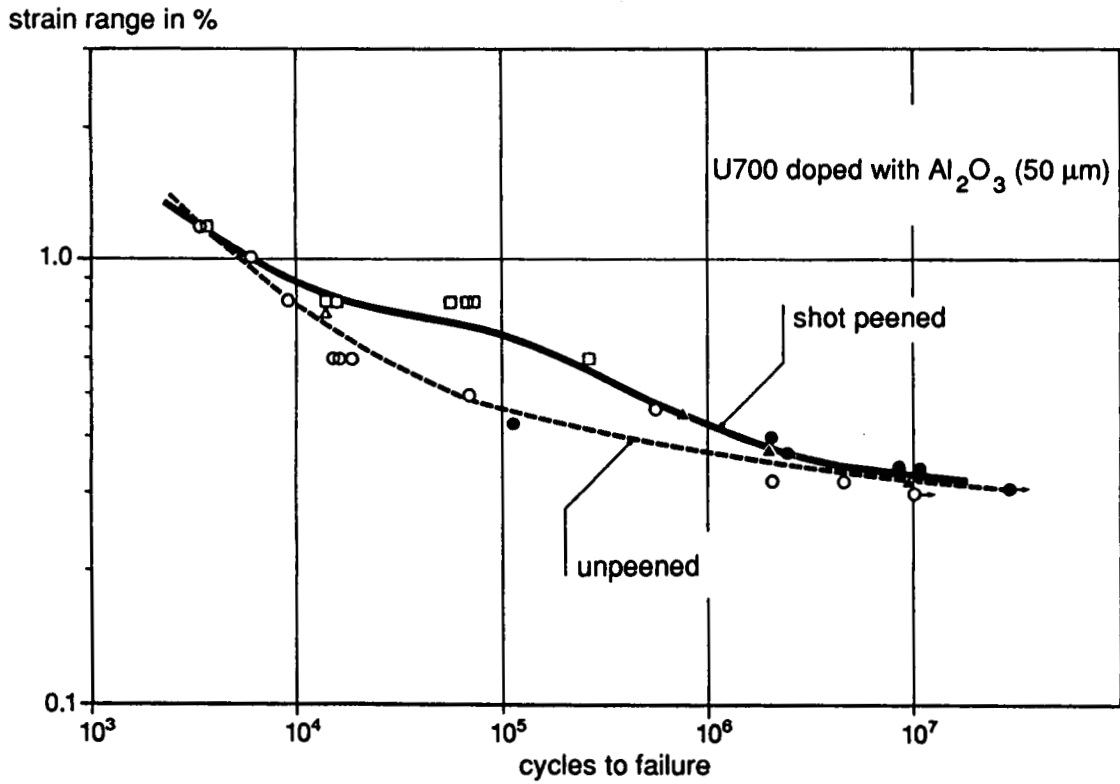
Fig. 15 : Influence of shot peening
