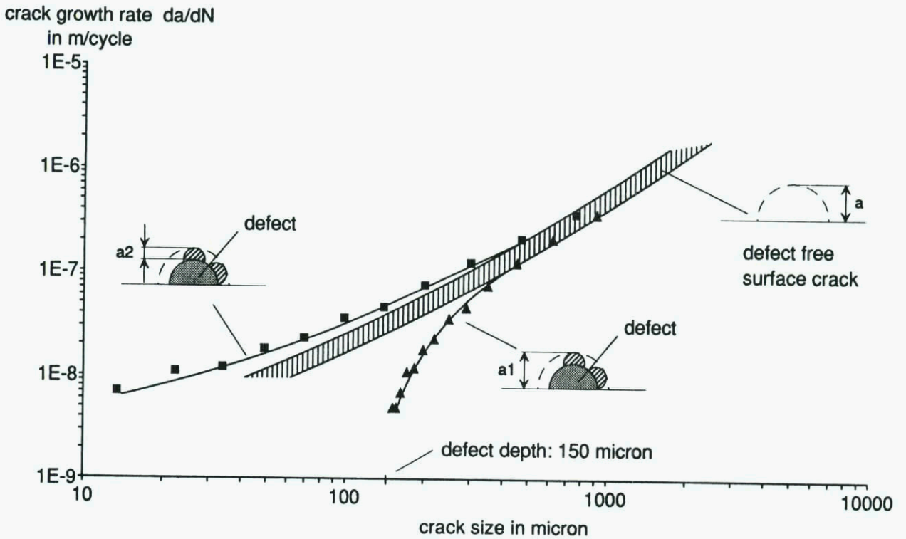
Fig. 7 : Behaviour of cracks starting from defects
