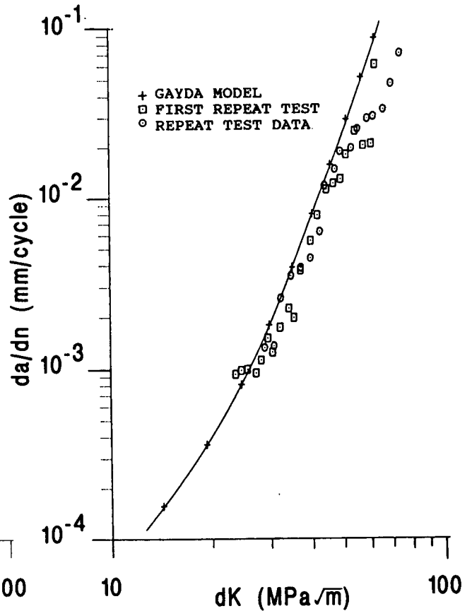
Fig 11 Comparison of predicted and experimental crack growth for Waspaloy at 650 Deg.C
