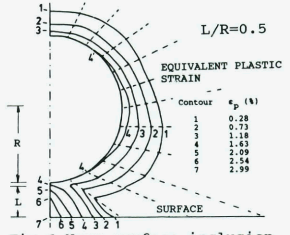
Fig 6 Near surface inclusion Residual strain field
