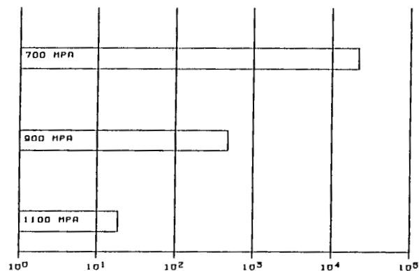
Fig. 8 Influence of the stress level on the ratio between SL and DT life.
