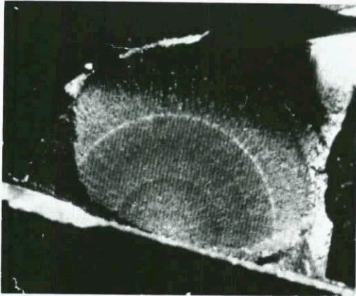
Fatigue crack : General view Final depth : 3.8 mm Final length : 6.2 mm
