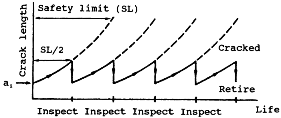
Fig 19 Schematic representation of Retirement for Cause inspection intervals
