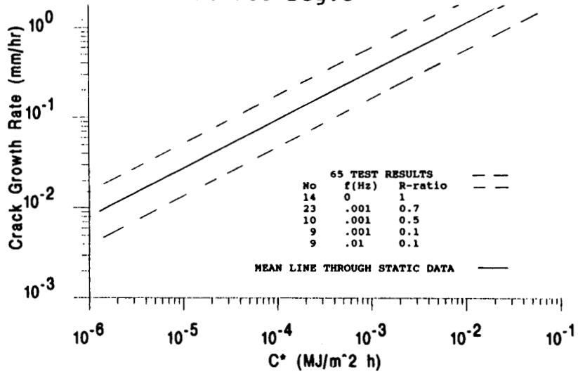
Fig 13 Sensitivity of crack growth rate to C* in AP1
