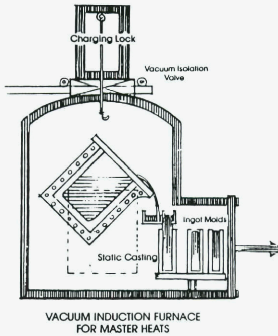
FIGURE 8: Vacuum Induction Melting Furnace.
