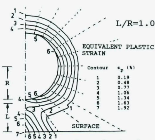
Fig 5 Near surface inclusion Residual strain field
