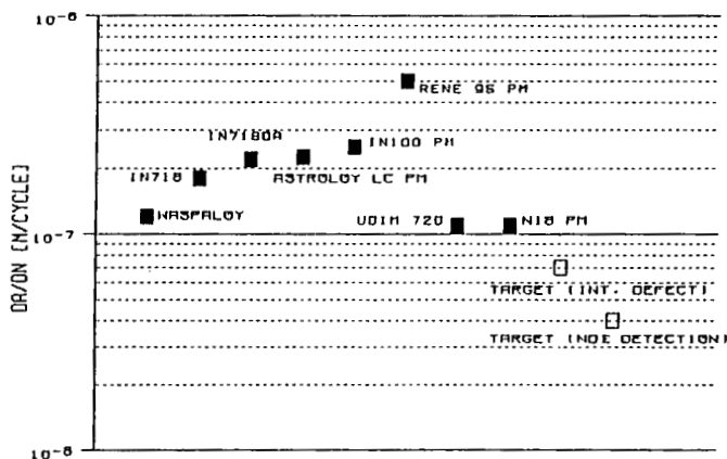
Fig. 10 Historical trend of disk alloy crack growth rates and targets to be assumed for future materials development.
