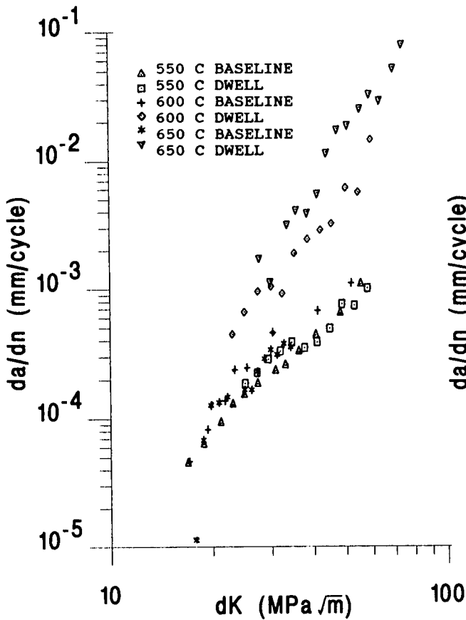
Fig 10 Base line (0.25 Hz) and 5 minute dwell crack growth in Waspaloy
