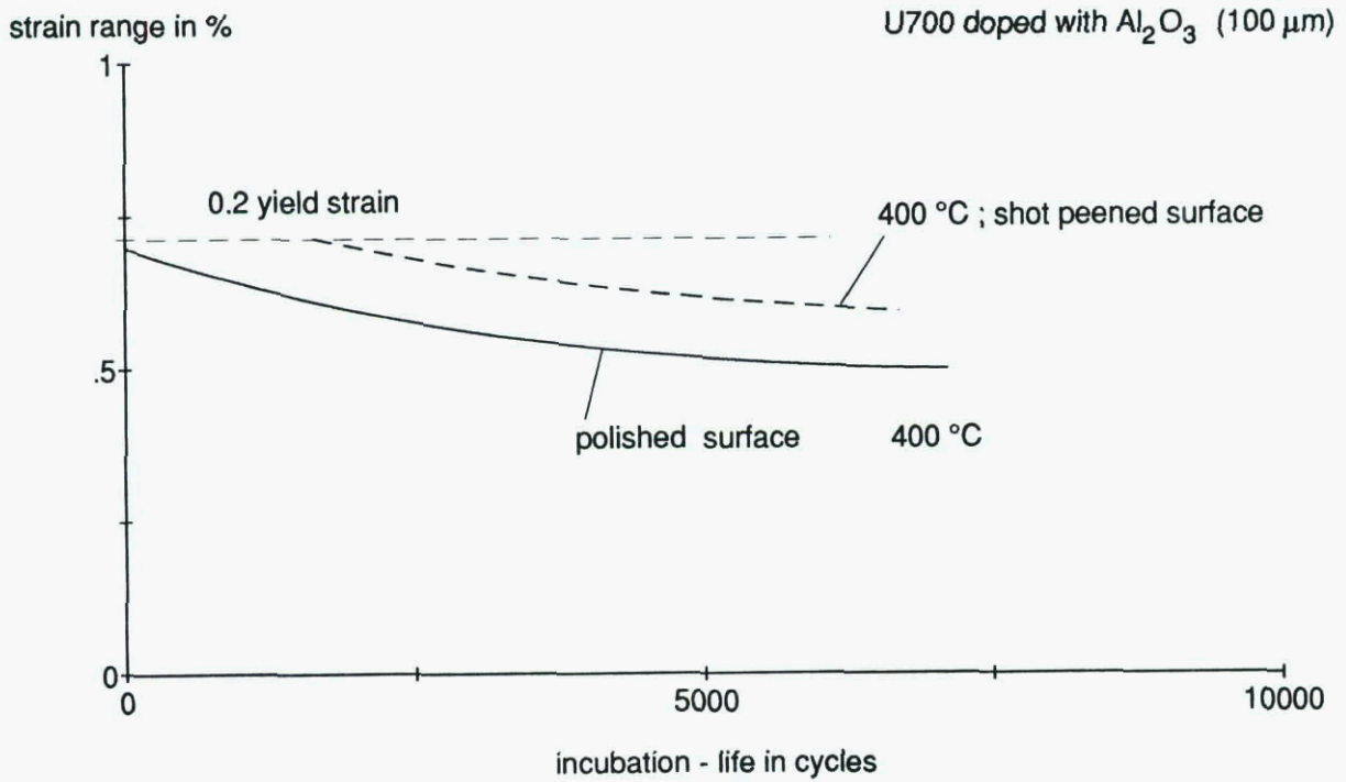
Fig. 9 : Strain dependent incubation - life
