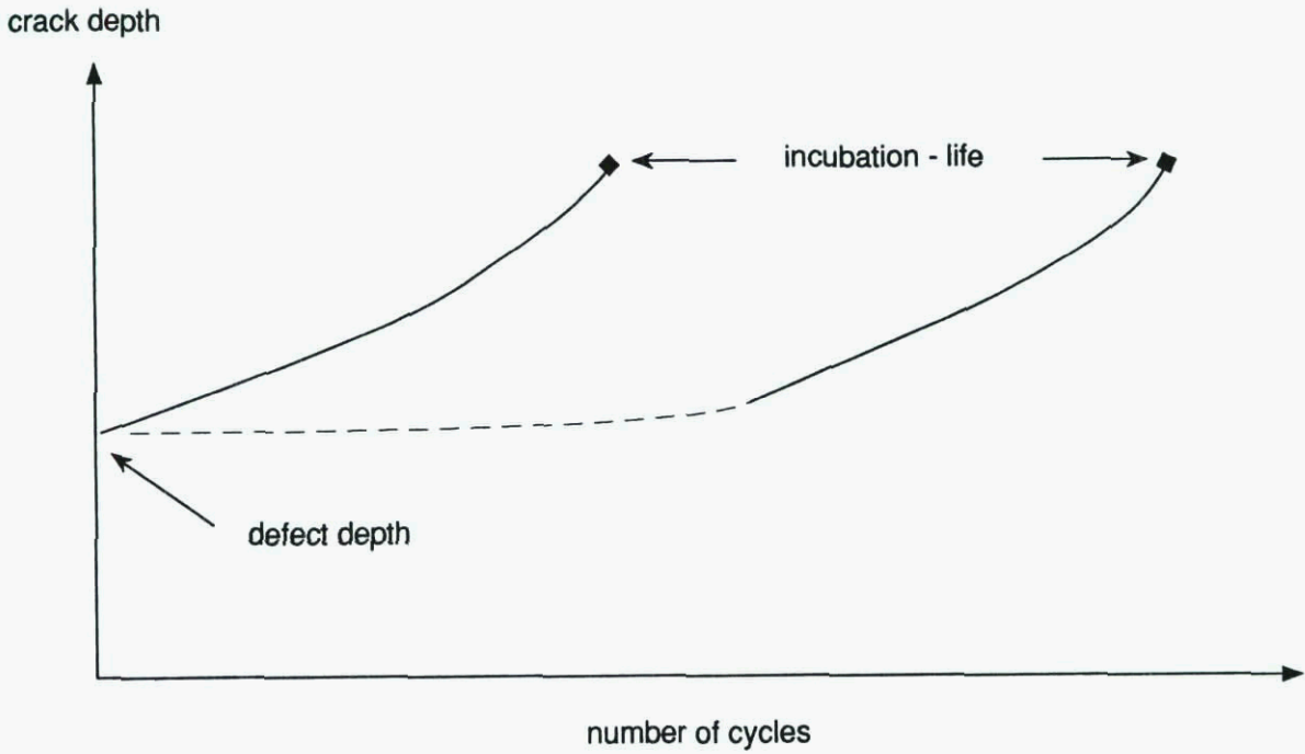
Fig. 8 : Definition of incubation - life
