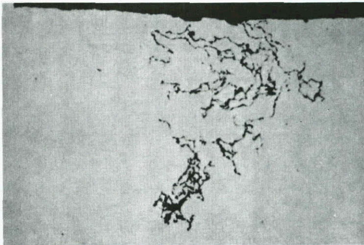
FIGURE 6: Lacy dross film penetrating casting surface. Mag 200X
