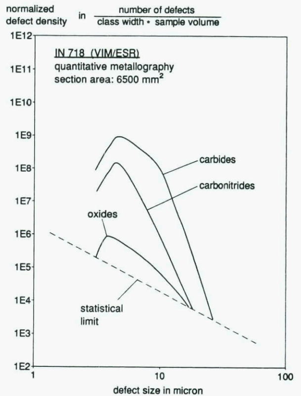
Fig. 3 : Density for various types of defects
