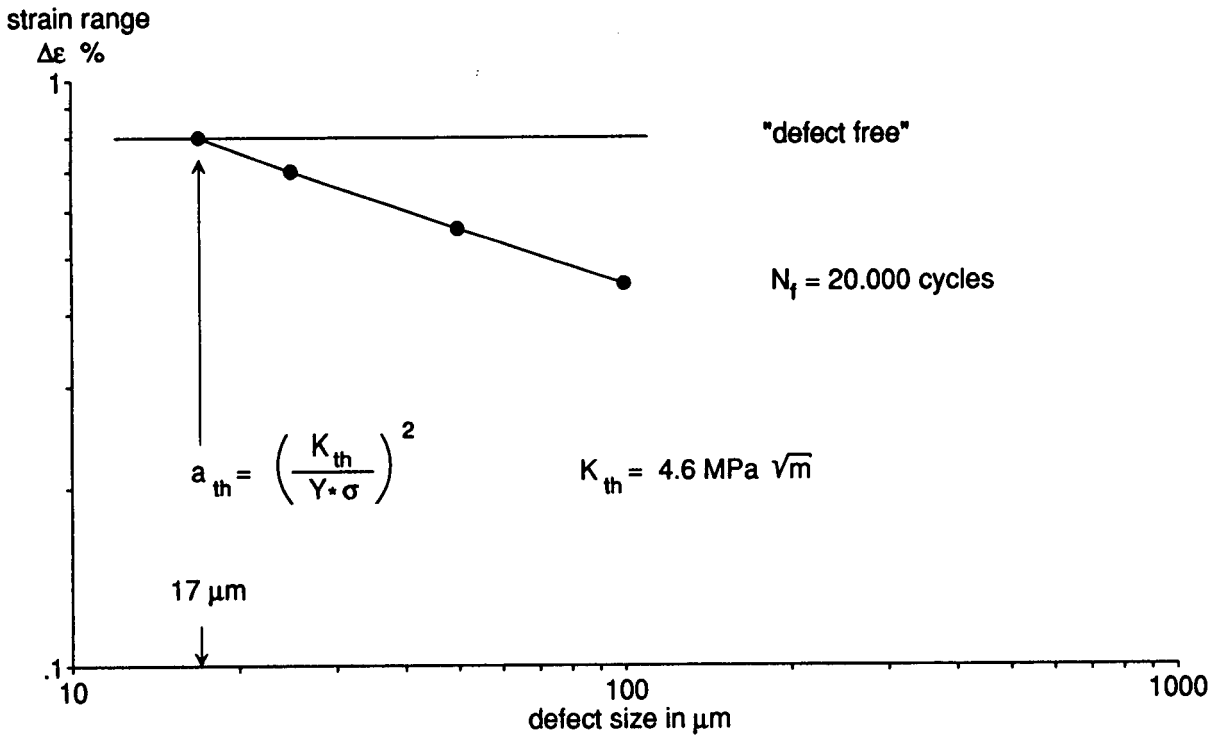
Fig. 12 : Defect size dependent threshold values
