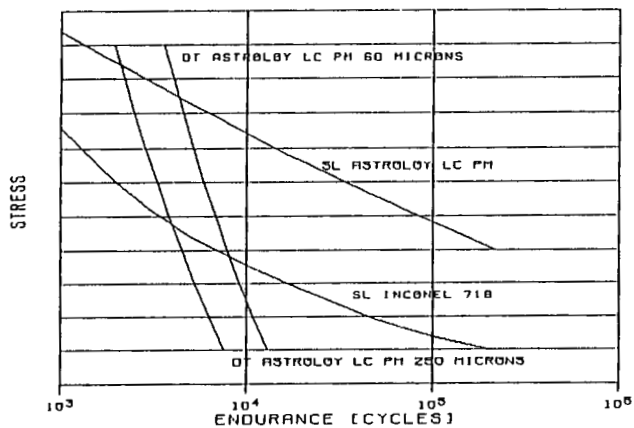
Fig. 5 Summary of LCF design curves for IN718 and Astroloy LC PM
