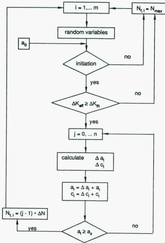
Fig. 2 : Simulation flow chart for the probabilistic living concept
