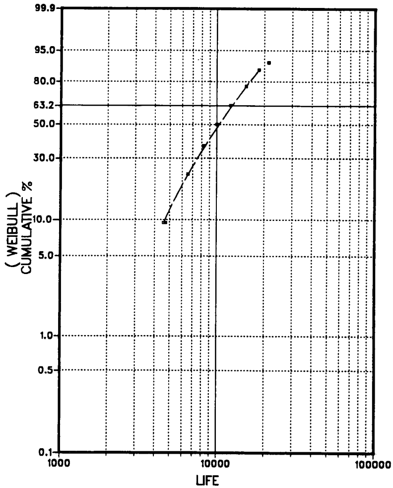
Figure 7: 3 Parameter Weibull CDF for Fatigue-type Data
