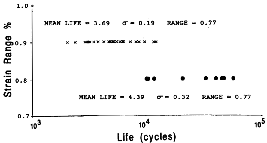
Fig 14 Fatigue scatter in AP1 under strain control cycling at 600 Deg.C
