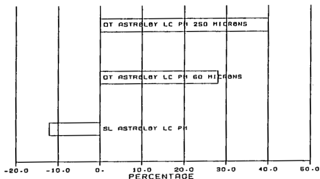
Fig. 7 Impact of lifing approach on the weight of an existing configuration disk (life as datum).
