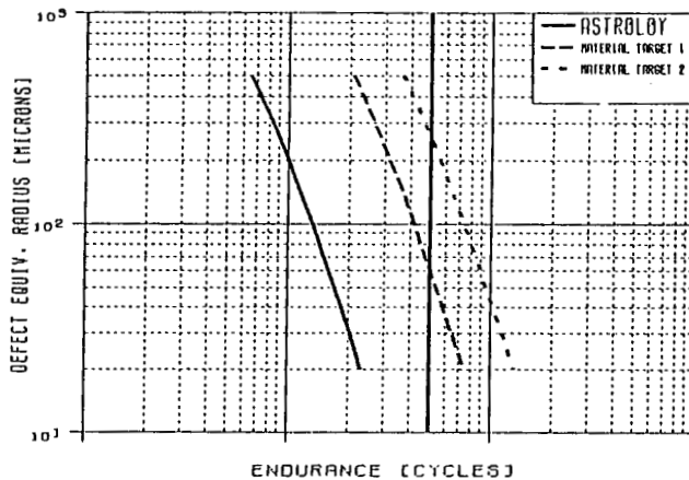
Fig. 9 Cyclic life target for future material development able to keep weight and life of current SL lived conventional disks.
