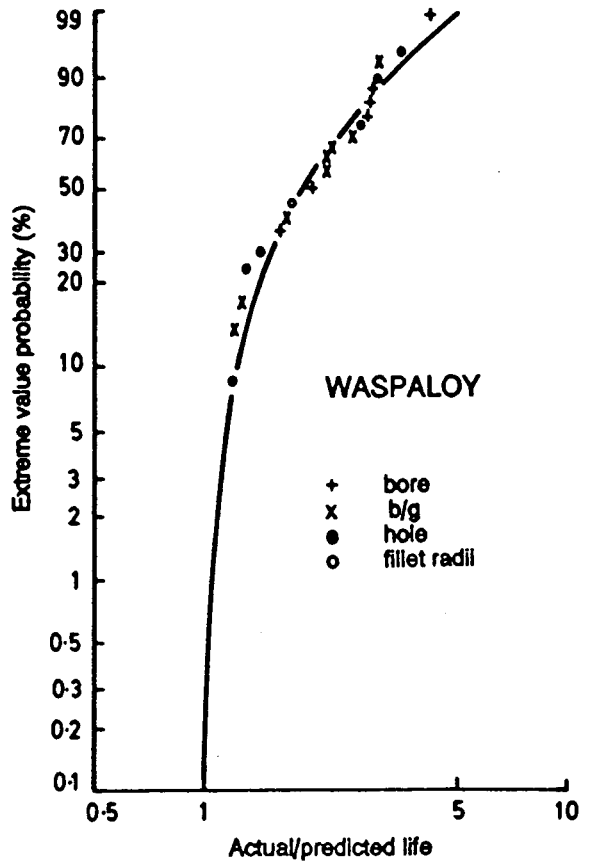
Fig 17 Comparison of actual and data base fatigue life predictions
