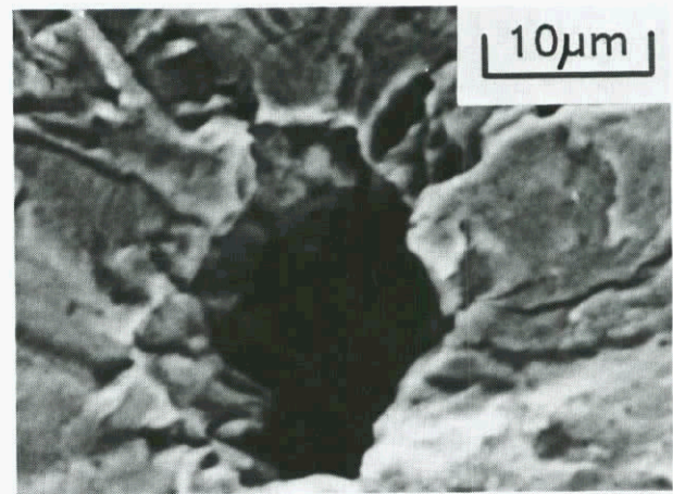
Fig 3 Failure site - Porosity
