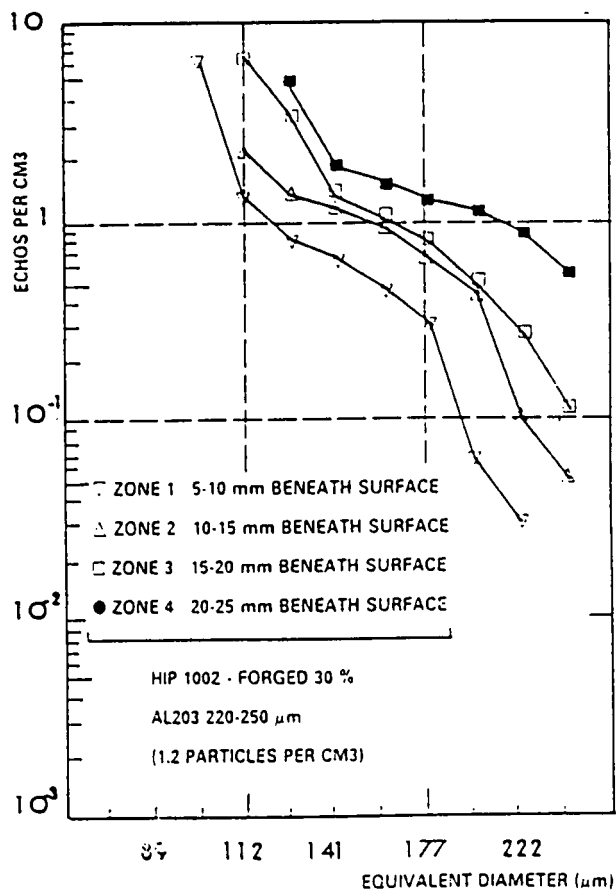
FIG. 5 Effect of zone position (forged 30%)
