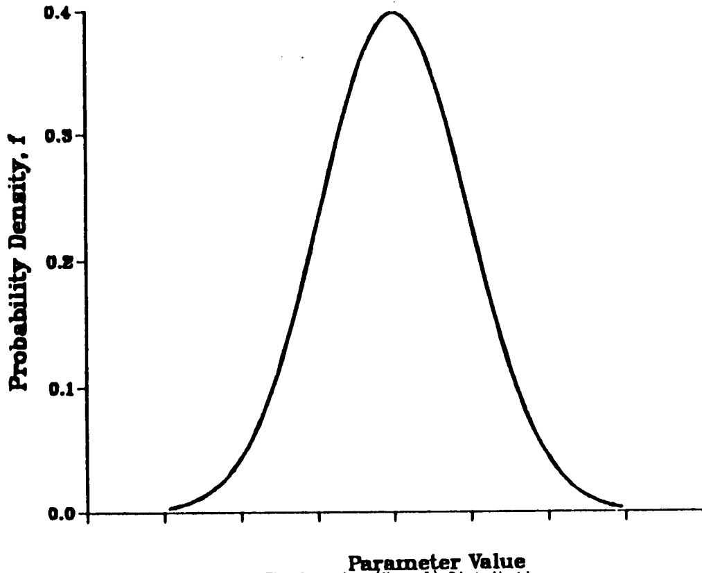
Figure 1: The Gaussian (Normal) Distribution
