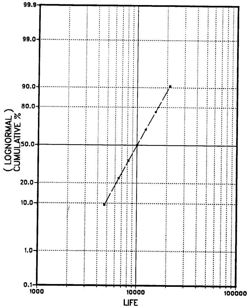
Figure 4: Lognormal CDF for Fatigue-type Data
