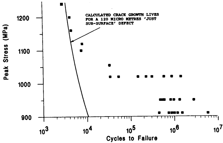
Fig 9 Load controlled LCF lives in AP1 at 600 Deg.C
