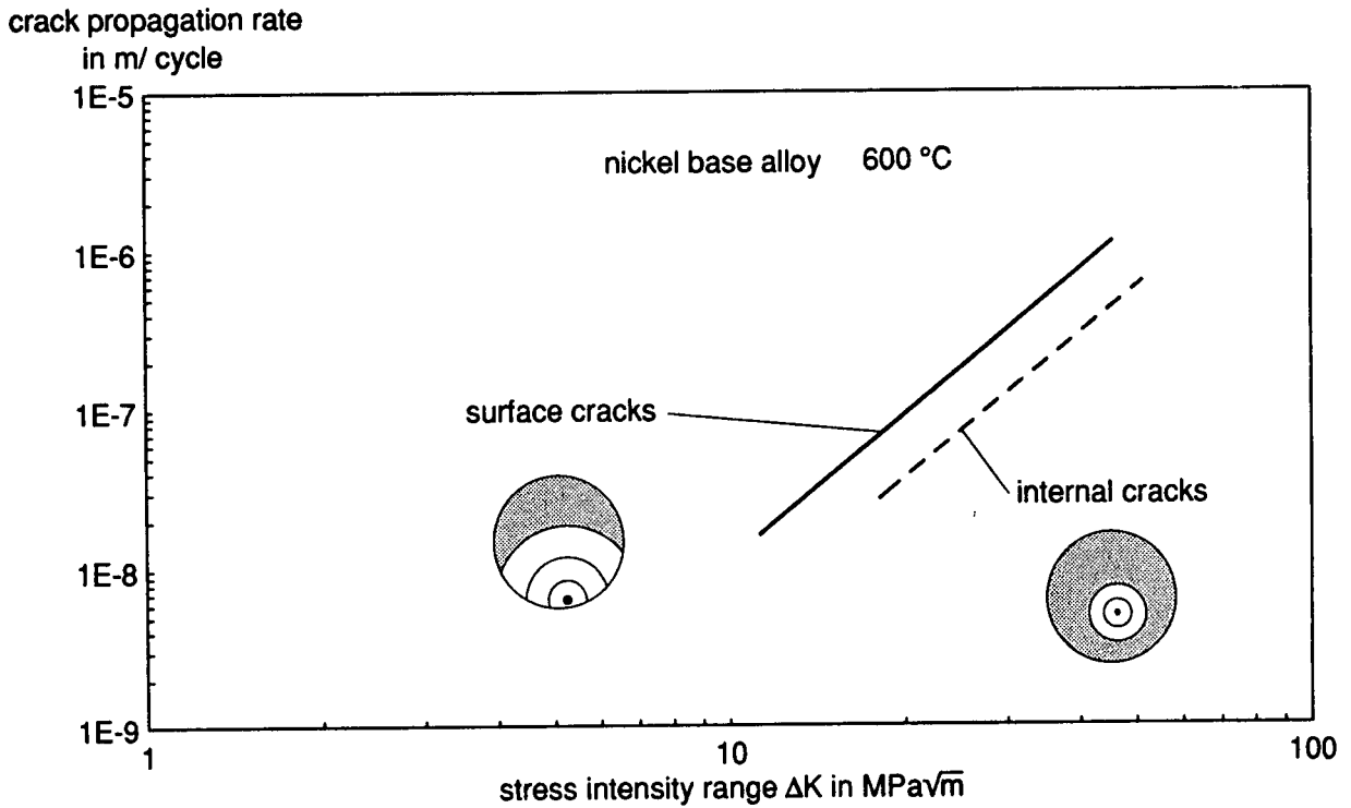
Fig. 13 : Crack propagation of surface and internal cracks
