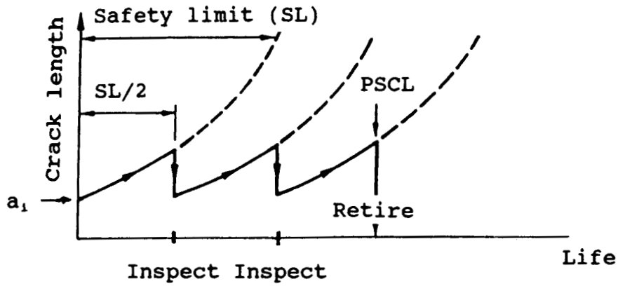
Fig 18 Schematic representation of combined Damage Tolerant-Predicted Safe Cyclic Life
