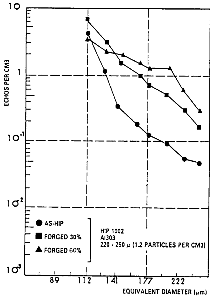
FIG. 4 Effect of hot working
