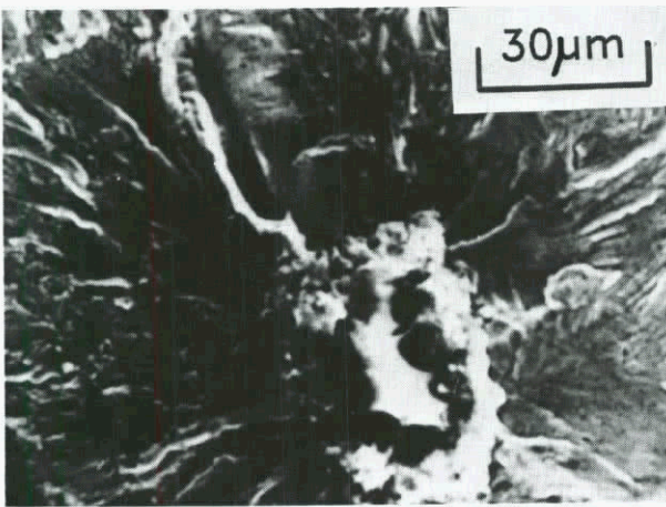
Fig 2 Failure site - Non metallic inclusion
