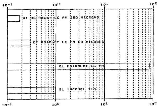
Fig. 6 Impact of lifing approach on the releasable life of an actual disk (geometry as datum).
