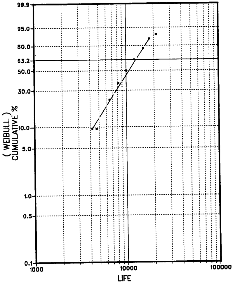
Figure 6: 2 Parameter Weibull CDF for Fatigue-type Data
