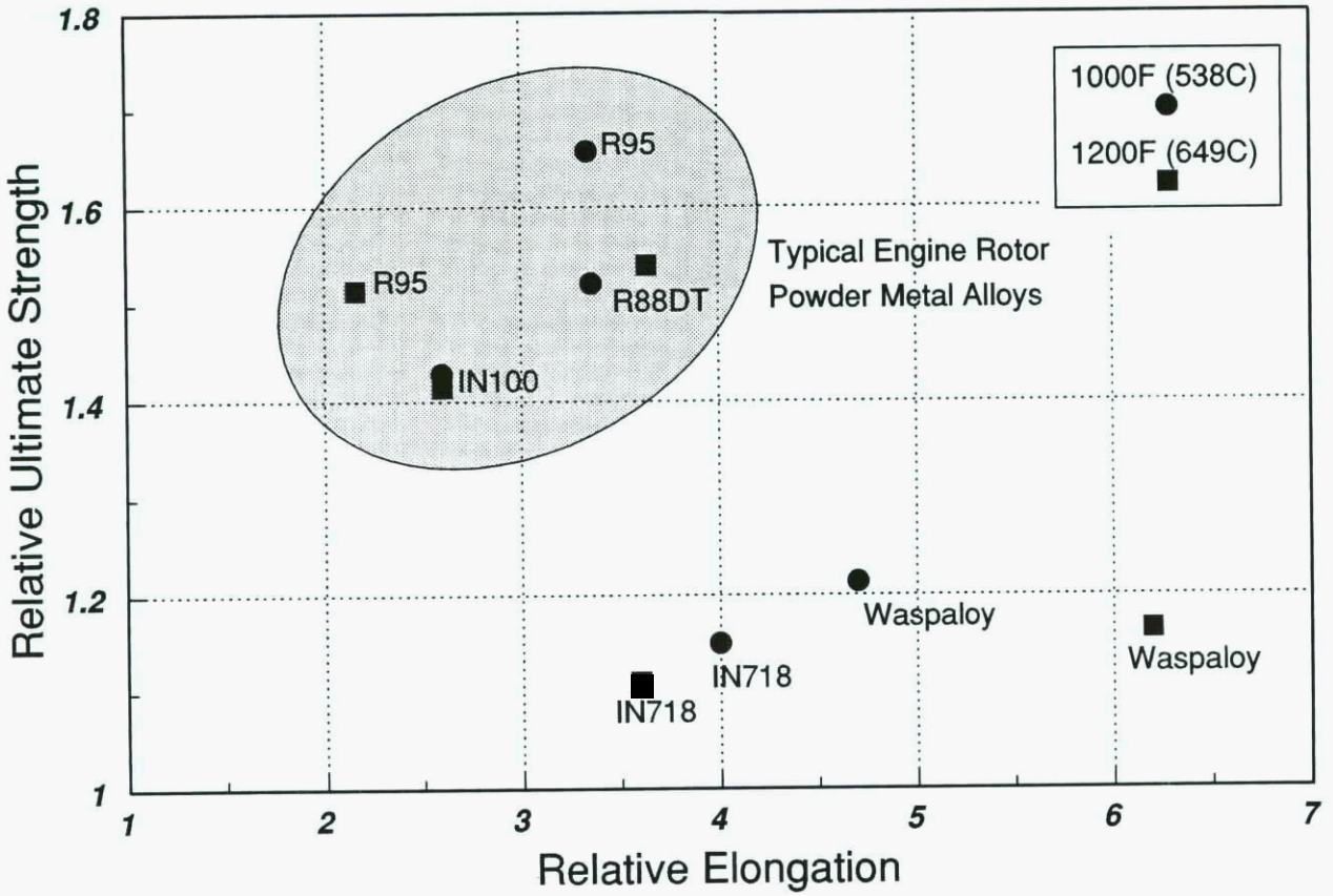
Figure 1. Relative strength and ductility Comparison.
