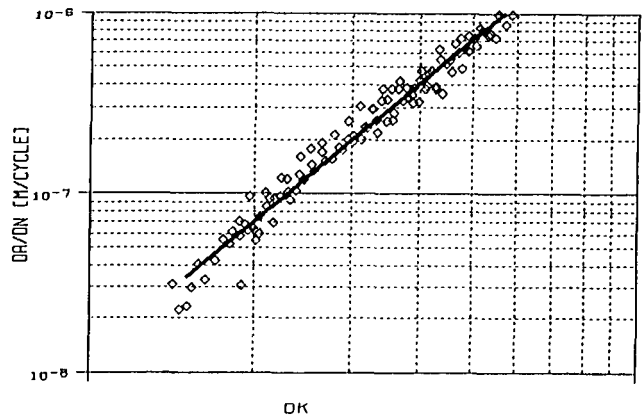
Fig. 3 Crack growth test results obtained on Astroloy LC PM at 500°C and R = 0.1.
