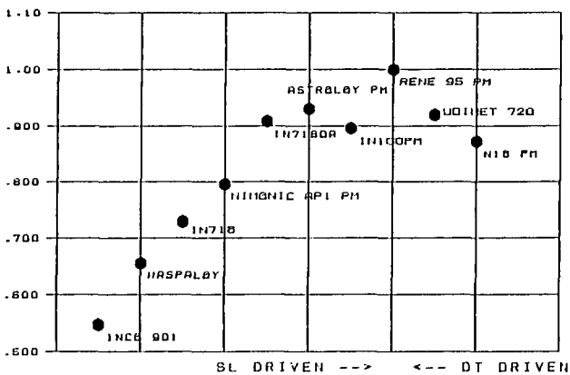
Fig. 1 Development of turbine disk alloys with reference to the specific yield strenght (Fiat data and data from ref. 4).
