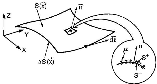
Fig. 2.4 Definition of doublet distribution
