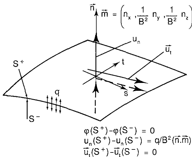
SOURCE DISTRIBUTION
