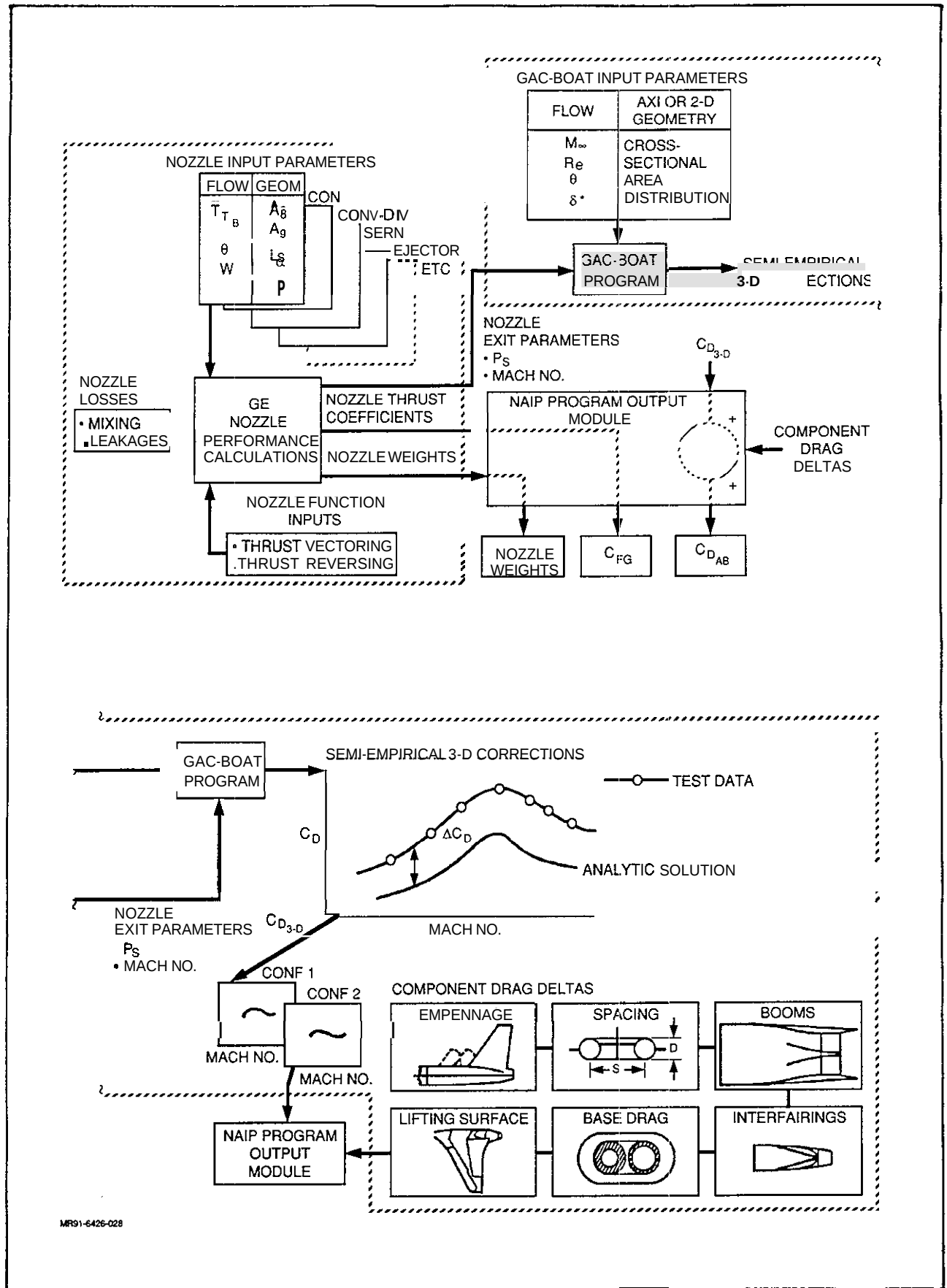
Fig. 47-B Level II Nozzle/Afterbody Installed Performance Prediction Program
