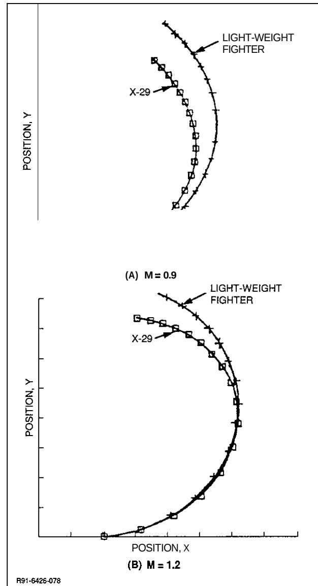
Fig. 95 Aircraft Dynamic Turn Performance at 35,000 ft (Ref. 83)
