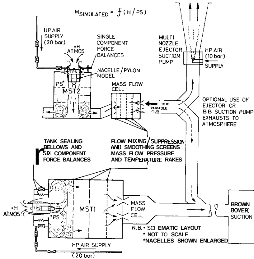
FIG 38 ARA MACH SIMULATION TANKS (FROM REF.10)
