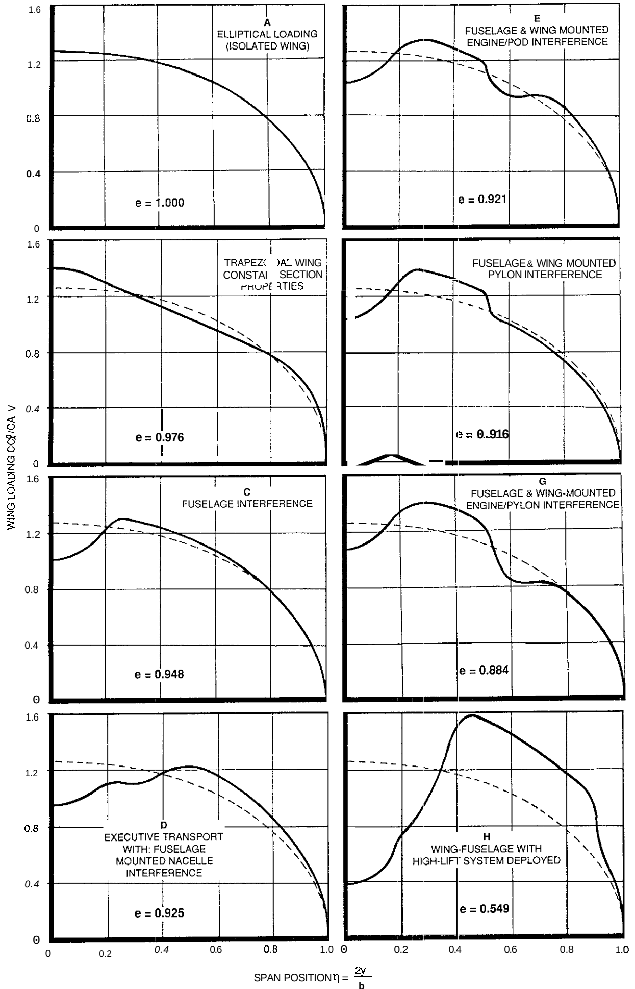
Fig. 17 Examples of Aircraft Symmetric Loading Distributions With Lift-Induced Drag Efficiency Factor
