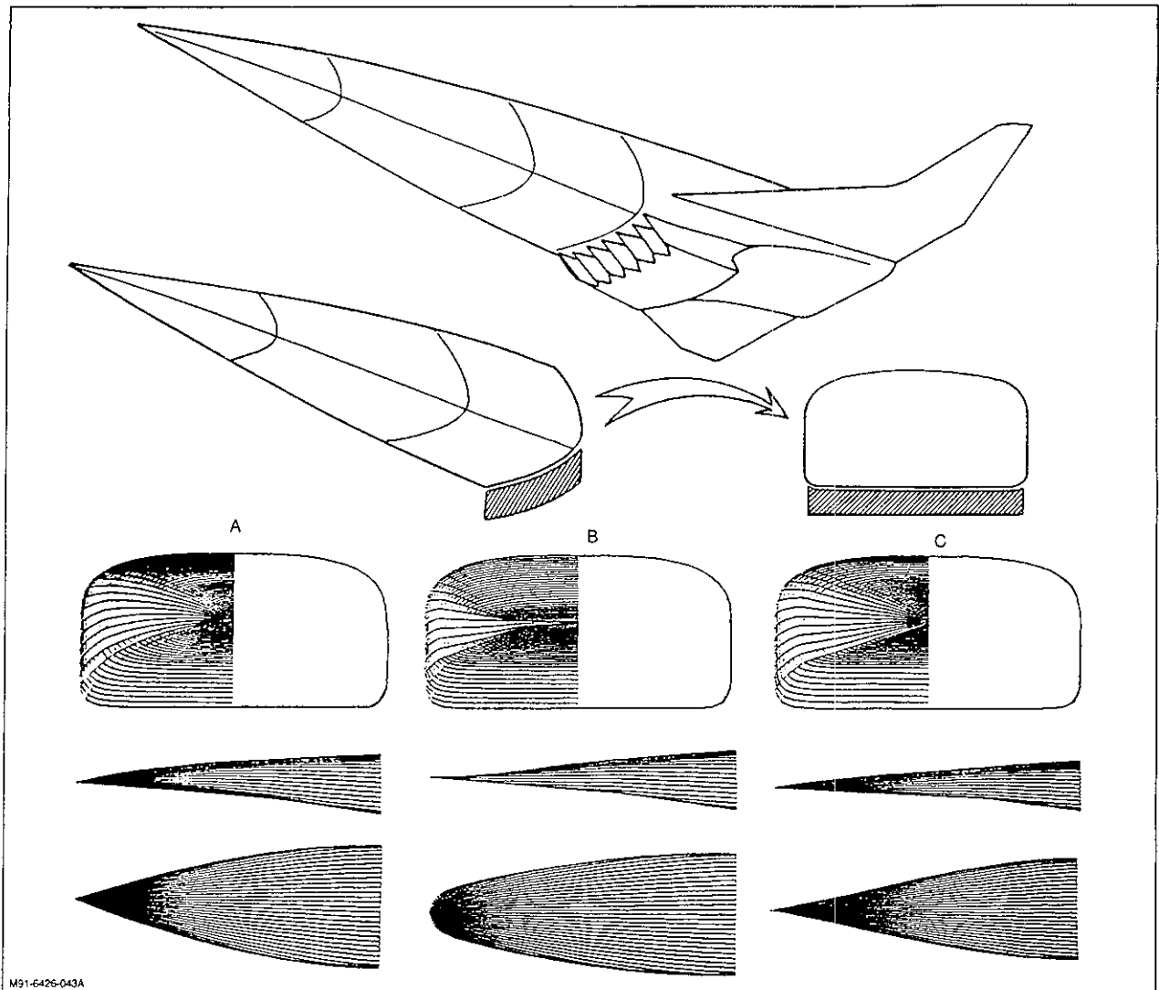
Fig. 85 Hypersonic Forebody Shapes for Drag-Due-To-Incidence Study
