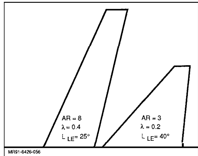
Fig. 24 Transport & Fighter Wing Planforms
