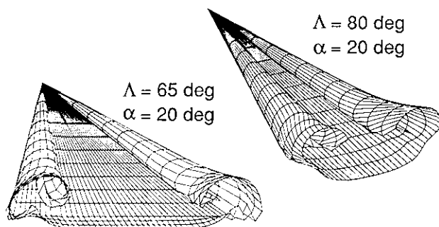
Fig. 8.6 Solution of nonlinear panel method VORSEP for 3D flow about wings with leading-edge vortex separation
