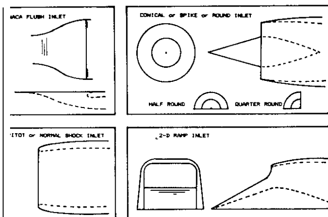
Fig. 30 Inlet types.
