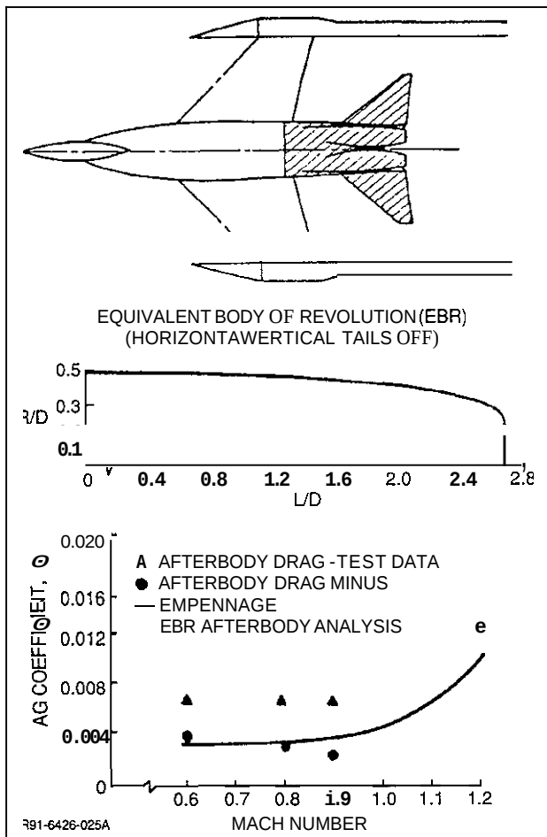
Fig. 45 Equivalent Body Approach Simulating Research Model Afterbody Drag
