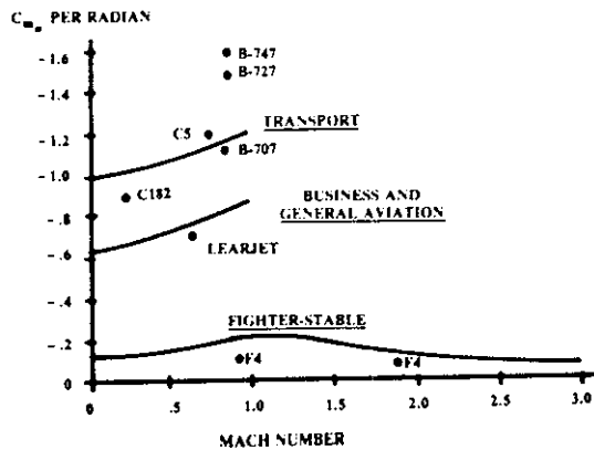
Fig. 21 Typical pitching moment derivative values
