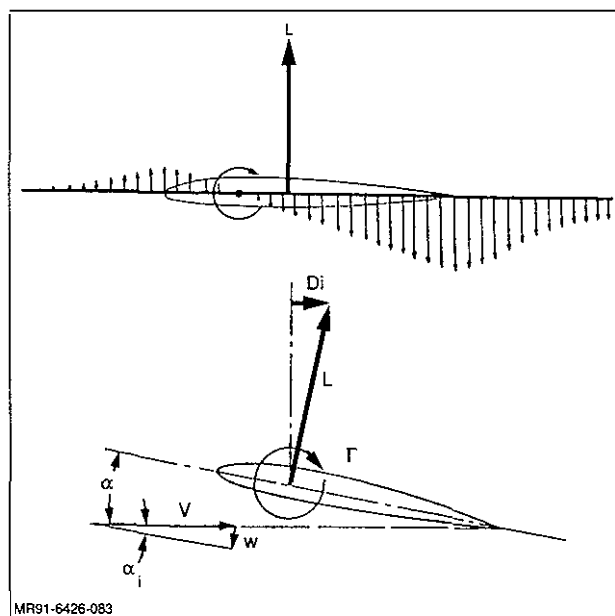
Fig. 4 induced Upwash/Downwash Field with Rotated Lift Vector
