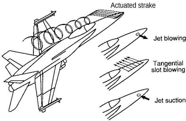
Fig. 80. Forebody flow control concepts.
