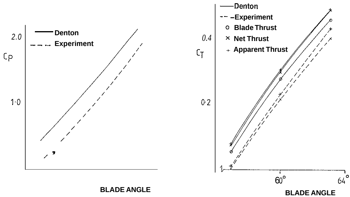
FIG 43 PROPELLER PERFORMANCE: EFFECTS OF THRUST DEFINITION (FROM REF.111)
