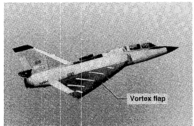
Fig. 54. F-106B with leading-edge vortex flap in flight.
