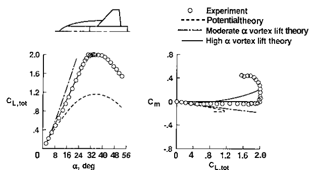
Fig. 66. Complete longitudinal aerodynamic characteristics for strake-wing-body; strake AD 24, A = 44^\circ , M = 0.2 .
