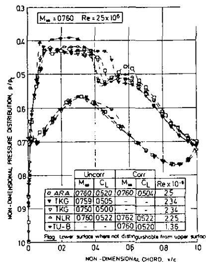
Fig. 7 Experimental approach - uncertainty and sensitivity for identical models in different windtunnels (GARTEUR AG02)
