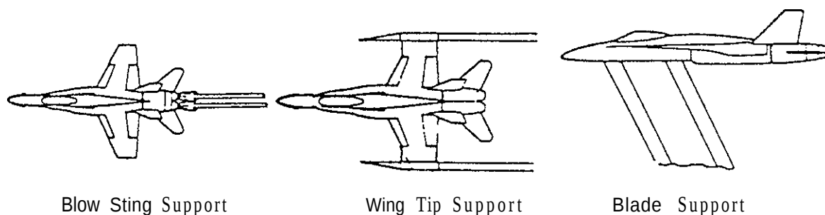
FIG 50 ALTERNATIVE RIGS FOR AFTERBODY PERFORMANCE TESTING (FROM REF. 12)
