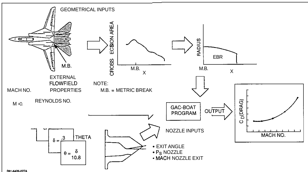
Fig. 47-A Equivalent Body of Revolution Methodology Using GAC-BOAT Code
