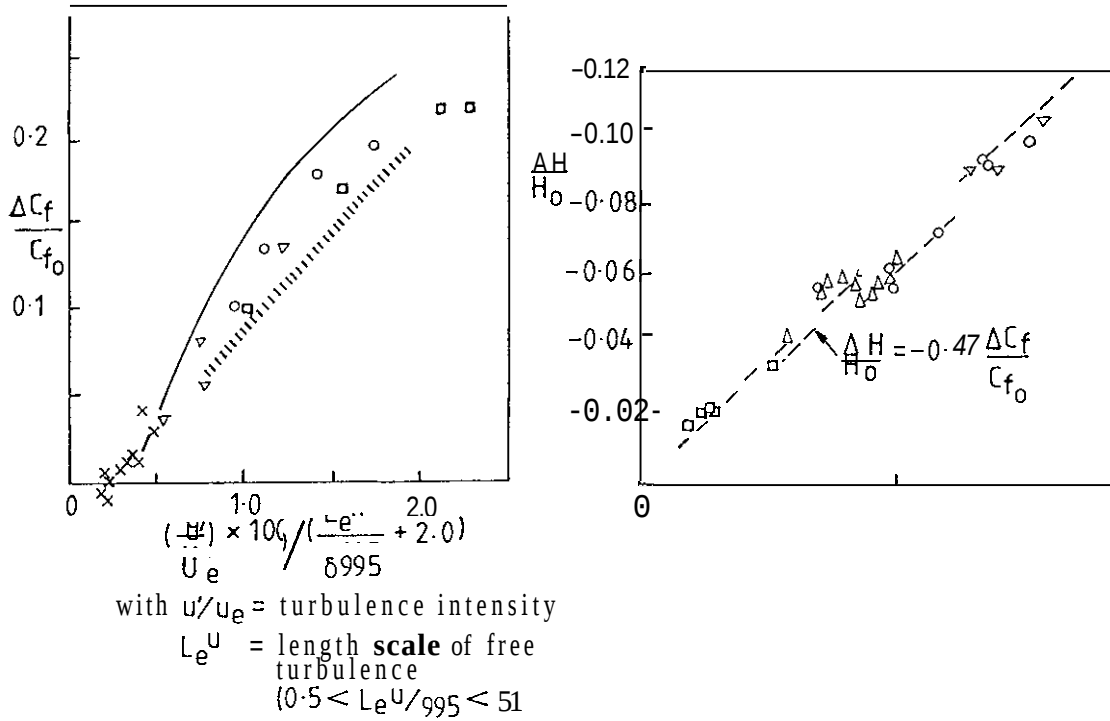
FIG 15 DEPENDENCE OF SKIN FRICTION AND SHAPE FACTOR ON TUNNEL TURBULENCE
