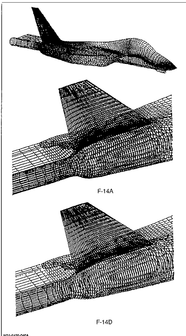
Fig. 74 Surface Gridding for Navier-Stokes Analysis
