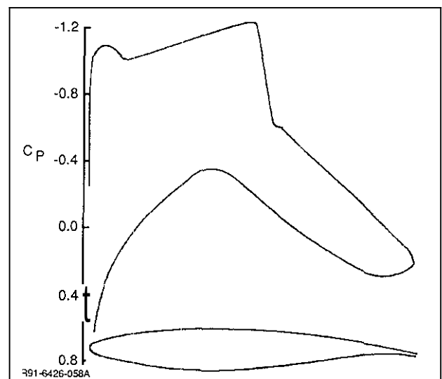
Fig. 22 RAE 2822 Airfoil Pressure Distribution at M_\infty = 0.725 , \alpha = 2.9^\circ
