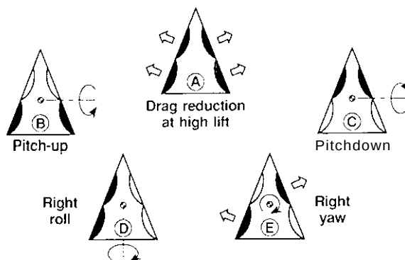
Fig. 75. Hypothesized application of segmented upper vortex flaps for drag reduction and aerodynamic control at high angles of attack; filled segment denotes deployed.
