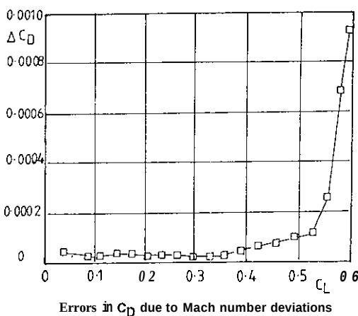
FIG 11 EFFECTS OF VARIABILITY IN MACH NUMBER (FROM REF.15)
