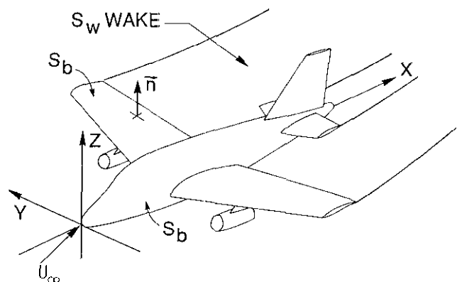
Fig. 2.3 Airplane configuration
