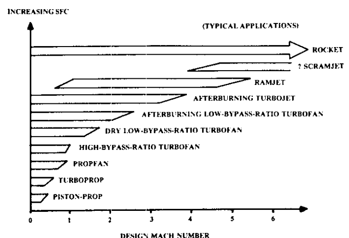
Fig. 29 Propulsion system speed limits.
