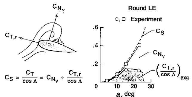
Fig. 30. Relationship between vortex normal force and residual thrust; A = 1.0 , \Lambda = 76^\circ , t/c = 0.1 , FFA 104-5601 airfoil.
