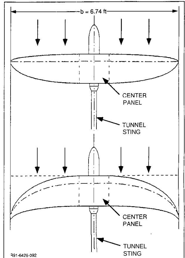
Fig. 81 Swept-Back Wing-Tip Wind Tunnel Models (Ref. 73)
