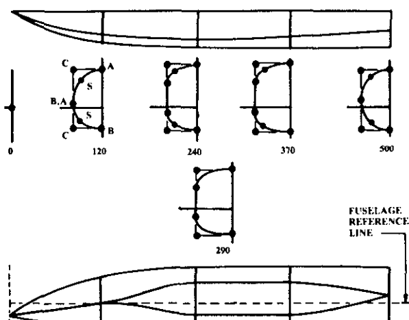
Fig. 47 Typical fuselage lofting
