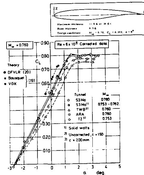
Fig. 7 Experimental approach - uncertainty and sensitivity for identical models in different windtunnels (GARTEUR AG02)
