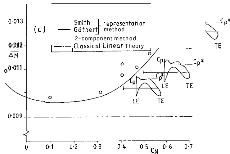
FIG 24 COMPARISON OF PREDICTIONS OF BLOCKAGE CORRECTION: 2D MODEL, RAE 8 FT x 8 FT TUNNEL, M = 0.73 (FROM REF 64)
