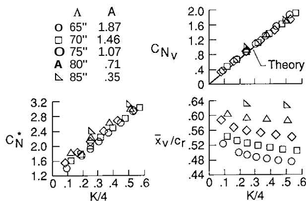
Fig. 15. Similarity for computational solutions for thin delta wings; M = 0 , K/4 = \tan \alpha / A .
