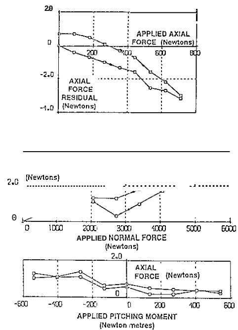
FIG 6b BALANCE CALIBRATION: UNACCEPTABLE RESULTS
