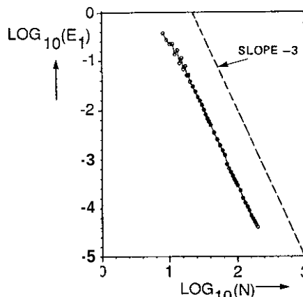
Fig. 5.2 Accuracy of solution for 2D flow using Dirichlet boundary condition and second-order formulation (Ref. 28)
