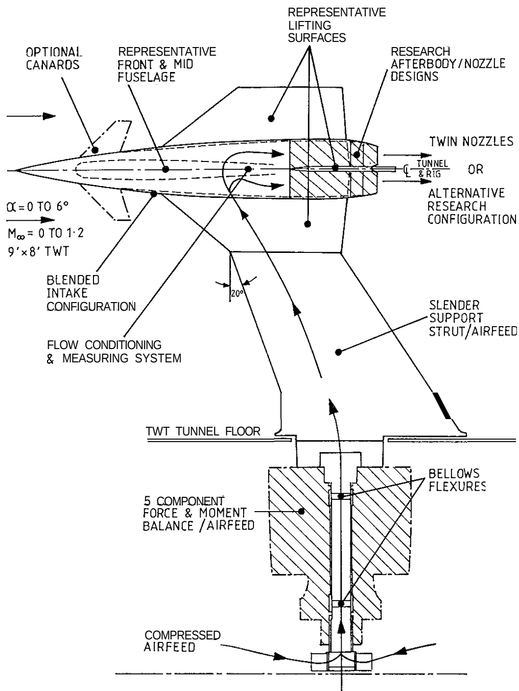
FIG 49 NEW RIG FOR AFTERBODY PERFORMANCE TESTING
