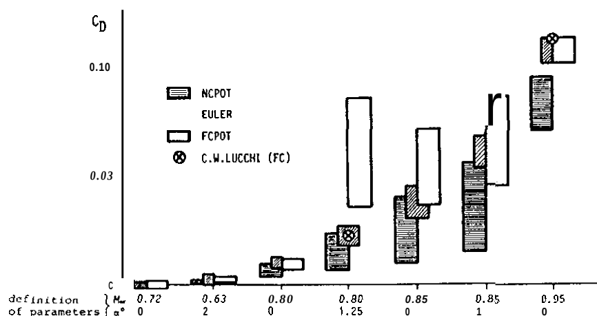
Fig. 6 Test-cases for code validation (NACA 0012) Prediction of drag using CFD codes
