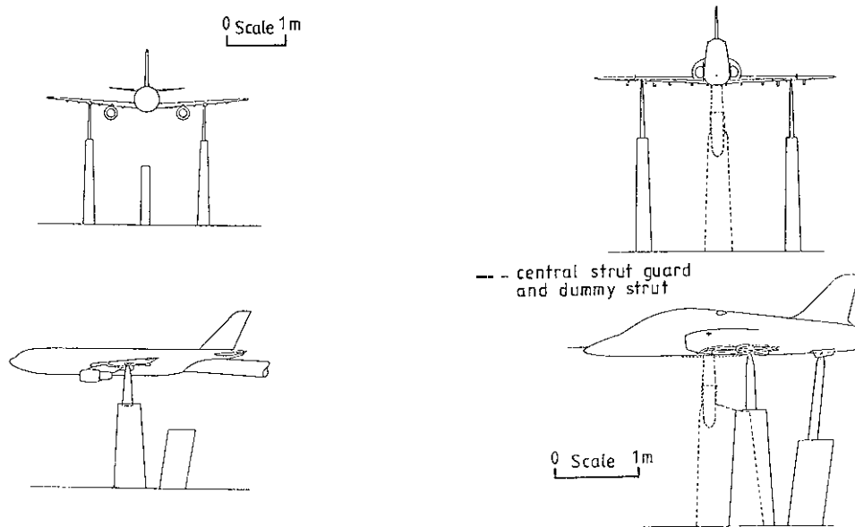
FIG 29 (a) 3-STRUT ARRANGEMENT (b) SINGLE STRUT ARRANGEMENT LAYOUTS FOR STRUT INTERFERENCE TESTS IN RAE 5 METRE TUNNEL
