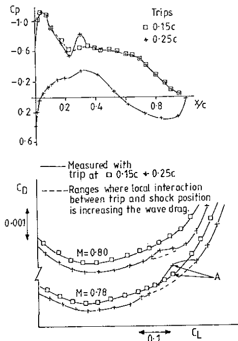
FIG 32b METHOD FOR DETERMINING LOWER C_L - M LIMIT TO RANGE OF VALID DATA
