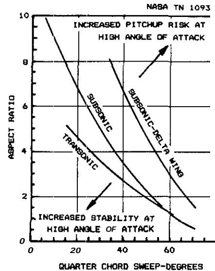
Fig. 9 Tail-off pitchup boundaries.
