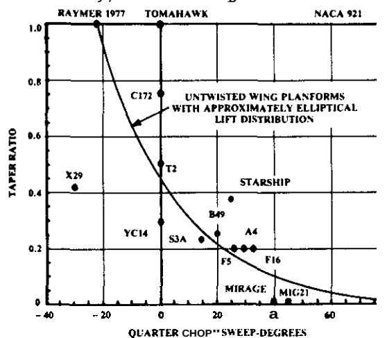
Fig. 11 Effect of sweep on desired taper ratio.
