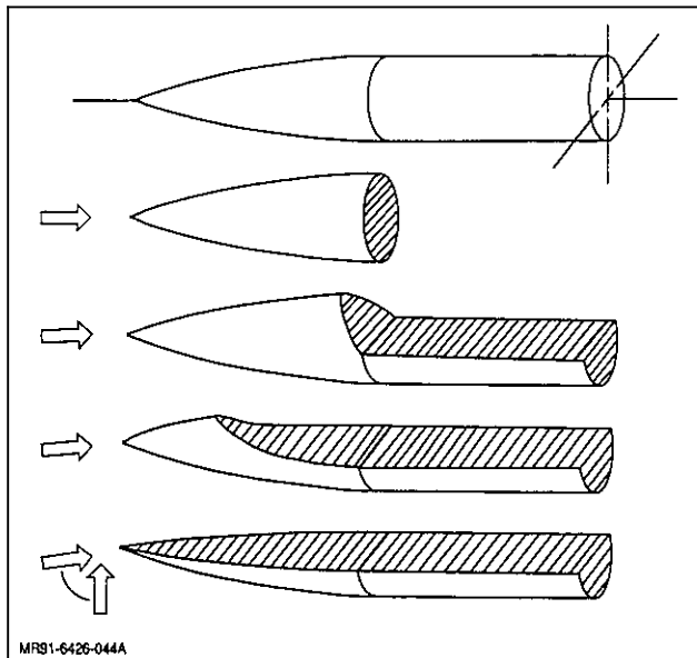
Fig. 89 Effective Body Shape in Newtonian Flow
