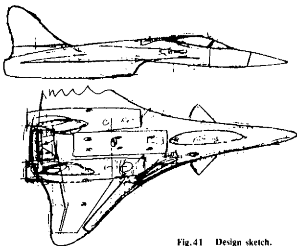
Fig. 41 Design sketch.
