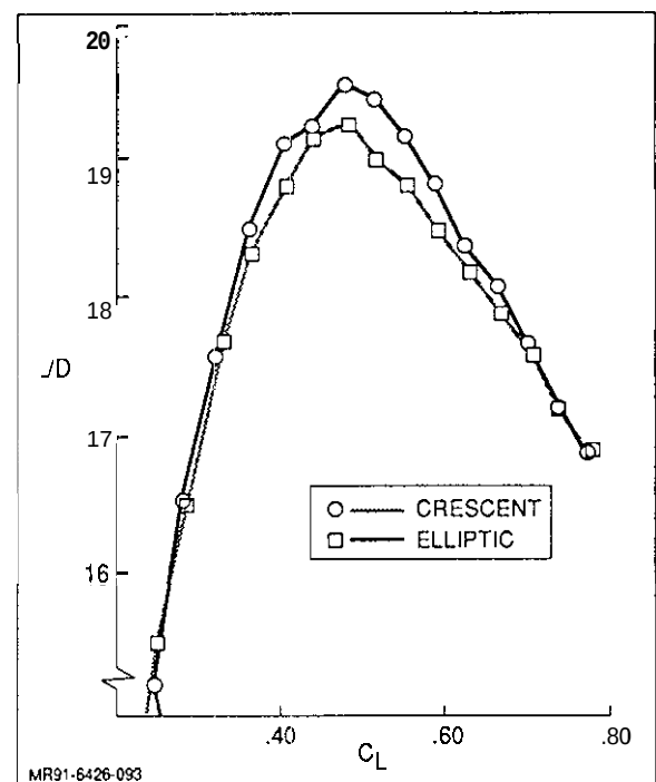
Fig. 82 Experiment Drag Reduction due to Swept-Back Wing Tips (Ref. 73)
