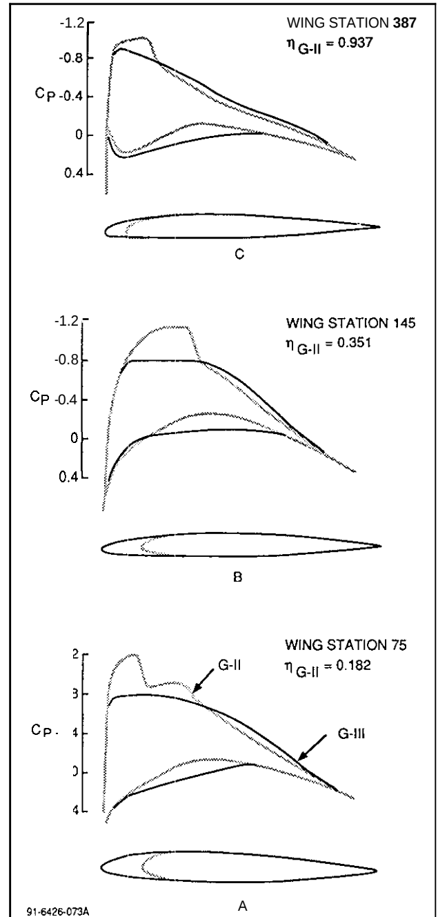
Fig. 63 Airfoil Shape/Wing Pressure Distribution Refinement for Gulfstream III
