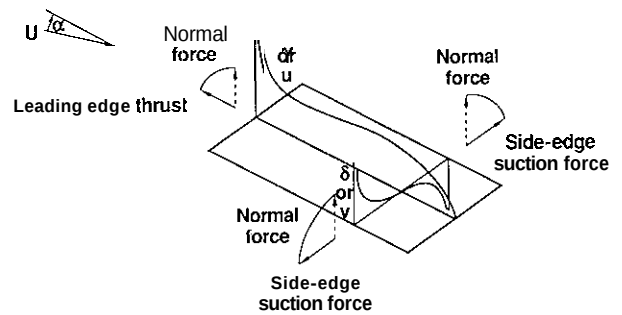
Fig. 16. Vortex-lift concept; suction analogy applied to LE and SE.
