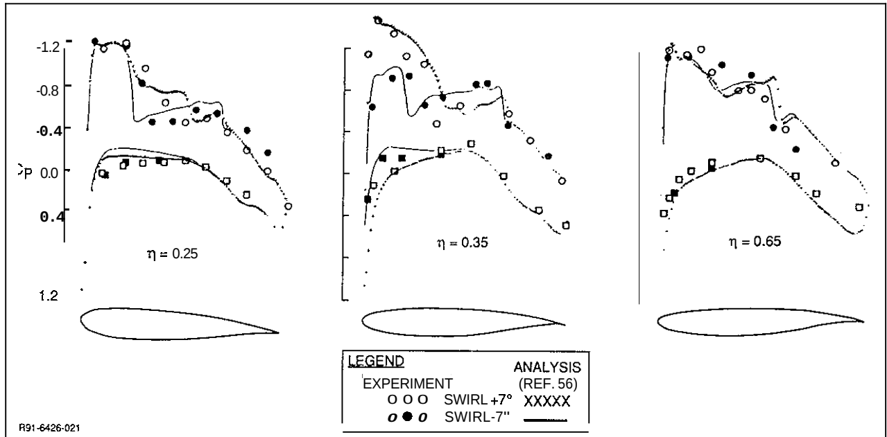
Fig. 38 Wing Pressure Distribution Correlation Illustrating Propfan Slipstream Interference Effects ( M = 0.8 \alpha = 3 Deg)
