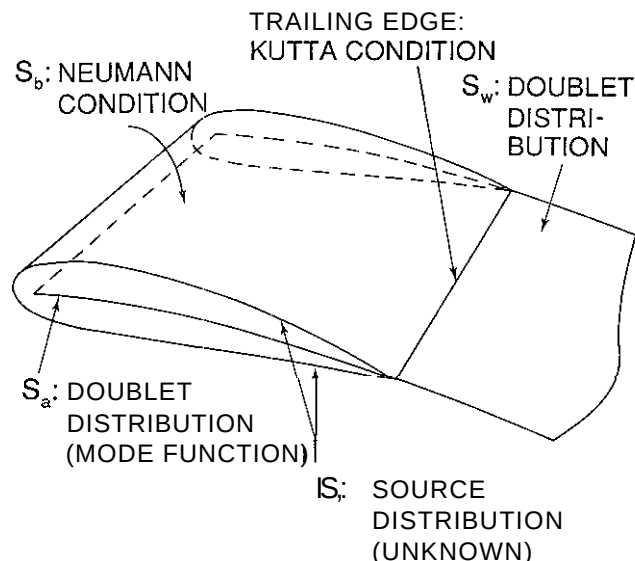
Fig. 3.1 Example of formulation of first generation panel method
