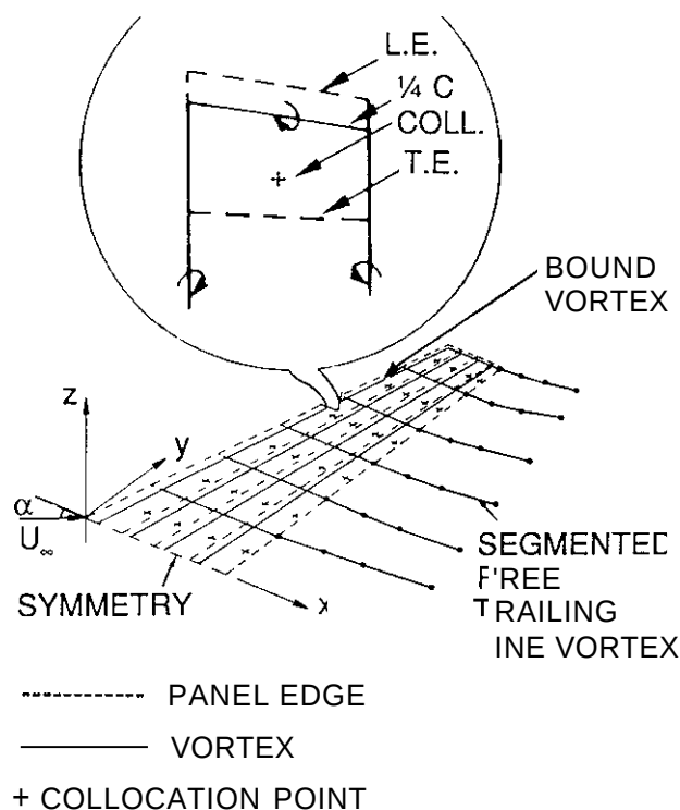
Fig. 4.5 Vortex lattice method
