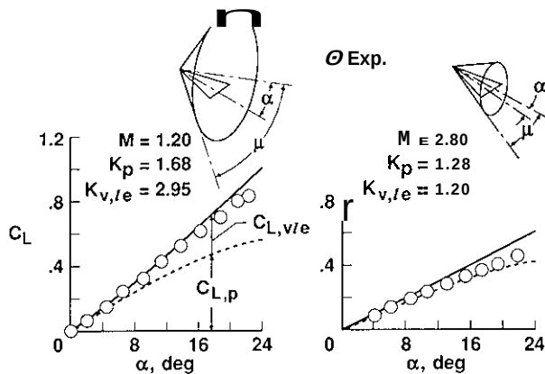
Fig. 13. Effect of supersonic Mach number on C_L for A = 1.147 delta wing.
