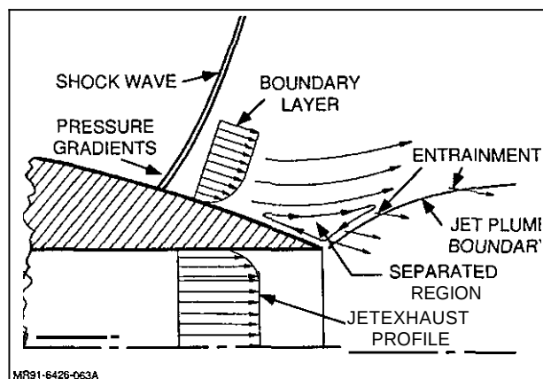
Fig. 9 Elements of Complex Nozzle/Plume Interaction Flow Fields
