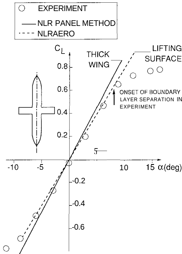
Fig. 8.2 Correlation of computed and measured lift coefficients.
