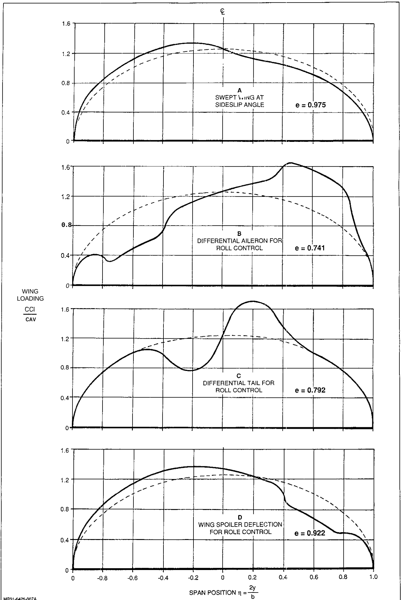
Fig. 18 Examples of Aircraft Unsymmetric Loading Distributions with Lift-Induced Drag Efficiency Factor
