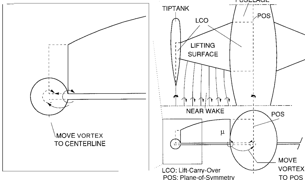
Fig. 3.2 Example of the use of lift-carry-over (LCO) segments
