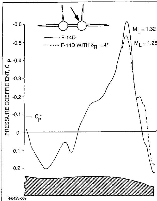
Fig. 78 Effect of Inboard Rudder Deflection on F-14 Afterbody Pressure Field at M = 0.95
