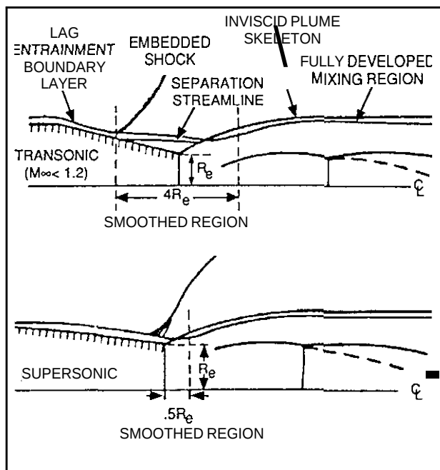
Fig. 33 Boattail Analysis Method Computational Regions
