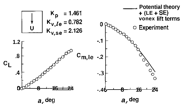
Fig. 17. Aerodynamic characteristics of A = 1 rectangular wing; M \approx 0 .
