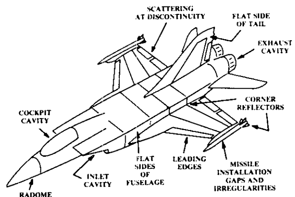
Fig. 38 Major RCS contributors.
