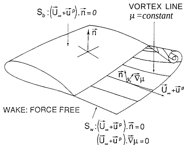
Fig. 3.11 Full wake relaxation
