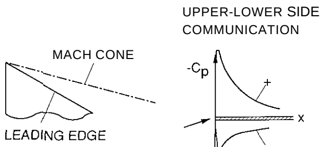
Fig. 2.7a Subsonic leading edge
