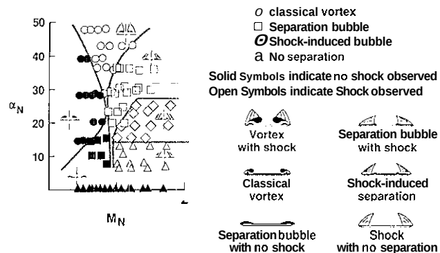
Fig. 4. Classification of experimental data for sharp-leading-edge delta wings.
