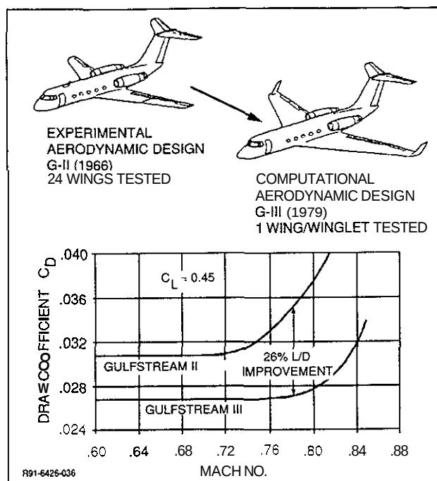
Fig. 65 G-II/G-III Drag Comparison
