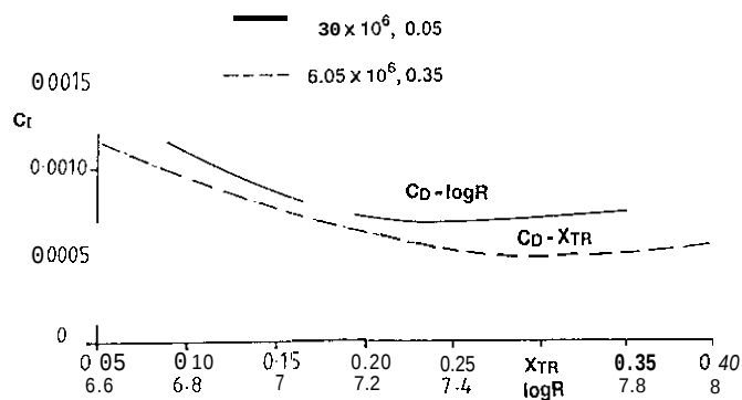
FIG 36(d) CONSEQUENCE OF FAILURE TO SIMULATE SUPERCRITICAL FLOW DEVELOPMENT (FROM REF.86)
