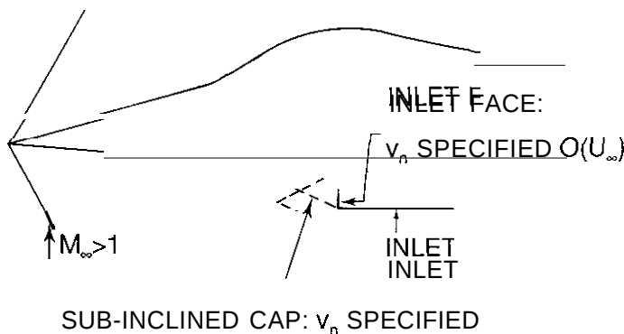
Fig. 3.15 Inlet modeling in supersonic flow
