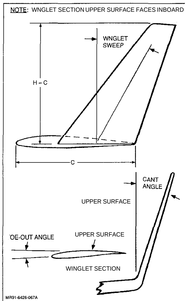
Fig. 59 Details of Winglet Geometry
