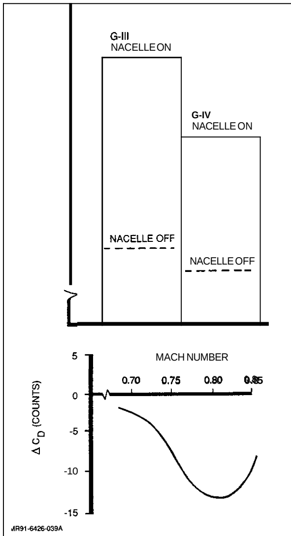
Fig. 70 G-IV/G-III Drag Reduction Showing Engine-Airframe Integration Benefit
