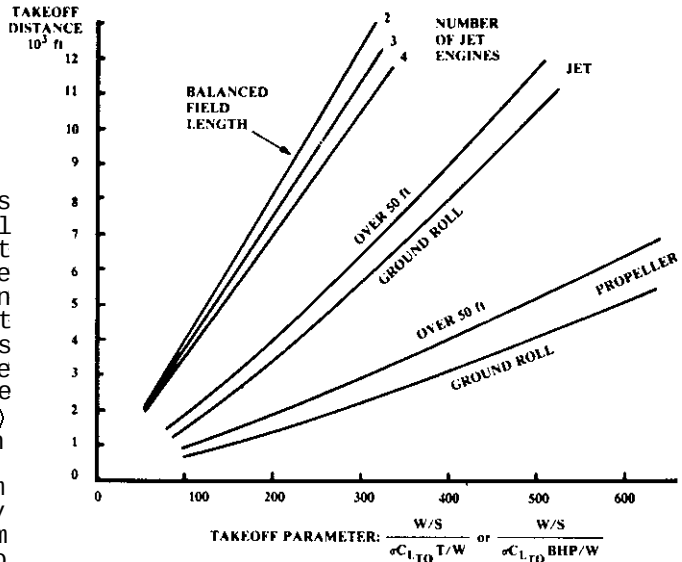
Fig. 14 Takeoff distance estimation.
