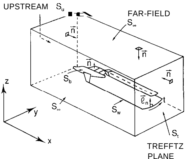
Fig. 4.11 Far-field momentum analysis
