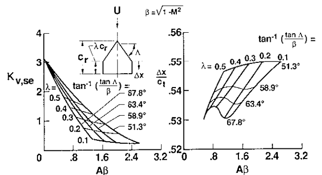
Fig. 18. Theoretical values of K_{v,se} and \Delta x/c_t for cropped delta wings.
