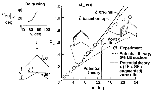
Fig. 26. Effect on \tilde{c} definition on estimated C_L .
