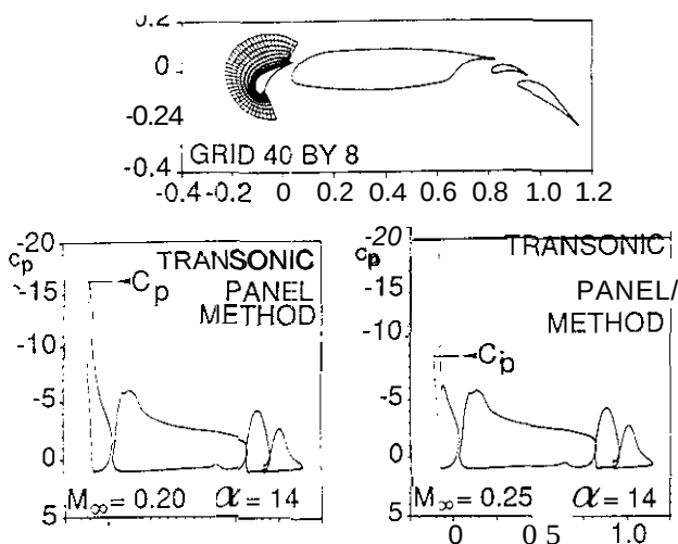
Fig. 9.1 Application of field panel method to 4-component airfoil section (Ref. 41)
