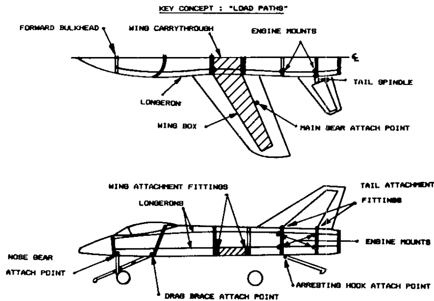
Fig. 26 Structural arrangement.
