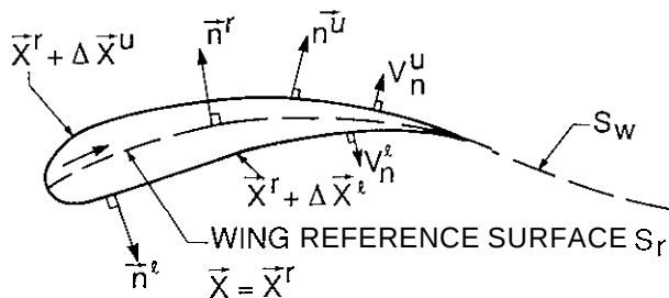
Fig. 3.7 Lifting surface approximation
