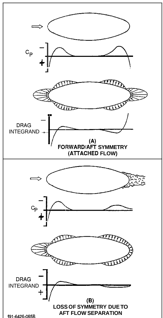
Fig. 2 Body Pressure Field With Drag Integrant
