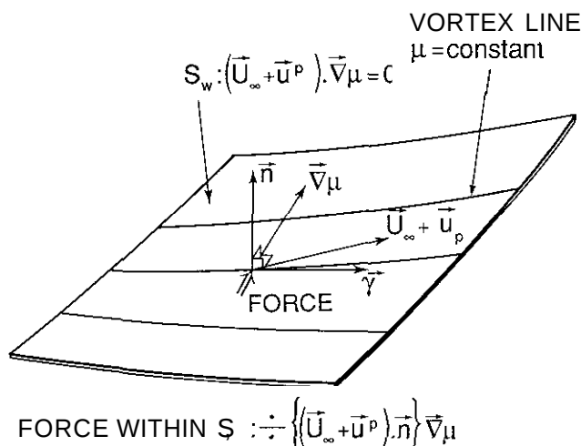
Fig. 3.13 Partial wake relaxation · Force on wake
