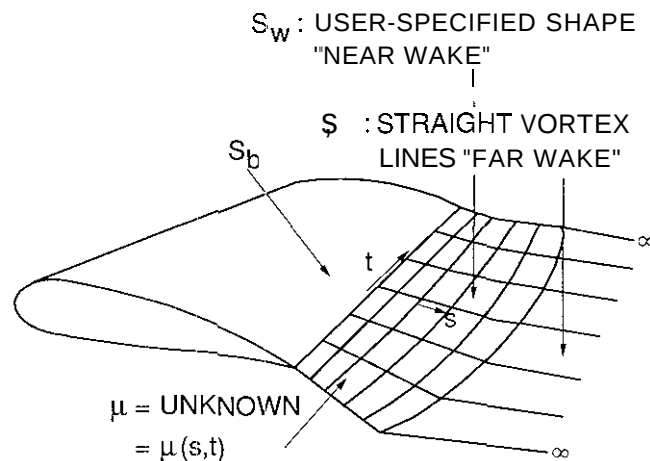
Fig. 3.12 Partial wake relaxation
