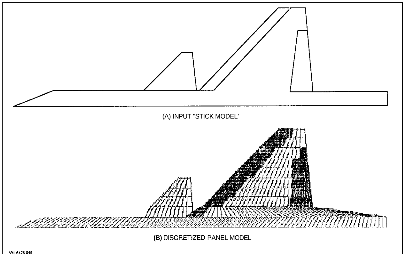
Fig. 55 Trim Optimization Code Modeling
