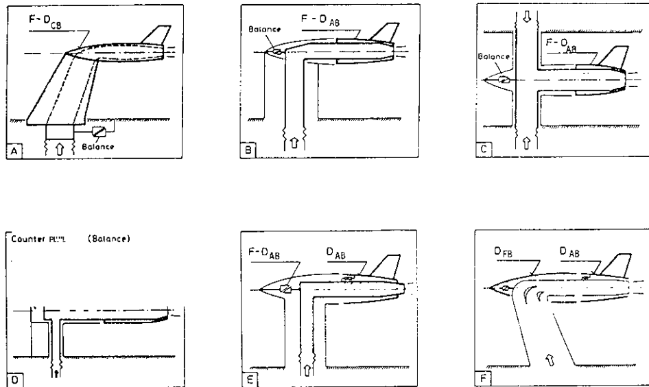
FIG 51 AFTERBODY TEST RIGS (FROM REF.12)
