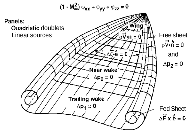
Fig. 35. Theoretical formulation - panel method - FVS.
