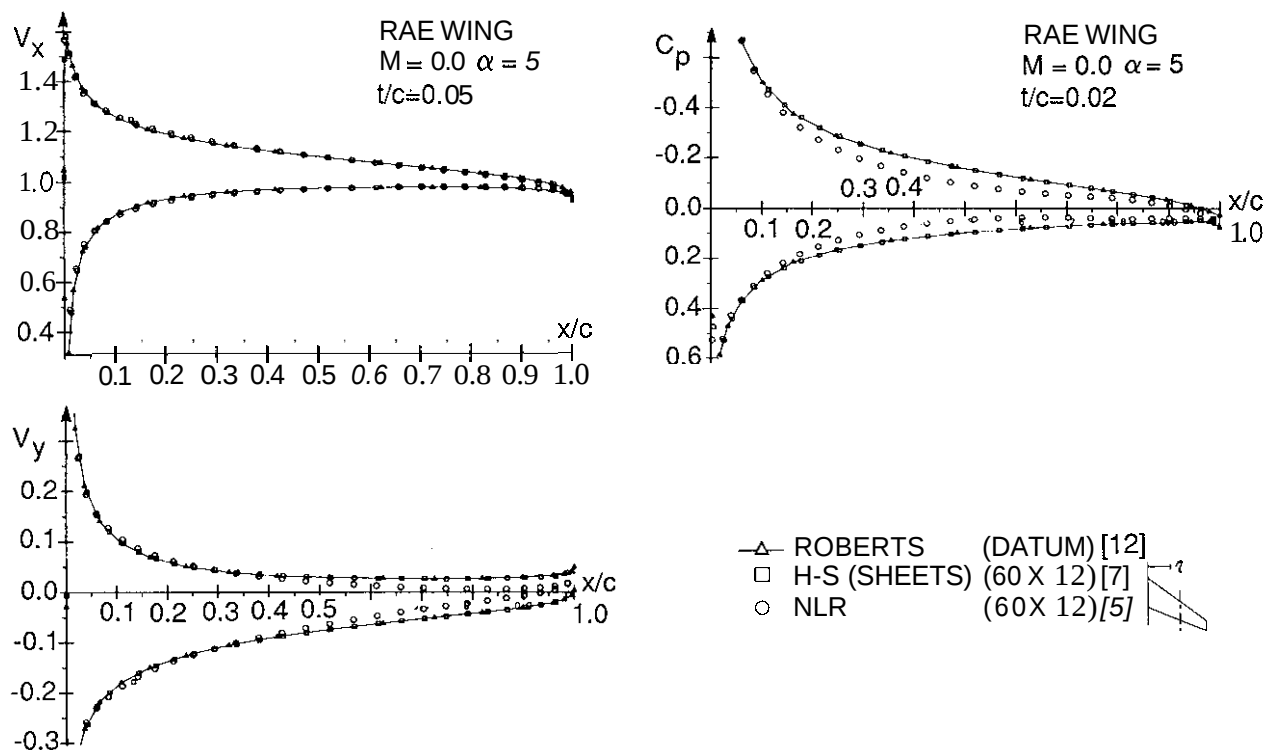
Fig. 5.1 Comparison of first-generation panel methods, Ref. 27
