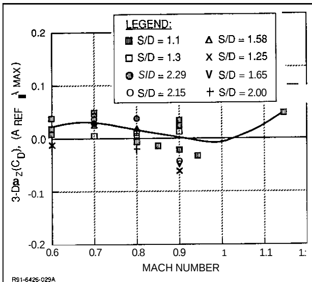
Fig. 48 ERB/Spacing Effects – Cruise Nozzle
