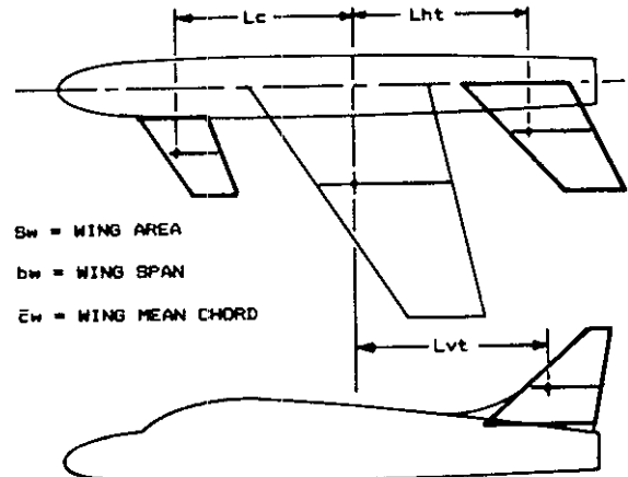
Fig. 22 Initial tail sizing.
