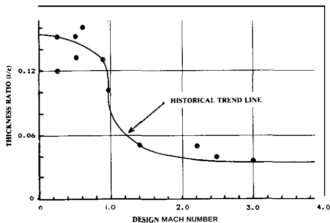
Fig. 12 Thickness ratio historical trend.
