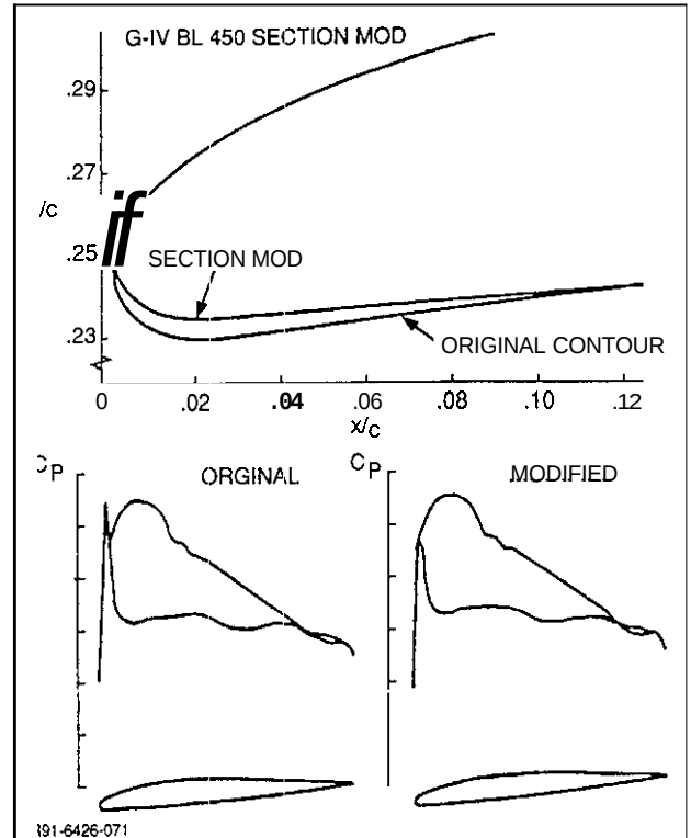
Fig. 68 G-IV Wing Tip Mod to Eliminate Lower Surface Pressure Spike, M = 0.78 , \alpha = 3.5^\circ , \eta = 0.95
