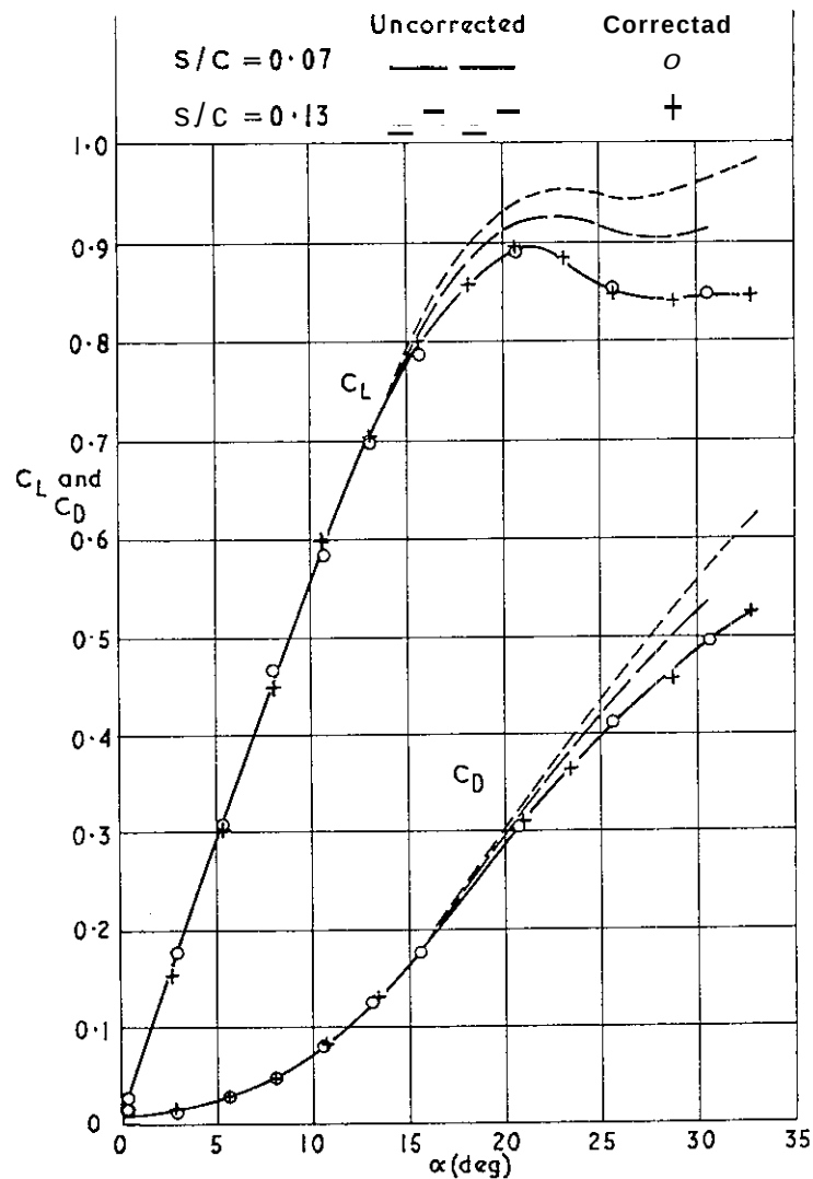
FIG 18 APPLICATION OF BLOCKAGE CORRECTIONS AT HIGH LIFT (FROM REF 42)
