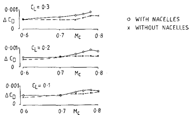
FIG 3b STING CORRECTIONS, WITH AND WITHOUT NACELLES FOR MODEL IN FIG 3a
