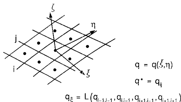
Fig. 4.7 Possible numerical schemes
