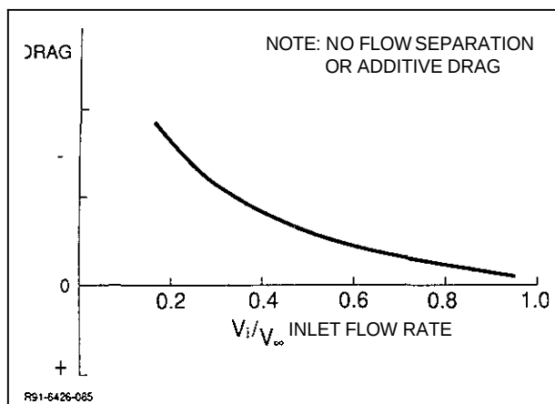
Fig. 31 Effect of Inlet Spillage on Inlet Lip Drag
