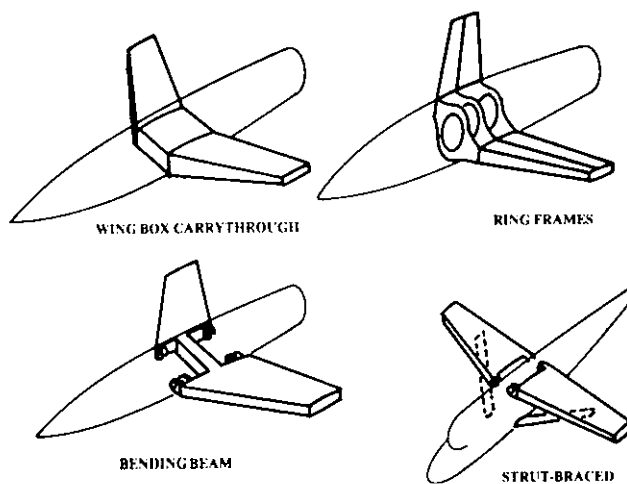
Fig. 27 Wing carrythrough structure.
