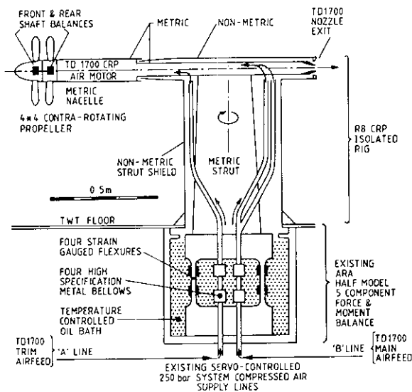
FIG 42(a) AIR-DRIVEN SMALL PROPELLER RIG IN ARA TRANSONIC TUNNEL (FROM REF.105)
