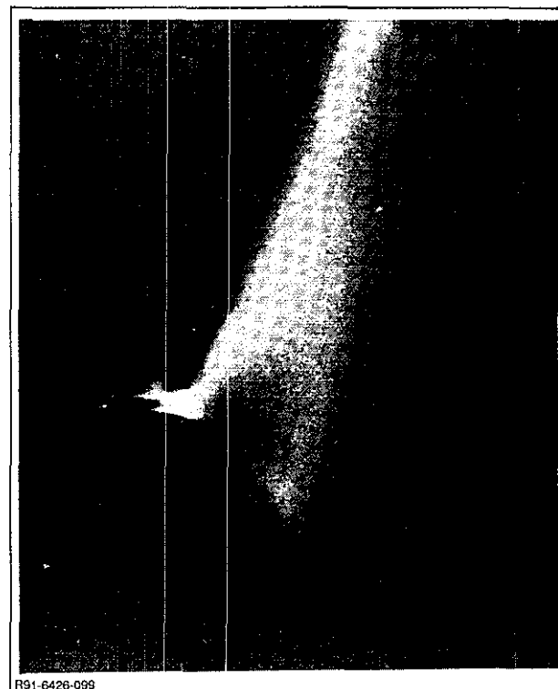
Fig. 6 Extent of 1-14 Shock Wave Pattern at Supersonic Speeds
