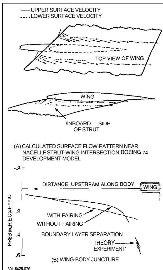
Fig. 35 Component Interference Effects (Refs. 54 & 55)
