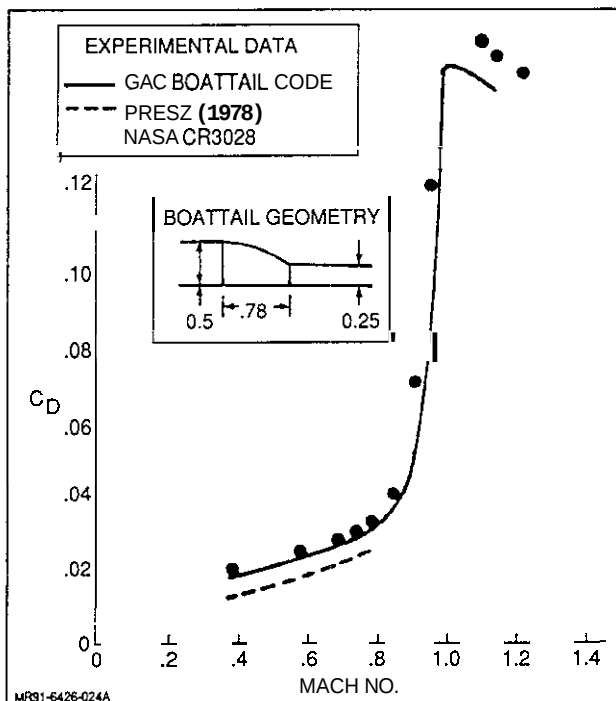
Fig. 44 Prediction of Tri-Sonic Drag Characteristics of Boattail-Sting Configuration (Case No.2)
