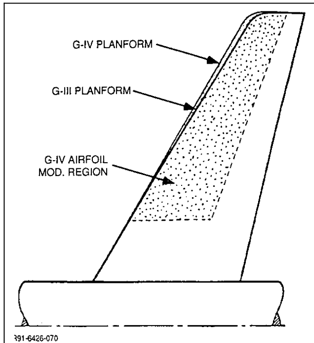
Fig. 67 Gulfstream III/IV Planforms with G-IV Airfoil Contour Modification Region
