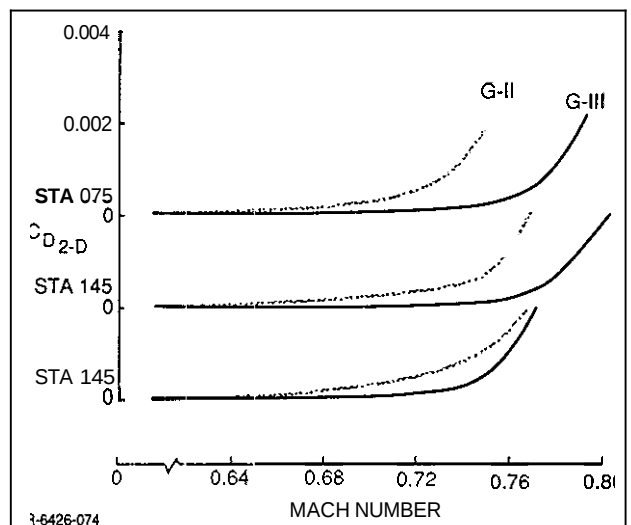
Fig. 64 Analytically Predicted Improvement in G-III Wing Section Drag Divergence Mach Number
