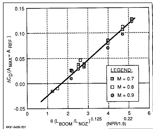
Fig. 52 Boom Correlation – Cruise Nozzle
