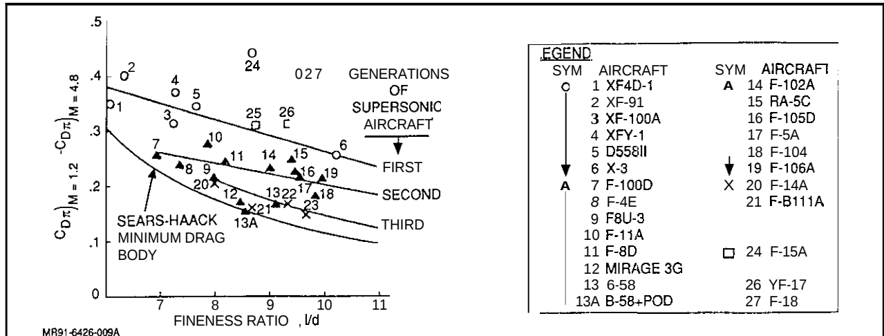
Fig. 28 Supersonic Wave Drag Trending (Ref. 8)
