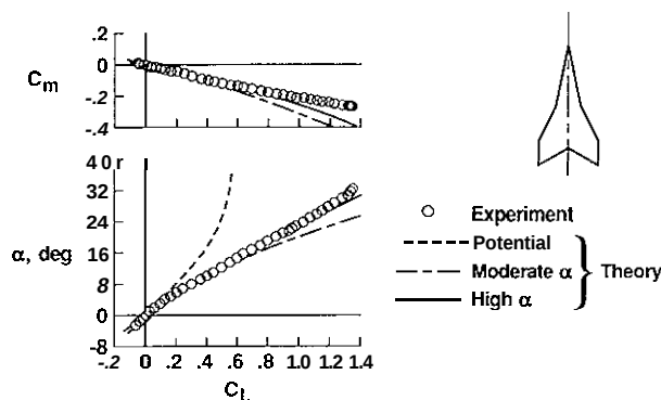
Fig. 64. Longitudinal aerodynamic characteristics for cranked wing; A = 1.10 ; A = 80^\circ/65^\circ , M \approx 0 , VLM-SA.
