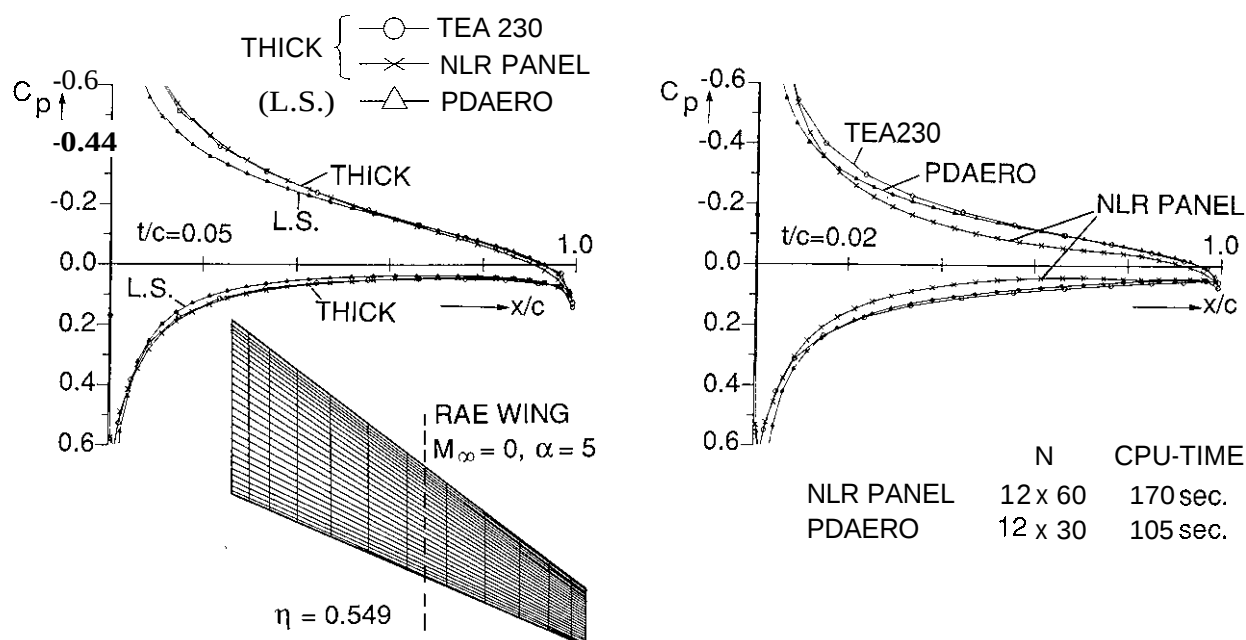
Fig. 5.4 Comparison between thick wing and lifting surface model
