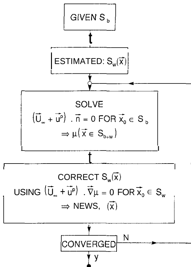
Fig. 3.10 Wake relaxation procedure
