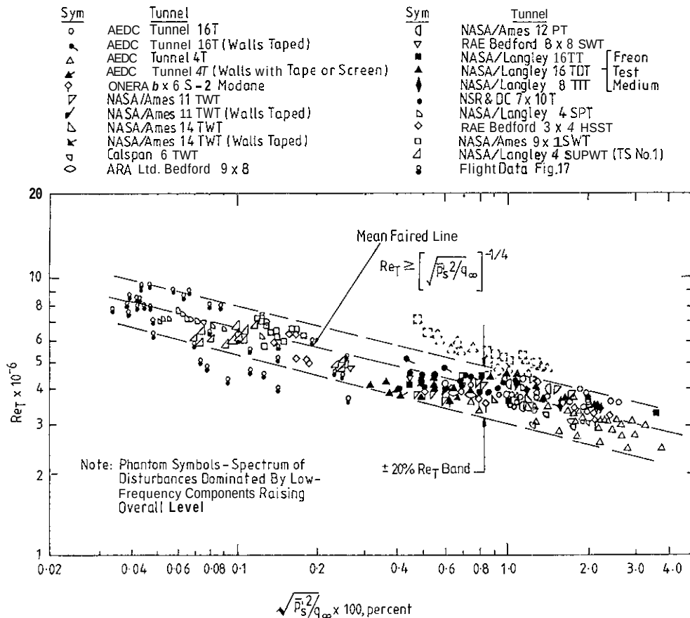
FIG 13 TRANSITION REYNOLDS NUMBERS DEDUCED FROM TESTS WITH 10' CONE (FROM REF 33)
