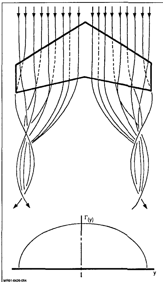
ig. 3 Lifting Surface Upper/Lower Flow Pattern with Load Distribution
