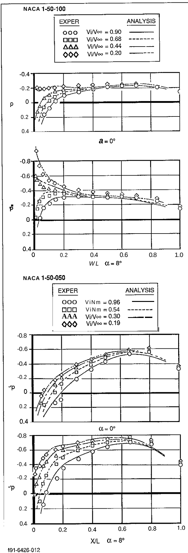
Fig. 30 Inlet Top Centerline Pressure Distribution Correlations
