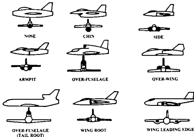
Fig. 34 Inlet locations—buried engines.
