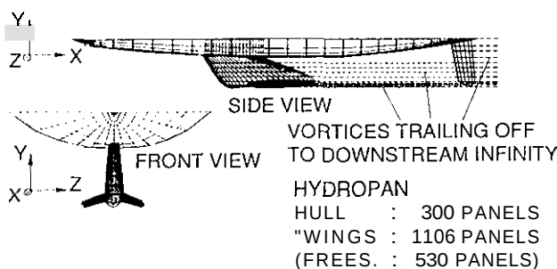
Fig. 8.7 Example of panelling of hydrodynamical application (Ref. 39)
