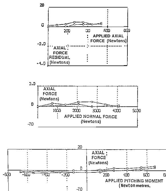
FIG 6a BALANCE CALIBRATION: ACCEPTABLE RESULTS
