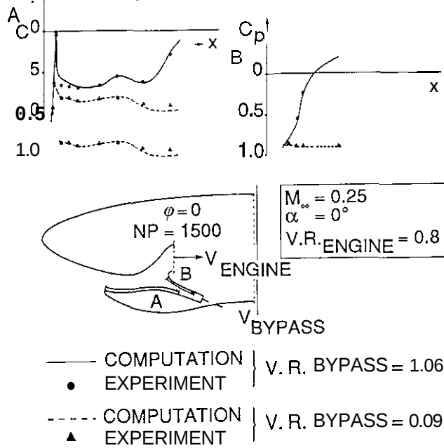
Fig. 5.5 Detail study of the flow into an engine intake
