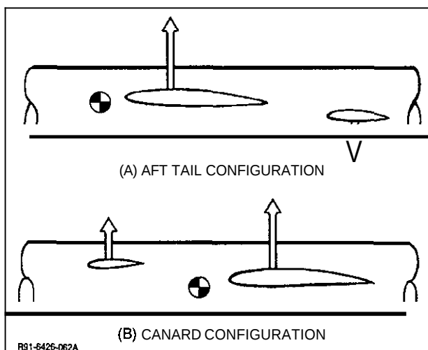
Fig. 10 Balance & Trim for Conventional Aft-Tail & Canard Configurations
