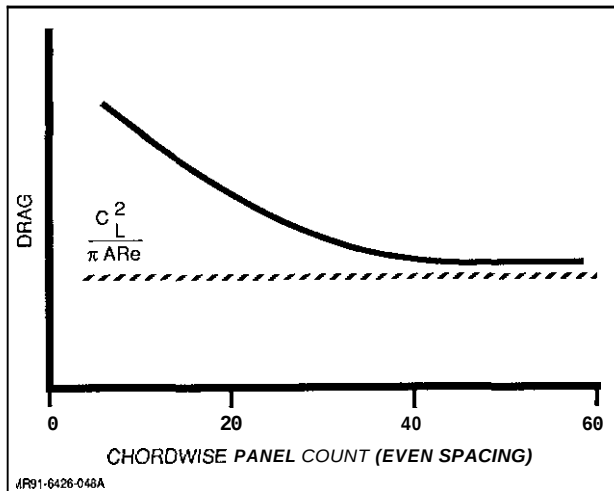
Sketch A Effect of Chordwise Panel Density on Computed Lift-Induced Drag Level
