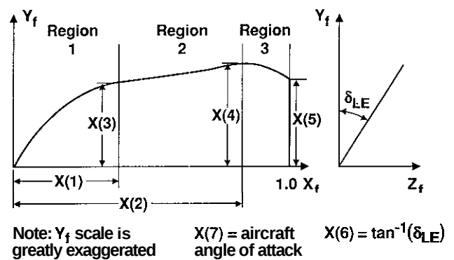
Fig. 55. Analytical vortex flap model with design variables.
