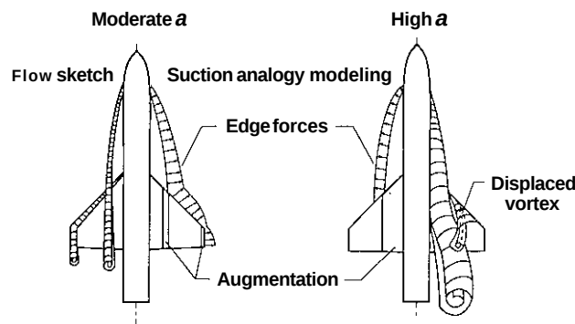
Fig. 27. Effect of a on vortex flow models for conical configurations; VLM-SA.
