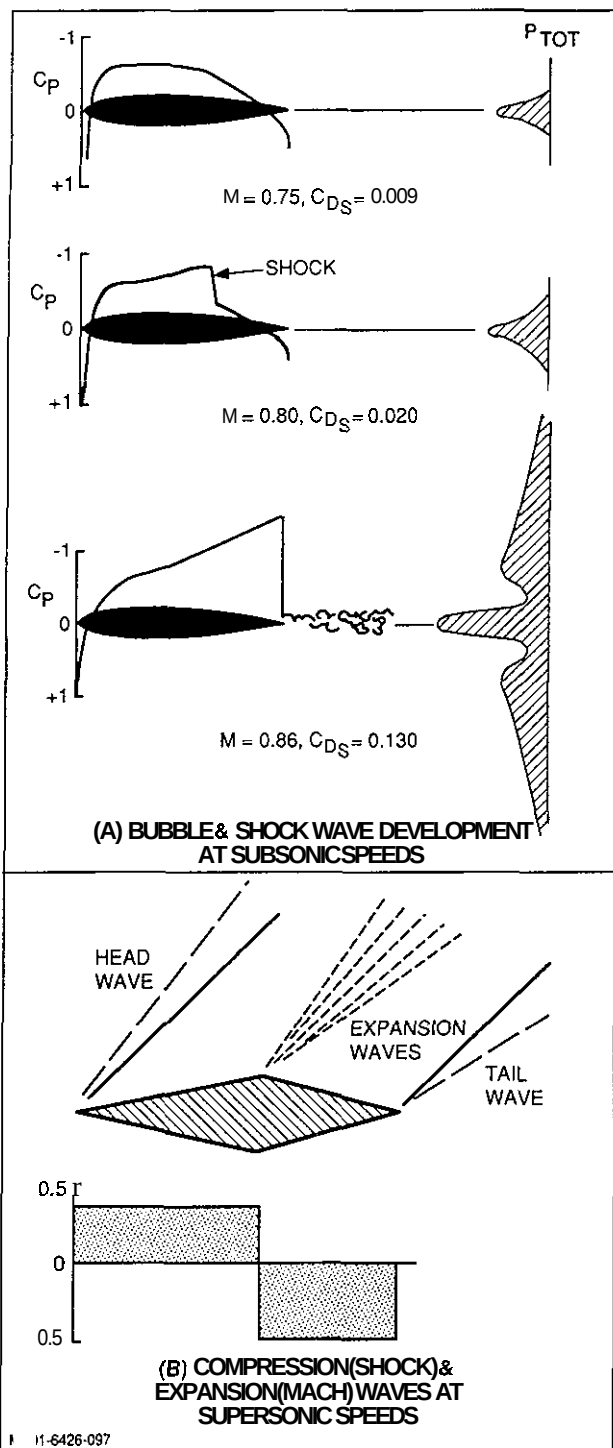
Fig. 5 Sources of Wave Drag at Subsonic & Supersonic Speeds (Ref. 16)
