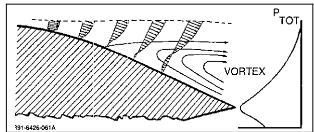
Fig. 1 Boundary Layer Velocity Characteristics with Wake Total Pressure
