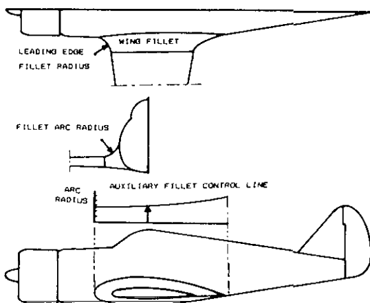
Fig. 16 Wing fillet layout.
