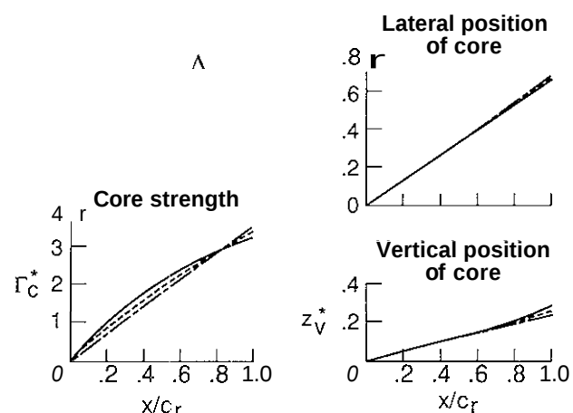
Fig. 5. Leading-edge vortex characteristics for thin delta wings; M = 0 , K = 1 .
