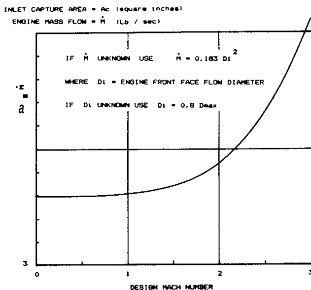
Fig. 36 Preliminary capture area sizing.
