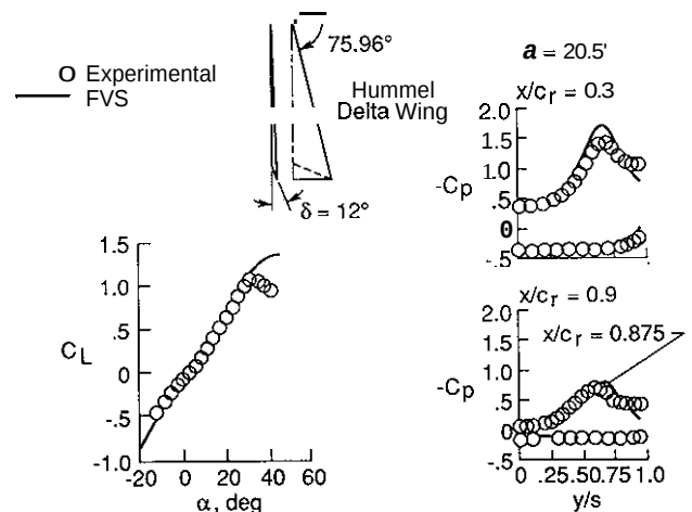
Fig. 36. FVS solution; A = 1 delta, M \approx 0
