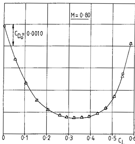
FIG 1 REPEATABILITY STANDARD WITHIN A GIVEN TEST (ARA TRANSONIC TUNNEL; FROM REF 15)
