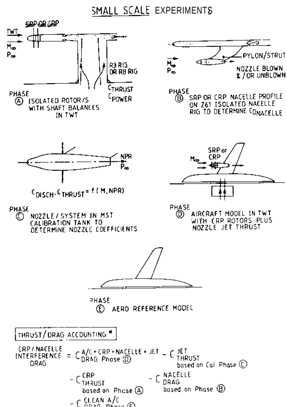
FIG 42(d) TYPICAL MODEL TEST PROGRAMME FOR TURBOPROP PROPELLER PERFORMANCE (FROM REF.105)
