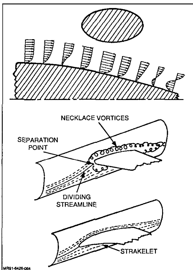
Fig. 8 Examples of Component Interference Effects
