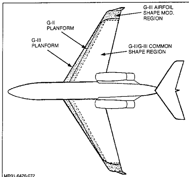
Fig. 62 Gulfstream II/III Wing Planforms with G-III Airfoil Contour Modification Region
