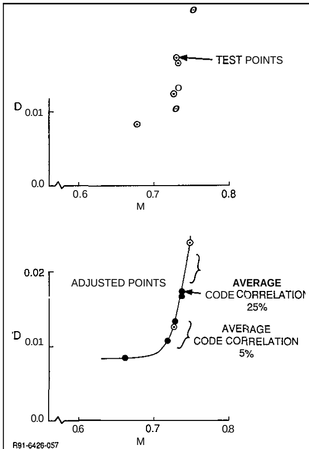
Fig. 23 RAE-2822 Airfoil Drag Divergence Curve Data & Adjusted Data ( C_L = 0.74 )
