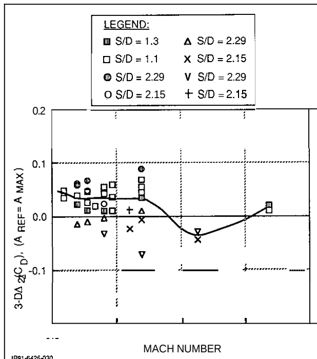
Fig. 49 ERB/Spacing Effects – Maximum A/B Nozzle
