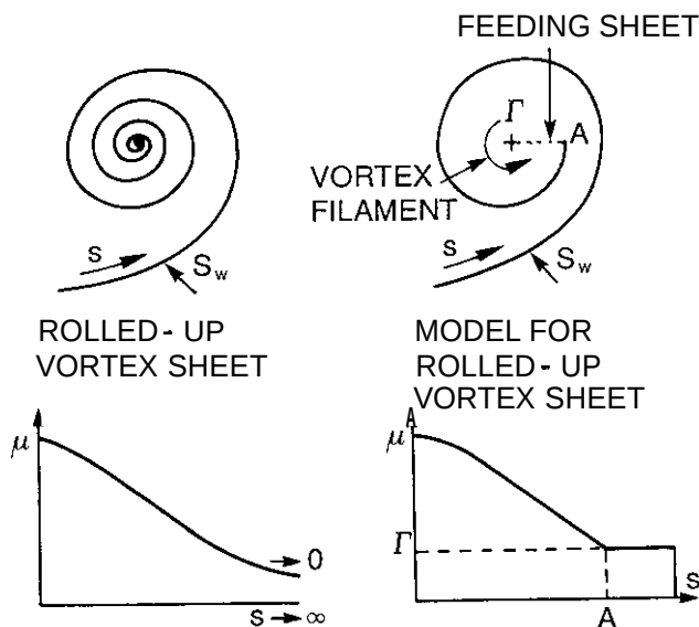
Fig. 4.4 Model for rolled-up vortex sheet
