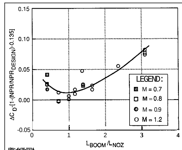
Fig. 53 Boom Correlation – Maximum A/B Nozzle
