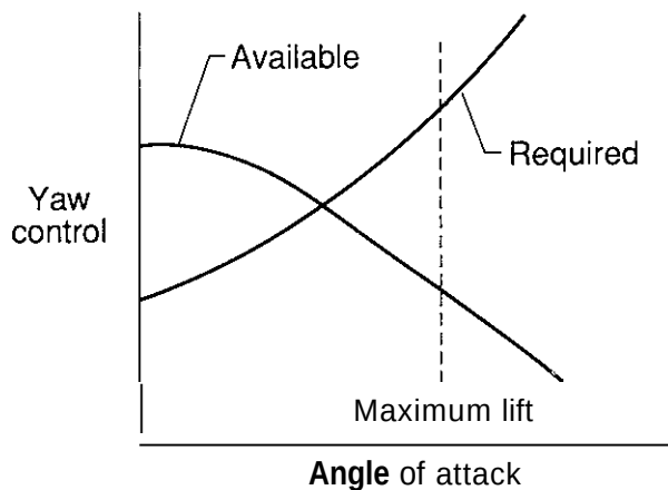
Fig. 76. Typical yaw control requirements for maneuvering.
