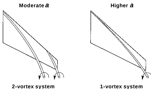
Fig. 3. Vortex systems on high aspect ratio wing; \Lambda = 65^\circ .
