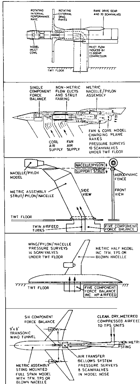
FIG 40 MODELS FOR TURBOFAN PERFORMANCE TESTING (FROM REF.10)
