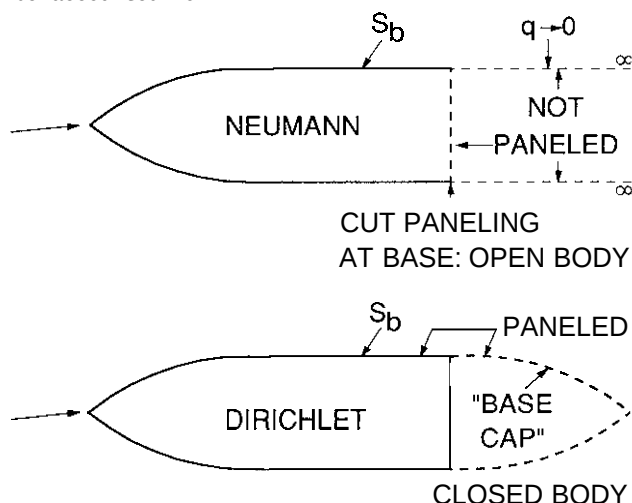
Fig. 8.4 Modeling separation from a body-like component
