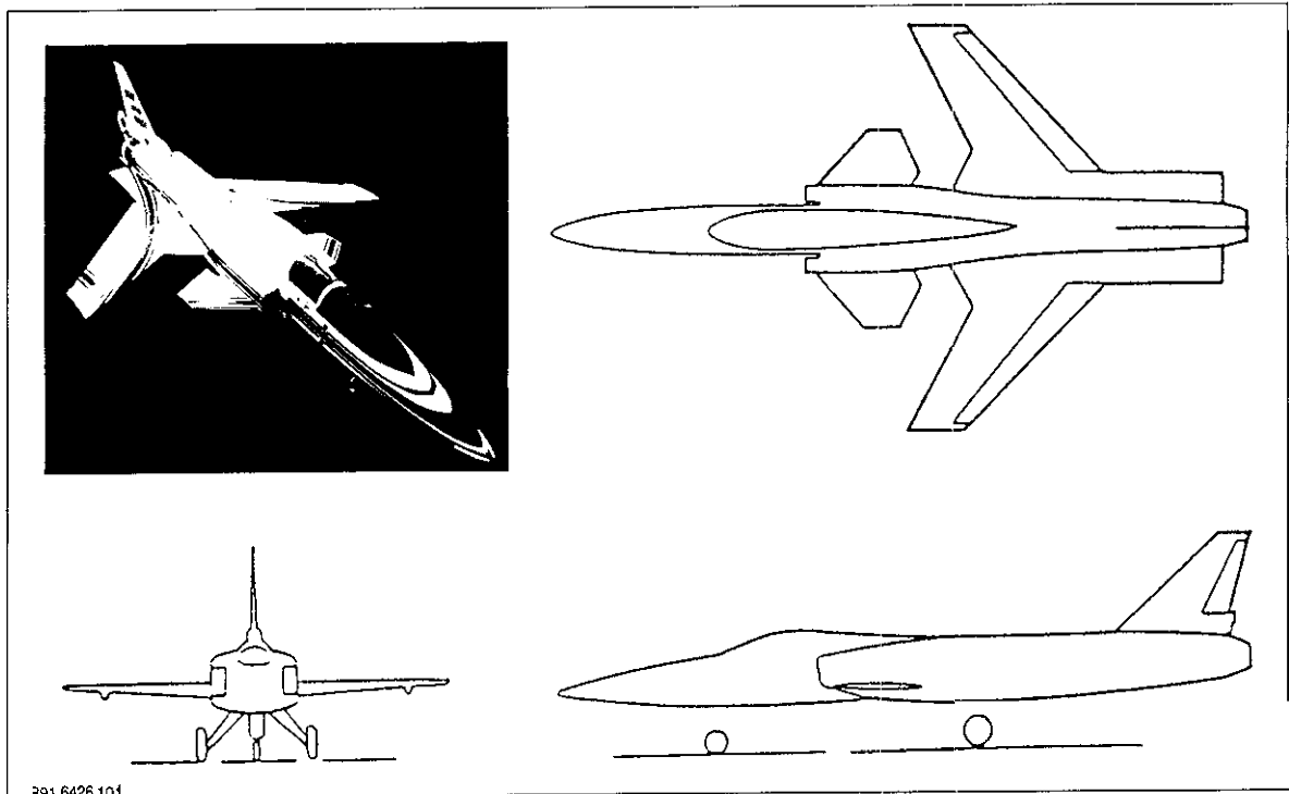
Fig. 91 X-29 Configuration
