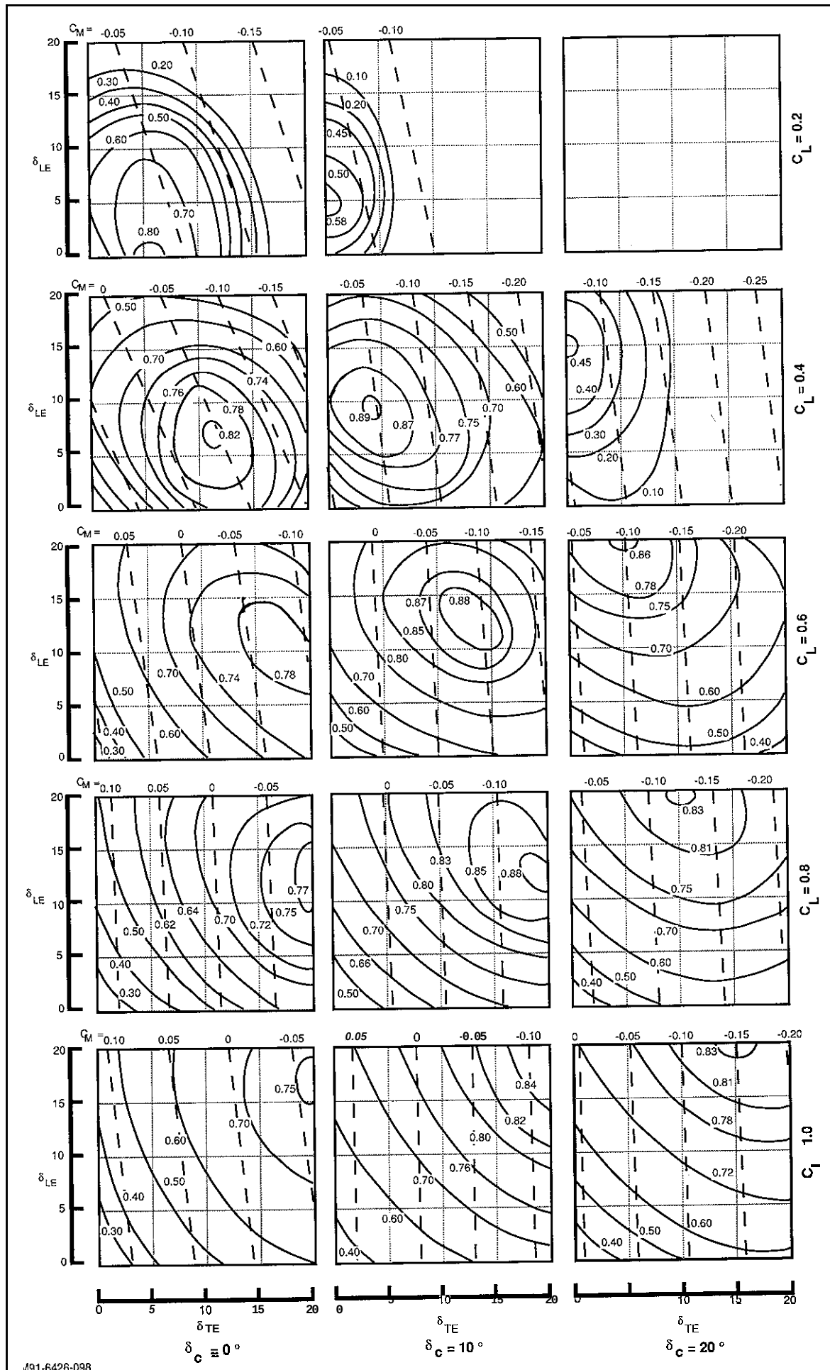
Fig. 57 Predicted Lift-Induced Drag Characteristics ( S_D Contours) for a Canard Configuration at Different Lift Levels as a Function of Canard & Leading/Trailing Edge Flap Deflections
