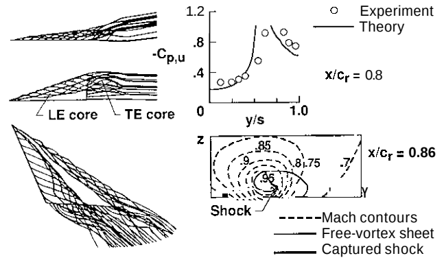
Fig. 34. Typical free vortex filament solution; A = 1.5 delta, M = 0.7 , a = 15^\circ .
