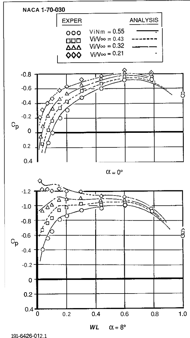
Fig. 30 Inlet Top Centerline Pressure Distribution Correlations (cont'd)
