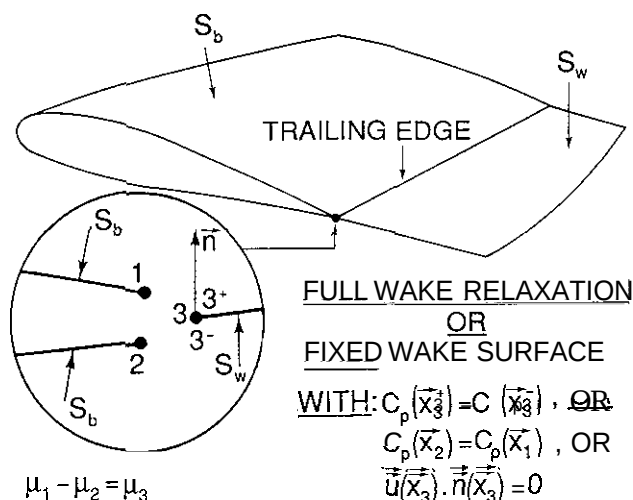
Fig. 3.14 Kutta conditions
