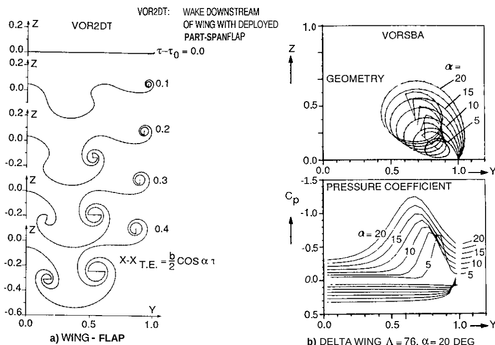
Fig. 8.5 Example of results of panel methods for configurations with free vortex sheets; approximate frame works, a) time-dependent analogy, b) slender-body approximation
