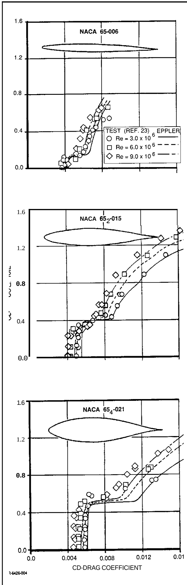
Fig. 13 2-D Airfoil Drag Correlation-Thickness Effects
