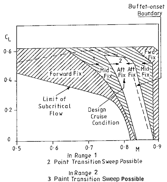
FIG 32c USEFUL RANGES WITH DIFFERENT TRANSITION TRIPS
