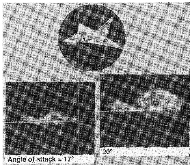
Fig. 6. Multiple vortices found above wing of F-106B during flight; alt. = 25,000 ft., M = 0.4 , R_n = 33 \times 10^6 .
