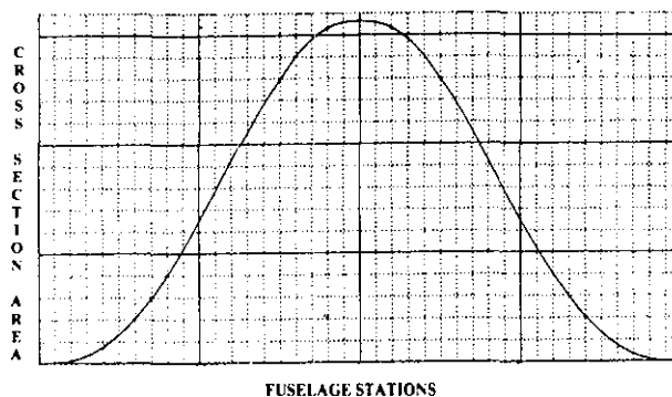
Fig. 18 Sears-Haack volume distribution
