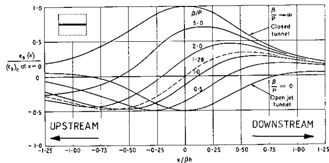
FIG 19 LONGITUDINAL DISTRIBUTION OF BLOCKAGE IN A 2D PERFORATED WALL TUNNEL (FROM REF 48)
