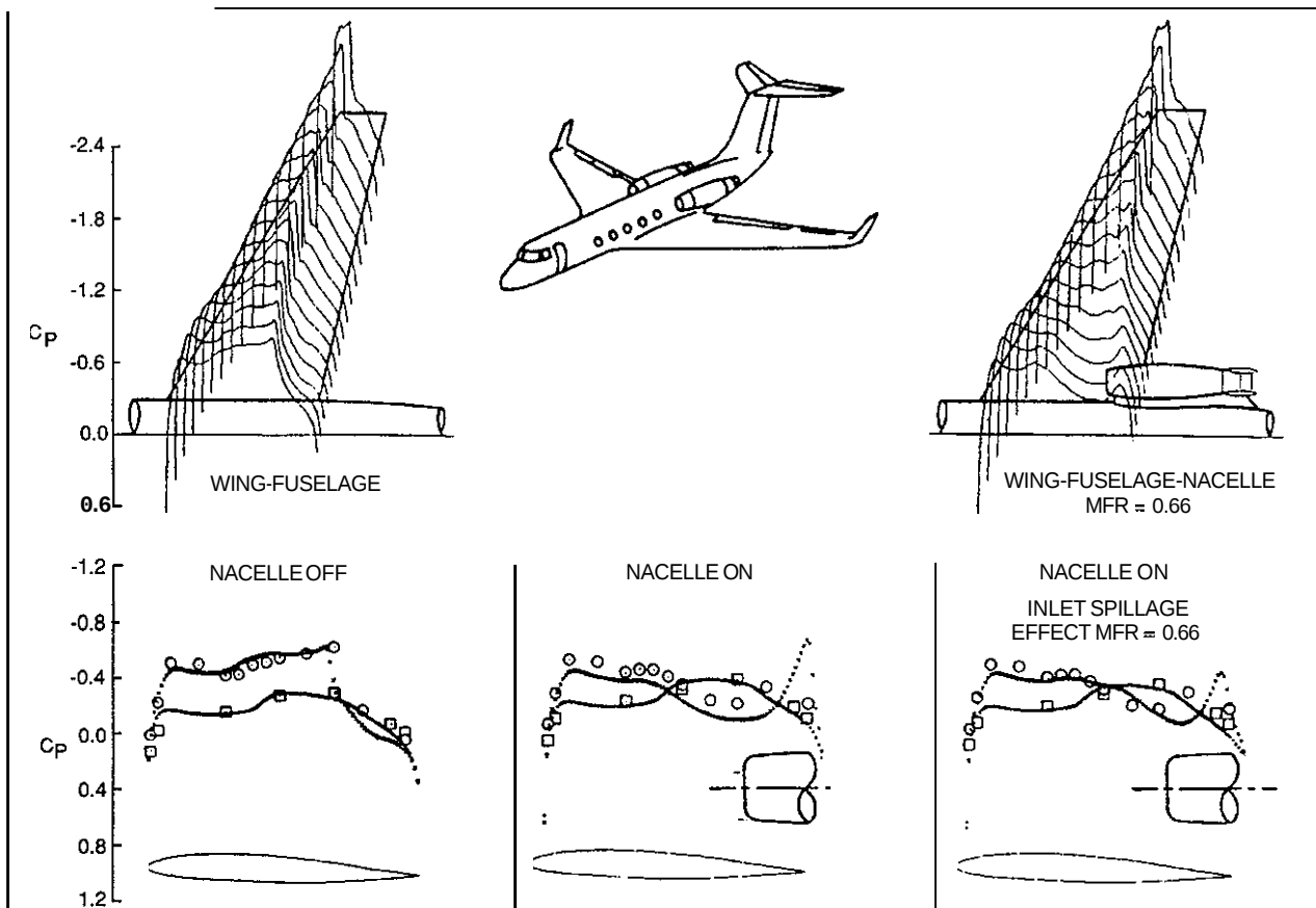
Fig. 42 Superimposed Computed Pressure Distributions & Wing Root Pressure Correlation for G-III Configuration ( M = 0.85 , \alpha = \text{Deg} )
