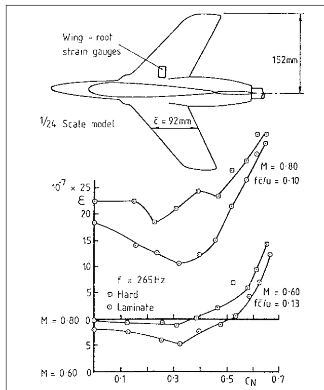
FIG 16 DEPENDENCE OF RMS UNSTEADY WING-ROOT STRAIN ON SURFACE OF TUNNEL SLOTTED WALLS (FROM REF 41)
