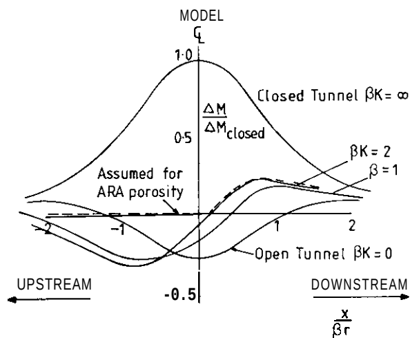
FIG 21 BLOCKAGE BUOYANCY CORRECTIONS FOR ARA TRANSONIC TUNNEL
