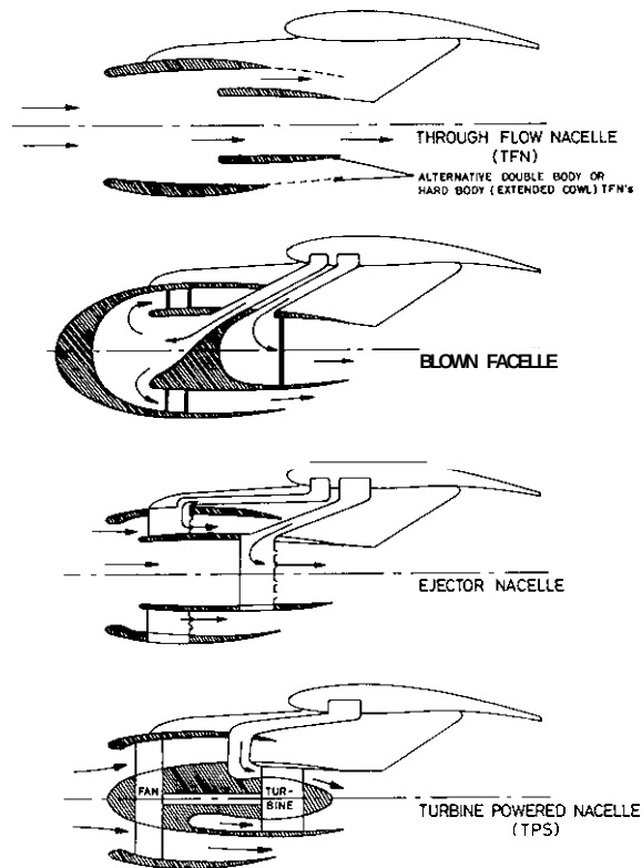
FIG 37 TYPES OF SIMULATOR (FROM REF.9)
