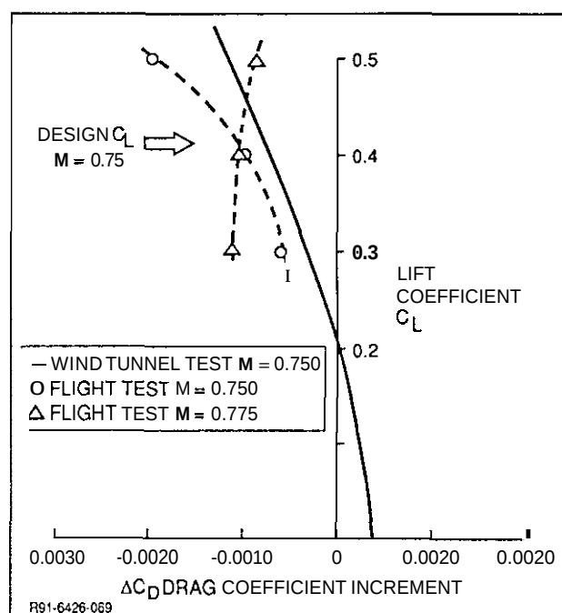
Fig. 61 G-III Winglet Drag Increment
