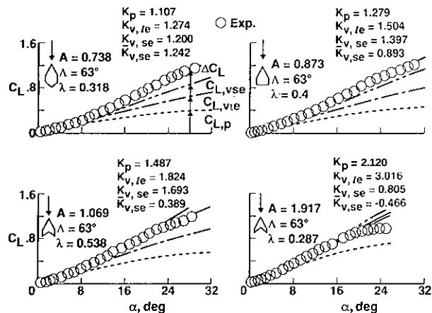
Fig. 25. Lift characteristics of wings with streamwise tips; M \approx 0 .
