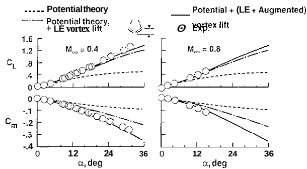
Fig. 62. Effect of Mach number on augmented vortex lift and pitch; diamond wing, A = 0.943 , A = 74^\circ
