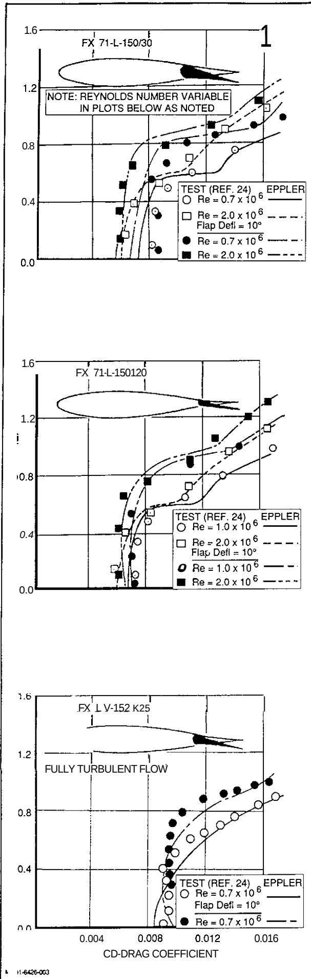
Fig. 15 2-D Foil Drag Correlation-Tab Deflection/Length Effects
