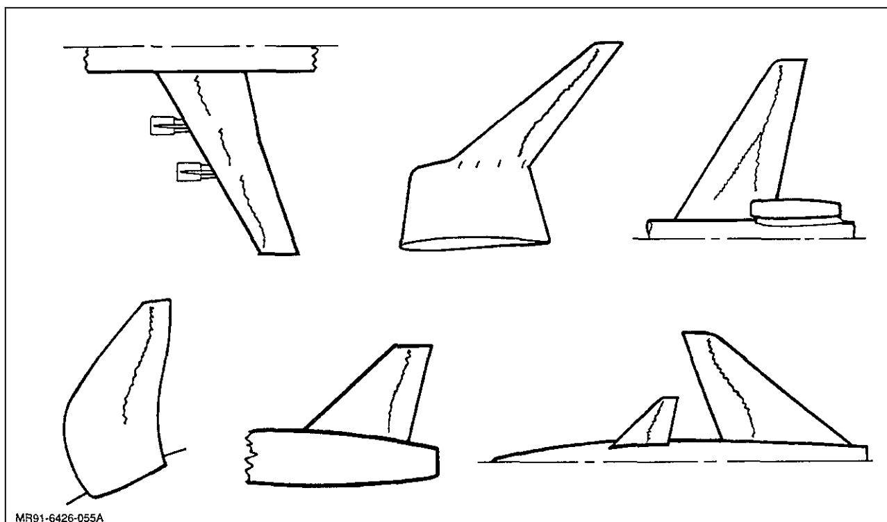
Fig. 19 Shock Wave Unsweep Regions
