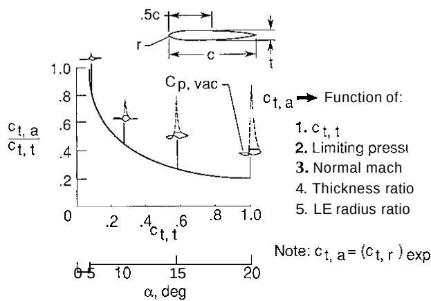
Fig. 32. Carlson's method for predicting residual thrust; M = 0.6 , t/c = 0.12 , r/c = 0.0048 .
