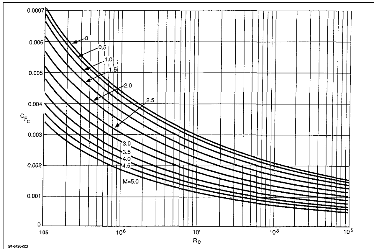
Fig. 12 Karman-Schoenherr Compressible Average Skin Friction Coefficient T_w = T_{ad}
