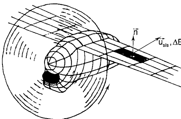
Fig. 8.1 Simple modeling of effect of propeller slipstream on flow about the wing
