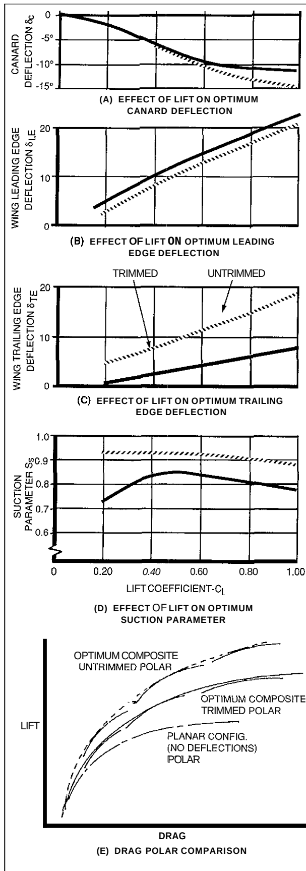
Fig. 58 Optimum Drag Polar Shape Constructed Using Multiple "Lift" Polars Generated with Control Surface Deflections
