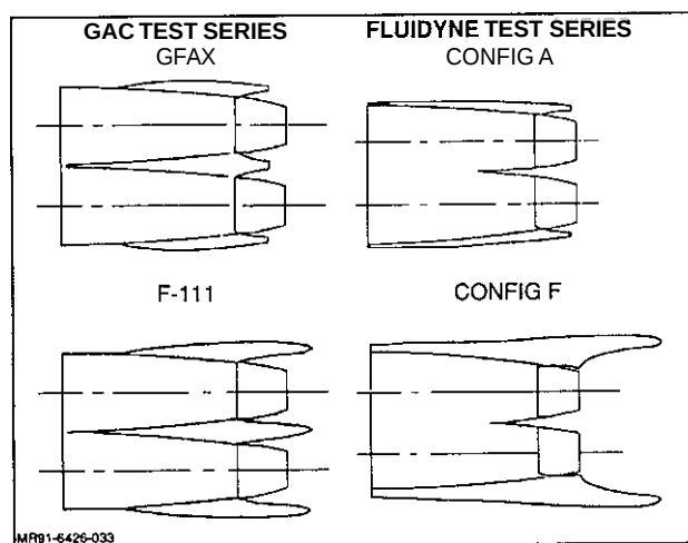
Fig. 50 Boom Configurations
