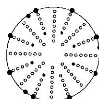
FIG 46 TYPICAL ENGINE FACE INSTRUMENTATION
