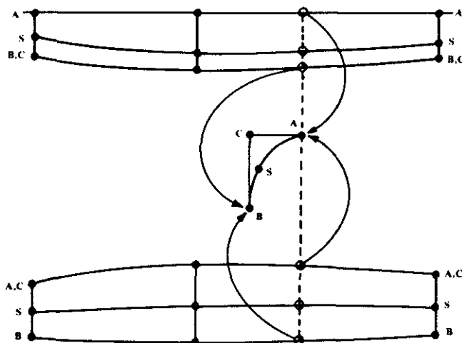
Fig. 46 Cross section development from longitudinal control lines.
