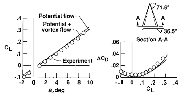
Fig. 28. Longitudinal aerodynamic characteristics of delta wing with conical LE flap; A = 1.333 , M = 1.4 , VORCAM.
