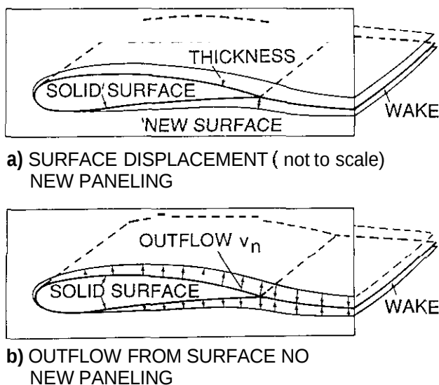
Fig. 8.3 Simulation of boundary-layer effects
