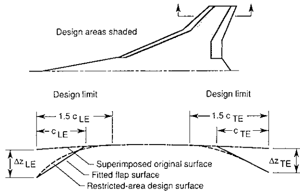
Fig. 50. Fitting of flap surfaces to wing-design surface.
