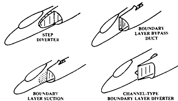
Fig. 37 Boundary layer removal.
