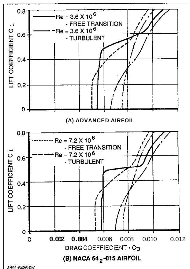
Fig. 72 Predicted Drag Polar Characteristics for NACA 64 2 -015/Advanced Airfoil Sections
