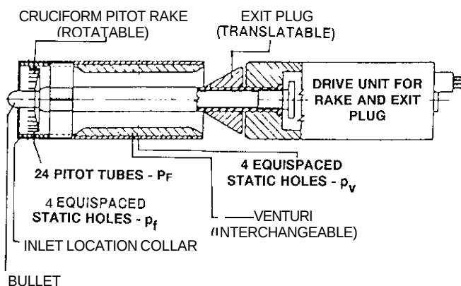
FIG 47 RAE UNIT FOR MEASURING MASS FLOW AND PRESSURE RECOVERY (FROM REF. 123)
