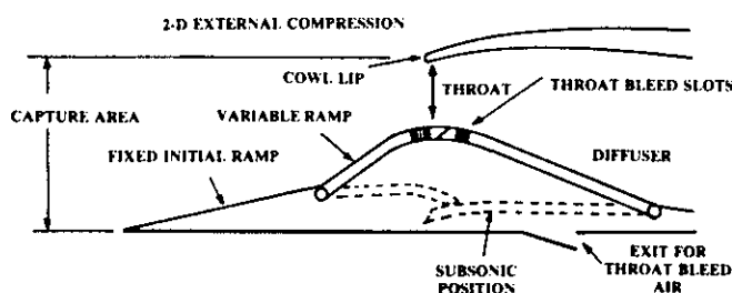
Fig. 32 Variable inlet geometry.
