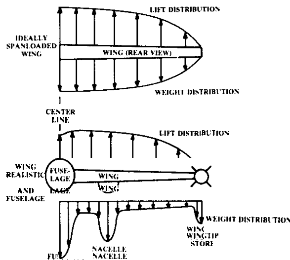
Fig. 25 Spanloading for weight reduction
