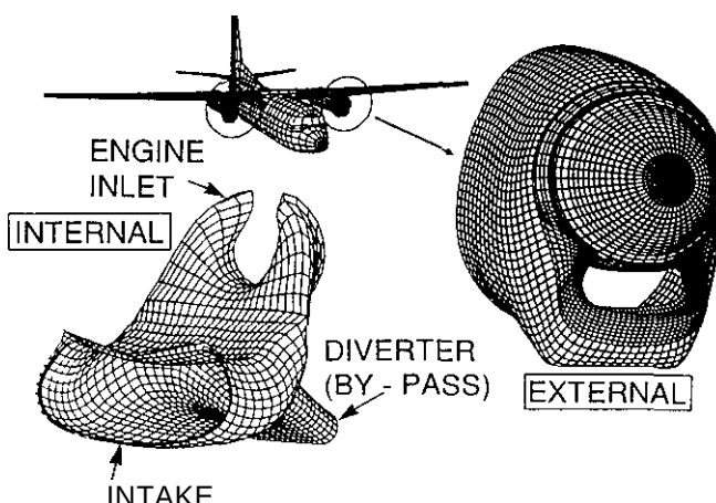
Fig. 6.2 Geometry modeling (Courtesy Fokker Aircraft B.V.)
