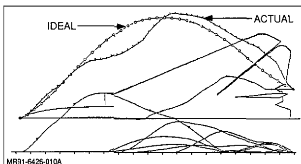
Fig. 27 F-14 Optimized Normal Area Distribution
