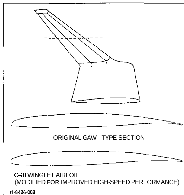
Fig. 60 Originally Proposed & Final G-III Winglet Airfoil Section
