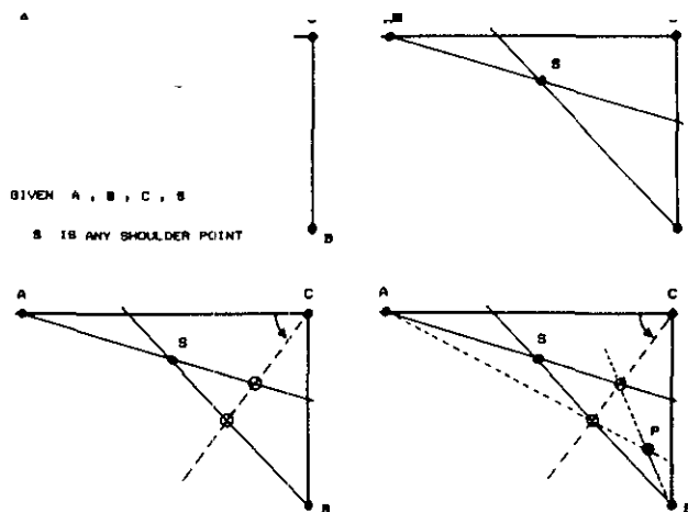
Fig. 44 Conic layout.
