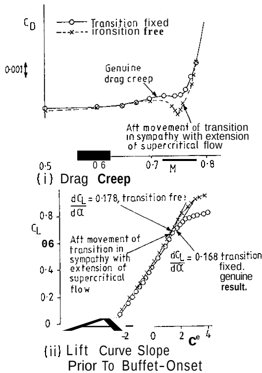
FIG 31 EXAMPLES OF SPURIOUS RESULTS WITH FREE TRANSITION
