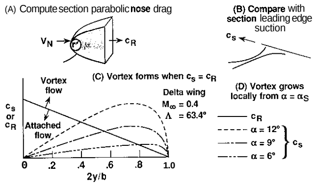
Fig. 31. Kulfan's method of predicting vortex normal force
