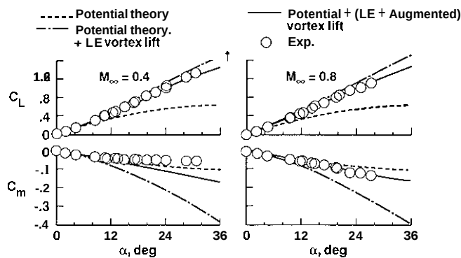
Fig. 63. Effect of Mach number on augmented vortex lift and pitch; arrow wing, A = 1.463 , A = 74^\circ
