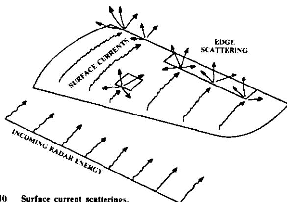
Fig. 40 Surface current scatterings.
