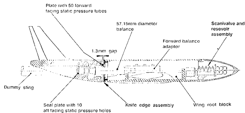
FIG 27a DETAILS OF BALANCED REAR FUSELAGE TO OBTAIN STING CORRECTIONS USING CURRENT TWIN STING RIG AT ARA (FROM REF 15)
