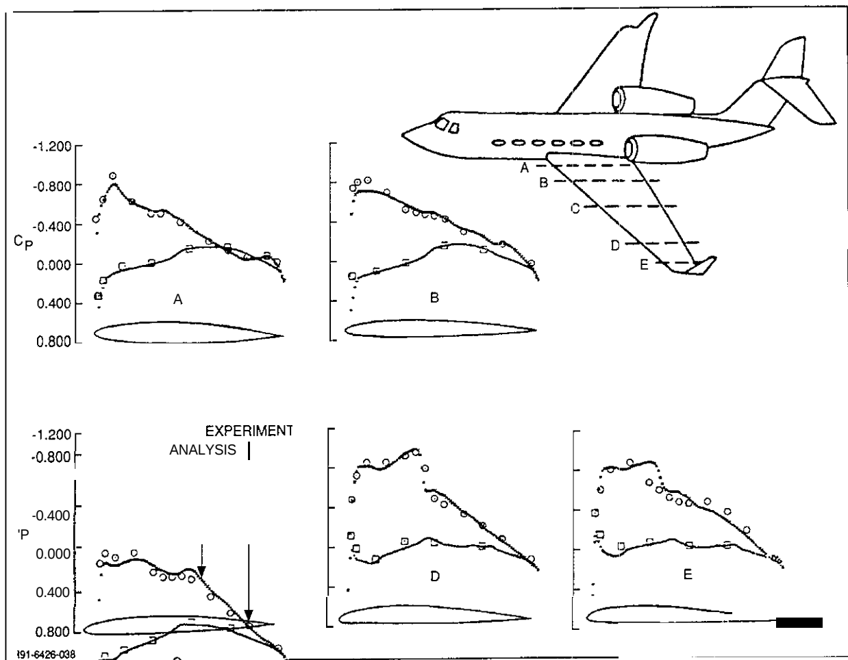
Fig. 69 Correlation of G-IV Wind Tunnel Test Pressure Distributions with Pre-Test Code Prediction ( M = 0.78 , \alpha = 4.0^\circ )
