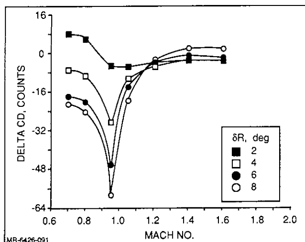
Fig. 80 F-14D Delta C_D for Rudder Deflection Angles
