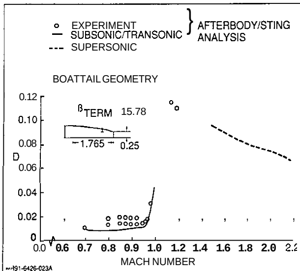
Fig. 43 Prediction of Tri-Sonic Drag Characteristics of Boattail-Sting Configuration (Case No.1)
