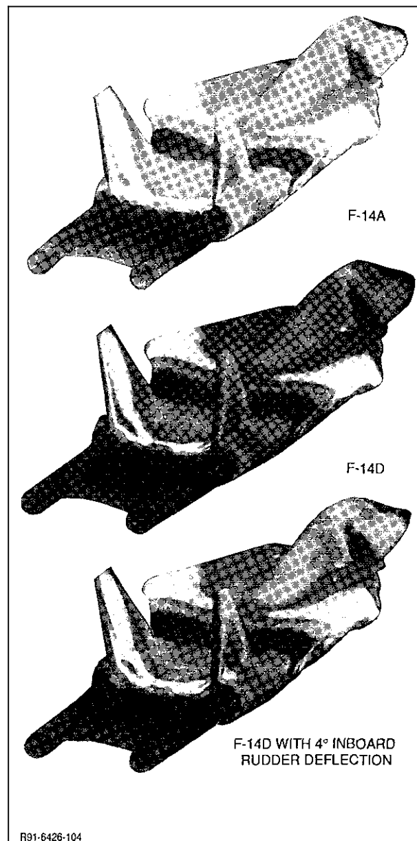
Fig. 77 Navier-Stokes Analysis for F-14 Buffet at M = 0.95
