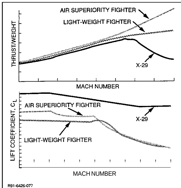
Fig. 94 Maximum Lift & Thrust/Weight Comparison (Ref. 83)
