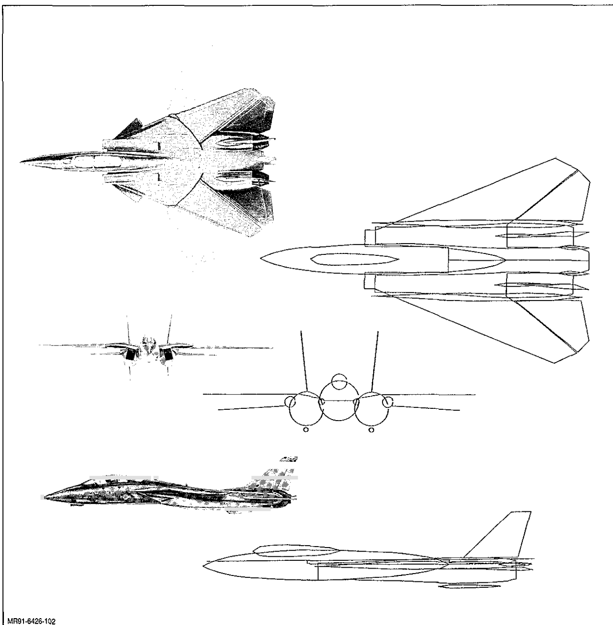
Fig. 26 F-14 Harris Wave Drag Program Model (Body & Wing Elements)
