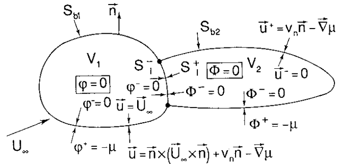
Fig. 3.6 Dirichlet condition on \varphi and \Phi
