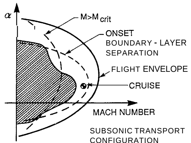
Fig. 2.1 Domain of applicability of panel method (adapted from Ref. 33)
