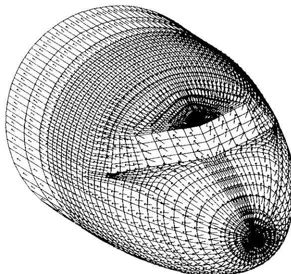
Fig. 6.3 Surface velocity vectors (Courtesy Fokker Aircraft B.V.)
