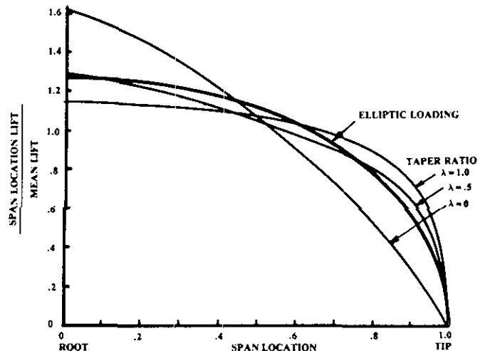
Fig. 10 Effect of taper on lift distribution.
