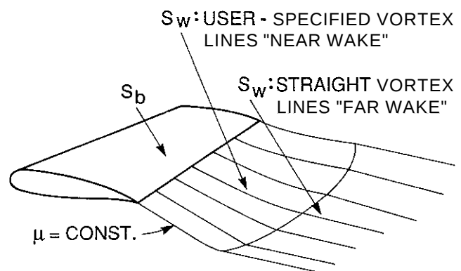
Fig. 3.9 Variation on rigid-wake approximation
