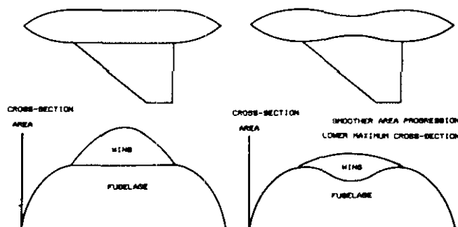
Fig. 19 Design for low wave drag.
