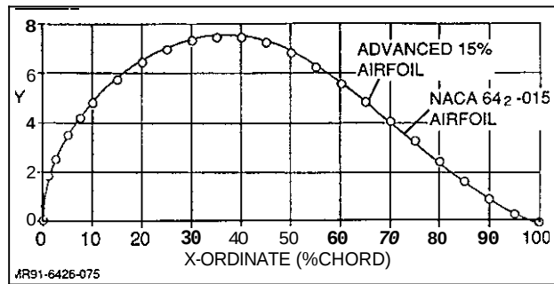
Fig. 71 NACA 64 2 -015/Advanced Airfoil Shape Comparison
