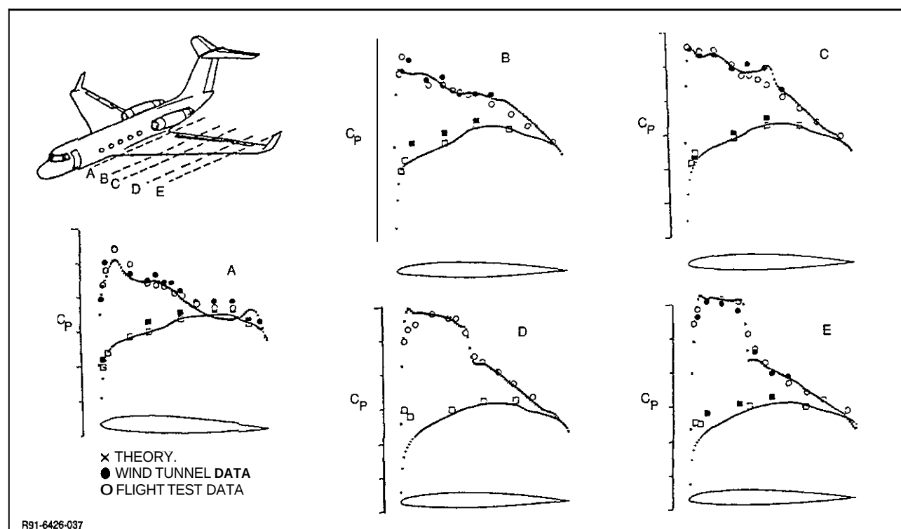
Fig. 66 G-III Wing Pressure Distribution Comparison at Cruise Condition ( M = 0.78 , \alpha = 4^\circ )
