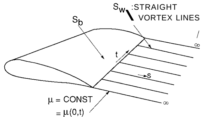
Fig. 3.8 Classical rigid-wake approximation
