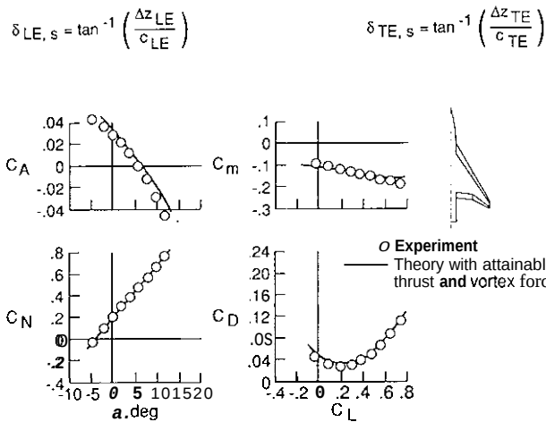
Fig. 51. Theoretical and experimental data for 60°-swept trapezoidal wing fighter; M = 0.3 , R_n = 1.9 \times 10^6 , \delta_{LE,s} = 15^\circ/20^\circ , \delta_{TE,s} = 15^\circ/12^\circ
