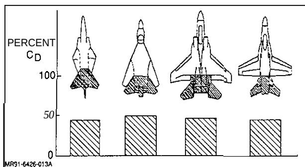
Fig. 32 Fighter Afterbody Drag Levels at Subsonic Speeds, C_L = 0
