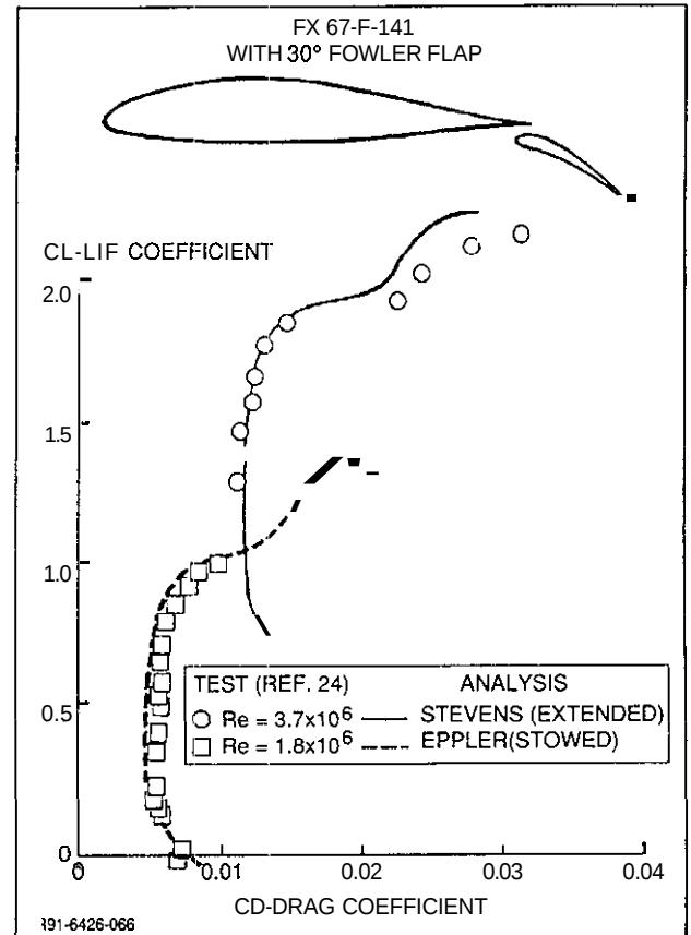
Fig. 16 Eppler & Stevens Method Prediction of Airfoil-Fowler Flap (Extended & Stowed) Drag Polars
