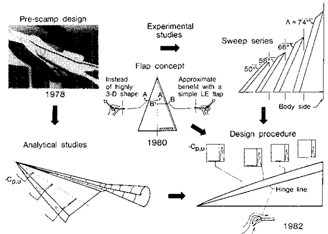
Fig. 53. Vortex flap history; transonic aerodynamics.
