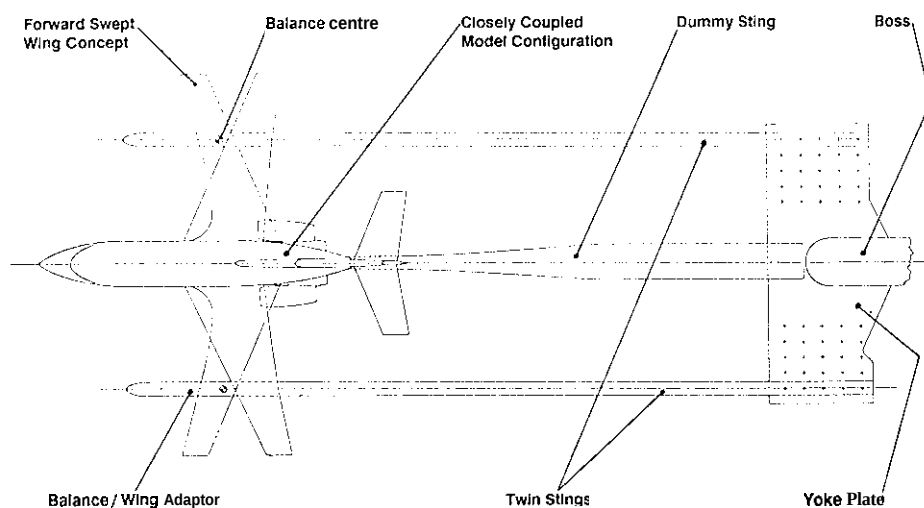
FIG 28 GENERAL LAYOUT OF MODEL IN ENHANCED TWIN STING RIG
