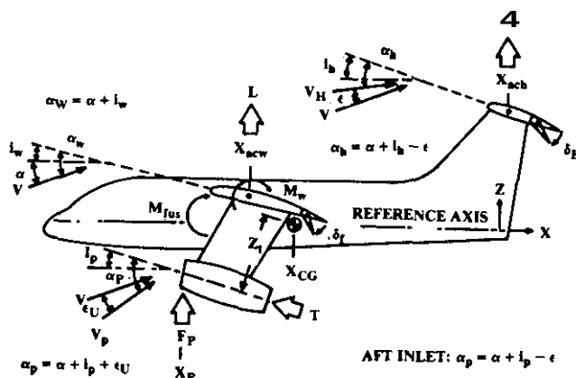
Fig 20 Longitudinal moments.
