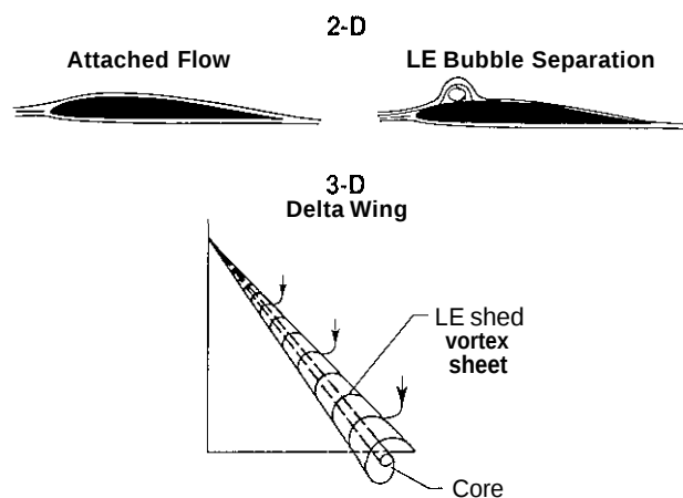
Fig. 2. Flow sketches.
