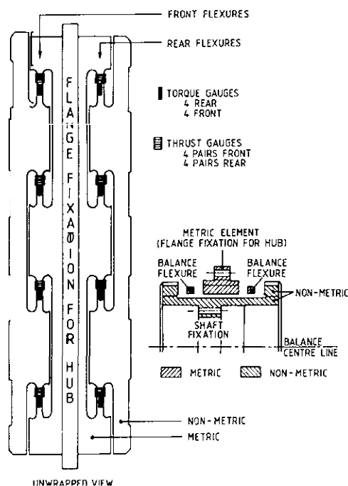
FIG 42(c) BALANCE DESIGN FOR CONTRA-ROTATING PROPELLER
