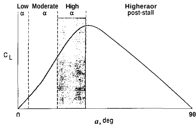
Fig. 1. Schematic of lift curve by \alpha ranges
