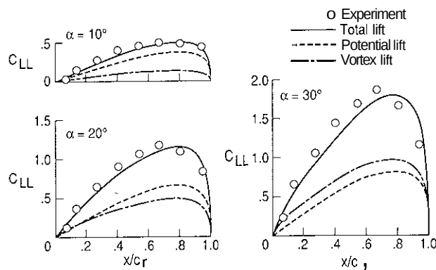
Fig. 14. Longitudinal load distribution; A = 1.147 delta. M \approx 0 .
