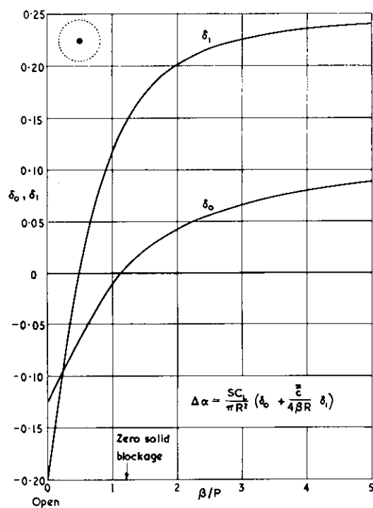
FIG 20 LIFT TUNNEL CONSTRAINT FOR A SMALL MODEL IN A PERFORATED CIRCULAR TUNNEL (FROM REF 42)
