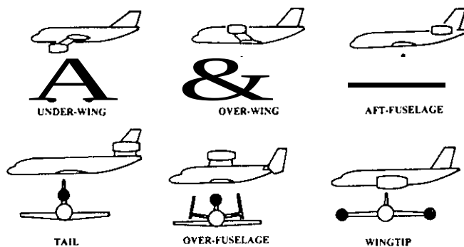
Fig. 35 Inlet locations—podded engines.
