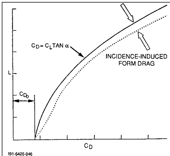
Fig. 88 Hypersonic Body Drag Polar "Dent"
