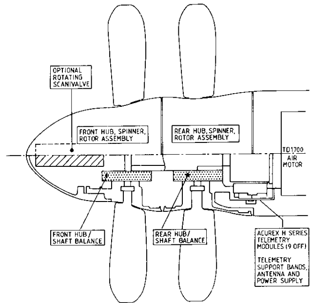
FIG 42(b) FRONT AND REAR HUB ASSEMBLIES
