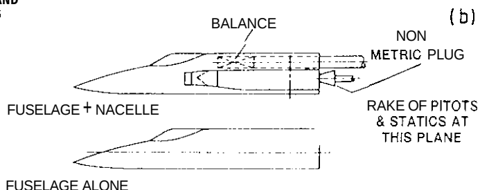
FIG 48 POSSIBLE SCHEMES FOR INTERNAL FLOW SURVEY AND FORCE MEASUREMENT
