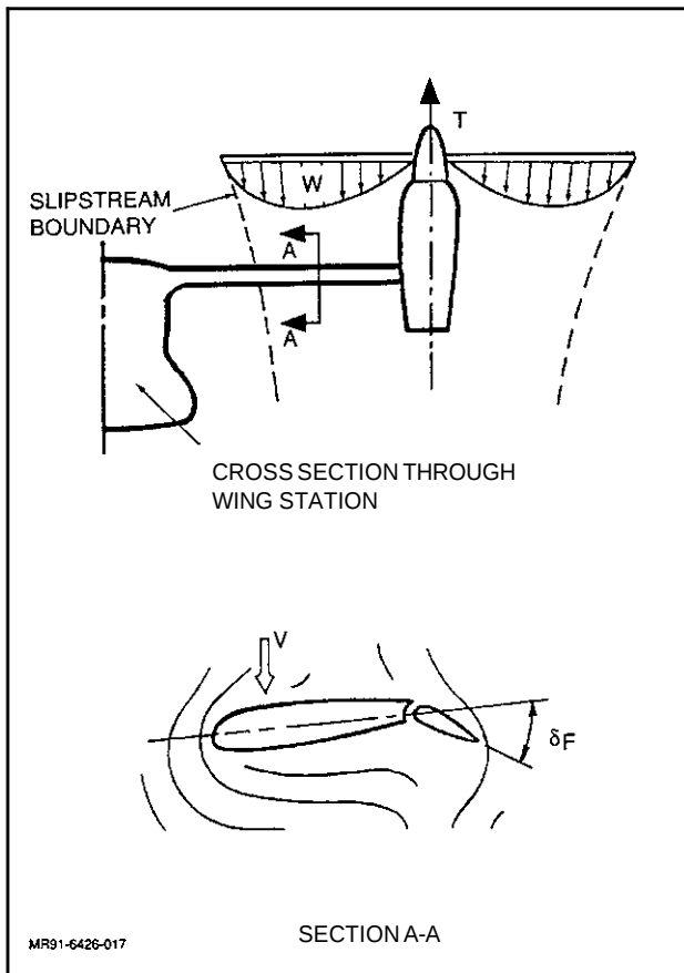
Fig. 40 Rotor Download Schematic (Ref. 58)
