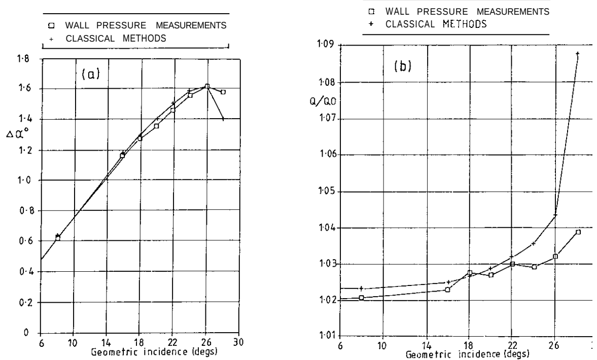
FIG 23 COMPARISON OF 2-COMPONENT WALL PRESSURE MEASUREMENTS AND CLASSICAL METHODS FOR PREDICTION OF TUNNEL INTERFERENCE (FROM REF 66)
