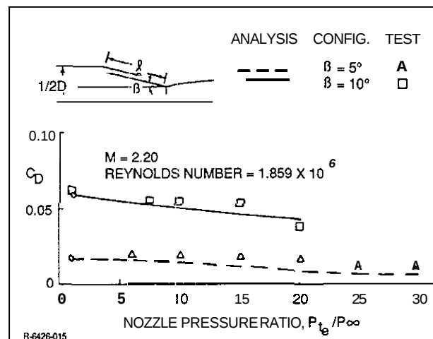
Fig. 34 Correlation of Nozzle Pressure Ratio Effects on Afterbody Drag Levels
