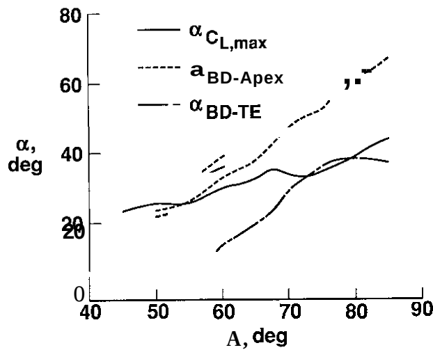
Fig. 8. Variation of \alpha for vortex breakdown and C_{L,max} for delta wings.
