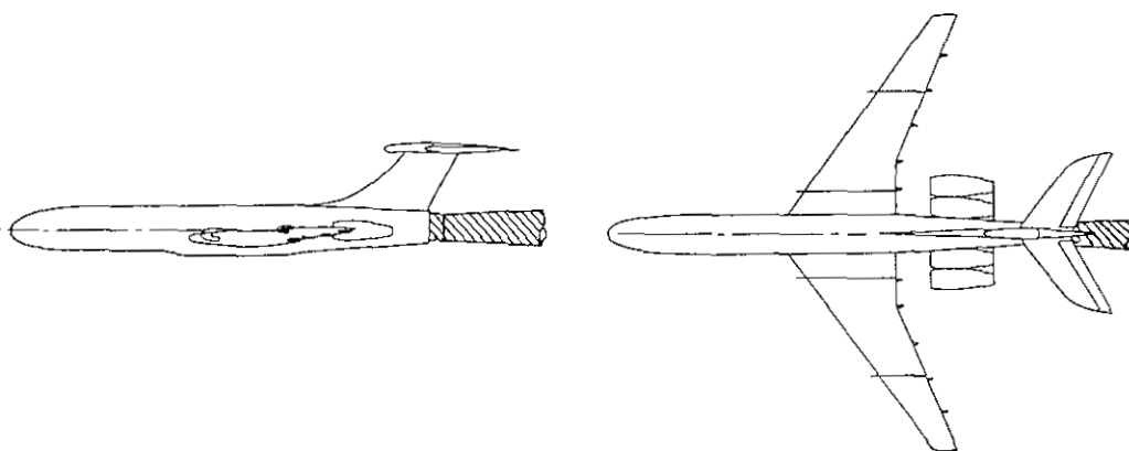
FIG 3c AIRCRAFT MODEL WITH 4 AFT-MOUNTED NACELLES
