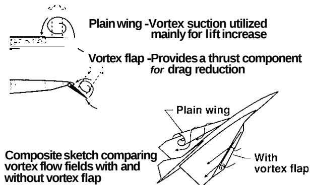
Fig. 52. The vortex flap concept.
