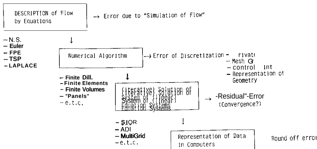
Fig. 5 Sources of errors in computational flow simulation codes
