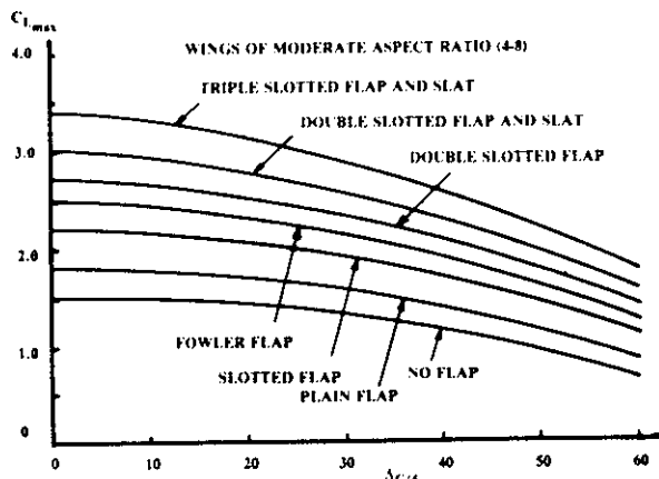
Fig. 13 Maximum lift coefficient.
