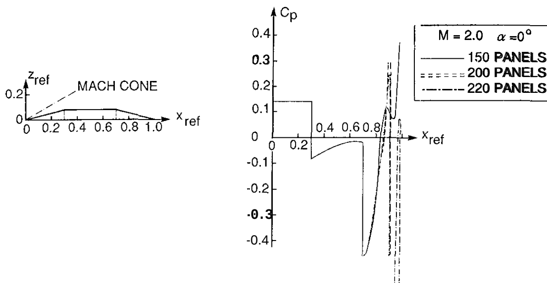
Fig. 4.10 Result of panel method with Neumann boundary conditions for supersonic flow (Ref. 9)
