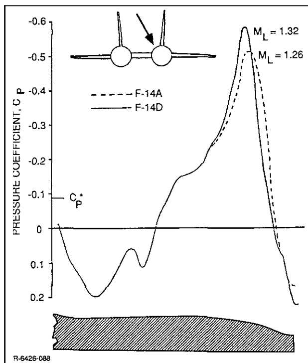
Fig. 76 Predicted F-14 Afterbody Pressure Field at M = 0.95
