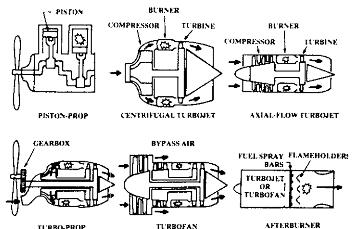
Fig. 28 Propulsion system options.
