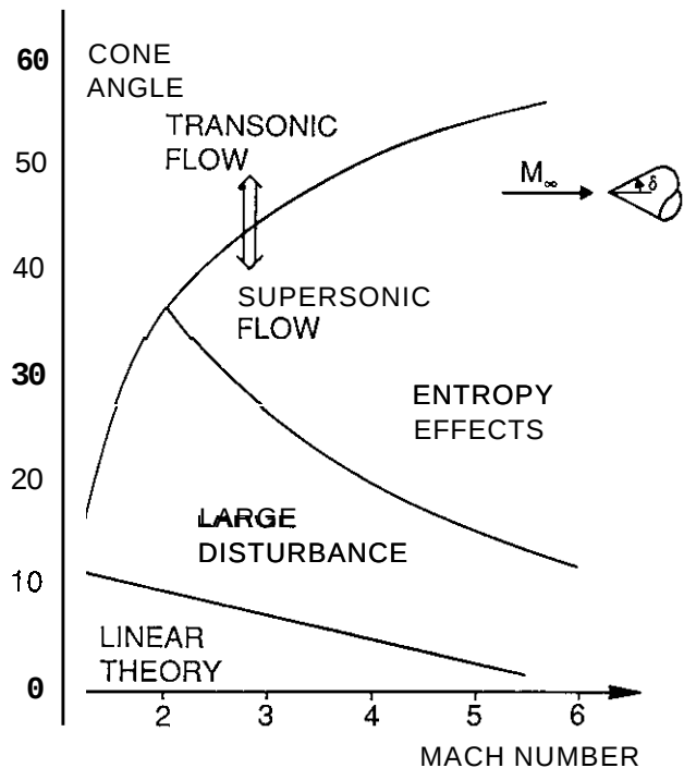
Fig. 2.2 Attached conical flow on a circular cone at zero incidence
