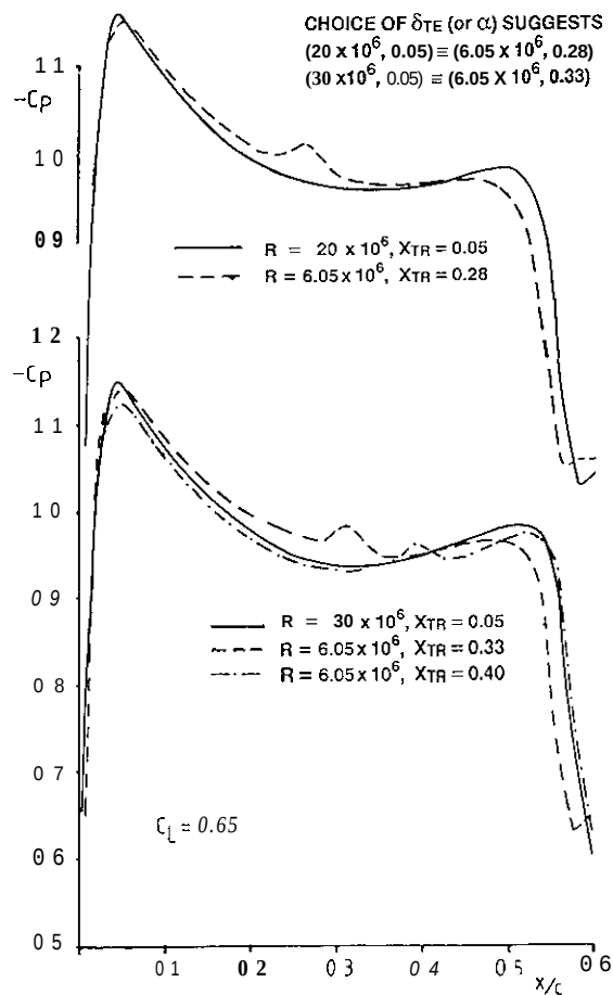
FIG 36c APPLICABILITY OF \delta_{TE}^* CRITERION: C_L = 0.65
