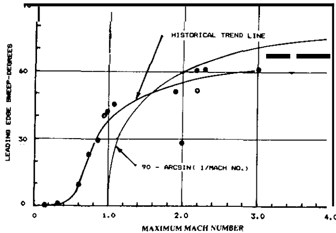
Fig. 8 Wing sweep historical trend.
