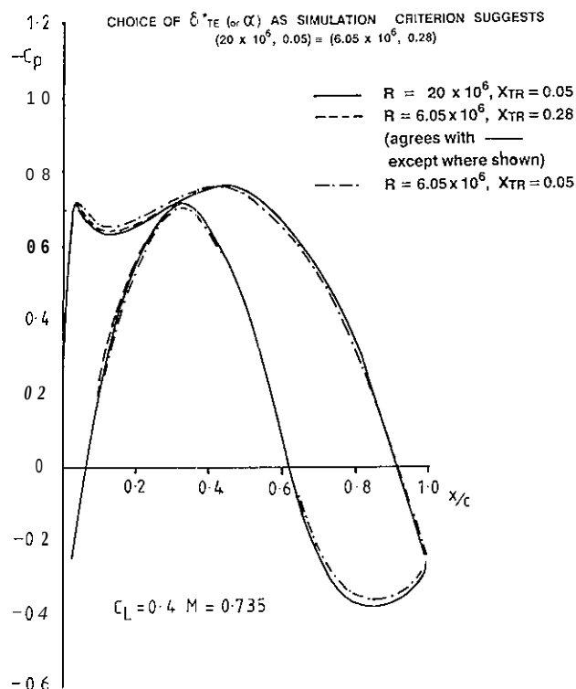
FIG 36b APPLICABILITY OF \delta_{TE}^* CRITERION: C_L = 0.4
