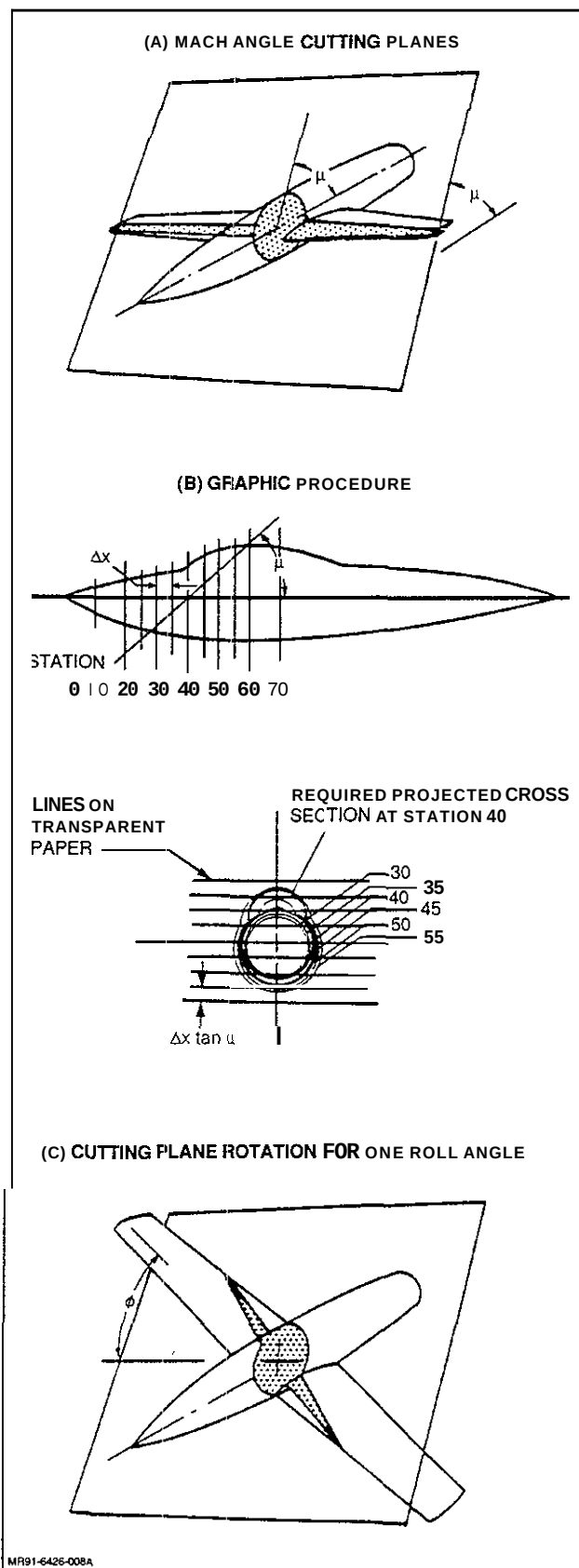
Fig. 25 Generation of Equivalent Body-of-Revolution for Supersonic Area Rule (Refs 17 and 39)
