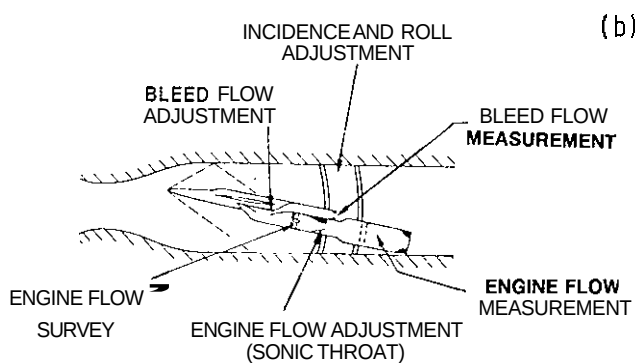
FIG 46 TYPICAL ENGINE FACE INSTRUMENTATION
