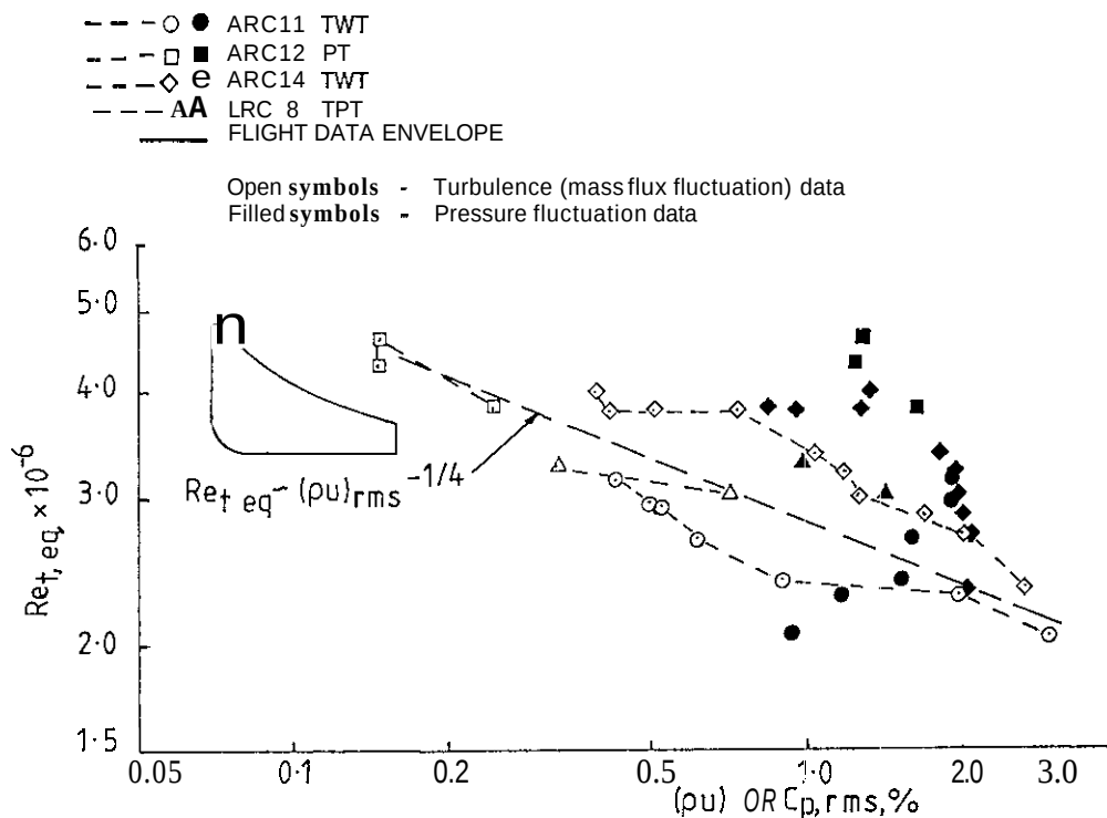
FIG 14 RESULTS OF REVISED ANALYSIS OF 10' CONE DATA (FROM REF 35)
