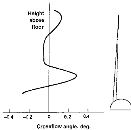
FIG 9 MEASURED WIND TUNNEL CROSSFLOW DISTRIBUTION (NASA AMES 11 x 11 TUNNEL; FROM REF 11)
