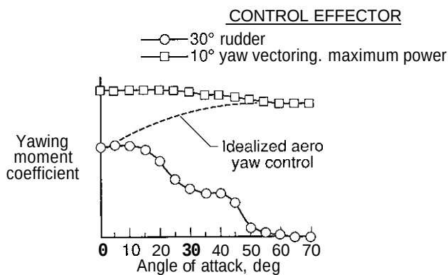
Fig. 82. Low-speed yaw control effectiveness; alt. = 20,000 ft. , M = 0.3 .
