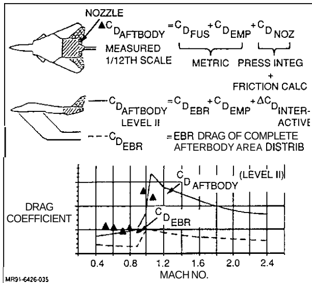
Fig. 54 F14 Afterbody Drag Prediction - Maximum A/B Nozzle
