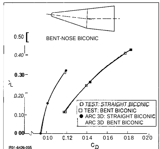
Fig. 87 Straight & Bent Biconic Drag Polar at Mach 6.0
