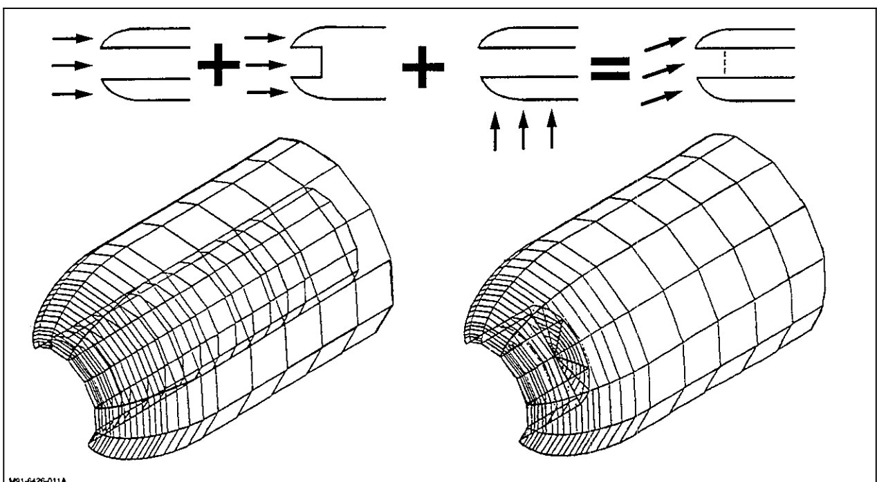
Fig. 29 Open/Closed Models for NACA Inlet Cases
