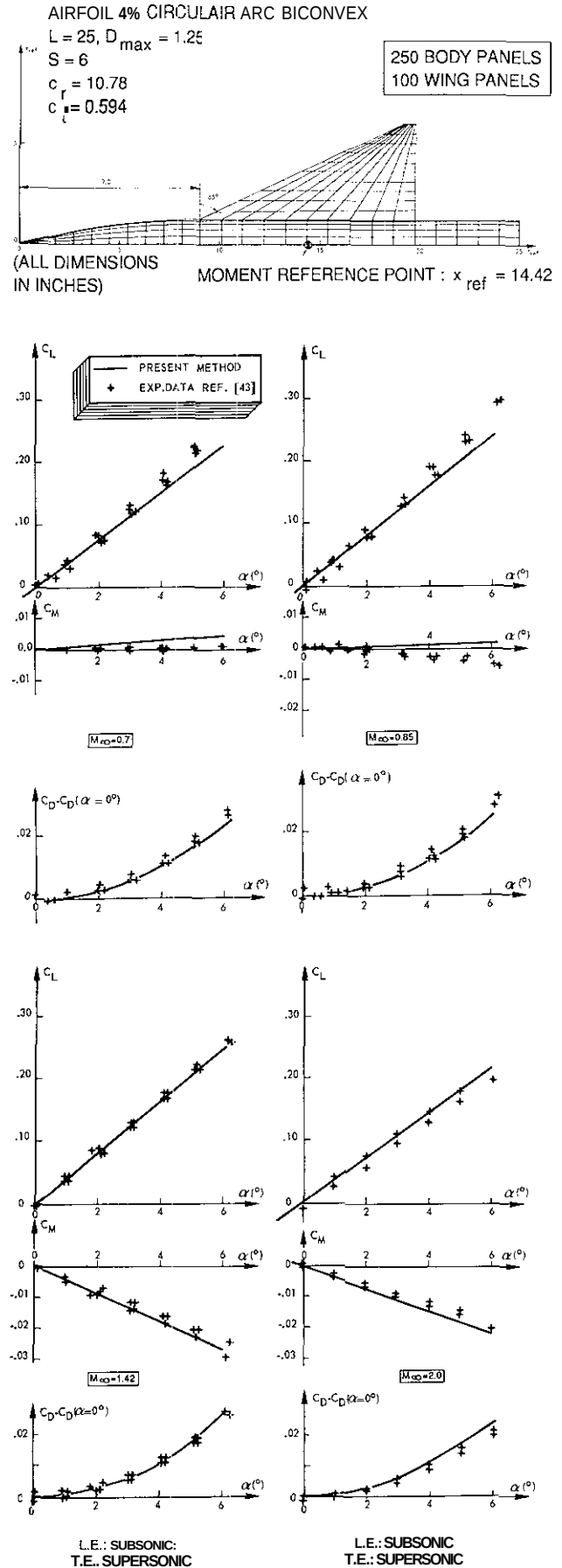
Fig. 5.6 Aerodynamic characteristics wing-body configuration predicted by NLRAERO method for sub- and supersonic flow.
