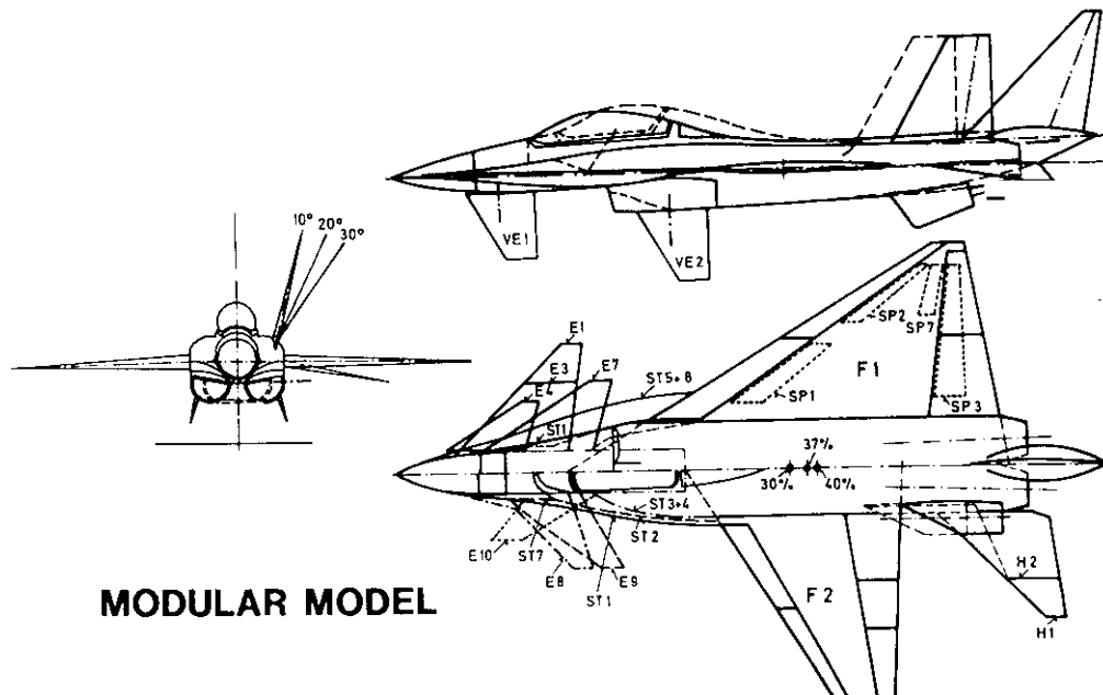
Fig. 3 Complexity of modular models during experimental configuration optimization
