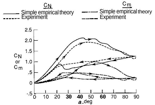
Fig. 83. Aerodynamic characteristics during pitching motions; A = 1 delta, M \approx 0 , K = 0.04 .
