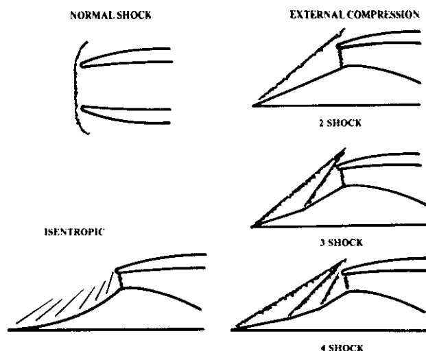
Fig. 31 Supersonic inlets--external shocks.
