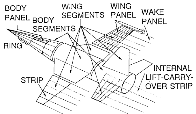
Fig. 4.2 Example of configuration paneling
