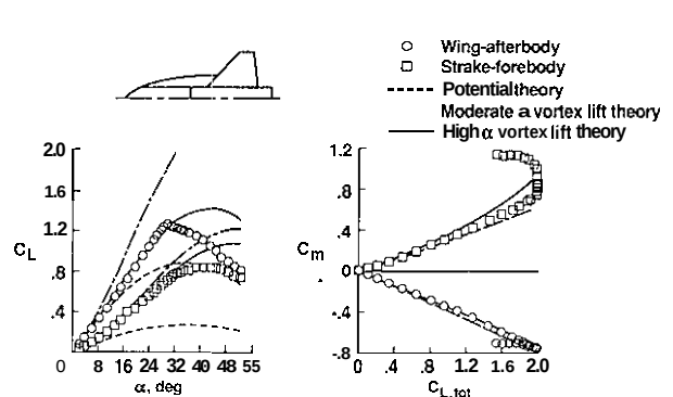
Fig. 67. Component longitudinal aerodynamic characteristics for strake-wing-body; strake AD 24, A = 44^\circ , M = 0.2 .
