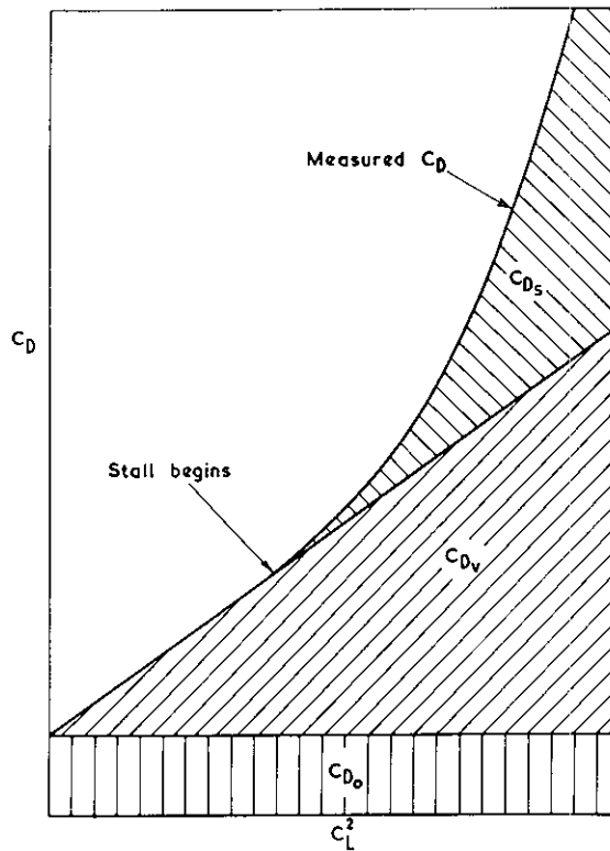
FIG 17 DRAG ANALYSIS FOR A LIFTING WING
