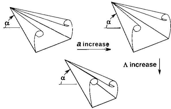
Fig. 10. Effect of \alpha and delta-wing sweep on vortex system displacement.
