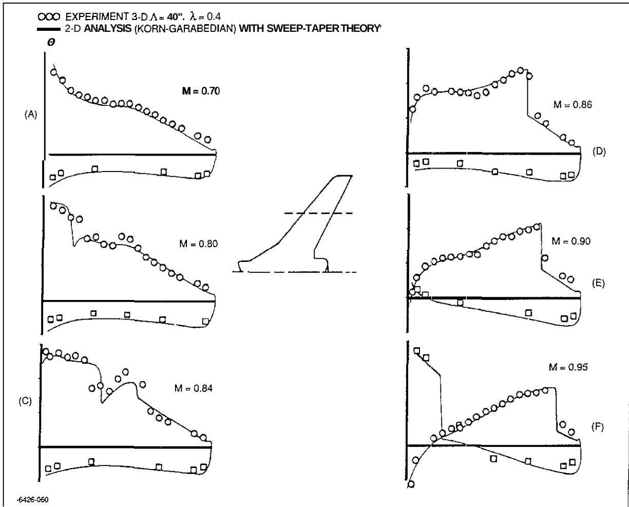
Fig. 21 Wing (3-D) Pressure Distribution Correlation using 2-D Airfoil Analysis & Sweep-Taper Theory
