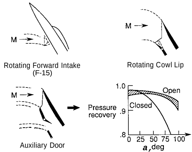
Fig. 84. High \alpha special inlet devices.
