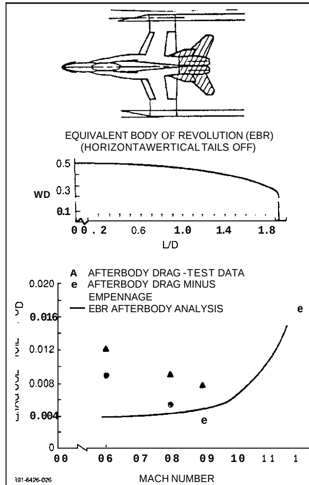
Fig. 46 Equivalent Body Approach Simulating F-18 Research Model Afterbody Drag
