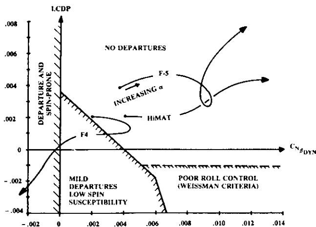
Fig. 23 Departure susceptibility.
