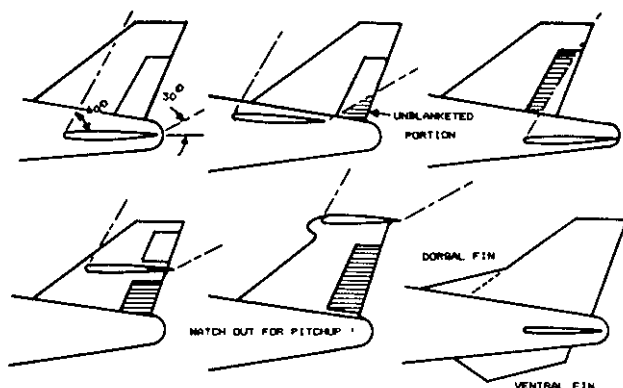
Fig. 24 Tail geometry for spin recovery.
