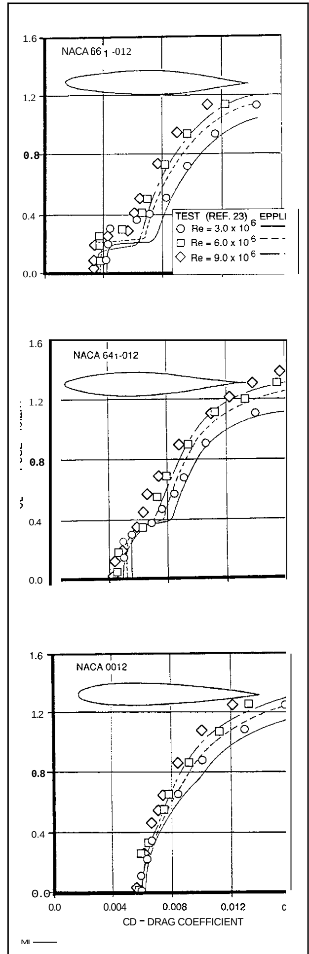
Fig. 14 2-D Airfoil Drag Correlation Laminar Flow Extent Effects
