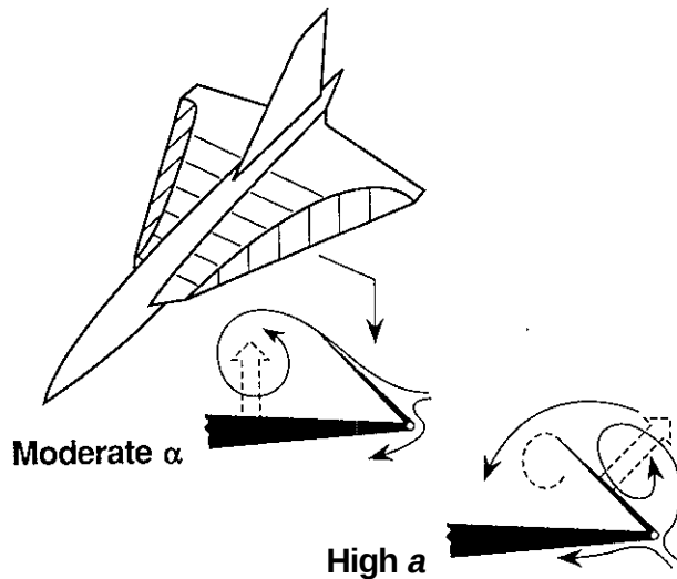
Fig. 74. Upper vortex flap concept.
