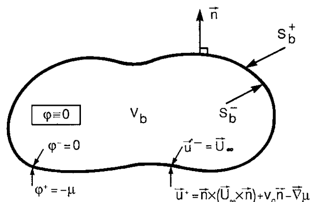
Fig. 3.3 Dirichlet condition on the perturbation potential
