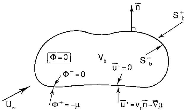
Fig. 3.5 Dirichlet condition on \Phi
