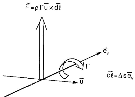
Fig. 4.6 Force on a vortex segment
