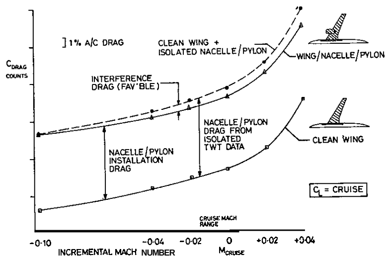
FIG 41 EXAMPLE OF FAVOURABLE INTERFERENCE (FROM REF.9)
