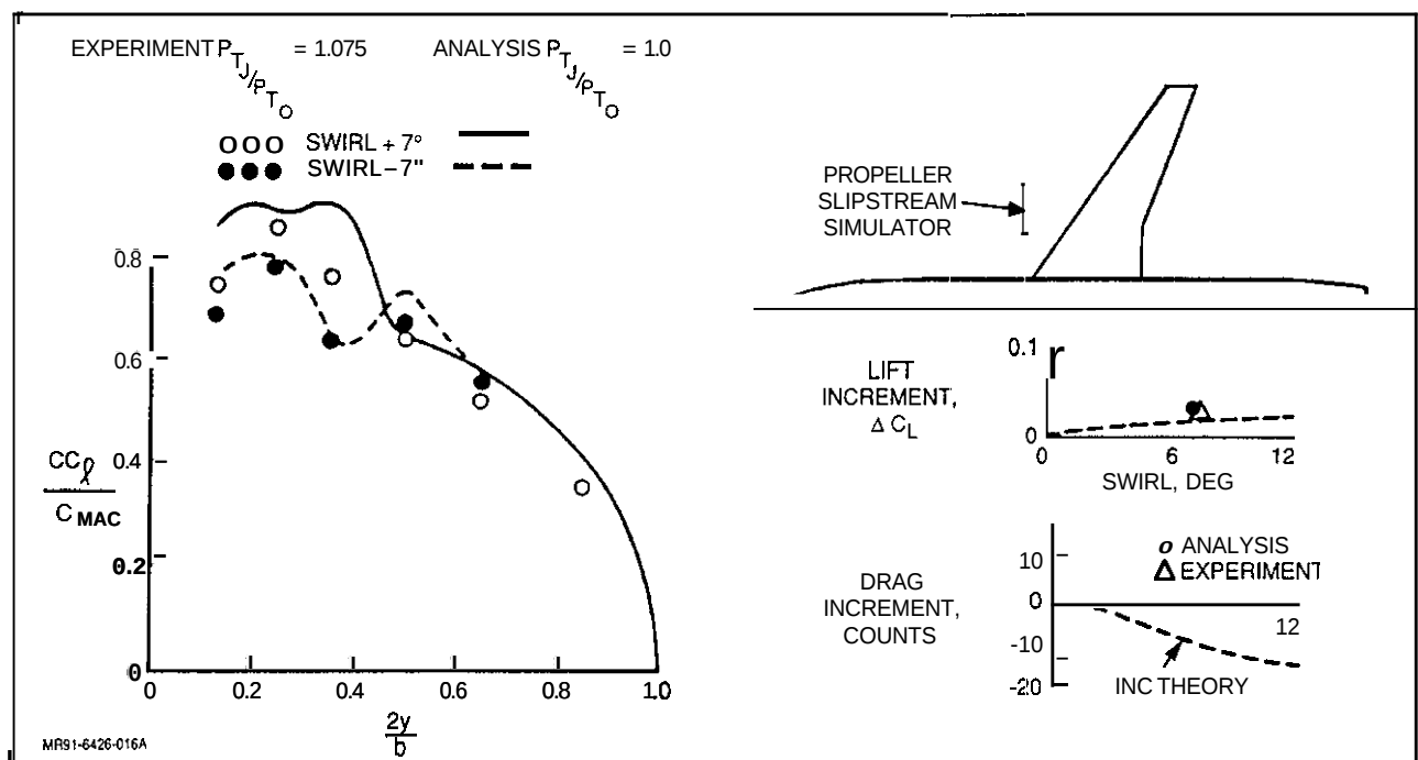
Fig. 39 Propfan Interference Effects—Wing Spanload, Lift, & Drag Increments ( M = 0.8 \alpha = 3 Deg)
