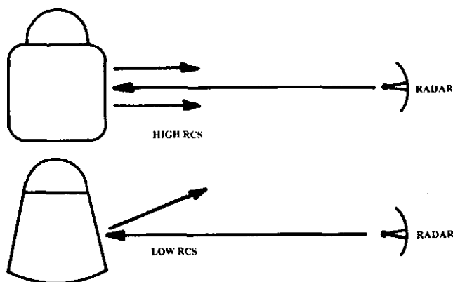
Fig. 39 Flat side RCS reduction.
