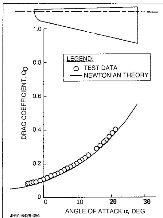
Fig. 86 Hypersonic Body Drag Polar Correlation with Newton Theory
