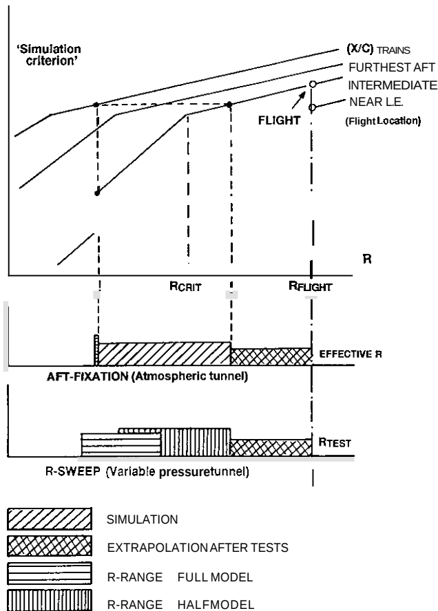
FIG 35a SIMULATION SCENARIO 3
