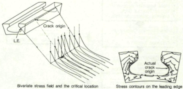
Bivariate stress field and the critical location
