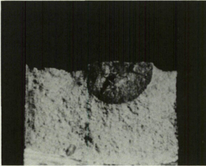
Fig 7 - Disc burst from subsurface failure.
