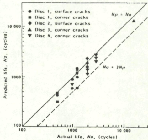
Bore crack propagation results for artificially cracked Ti 6-4 discs
