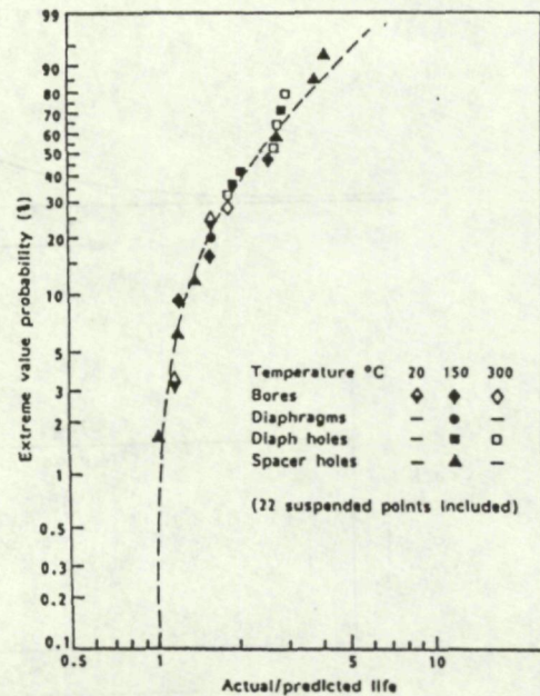
Ti6Al4V Comparison of predicted and actual lives
