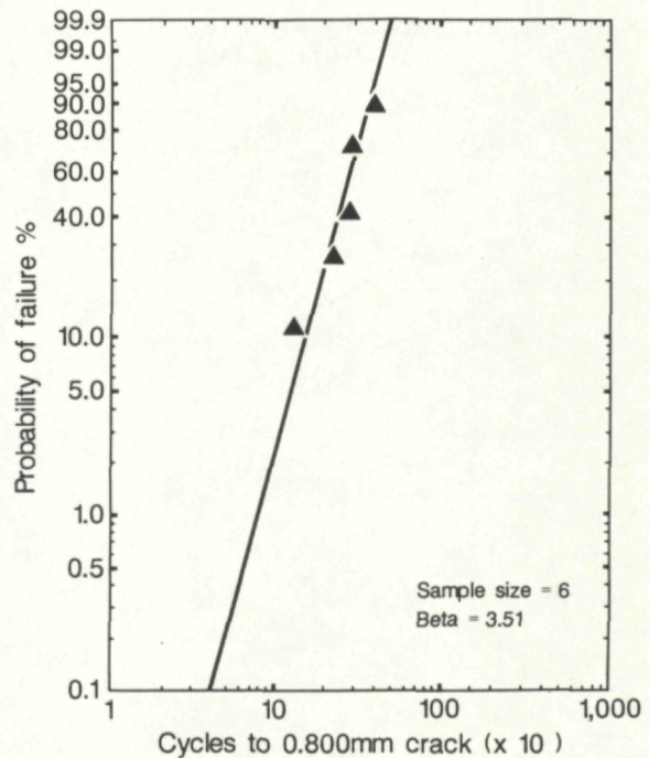
Fig. 7 WEIBULL STATISTICAL ANALYSIS OF THE FAN HUB L.C.F. DATA
