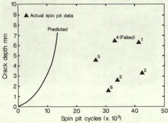
Fig.10 PREDICTED CRACK GROWTH BASED ON A 0.250MM INITIAL FLAW
