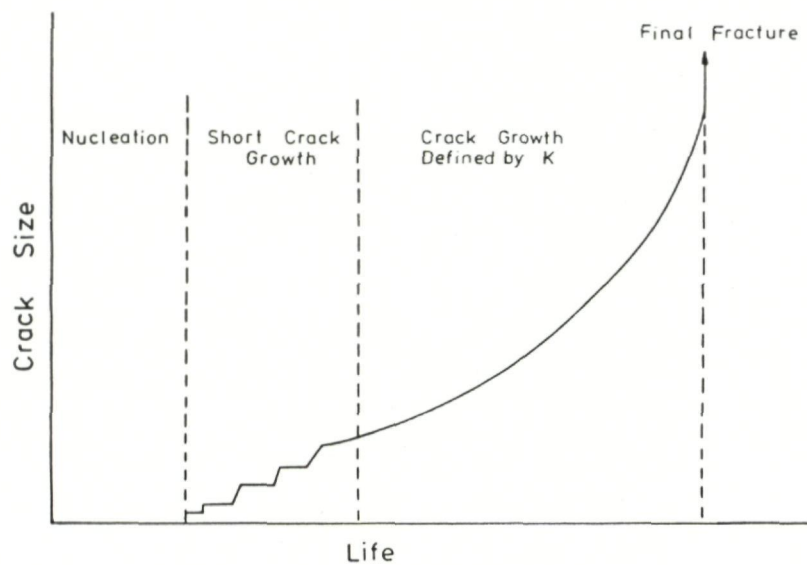
Fig 2 - Stages of Cyclic Life.
