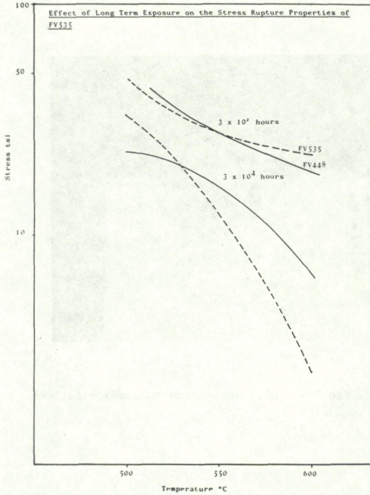
Fig 5 - Creep curve of FV535 showing deterioration with time of exposure compared to FV448
