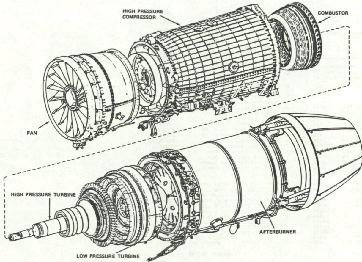
ENGINE MODULES
