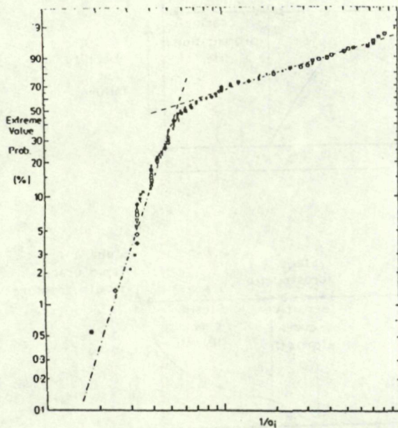
Ti 6Al 4V Full Effective Initial Crack Size Distribution
