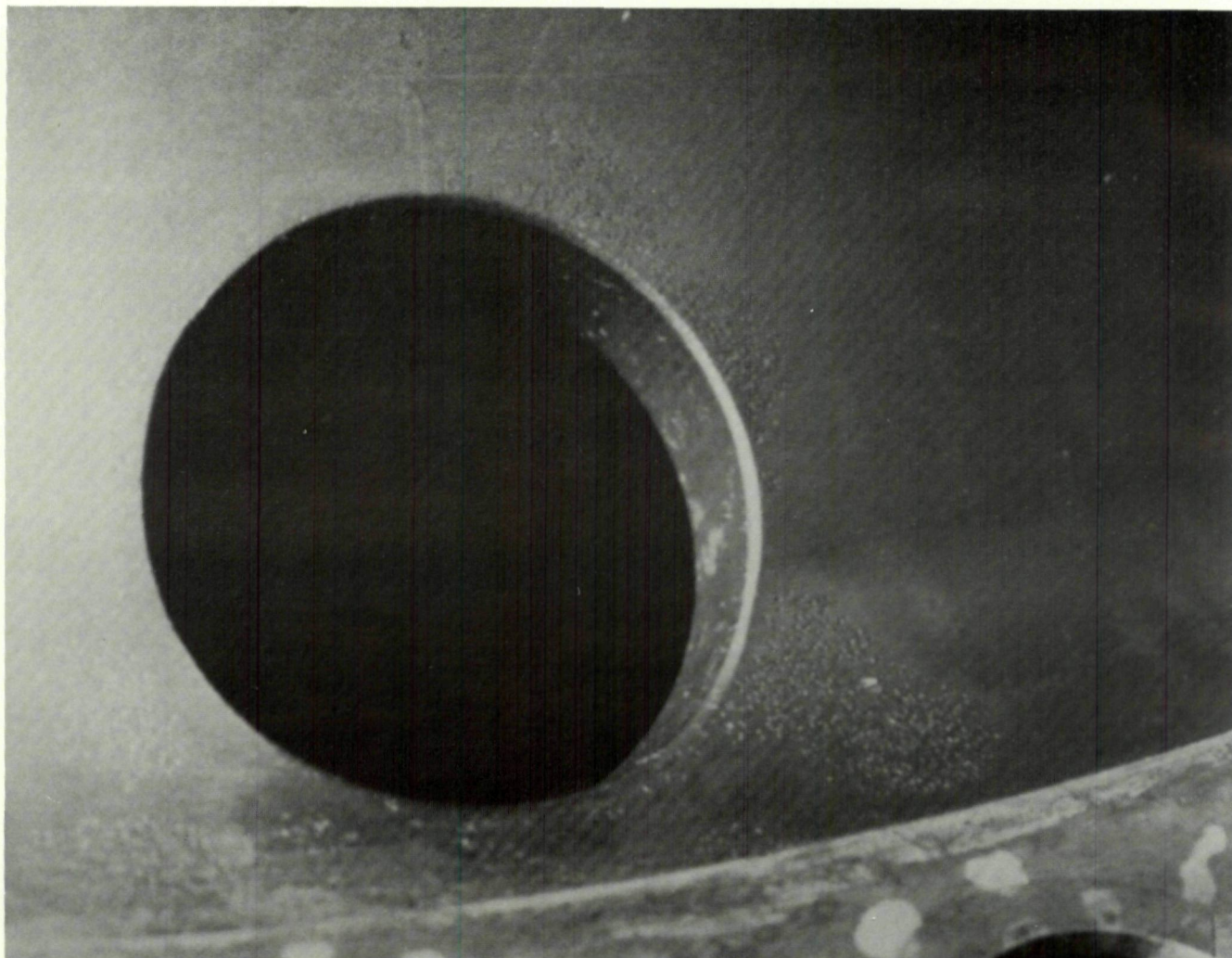
Fig 4 - Corrosion pits on shaft.
