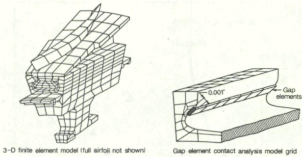
3-D finite element model (full airfoil not shown)
