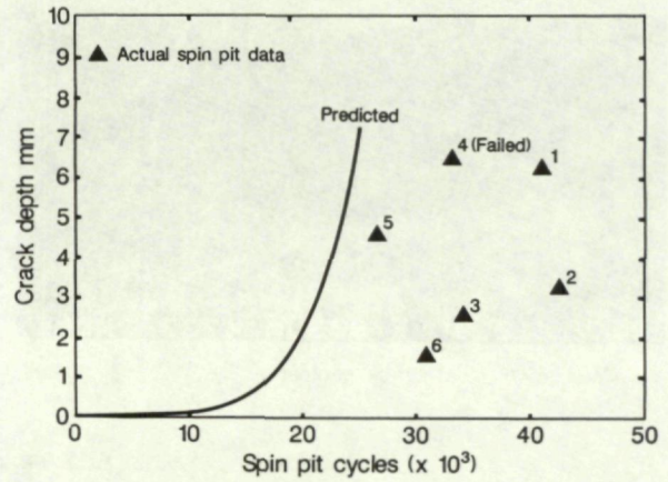
Fig.11 PREDICTED CRACK GROWTH BASED ON A 0.025MM 'PSEUDO' INITIAL FLAW
