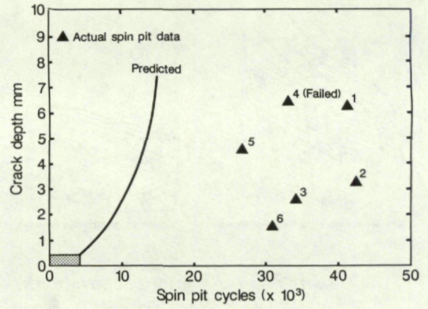
Fig.9 PREDICTED CRACK GROWTH BASED ON A 0.800MM INITIAL FLAW
