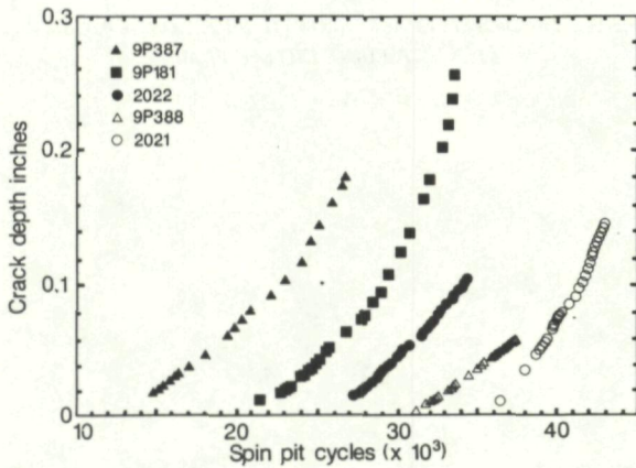
Fig. 6 STRIATION COUNT DATA OF FIVE NEW DISCS, WHICH DEVELOPED CRACKS IN THE SPIN PIT TEST
