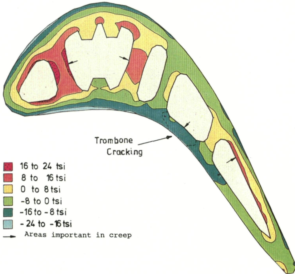
Fig 1 - FE model of blade showing area where creep is important.
