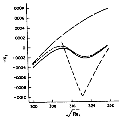
Figure 1. Spatial growth rate -k_i versus R ( =/Re_x ). Single strip with Vo/U_o = 2.3 \times 10^{-4} , F = 21 \times 10^{-6} . From Reed and Nayfeh (1981).
