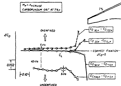
Fig. 17: Effect of Roughness Height on Drag for a Transport Configuration, Ref. 21
