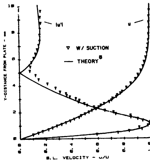
Figure 3. Profiles of Mean Velocity U(y)/U_o and Disturbance Velocity |u'(y)|/|u'|_{max} at R = 1380 , Vo/U_o = 3.7 \times 10^{-3} at R = 1340 , F = 20 \times 10^{-6} . Data from Reynolds and Seric (1982). Theory from Reed and Nayfeh (1981).
