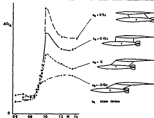
Fig 37 BELOW 60 THICK 55° L.E. BLUNT WING (FROM TESTS AT A.R.A.)
