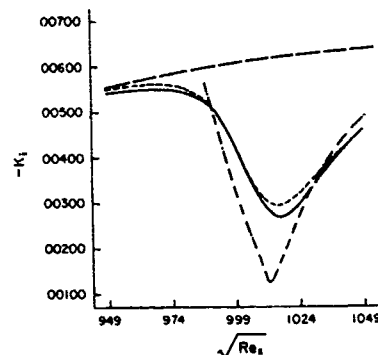
Figure 2. Spatial growth rate -k_i versus R ( =/Re_x ). Single strip with Vo/U_o = 2.3 \times 10^{-4} , F = 40 \times 10^{-6} . From Reed and Nayfeh (1981).
