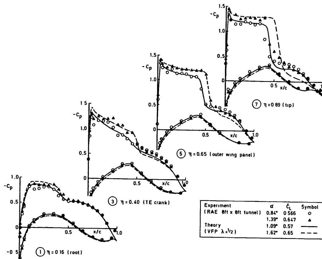
Fig 32 Wing-body (1): Half-model pressures, M_\infty = 0.78 , Re_c = 12 \times 10^6
