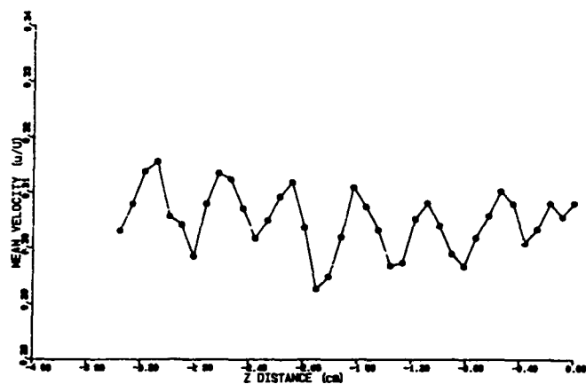
Figure 6. Tangential Velocity, U_x/U_\infty , and Crossflow Velocity, U_y/U_\infty , at x = 170\text{cm} and U_\infty = 10\text{m/s} .
