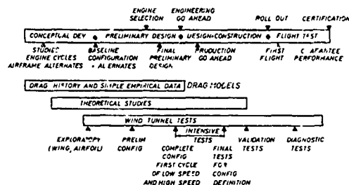
Fig. 13: Airplane Development Schedule, Ref. 12
