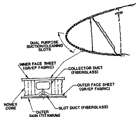
Figure 48. Slotted leading-edge box design
