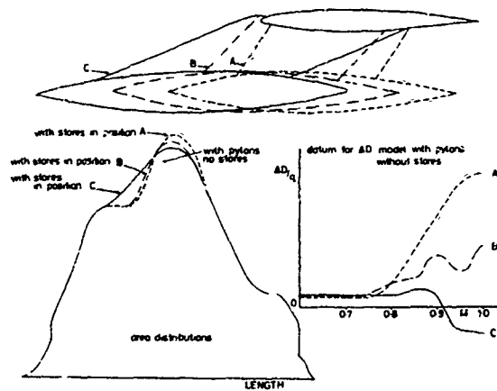
Fig 36 CORRELATION OF DRAG NEAR M = 1.0 AND CROSS-SECTIONAL AREA DISTRIBUTIONS (FROM AERITALIA TESTS)
