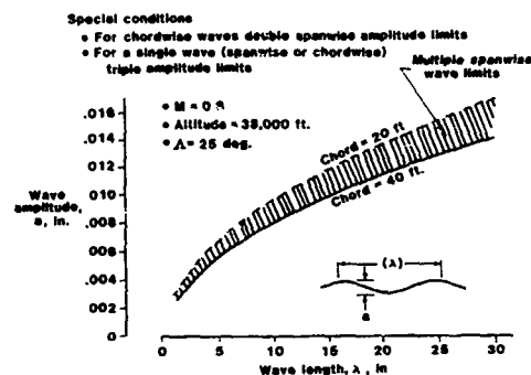
Figure 4. Typical permissible surface waviness
