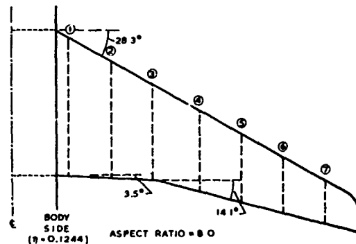
Fig 31 Wing-body (1)
