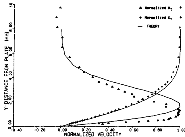
Figure 6. Tangential Velocity, U_x/U_\infty , and Crossflow Velocity, U_y/U_\infty , at x = 170\text{cm} and U_\infty = 10\text{m/s} .
