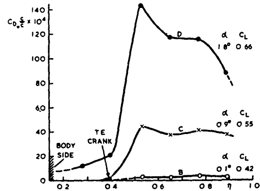
Fig 37 Wing-body (1): Local contributions to wave drag: C_{D/C}
