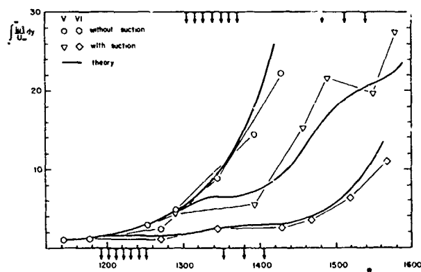
Figure 6. Disturbance Amplitude versus Reynolds Number for two cases. Case VI: 7 strips on panel #1 @ V_o/U_o = .00042 , 3 strips on panel #2 @ V_o/U_o = .0011 . Case V: 7 strips on panel #1 @ V_o/U_o = .0005 , 3 strips on panel #2 @ V_o/U_o = .0013 . Mass flow is the same in V and VI. Suction locations shown by arrows for each case. Data from Reynolds and Saric (1982). Theory from Reed and Nayfeh (1981).
