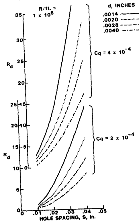
Figure 51. Variation of perforation diameter Reynolds number with perforation spacing
