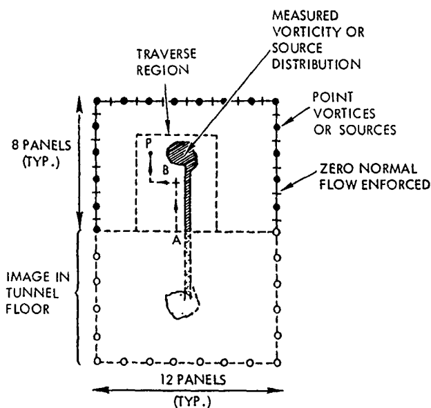
Figure 5. Establishment of the Tunnel-Wall Boundary Condition
