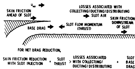
Fig. 8. - Force balance associated with slot injection.
