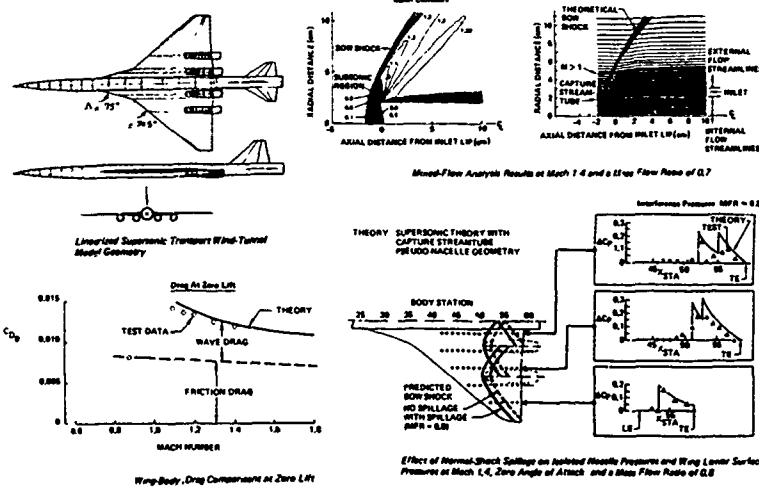
Fig 34b AIRFRAME/NACELLES AERO INTERFERENCE PREDICTIONS on a 55T AIRCRAFT PROJECT and COMPARISON with WIND-TUNNEL TESTS at MACH M=1.4 , \alpha=0 .
