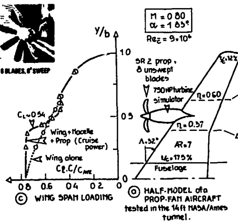
Fig 32 PROP-FAN SLIPSTREAM EFFECT on a SWEEP-WING at CRUISE M = 0.8 .
