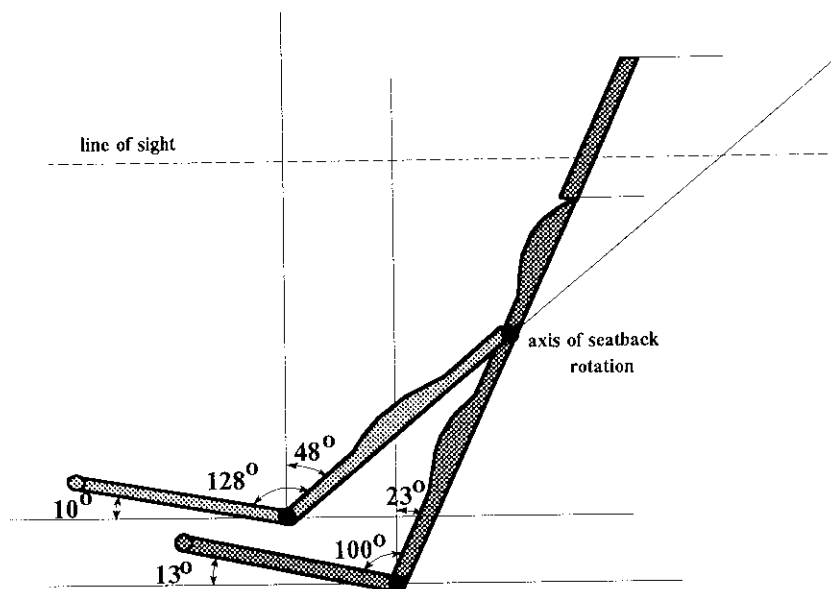
Fig. 5. Scheme of supination of variable geometry seat
