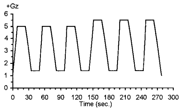
Fig. 4: maximum level interval training profile TP ID: first 3 plateaus 5.0 \text{ g}_z , second 3 plateaus 5.5 \text{ g}_z , onset: 0.5 \text{ gs}^{-1} , 0.7 \text{ gs}^{-1} , 1.0 \text{ gs}^{-1} , offset 0.3 \text{ gs}^{-1} , plateau duration 15 seconds
