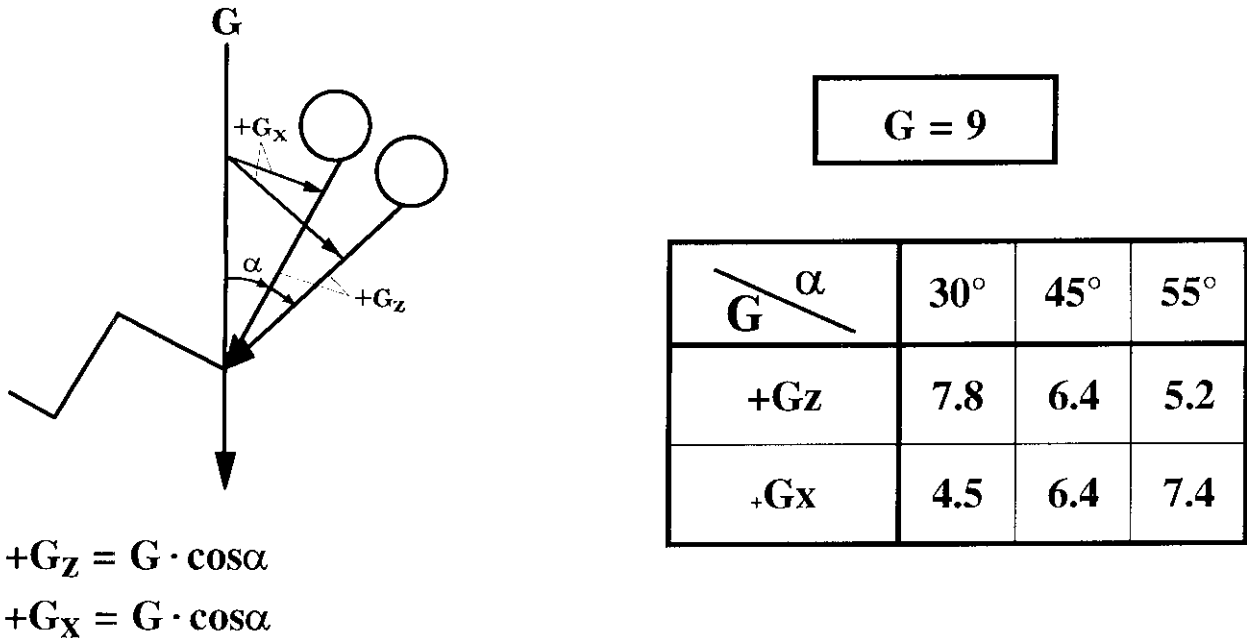
Fig. 1. Anti-G protective efficiency of seatback supination angles
