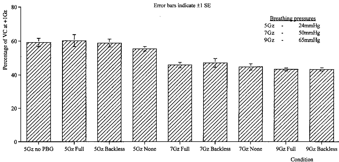
Figure 5. The effect of different degrees of chest counter pressure garment coverage upon lung distension, as expressed as a percentage of the subject's vital capacity at 1Gz, at 5, 7 and 9Gz. There is no significant difference between the conditions of no PBG, full chest coverage, coverage of the front of the chest only and no chest counter pressure. From Green (1994).
