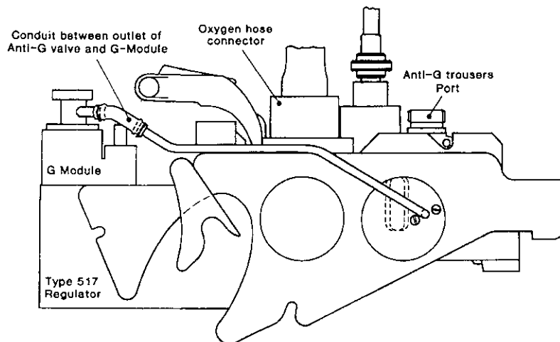
Figure 15. An implementation of the schematic diagram shown in figure 14. This arrangement is currently fitted to the RAF School of Aviation Medicine Hawk aircraft.
