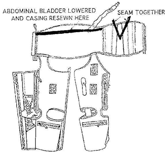
Figure 2. Armstrong Laboratory (AL) anti-G suit modification allows for lowering the abdominal bladder for comfort, and placement of a dart in the lumbar restraint for a better female fit.
