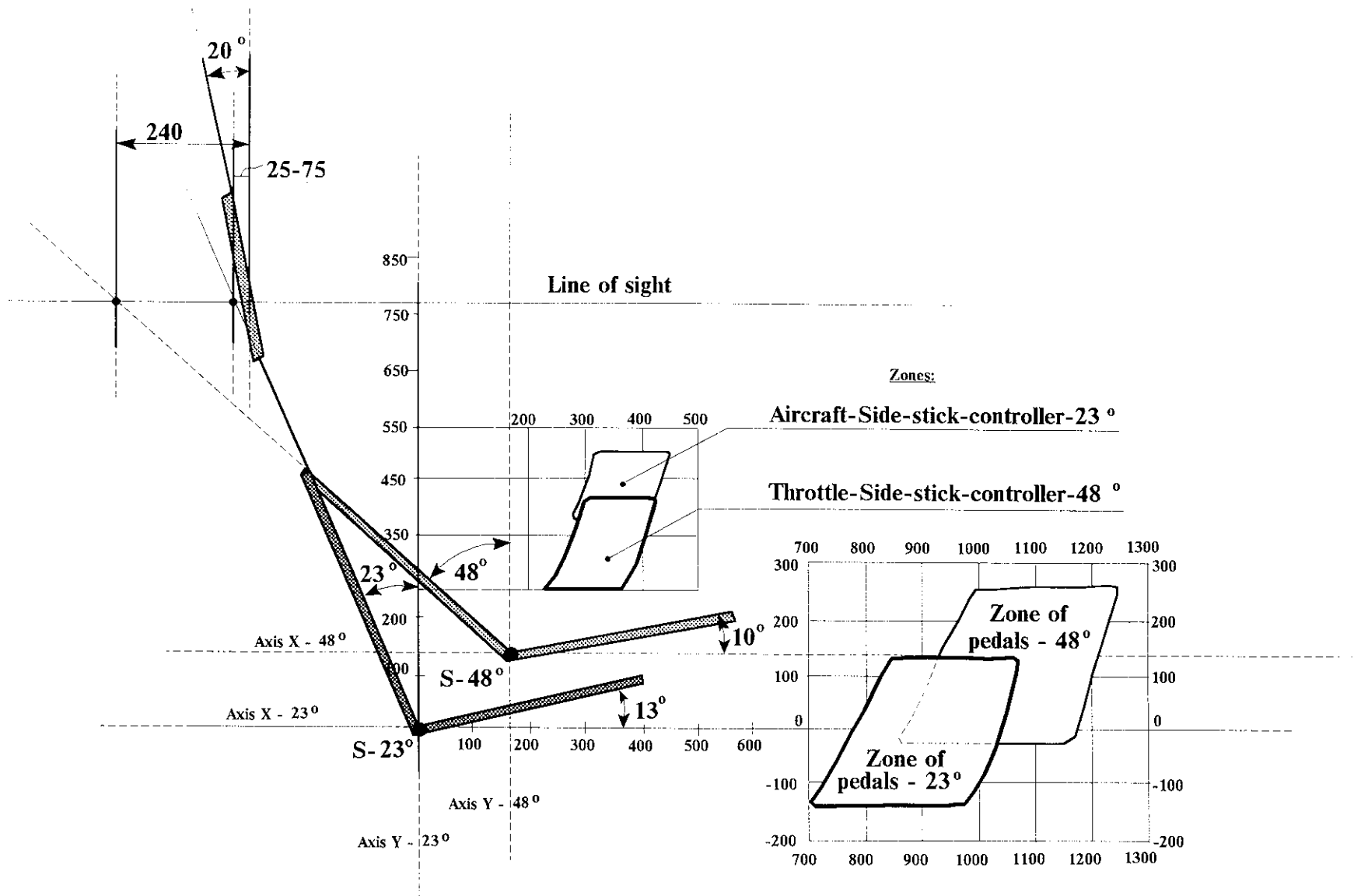
Fig. 12. Arrangement scheme of control organs at installation of changeable geometry seat in aircraft cabin.
