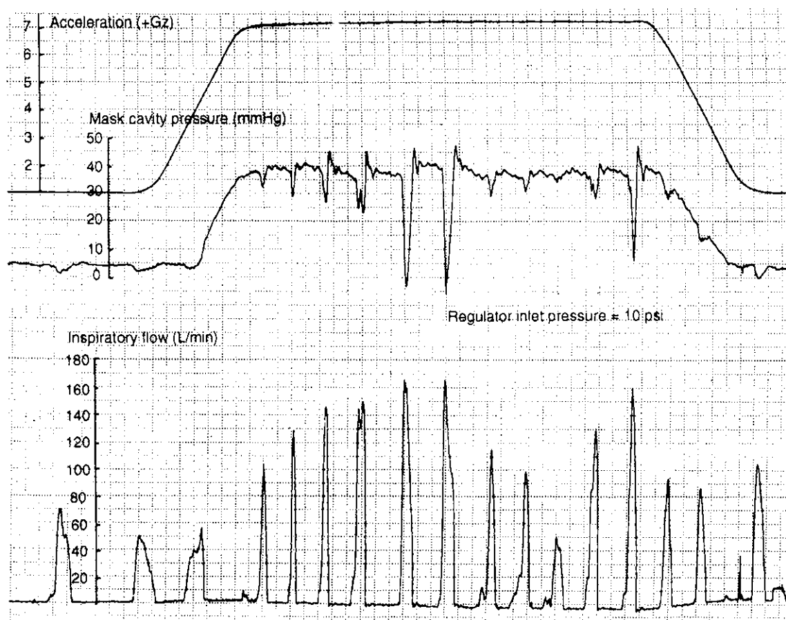
Figure 17. Original trace showing that a demanded inspiratory flow in excess of the capabilities of the regulator causes a fall in PBG mask cavity pressure.
