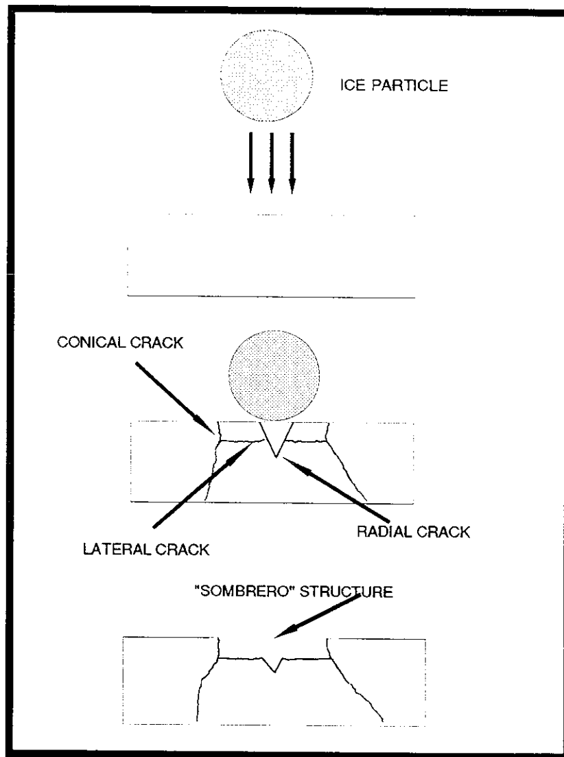
Figure 2 -- Crack Formation and Erosion by Fracture.
