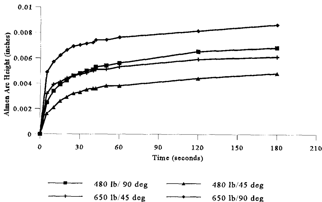
Figure 2 Comparison of Almen arc data for Type V media at two blast angles and media flow rates using a 12" standoff distance (AL 2024-T3).
