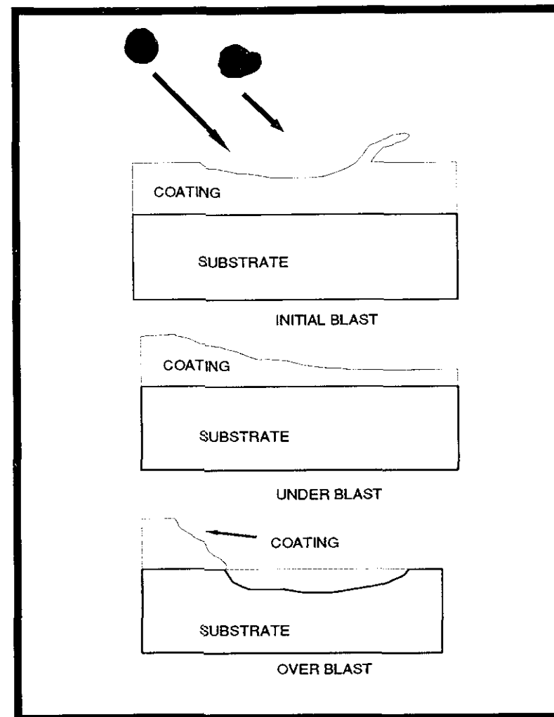
Figure 1 -- Coating Removal By Abrasion.
