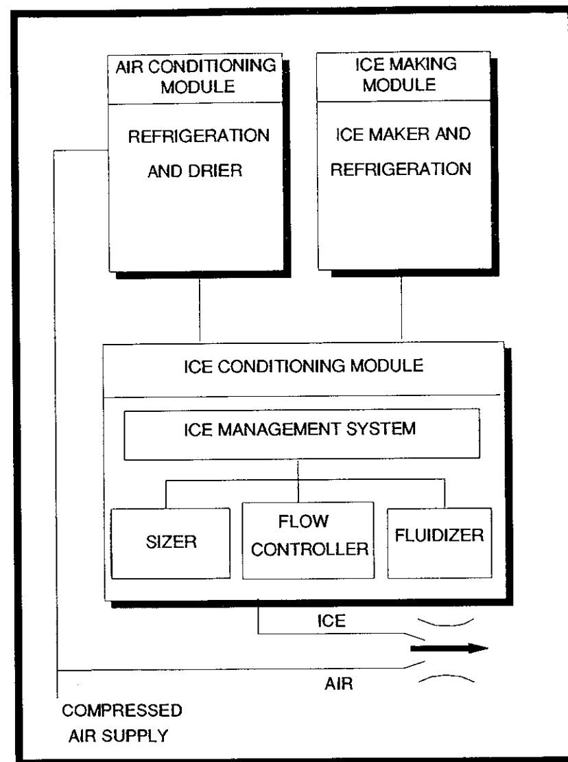
Figure 5 -- Schematic of Ice Blasting Equipment.
