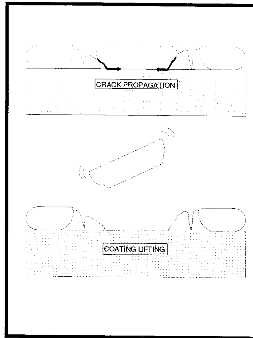
Figure 3 -- Crack Propagation and Coating Lifting.
