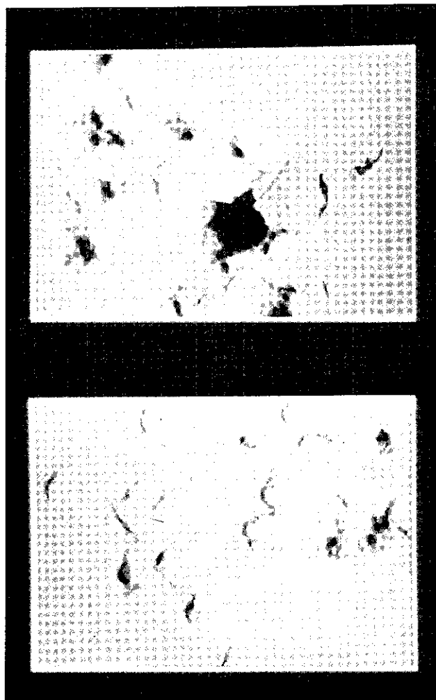
Figure 4 -- Surface Cracks Due to Ice Particle Impact.
