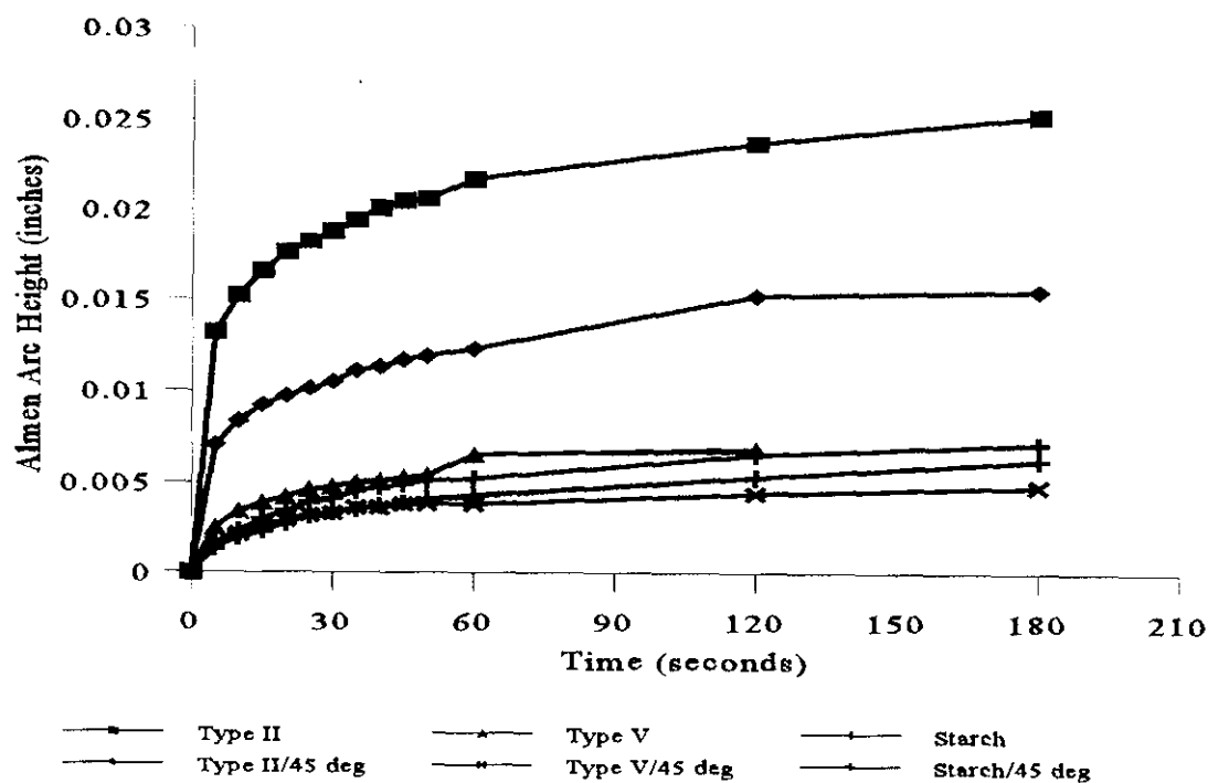
Figure 3 Comparison of the Almen arc data for Type II, Type V and Wheat Starch media at 45° and 90° at a media flow rate of 480 lb/hr and 12" standoff distance (Al 2024-T3).
