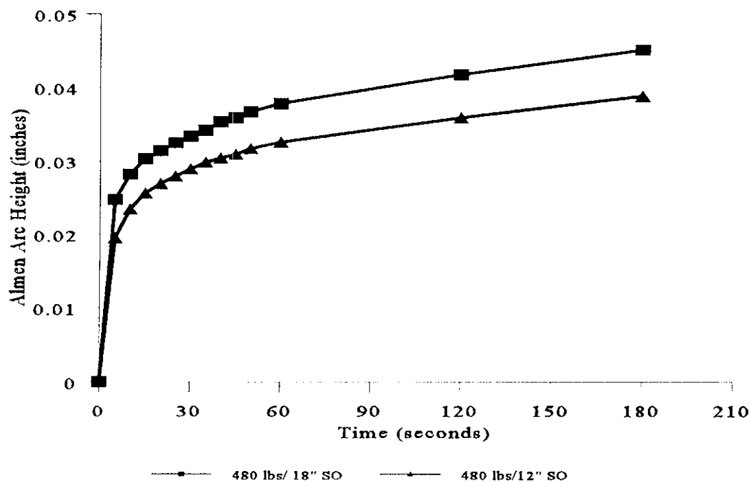
Figure 4 Comparison of the effects of standoff distance on the Almen arc data for Type V on magnesium alloy at 90 deg and 30 psi.
