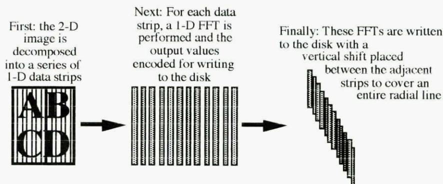
Figure 5: Image encoding in UCSD's parallel readout optical disk system.
