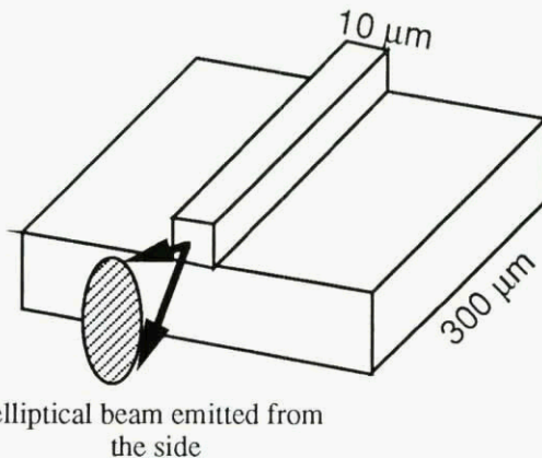
Figure 1. "Horizontal" cavity laser.
