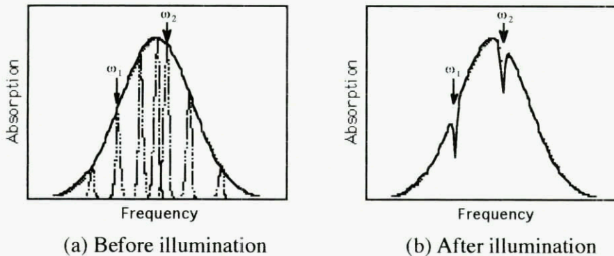
(a) Before illumination (b) After illumination Figure 10: The effect of spectral hole burning on the absorption profile. The frequencies of the illuminating sources at \omega_1 and \omega_2 are indicated with arrows. (a) The smooth absorption profile for an unwritten molecule. (b) The modified absorption profile after illumination.
