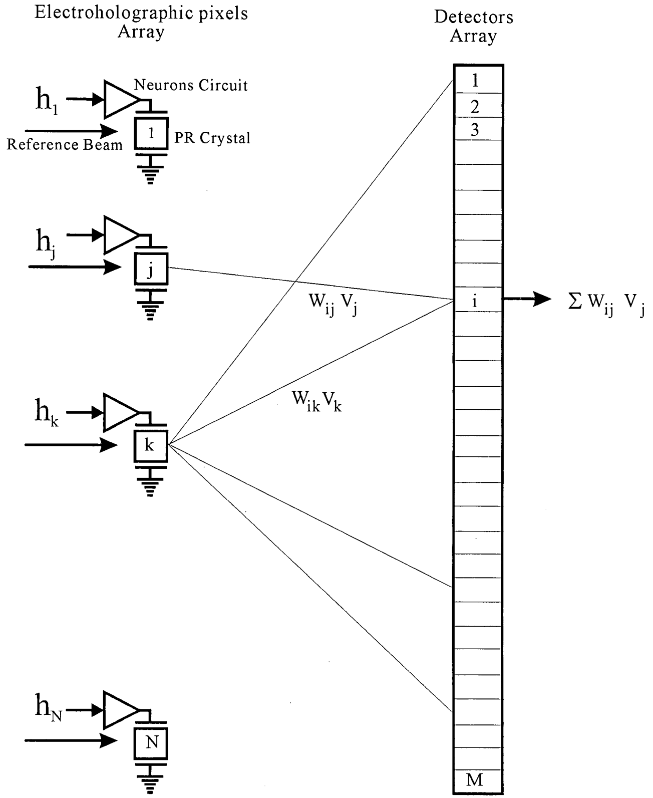
Figure 7: Basic architecture of electroholographic neural network.
