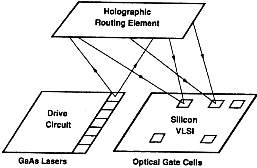
Fig.1 Typical optical interconnection geometry
