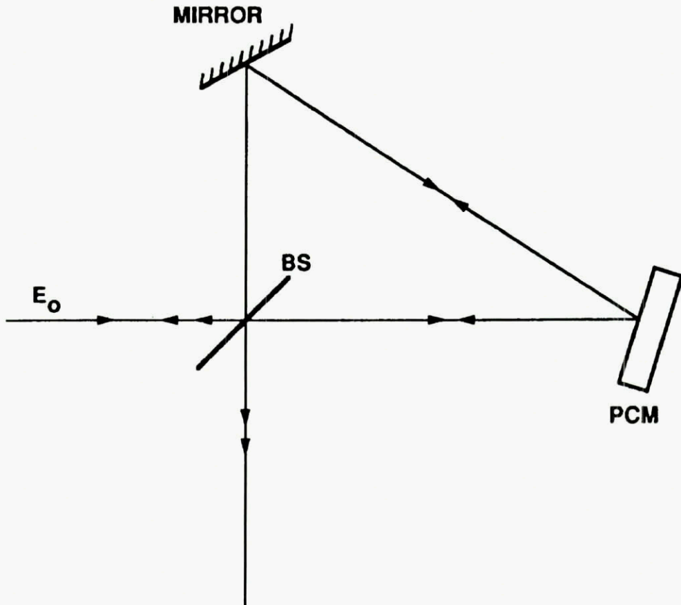
Fig.10 Phase-conjugate Michelson interferometer
