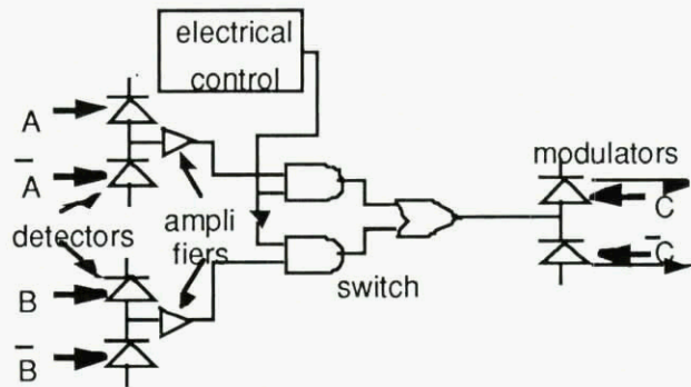
Figure 3. One FET-SEED based optoelectronic circuit that can be integrated ; the circuit contains three pairs of SEEDs arranged into pairs, two of which are used as optical data inputs and one as optical data output.
