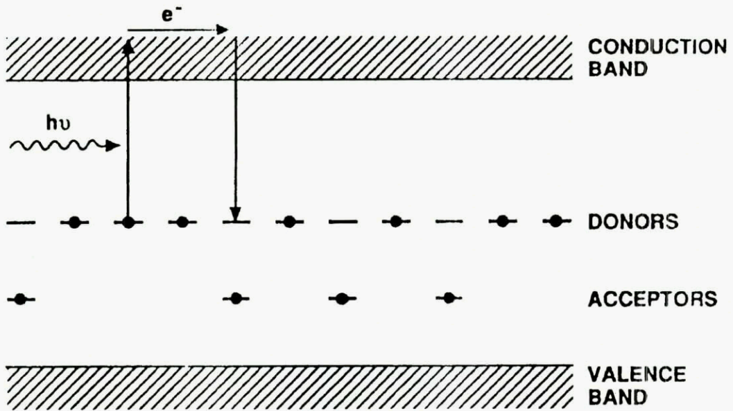
Fig.6 Charge migration and trapping in photorefractive crystals
