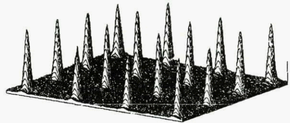
Figure 4 Illumination distribution generated by a 16 points array illuminating grating.
