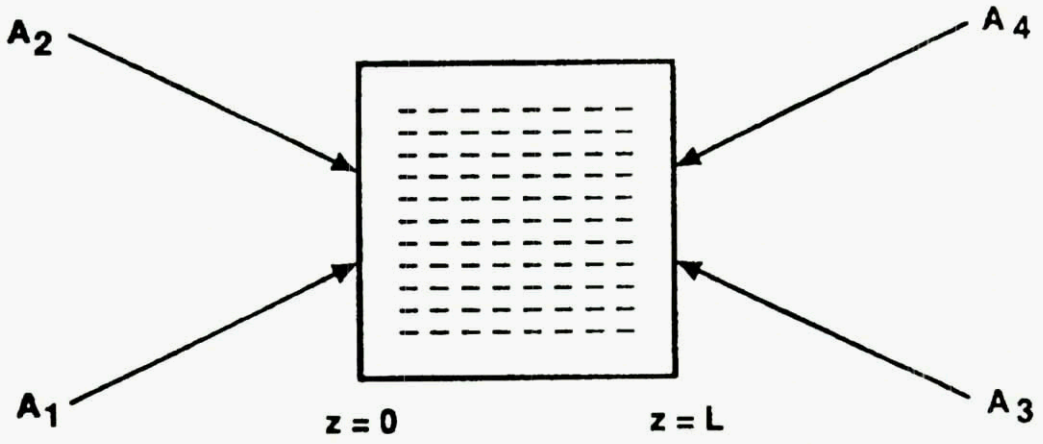
Fig.8 Four-wave mixing geometry
