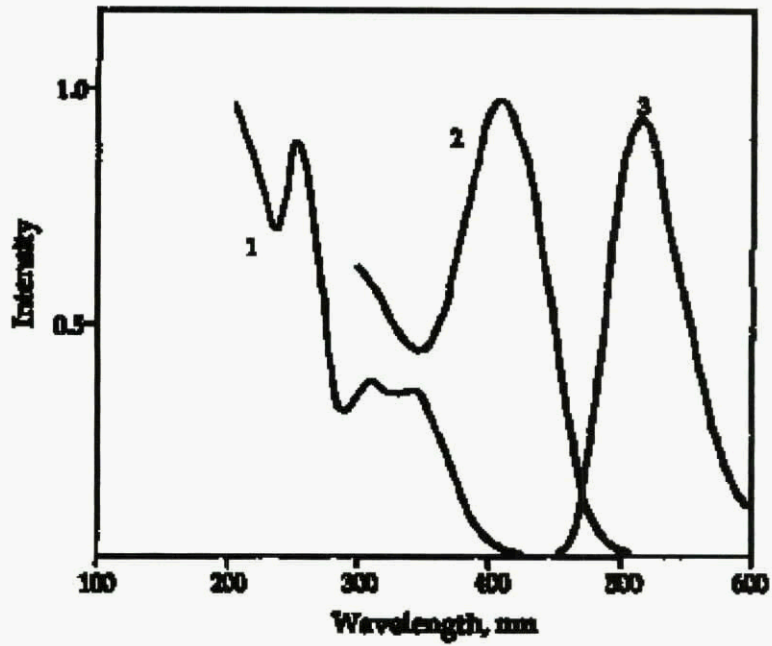
Figure 16: Spectral response for the bridged SP1 material, showing the absorption of the unwritten (I) and written (II) forms of SP1, as well as the fluorescence spectrum of the written form (III).
