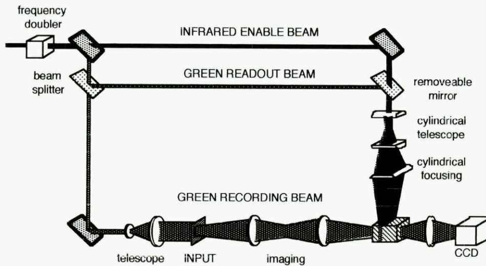
Figure 19: Experimental image recording set up.
