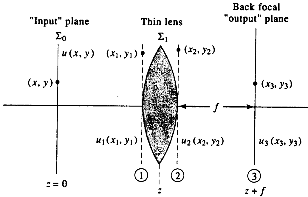
Fig.3 Fourier-transform scheme using a thin lens
