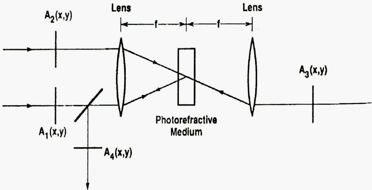
Fig.9 Convolution and correlation via four-wave mixing
