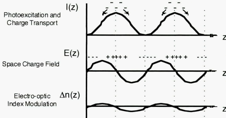
Figure 8: The photorefractive effect.
