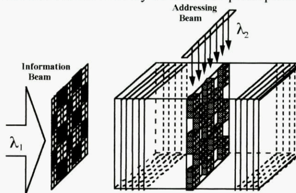
Figure 17: Image storage in two photon 3-D memory materials using orthogonal beam addressing.
