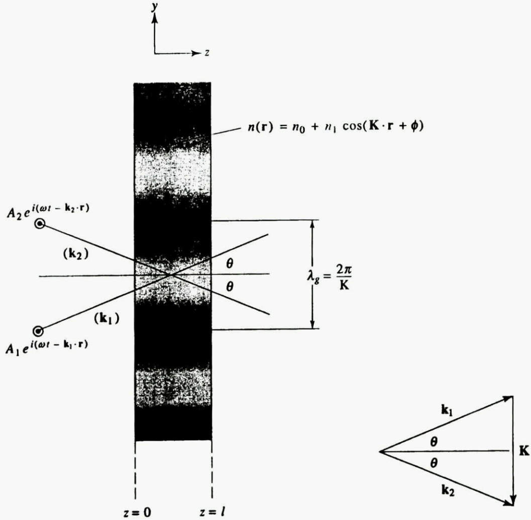
Fig.5 Two-beam coupling
