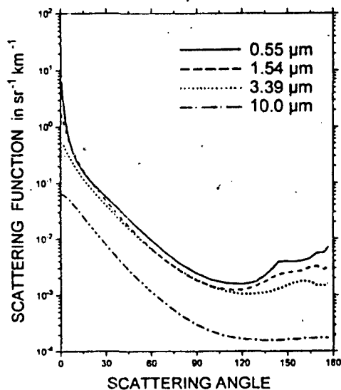
Fig. 2.7: Angular scattering function for the Shettle & Fienn (1979) maritime aerosol model with a relative humidity of 80% and a number density of 4.0 \text{ cm}^{-3} for several wavelengths.
