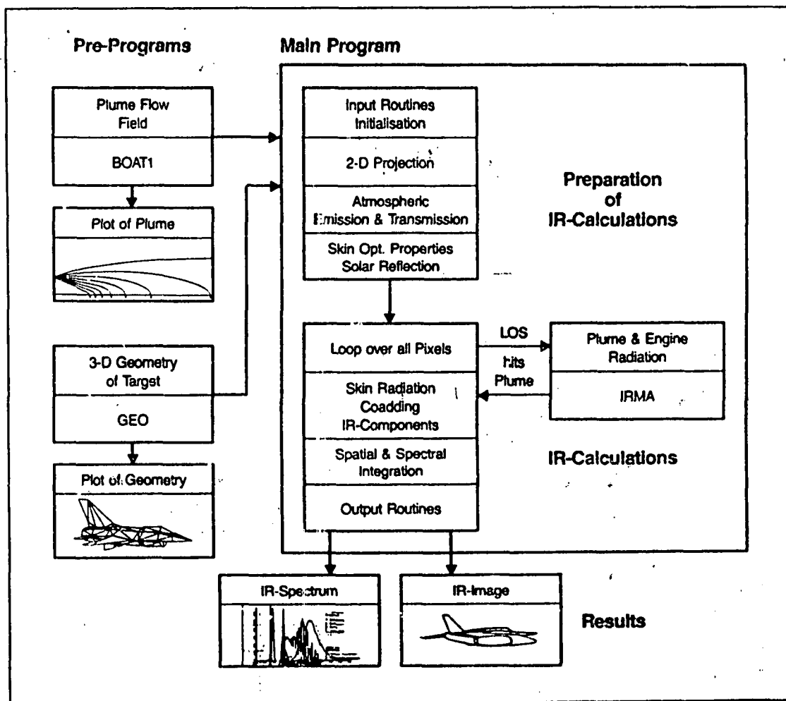
Fig. 6.3: Simplified flow diagram of NIRATAM.
