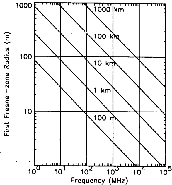
Figure 2. The radius of the first Fresnel zone at the midpoint of a path of given length.
