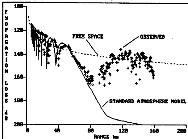
Figure 15. Propagation loss versus range in a surface-based duct for 3.0 GHz. Transmitter and receiver heights were 21 and 152 m above mean sea level.
