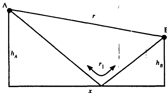
Figure 3. Antennas at A and B, separated by horizontal distance x , on towers of heights h_A and h_B on a plane earth.
