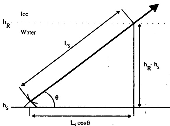
Figure 15: Earth-space satellite path geometry
