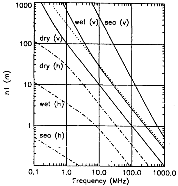
Figure 5. The 'minimum effective antenna height' h_1 for very dry and for wet earth, and for the sea, for vertical (v) and horizontal (h) polarization, using CCIR electrical constants for these types of ground. The dotted line indicates the wavelength at each frequency.
