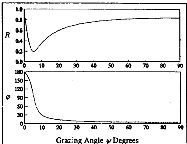
Figure 5. Reflection coefficient magnitude R and phase lag \phi for vertical polarization at 1.0 GHz over sea water versus grazing angle \psi . Both \phi and \psi are in degrees.
