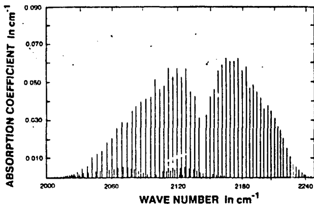
Fig.3.5: Carbon-monoxide absorption spectrum for P_{CO} = 3 Torr and T = 295 K [1].
