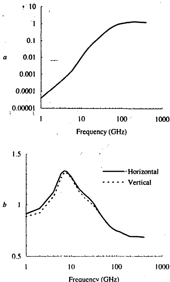
Figure 11: Coefficients required for estimating the specific attenuation due to rain
