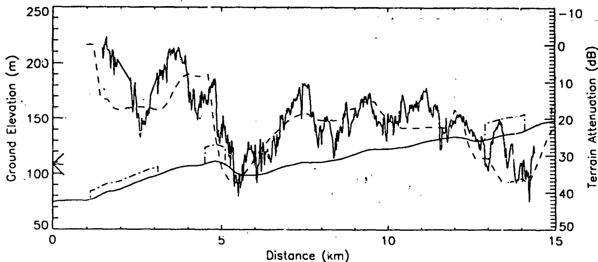
Figure 8. A terrain profile near Ottawa, and attenuation with respect to free space at vehicle height, for 910 MHz. The transmitting antenna is indicated at 110 m. On the terrain profile, suburban buildings are indicated at 2 km, and stands of trees at 5 and 13 km. The solid line is measured (20-m median) loss, and the broken line is predicted loss.
