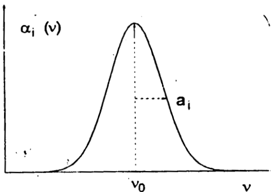
Fig.3.4: Spectral absorption coefficient of an absorption line.
