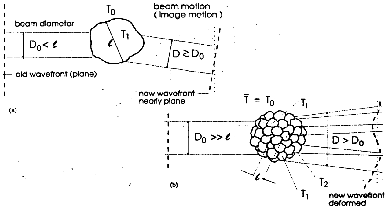
Fig. 3.15: Laser beam deflection by turbulence cells that are larger than the beam diameter (a) and laser beam break up by turbulence cells that are smaller than the beam diameter (b).
