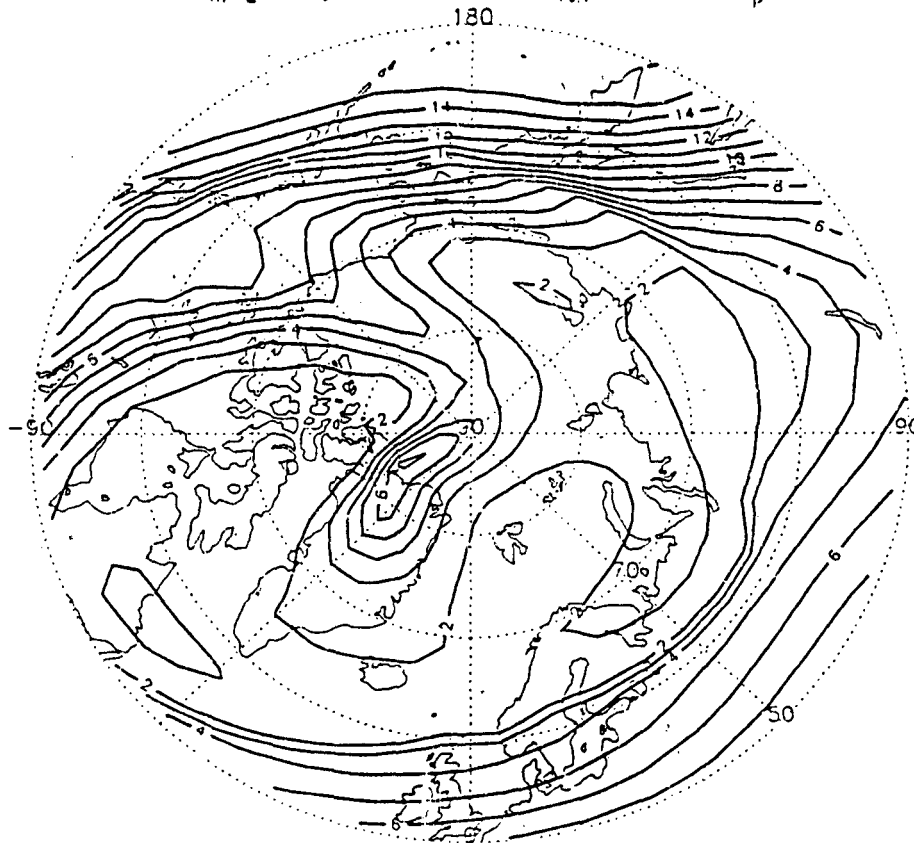
Figure 4. Contours of the maximum ionisation density in the F_2 region (in units of 10^5 \text{ cm}^{-3} ) in polar projection from PIM for high solar activity, moderate magnetic activity, at 00UT and at the December solstice. The "tongue of ionisation" produced by a steady convection pattern is clearly evident. Local midnight is at the bottom, from Daniell et al. [1994].
