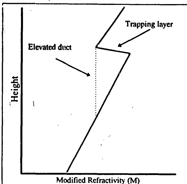
Figure 18. Modified refractivity versus height profile for an elevated duct.
