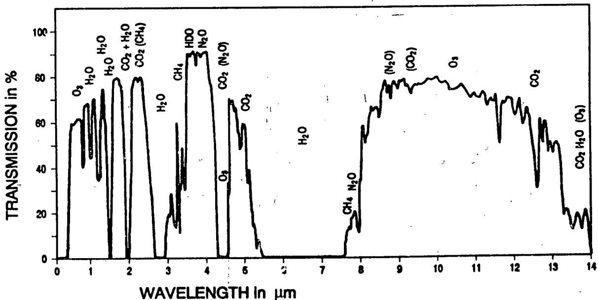
Fig. 2.1: Atmospheric transmission for a horizontal path length of 2 \text{ km} , absolute humidity 8.5 \text{ gm}^{-3} , visibility 15 \text{ km} , and rural aerosol.
