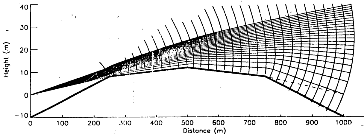
Figure 1. Wave front and wave normals for a 50-MHz wave diffracting over a hill constructed of perfectly reflecting planes.
