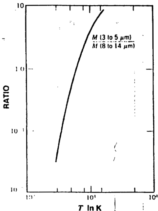
Fig. 2.7: Blackbody spectral band energy ratios [3].
