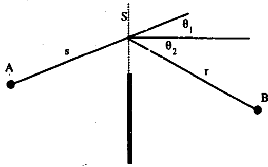
Figure 15. A knife edge (heavy black line) and the surface S above it over which E is integrated.
