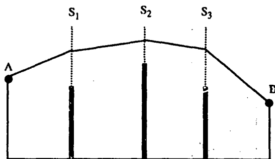
Figure 16. Three knife edges ( N = 3 ) between antennas A and B. The field is integrated over the vertical surfaces indicated by dotted lines using eqn. (25). The thin segmented line connects one of many sets of integration points.
