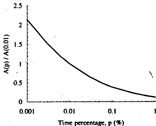
Figure 14: Scaling factor A_p / A_{0.01}
