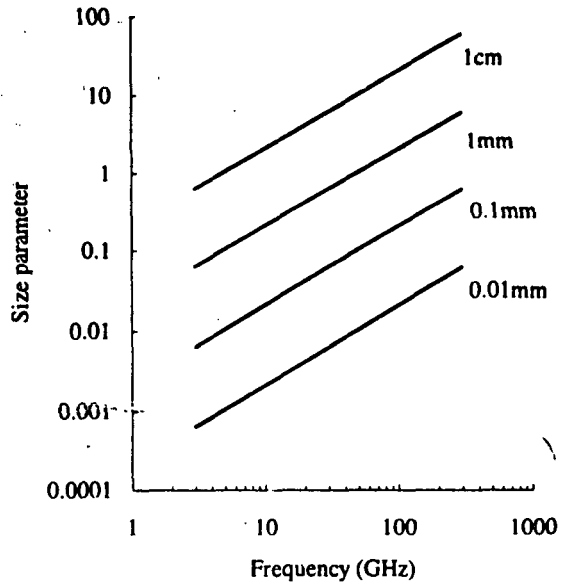
Figure 7: Size parameter as a function of particle radius and frequency
