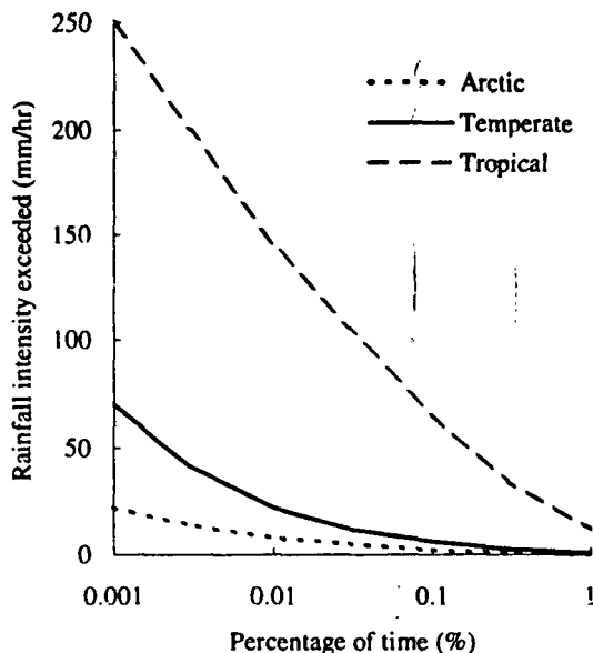
Figure 3: Typical rainfall rate distributions for three climates
