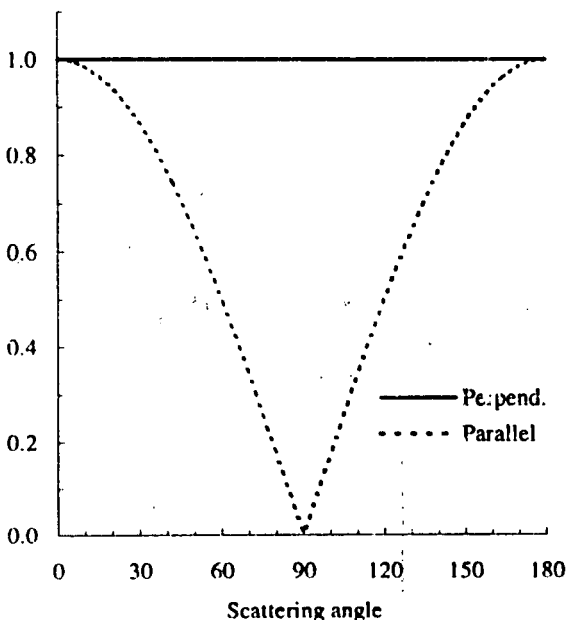
Figure 9: Rayleigh scattering diagram for perpendicular and parallel polarisation
