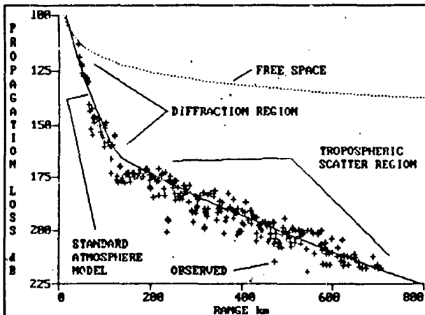
Figure 9. Example of diffraction and tropospheric scatter propagation mechanisms at 220 MHz over sea water. Terminals are 23.5 and 152 m above sea level.
