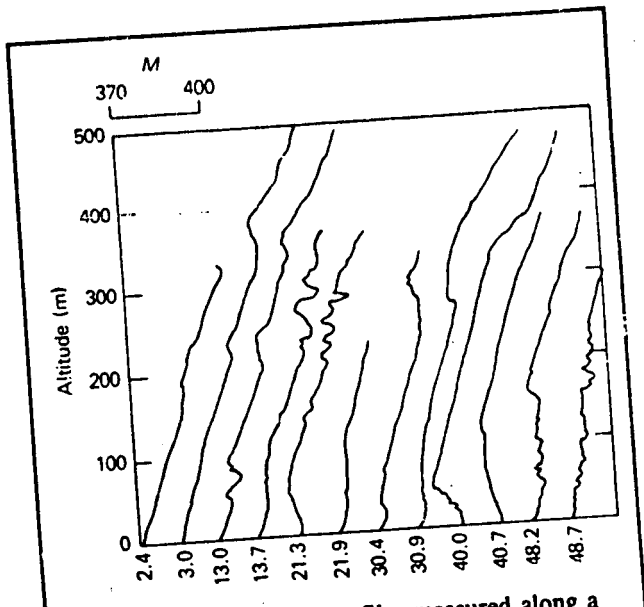
Figure 5. a) Refractivity profiles measured along a propagation path (Dockery and Konstanzer, 1987).
