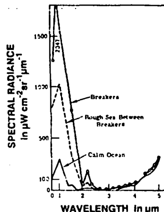
Fig. 2.4: Spectral radiance of the ocean under sunlit [1].
