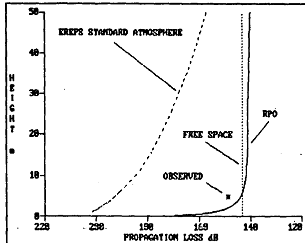
Figure 12. Modeled and observed propagation loss in a 10.4 m evaporation duct at 9.6 GHz. Transmitter height is 4.8 m and the range is 35.2 km.
