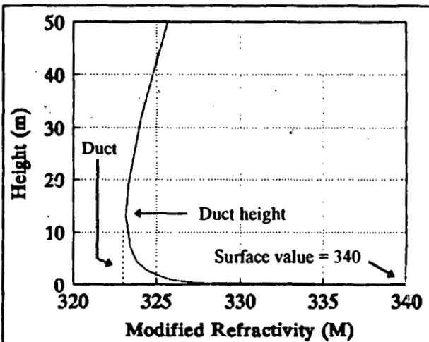
Figure 11. Modified refractivity versus height profile for an evaporation duct. The duct height is 13 m.
