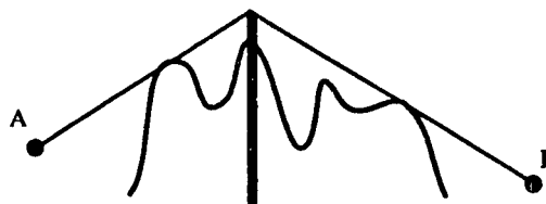
Figure 4. A complex obstacle (the irregular curve) and a Bullington equivalent knife edge (the thick vertical line).
