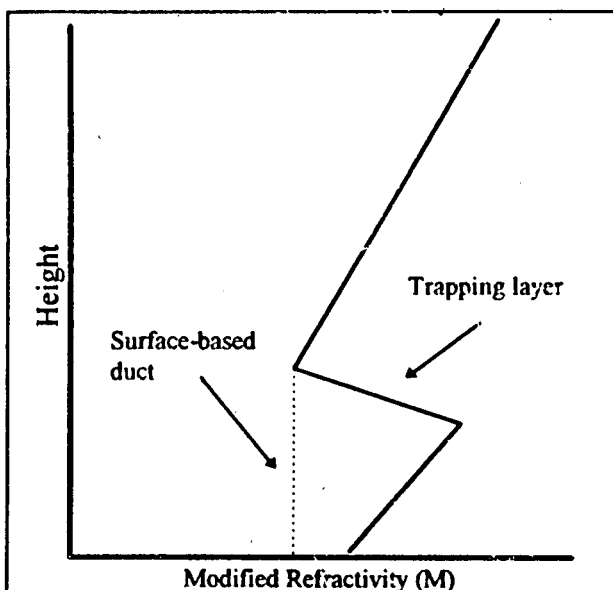
Figure 14. Modified refractivity versus height profile for a surface-based duct.
