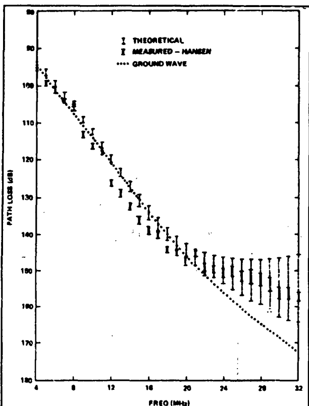
Figure 17. Path loss versus frequency showing effects of tropospheric ducting. From Hansen [24] and Pappert and Goodhart [25].
