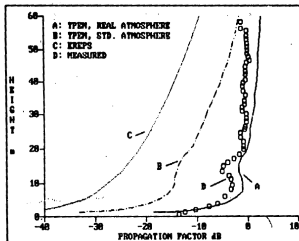
Figure 23. Modeled and measured propagation factor at 1.0 GHz over desert terrain. Transmitter height is 30.5 m and range is 43 km. EREPS assumes smooth earth and standard atmosphere. TPTEM includes terrain for both standard and observed (real) refractivity cases.
