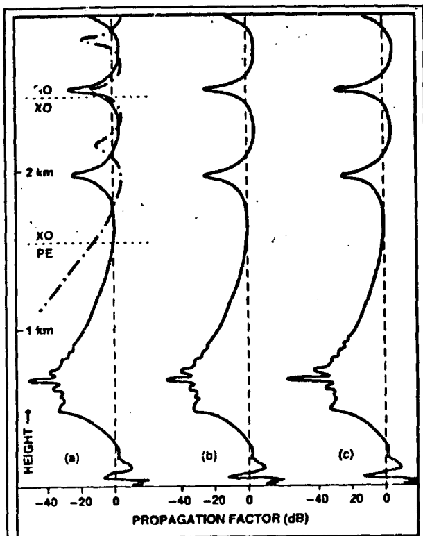
Figure 9. Comparisons of RPO (a), waveguide (b), and pure PE (c) models for a surface based duct at 3.0 GHz. Transmitter height is 30.5 m and range is 185 km.
