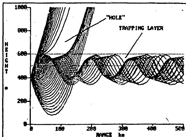
Figure 19. Ray trace diagram showing propagation in an elevated duct.
