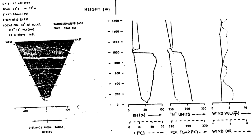
Figure 2. Scanning radar observation of refractivity structure and concurrent radiosonde data.
