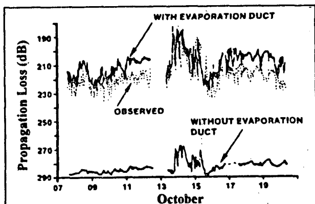
Figure 17. Modeled and observed propagation loss for a two week period at 94 GHz. Terminal heights are 5 and 9.7 m and range is 40.6 km. Absorption included.
