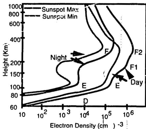
Figure 1. The ionosphere
