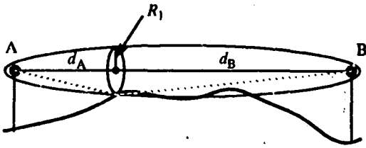
Figure 14. The first Fresnel ellipsoid between antennas A and B. A Fresnel zone has radius R_1 . In this illustration, the terrain penetrates the ellipsoid only a little. The line AB need not be horizontal.
