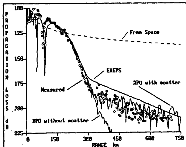
Figure 11. Comparisons of the EREPS and RPO troposcatter models to measurements. Frequency is 220 MHz, and terminal heights are 23.5 and 3048 meters.
