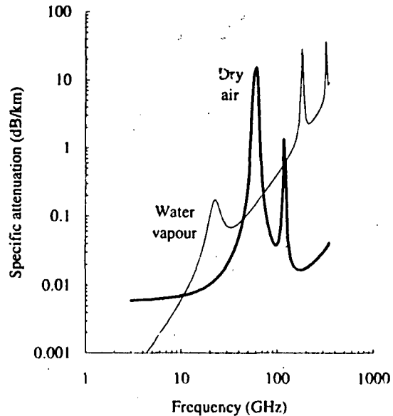
Figure 17: Specific attenuation due to atmospheric gases
