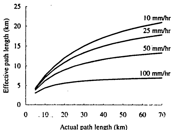
Figure 13: Effective path lengths for various 0.01% rain rates
