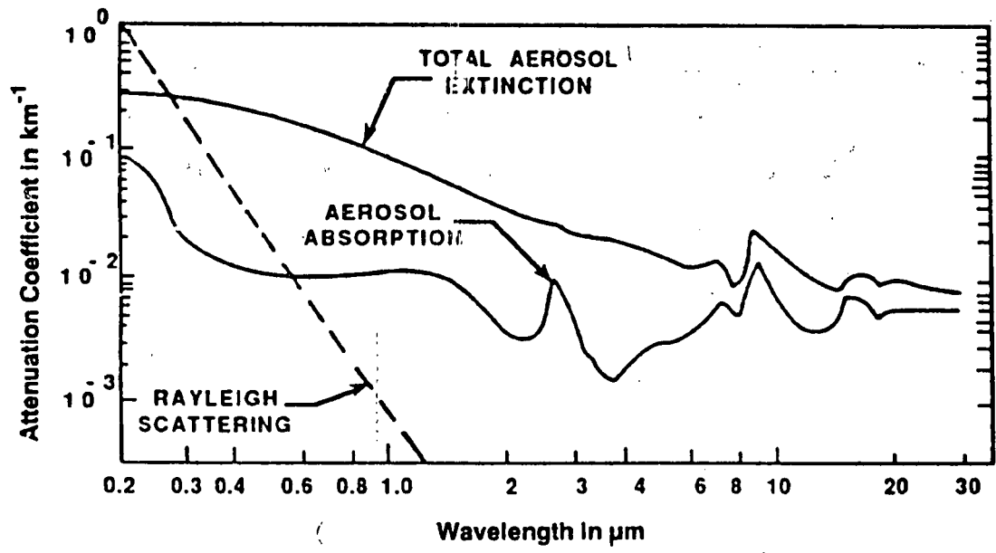
Fig. 3.9: Aerosol absorption and extinction coefficients for 23 km visibility and a continental aerosol model [13].
