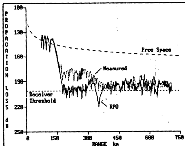
Figure 21. Modeled and measured propagation loss for the same case as Figure 19, except that the elevated duct is assumed to rise at a rate of 1:1500.
