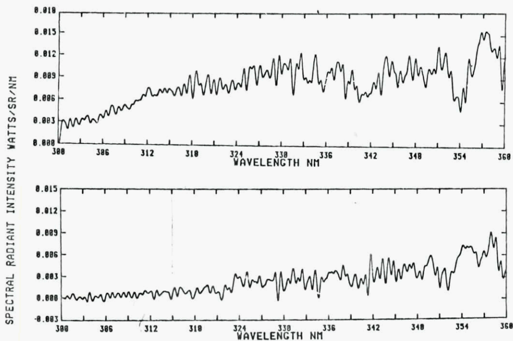
Figure 13 UV Radiometer Spectral Radiant Intensities
