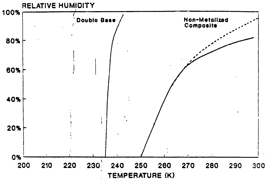
Figure 7 Predicted Secondary Smoke Formation at Sea Level
