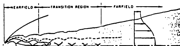
Figure 1. Structural features of plume nearfield, transition region, and farfield.
