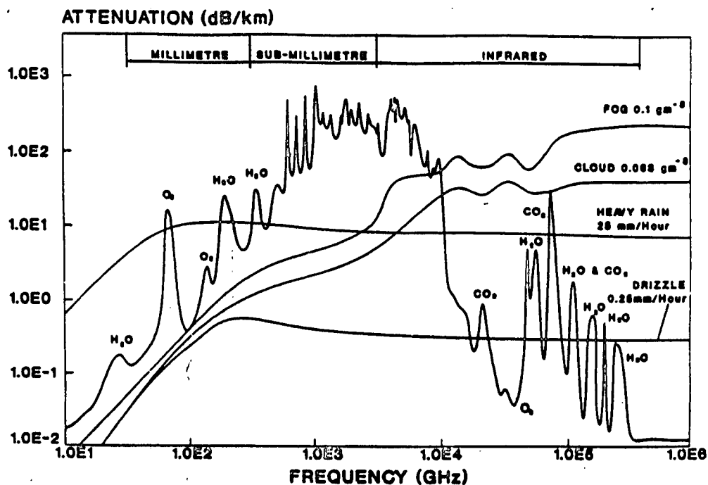
Figure 1 Atmospheric Attenuation
