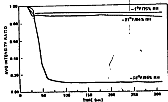
Figure 19: Courbe de transmission visible (US SCF).
