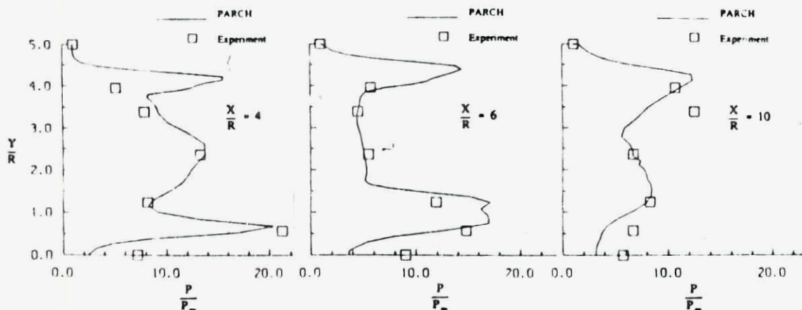
Figure 34. Pitot pressure profiles at several axial locations.
