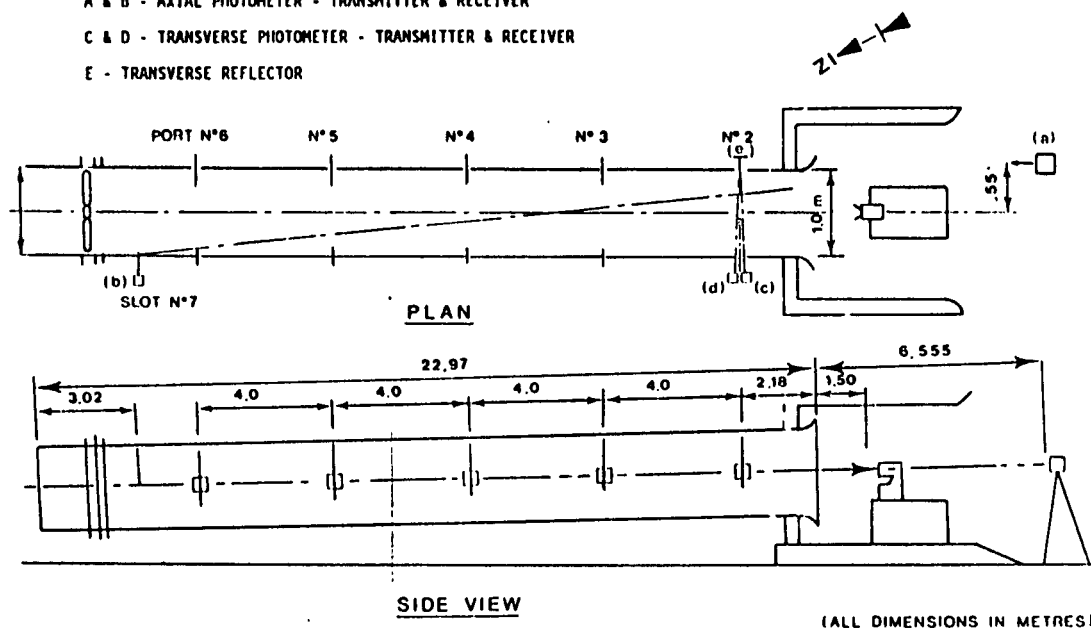
Figure 12: UK (RO) R7 Smoke Tunnel
