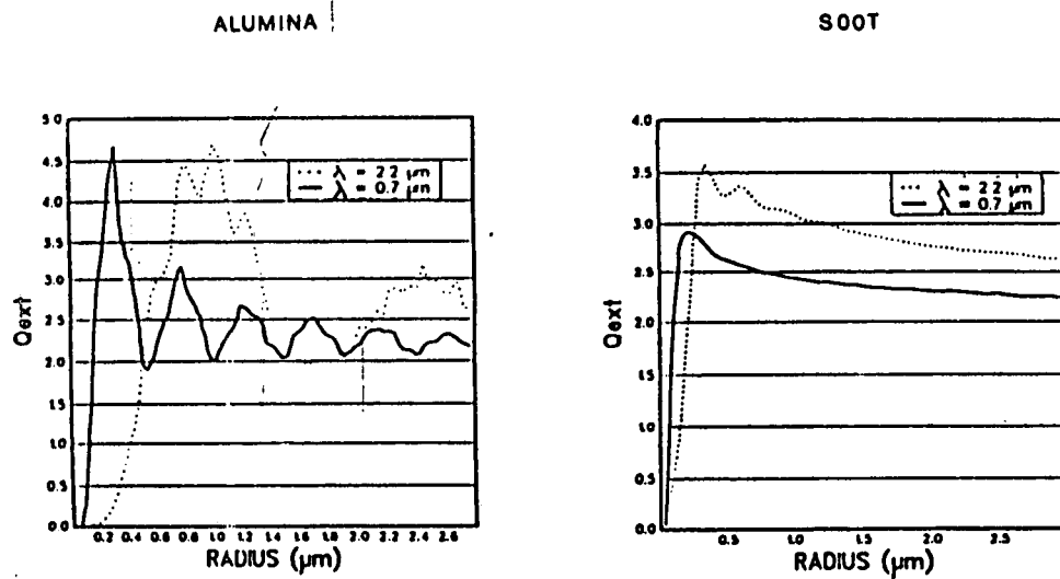
Figure 7: Typical variation of Q_{ext}
