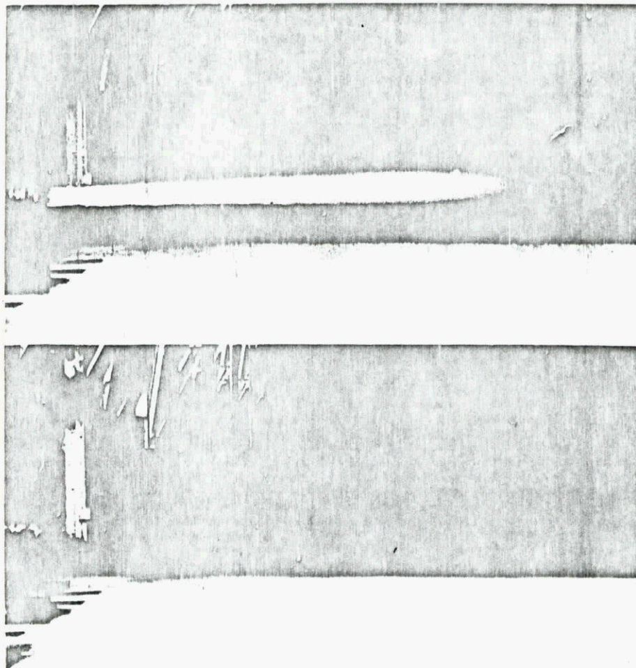
Figure 12 Flame Suppression in Nitramine Filled 7 kN Thrust Motor
