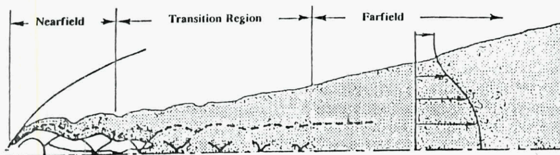
Fig.1 Regional Division of a Typical Plume
