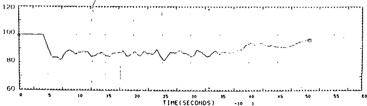
Figure 2. Transverse Smoke Transmission
