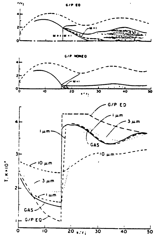
Figure 8. Influence of gas/particle nonequilibrium effects on Mach disc region structure.
