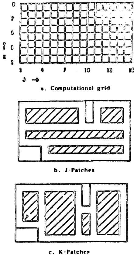
Figure 22. Patched grid methodology in PARC code for treating irregular geometries with simplified grids (from Ref. 99)
