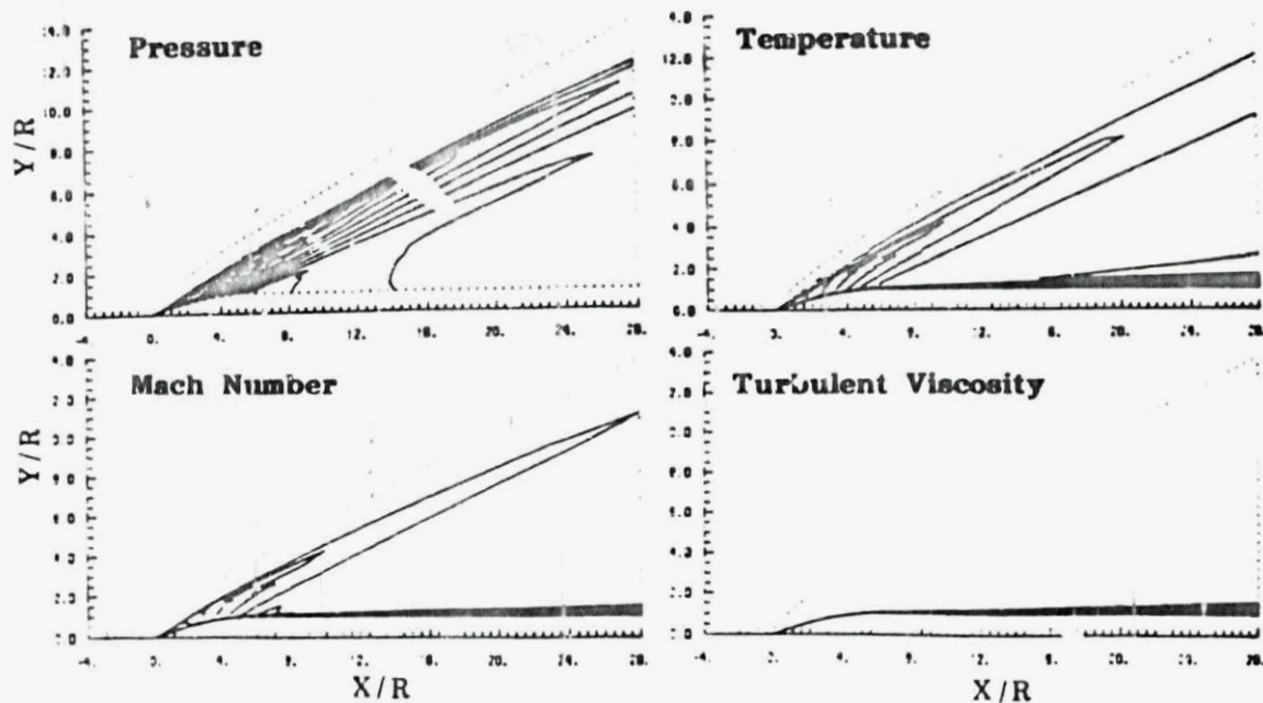
Figure 28. Computed pressure, temperature, Mach number and turbulent viscosity contours for Zone 1.
