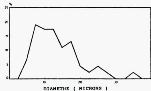
Figure 2: Particle Size Distribution of Condensed Products Collected in a Rocket Exhaust Plume. Analysed by Electro Microscope with X-rays Diffraction System. (SNPE)
