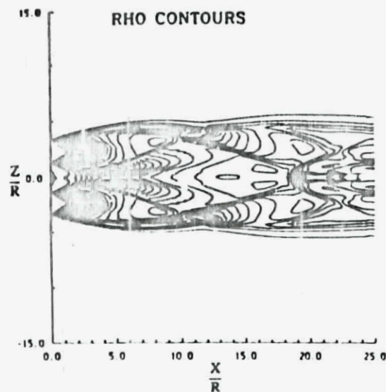
Figure 33. Computed density contours in X-Z symmetry plane
