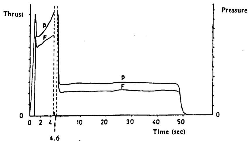
Fig. 26 Typical Thrust-Time and Pressure Curves for a Boost-Sustain Rocket Motor (see also Chapter 1)
