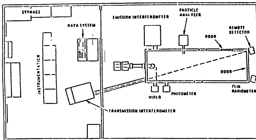
Figure 11: US Army Signature Characterization Facility (S.C.F.)
