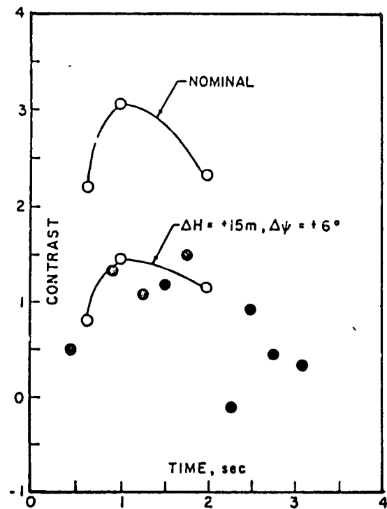
Fig. 9 Comparison of Contrast Predictions for Flight Test 2, ref 4.
