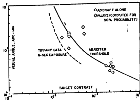
Fig. 5 Threshold of Perception, ref 4
