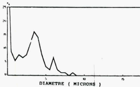
Figure 2: Particle Size Distribution of Condensed Products Collected in a Rocket Exhaust Plume. Analysed by Electro Microscope with X-rays Diffraction System. (SNPE)
