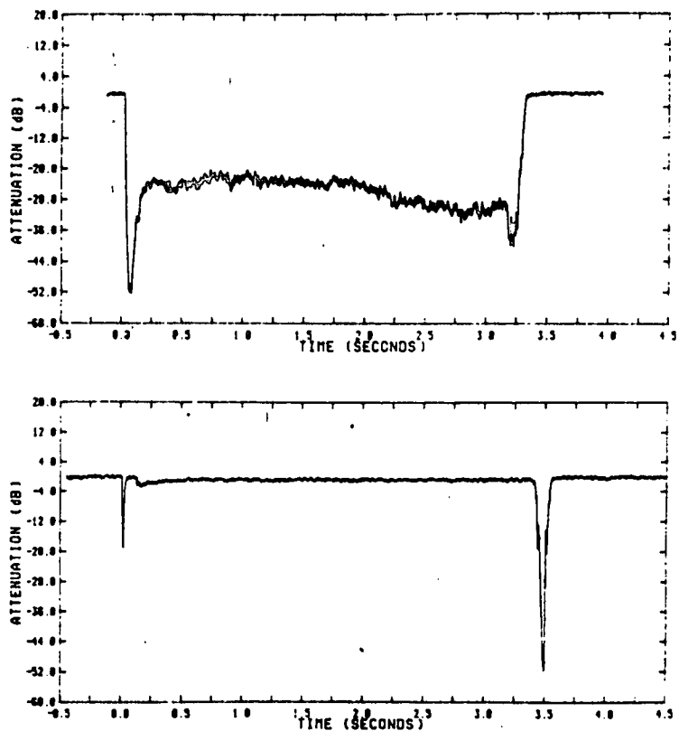
Figure 18 Millimetric Wave Radar Attenuation (30° to plume)
