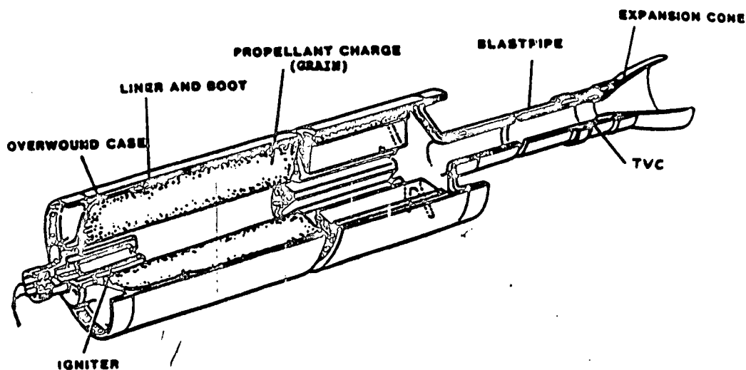
Figure 2 Solid Propellant Rocket Motor
