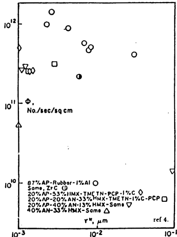
Fig. 7 Nucleation Data form MICOM Smoke Facility
