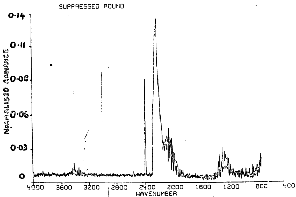
Figure 16 Infra Red Normalised Spectral Radiant Intensities
