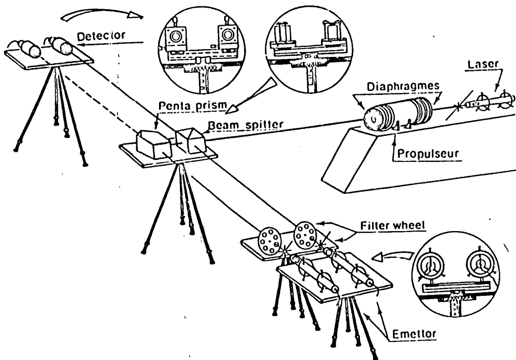
Figure 16: Free Jet Firing. Transmission at 0.63 \mu\text{m}
