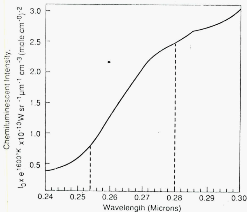
Fig. 2c Ultraviolet Portion: CO + O Chemiluminescence Intensity Spectrum
