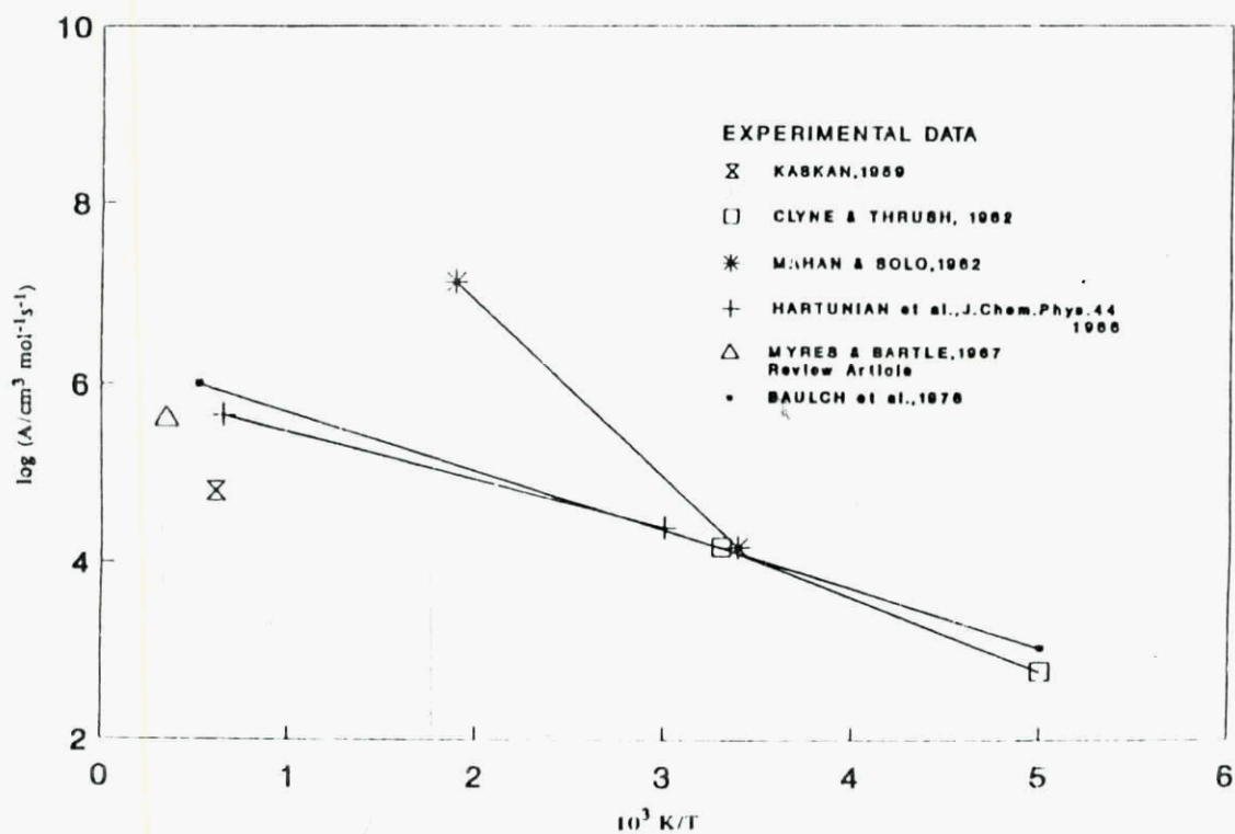
Fig. 2a CO + O Chemiluminescence Rate Constant Data
