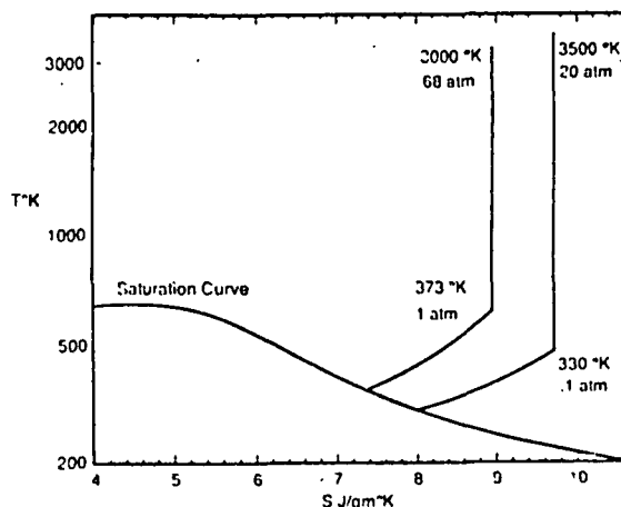
Fig. 1 Condensation Considerations on the T-S Plane.
