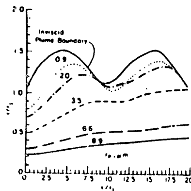
Figure 18. Limiting particle streamlines in nearfield of tactical missile exhaust plume.
