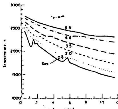
Figure 17. Gas and particle temperature variations along nozzle centerline.
