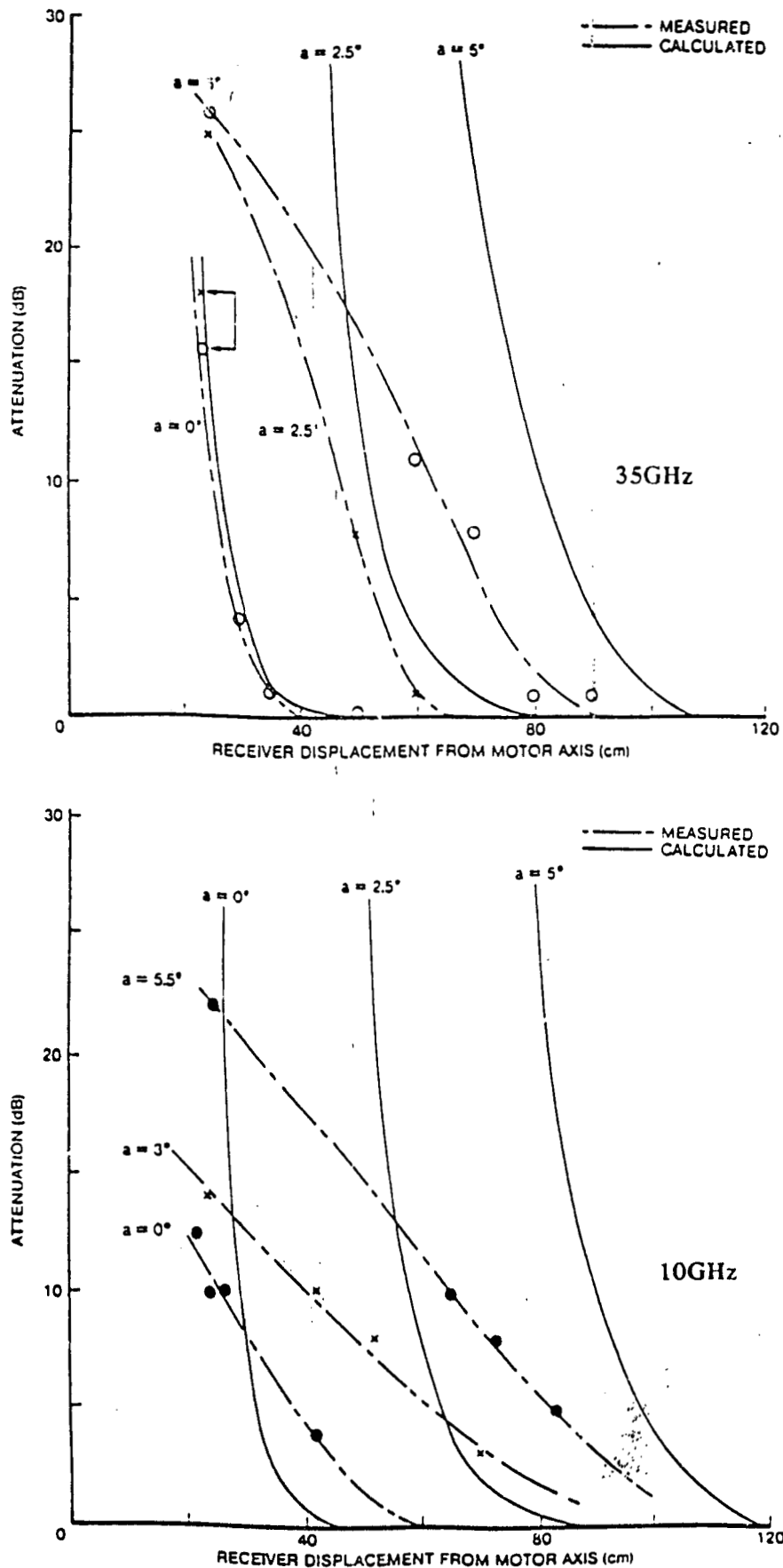
Fig. 10 Comparison of Predicted and Measured Attenuation Against Receiver Displacement for Three Aspect Angles
