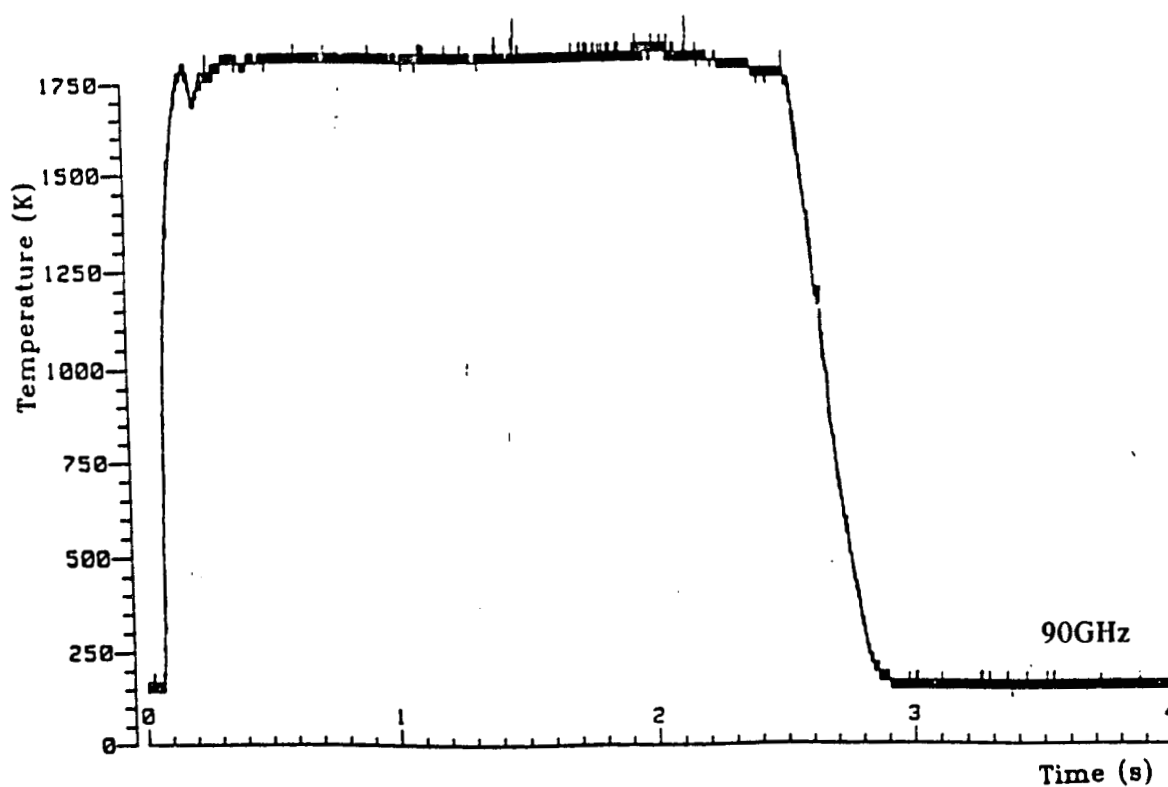
Fig. 19 Emission Apparent Brightness Temperatures for Double Base Propellant Motor in Two Wavebands
