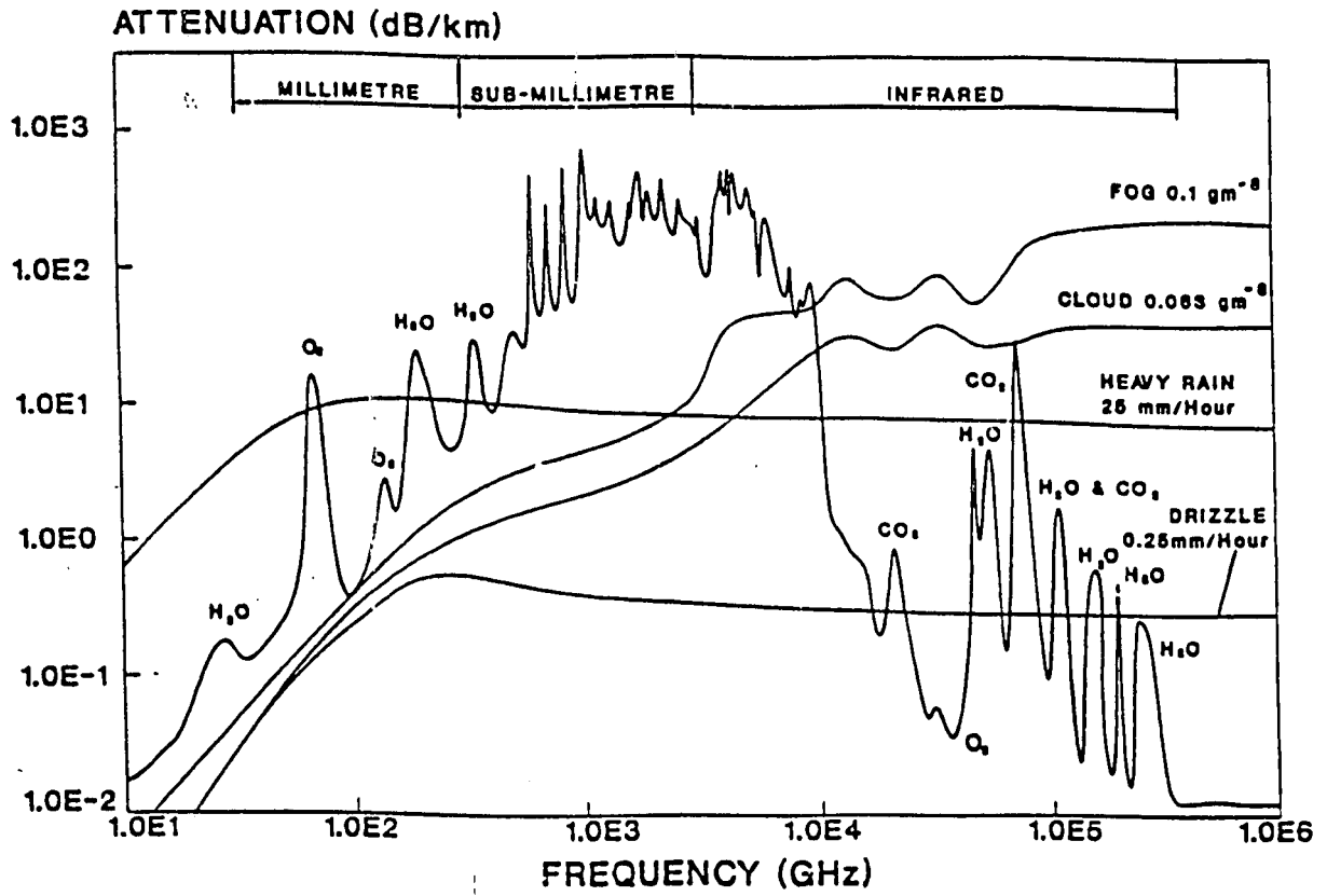
Fig. 17 Atmospheric Attenuation
