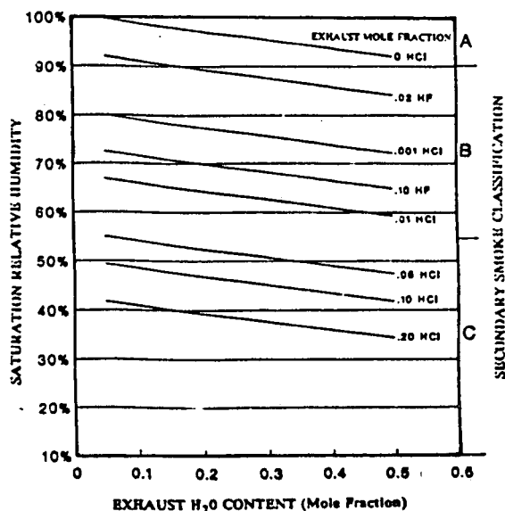
Fig. 12 Saturation Relative Humidity for AGARD Secondary Smoke Classification at 0°C, 1 atm., 1000 Dilution, ref 18.
