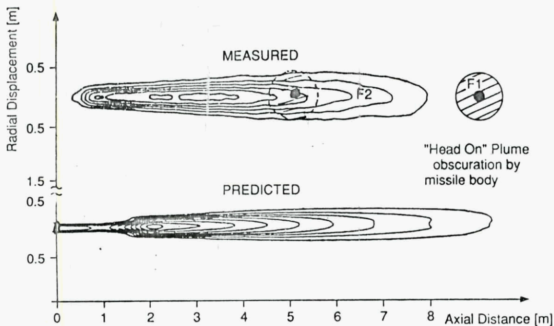
Fig. 3 ISO-radiance Contours for a Composite Propellant Rocket Motor Exhaust (IR) with "Head On" Obscuration
