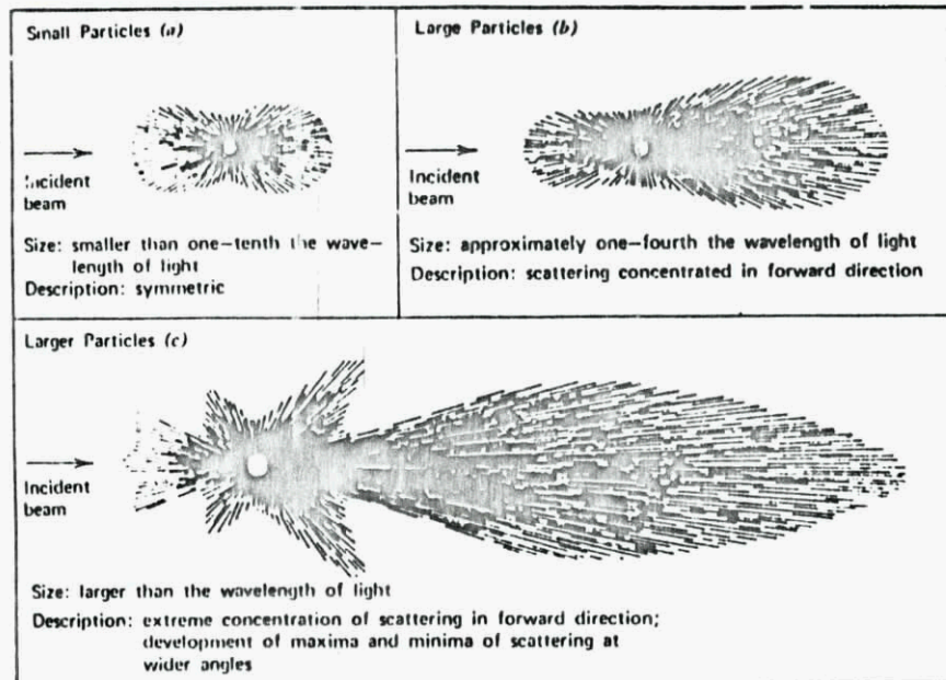
Figure 1: Angular pattern of scattered intensity from particules of three sizes : (a) Small particles, (b) large particles, (c) larger particles [2]
