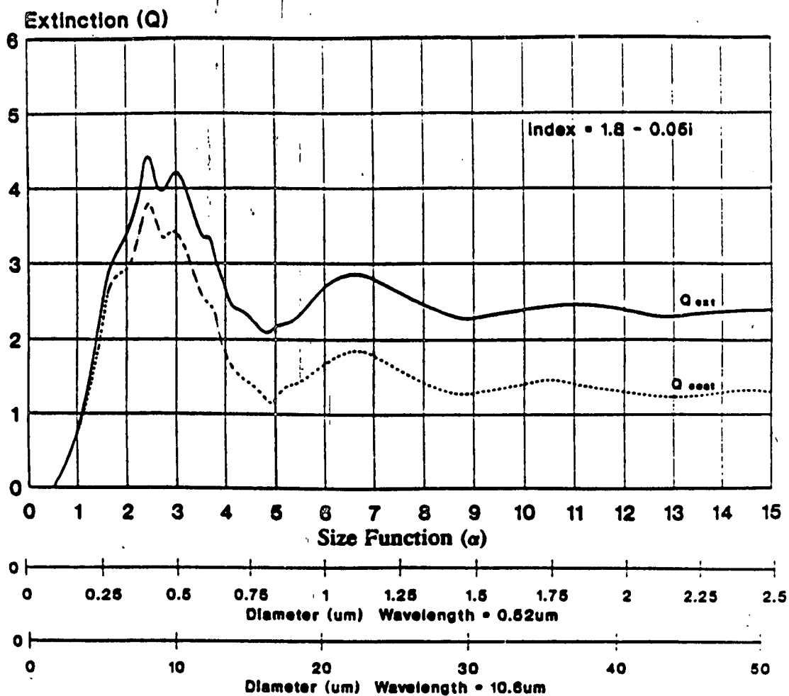
Figure 3 Extinction and Scattering Cross Sections for Typical Absorbing Solid Particle (Size function \alpha = \pi D / \lambda ).
