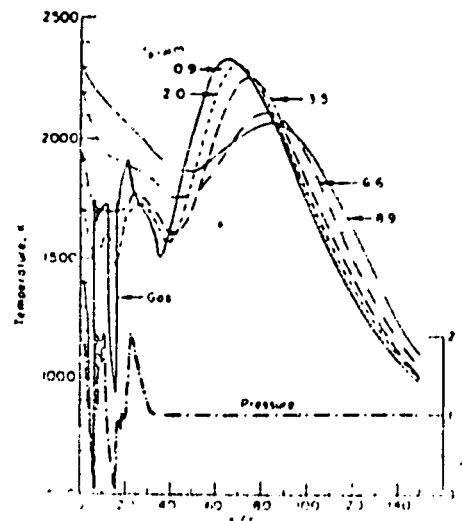
Figure 20. Gas and particle temperature and pressure variations along plume nearfield/farfield centerline.
