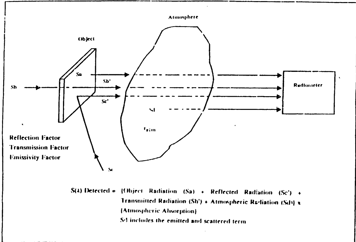
Fig. 13 Radiometric Essentials
