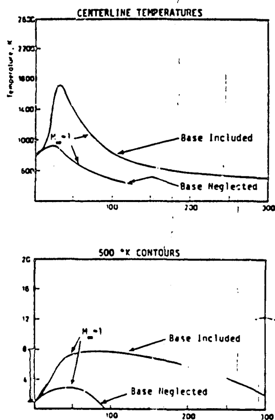
Figure 6. Base region flameholding effect: centerline temperatures and 500°K contours with and without base incorporated in plume solution.
