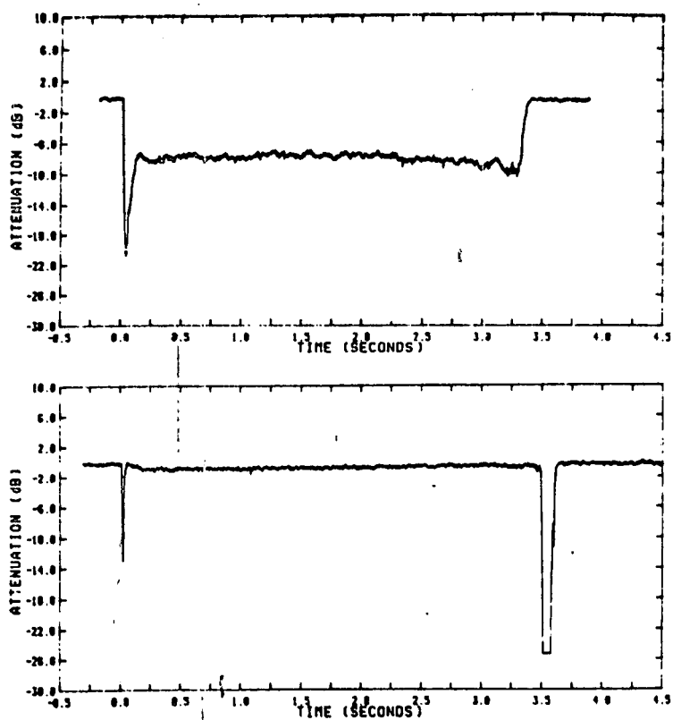
Figure 17 Millimetric Wave Radar Attenuation (Normal to plume)
