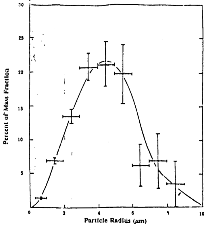
Fig. 6 Typical Measured Particle-Size Distribution
