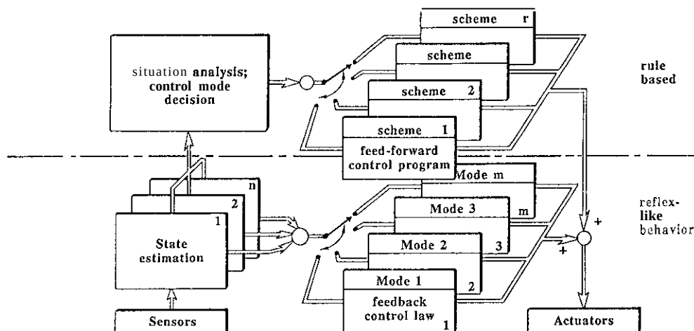
Figure 3. Stable fast, reflex like feedback control determination with triggered feed forward components; situation dependent control mode decision
