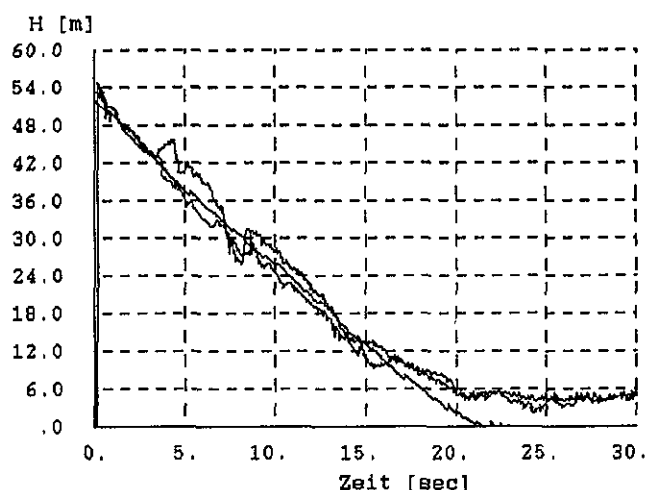
Figure 8. Estimated altitude time history
