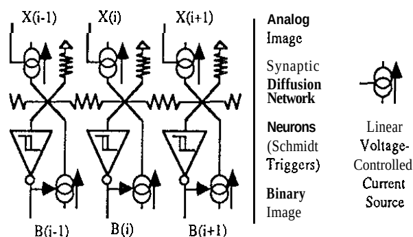
Figure 15 : 1-D resistive neural halftoning network.
