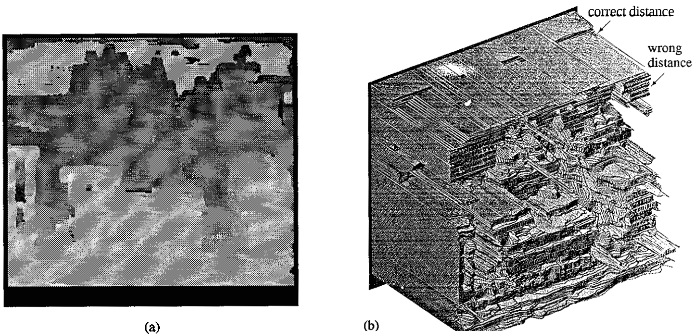
Figure 9: Result with a long baseline, B = 9b : (a) Distance map; (b) Isometric plot. The matching is less noisy when it is correct. However, there are many gross mistakes, especially in the top of the image where, due to a repetitive pattern, the matching is completely wrong.
