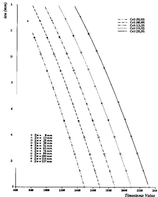
Figure 13: Time-stamp calibration result
