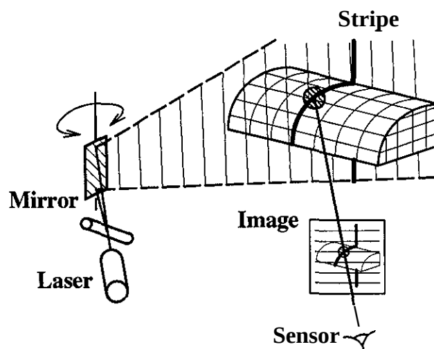
Figure 1: Traditional light-stripe range imaging
