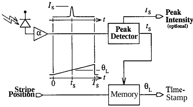
Figure 4 Basic sensing element block diagram.
