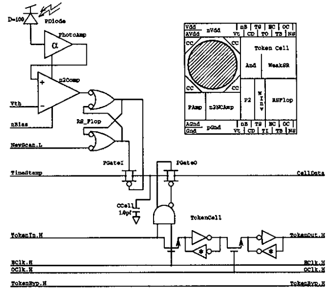
Figure 6 Sensing element circuitry.
