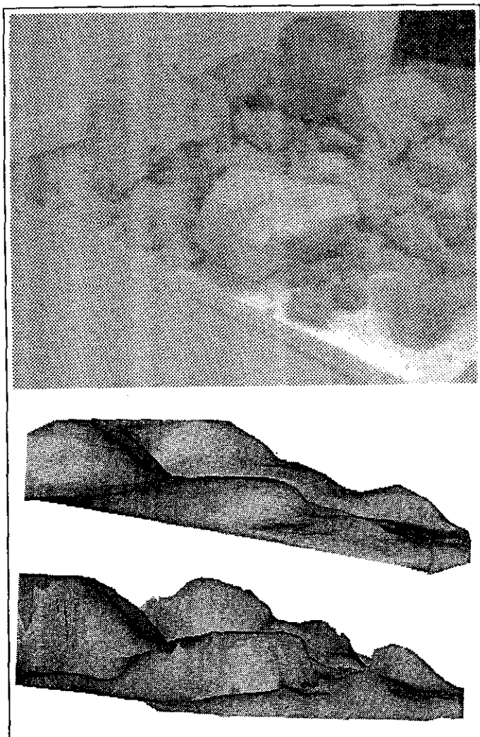
Fig. 6. Refined Scene Model from Stereo Sequence.
