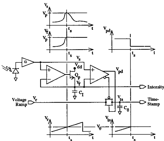
Figure 19: Second-generation sensing element circuitry.
