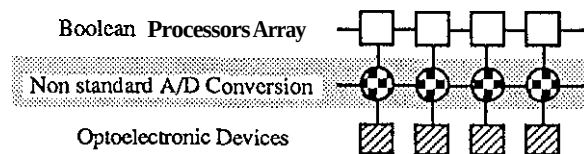
Figure 2 : The "Retina" circuit (cross section).
