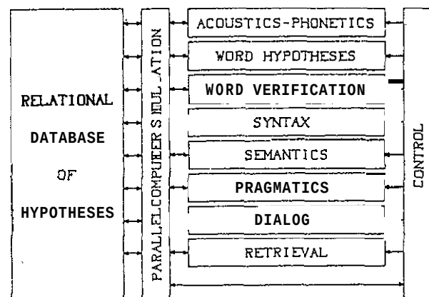
Fig.6.2: Blackboard approach for speech understanding.
