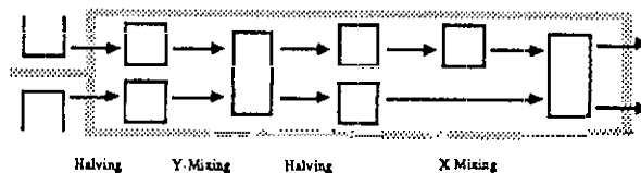
Figure 5 : 2-D Parallel and Pipelined Binomial Convolution
