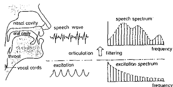
Fig.2.1: Principle of natural speech production (voiced sounds).
