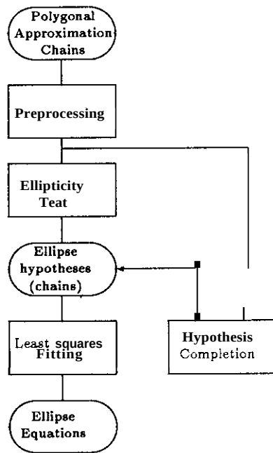
Figure 8: Flowchart of the ellipse detection algorithm
