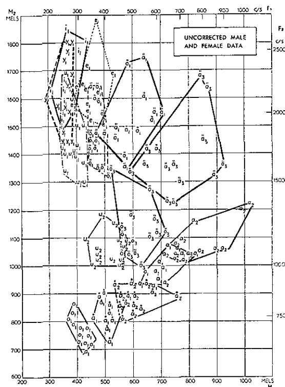
Fig. 6.5: F2/F1-Plot of the Swedish vowels. (Fan59)
