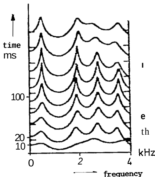
Fig.3.3: LPC-Spectrum of the word "They"
