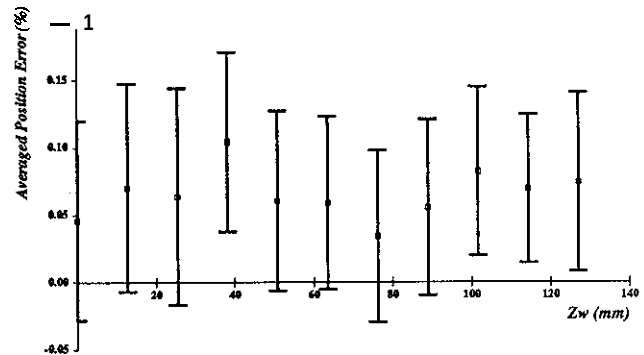
Figure 15: Range data accuracy and repeatability.
