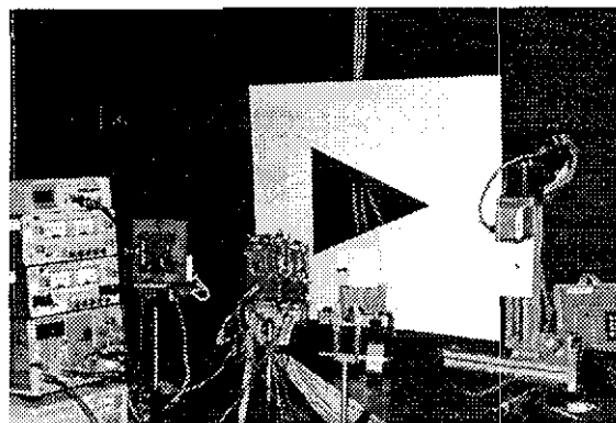
Figure 8: The cell-parallel range-finding system.
