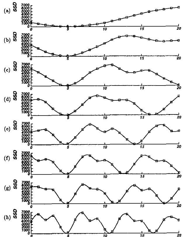
Figure 5: SSD values vs. inverse depth: (a) E = b ; (b) E = 2b ; (c) E = 3b ; (d) B = 4b ; (e) B = 5b ; (f) B = 6b ; (g) B = 7b ; (h) B = 8b . The horizontal axis is normalized such that 8bF = 1 .
