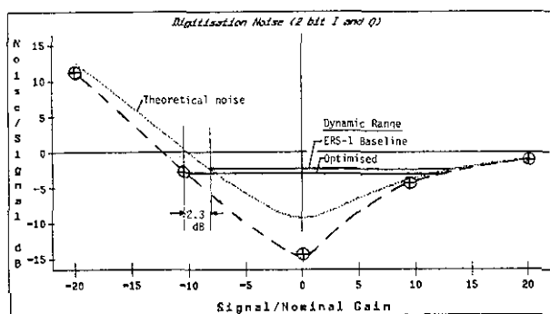
Fig. 23 2-bit quantisation noise curve.
