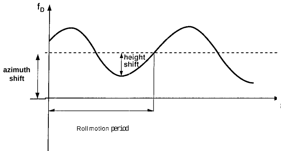
Figure 5: Evolution and interpretation of the Doppler frequency
