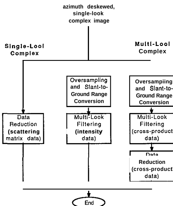
Figure 3b: Standard postprocessing algorithm flowchart.
