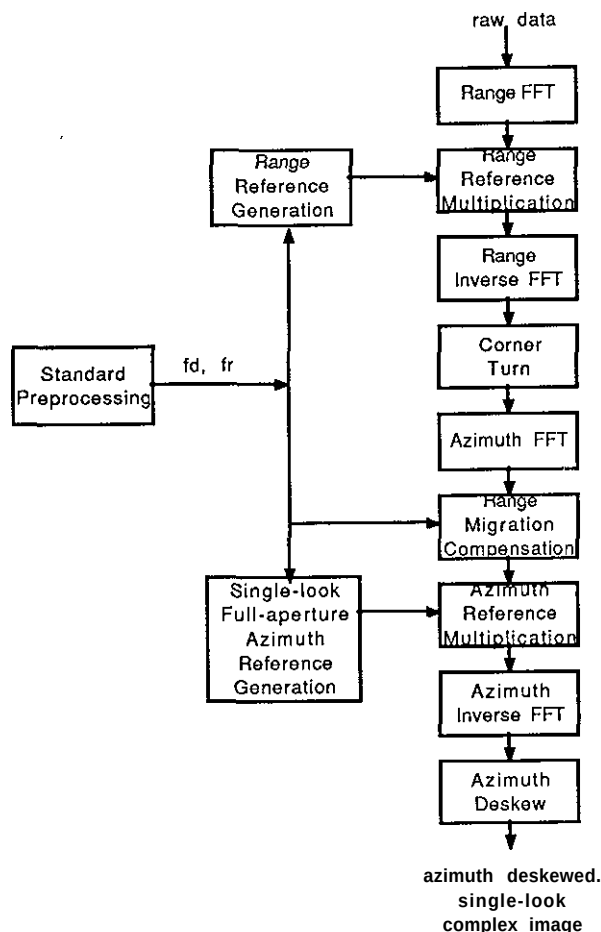
Figure 3a: Standard processing algorithm flowchart.
