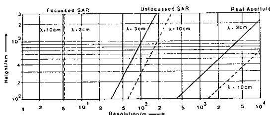
Fig. 1 represents the maximum azimuth resolution of different radar systems versus height for a 10 m antenna length typically used for spaceborne SAR as it is installed on ERS-1 for instance.
