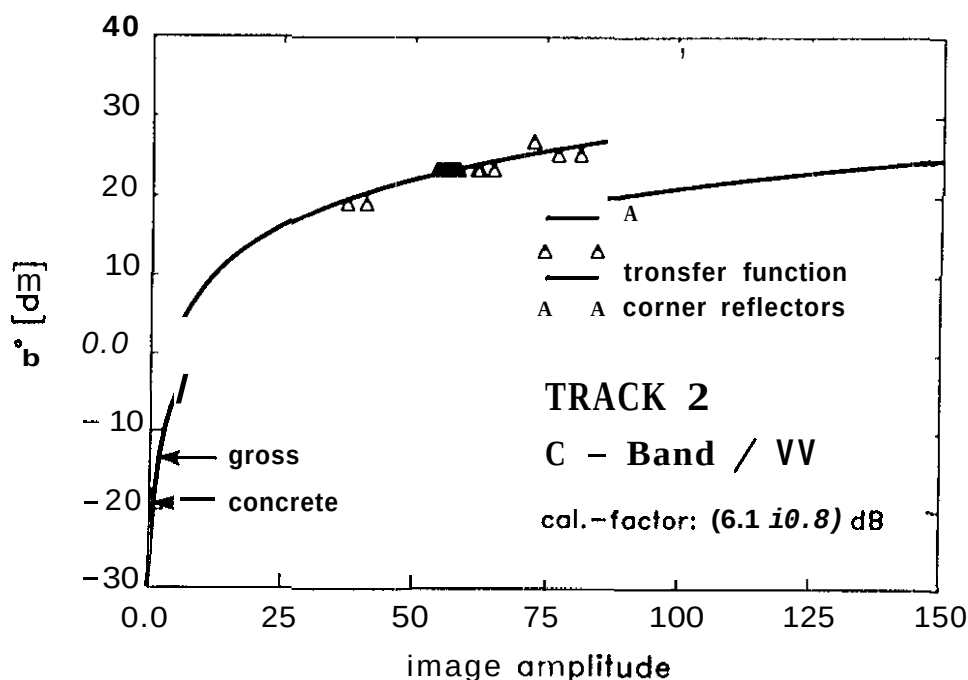
Fig. 10 DC-8 SAR system transfer function.
