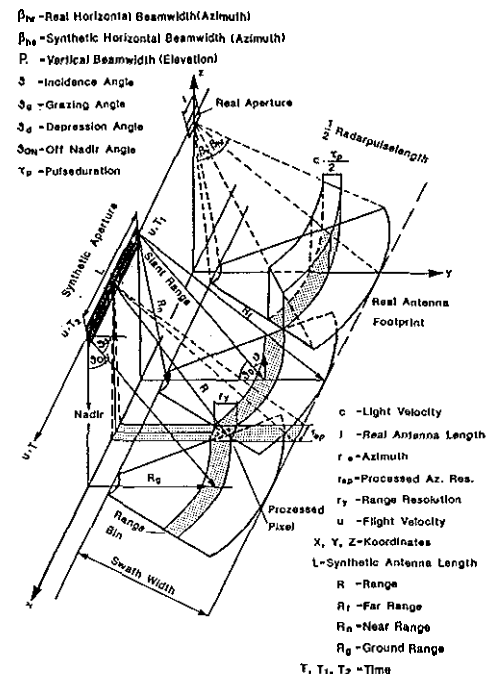
Fig. 1 Geometry and terminology for SAR in 3-dimensional representation.
