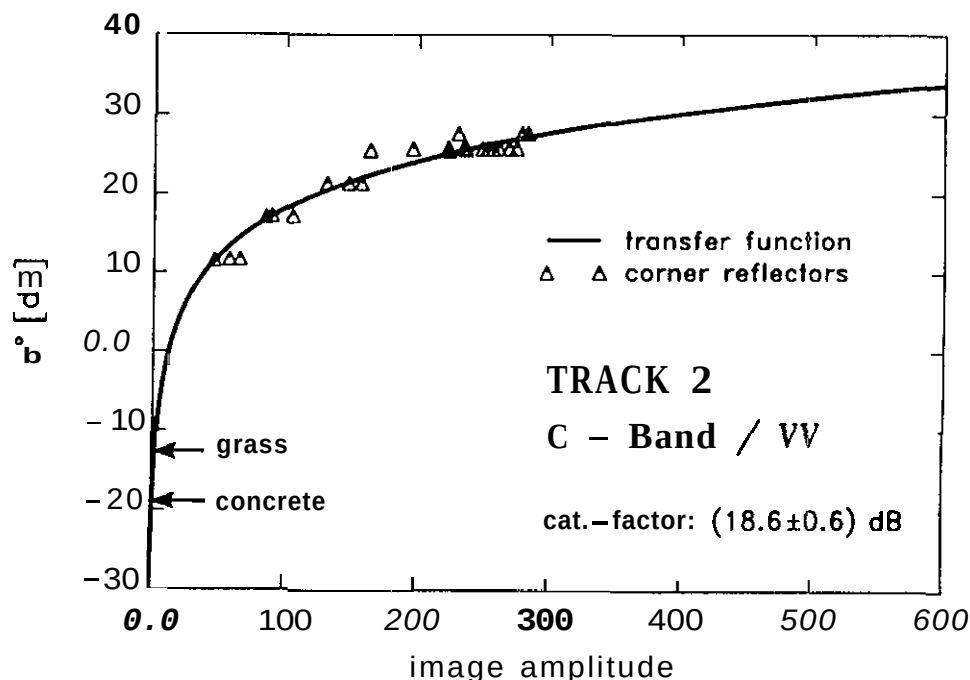
Fig. 9 E-SAR system transfer function.
