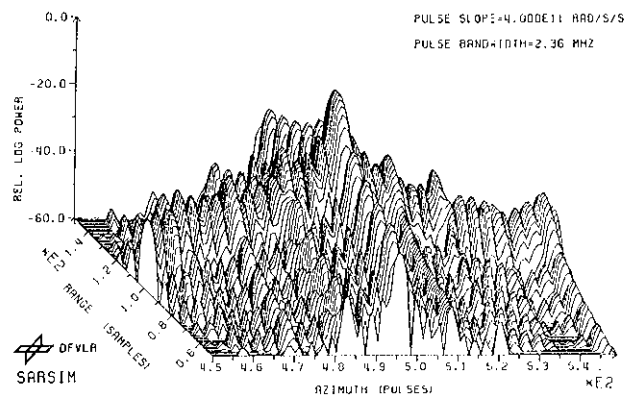
Fig. 19 Signal after azimuth compression.
