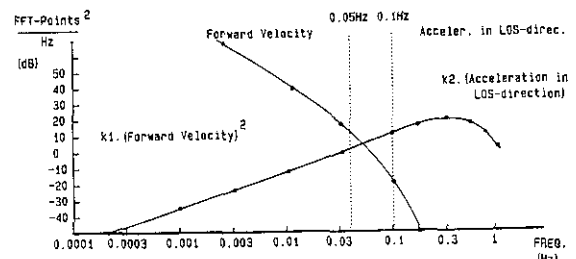
Fig. 16 Power spectral density of the forward velocity and acceleration in LOS for a D0 228 aircraft.
