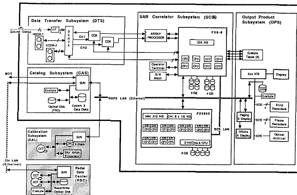
Figure 4: SIR-C ground data processing system hardware architecture.
