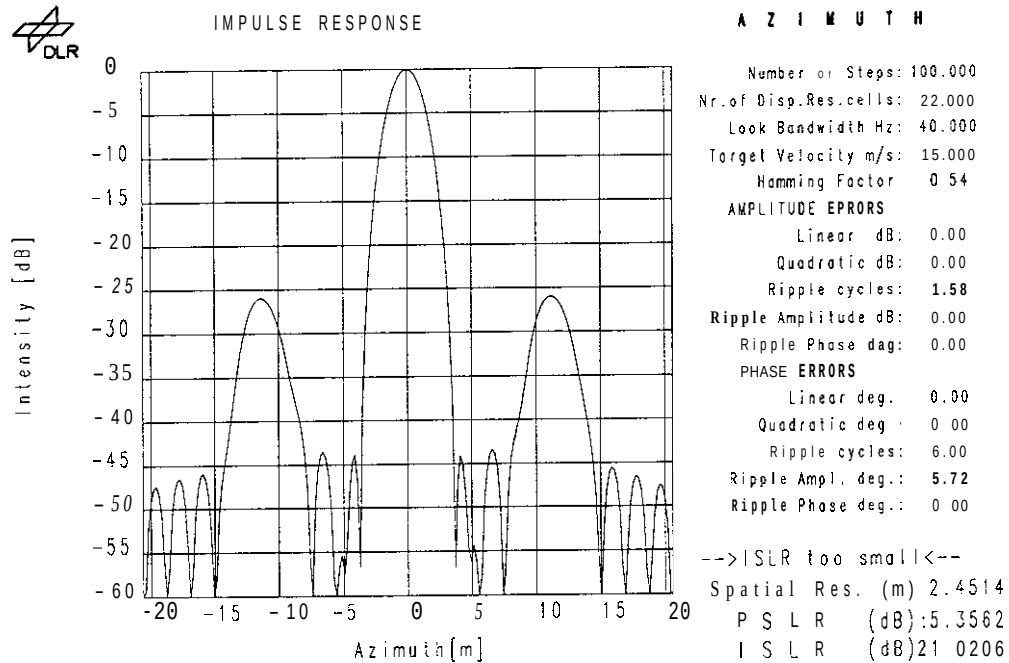
Fig. 2 Azimuth impulse response computed with IMPRES.
