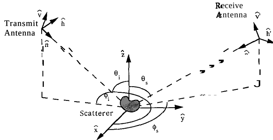
Fig. 3 Coordinate systems for radar scattering.
