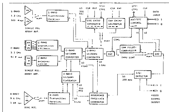
Fia. 24 E-SAR Sensor system blackdiagram (RF-elec-tronics)
