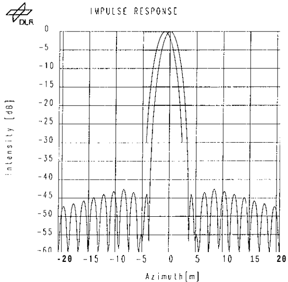
Fig. 4a Impulse response with no phase errors and the shift due to a linear error of \pi rad.
