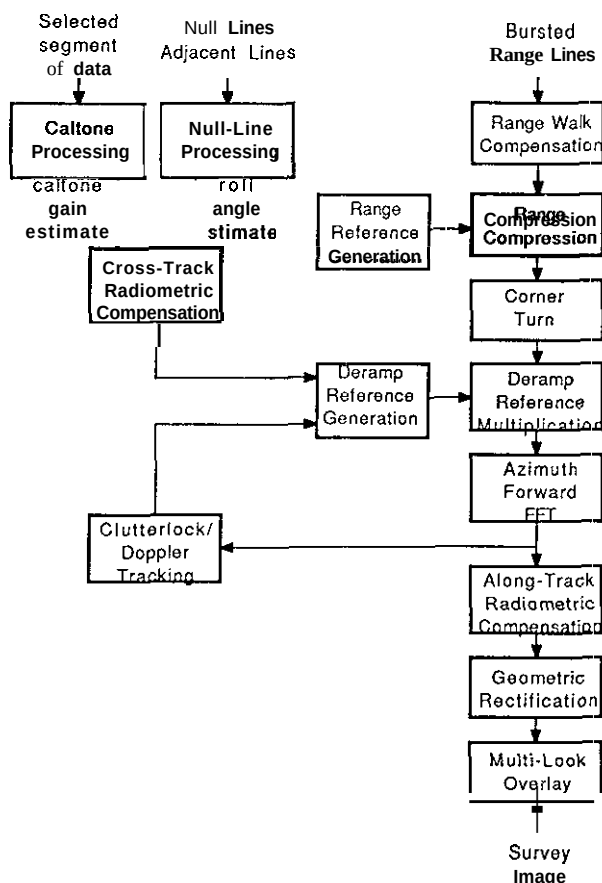
Figure 2: Survey processing algorithm flowchart
