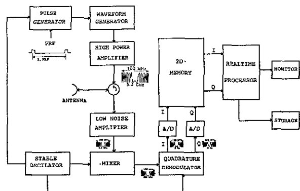
Fig. 23 Block diagram of a SAR (schematically).
