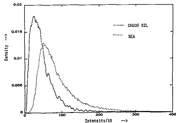
Fig. 10 Histogram of the filtered SAR image of Fig. 6. (Oil slick A2, 660 m flight altitude.) Both curves follow a Rayleigh distribution.
