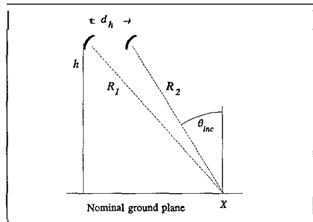
Figure 3. Basic geometry for topographic interferometric imaging radars.
