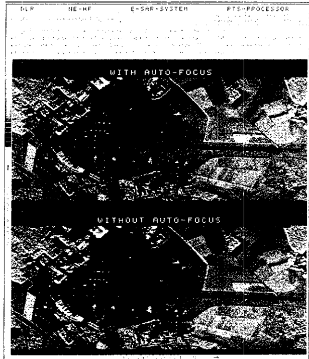
Fig. 4 Example for focus influence of an image quality. The lower image is unfocused (errors result from velocity) the upper image is focussed.
