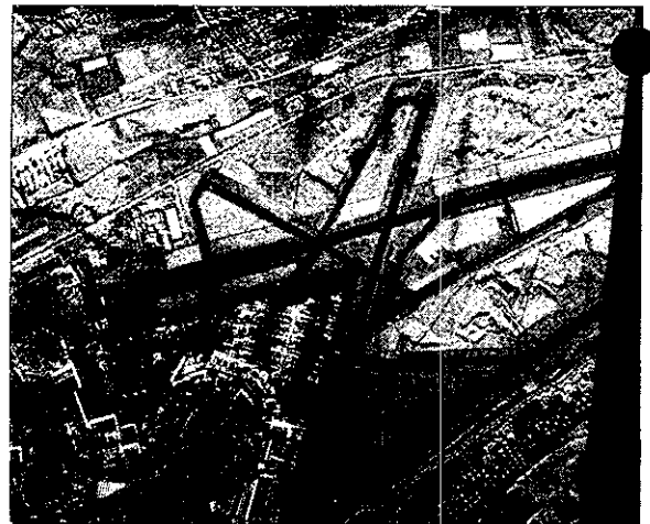
Fig. 7b SAR image of Fig. 7a, correctly processed to the squint angle 6.8°; all ambiguities are eliminated (measurement Horn, Moreira).
