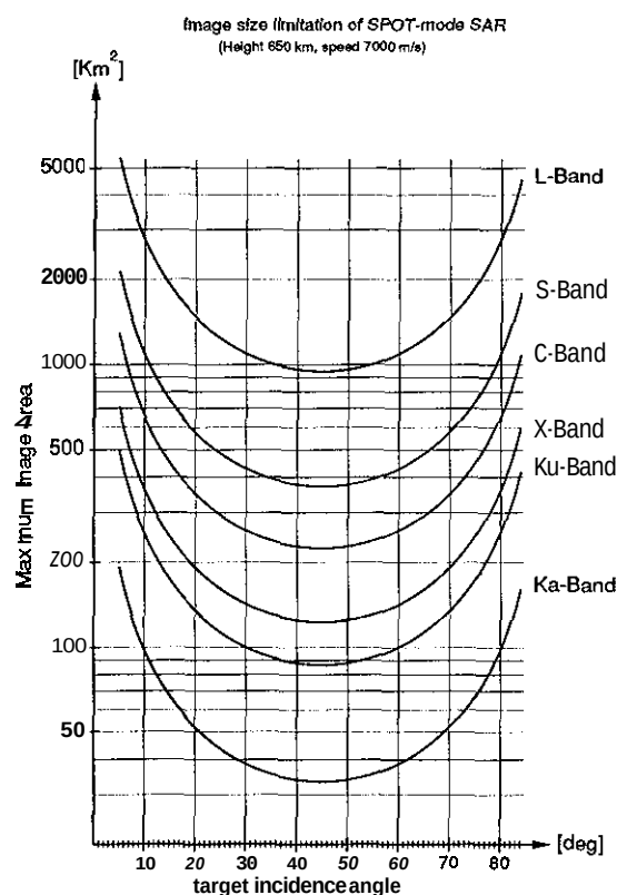
Fig. 9 Illuminated area for spot lightmode and/or azimuth look steering mode increases approximately proportionally with the wavelength.
