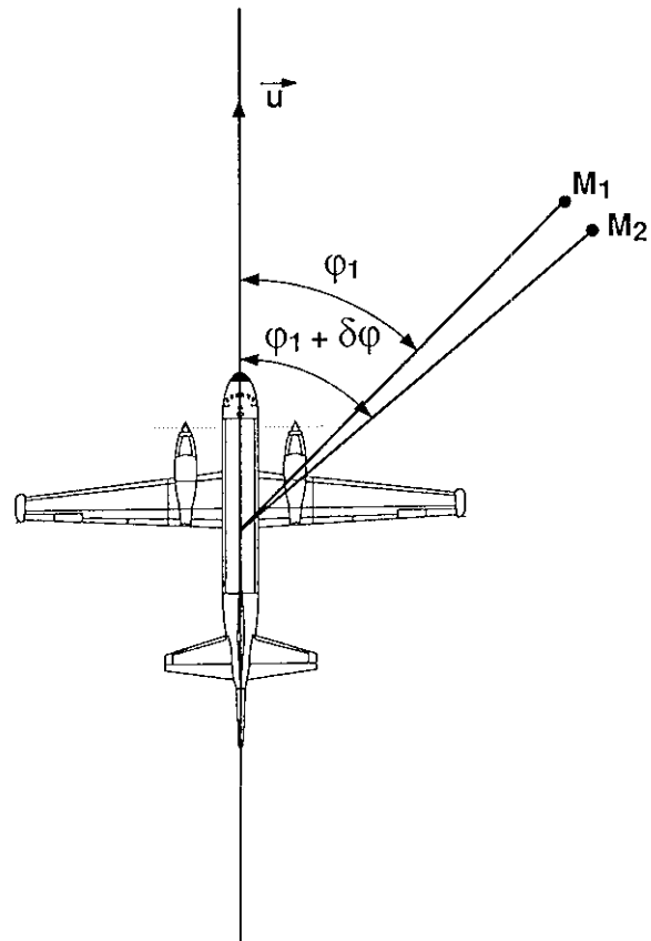
Figure 3: SAR geometry
