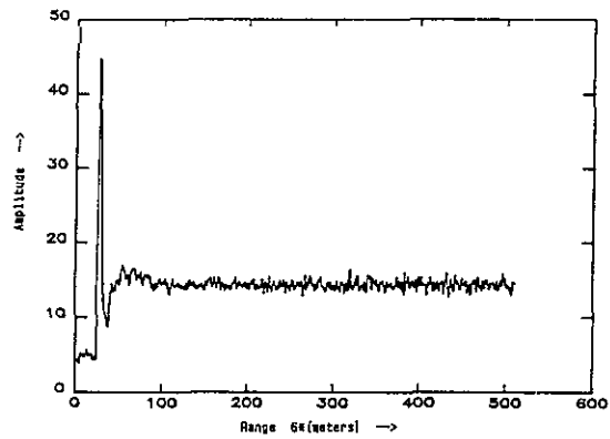
Fig. 8 Signal intensity curve of the image in Fig. 6 after radiometric correction using the curve in Fig. 1b. (660 m flight altitude, 30 deg depression angle.)
