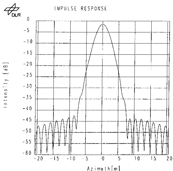
Fig. 4b Impulse response with a quadratic phase error of \pi rad.
