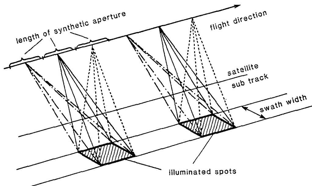
Fig. 8 Azimuth look steering mode increases the overall synthetic aperture (for multi look images with azimuth resolution r_{ap} ). Only spot-wise data take are possible in this mode.
