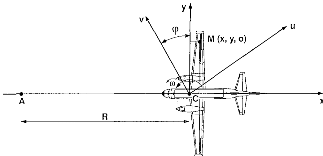
Figure 1: Basic ISAR geometry
