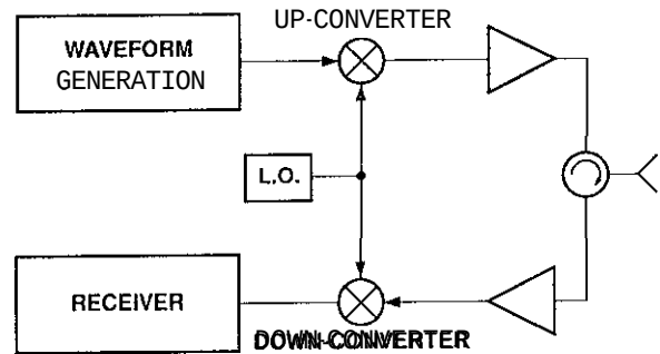
Figure 7: Transmission/Reception bloc-diagram
