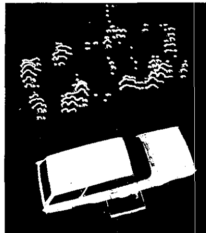
Fig. 9 Distribution of reflection centers on a car in a two-dimensional representation. Resolution is about 15 cm x 15 cm (measurement Graf DLR [2]).
