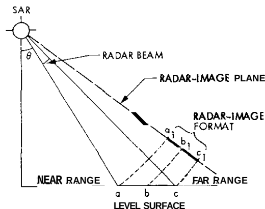
Fig. 15 Radar-image format showing slant-range presentation a_1, b_1, c_1 relative to ground-range abc , assuming a level surface long-dashed line represents radar-image plane. Look angle is inclination of the radar beam off vertical [14].
