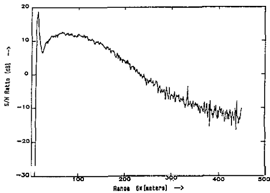
Fig. 1a Signal to noise ratio over the whole scene in Fig. 6 as a function of range. (660 m flight altitude, 30 deg depression angle [7].) The Altitude line echo (ALE) clearly can be identified.
