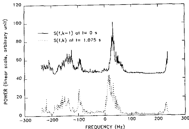
Fig. 16 Power spectral density of the forward velocity and acceleration in LOS for a D0 228 aircraft.
