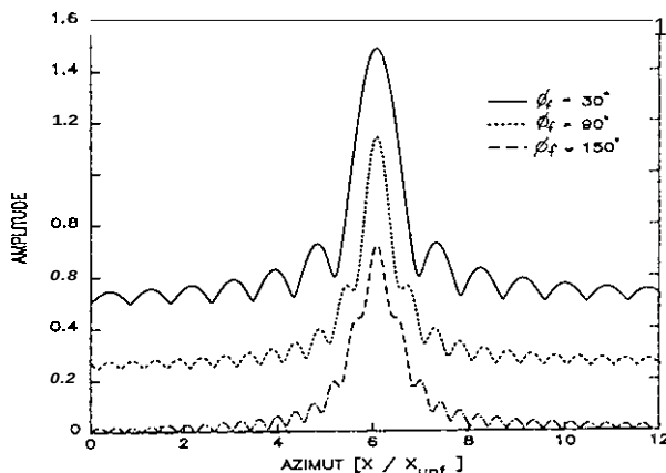
Fig. 3 Point target impulse response degradation for unfocused processing with different phase deviations (30°, 90°, 180°).
