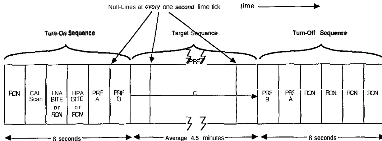
Figure 1: SIR-C input data run format. Each Segment in turn-on and turn-off sequence is 1 second duration. RON: Receive Only Noise, LNA: Low Noise Amplifier, HPA: High Power Amplifier, CAL scan: Caltone Scan.
