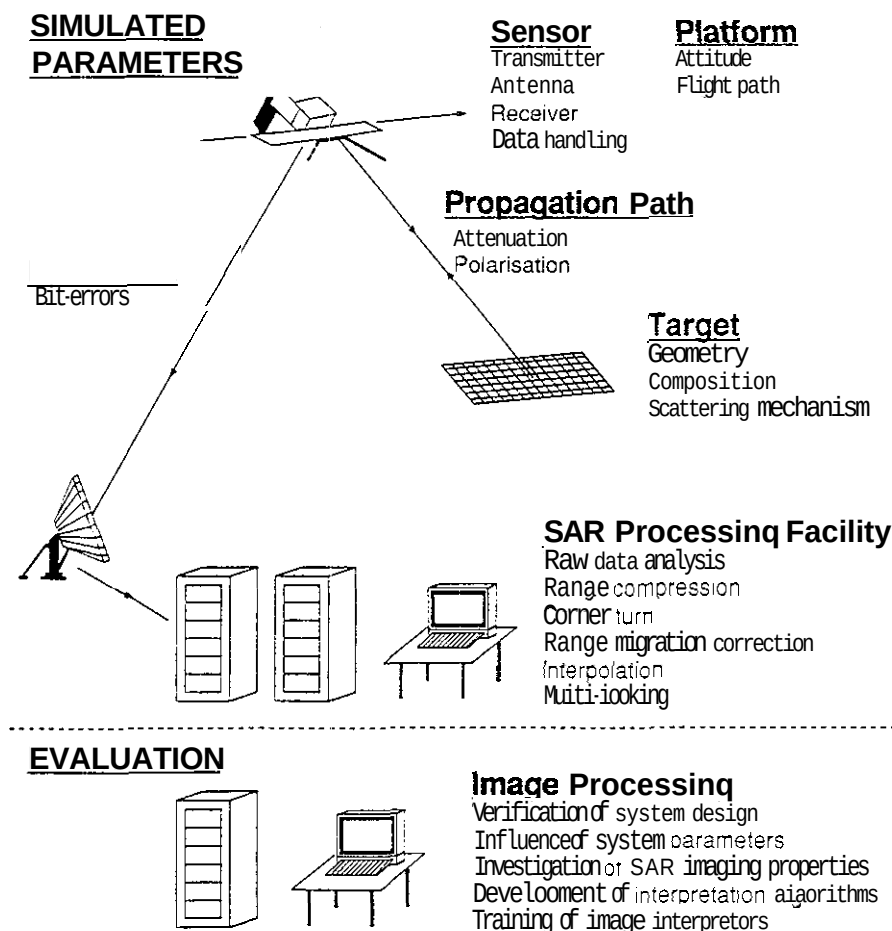
Fig. 1 Simulated elements and evaluation tasks of a comprehensive SAR simulator.
