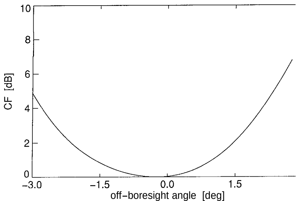
Fig. 2 Correction function CF across the swath. Near range is on the left, far range on the right; boresight angle of antenna is 0^\circ .
