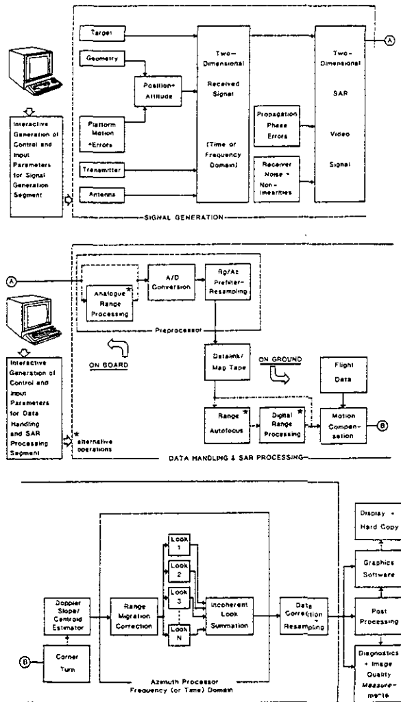
Fig. 10 Sarsim configuration.
