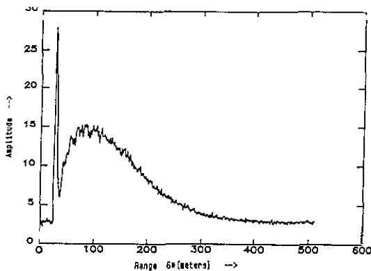
Fig. 7b Signal intensity curve of Fig. 1a as a function of range integrated over 50 s. (660 m flight altitude, 30 deg depression angle.)
