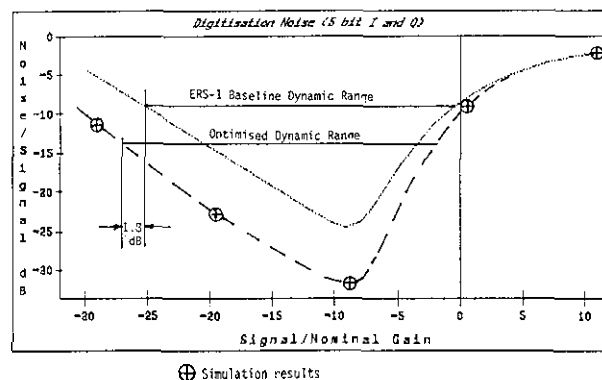
Fig. 24 5-bit quantisation noise curve.
