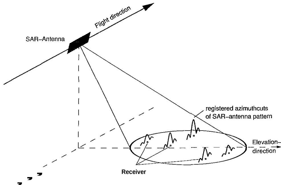
Fig. 5: Schematic experiment set-up.
