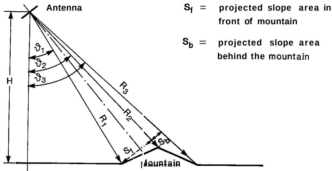
Fig. 12 illumination geometry for a mountain
