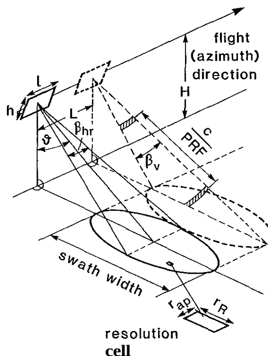
Fig. 1 Coordinate system and illumination geometry.
