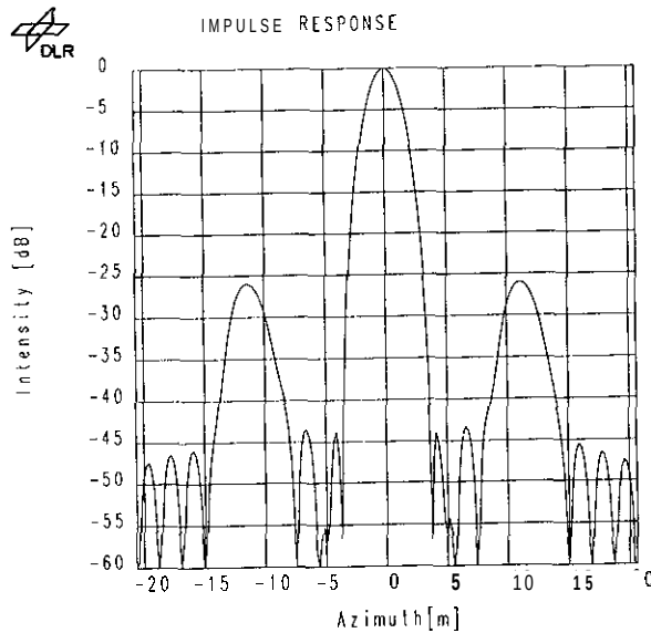
Fig. 4c Impulse response with a sinusoidal phase error of 0.1 rad amplitude and 6 cycles across the interval showing paired echoes.
