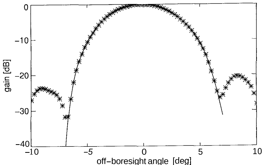
Fig. 3 Predetermined X-SAR elevation pattern.
