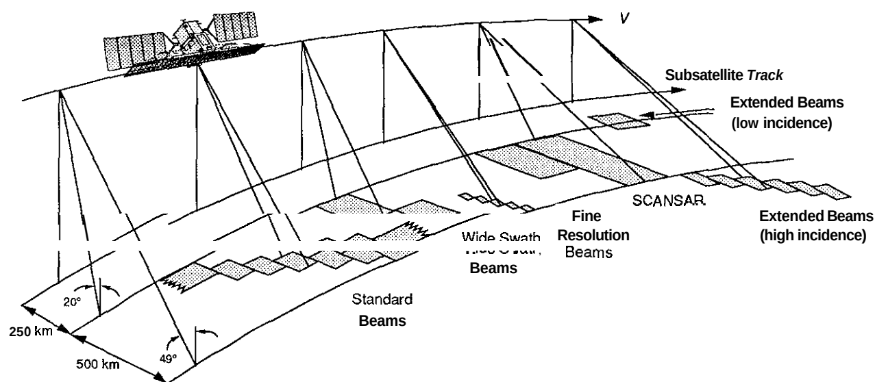
Figure 2. RADARSAT Imaging Modes
