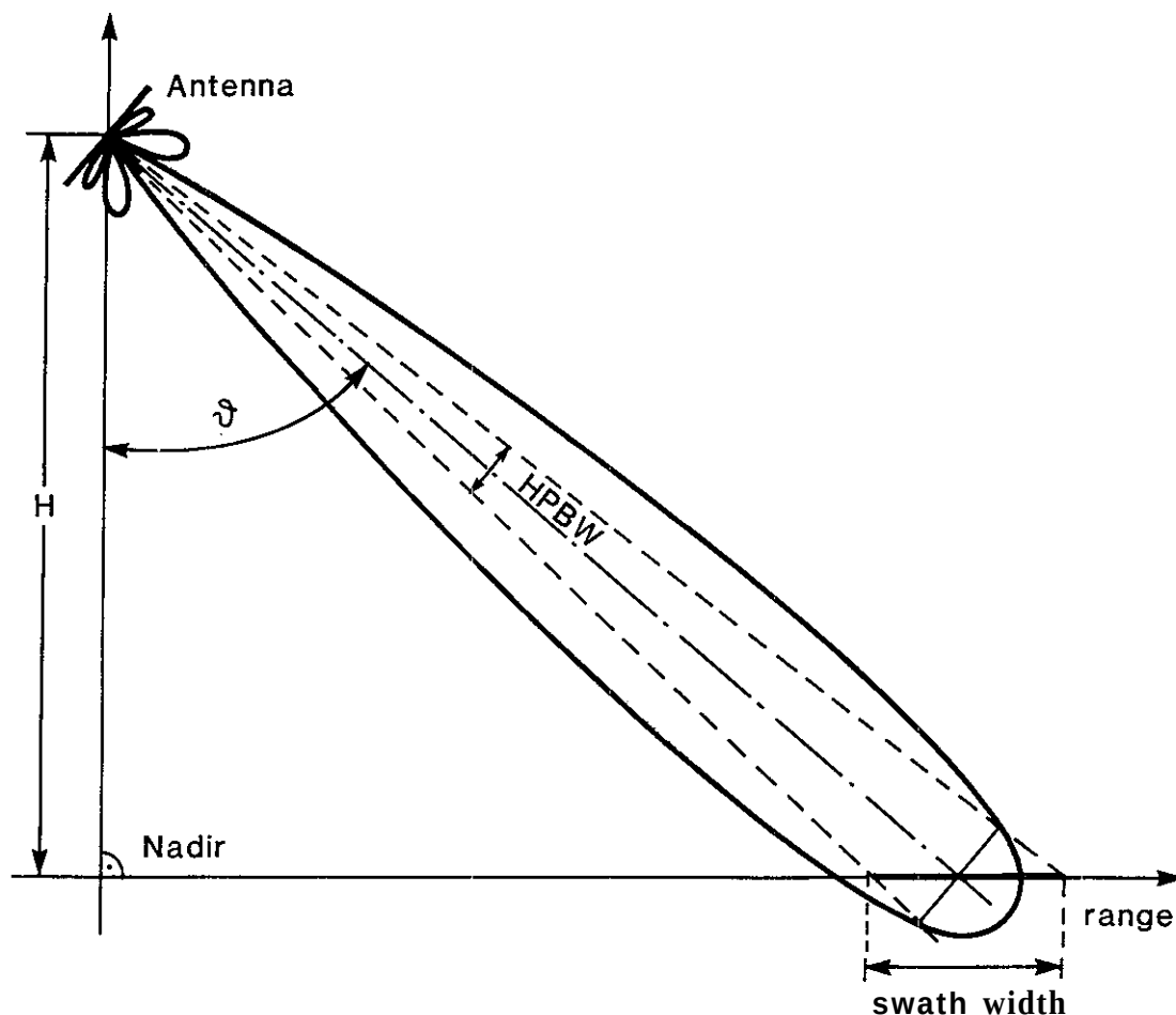
Fig. 1 Illumination geometry; swath width corresponds to HPBW.
