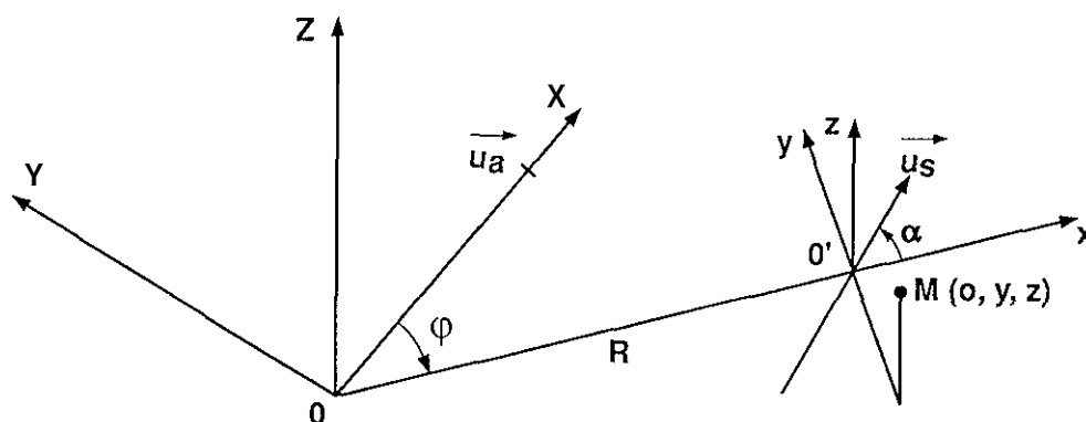
Figure 4: Ship imaging by an airborne radar
