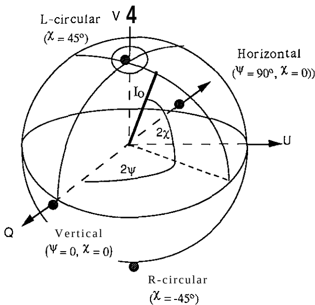
Fig. 2 Poincare' sphere.
