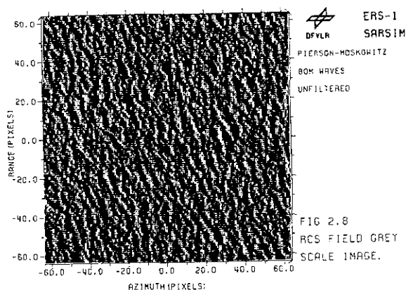
Fig. 20 Simulated ocean wave scene. 4 BIT ADC, MISMATCH 0 DB, 80 M DEER WAVES ANALOGUE ON BOARD RANGE COMPRESSION, NO FILTER
