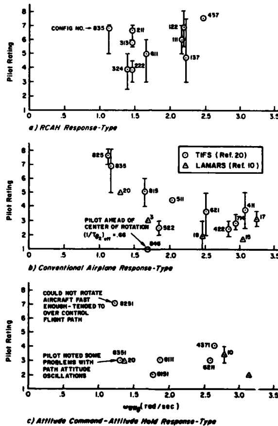
Figure 23. Correlation of w_{\theta} with Pilot Rating for Each Response-Type (Ref. 10 and 20 Data)
