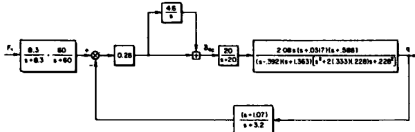
a) Pitch Rate Feedback Block Diagram
