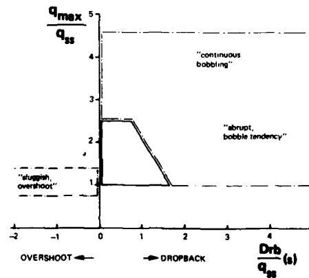
Fig. 4.5 NLR-modified Gibson criterion
