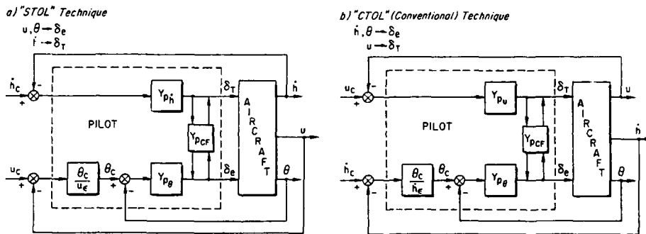
Figure 23. Two Representative Piloting Techniques
