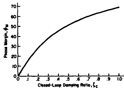
Figure 2. Open- to Closed-Loop Characteristics
