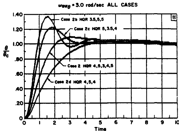
Figure 17. Illustration of Insensitivity of Pilot Rating to Rise-Time if \omega_{w0} = \text{Const.} (Ref. 5)
