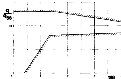
Fig. 4.3 Space Shuttle Orbiter Criterion; pitch-rate time-history envelope.
