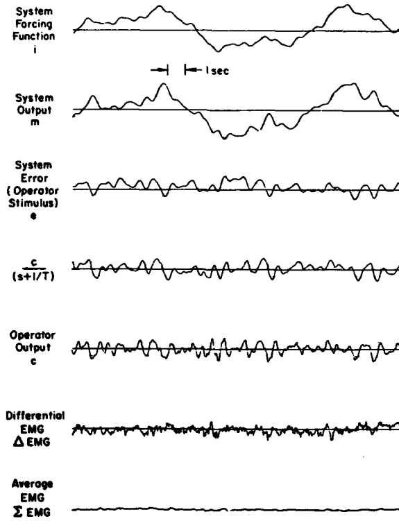
Figure 3. Simple Compensatory System and Operator Responses
