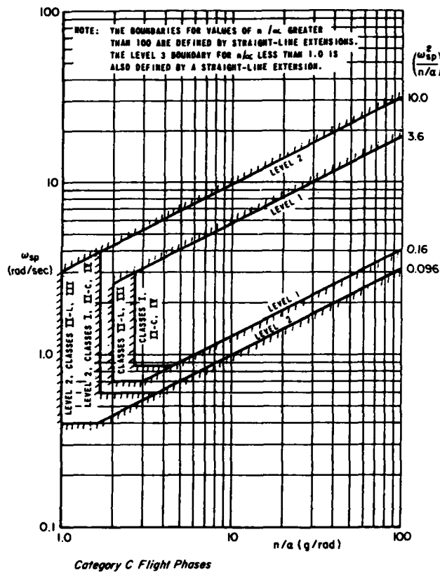
Figure 3. Typical CAP Boundaries From Ref. 3
