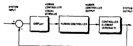
Fig. 3.2 Compensatory control structure for visual inputs.
