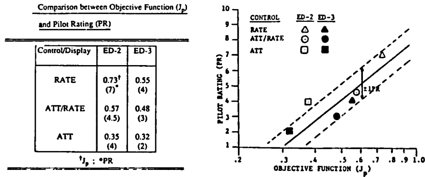
Figure 13. Correlation between Pilot Rating and Performance Index for Various Control/Display Combinations. [33]
