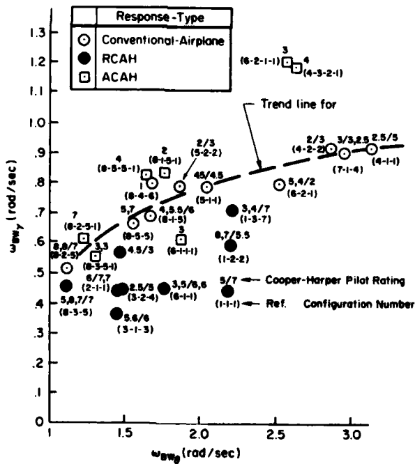
Figure 25. Pilot Rating Correlations with (1/T_{\theta_2}) and \omega_{wg} Ref. 20 Flared Landing Experiment
