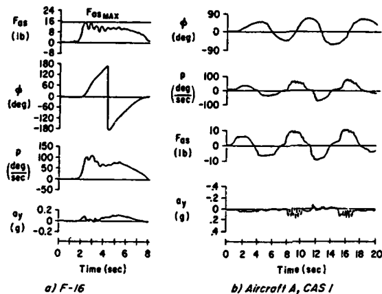
Figure 10. Roll Ratchet During Banking Maneuver
