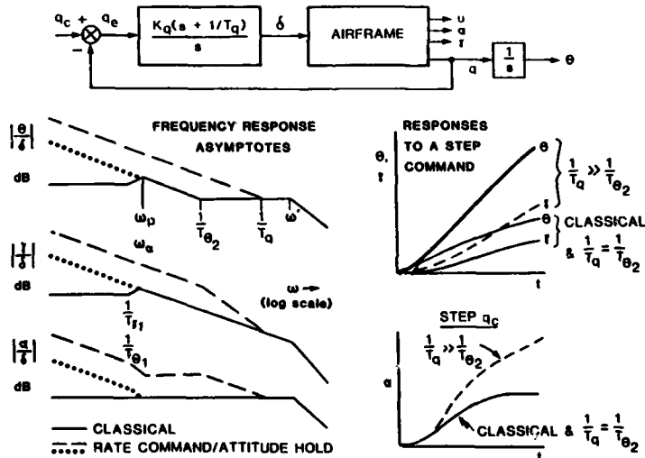
Figure 11. Frequency and Time Response Comparison
