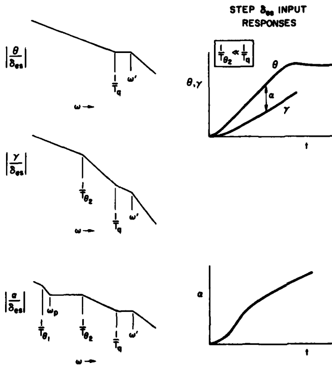
Figure 21. Generic Characteristics of Rate Command/Attitude Hold Response-Type (RCAH) ( q + f_{qd} \rightarrow \delta_e )
