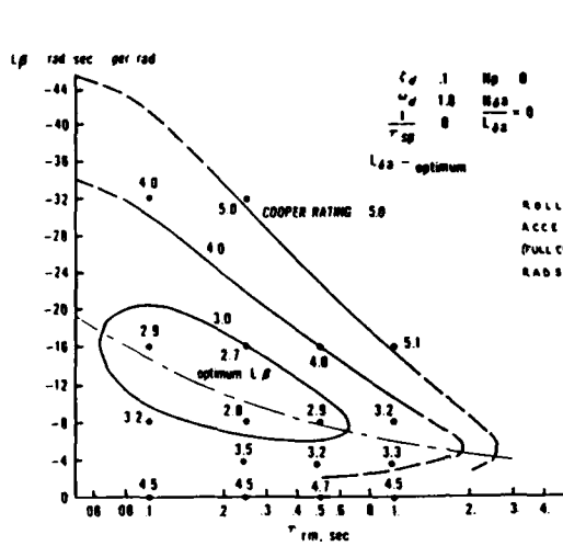
Figure 17 Lateral/Directional H.Q.
