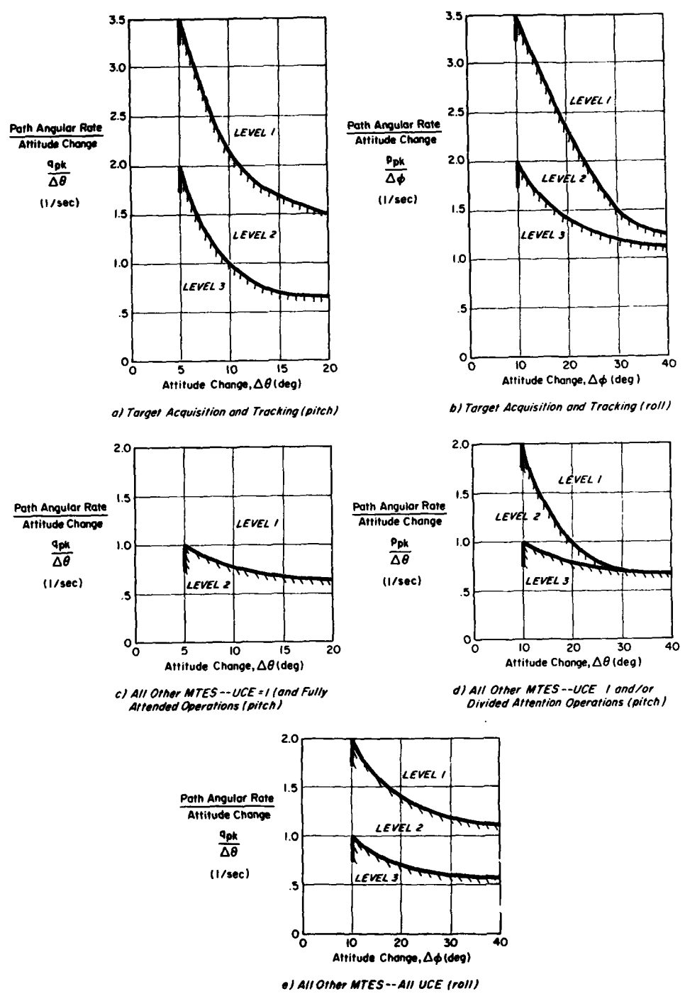
Figure 11. Requirements for Moderate-Amplitude Pitch (Roll) Attitude Changes -- Hover and Low Speed (from Ref. 6)
