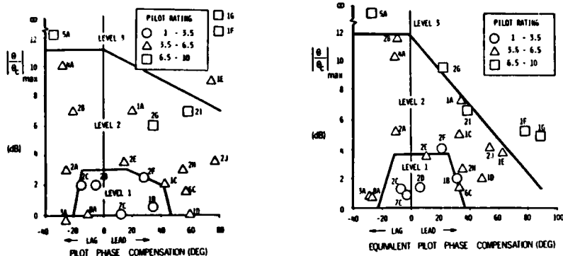
Figure 5. Reproduction of Neal-Smith Results using OCM. [18]
