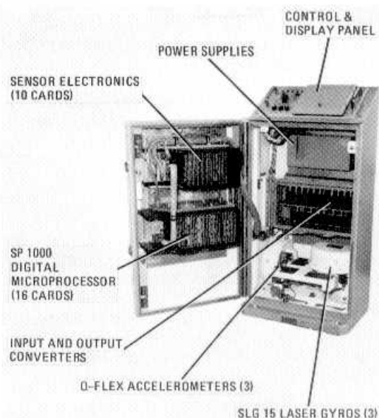
Figure 15. MK-16 MOD-11 Stable Element
