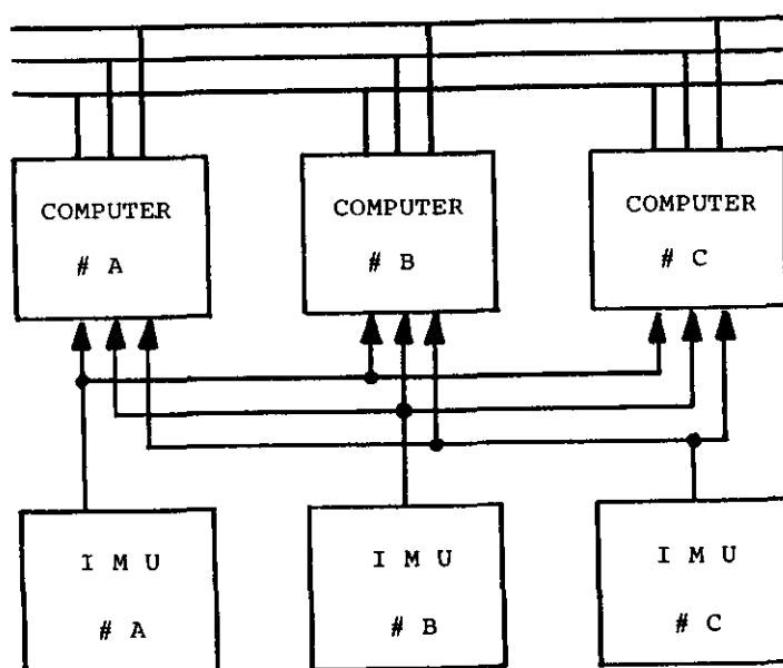
Figure 24. Strapdown sensor data-bus configuration for accommodating untolerable phase lag.
