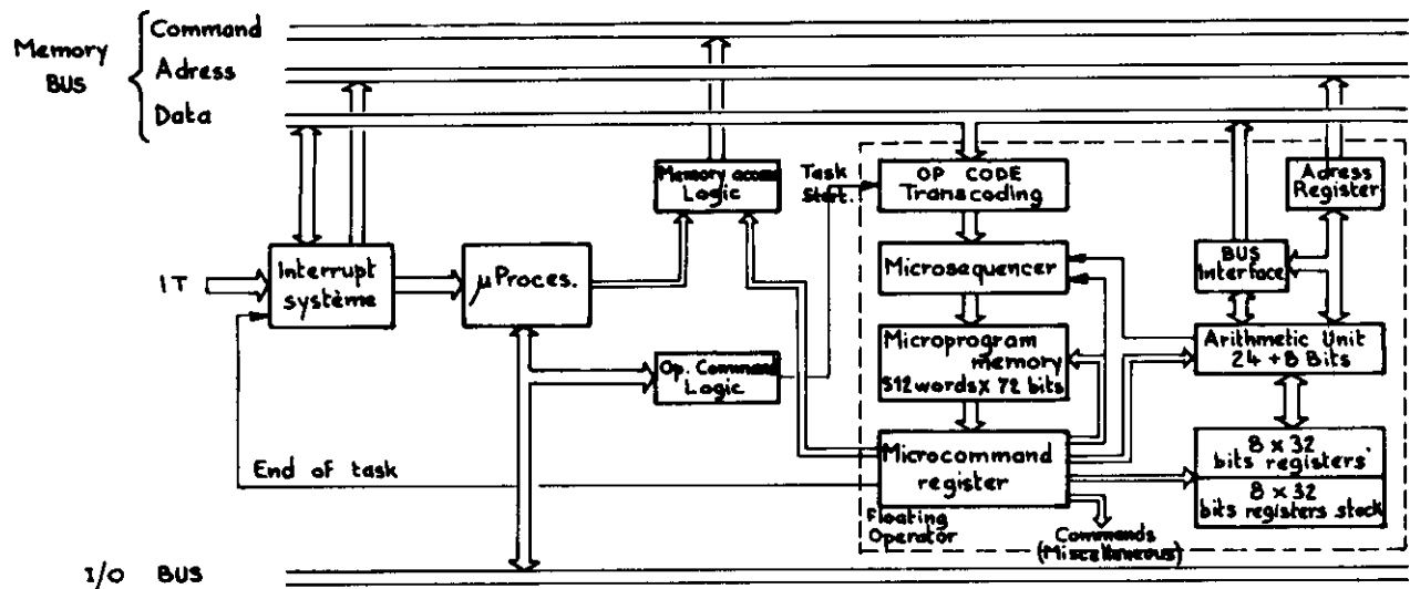
Figure 19 - SYCOMORE Functional diagram
