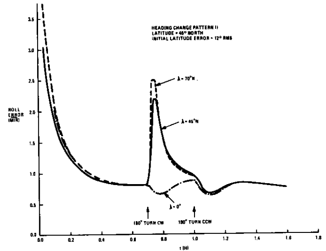
Figure 24. Effect of Operating Latitude on Roll Error
