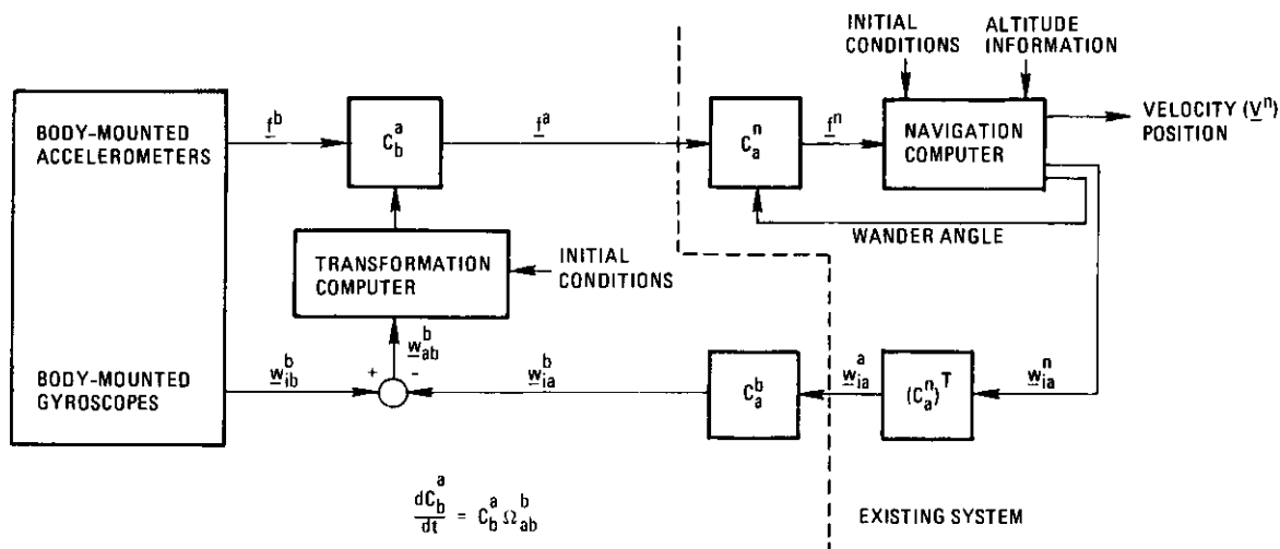
Figure 6. Strapdown wander-azimuth mechanization.
