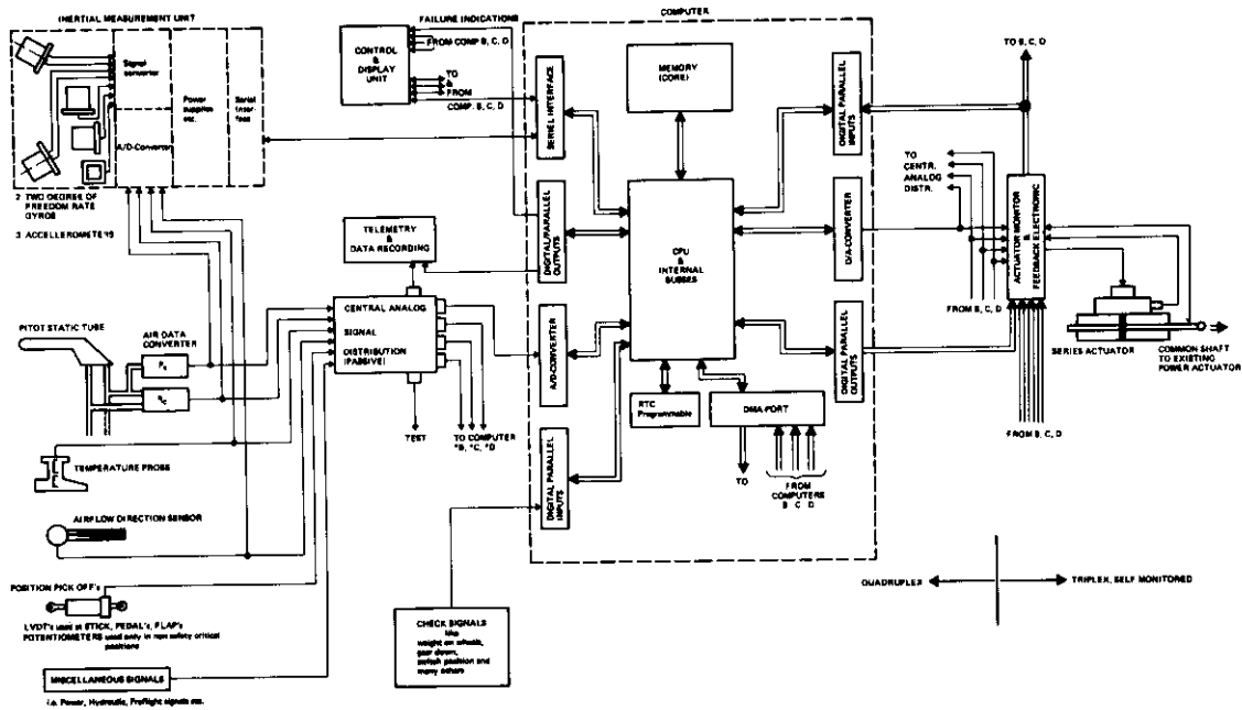
Figure 5. CCV-F104G guidance and control system (one channel).
