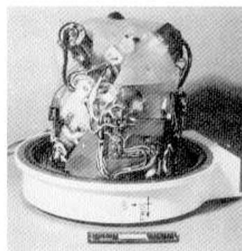
Figure 8. SLIC-15 Sensor Assembly
