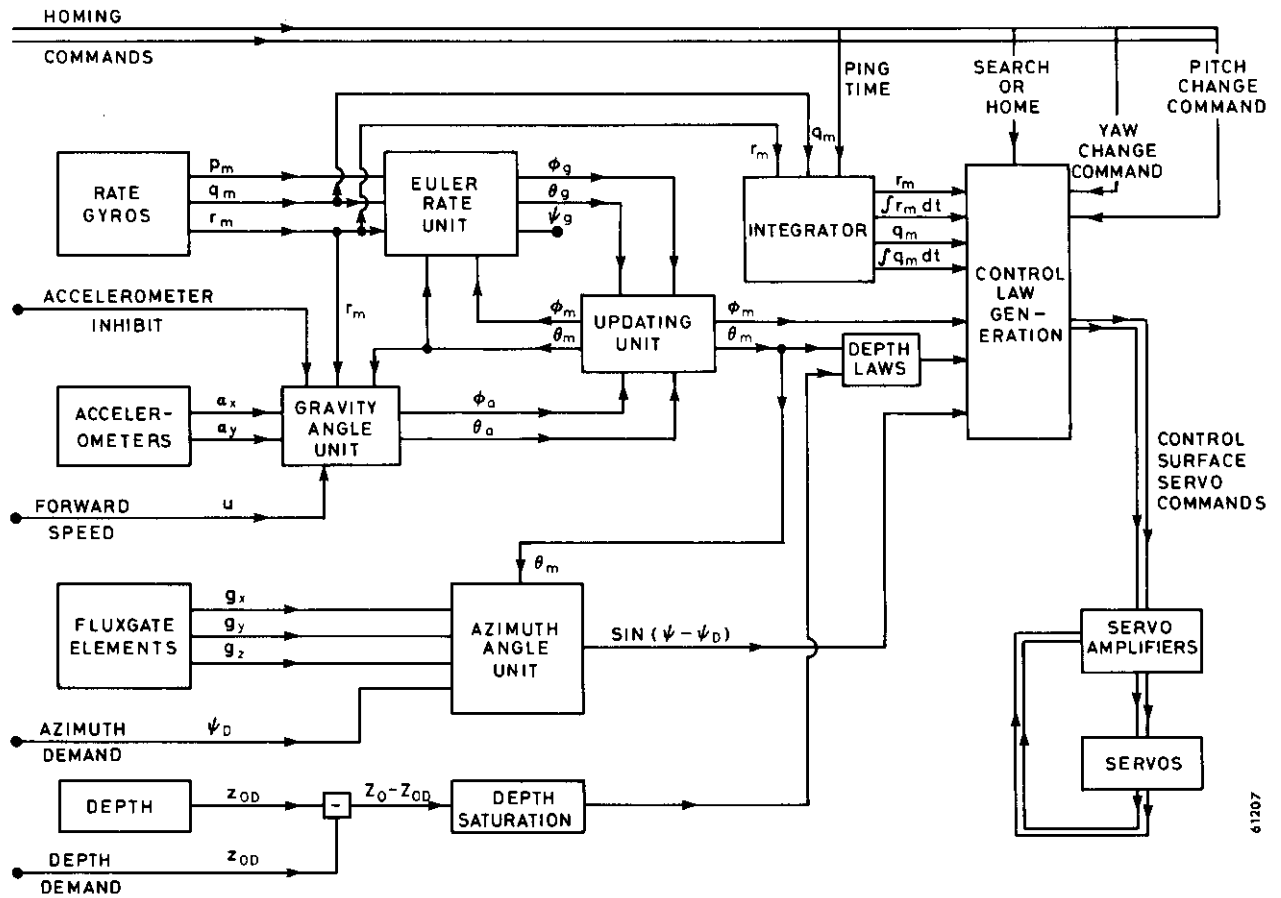
Fig.5 Block Diagram of Attitude Sensor
