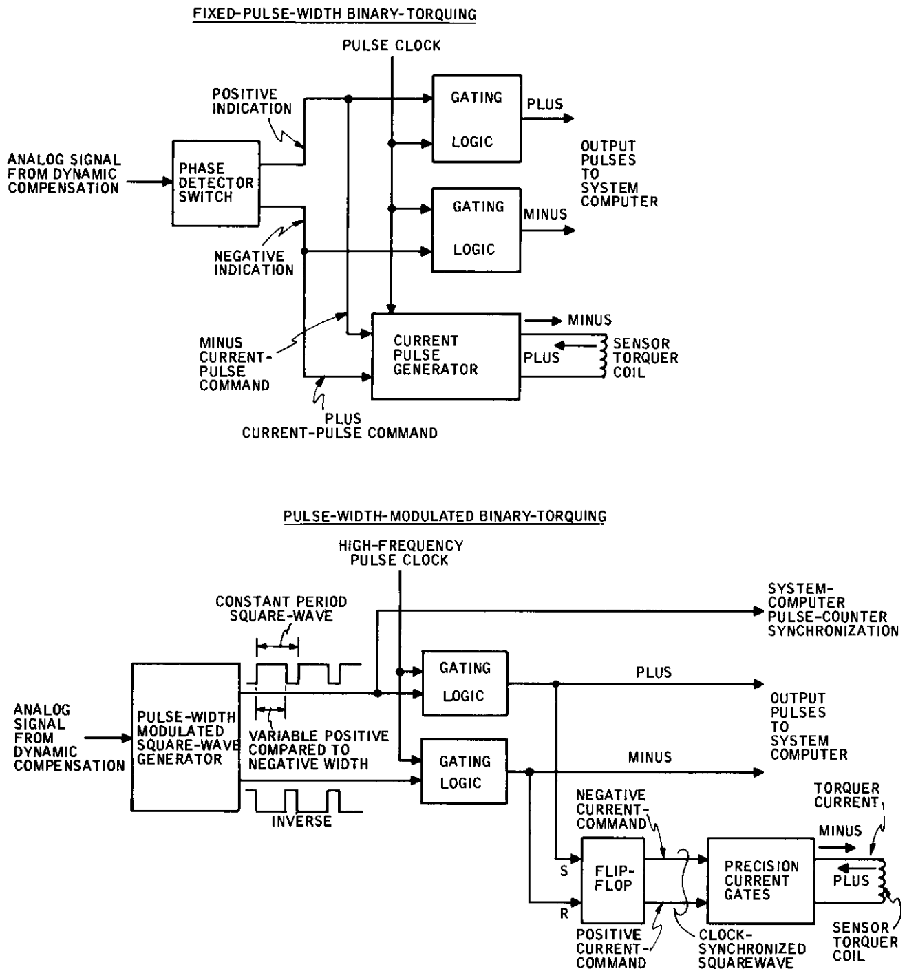
Figure 6. Binary torquer-current command-logic concepts.
