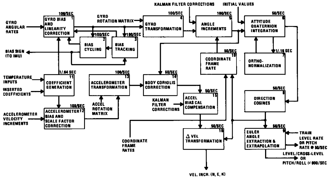
Figure 20. Strapdown Computation Function Flow Diagram
