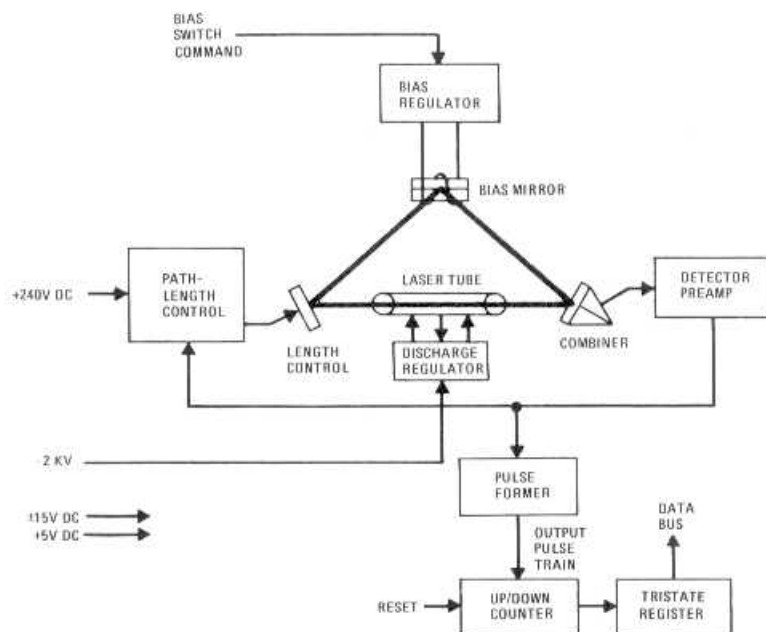
Figure 18. Laser Gyro Electronics Schematic Diagram
