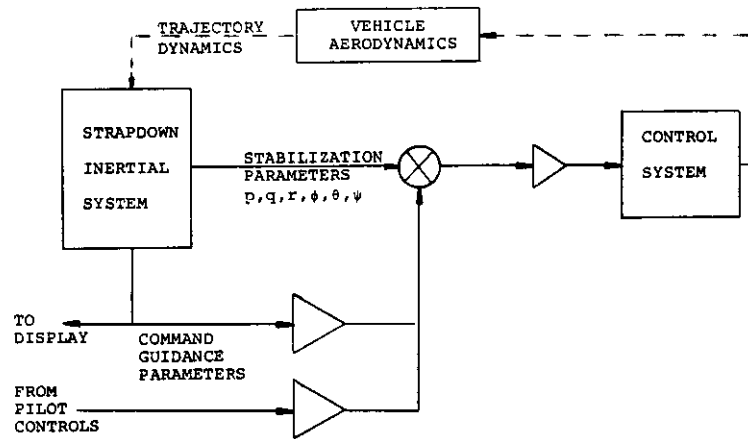
Figure 12. Systems operations block diagram
