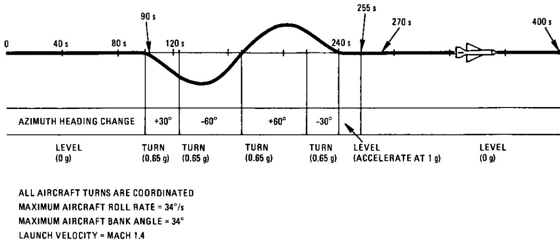
Figure 7. Calibration and alignment maneuver (viewed from above).
