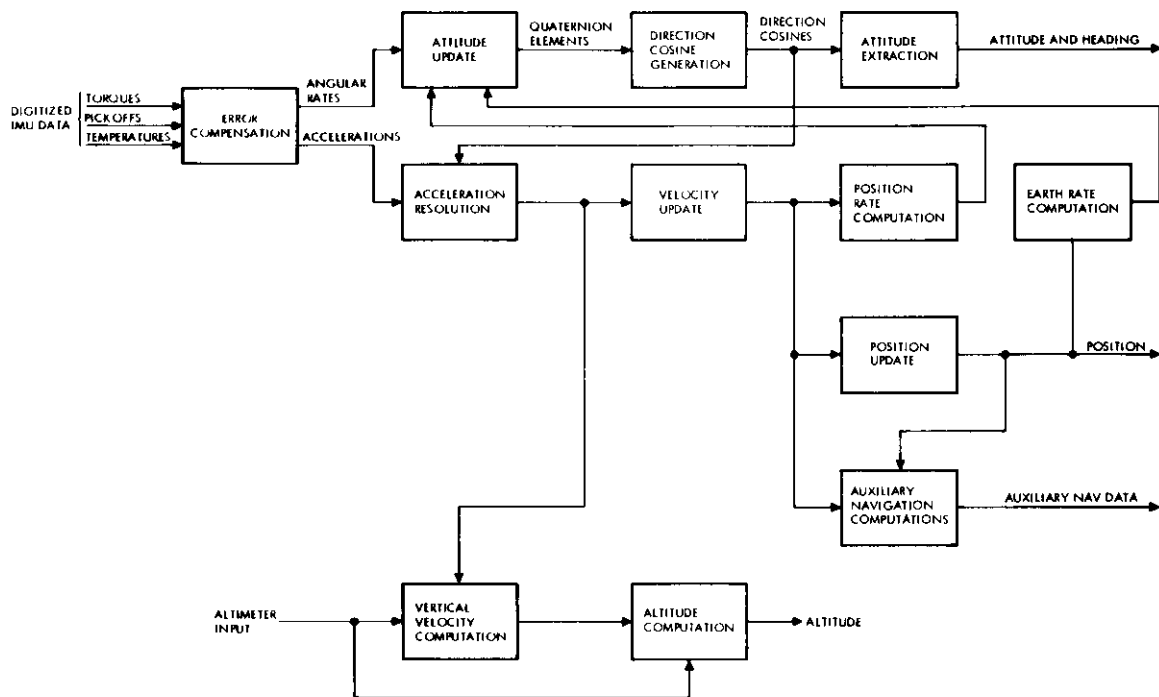
Figure 11. Computational flow diagram.
