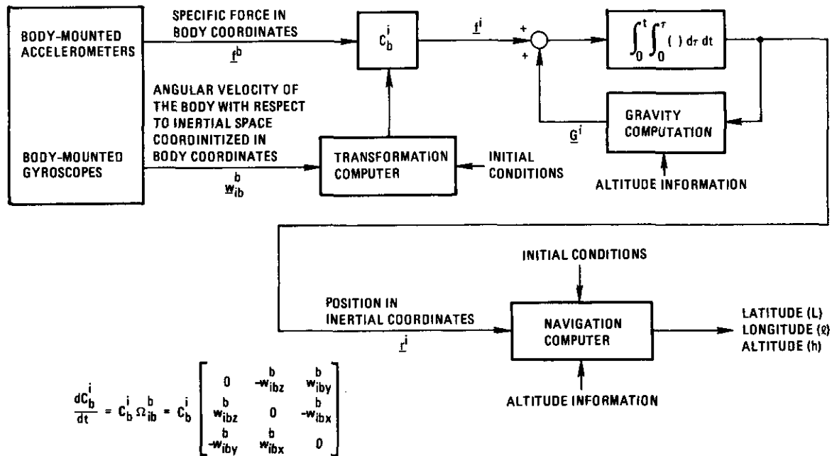
Figure 2. Strapdown system computing in inertial coordinates.
