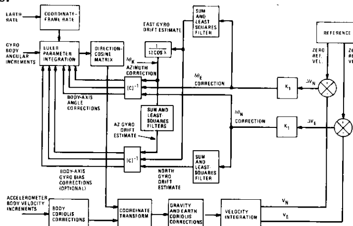
Figure 27. Leveling, Gyrocompassing Ground-Align Configuration.
