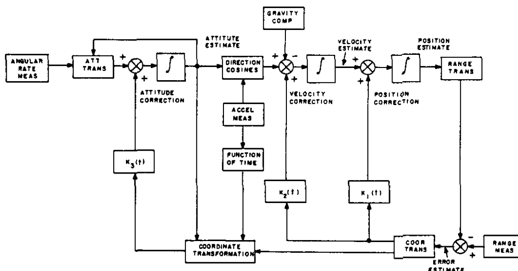
Figure 4. Least squares integration filter.
