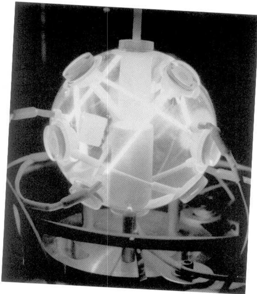
Figure 16. Honeywell GG1330 laser triad rate gyro.
