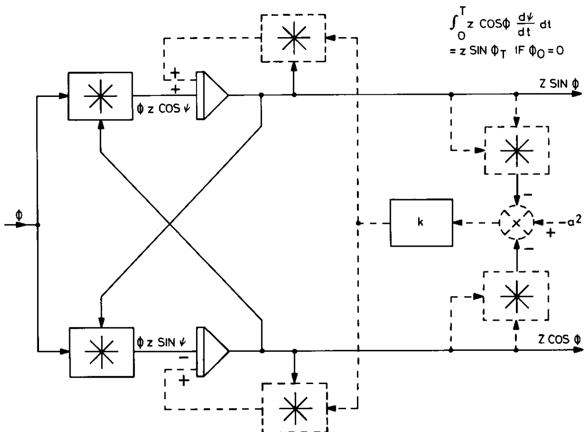
Fig.8 Integrating Sin Cos Generator
