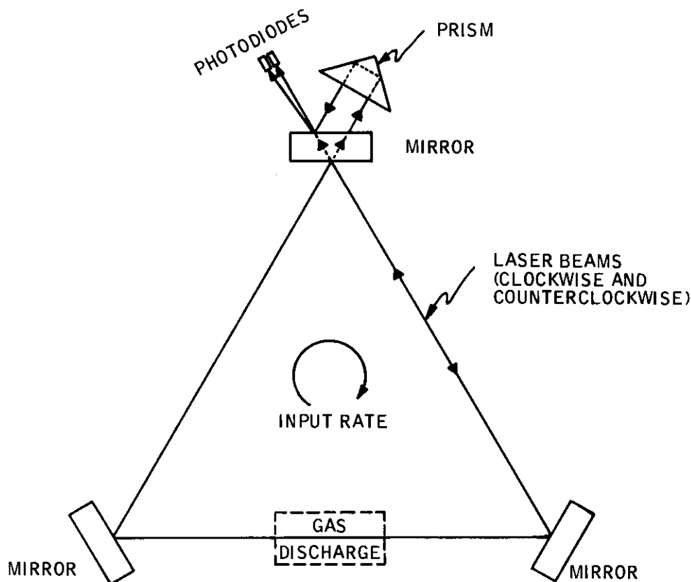
Figure 12. Laser-gyro operating elements.
