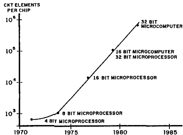
Figure 9. Projected advances in processor technology.
