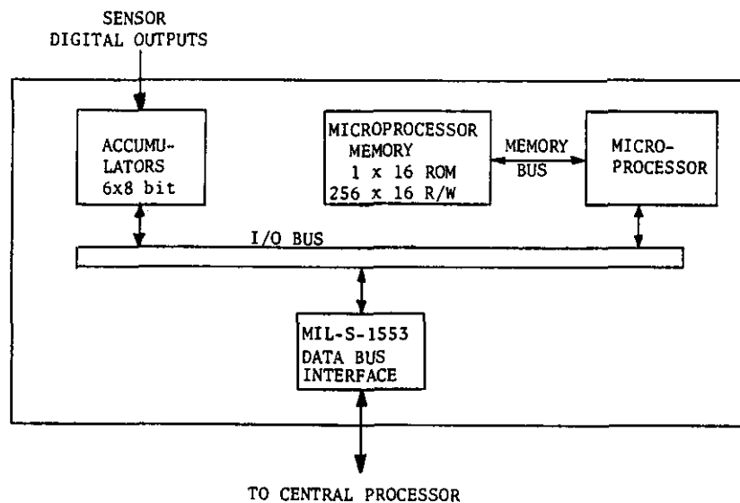
Figure 7. Strapdown processor block diagram.
