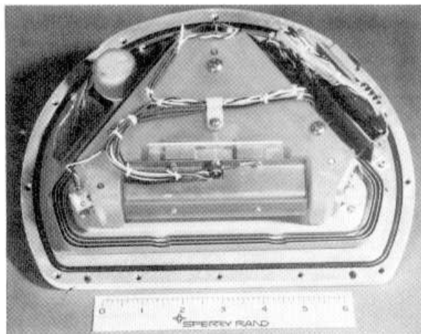
Figure 17. Stable Element Laser Gyro
