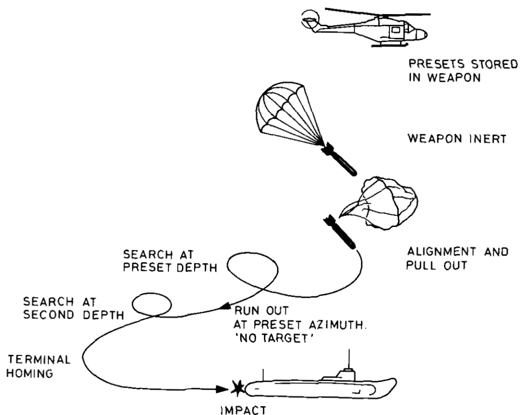
Fig.2 Possible Weapon Trajectory
