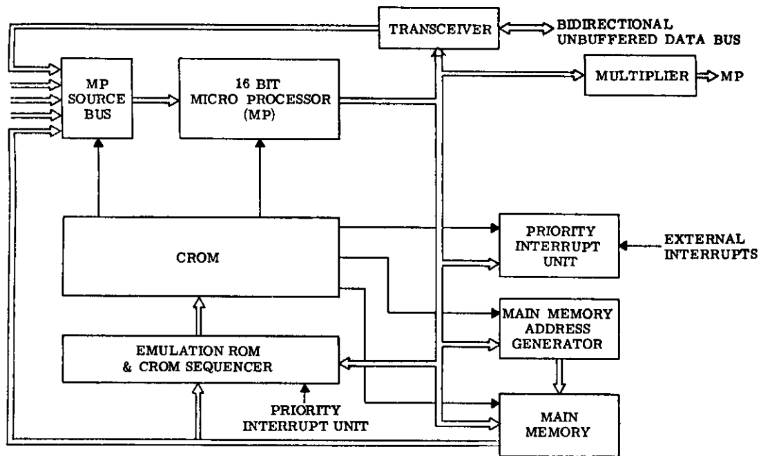
Figure 19. DMP Data and Control
