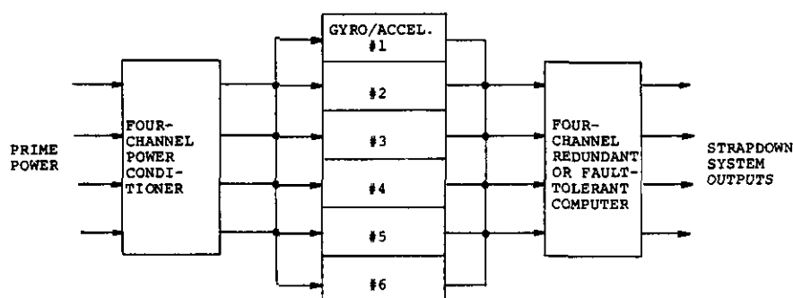
Figure 11. Full fail-op/fail-op/fail-safe strapdown system configuration.
