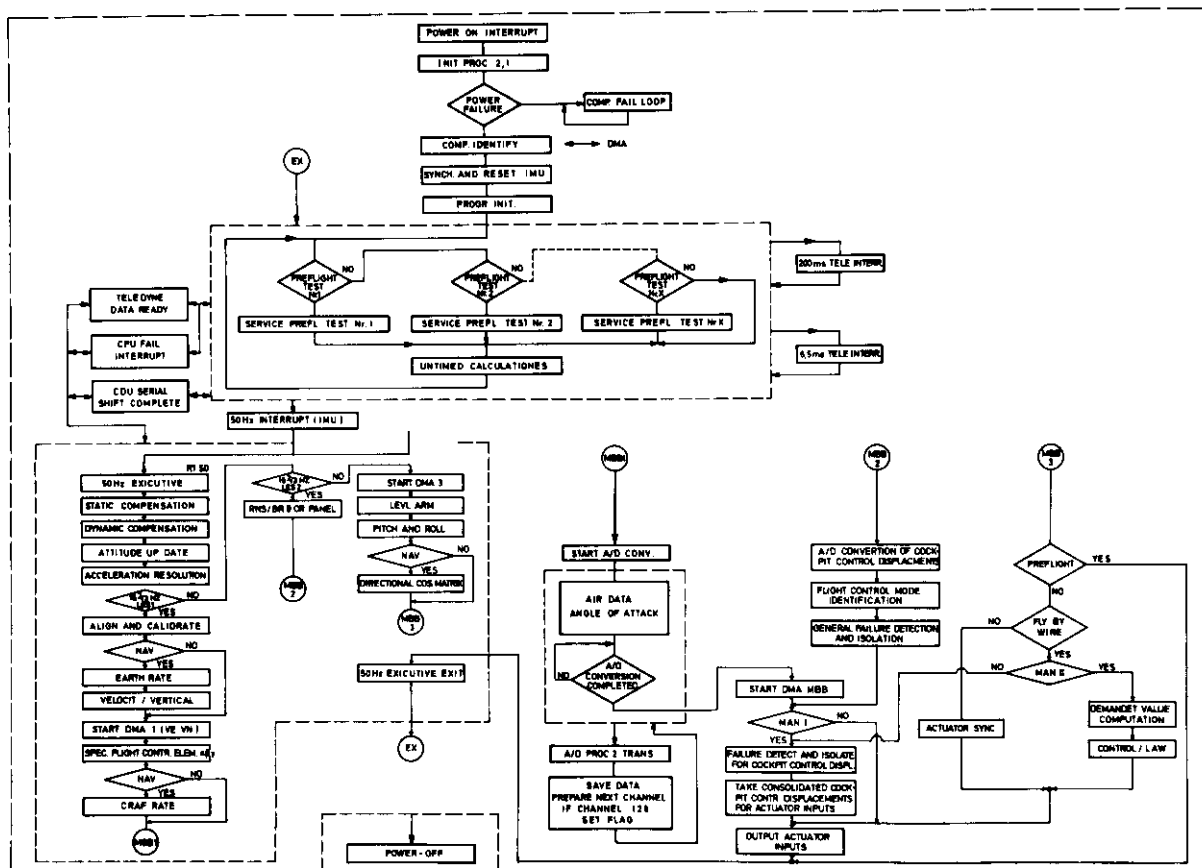
Figure 12. CCV program flow.
