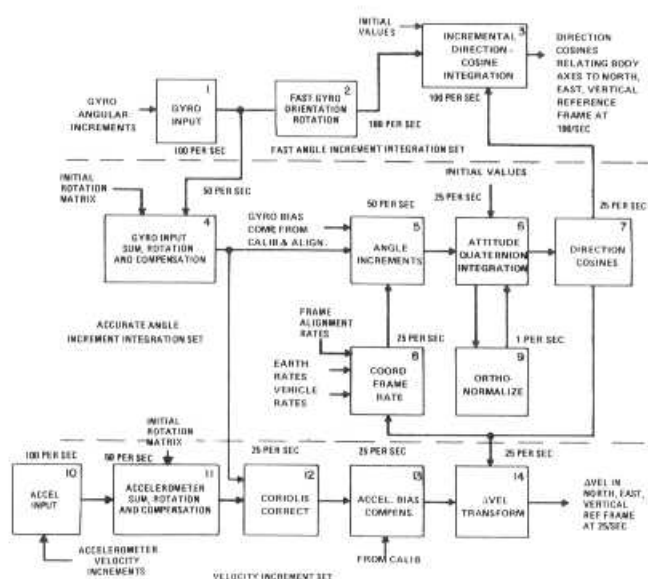
Figure 10. Strapdown Computational Flow Diagram
