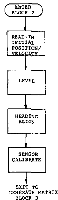
Figure 3. Functional flow diagram, initialization algorithms.
