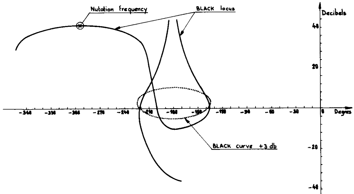
Figure 14 — Sampled gyrometric loop analysis [BLACK locus]
