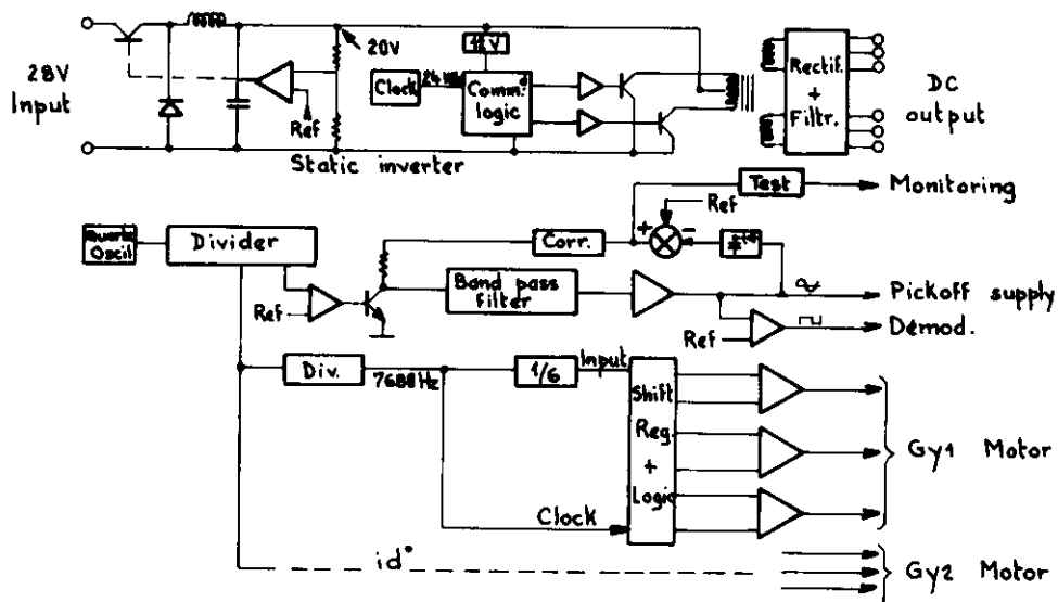
Figure 12 - General functions
