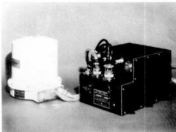
Figure 7. SLIC-15 IMU
