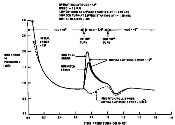
Figure 22. At-Sea Performance-Effects of Initial Latitude Errors
