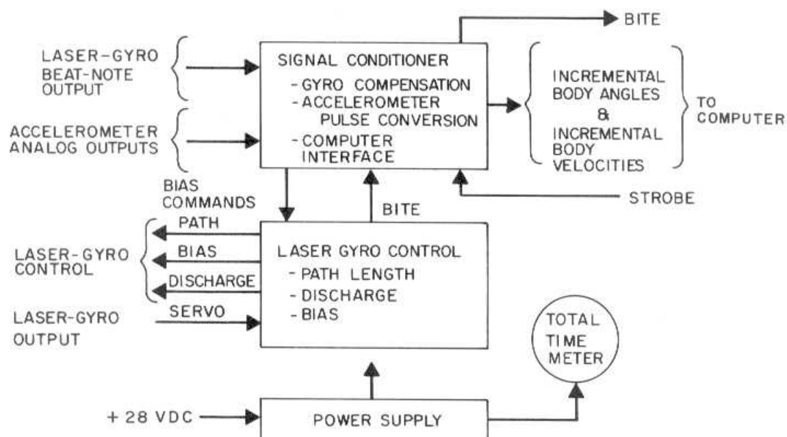
Figure 9. Electronics Assembly Block Diagram
