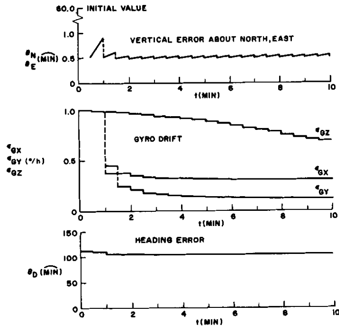
Figure 5. Ground Align Mode Analysis Results, Magnetic Flux Valve Reference
