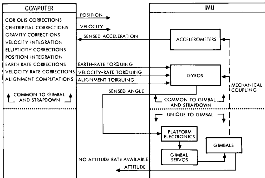
Figure 1. Computer-IMU interface: gimballed system.
