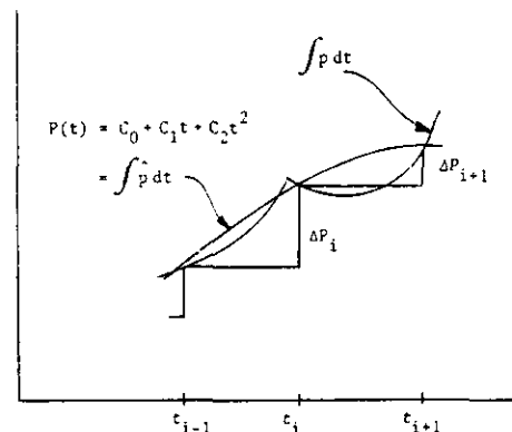
Figure 13. Second-order fit rate extraction.
