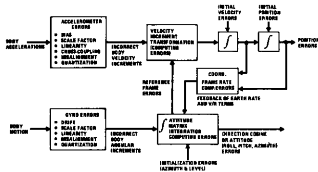
Figure 11. Simplified Error Flow Diagram For Strapdown Inertial System
