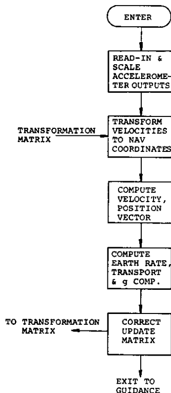
Figure 9. Functional flow diagram, navigation algorithms
