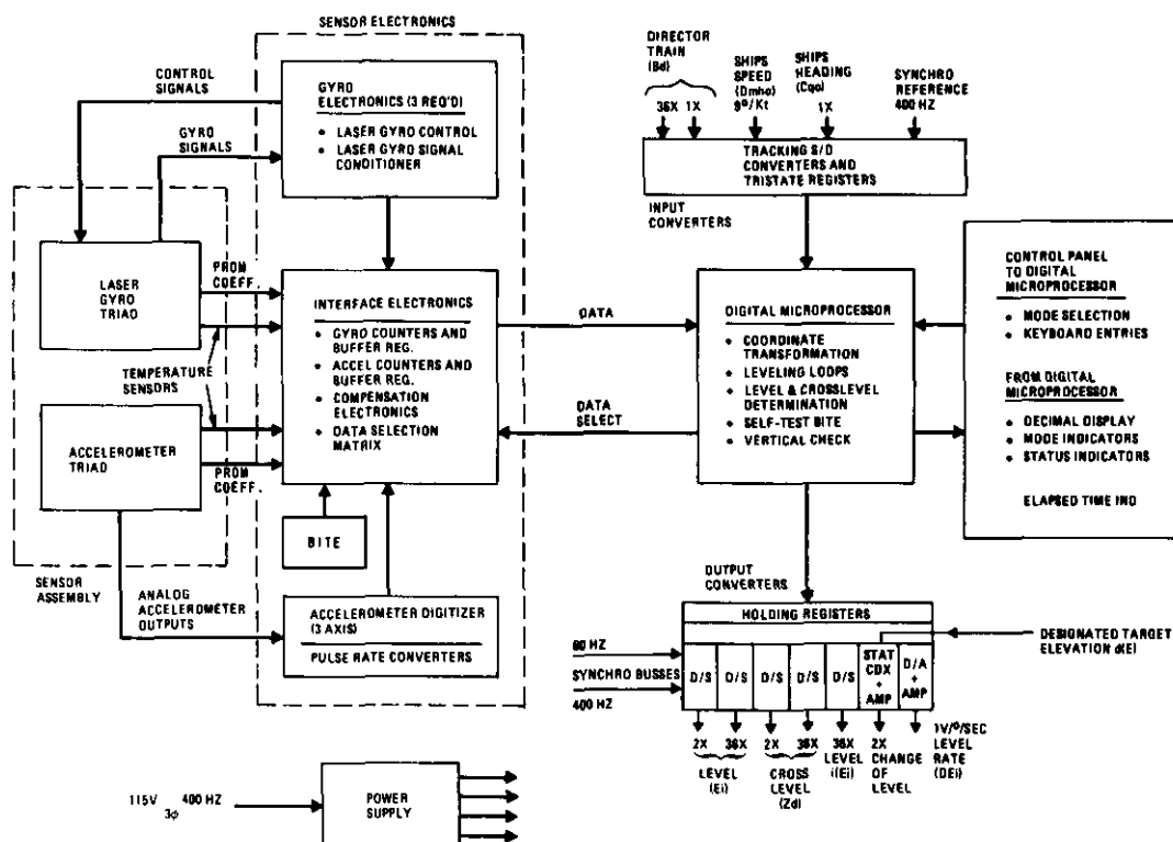
Figure 13. Stable Element Functional Block Diagram
