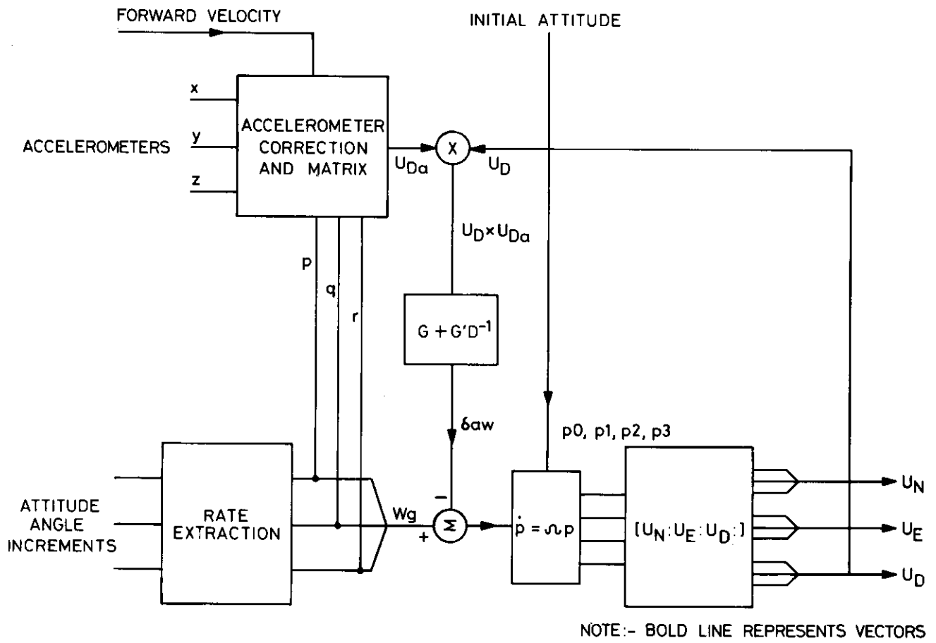
Fig.9 System Block Diagram
