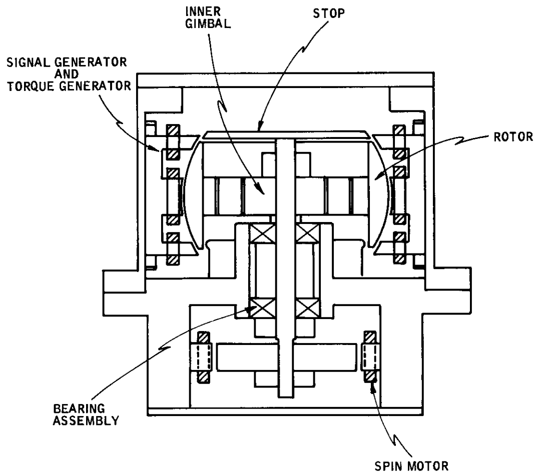
Figure 7. Typical tuned-rotor gyro configuration.
