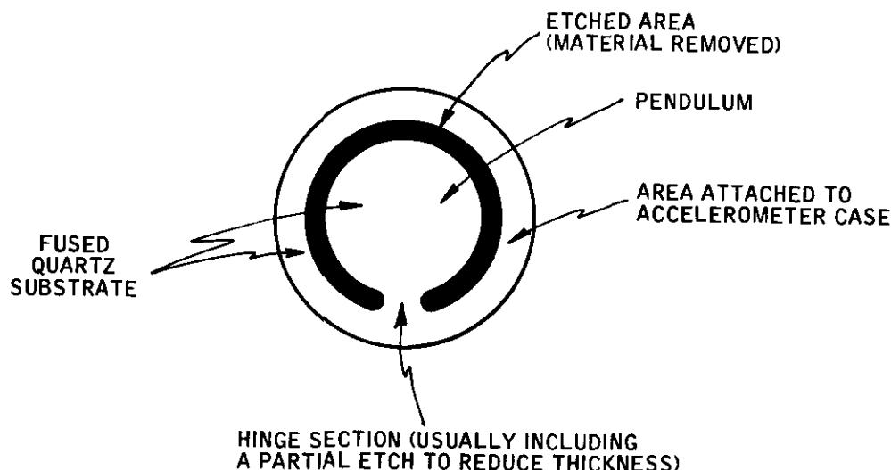
Figure 19. Quartz-flexure pendulum/hinge concept.
