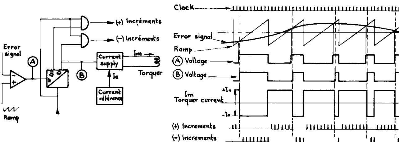
Figure 13 - PWM Rebalance loop
