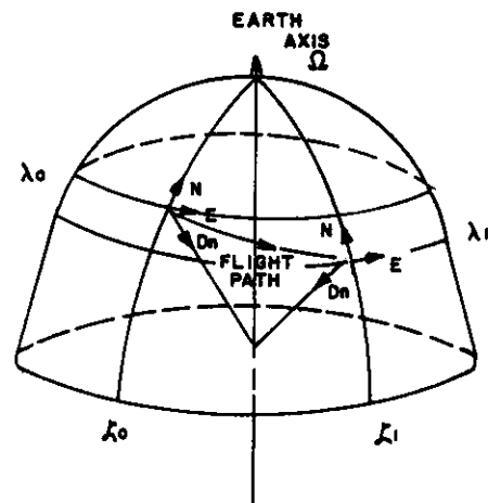
Figure 10. Local-level coordinate system geometry
