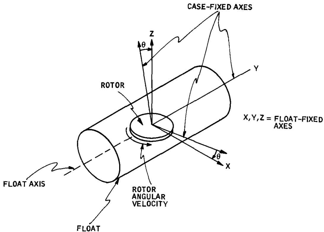
Figure 2. Gyro gimbal and case axes.
