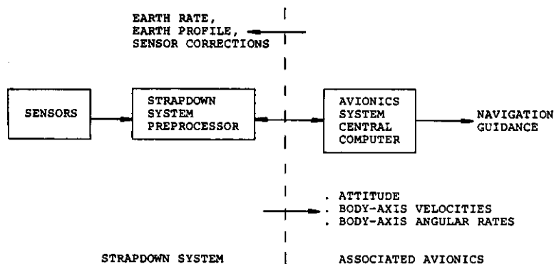
Figure 3. Typical strapdown system software partitioning.
