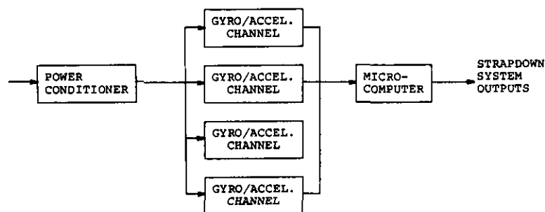
Figure 10. Minimum fail-safe strapdown system configuration.
