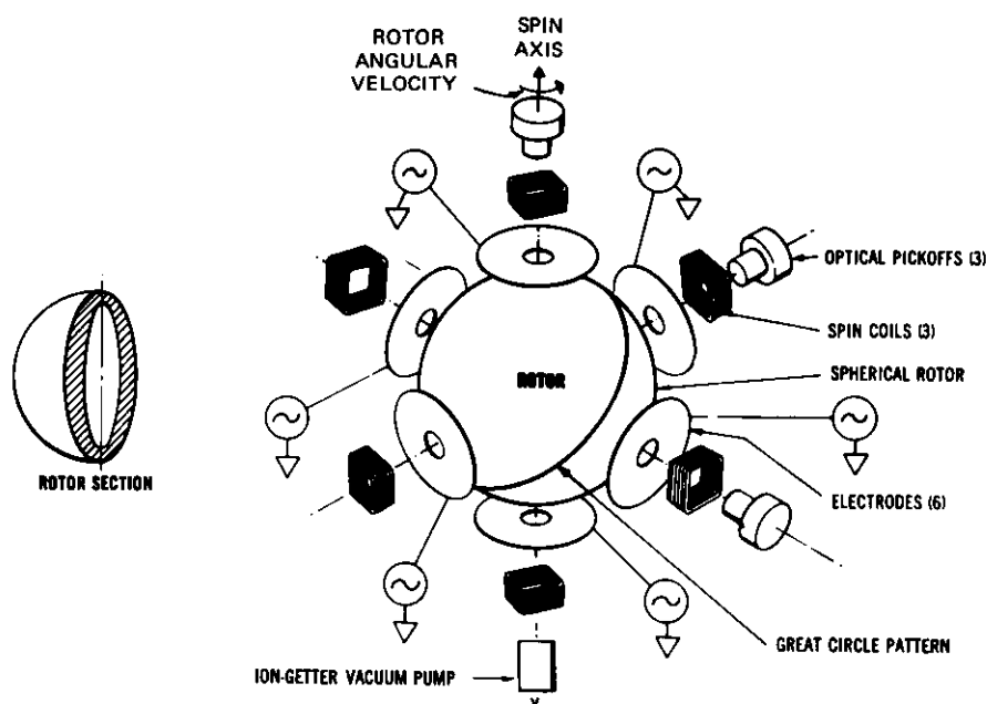
Figure 11. Electrostatic-gyro configuration.
