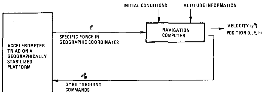
Figure 3. Platform geographic local-vertical mechanization.
