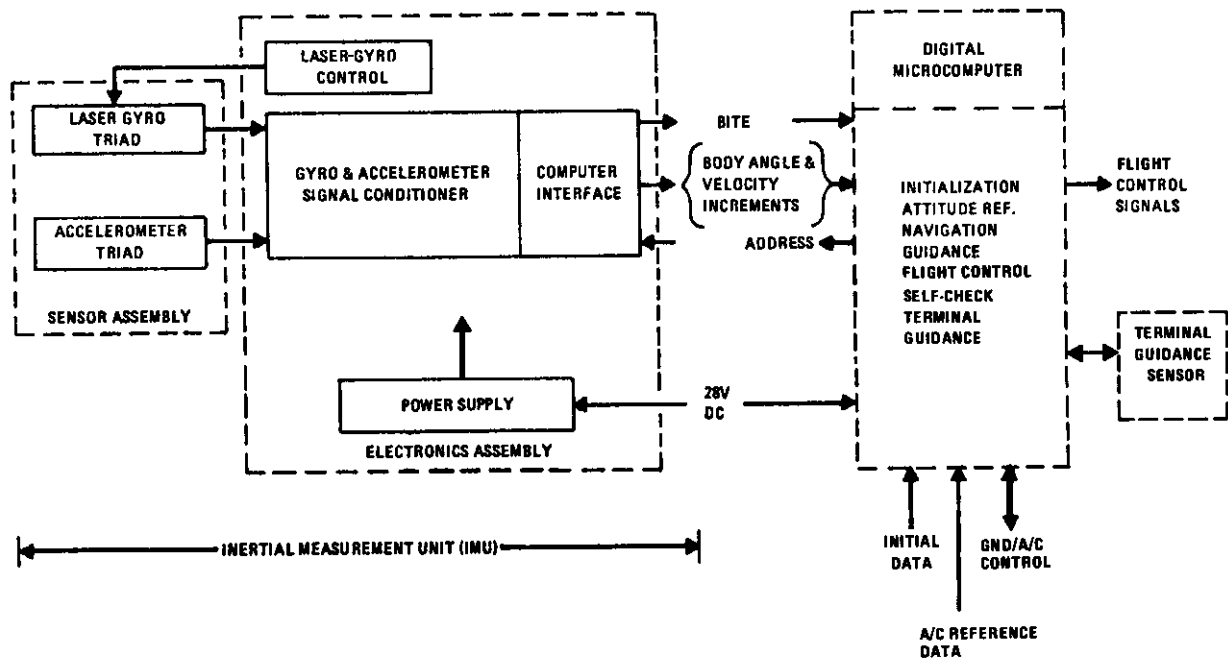
Figure 3. Laser Gyro Strapdown System Functional Block Diagram
