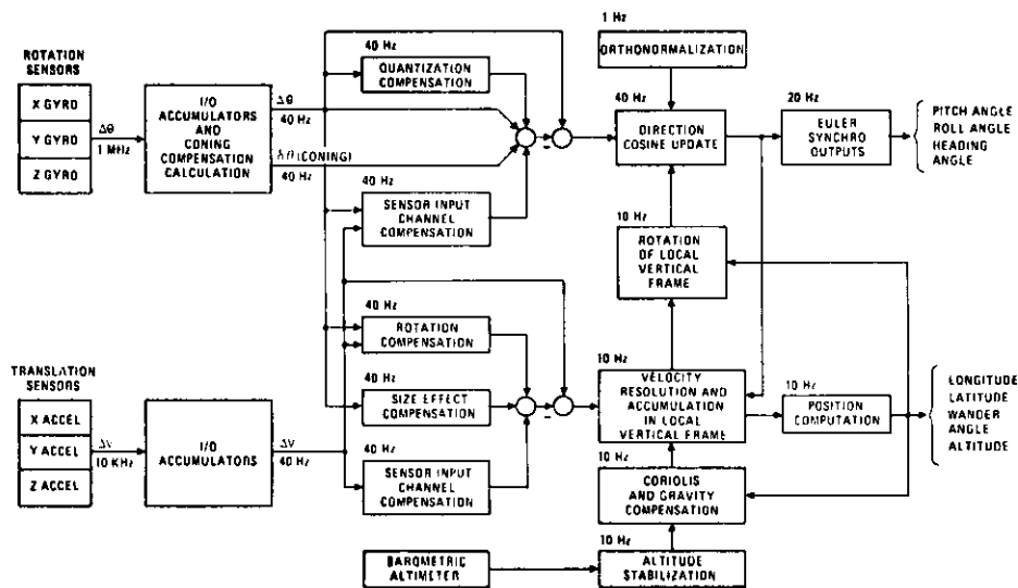
Figure 30. LINS Software Flow Diagram
