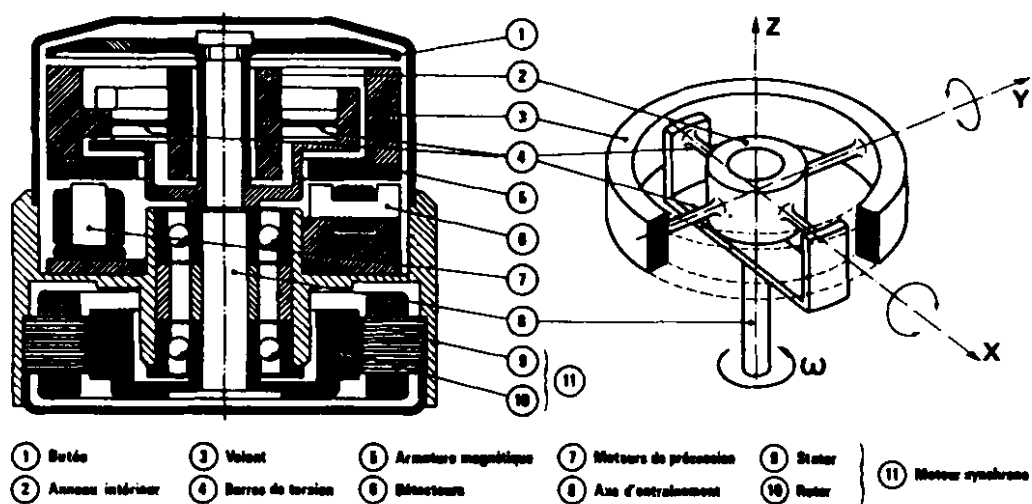
Figure 1 - Gyroscope GAM1
