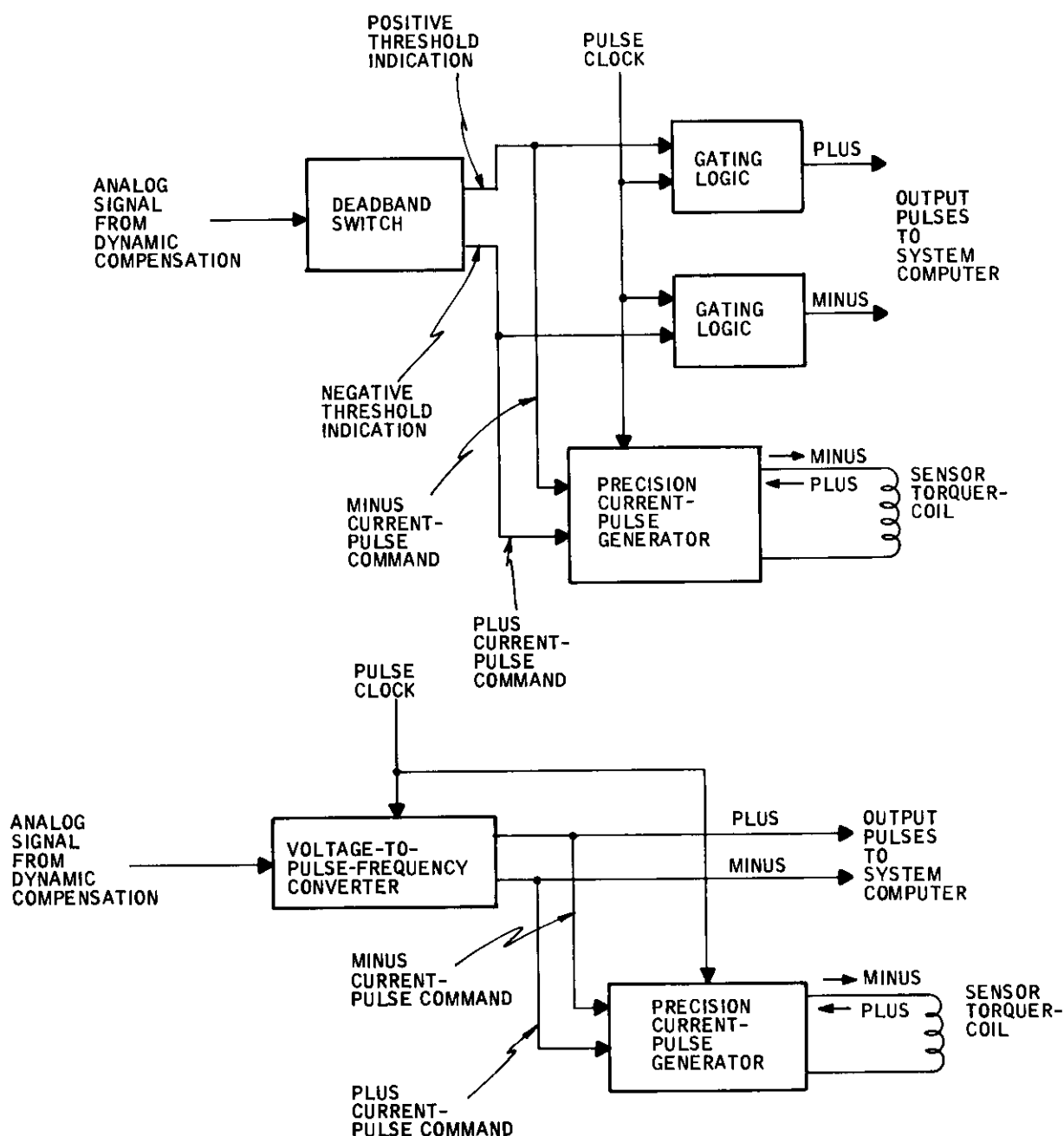
Figure 5. Pulse-on-demand torquer-current command-logic concepts.
