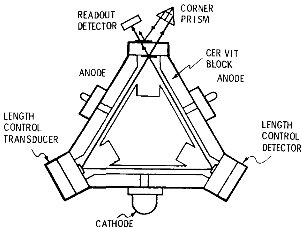
Figure 13. Laser-gyro block assembly.
