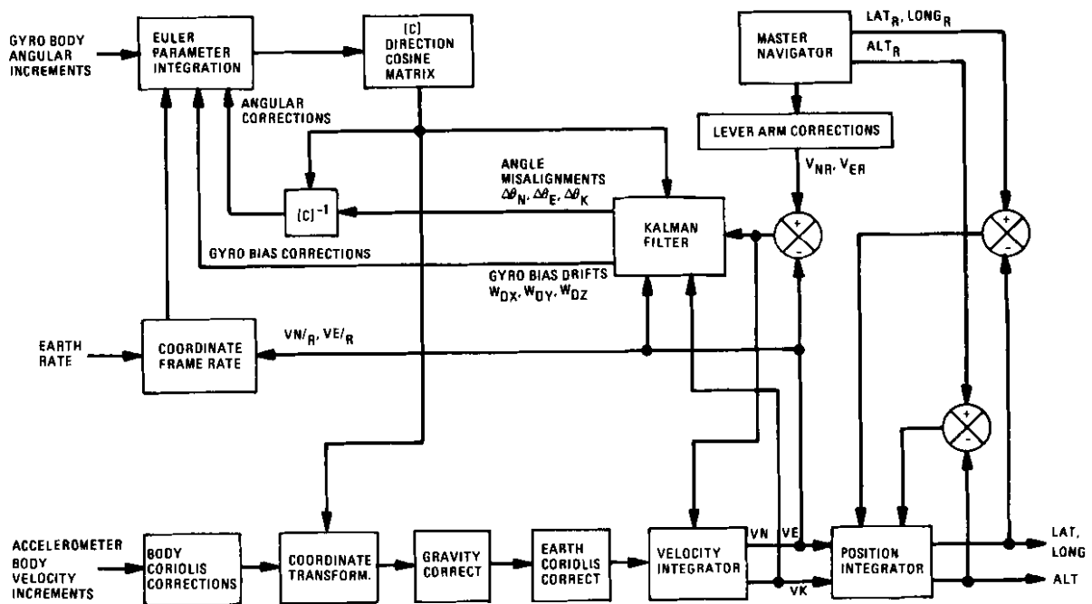
Figure 6. Simplified Kalman Filter Align/Calibrate
