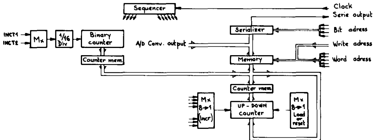
Figure 17 - Counting and serializing logic
