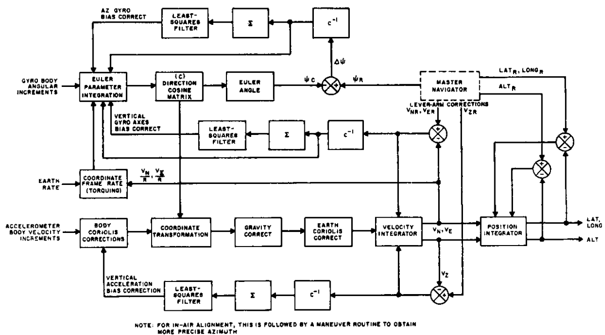
Figure 4. Leveling, Alignment, and Calibration
