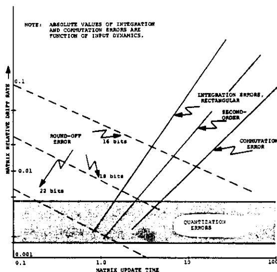
Figure 7. Relative error effects.
