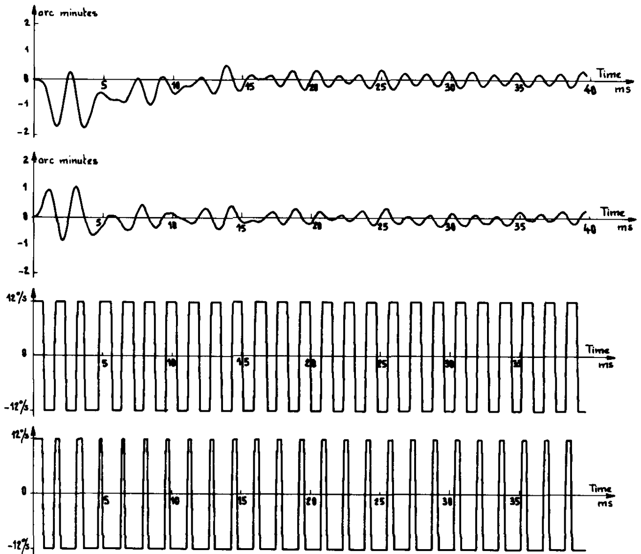
Figure 23 - GAM3 gyrometer simulation - Response to an angular rate step input
