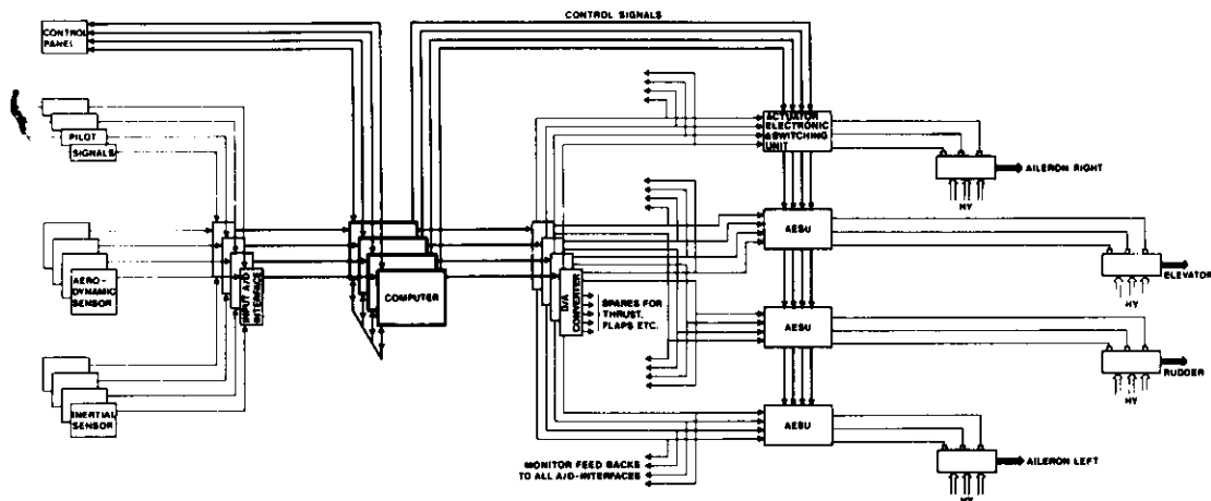
Figure 6. CCV-F104G guidance and control system.
