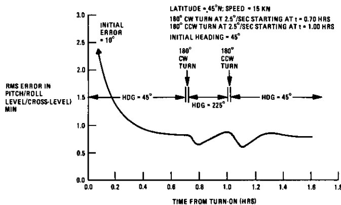
Figure 21. RMS Pitch/Roll Error for Laser Gyro Stable Element
