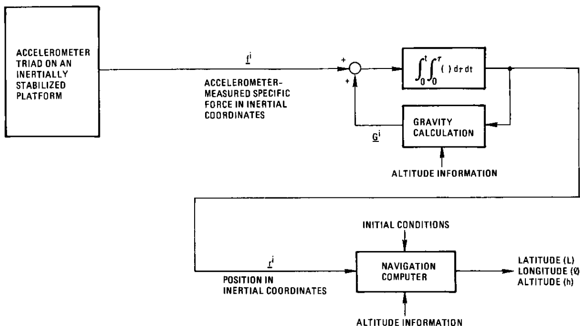
Figure 1. Platform space-stable inertial mechanization.
