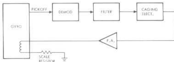
Figure 8. Simplified 1-axis caging loop
