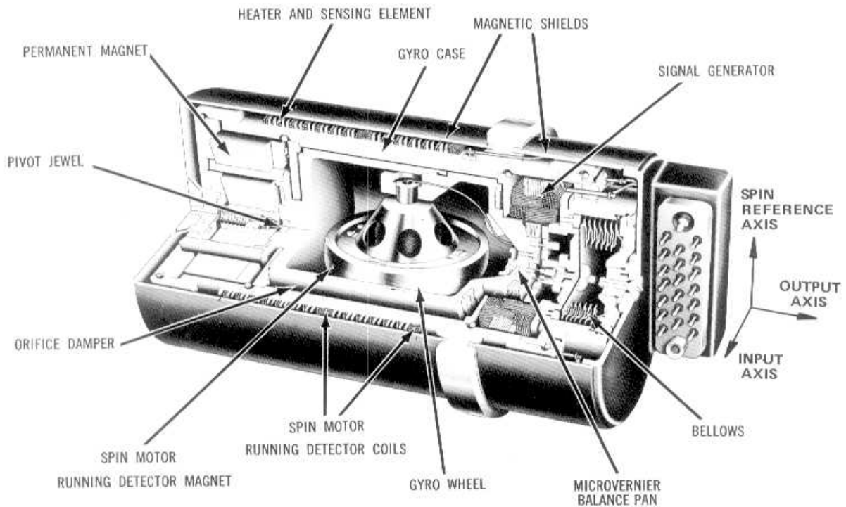
Figure 1. Honeywell GG87 single-degree-of-freedom floated-rate-integrating gyro.
