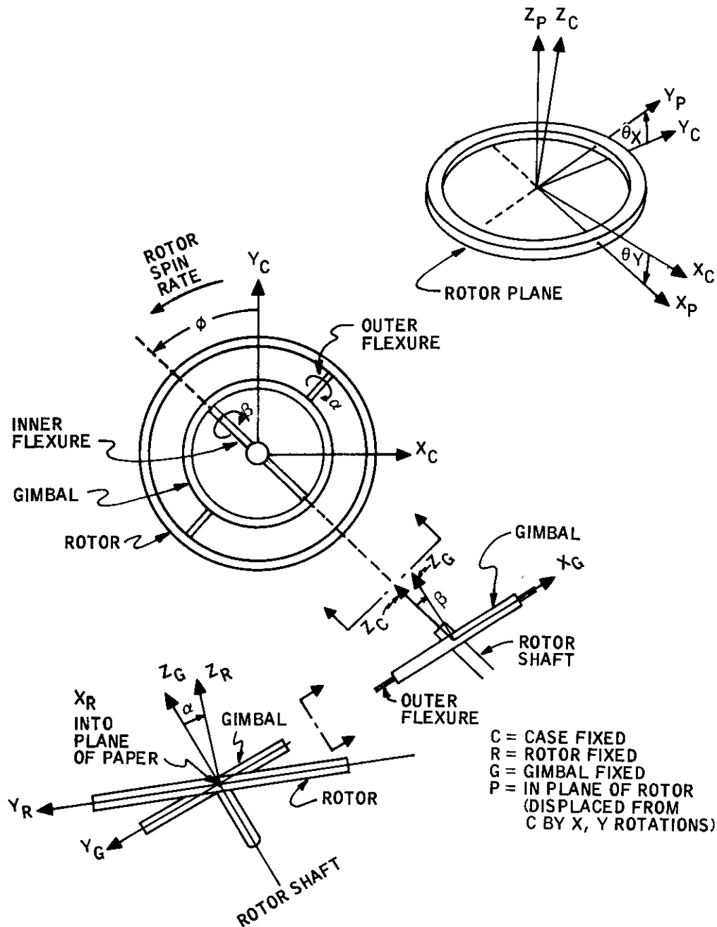
Figure 9. Tuned-rotor-gyro coordinate-frame geometry.
