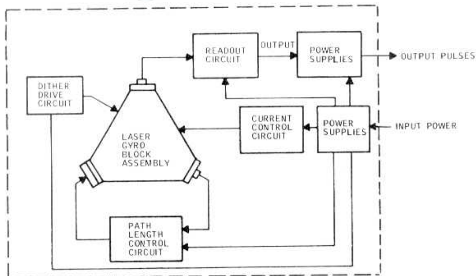
Figure 14. Laser-gyro electronic elements.
