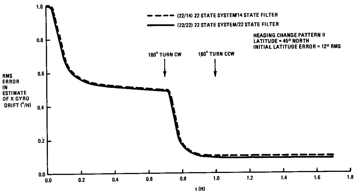
Figure 26. Error in Estimate of "X" Gyro Bias Drift 22/14 Sensitivity Analyses
