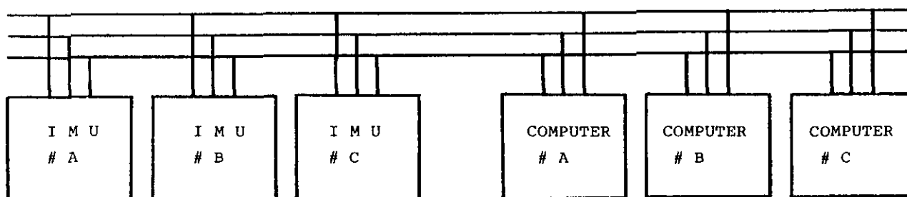
Figure 23. Strapdown sensor data-bus configuration for accommodating bus overload.
