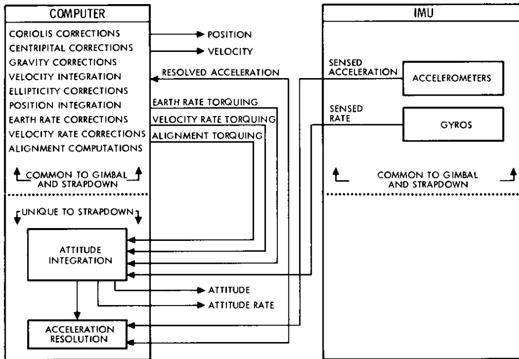
Figure 2. Computer-IMU interface: strapdown system
