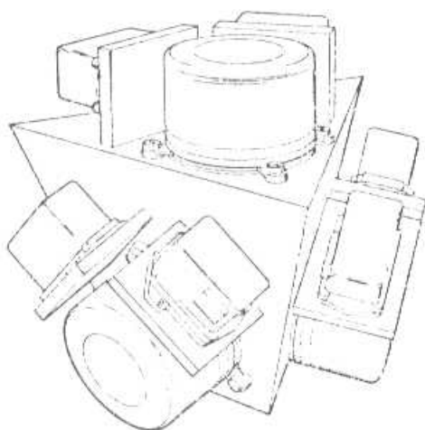
Figure 20. Fail-op 2 gyro and accelerometer Figure 21. Semi-octahedral gyro axis full skewed arrangement using two-degree-of-freedom gyros. orientation as proposed by [4].
