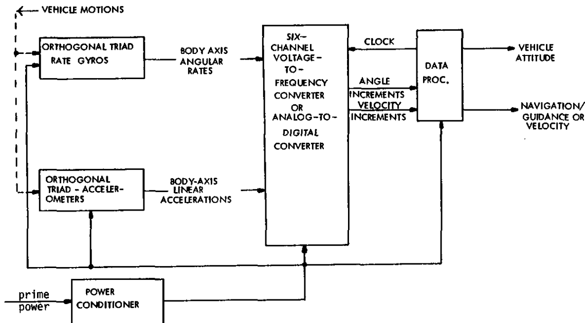
Figure 5. Strapdown system block diagram
