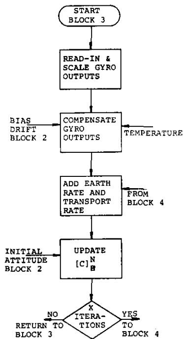
Figure 5. Functional flow diagram matrix updating algorithm.
