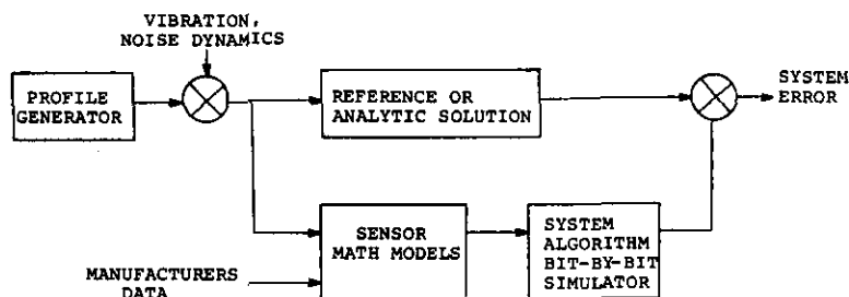
Figure 8. Simulation facility functional block diagram.
