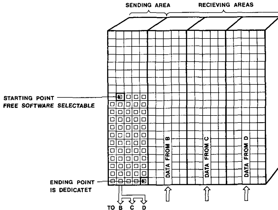
Figure 15. Principle of DMA data exchange.
