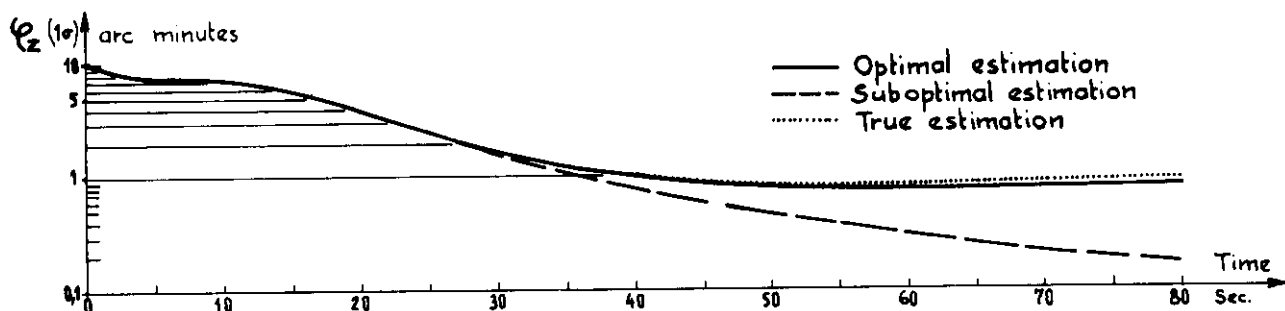
— Figure 29 — Alignment simulation
