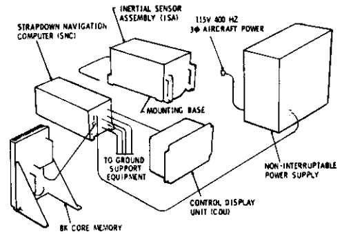
Figure 29. LINS-O Engineering Hardware
