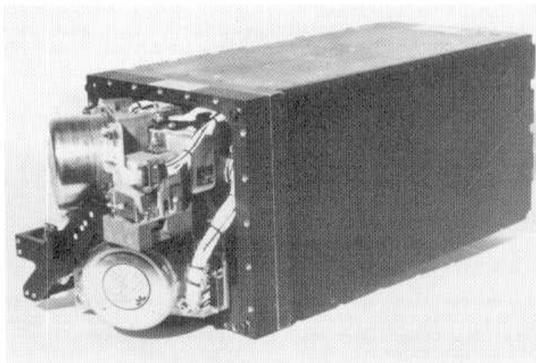
Figure 7. Strapdown inertial measurement unit TDS-3D.
