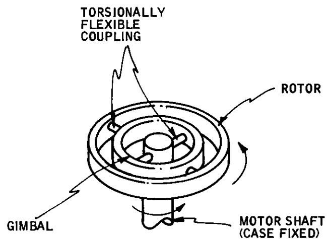
Figure 8. Tuned-rotor-gyro rotor assembly.
