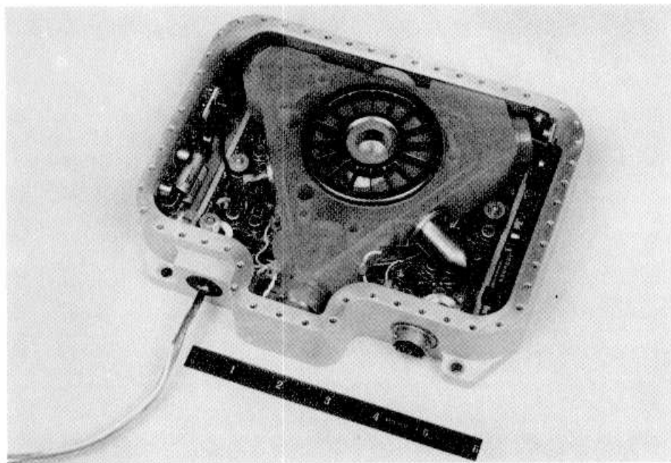
Figure 15. Honeywell GG1300 laser gyro.
