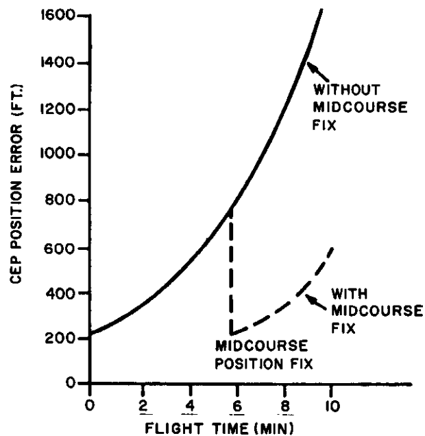
Figure 12. CEP Position Error Without and With a Mid-Course Fix
