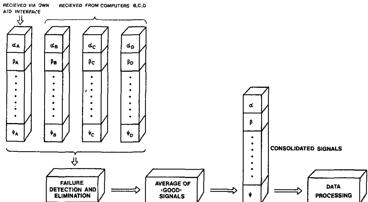
Figure 16. Principle of signal consolidation.
