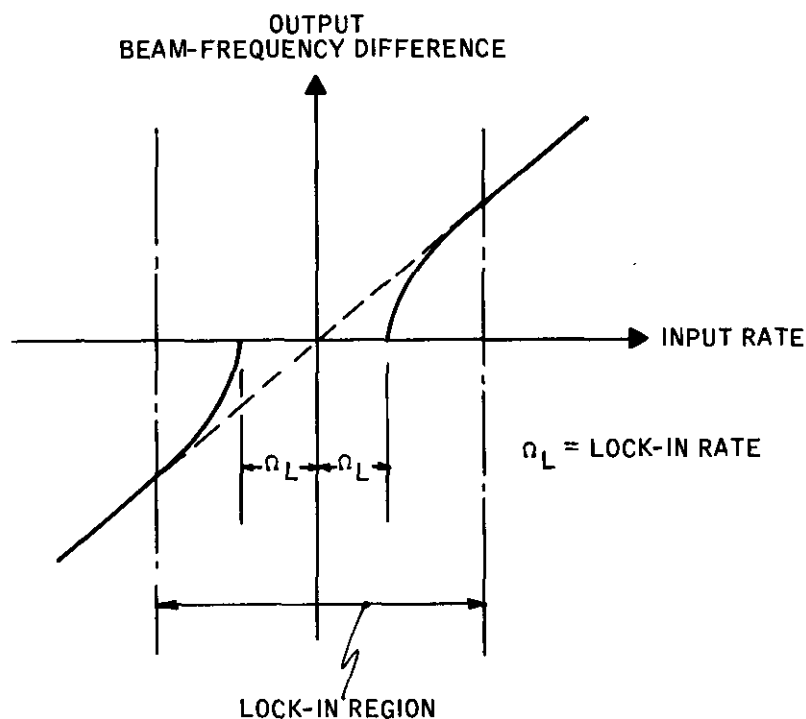
Figure 17. Laser gyro lock-in.
