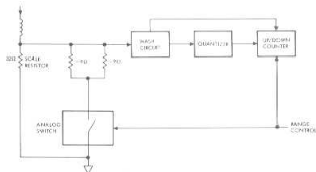
Figure 9. Gyro-axis conversion diagram.
