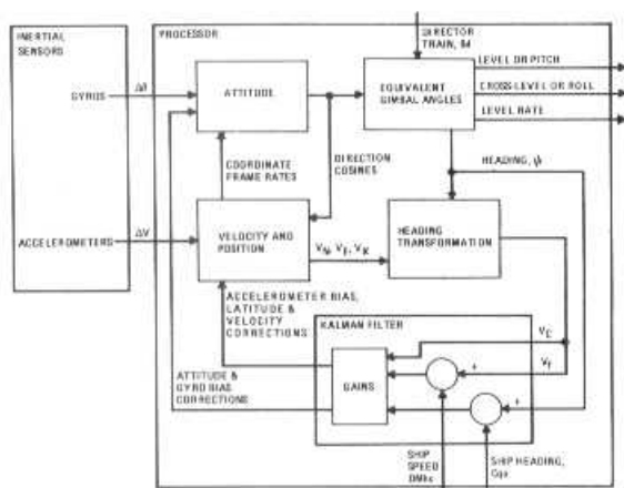
Figure 14. Stable Element Basic Processor Functions
