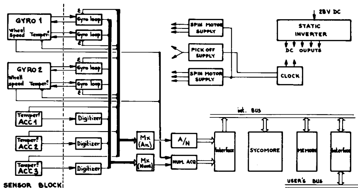
Figure 7 - SIL3 Functional diagram
