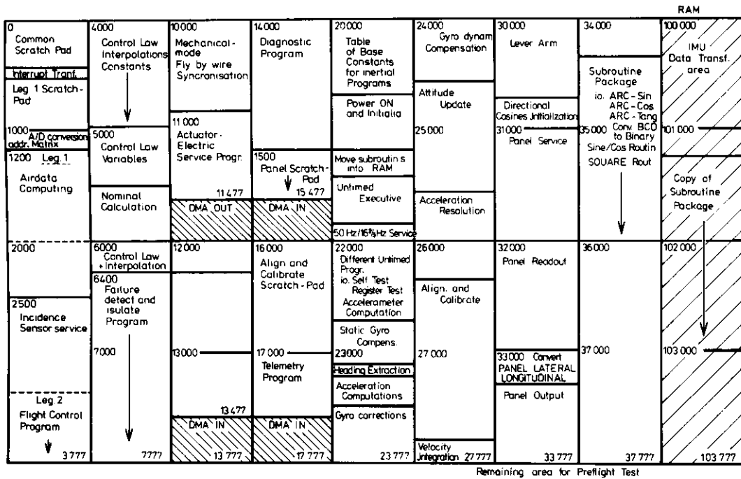
Figure 13. Computer memory occupation: 16k + 2k RAM.
