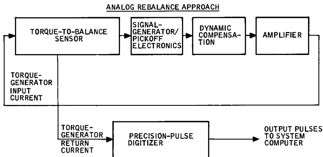
Figure 4. Torque-rebalance-loop concepts.
