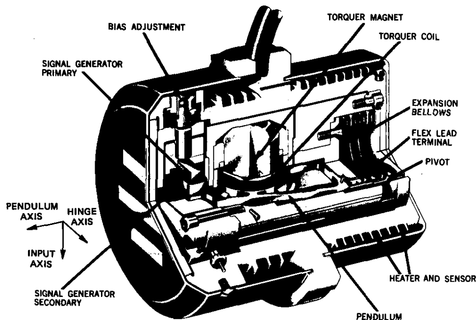
Figure 18. Honeywell GG177 fluid-damped pendulous accelerometer.
