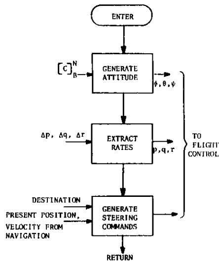
Figure 11. Functional flow diagram, guidance and control algorithms
