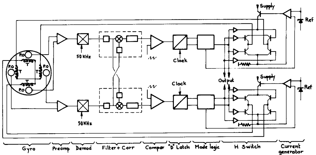
Figure 15 — Gyro rebalance loop
