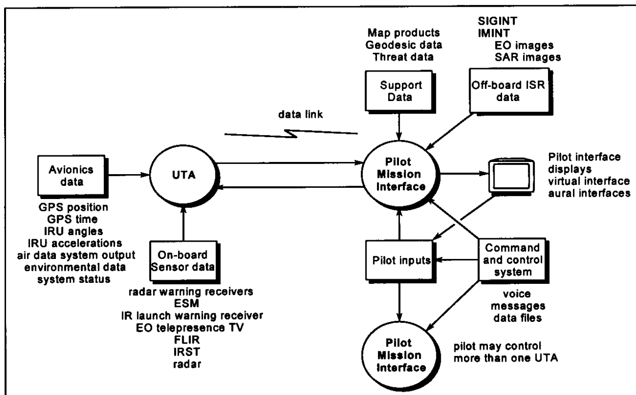
Figure 8-2: Schematic of Conceptual UTA System
