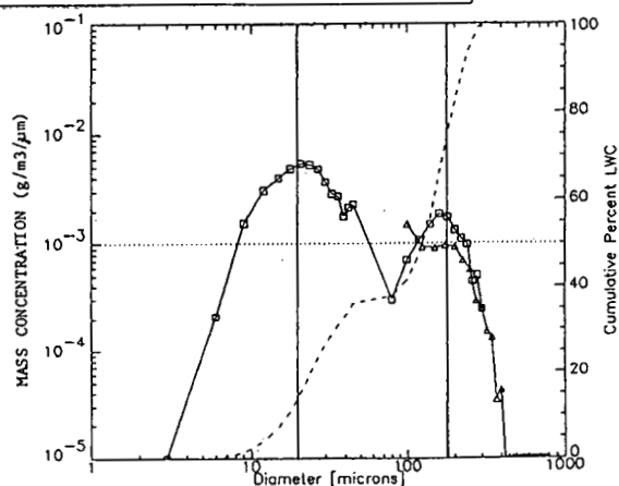
Figure 4.3-4 Mass-Weighted Tanker Distribution, Larger Droplet Test Condition
