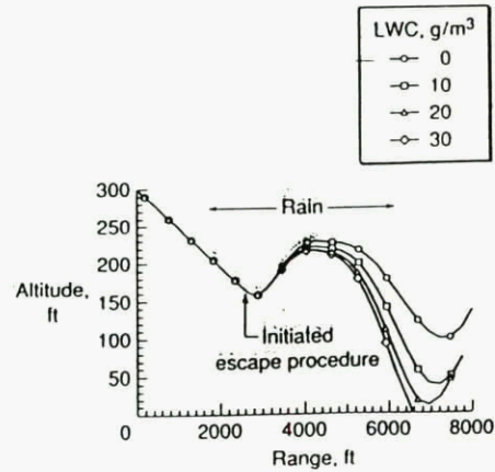
FIG. 59. EFFECT OF RAIN ON A WIND SHEAR ESCAPE PERFORMANCE OF A BOEING 737-100 IN A LANDING CONFIGURATION.
