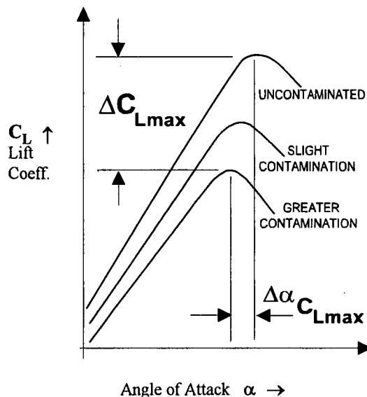
Fig. 1.3-1: Effect of Ice Contamination on Lift
