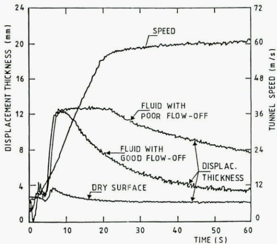
Fig. 17 : Typical results of CWT-1 flow-off tests, with bottom flat wall of test section clean or covered with fluid
