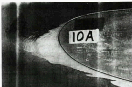
Fig. 3.1-9 Typical rime ice formation on a swept airfoil
