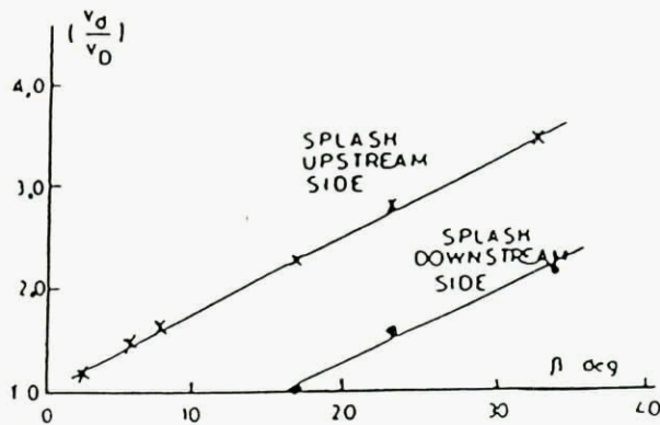
FIG. 13. INITIAL EJECTION VELOCITIES ( t=0 )
