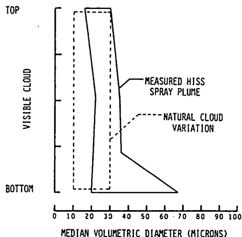
Figure 4.3-6 Vertical Variation-Droplet MVD
