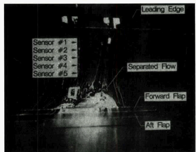
FIG. 47. WATER FILM PATTERN ON UPPER SURFACE. \alpha = 20^\circ ; LWC = 45 g/m 3 ; q_\infty = 30 \text{ LB/FT}^2 . HIGH -LIFT CONFIGURATION.
