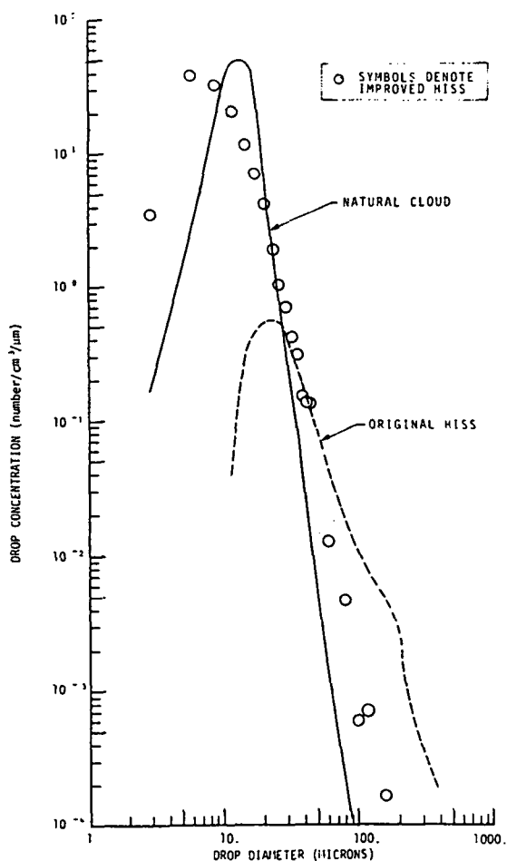
Figure 4.3-8 Drop Size Spectra
