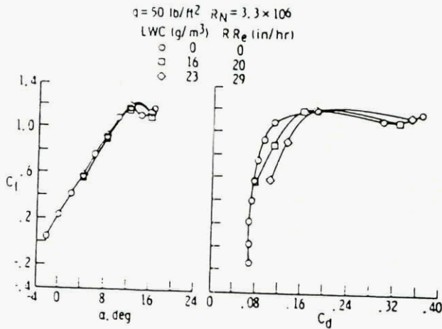
FIG. 43. WATER SPRAY EFFECTS ON LIFT AND DRAG AT DYNAMIC PRESURE 50 LB/FT 2 ; CRUISE CONFIGURATION.
