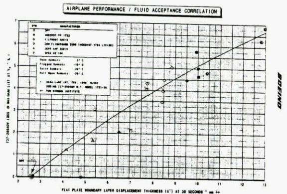
Fig. 24 : Correlation between flat plate boundary layer displacement thickness and 3-D lift loss
