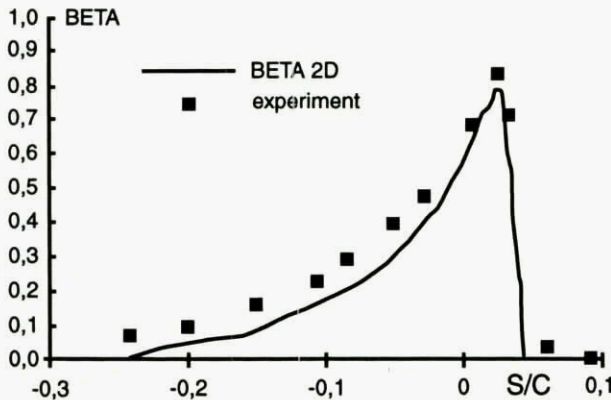
Figure 5-2. Collection Efficiency for a NACA 65018 Airfoil, chord=0.33m, d=20μm, a=8°, T=94.5kPa, M=0.24
