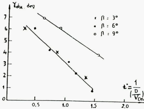
FIG. 8. LOW INCIDENCE EJECTION ANGLES
