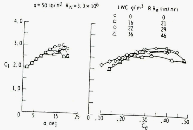
FIG. 45. WATER SPRAY EFFECTS ON LIFT AND DRAG AT DYNAMIC OF 30 LB /FT 2 HIGH -LIFT CONFIGURATION.
