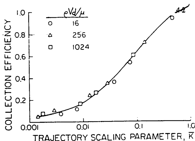
Fig. 4.1-1 Comparison of K_0 and \bar{K} in scaling the local droplet impingement (Bragg, 1982)
