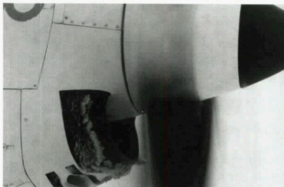
Fig. 3.1-8 Runback ice on nacelle intake
