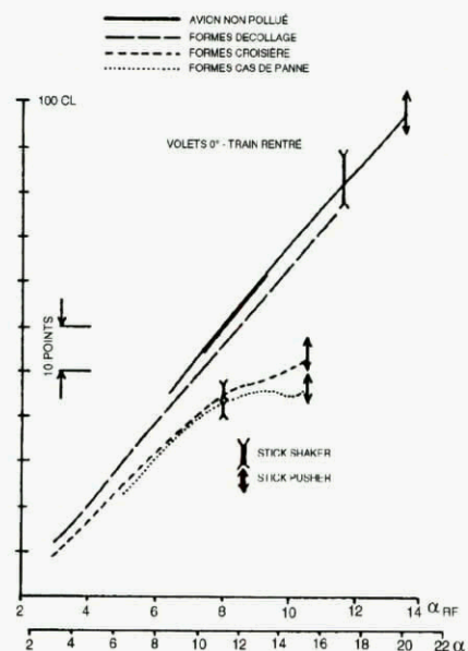
Fig. 3.2-30 Adjustment of stick shaker/pusher setting
