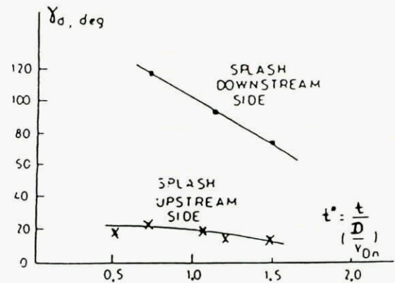
FIG. 12. INTERMEDIATE INCIDENCE EJECTION ANGLES. \beta = 24^\circ
