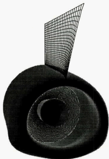
Figure 5-19. Grid model for a Boeing 737-300 engine inlet.
