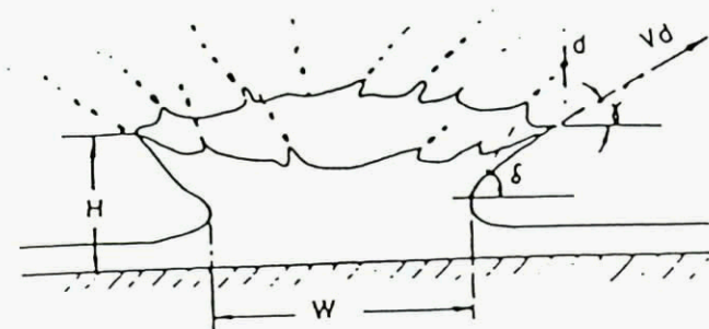
FIG. 16. SCHEMATICS OF A PERPENDICULAR IMPACT.
