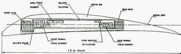
Fig. 6 : Test airfoil model and internal balance arrangement
