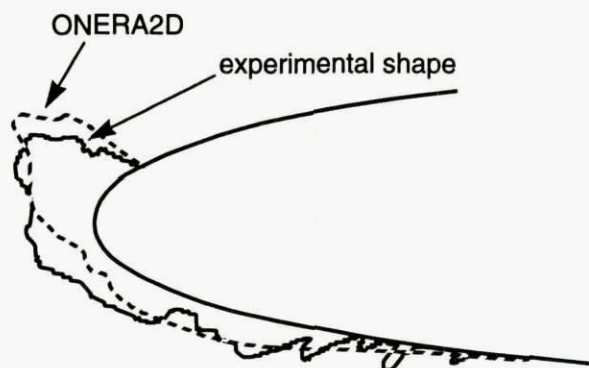
Figure 5-11. Comparison between ONERA 2D code and experimental shape.
