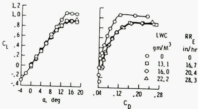
FIG. 38. RAIN EFFECT ON A NACA 0012 WING MODEL.
