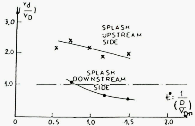
FIG. 11 INTERMEDIATE INCIDENCE EJECTION VELOCITIES. \beta = 24^\circ
