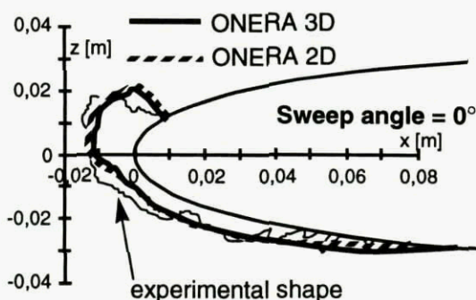
Figure 5-12. Comparison of ONERA 2D code, ONERA 3D code, and experimental shape.
