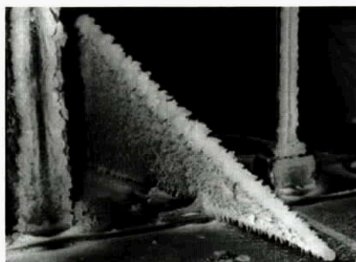
Fig. 3.1-11 Glaze ice formation on a delta wing
