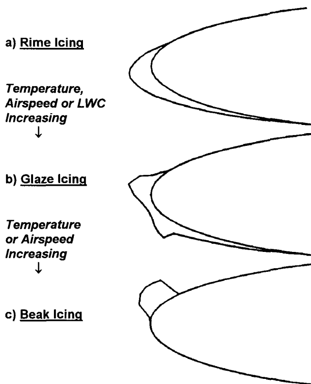
Fig. 1.2-1: Types of Ice Accretion
