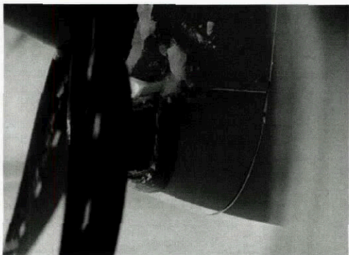
Fig. 3.1-21 Residual ice on intake lip after one de-icing cycle
