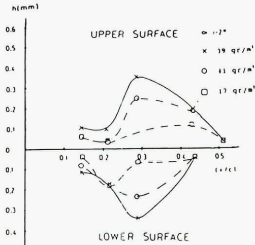
FIG. 18. EFFECT OF LWC ON FILM THICKNESS DISTRIBUTION.
