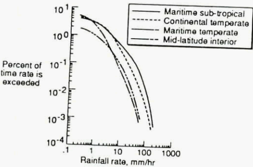
FIG. 2. CLIMATOLOGY OF INSTANTANEOUS RAIN RATES.
