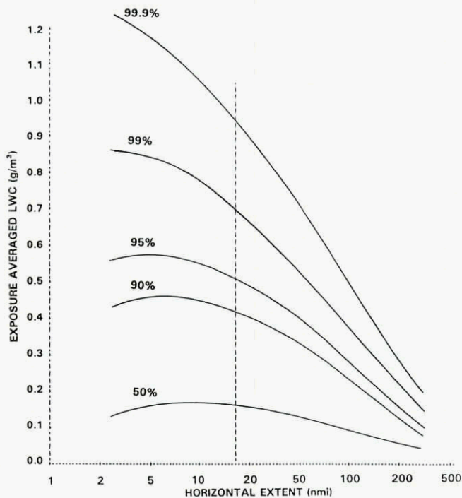
Fig. 2.2-3: Computed LWC Percentiles for Stratiform Clouds with Average MVD's (15 \mu m) and Temperatures from 0 C to -10 C.
