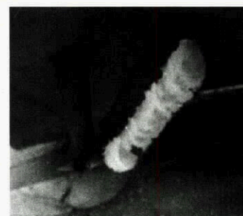
Fig. 3.1-18 Ice accretion on a protruding flap hinge bracket
