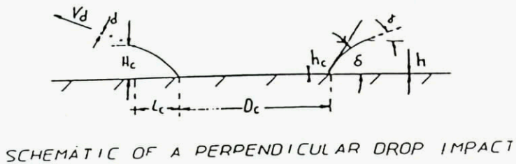
FIG. 16. SCHEMATICS OF A PERPENDICULAR IMPACT.
