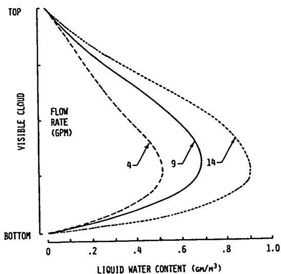
Figure 4.3-7 Vertical Variation-Cloud LWC
