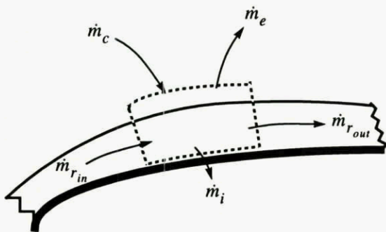
Figure 5-6. Mass Balance Control Volume.
