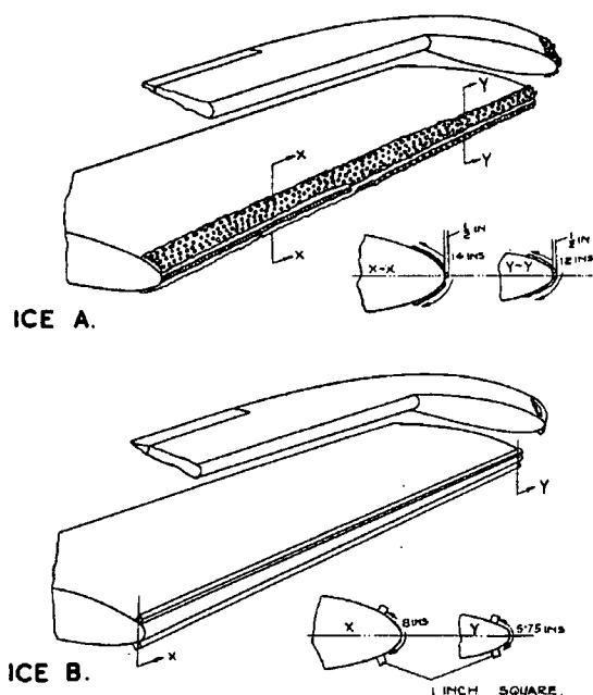
Fig. 3.4-3 Ice shapes tested
