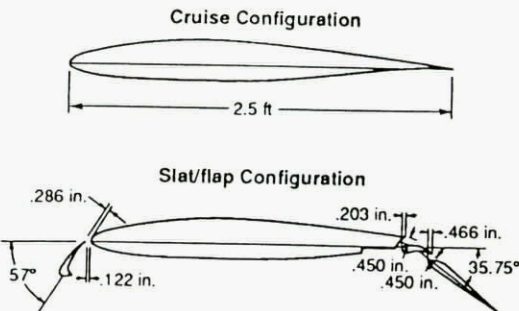
FIG. 41. CROSS SECTION OF 64-210 AIRFOIL.
