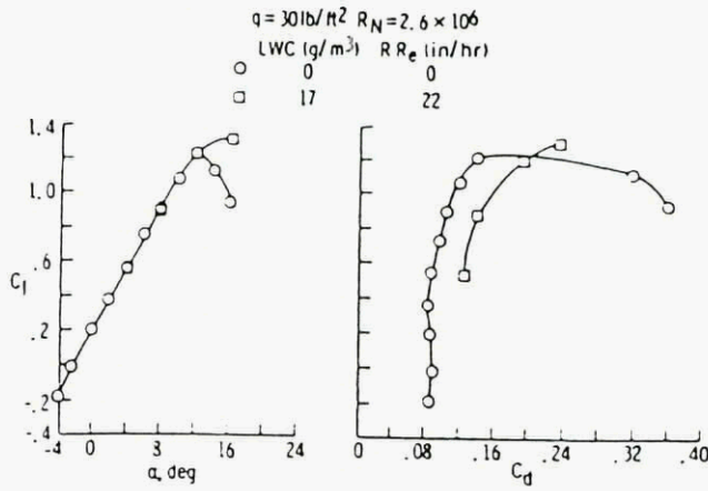
FIG. 42. WATER SPRAY EFFECTS ON LIFT AND DRAG AT DYNAMIC PRESURE OF 30 LB/FT 2 ; CRUISE CONFIGURATION
