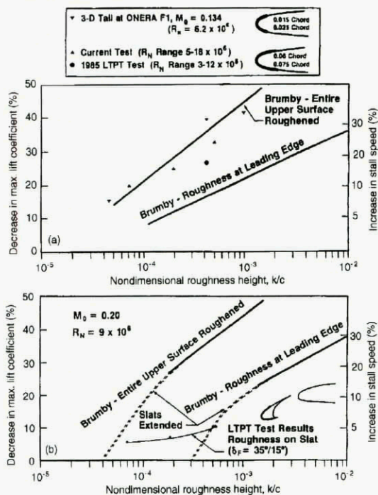
-Effect of roughness on maximum lift (a) Single element airfoil and tail. (b) Four element airfoil
