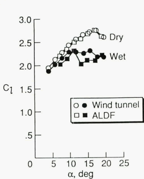
FIG. 54. LIFT COEFFICIENT COMPARISON BETWEEN WIND TUNNEL AND LARGE SCALE TESTS.
