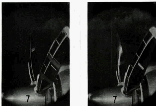
Fig. 3.1-19b Ice formation on a rotating propeller (thrust face)
