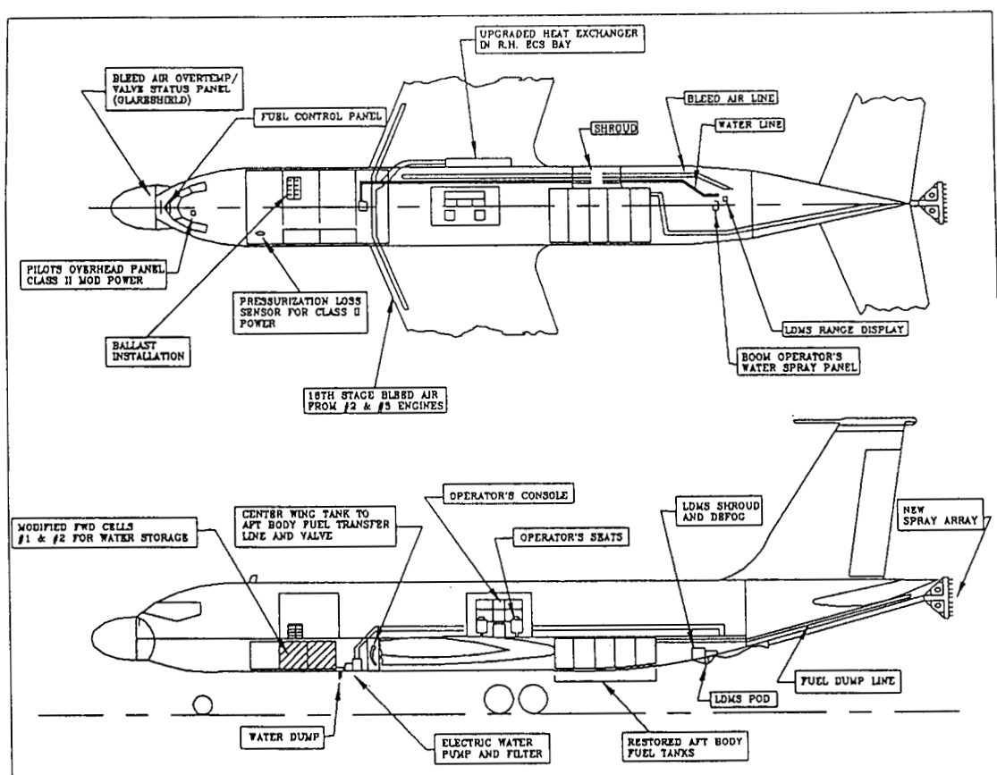
Figure 4.3-2 NKC-135A Tanker Aircraft
