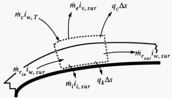
Figure 5-7. Energy Balance Control Volume.
