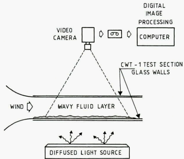
Fig. 2 : Set-up for measurement of local thickness of a dyed fluid layer by a light absorption technique
