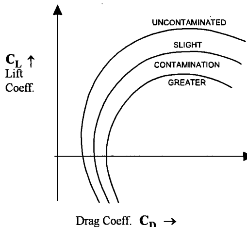
Fig. 1.3-2: Effect of Ice Contamination on Drag
