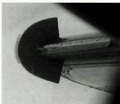
Fig. 3.1-16 Residual ice on the outer wing part
