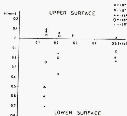
FIG. 23. EFFECT OF ANGLE OF ATTACK ON FILM THICKNESS DISTRIBUTIONS. HIGH-LIFT CONFIGURATION LWC = 39 \text{ gr/m}^3 ; v_\infty = 78 m/s
