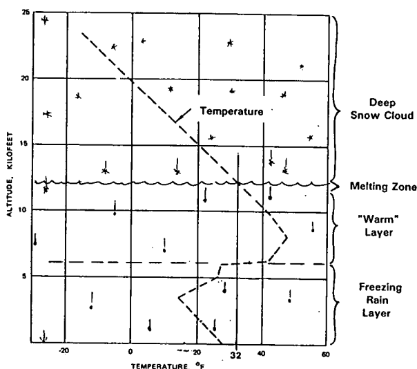
Fig. 2.3-1: Schematic Representation of Freezing Rain Conditions.
