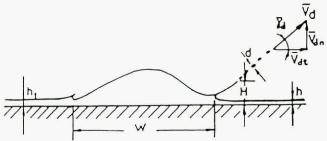
FIG. 6. SCHEMATICS OF A LOW INCIDENCE SPLASH. (DROP COALESCENCE STAGE)
