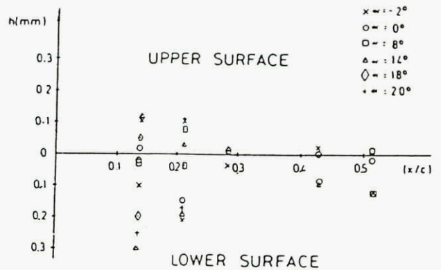
FIG. 22. EFFECT ON ANGLE OF ATTACK ON FILM THICKNESS DISTRIBUTION. HIGH-LIFT CONFIGURATION. LWC = 39 \text{ gr/m}^3 ; v_\infty = 48 m/s
