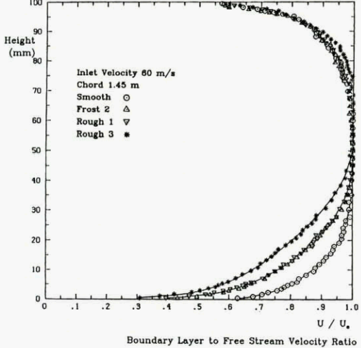
Fig. 15 : Vertical profile of velocity at the exit of the test section of the VKI CWT-1 facility
