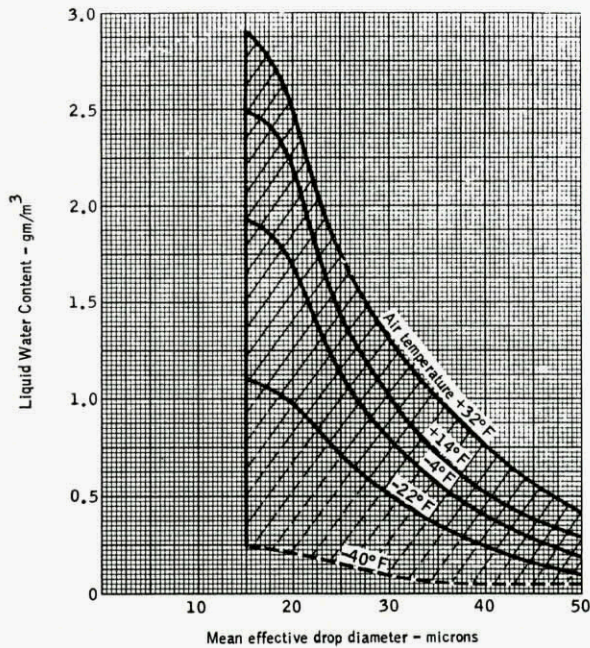
Fig. 2.1-3: Conventional LWC vs. MVD Envelopes for Cumuliform Icing Clouds (FAA, 1994a).
