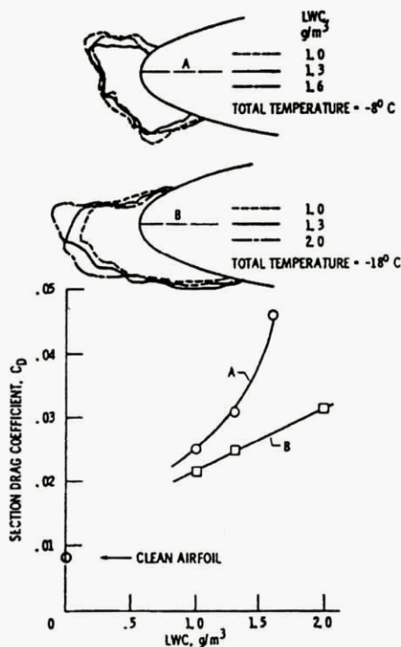
Fig. 3.2-15 Effect of LWC on ice shape and section drag
