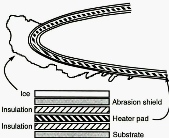
Figure 5-10 Two-dimensional finite-difference model of an electrothermal heater.
