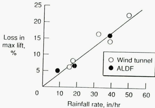
FIG. 56. EFFECT OF RAIN ON MAXIMUM LIFT.
