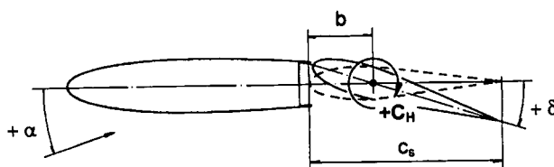
Fig. 3.4-2 Sign convention for control surfaces
