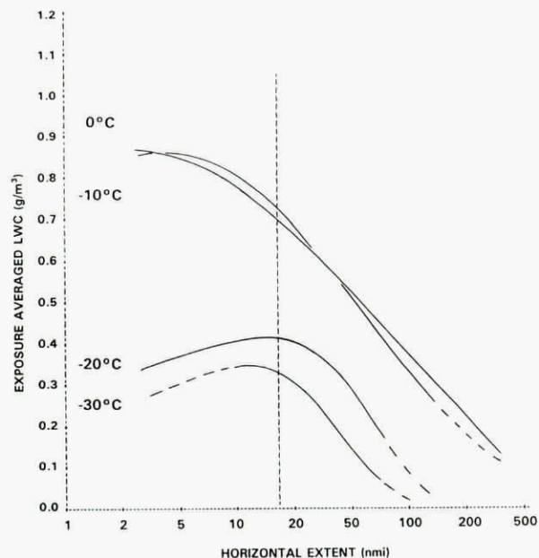
Fig. 2.2-4: Computed 99th Percentile Limits to LWC for 10 C Temperature Intervals in Stratiform Clouds with Average MVD's (15 \mu m).
