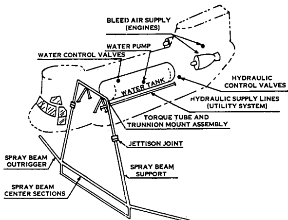
Figure 4.3-5 HISS Tanker
