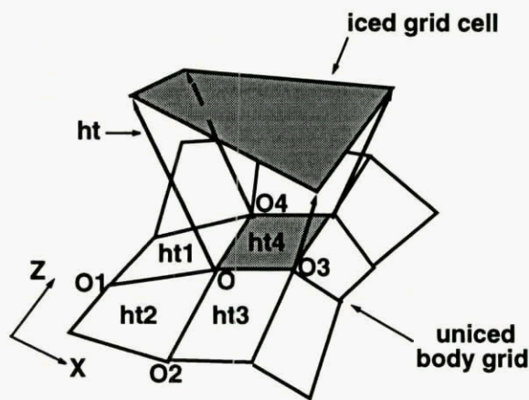
Figure 5-9 Ice Growth on a 3D Grid Cell.
