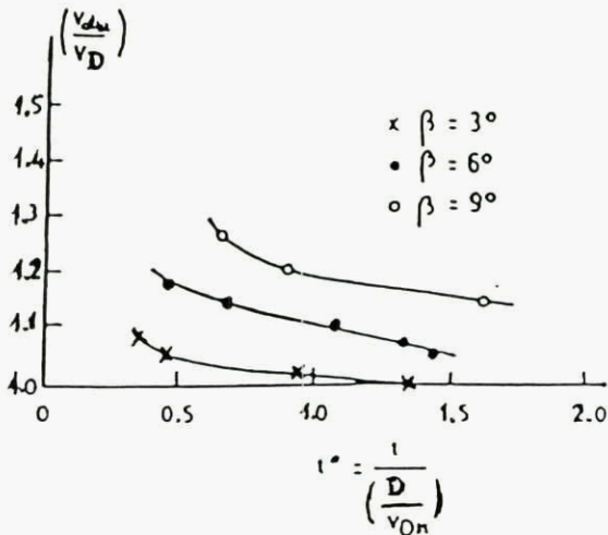
FIG. 7 LOW INCIDENCE EJECTION VELOCITIES.
