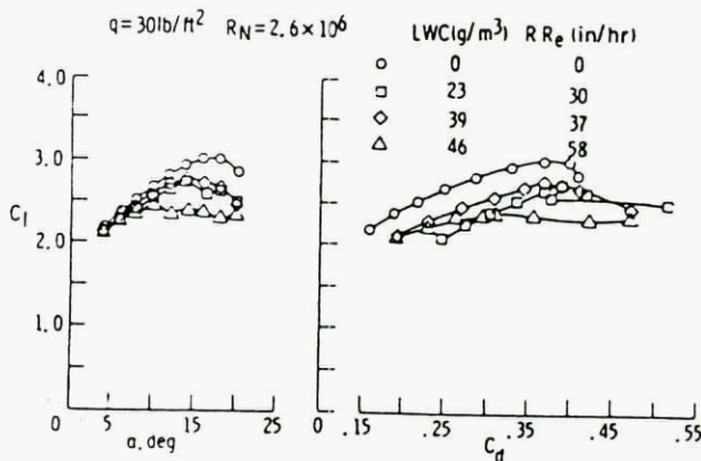
FIG. 44. WATER SPRAY EFFECTS ON LIFT AND DRAG AT DYNAMIC PRESURE OF 30 LB /FT 2 . HIGH -LIFT CONFIGURATION.
