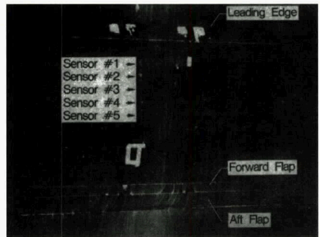
FIG. 46. WATER FILM PATTERN ON UPPER SURFACE. \alpha = 8^\circ ; LWC = 45 g/m 3 q_\infty = 30 \text{ LB/FT}^2 . HIGH -LIFT CONFIGURATION.
