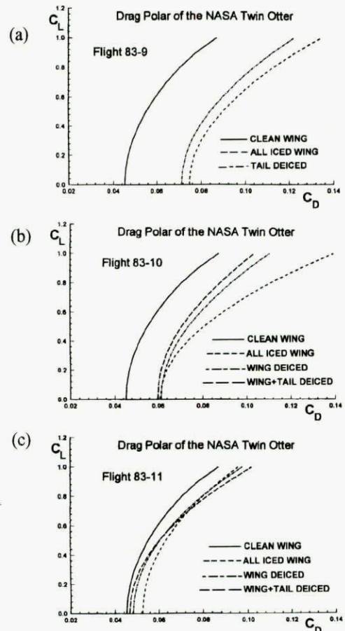
Fig. 3.2-19 Effect of heavy glaze icing (a), effect of glaze icing (b), effect of rime icing (c) on aircraft linearized drag polar
