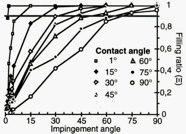
Figure 5-17. Filling ratio \Xi as a function of impingement angle and contact angle.
