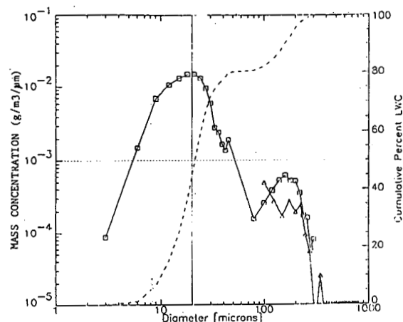
Figure 4.3-3 Mass-Weighted Tanker Distribution FAR Part 25 Conditions
