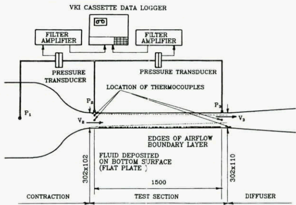
Fig. 16 : CWT-1 test section and instrumentation setup
