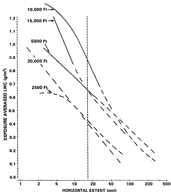
Fig. 2.2-6: The 99% Cumulative Maximum LWC at Different Altitudes (AGL) for Supercooled Clouds with Average MVD's (15 μm) and Highest Temperatures Available at the Altitude. (Summertime convective clouds excluded).
