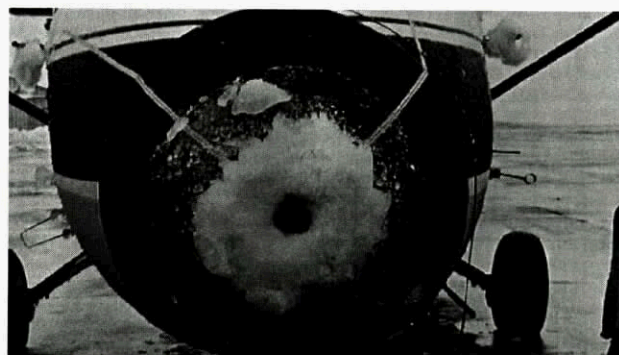
Fig. 3.1-28 Ice formation from freezing rain on radome
