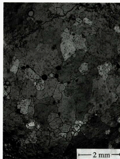
Fig. 3.1-5 300 µm thick slice of glaze ice
