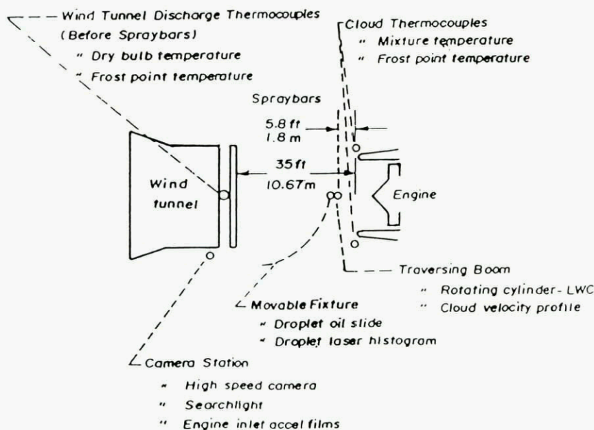
FIG 4.2-2.- Schematic of the General Electric engine icing test facility in Peebles, Ohio, USA
