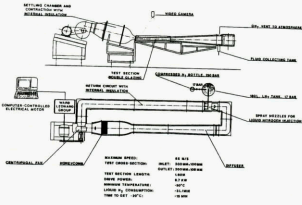
Fig. 1 : The VKI Cold Wind Tunnel
